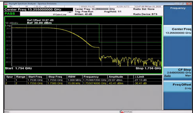
Band4-1.4MHz-16QAM-20393-1RB#0-PASS
