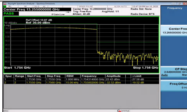
Band4-1.4MHz-QPSK-20393-6RB#0-PASS
