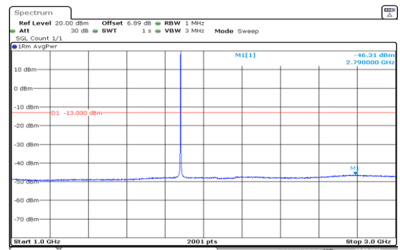
Band2-1.4MHz-QPSK-18900-6RB#0-1000~3000-PASS
