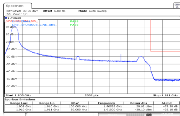
Band2-5MHz-16QAM-19175-1RB#0-PASS
