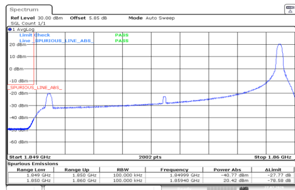
Band2-10MHz-16QAM-18650-1RB#49-PASS
