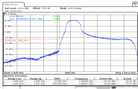
Band2-1.4MHz-16QAM-18607-1RB#0-PASS
