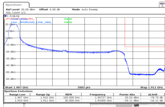
Band2-3MHz-16QAM-19185-1RB#0-PASS
