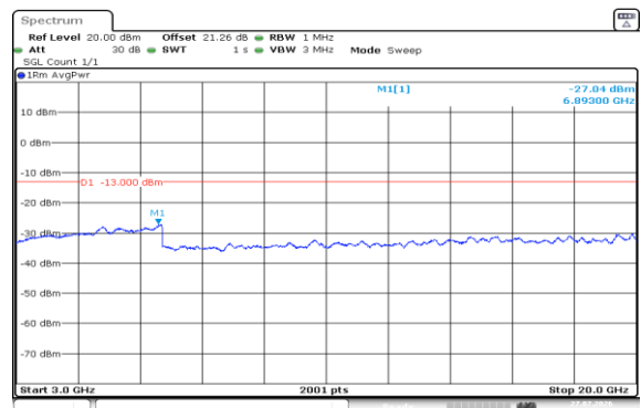
Band2-1.4MHz-16QAM-18607-1RB#5-3000~20000-PASS
