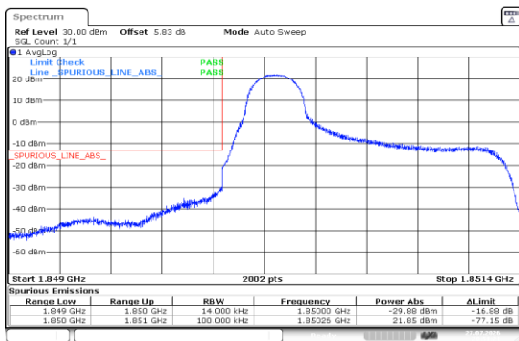
Band2-1.4MHz-QPSK-18607-1RB#0-PASS
