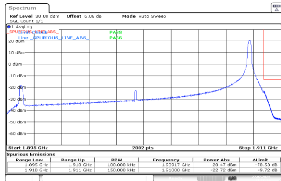
Band2-15MHz-16QAM-19125-1RB#74-PASS
