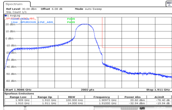
Band2-1.4MHz-16QAM-19193-1RB#5-PASS
