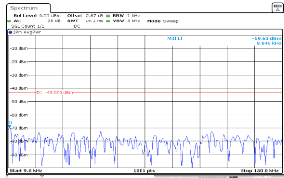
Band2-1.4MHz-16QAM-18900-6RB#0-0.009~0.15-PASS
