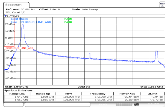
Band2-15MHz-16QAM-18675-1RB#0-PASS
