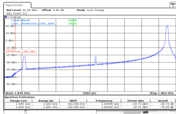
Band2-15MHz-16QAM-18675-1RB#74-PASS
