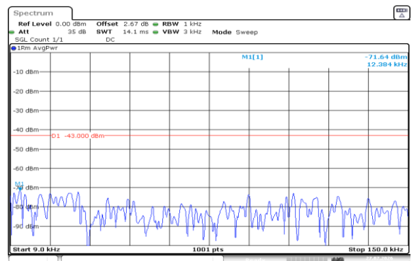
Band2-1.4MHz-16QAM-19193-1RB#0-0.009~0.15-PASS
