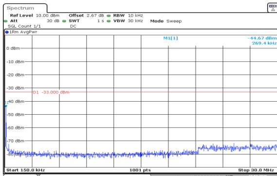
Band2-1.4MHz-16QAM-18900-1RB#5-0.15~30-PASS
