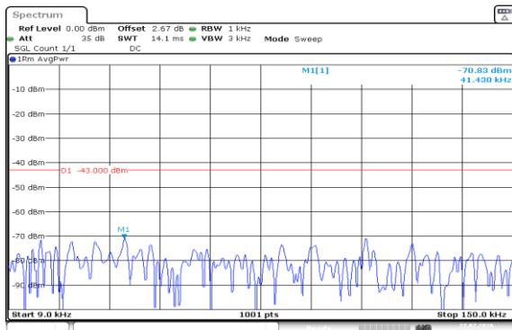
Band2-1.4MHz-QPSK-19193-1RB#5-0.009~0.15-PASS
