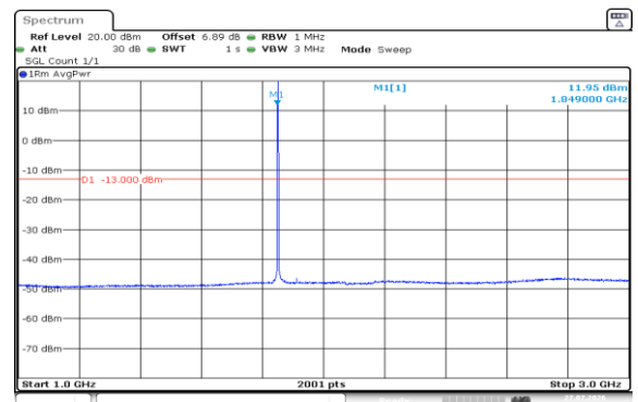
Band2-1.4MHz-16QAM-18607-1RB#0-1000~3000
