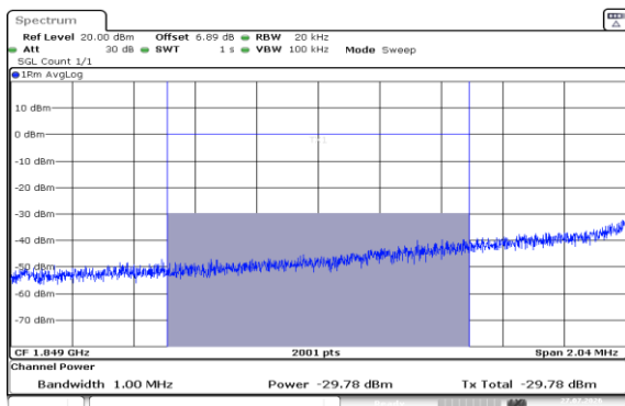
Band2-1.4MHz-16QAM-18607-6RB#0-1000~3000-PASS
