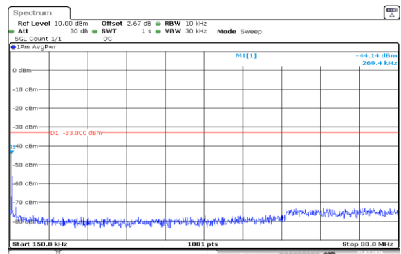
Band2-1.4MHz-16QAM-19193-1RB#5-0.15~30-PASS
