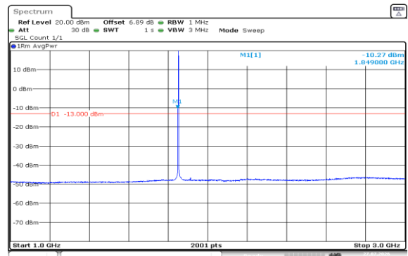
Band2-1.4MHz-16QAM-18607-1RB#5-1000~3000
