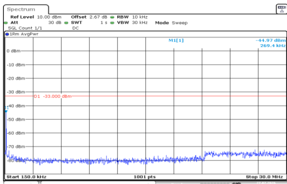
Band2-1.4MHz-16QAM-18900-6RB#0-0.15~30-PASS
