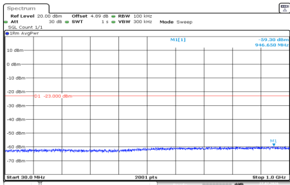
Band2-1.4MHz-16QAM-18607-1RB#5-30~1000-PASS
