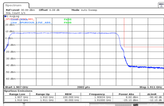
Band2-3MHz-16QAM-19185-15RB#0-PASS
