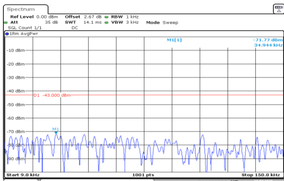
Band2-1.4MHz-QPSK-19193-1RB#0-0.009~0.15-PASS
