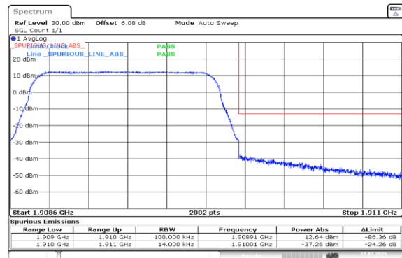
Band2-1.4MHz-16QAM-19193-6RB#0-PASS
