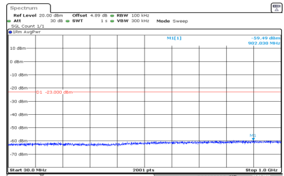
Band2-1.4MHz-16QAM-18900-1RB#5-30~1000-PASS
