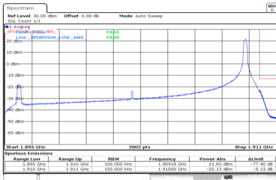
Band2-15MHz-QPSK-19125-1RB#74-PASS
