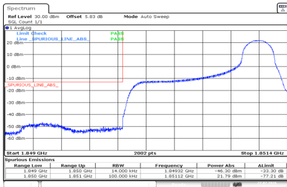
Band2-1.4MHz-QPSK-18607-1RB#5-PASS
