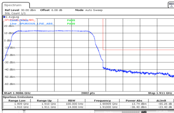
Band2-1.4MHz-QPSK-19193-6RB#0-PASS
