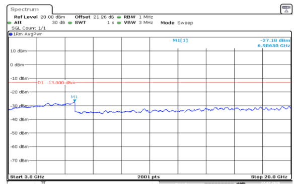
Band2-1.4MHz-16QAM-18900-1RB#5-3000~20000-PASS
