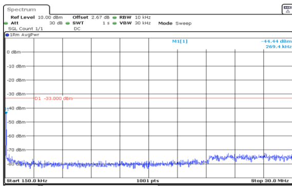
Band2-1.4MHz-16QAM-18900-1RB#0-0.15~30-PASS
