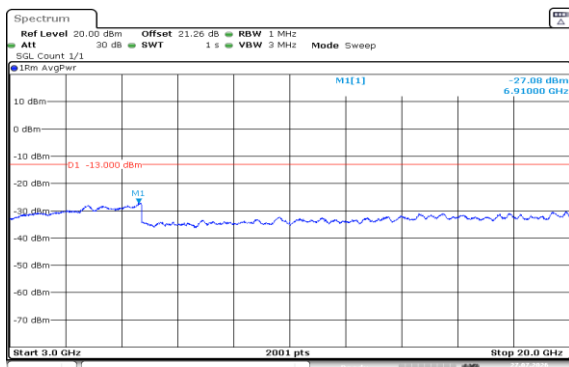
Band2-1.4MHz-QPSK-18900-1RB#5-3000~20000-PASS
