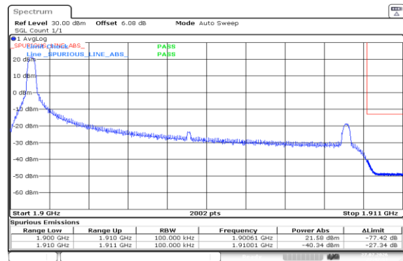
Band2-10MHz-16QAM-19150-1RB#0-PASS
