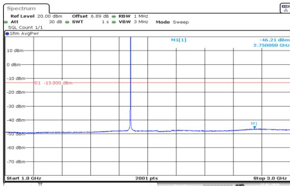
Band2-1.4MHz-16QAM-18900-1RB#0-1000~3000-PASS
