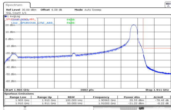
Band2-5MHz-16QAM-19175-1RB#24-PASS
