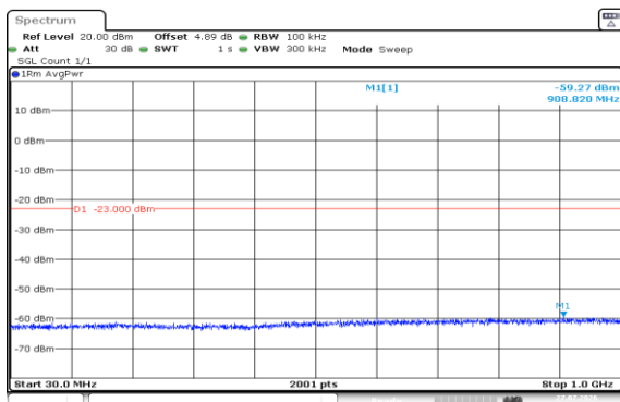
Band2-1.4MHz-16QAM-18607-1RB#0-30~1000-PASS
