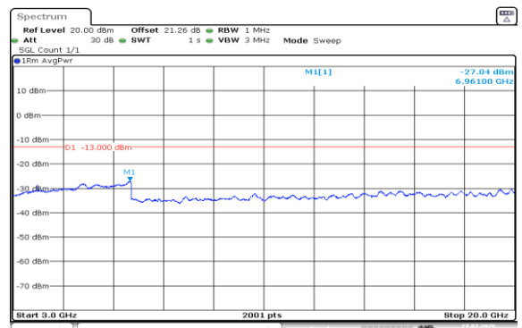
Band2-1.4MHz-16QAM-19193-1RB#0-3000~20000-PASS
