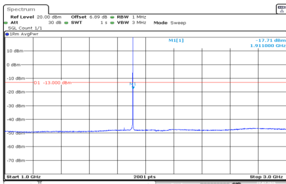
Band2-1.4MHz-16QAM-19193-1RB#0-1000~3000-PASS
