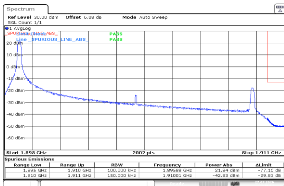
Band2-15MHz-QPSK-19125-1RB#0-PASS
