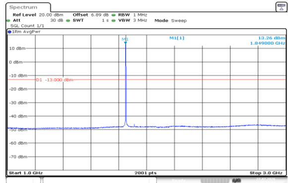
Band2-1.4MHz-QPSK-18607-1RB#0-1000~3000
