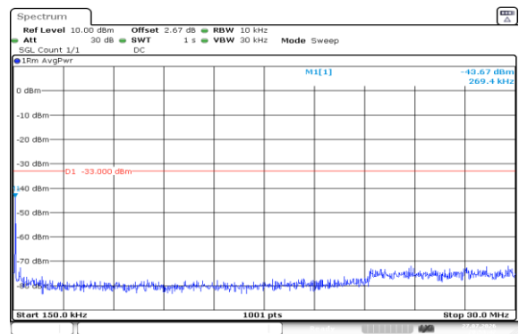
Band2-1.4MHz-QPSK-18607-1RB#0-0.15~30-PASS
