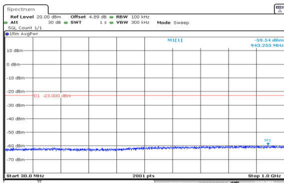
Band2-1.4MHz-QPSK-19193-1RB#5-30~1000-PASS
