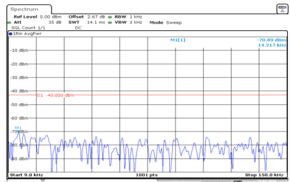
Band2-1.4MHz-16QAM-18900-1RB#5-0.009~0.15-PASS
