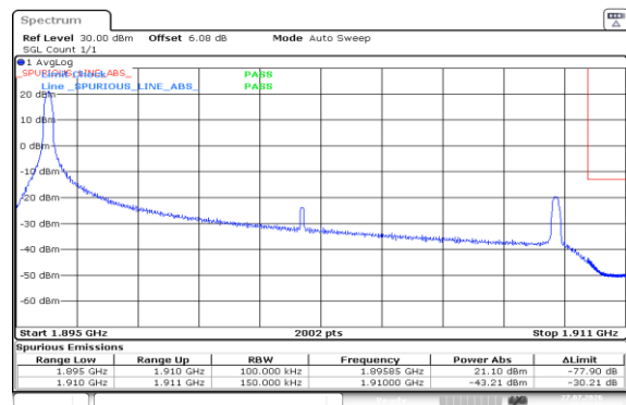
Band2-15MHz-16QAM-19125-1RB#0-PASS
