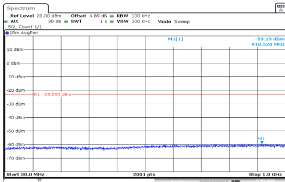
Band2-1.4MHz-QPSK-19193-1RB#0-30~1000-PASS
