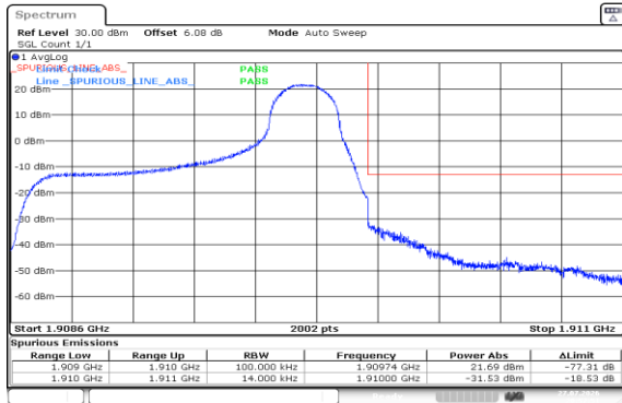
Band2-1.4MHz-QPSK-19193-1RB#5-PASS
