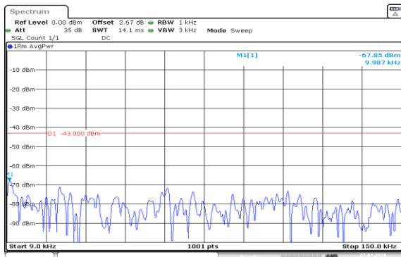
Band2-1.4MHz-QPSK-18900-1RB#0-0.009~0.15-PASS
