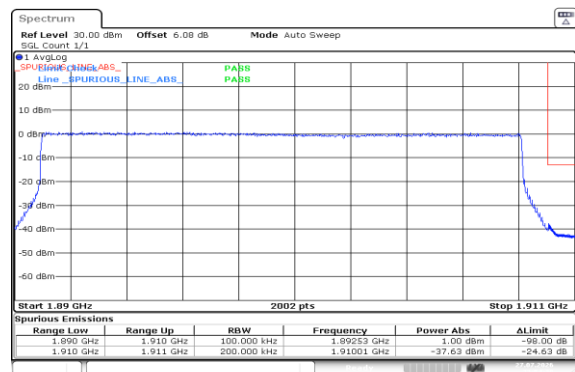
Band2-20MHz-16QAM-19100-100RB#0-PASS
