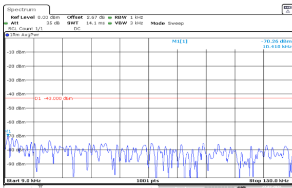
Band2-1.4MHz-16QAM-19193-1RB#5-0.009~0.15-PASS
