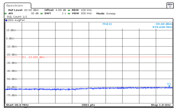
Band2-1.4MHz-16QAM-18900-1RB#0-30~1000-PASS
