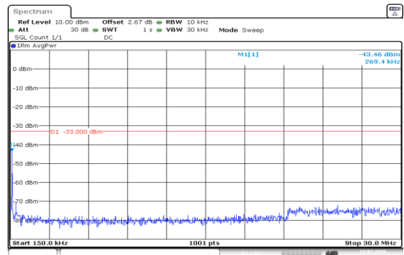
Band2-1.4MHz-QPSK-19193-1RB#5-0.15~30-PASS
