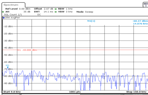
Band2-1.4MHz-QPSK-18607-1RB#5-1000~3000-PASS
