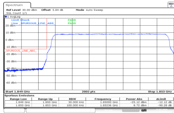
Band2-3MHz-16QAM-18615-15RB#0-PASS
