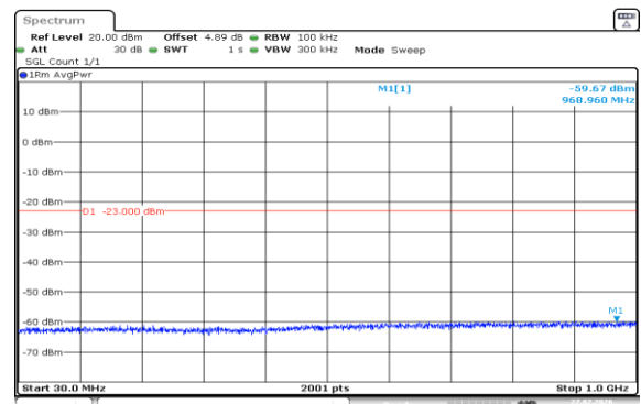
Band2-1.4MHz-16QAM-18900-6RB#0-30~1000-PASS
