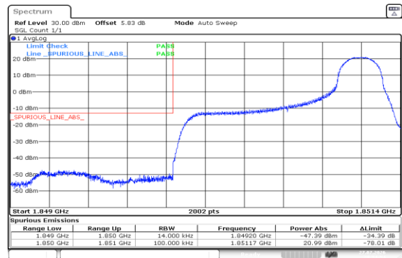
Band2-1.4MHz-16QAM-18607-1RB#5-PASS
