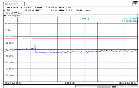
Band2-1.4MHz-QPSK-18607-6RB#0-3000~20000-PASS
