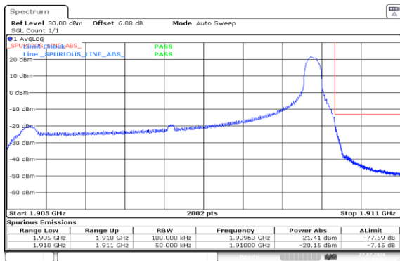
Band2-5MHz-QPSK-19175-1RB#24-PASS
