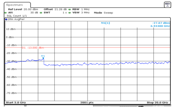
Band2-1.4MHz-16QAM-18900-1RB#0-3000~20000-PASS
