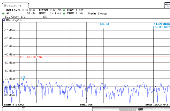
Band2-1.4MHz-QPSK-18607-1RB#0-0.009~0.15-PASS
