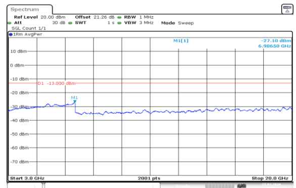
Band2-1.4MHz-16QAM-18607-1RB#0-3000~20000-PASS
