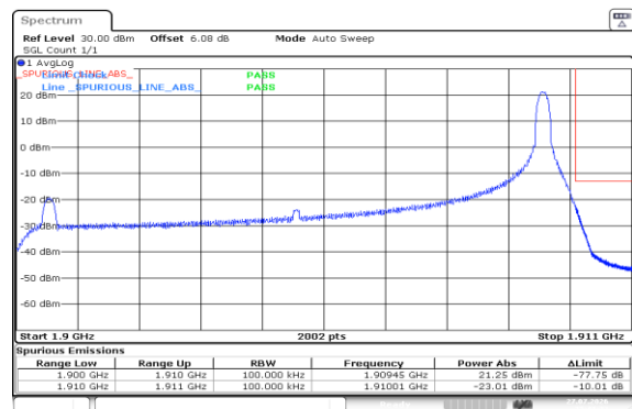
Band2-10MHz-16QAM-19150-1RB#49-PASS
