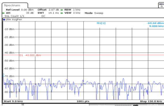
Band2-1.4MHz-16QAM-18607-6RB#0-0.009~0.15-PASS
