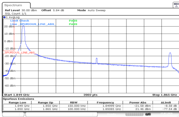
Band2-15MHz-QPSK-18675-1RB#0-PASS
