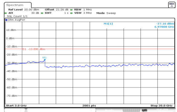
Band2-1.4MHz-QPSK-18607-1RB#0-3000~20000-PASS
