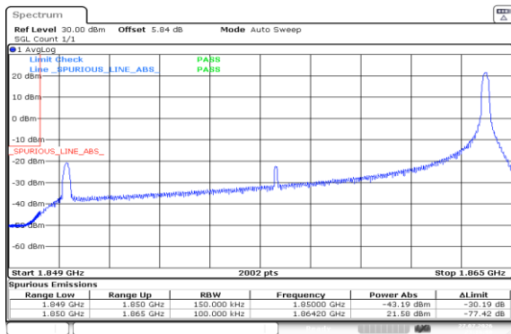
Band2-15MHz-QPSK-18675-1RB#74-PASS
