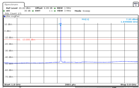
Band2-1.4MHz-QPSK-18607-6RB#0-1000~3000
