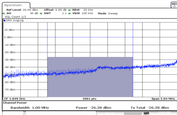
Band2-1.4MHz-QPSK-18607-6RB#0-1000~3000-PASS
