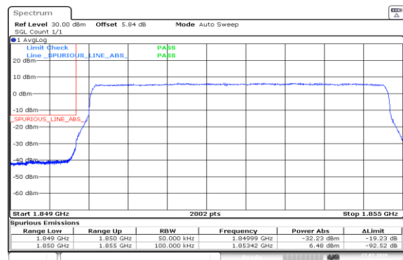
Band2-5MHz-16QAM-18625-25RB#0-PASS
