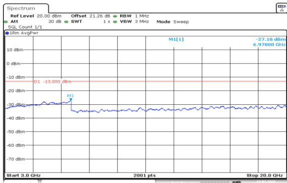
Band2-1.4MHz-QPSK-18900-6RB#0-3000~20000-PASS
