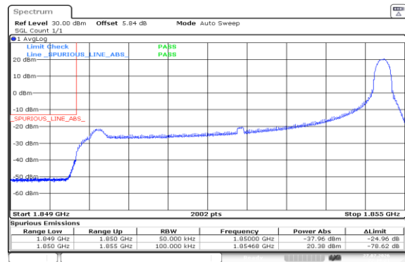
Band2-5MHz-16QAM-18625-1RB#24-PASS
