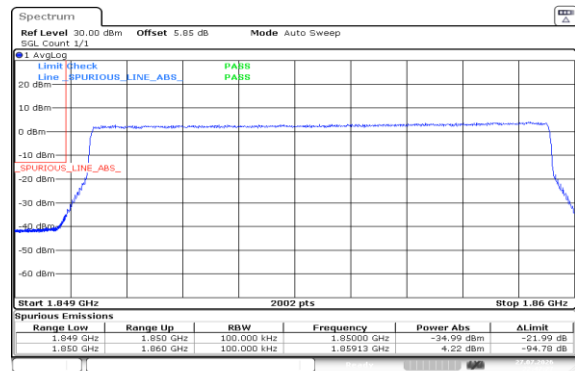
Band2-10MHz-16QAM-18650-50RB#0-PASS
