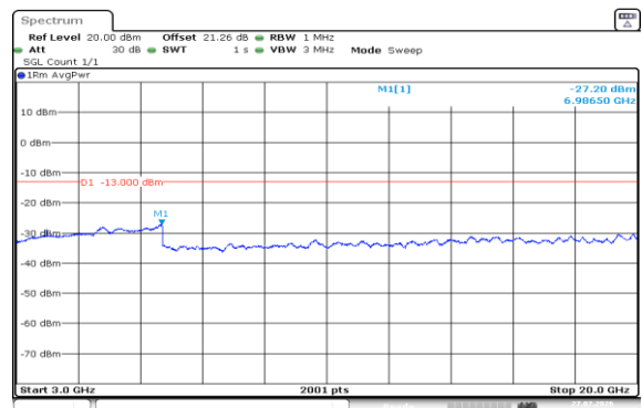
Band2-1.4MHz-QPSK-19193-1RB#5-3000~20000-PASS
