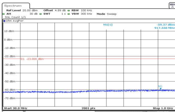
Band2-1.4MHz-QPSK-18900-6RB#0-30~1000-PASS
