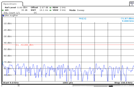
Band2-1.4MHz-16QAM-18607-1RB#0-0.009~0.15-PASS
