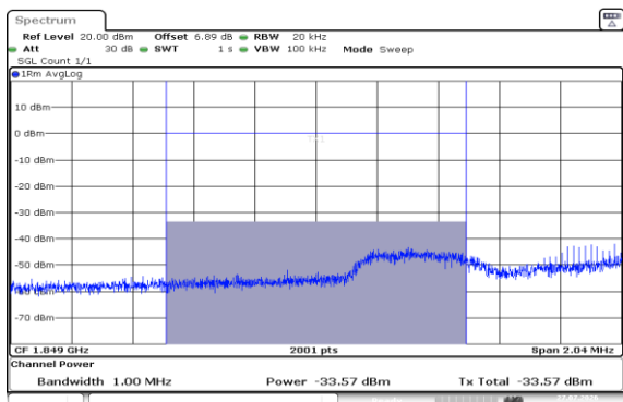
Band2-1.4MHz-16QAM-18607-1RB#5-1000~3000-PASS
