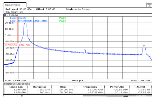
Band2-10MHz-16QAM-18650-1RB#0-PASS
