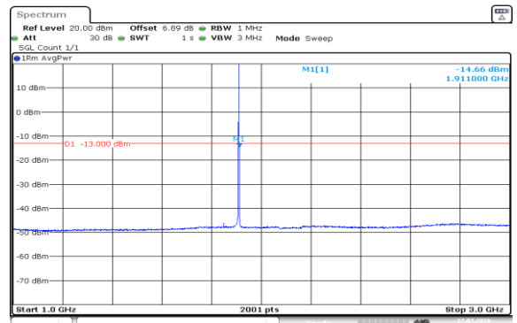
Band2-1.4MHz-QPSK-19193-1RB#0-1000~3000-PASS
