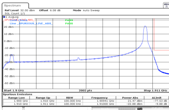
Band2-10MHz-QPSK-19150-1RB#49-PASS
