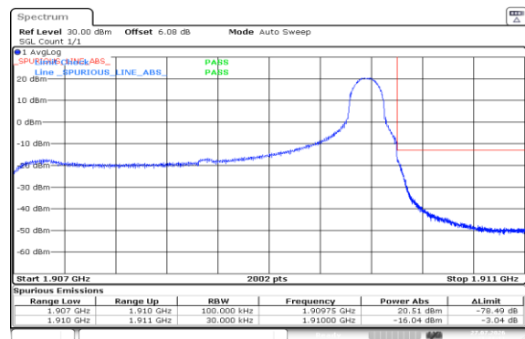
Band2-3MHz-16QAM-19185-1RB#14-PASS
