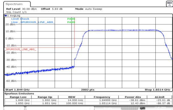
Band2-1.4MHz-16QAM-18607-6RB#0-PASS
