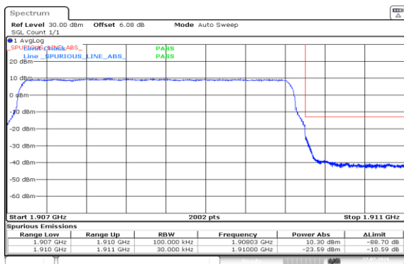
Band2-3MHz-QPSK-19185-15RB#0-PASS
