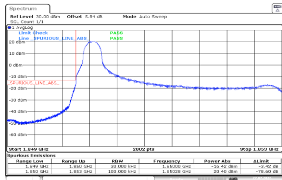
Band2-3MHz-16QAM-18615-1RB#0-PASS
