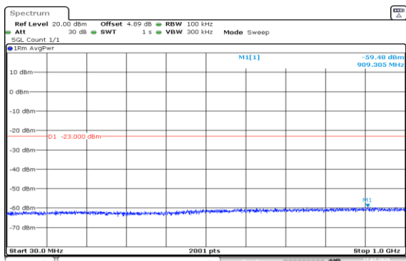
Band2-1.4MHz-QPSK-18607-6RB#0-30~1000-PASS
