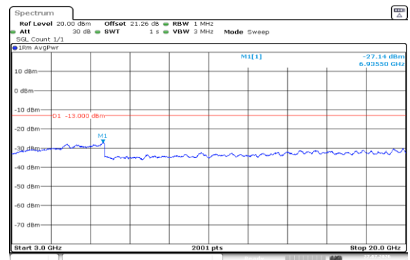
Band2-1.4MHz-16QAM-18607-6RB#0-3000~20000-PASS
