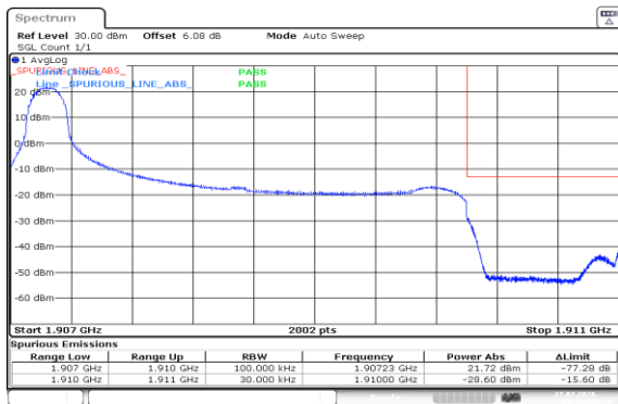
Band2-3MHz-QPSK-19185-1RB#0-PASS
