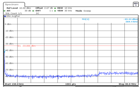
Band2-1.4MHz-QPSK-19193-1RB#0-0.15~30-PASS
