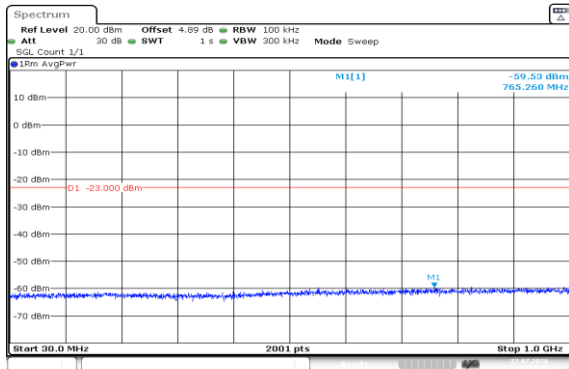
Band2-1.4MHz-QPSK-18607-1RB#0-30~1000-PASS
