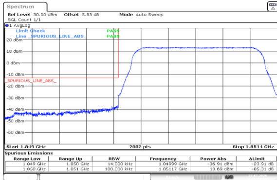
Band2-1.4MHz-QPSK-18607-6RB#0-PASS
