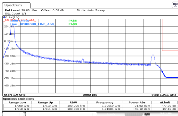
Band2-10MHz-QPSK-19150-1RB#0-PASS
