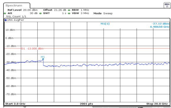
Band2-15MHz-QPSK-18675-1RB#74-3000~20000-PASS
