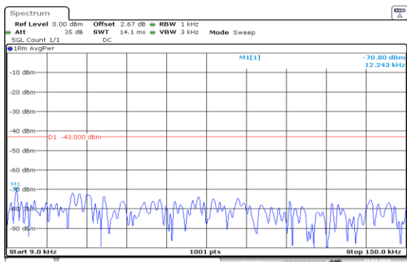
Band2-5MHz-16QAM-19175-1RB#0-0.009~0.15-PASS
