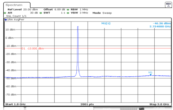
Band2-10MHz-16QAM-18900-50RB#0-1000~3000-PASS
