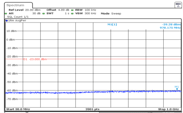
Band2-10MHz-QPSK-18650-1RB#49-30~1000-PASS
