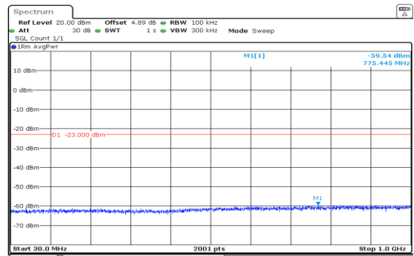
Band2-5MHz-QPSK-19175-25RB#0-30~1000-PASS
