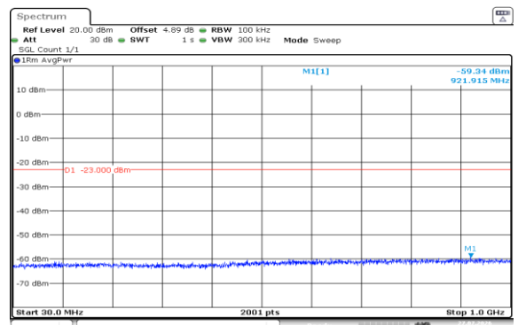
Band2-5MHz-16QAM-19175-1RB#24-30~1000-PASS
