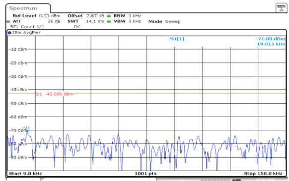
Band2-5MHz-QPSK-19175-1RB#0-0.009~0.15-PASS
