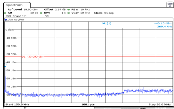
Band2-15MHz-16QAM-18900-1RB#0-0.15~30-PASS
