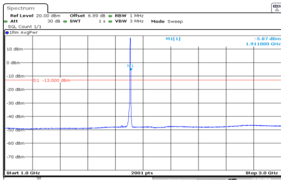
Band2-5MHz-QPSK-19175-25RB#0-1000~3000
