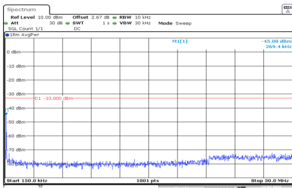
Band2-10MHz-QPSK-19150-1RB#49-0.15~30-PASS
