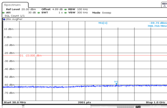
Band2-10MHz-16QAM-18900-50RB#0-30~1000-PASS
