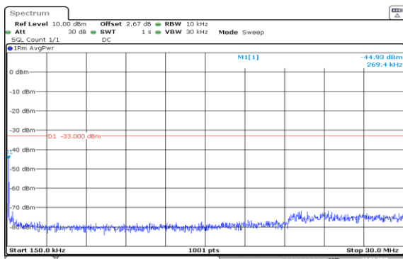
Band2-15MHz-QPSK-18900-1RB#74-0.15~30-PASS
