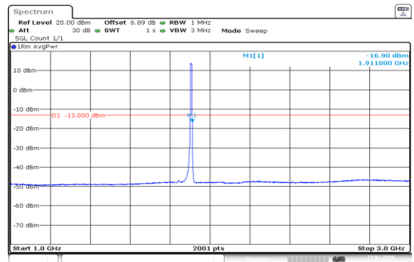
Band2-10MHz-16QAM-19150-50RB#0-1000~3000-PASS
