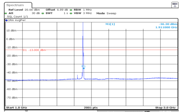
Band2-10MHz-16QAM-19150-1RB#0-1000~3000-PASS
