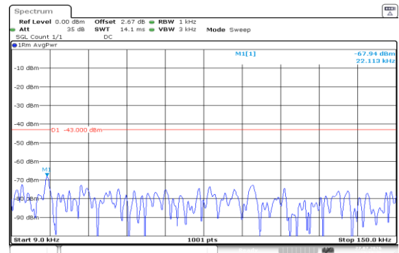
Band2-15MHz-16QAM-18675-1RB#0-0.009~0.15-PASS
