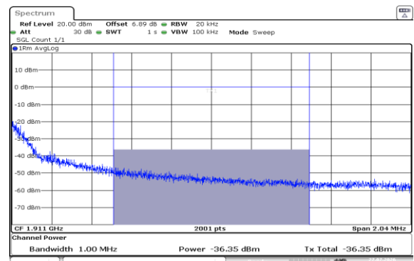
Band2-5MHz-QPSK-19175-1RB#24-1000~3000-PASS
