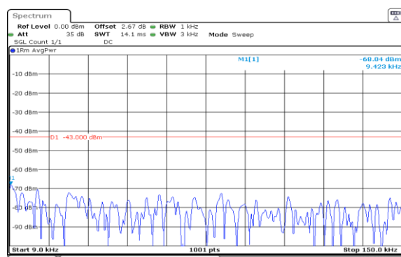
Band2-15MHz-QPSK-18900-75RB#0-0.009~0.15-PASS
