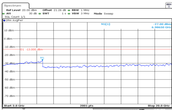
Band2-10MHz-16QAM-18650-1RB#0-3000~20000-PASS
