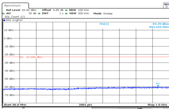
Band2-10MHz-16QAM-18900-1RB#49-30~1000-PASS
