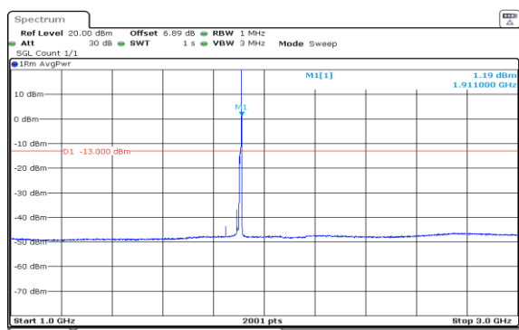
Band2-10MHz-QPSK-19150-1RB#49-1000~3000
