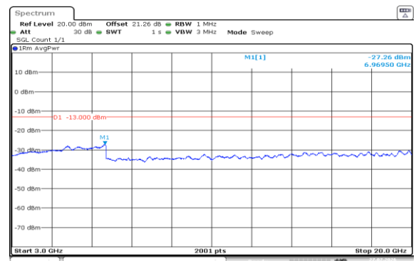
Band2-10MHz-QPSK-18650-1RB#49-3000~20000-PASS
