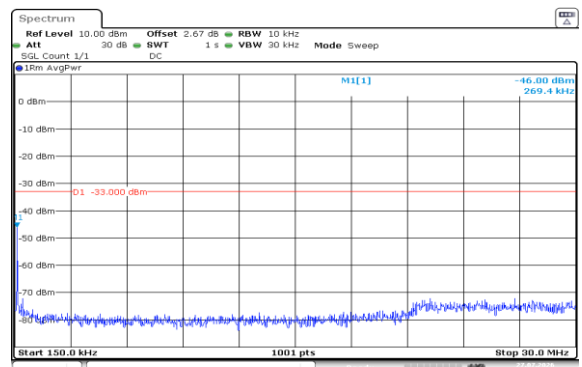
Band2-5MHz-16QAM-19175-1RB#0-0.15~30-PASS
