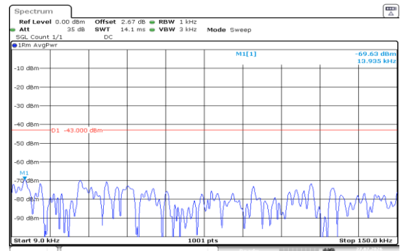
Band2-10MHz-QPSK-18900-50RB#0-0.009~0.15-PASS
