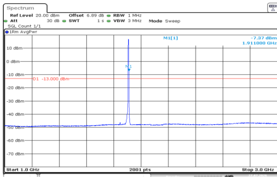
Band2-5MHz-16QAM-19175-25RB#0-1000~3000
