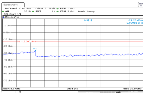
Band2-15MHz-16QAM-18675-1RB#0-3000~20000-PASS
