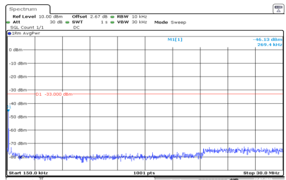
Band2-10MHz-16QAM-19150-50RB#0-0.15~30-PASS
