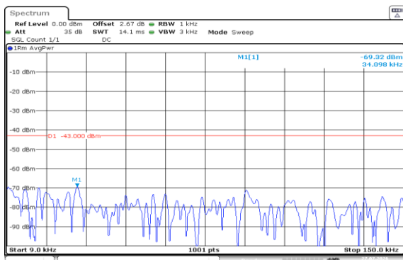
Band2-15MHz-16QAM-18675-75RB#0-0.009~0.15-PASS
