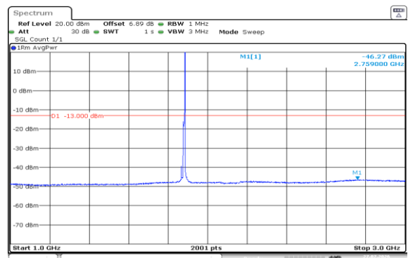
Band2-10MHz-16QAM-18900-1RB#49-1000~3000-PASS
