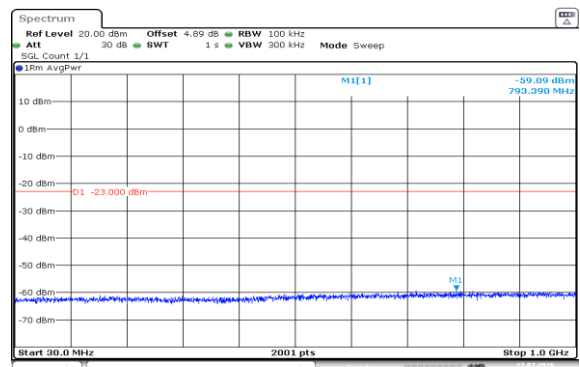
Band2-10MHz-QPSK-18900-1RB#0-30~1000-PASS
