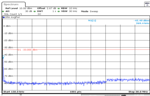
Band2-10MHz-QPSK-19150-50RB#0-0.15~30-PASS
