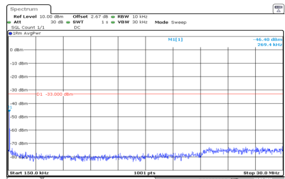
Band2-10MHz-16QAM-18900-50RB#0-0.15~30-PASS
