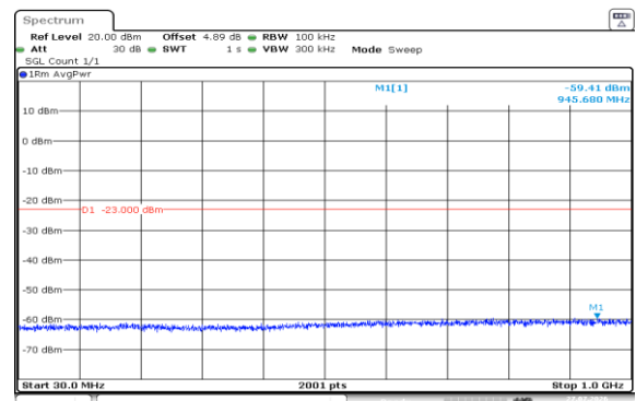
Band2-10MHz-QPSK-19150-1RB#49-30~1000-PASS
