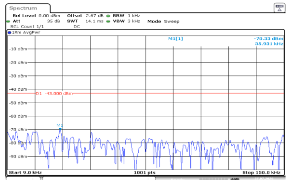
Band2-5MHz-16QAM-19175-1RB#24-0.009~0.15-PASS
