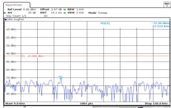
Band2-15MHz-QPSK-18675-75RB#0-0.009~0.15-PASS
