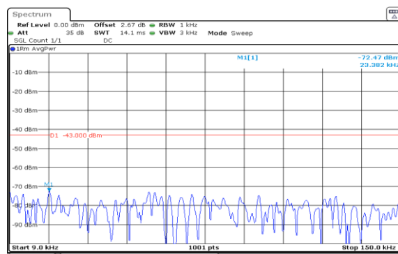
Band2-10MHz-16QAM-19150-1RB#49-0.009~0.15-PASS
