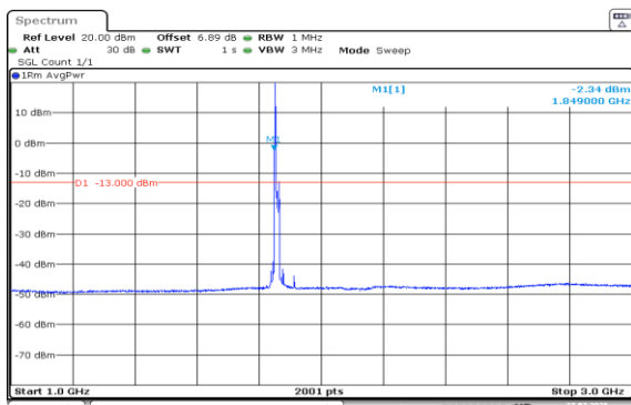
Band2-15MHz-QPSK-18675-1RB#0-1000~3000
