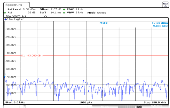
Band2-10MHz-QPSK-18650-50RB#0-0.009~0.15-PASS
