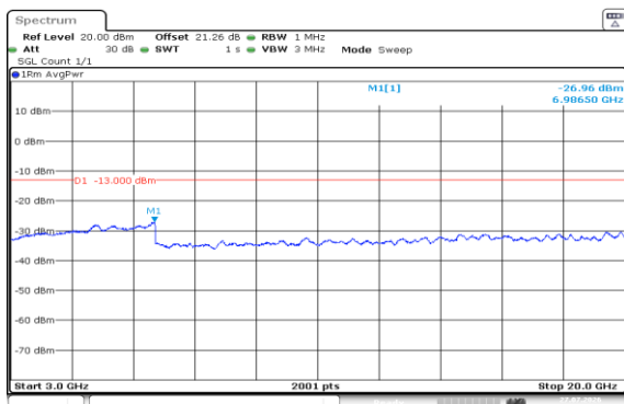
Band2-10MHz-16QAM-18900-50RB#0-3000~20000-PASS
