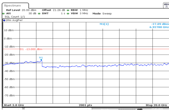
Band2-15MHz-16QAM-18675-75RB#0-3000~20000-PASS
