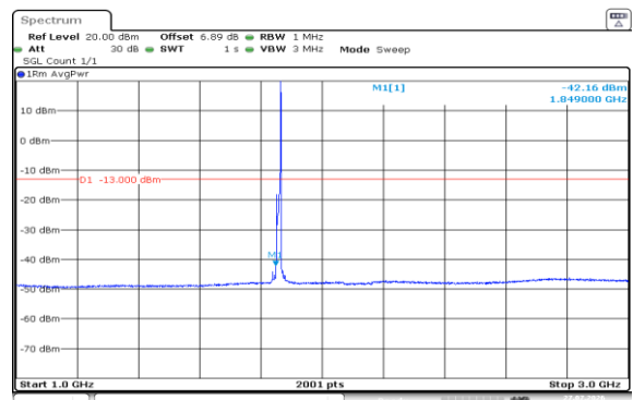
Band2-15MHz-16QAM-18675-1RB#74-1000~3000-PASS
