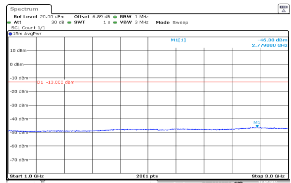
Band2-10MHz-16QAM-18650-1RB#49-1000~3000-PASS
