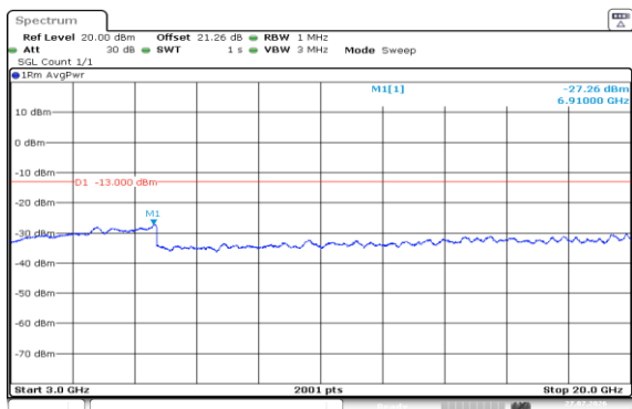
Band2-10MHz-16QAM-18900-1RB#0-3000~20000-PASS
