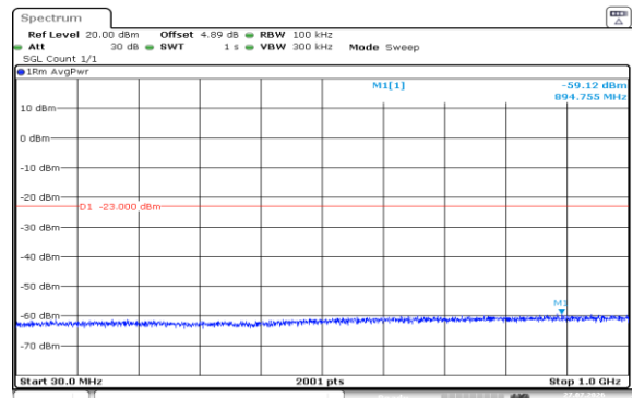
Band2-15MHz-QPSK-18675-1RB#74-30~1000-PASS
