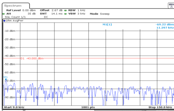
Band2-10MHz-16QAM-18900-50RB#0-0.009~0.15-PASS
