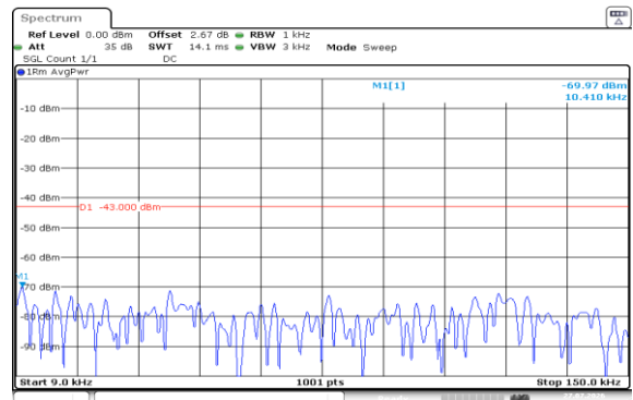
Band2-10MHz-QPSK-18650-1RB#0-0.009~0.15-PASS
