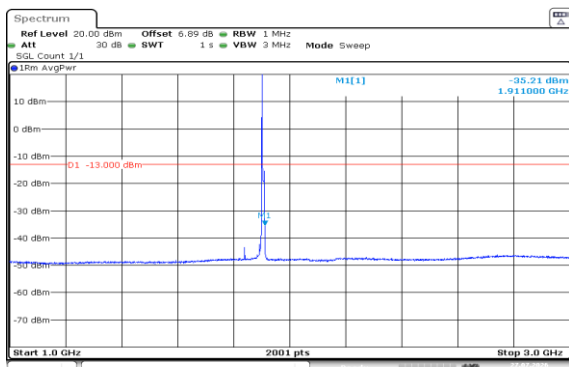
Band2-10MHz-QPSK-19150-1RB#0-1000~3000-PASS
