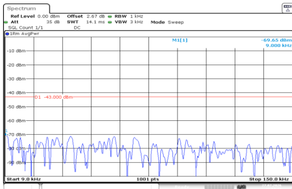
Band2-10MHz-16QAM-19150-1RB#0-0.009~0.15-PASS
