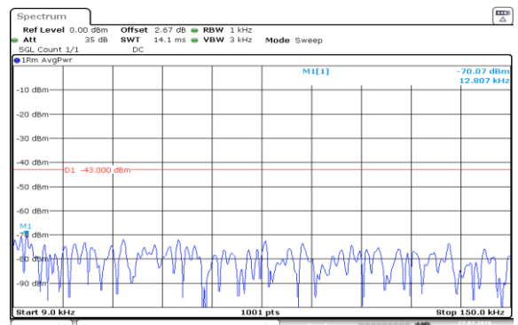
Band2-10MHz-QPSK-18650-1RB#49-0.009~0.15-PASS
