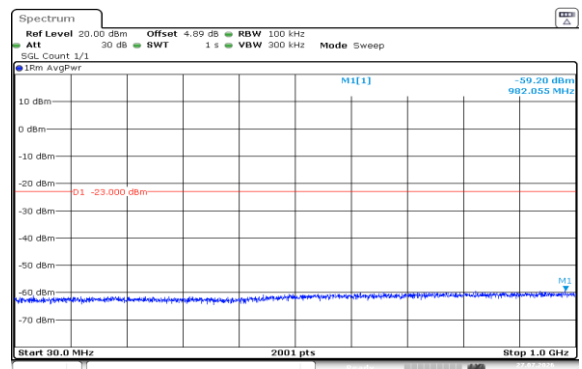
Band2-5MHz-QPSK-19175-1RB#0-30~1000-PASS
