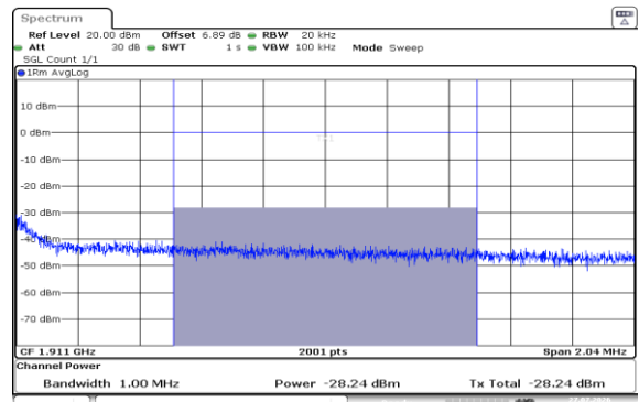
Band2-5MHz-QPSK-19175-25RB#0-1000~3000-PASS
