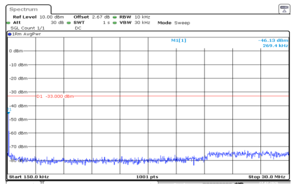
Band2-15MHz-16QAM-18675-75RB#0-0.15~30-PASS
