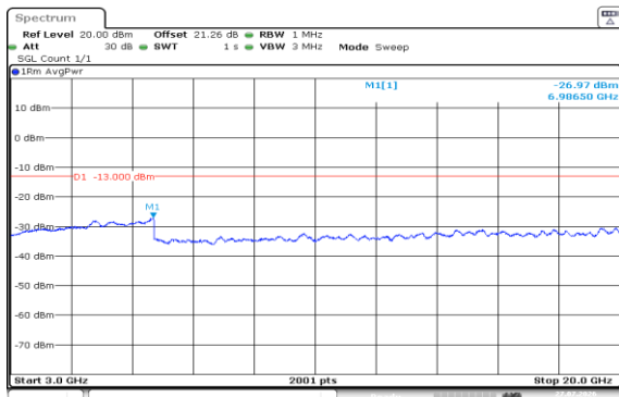
Band2-10MHz-16QAM-18900-1RB#49-3000~20000-PASS
