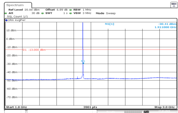
Band2-5MHz-16QAM-19175-1RB#0-1000~3000-PASS
