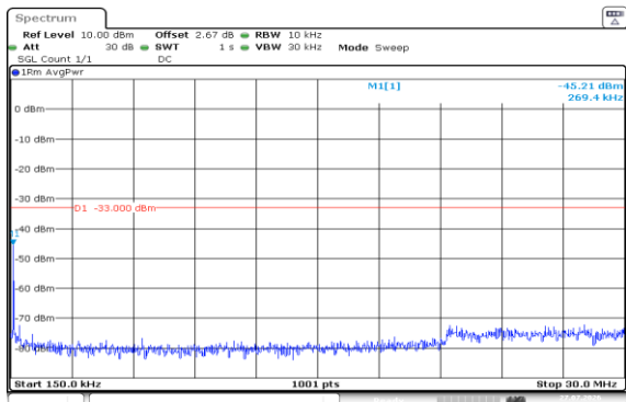
Band2-10MHz-QPSK-18650-50RB#0-0.15~30-PASS
