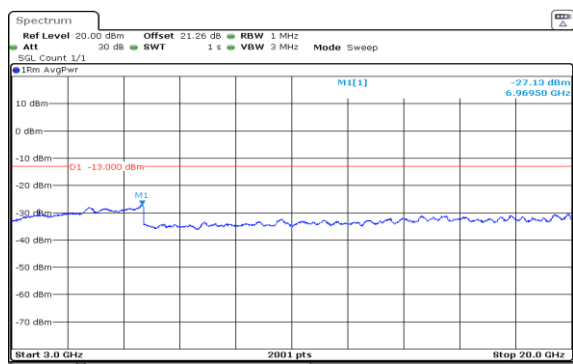
Band2-10MHz-QPSK-19150-1RB#49-3000~20000-PASS
