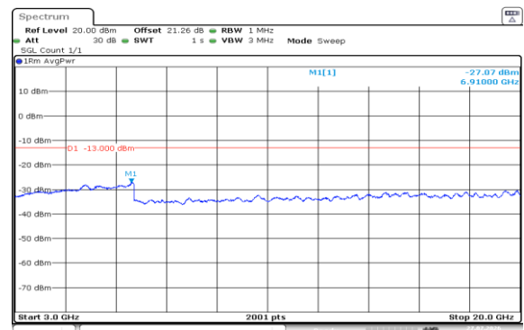
Band2-15MHz-QPSK-18900-1RB#0-3000~20000-PASS
