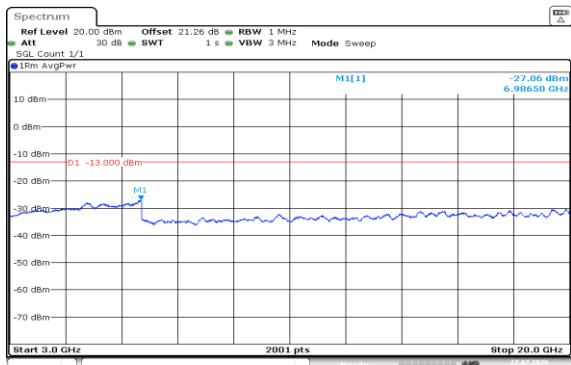
Band2-5MHz-16QAM-18900-25RB#0-3000~20000-PASS
