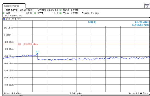
Band2-15MHz-16QAM-18900-1RB#74-3000~20000-PASS
