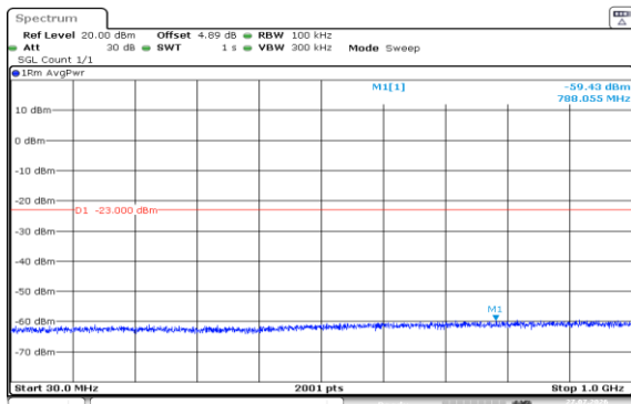
Band2-10MHz-16QAM-19150-1RB#0-30~1000-PASS
