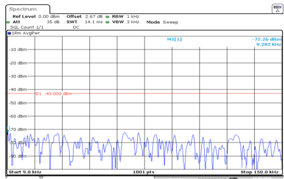
Band2-15MHz-QPSK-18900-1RB#74-0.009~0.15-PASS
