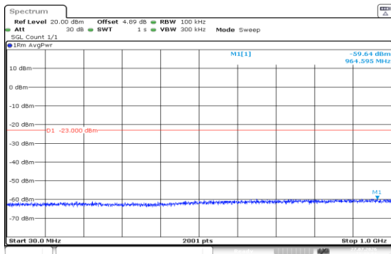
Band2-5MHz-16QAM-19175-1RB#0-30~1000-PASS
