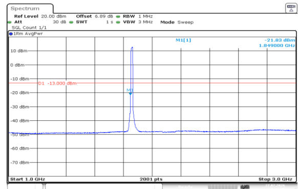
Band2-15MHz-16QAM-18675-75RB#0-1000~3000-PASS
