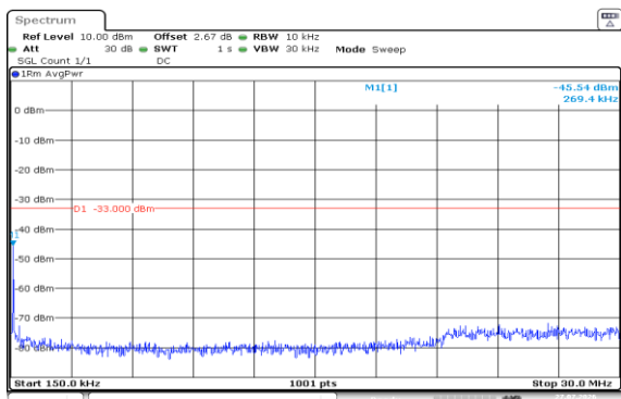
Band2-5MHz-16QAM-19175-1RB#24-0.15~30-PASS
