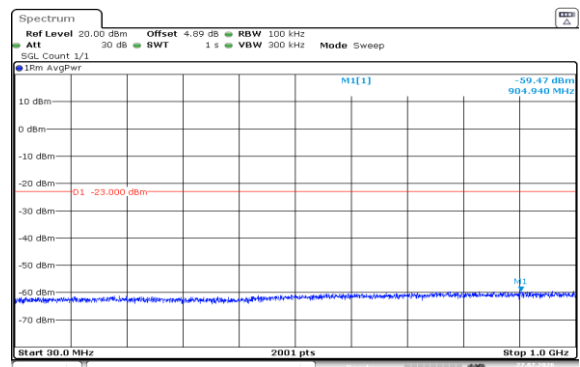
Band2-15MHz-QPSK-18675-75RB#0-30~1000-PASS
