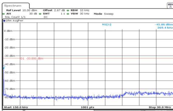
Band2-5MHz-16QAM-19175-25RB#0-0.15~30-PASS
