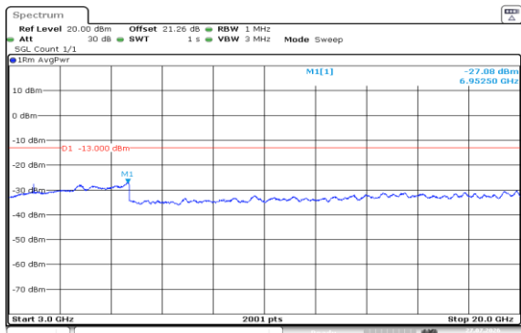
Band2-10MHz-16QAM-19150-1RB#49-3000~20000-PASS
