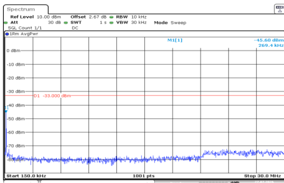
Band2-10MHz-QPSK-18900-1RB#0-0.15~30-PASS
