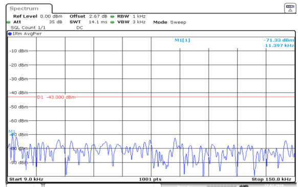
Band2-10MHz-QPSK-19150-50RB#0-0.009~0.15-PASS
