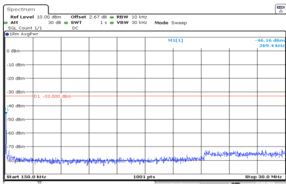
Band2-10MHz-16QAM-18650-1RB#0-0.15~30-PASS
