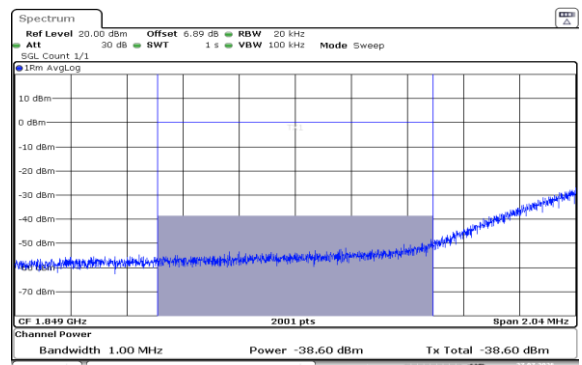
Band2-15MHz-QPSK-18675-1RB#0-1000~3000-PASS
