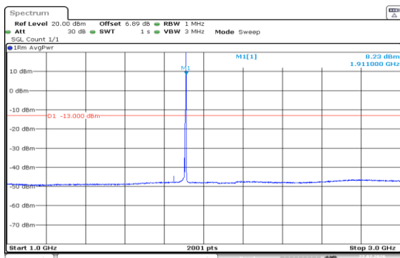
Band2-5MHz-QPSK-19175-1RB#24-1000~3000
