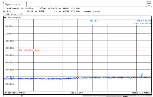
Band2-10MHz-QPSK-19150-50RB#0-30~1000-PASS
