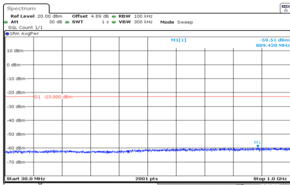
Band2-15MHz-16QAM-18900-1RB#0-30~1000-PASS
