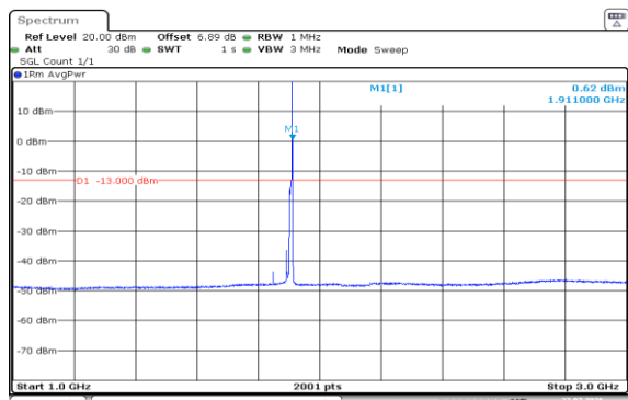
Band2-10MHz-16QAM-19150-1RB#49-1000~3000
