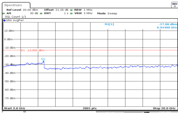
Band2-5MHz-QPSK-19175-1RB#24-3000~20000-PASS
