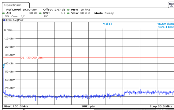
Band2-10MHz-16QAM-18650-50RB#0-0.15~30-PASS
