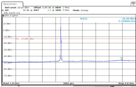
Band2-10MHz-QPSK-18900-1RB#0-1000~3000-PASS
