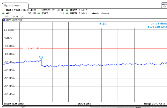
Band2-15MHz-16QAM-18900-1RB#0-3000~20000-PASS
