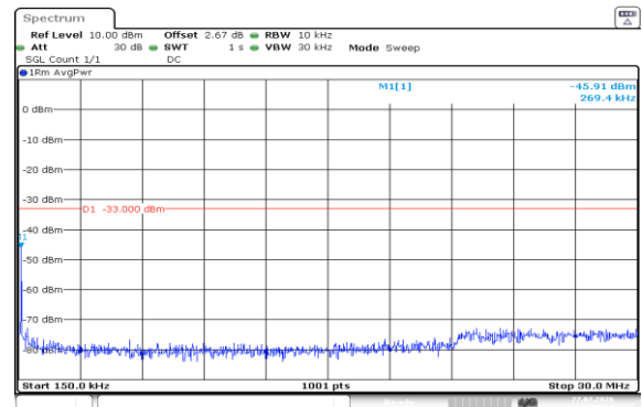
Band2-10MHz-16QAM-19150-1RB#0-0.15~30-PASS
