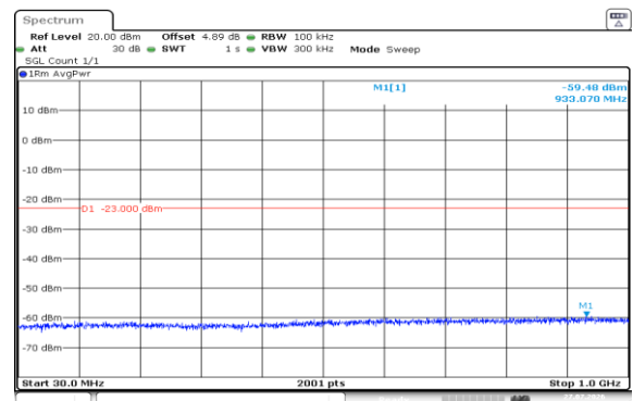
Band2-5MHz-QPSK-19175-1RB#24-30~1000-PASS
