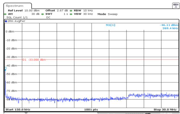
Band2-10MHz-16QAM-18900-1RB#0-0.15~30-PASS
