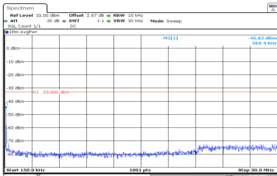
Band2-10MHz-QPSK-18650-1RB#49-0.15~30-PASS
