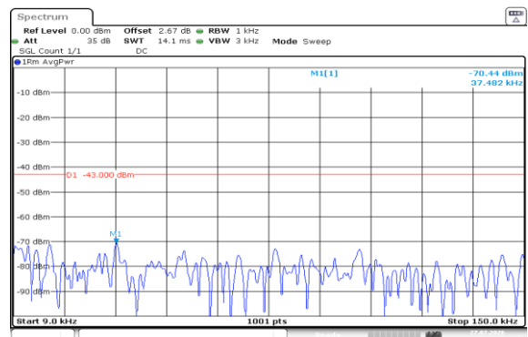
Band2-10MHz-QPSK-18900-1RB#49-0.009~0.15-PASS
