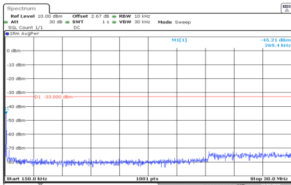
Band2-10MHz-QPSK-18900-1RB#49-0.15~30-PASS
