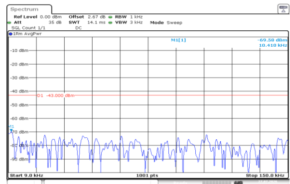
Band2-15MHz-QPSK-18675-1RB#74-0.009~0.15-PASS
