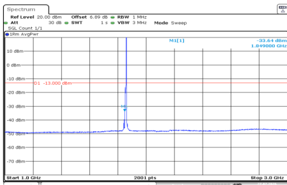
Band2-10MHz-QPSK-18650-1RB#49-1000~3000-PASS
