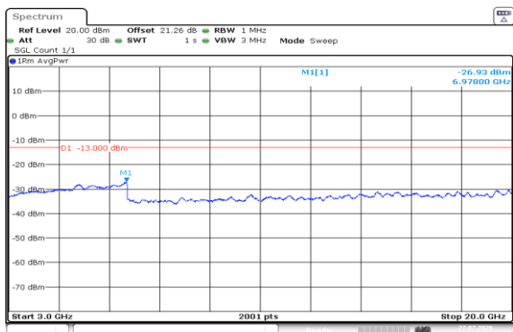
Band2-10MHz-QPSK-18650-50RB#0-3000~20000-PASS
