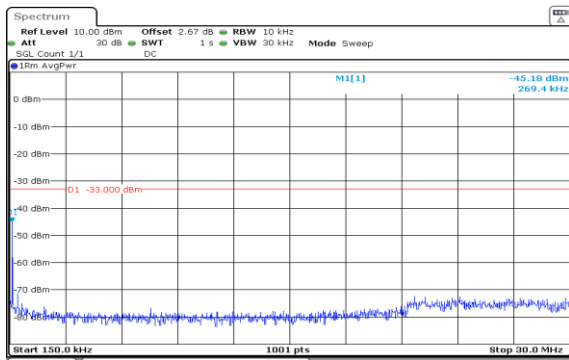
Band2-5MHz-QPSK-19175-25RB#0-0.15~30-PASS
