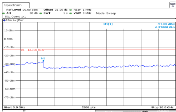
Band2-10MHz-QPSK-18650-1RB#0-3000~20000-PASS
