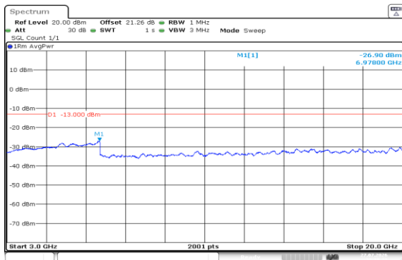
Band2-15MHz-QPSK-18675-1RB#0-3000~20000-PASS
