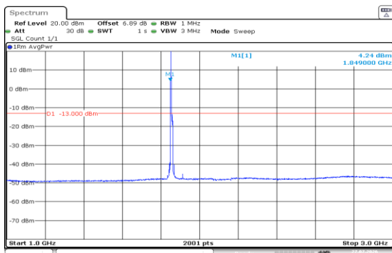
Band2-10MHz-QPSK-18650-1RB#0-1000~3000
