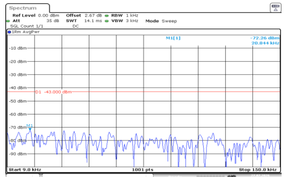
Band2-10MHz-16QAM-18650-1RB#0-0.009~0.15-PASS
