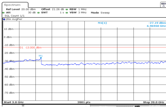
Band2-5MHz-16QAM-19175-1RB#0-3000~20000-PASS
