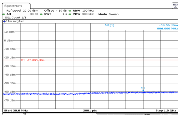
Band2-10MHz-16QAM-18650-1RB#49-30~1000-PASS
