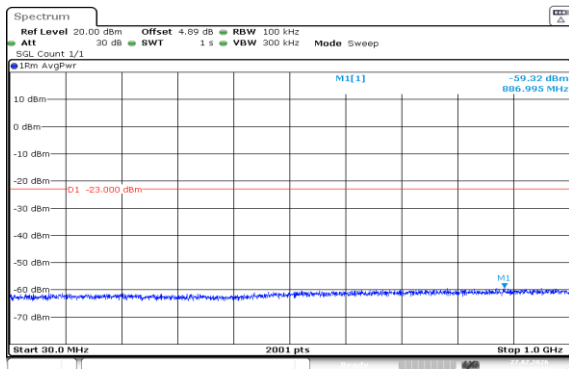
Band2-15MHz-16QAM-18675-75RB#0-30~1000-PASS
