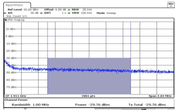
Band2-5MHz-16QAM-19175-25RB#0-1000~3000-PASS
