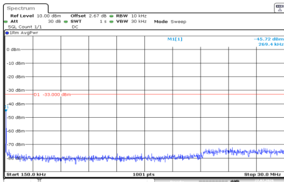
Band2-15MHz-QPSK-18675-1RB#74-0.15~30-PASS
