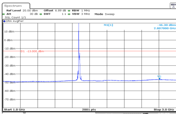
Band2-15MHz-QPSK-18900-1RB#0-1000~3000-PASS
