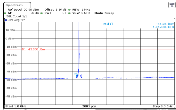
Band2-15MHz-16QAM-18900-1RB#0-1000~3000-PASS
