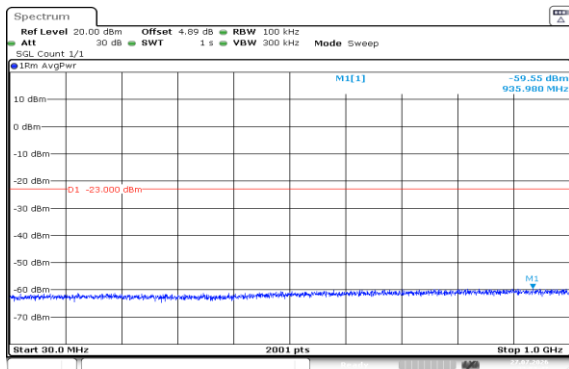
Band2-10MHz-16QAM-19150-50RB#0-30~1000-PASS
