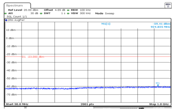
Band2-15MHz-16QAM-18675-1RB#0-30~1000-PASS
