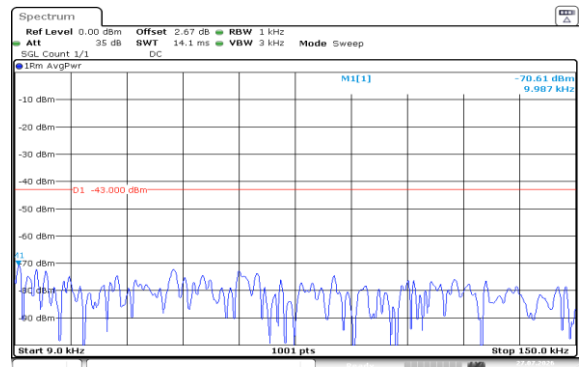
Band2-15MHz-QPSK-18675-1RB#0-0.009~0.15-PASS
