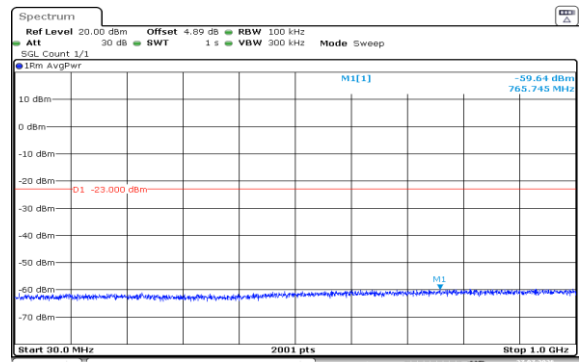
Band2-10MHz-16QAM-18650-50RB#0-30~1000-PASS
