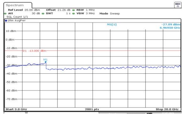
Band2-10MHz-QPSK-18900-1RB#0-3000~20000-PASS
