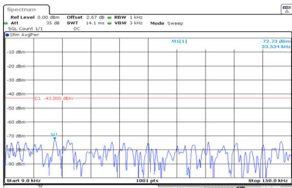
Band2-10MHz-16QAM-19150-50RB#0-0.009~0.15-PASS
