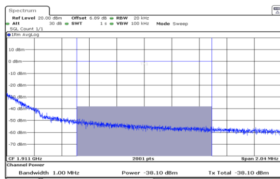
Band2-10MHz-QPSK-19150-1RB#49-1000~3000-PASS
