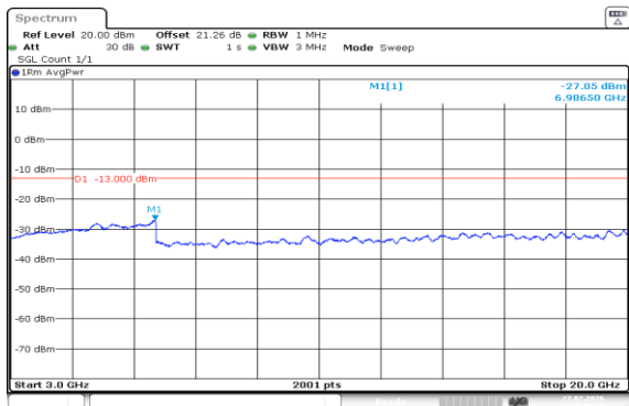
Band2-10MHz-16QAM-18650-1RB#49-3000~20000-PASS
