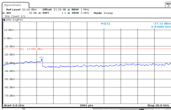
Band2-15MHz-16QAM-18675-1RB#74-3000~20000-PASS
