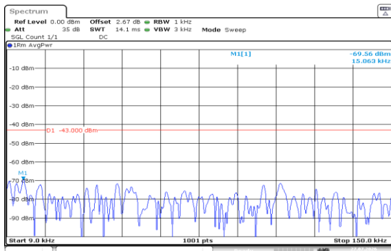
Band2-15MHz-16QAM-18900-1RB#0-0.009~0.15-PASS
