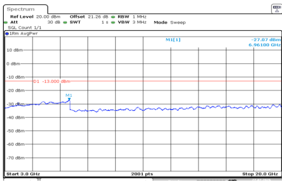
Band2-5MHz-16QAM-19175-1RB#24-3000~20000-PASS
