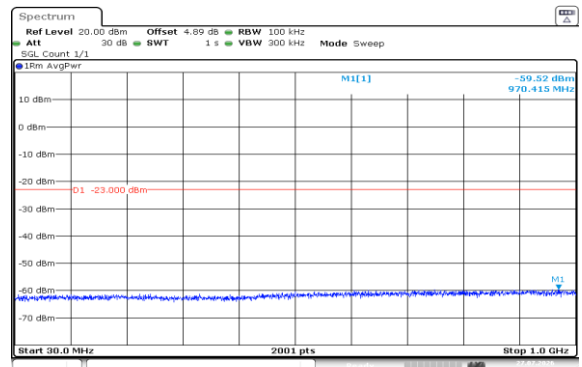
Band2-10MHz-QPSK-18650-50RB#0-30~1000-PASS
