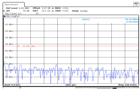
Band2-10MHz-16QAM-18650-50RB#0-0.009~0.15-PASS
