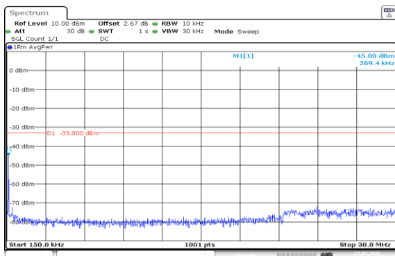
Band2-5MHz-QPSK-19175-1RB#24-0.15~30-PASS
