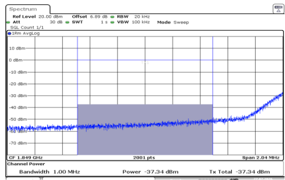
Band2-10MHz-QPSK-18650-1RB#0-1000~3000-PASS
