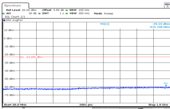
Band2-15MHz-16QAM-18675-1RB#74-30~1000-PASS
