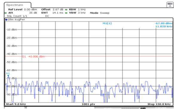
Band2-5MHz-QPSK-19175-1RB#24-0.009~0.15-PASS
