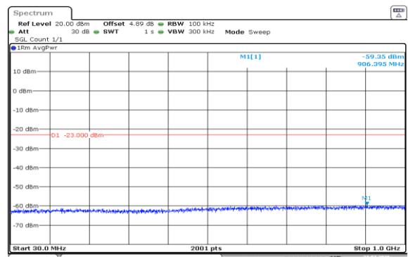
Band2-5MHz-16QAM-19175-25RB#0-30~1000-PASS
