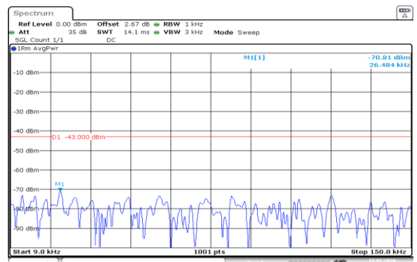
Band2-5MHz-QPSK-19175-25RB#0-0.009~0.15-PASS
