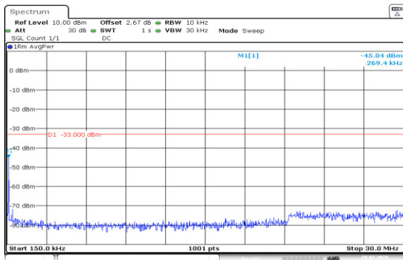
Band2-20MHz-QPSK-19100-1RB#99-0.15~30-PASS
