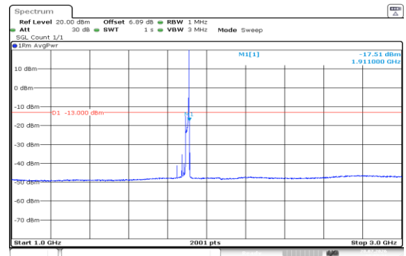
Band2-20MHz-16QAM-19100-1RB#99-1000~3000-PASS
