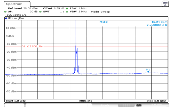
Band2-20MHz-16QAM-18900-1RB#0-1000~3000-PASS
