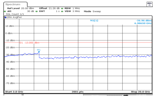
Band2-20MHz-QPSK-18900-1RB#99-3000~20000-PASS
