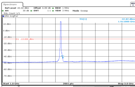
Band2-15MHz-QPSK-18900-75RB#0-1000~3000-PASS
