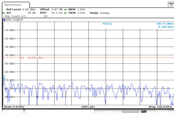
Band2-20MHz-16QAM-19100-1RB#0-0.009~0.15-PASS
