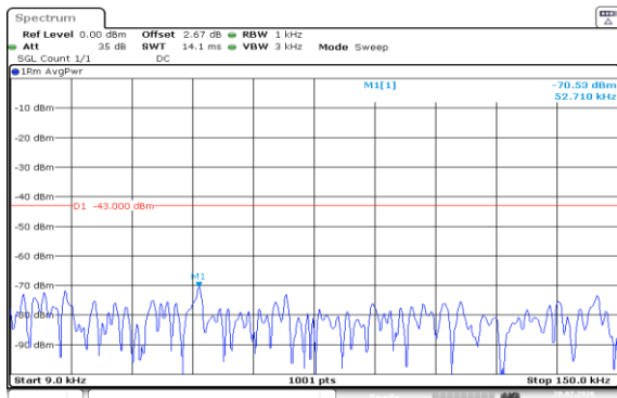
Band2-20MHz-16QAM-19100-1RB#99-0.009~0.15-PASS
