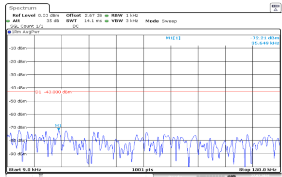
Band2-15MHz-16QAM-19125-1RB#74-0.009~0.15-PASS
