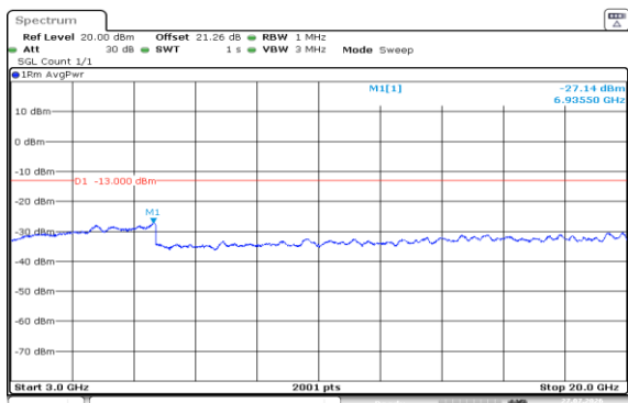
Band2-20MHz-QPSK-18700-1RB#0-3000~20000-PASS
