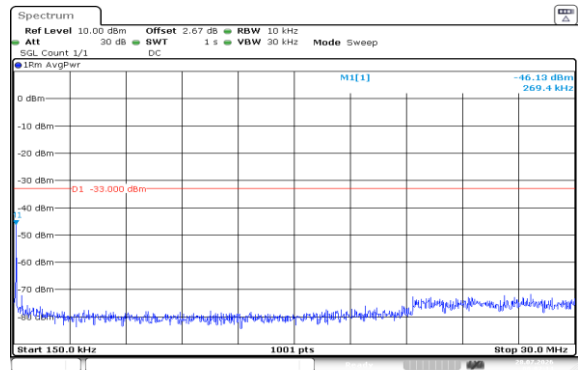
Band2-20MHz-16QAM-19100-1RB#0-0.15~30-PASS
