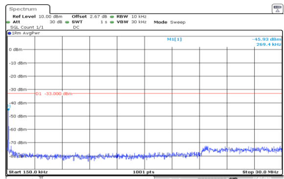
Band2-20MHz-16QAM-18700-1RB#99-0.15~30-PASS
