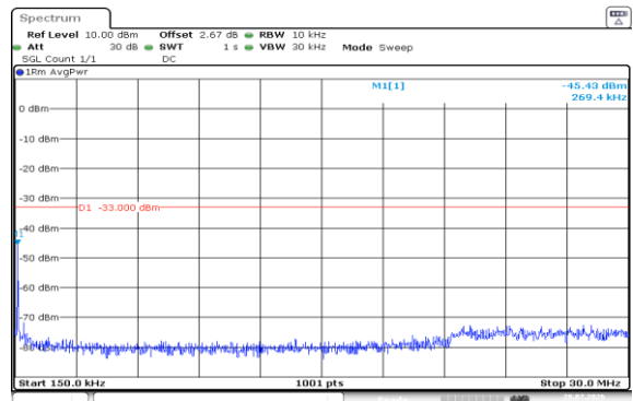
Band2-20MHz-16QAM-19100-1RB#99-0.15~30-PASS
