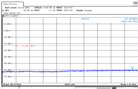
Band2-15MHz-16QAM-19125-1RB#0-30~1000-PASS
