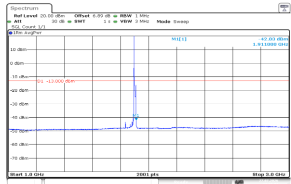
Band2-15MHz-16QAM-19125-1RB#0-1000~3000-PASS
