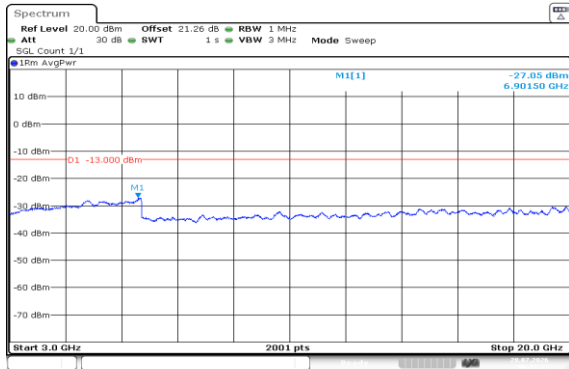
Band2-20MHz-16QAM-19100-1RB#0-3000~20000-PASS
