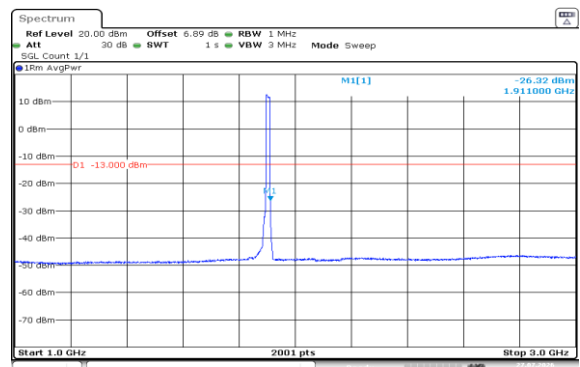
Band2-15MHz-16QAM-19125-75RB#0-1000~3000-PASS
