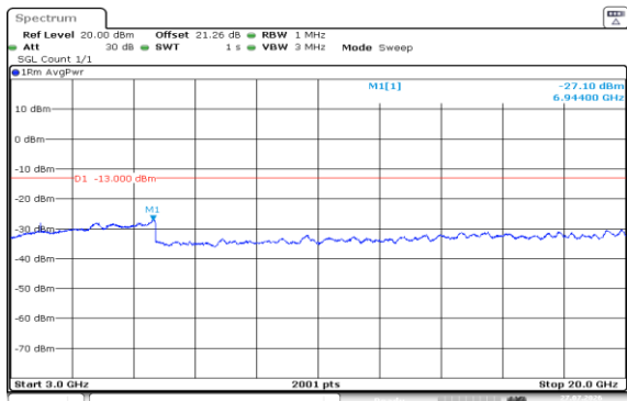
Band2-15MHz-QPSK-19125-1RB#74-3000~20000-PASS
