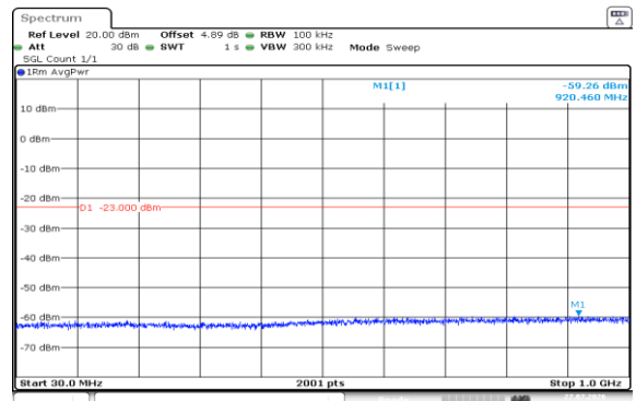
Band2-15MHz-QPSK-19125-1RB#0-30~1000-PASS
