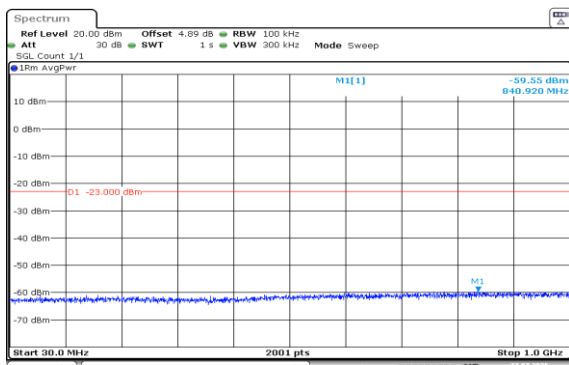
Band2-15MHz-16QAM-18900-75RB#0-30~1000-PASS
