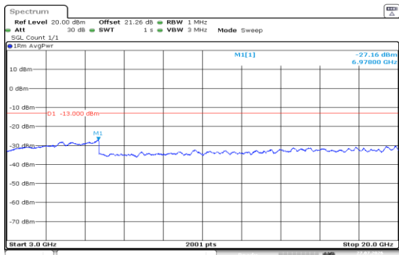
Band2-15MHz-16QAM-18900-75RB#0-3000~20000-PASS
