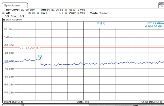
Band2-20MHz-16QAM-18700-1RB#99-3000~20000-PASS
