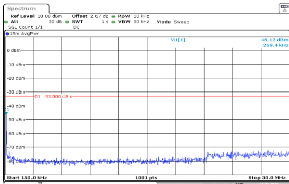
Band2-20MHz-16QAM-18700-1RB#0-0.15~30-PASS
