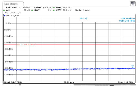
Band2-15MHz-16QAM-19125-1RB#74-30~1000-PASS
