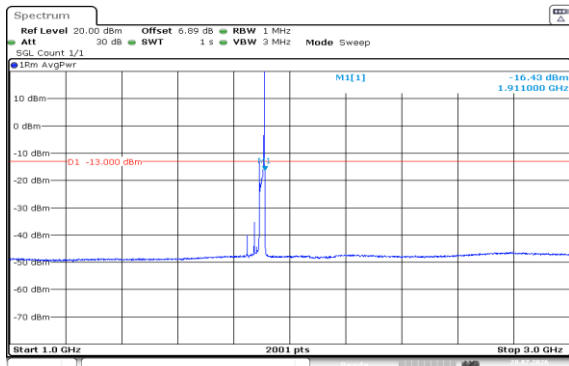
Band2-20MHz-QPSK-19100-1RB#99-1000~3000-PASS
