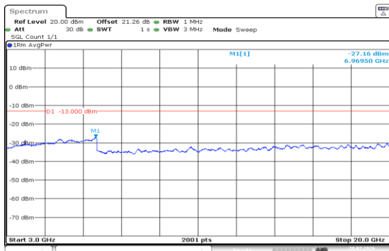
Band2-20MHz-16QAM-19100-1RB#99-3000~20000-PASS
