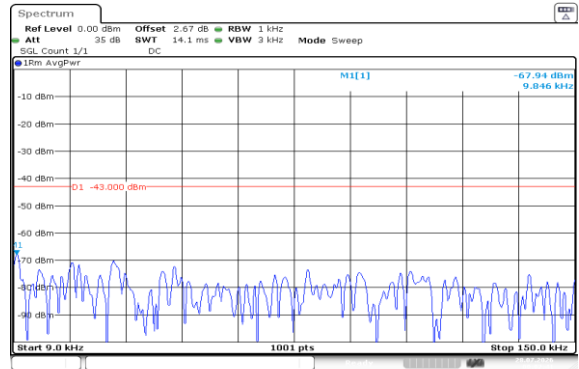
Band2-20MHz-QPSK-19100-1RB#99-0.009~0.15-PASS
