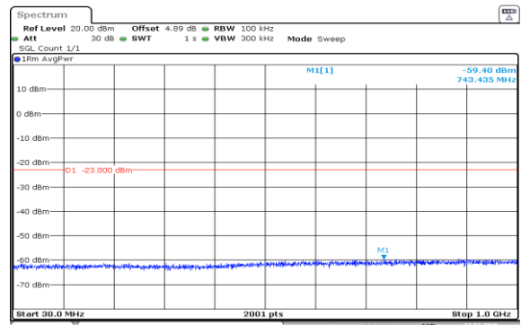
Band2-15MHz-QPSK-18900-75RB#0-30~1000-PASS
