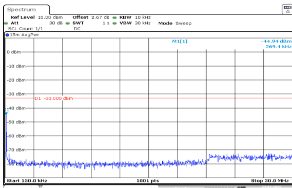
Band2-15MHz-QPSK-19125-1RB#74-0.15~30-PASS
