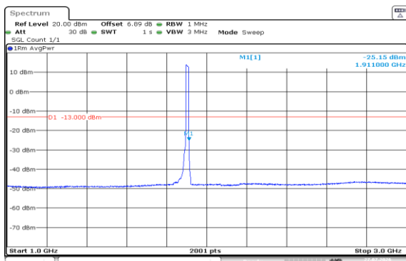
Band2-15MHz-QPSK-19125-75RB#0-1000~3000-PASS
