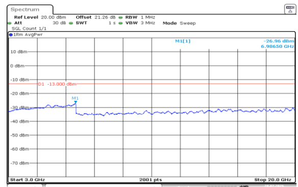
Band2-20MHz-QPSK-19100-100RB#0-3000~20000-PAS
