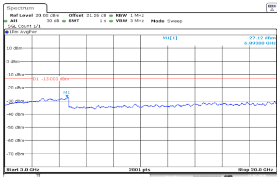
Band2-15MHz-16QAM-19125-75RB#0-3000~20000-PASS
