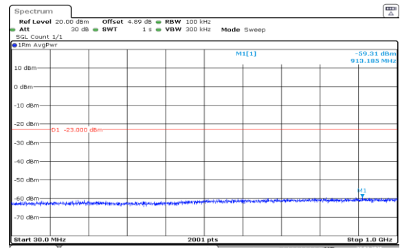
Band2-20MHz-16QAM-18700-1RB#0-30~1000-PASS
