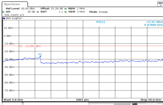
Band2-20MHz-16QAM-18900-1RB#0-3000~20000-PASS
