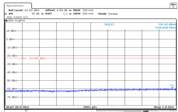
Band2-20MHz-QPSK-19100-100RB#0-30~1000-PASS
