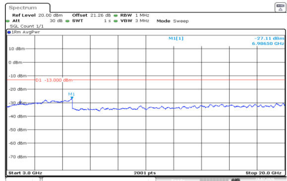
Band2-20MHz-QPSK-19100-1RB#99-3000~20000-PASS
