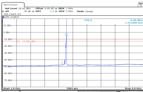
Band2-15MHz-QPSK-19125-1RB#74-1000~3000
