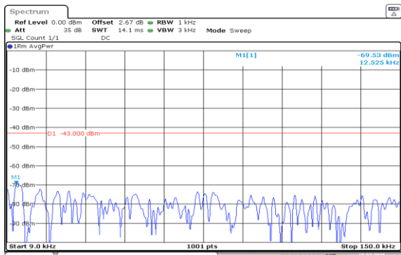
Band2-20MHz-16QAM-18700-100RB#0-0.009~0.15-PASS
