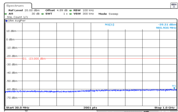
Band2-15MHz-QPSK-19125-1RB#74-30~1000-PASS
