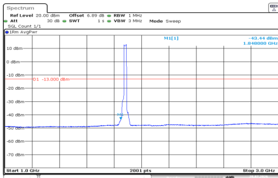
Band2-20MHz-QPSK-18900-100RB#0-1000~3000-PASS
