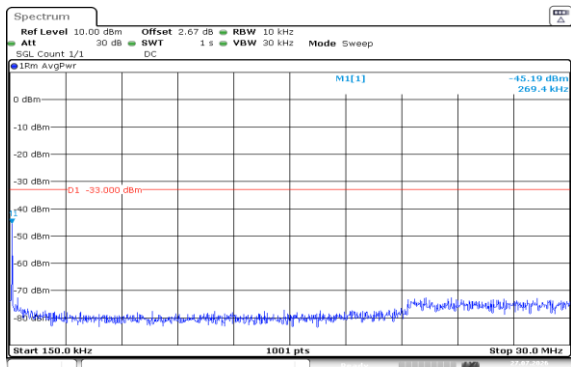
Band2-15MHz-16QAM-19125-1RB#74-0.15~30-PASS
