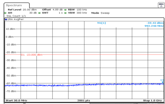
Band2-20MHz-QPSK-18900-100RB#0-30~1000-PASS
