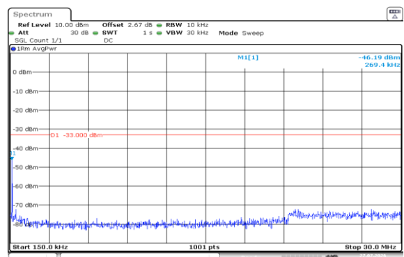
Band2-15MHz-16QAM-19125-75RB#0-0.15~30-PASS
