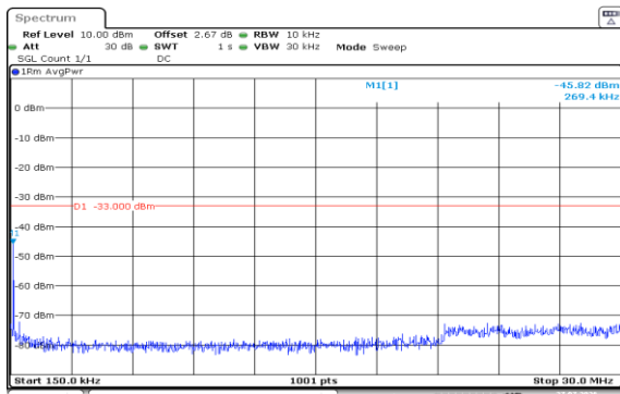
Band2-15MHz-QPSK-18900-75RB#0-0.15~30-PASS
