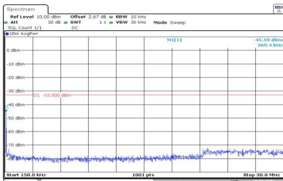
Band2-20MHz-QPSK-18900-100RB#0-0.15~30-PASS
