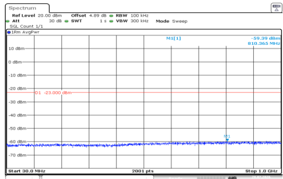
Band2-20MHz-QPSK-19100-1RB#99-30~1000-PASS
