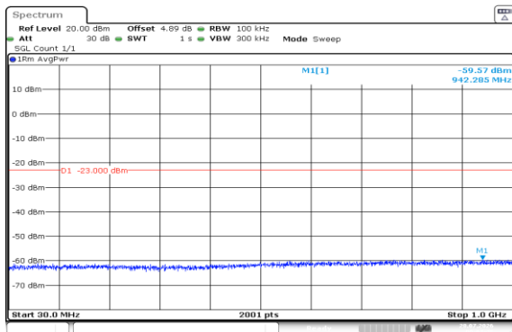
Band2-20MHz-16QAM-19100-1RB#99-30~1000-PASS
