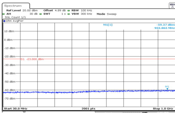
Band2-15MHz-16QAM-19125-75RB#0-30~1000-PASS
