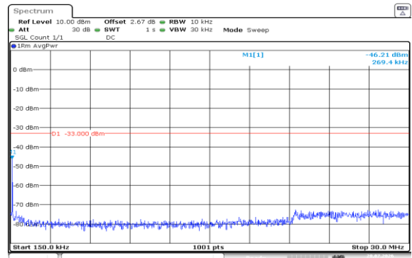
Band2-20MHz-16QAM-18900-100RB#0-0.15~30-PASS
