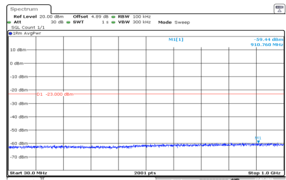
Band2-20MHz-QPSK-18700-1RB#99-30~1000-PASS
