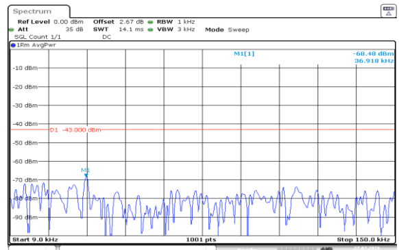
Band2-15MHz-QPSK-19125-1RB#0-0.009~0.15-PASS
