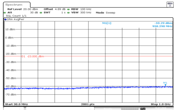
Band2-20MHz-QPSK-19100-1RB#0-30~1000-PASS
