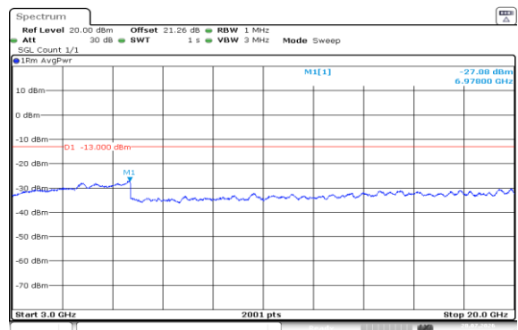
Band2-20MHz-QPSK-19100-1RB#0-3000~20000-PASS
