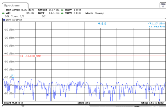
Band2-15MHz-16QAM-19125-1RB#0-0.009~0.15-PASS
