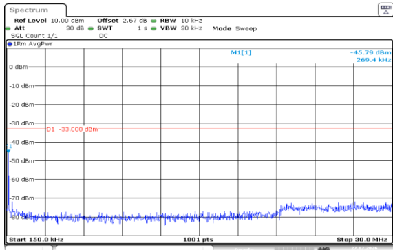
Band2-20MHz-QPSK-18700-100RB#0-0.15~30-PASS
