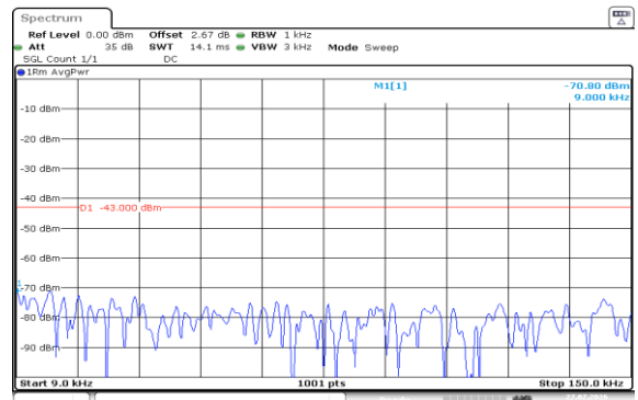
Band2-20MHz-QPSK-18700-1RB#0-0.009~0.15-PASS
