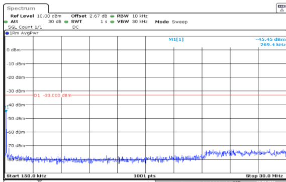
Band2-15MHz-QPSK-19125-75RB#0-0.15~30-PASS
