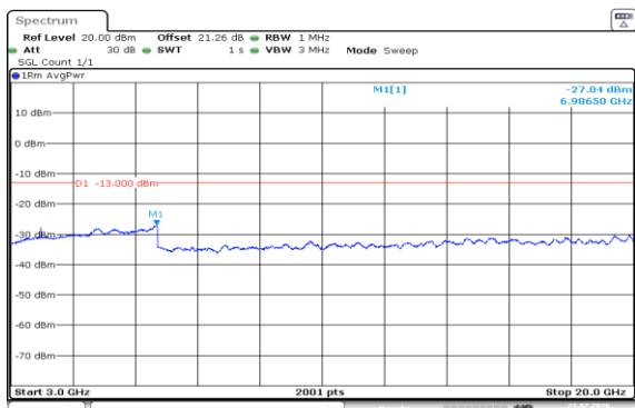
Band2-15MHz-16QAM-19125-1RB#74-3000~20000-PASS
