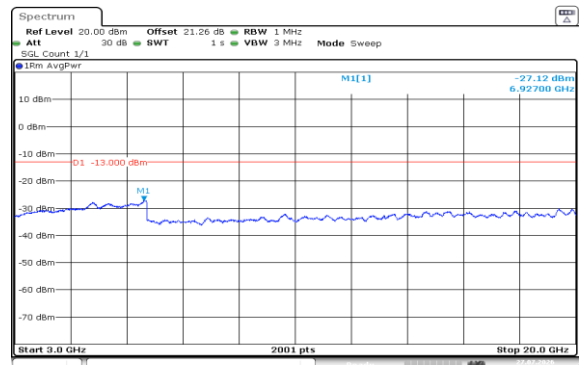
Band2-20MHz-QPSK-18700-1RB#99-3000~20000-PASS
