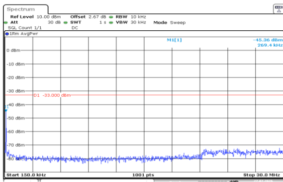
Band2-20MHz-QPSK-18700-1RB#99-0.15~30-PASS
