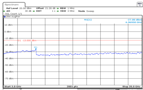
Band2-15MHz-QPSK-18900-75RB#0-3000~20000-PASS
