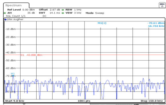
Band2-20MHz-QPSK-18700-100RB#0-0.009~0.15-PASS
