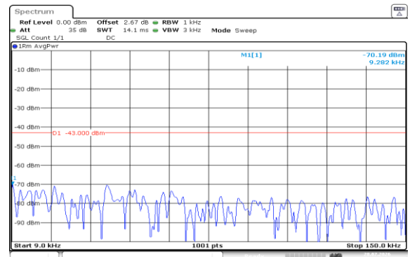
Band2-20MHz-QPSK-19100-100RB#0-0.009~0.15-PASS
