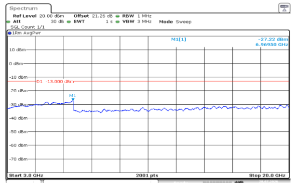
Band2-20MHz-QPSK-18900-100RB#0-3000~20000-PASS S
