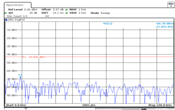
Band2-15MHz-QPSK-19125-1RB#74-0.009~0.15-PASS
