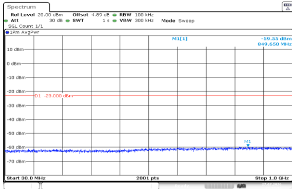
Band2-20MHz-16QAM-18900-1RB#0-30~1000-PASS
