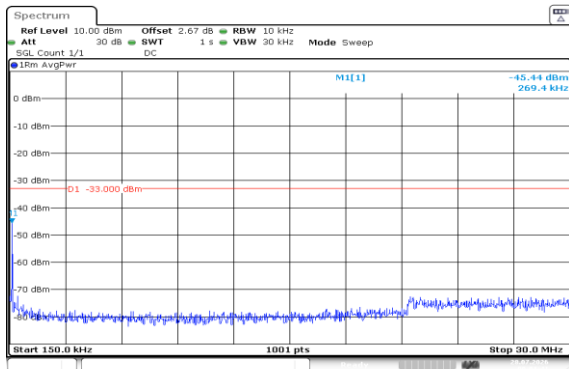
Band2-20MHz-QPSK-19100-1RB#0-0.15~30-PASS
