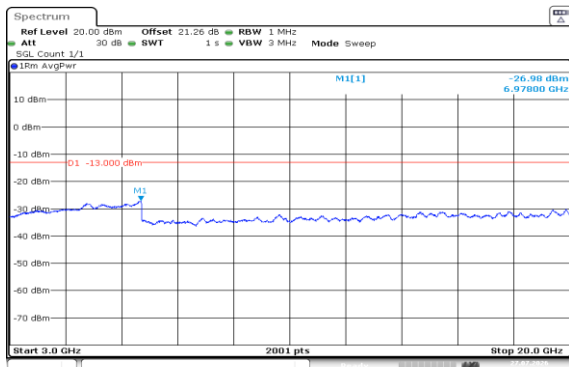
Band2-15MHz-16QAM-19125-1RB#0-3000~20000-PASS
