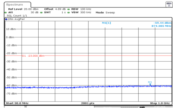
Band2-20MHz-QPSK-18900-1RB#99-30~1000-PASS
