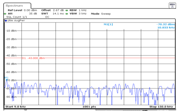
Band2-20MHz-16QAM-18700-1RB#0-0.009~0.15-PASS
