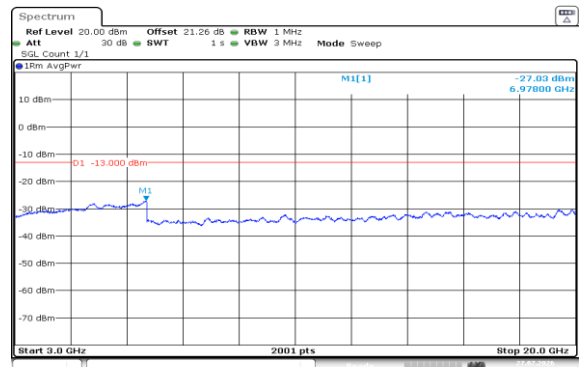
Band2-20MHz-QPSK-18700-100RB#0-3000~20000-PASS S
