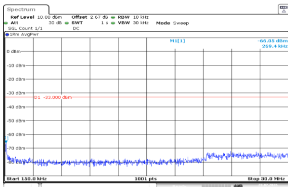
Band2-20MHz-QPSK-19100-100RB#0-0.15~30-PASS
