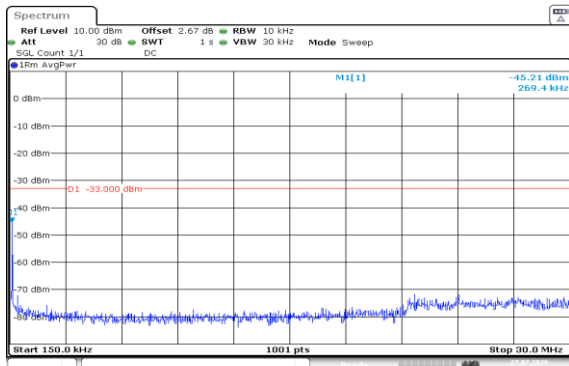
Band2-20MHz-QPSK-18900-1RB#99-0.15~30-PASS
