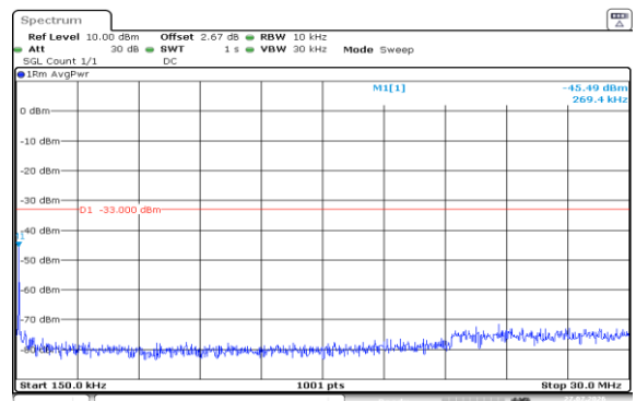
Band2-15MHz-16QAM-19125-1RB#0-0.15~30-PASS
