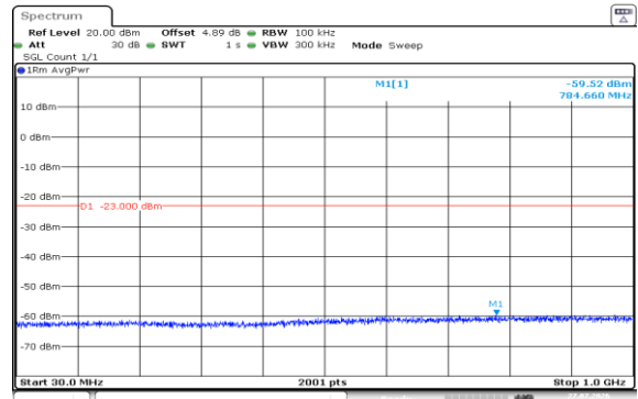
Band2-20MHz-QPSK-18700-100RB#0-30~1000-PASS
