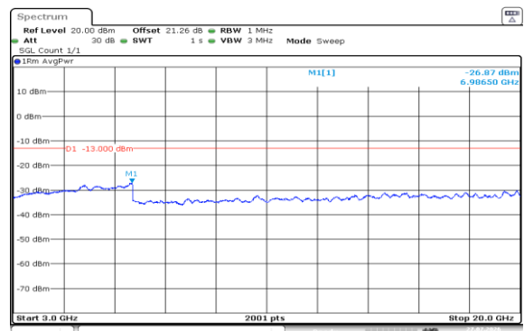
Band2-15MHz-QPSK-19125-75RB#0-3000~20000-PASS
