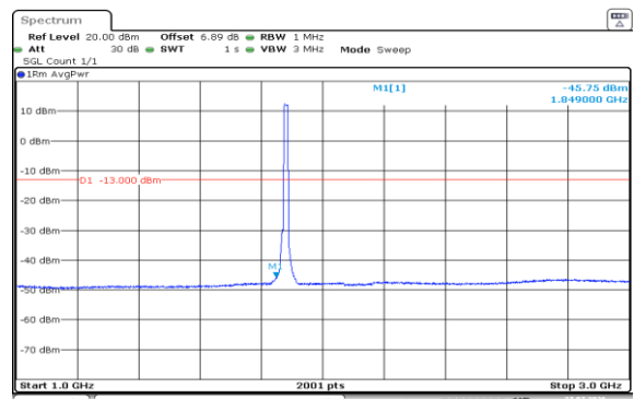
Band2-15MHz-16QAM-18900-75RB#0-1000~3000-PASS
