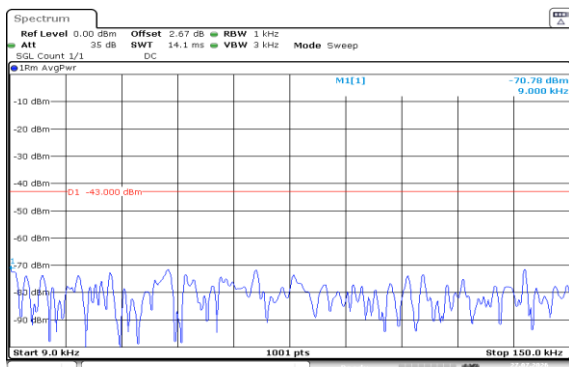
Band2-20MHz-16QAM-18700-1RB#99-0.009~0.15-PASS
