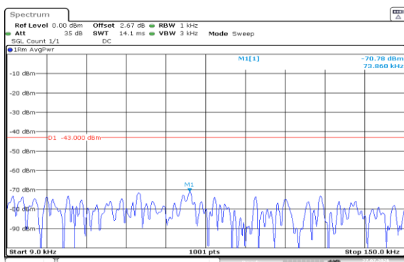
Band2-15MHz-16QAM-19125-75RB#0-0.009~0.15-PASS
