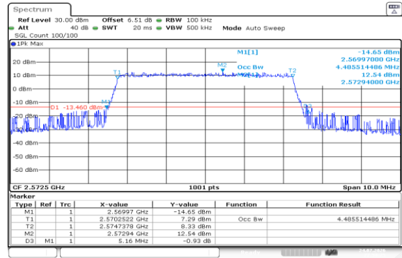
Band38-5MHz-16QAM-37775-25RB#0-PASS
