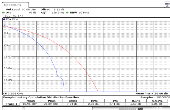
Band38-10MHz-QPSK-38000-50RB#0-PASS
