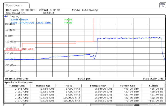
Band38-20MHz-16QAM-37850-1RB#99-PASS
