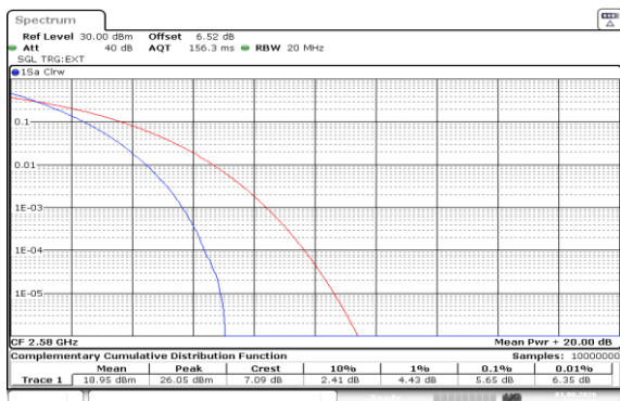
Band38-20MHz-QPSK-37850-100RB#0-PASS
