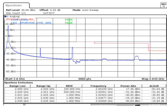
Band38-20MHz-16QAM-38150-1RB#0-PASS
