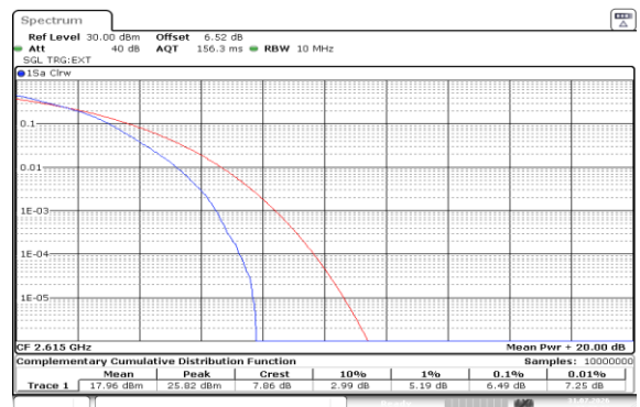
Band38-10MHz-16QAM-38200-50RB#0-PASS
