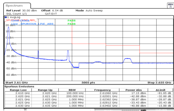
Band38-10MHz-16QAM-38200-1RB#0-PASS
