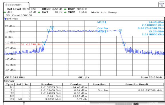
Band38-10MHz-16QAM-38200-50RB#0-PASS
