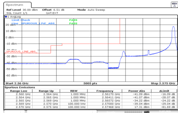
Band38-5MHz-16QAM-37775-1RB#24-PASS
