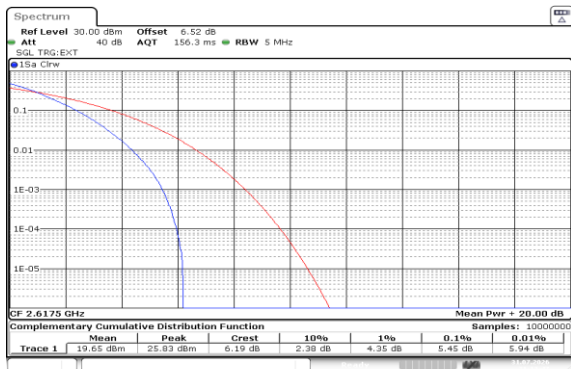
Band38-5MHz-QPSK-38225-25RB#0-PASS
