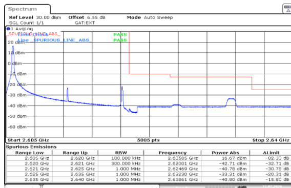
Band38-15MHz-16QAM-38175-1RB#0-PASS
