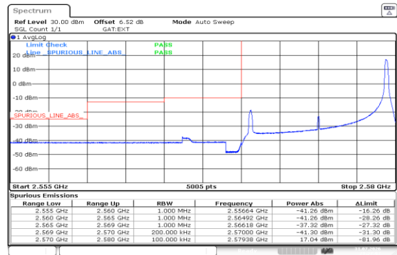
Band38-10MHz-16QAM-37800-1RB#49-PASS
