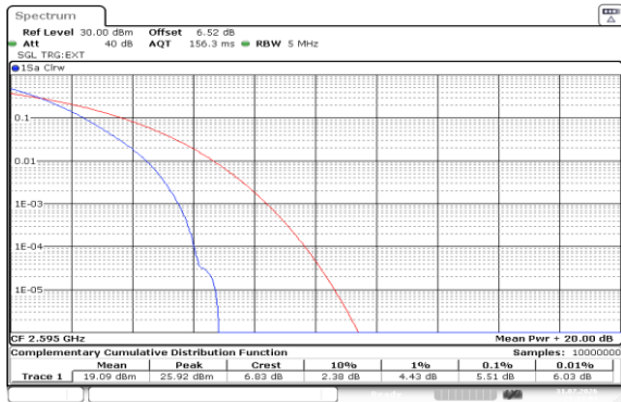
Band38-5MHz-QPSK-38000-25RB#0-PASS
