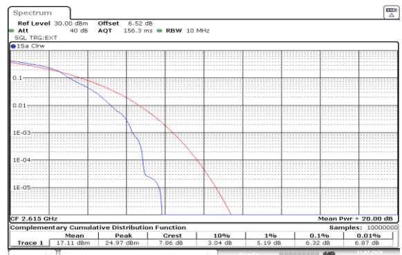
Band38-10MHz-16QAM-38200-1RB#0-PASS
