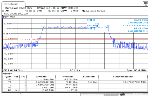
Band38-15MHz-QPSK-38175-75RB#0-PASS
