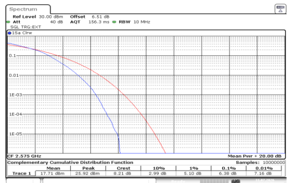
Band38-10MHz-16QAM-37800-50RB#0-PASS
