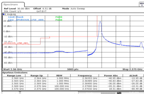
Band38-5MHz-QPSK-37775-1RB#0-PASS
