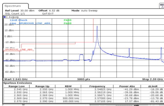
Band38-20MHz-16QAM-37850-1RB#0-PASS
