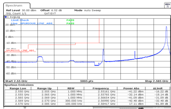
Band38-15MHz-16QAM-37825-1RB#74-PASS
