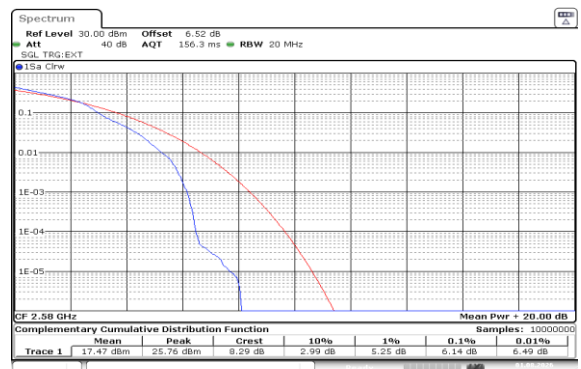
Band38-20MHz-16QAM-37850-1RB#0-PASS
