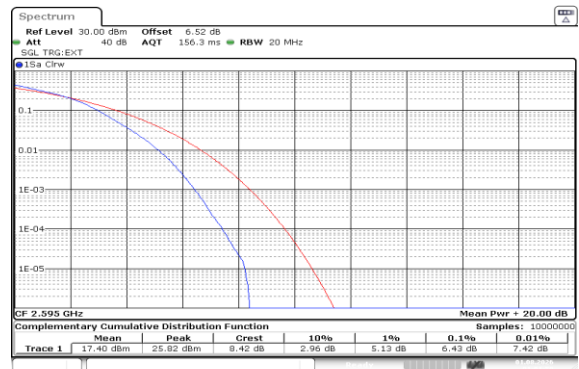
Band38-20MHz-16QAM-38000-100RB#0-PASS
