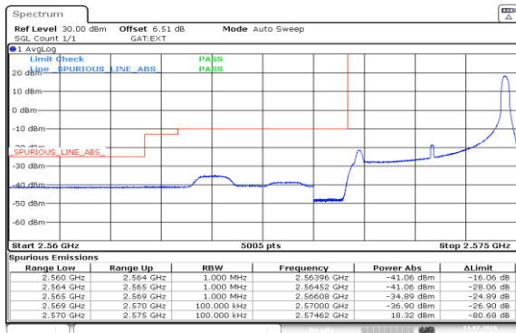
Band38-5MHz-QPSK-37775-1RB#24-PASS
