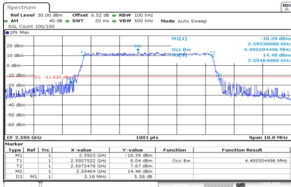
Band38-5MHz-QPSK-38000-25RB#0-PASS
