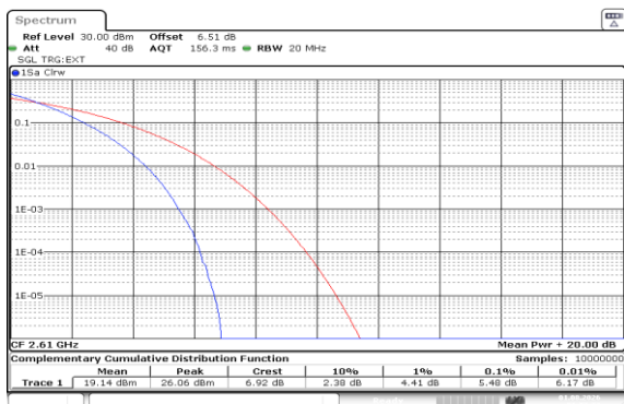
Band38-20MHz-QPSK-38150-100RB#0-PASS
