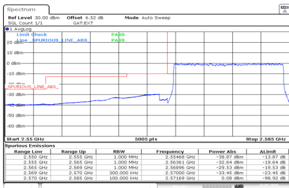
Band38-15MHz-QPSK-37825-75RB#0-PASS
