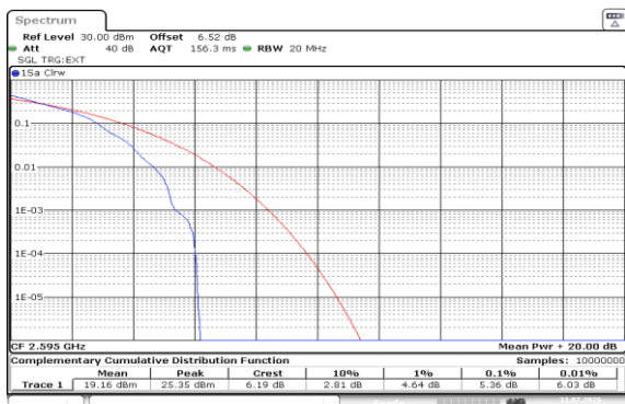
Band38-15MHz-QPSK-38000-1RB#0-PASS
