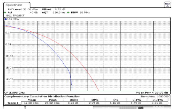
Band38-10MHz-16QAM-38000-50RB#0-PASS
