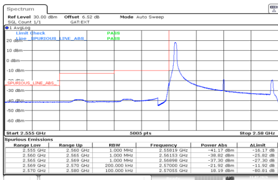
Band38-10MHz-QPSK-37800-1RB#0-PASS
