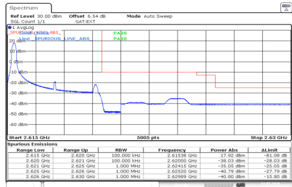
Band38-5MHz-16QAM-38225-1RB#0-PASS
