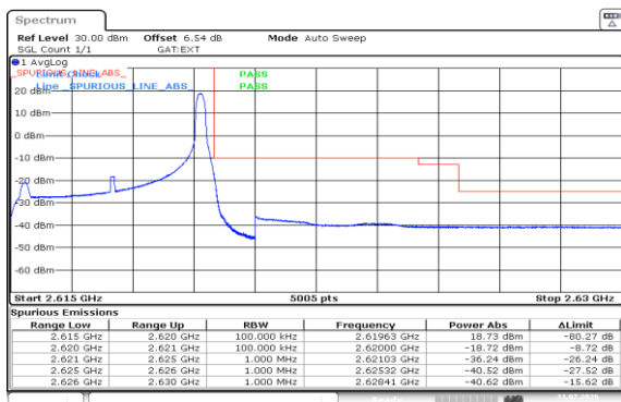
Band38-5MHz-QPSK-38225-1RB#24-PASS
