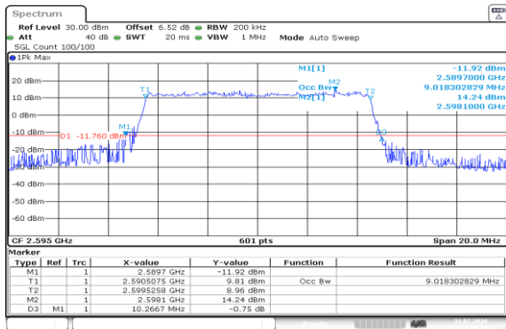
Band38-10MHz-QPSK-38000-50RB#0-PASS
