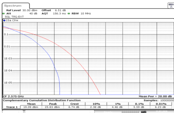
Band38-10MHz-QPSK-37800-50RB#0-PASS
