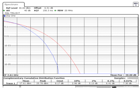
Band38-20MHz-16QAM-38150-100RB#0-PASS
