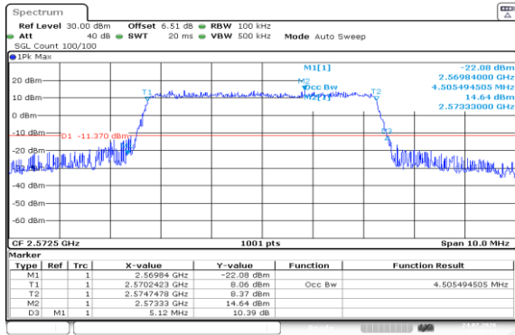
Band38-5MHz-QPSK-37775-25RB#0-PASS
