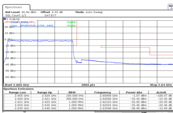
Band38-15MHz-16QAM-38175-75RB#0-PASS
