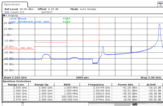
Band38-10MHz-QPSK-37800-1RB#49-PASS
