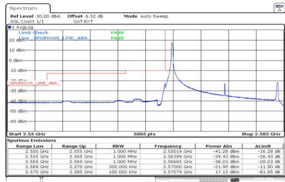
Band38-15MHz-16QAM-37825-1RB#0-PASS
