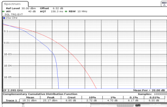
Band38-10MHz-QPSK-38000-1RB#0-PASS
