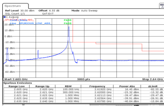
Band38-15MHz-16QAM-38175-1RB#74-PASS
