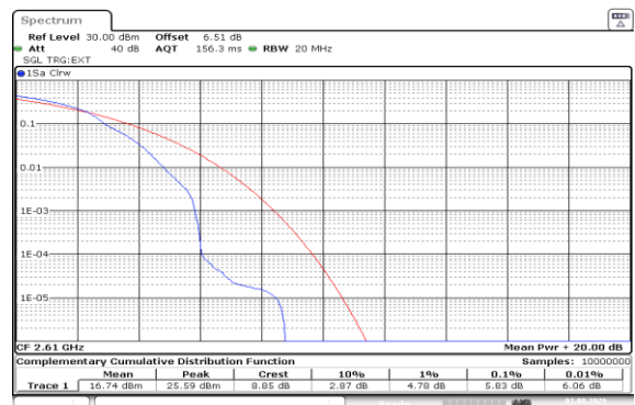
Band38-20MHz-16QAM-38150-1RB#0-PASS
