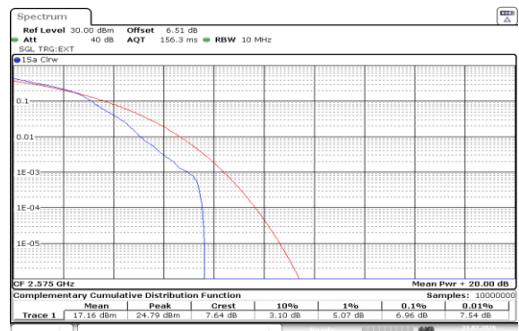
Band38-10MHz-16QAM-37800-1RB#0-PASS
