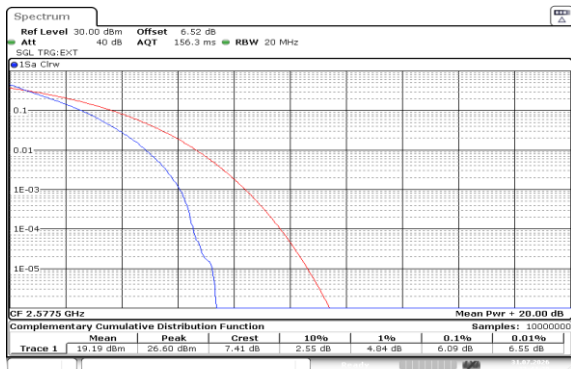
Band38-15MHz-QPSK-37825-75RB#0-PASS
