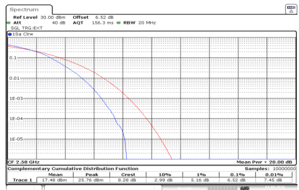
Band38-20MHz-16QAM-37850-100RB#0-PASS
