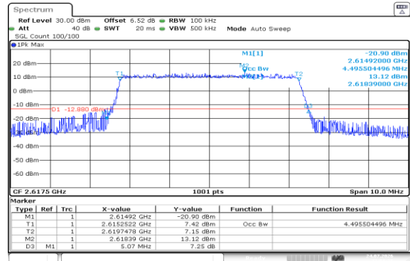
Band38-5MHz-16QAM-38225-25RB#0-PASS
