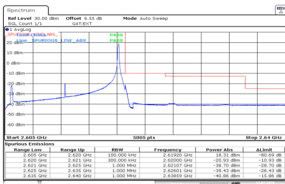
Band38-15MHz-QPSK-38175-1RB#74-PASS
