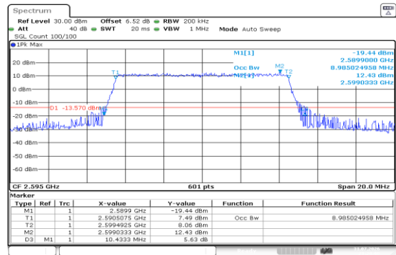
Band38-10MHz-16QAM-38000-50RB#0-PASS
