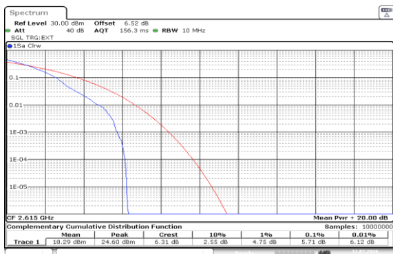
Band38-10MHz-QPSK-38200-1RB#0-PASS
