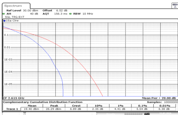
Band38-10MHz-QPSK-38200-50RB#0-PASS
