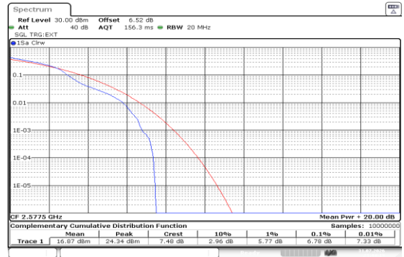
Band38-15MHz-16QAM-37825-1RB#0-PASS
