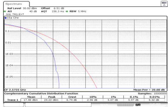
Band38-5MHz-16QAM-37775-1RB#0-PASS
