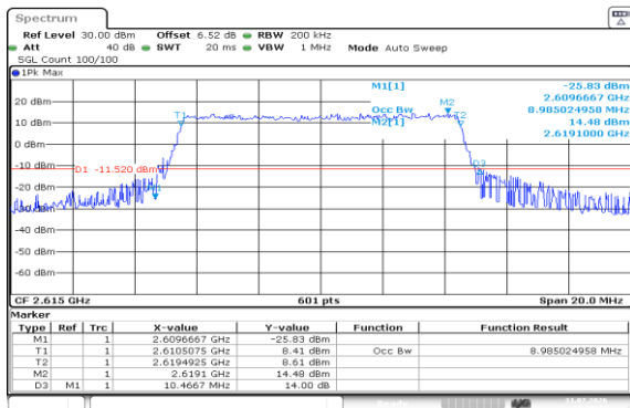
Band38-10MHz-QPSK-38200-50RB#0-PASS
