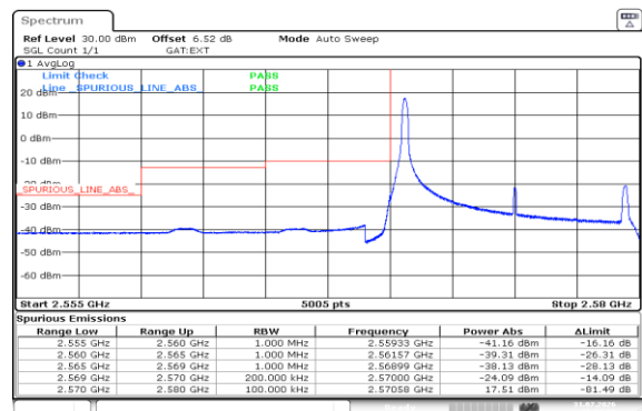
Band38-10MHz-16QAM-37800-1RB#0-PASS
