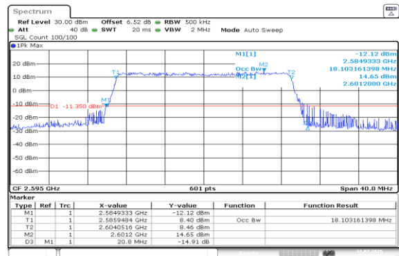
Band38-20MHz-16QAM-38000-100RB#0-PASS
