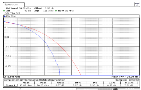
Band38-15MHz-16QAM-38000-75RB#0-PASS
