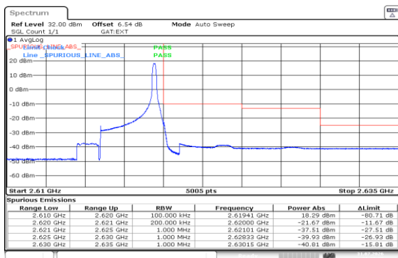
Band38-10MHz-QPSK-38200-1RB#49-PASS
