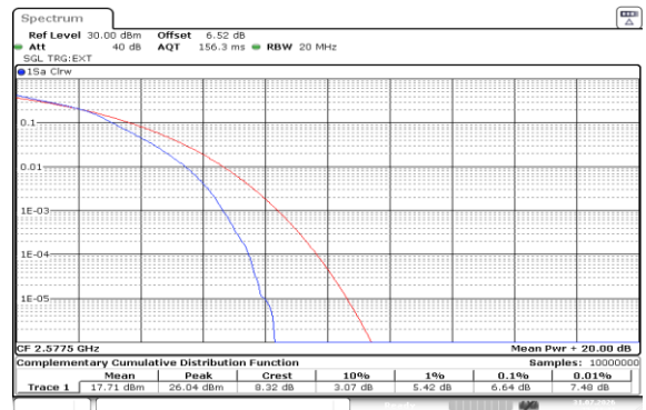
Band38-15MHz-16QAM-37825-75RB#0-PASS
