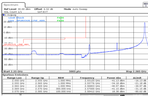
Band38-15MHz-QPSK-37825-1RB#74-PASS
