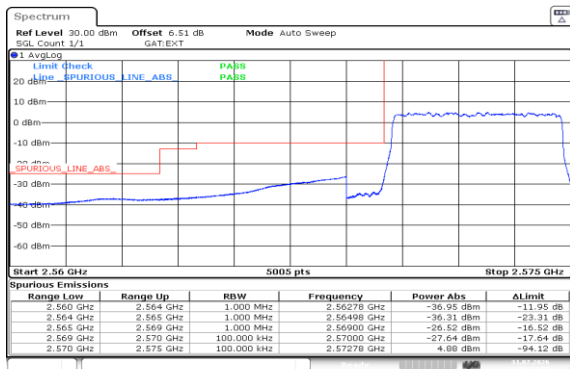
Band38-5MHz-QPSK-37775-25RB#0-PASS
