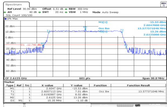
Band38-15MHz-16QAM-38175-75RB#0-PASS
