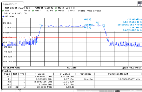
Band38-20MHz-QPSK-38000-100RB#0-PASS
