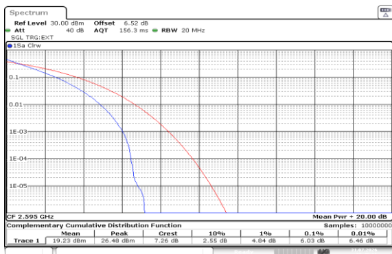
Band38-15MHz-QPSK-38000-75RB#0-PASS
