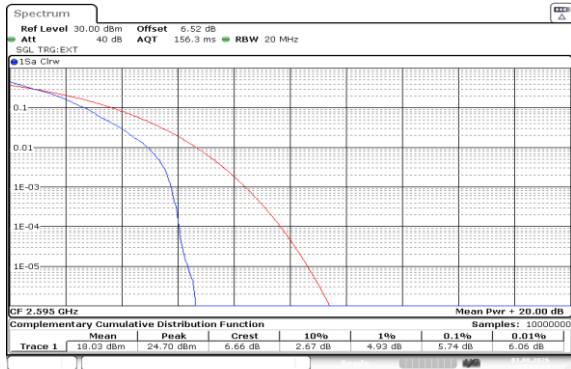
Band38-20MHz-QPSK-38000-1RB#0-PASS
