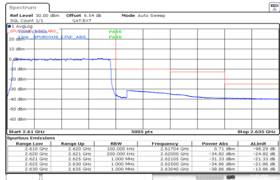
Band38-10MHz-16QAM-38200-50RB#0-PASS
