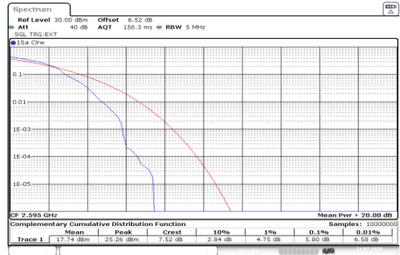
Band38-5MHz-16QAM-38000-1RB#0-PASS
