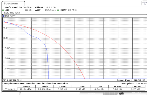
Band38-15MHz-QPSK-37825-1RB#0-PASS
