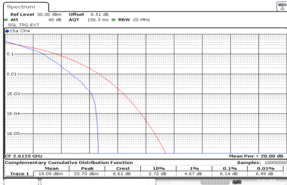
Band38-15MHz-QPSK-38175-1RB#0-PASS
