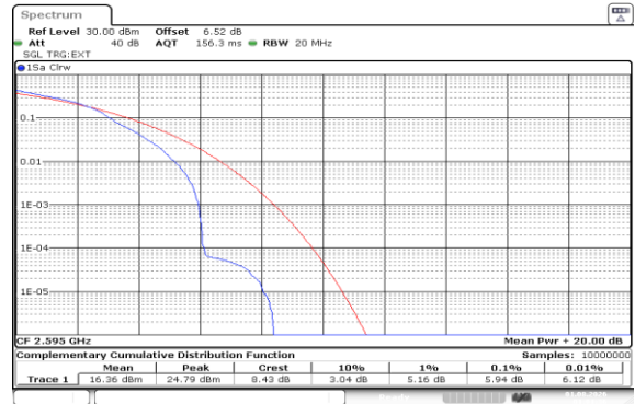
Band38-20MHz-16QAM-38000-1RB#0-PASS
