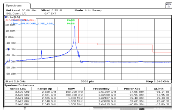
Band38-20MHz-16QAM-38150-1RB#99-PASS
