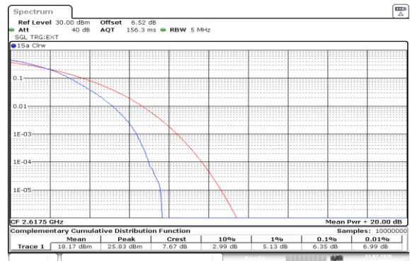
Band38-5MHz-16QAM-38225-25RB#0-PASS
