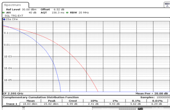
Band38-20MHz-QPSK-38000-100RB#0-PASS
