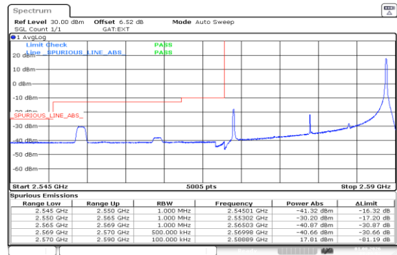
Band38-20MHz-16QAM-37850-1RB#99-PASS
