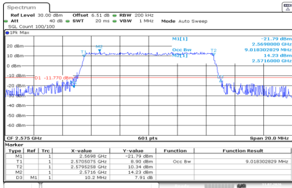
Band38-10MHz-QPSK-37800-50RB#0-PASS
