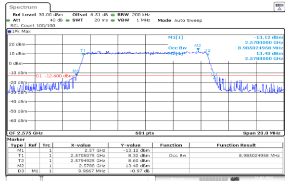
Band38-10MHz-16QAM-37800-50RB#0-PASS
