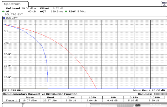
Band38-5MHz-QPSK-38000-1RB#0-PASS
