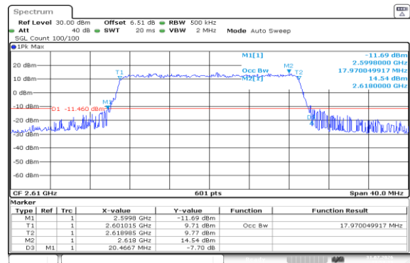
Band38-20MHz-16QAM-38150-100RB#0-PASS
