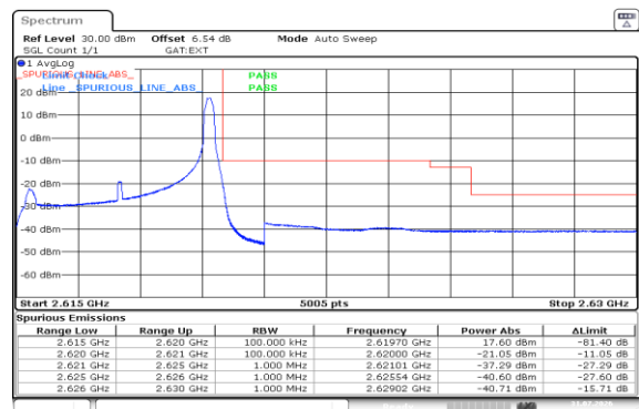
Band38-5MHz-16QAM-38225-1RB#24-PASS
