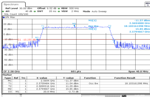
Band38-20MHz-QPSK-37850-100RB#0-PASS
