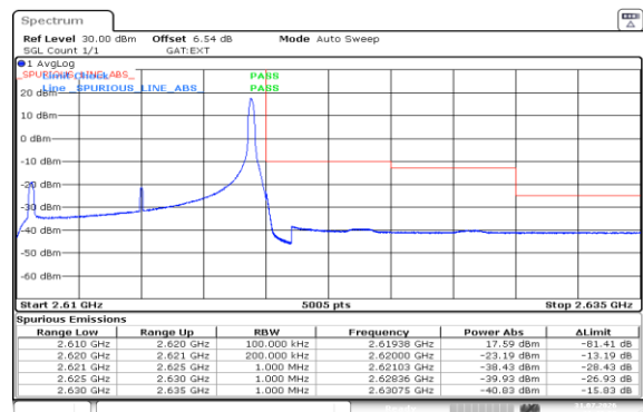
Band38-10MHz-16QAM-38200-1RB#49-PASS
