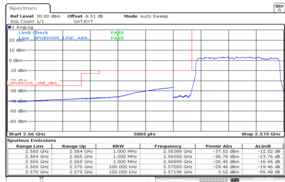
Band38-5MHz-16QAM-37775-25RB#0-PASS
