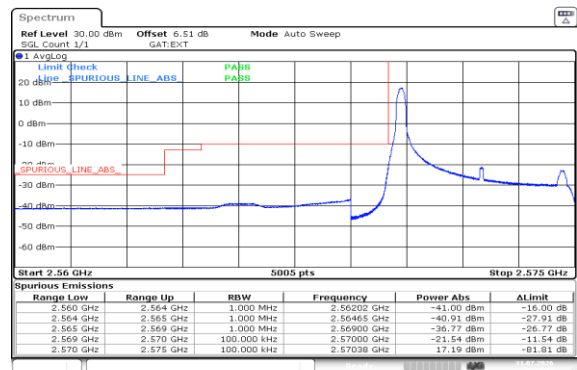
Band38-5MHz-16QAM-37775-1RB#0-PASS
