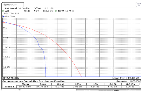
Band38-10MHz-QPSK-37800-1RB#0-PASS
