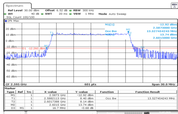
Band38-15MHz-16QAM-38000-75RB#0-PASS
