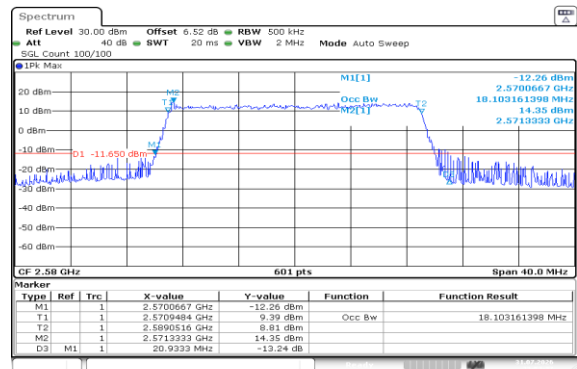
Band38-20MHz-16QAM-37850-100RB#0-PASS
