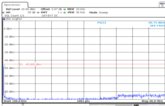
Band38-5MHz-16QAM-38225-25RB#0-0.15~30-PASS
