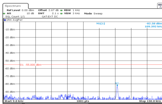
Band38-5MHz-16QAM-37775-1RB#24-0.009~0.15-PASS
