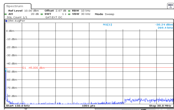
Band38-5MHz-QPSK-38000-1RB#24-0.15~30-PASS
