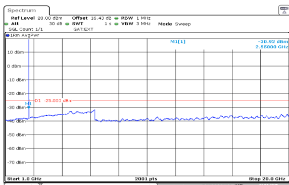
Band38-5MHz-16QAM-37775-25RB#0-1000~20000-PASS
