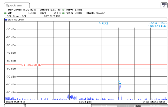
Band38-10MHz-16QAM-37800-50RB#0-0.009~0.15-PASS
