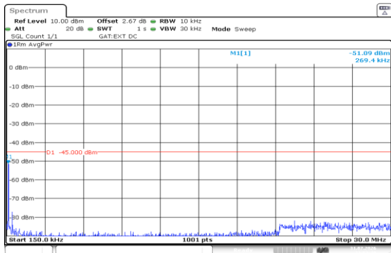
Band38-10MHz-16QAM-37800-50RB#0-0.15~30-PASS
