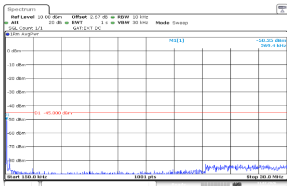
Band38-5MHz-16QAM-38225-1RB#0-0.15~30-PASS
