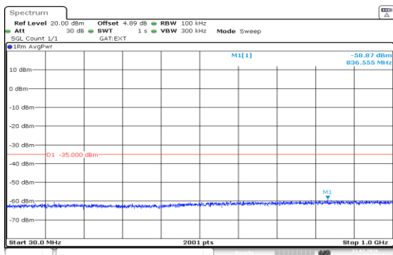
Band38-10MHz-QPSK-38200-1RB#49-30~1000-PASS
