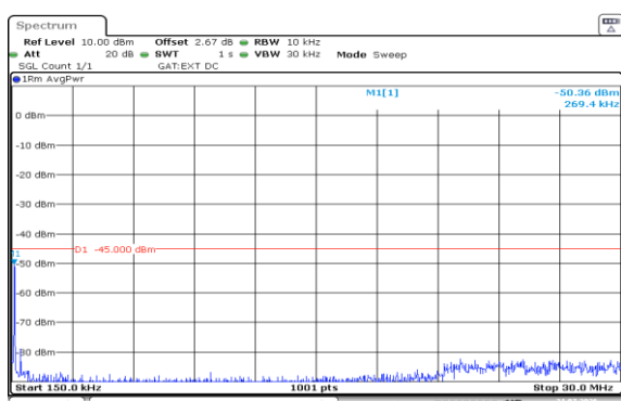
Band38-5MHz-16QAM-37775-1RB#24-0.15~30-PASS
