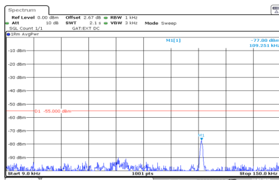
Band38-10MHz-16QAM-38200-1RB#0-0.009~0.15-PASS
