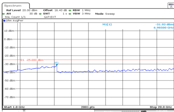
Band38-5MHz-16QAM-38225-25RB#0-1000~20000-PASS
