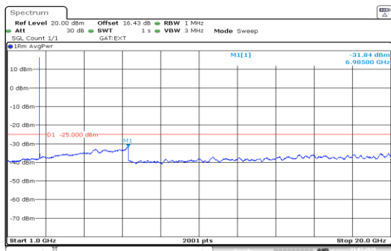
Band38-5MHz-16QAM-38000-25RB#0-1000~20000-PASS
