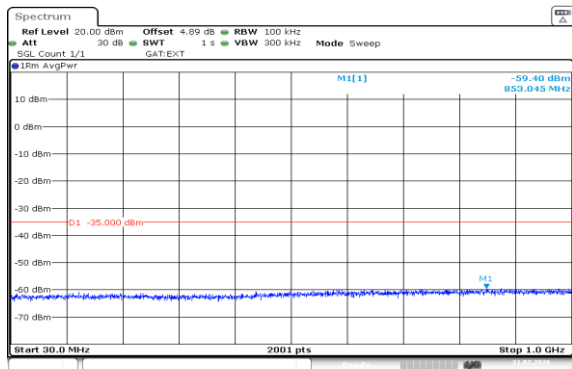
Band38-5MHz-QPSK-38225-1RB#0-30~1000-PASS
