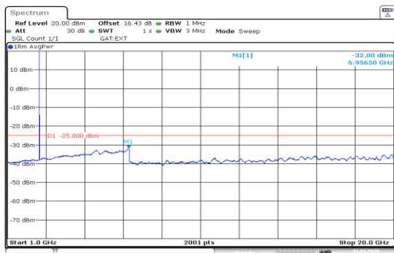
Band38-5MHz-16QAM-37775-1RB#24-1000~20000-PASS
