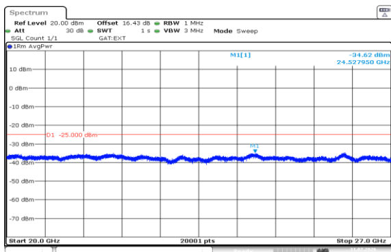
Band38-10MHz-QPSK-38000-50RB#0-20000~27000-PASS
