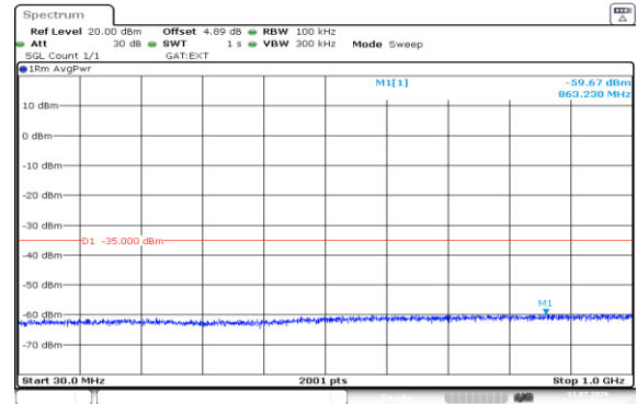
Band38-5MHz-16QAM-38225-1RB#24-30~1000-PASS
