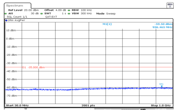
Band38-10MHz-16QAM-37800-1RB#49-30~1000-PASS
