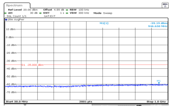
Band38-10MHz-16QAM-38000-50RB#0-30~1000-PASS
