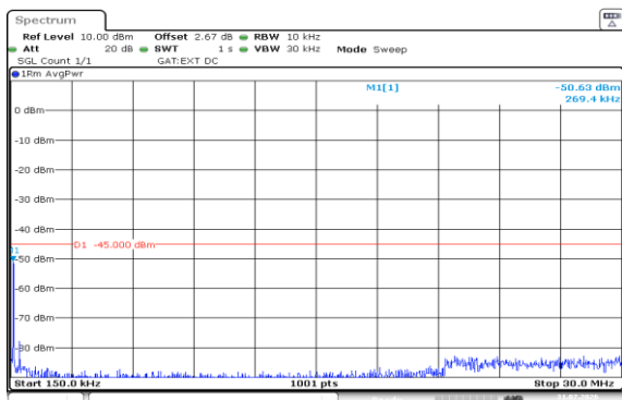
Band38-10MHz-16QAM-38000-50RB#0-0.15~30-PASS
