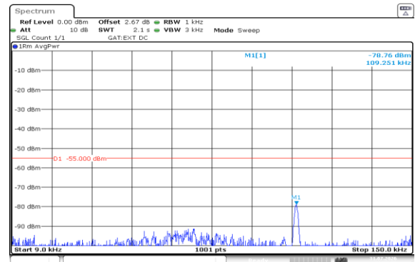
Band38-10MHz-16QAM-38000-1RB#0-0.009~0.15-PASS
