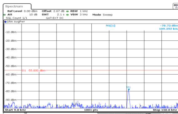
Band38-10MHz-16QAM-38000-1RB#49-0.009~0.15-PASS
