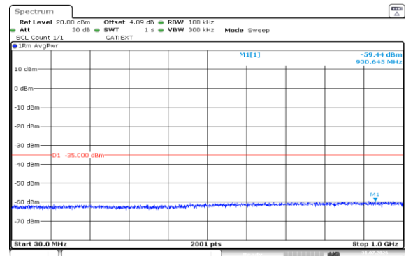
Band38-5MHz-16QAM-38225-25RB#0-30~1000-PASS
