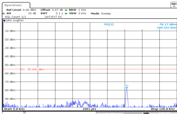
Band38-10MHz-QPSK-38000-1RB#0-0.009~0.15-PASS
