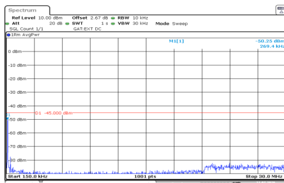
Band38-5MHz-QPSK-38000-1RB#0-0.15~30-PASS
