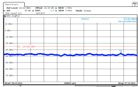
Band38-5MHz-16QAM-38000-1RB#24-20000~27000-PASS
