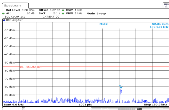
Band38-5MHz-QPSK-37775-1RB#24-0.009~0.15-PASS
