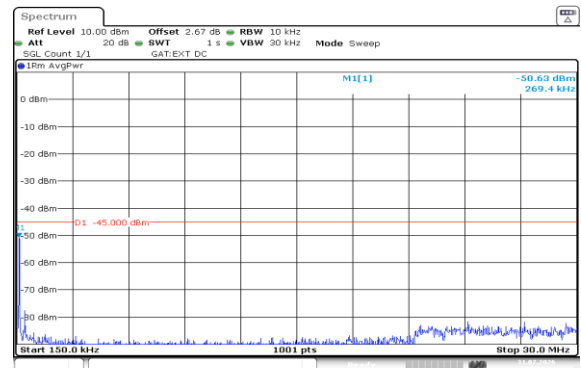
Band38-10MHz-QPSK-37800-1RB#0-0.15~30-PASS
