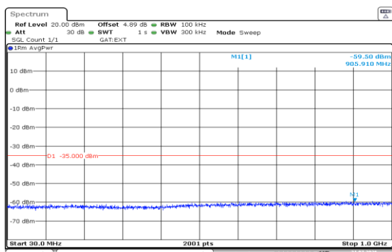
Band38-5MHz-QPSK-38000-25RB#0-30~1000-PASS
