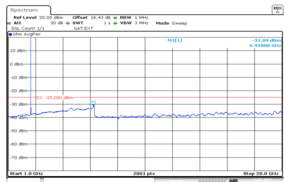
Band38-5MHz-QPSK-37775-1RB#0-1000~20000-PASS
