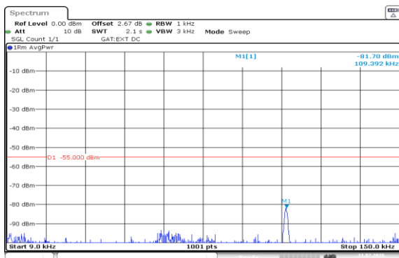
Band38-5MHz-QPSK-38225-25RB#0-0.009~0.15-PASS
