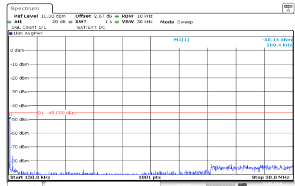
Band38-10MHz-QPSK-37800-50RB#0-0.15~30-PASS
