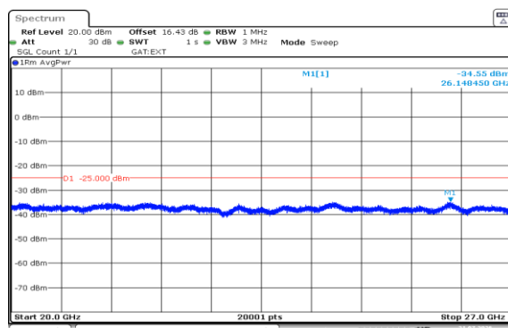
Band38-10MHz-16QAM-38000-50RB#0-20000~27000-PASS
