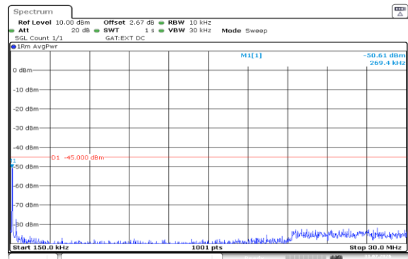
Band38-10MHz-QPSK-38000-1RB#0-0.15~30-PASS
