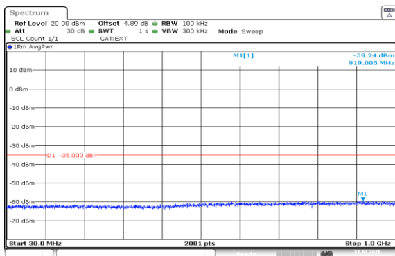
Band38-5MHz-QPSK-38225-25RB#0-30~1000-PASS
