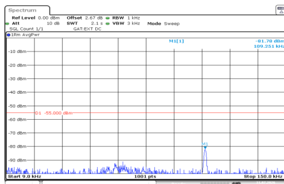
Band38-5MHz-16QAM-38225-1RB#24-0.009~0.15-PASS
