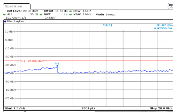
Band38-5MHz-QPSK-37775-1RB#24-1000~20000-PASS
