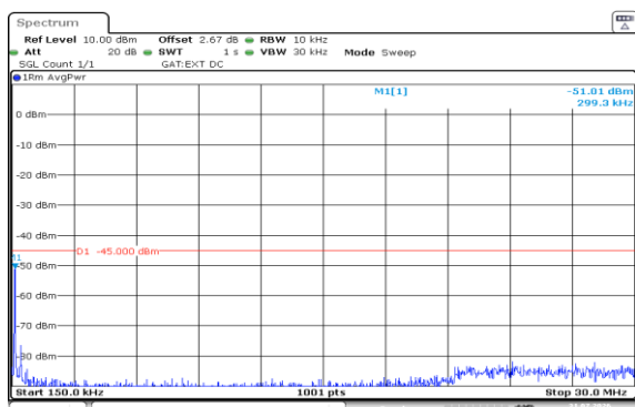
Band38-10MHz-16QAM-38200-1RB#49-0.15~30-PASS
