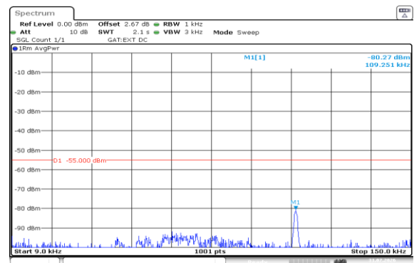
Band38-5MHz-16QAM-38225-1RB#0-0.009~0.15-PASS
