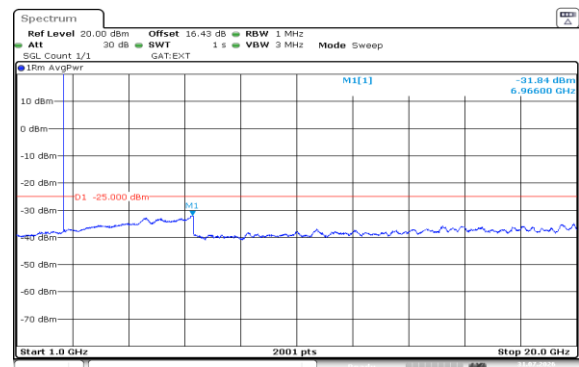
Band38-5MHz-QPSK-38000-1RB#24-1000~20000-PASS
