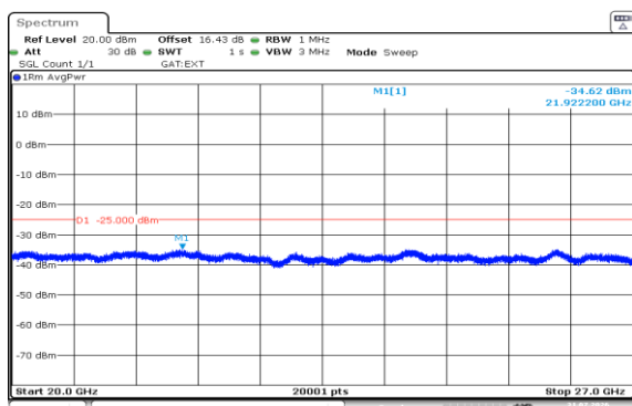
Band38-10MHz-QPSK-38000-1RB#49-20000~27000-PASS
