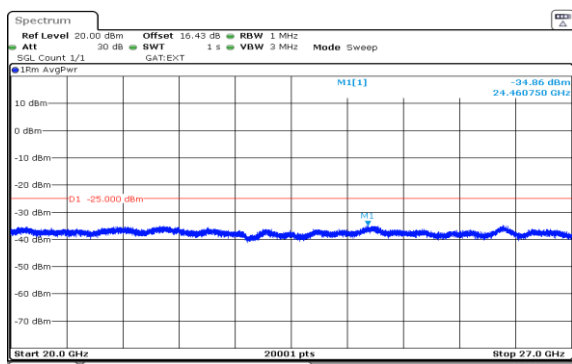
Band38-5MHz-QPSK-37775-1RB#24-20000~27000-PASS
