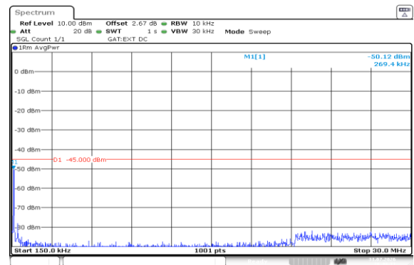
Band38-5MHz-QPSK-37775-1RB#0-0.15~30-PASS
