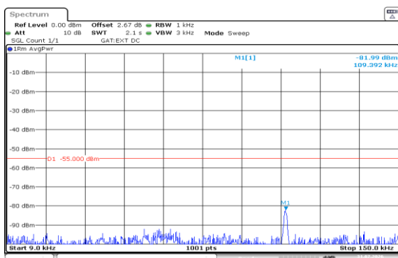
Band38-5MHz-QPSK-38000-1RB#24-0.009~0.15-PASS
