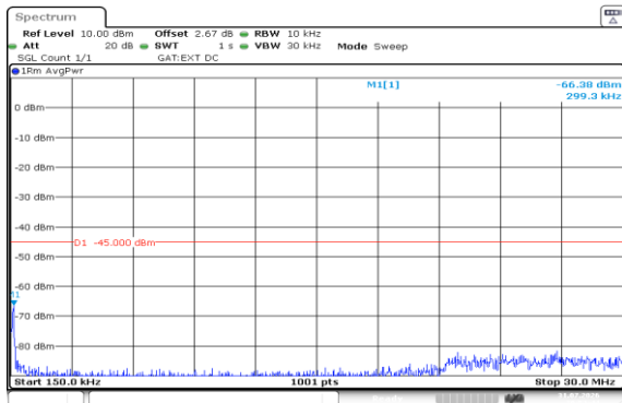
Band38-5MHz-16QAM-38000-1RB#0-0.15~30-PASS
