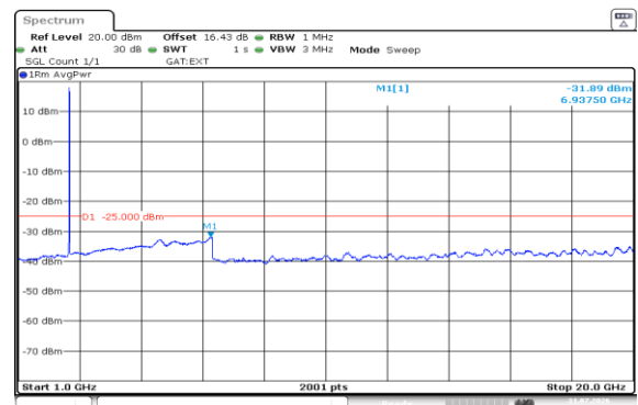
Band38-10MHz-QPSK-37800-50RB#0-1000~20000-PASS
