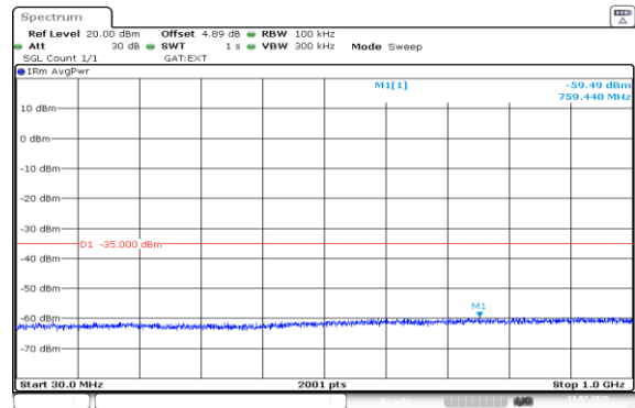
Band38-10MHz-16QAM-38200-1RB#0-30~1000-PASS
