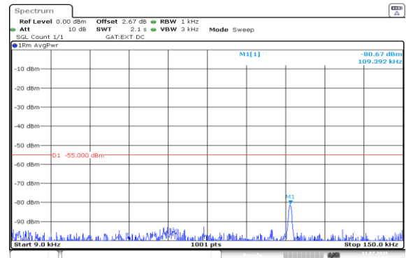
Band38-5MHz-16QAM-38000-1RB#24-0.009~0.15-PASS
