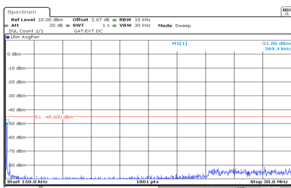
Band38-10MHz-16QAM-37800-1RB#0-0.15~30-PASS
