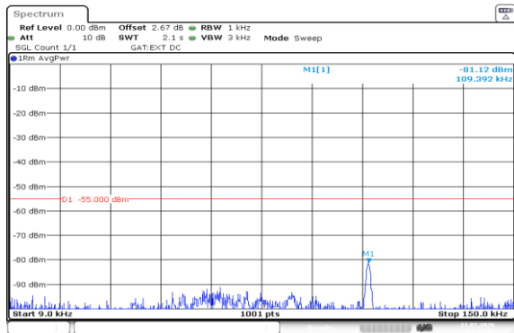
Band38-5MHz-QPSK-38225-1RB#0-0.009~0.15-PASS
