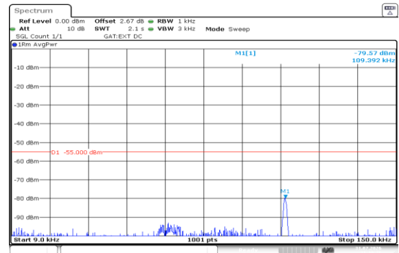
Band38-5MHz-16QAM-38225-25RB#0-0.009~0.15-PASS
