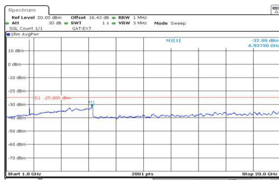
Band38-5MHz-QPSK-38000-25RB#0-1000~20000-PASS
