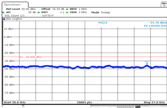
Band38-5MHz-QPSK-37775-1RB#0-20000~27000-PASS
