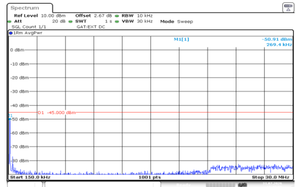
Band38-10MHz-QPSK-37800-1RB#49-0.15~30-PASS
