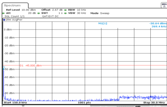
Band38-5MHz-16QAM-37775-25RB#0-0.15~30-PASS
