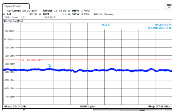
Band38-5MHz-QPSK-38225-1RB#24-20000~27000-PASS
