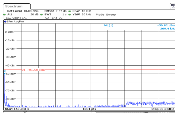
Band38-10MHz-QPSK-38200-1RB#0-0.15~30-PASS
