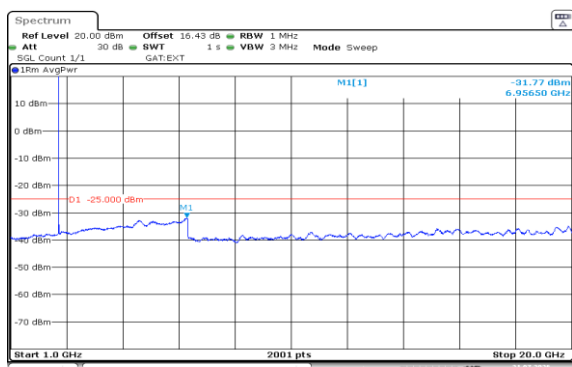
Band38-5MHz-16QAM-38225-1RB#0-1000~20000-PASS
