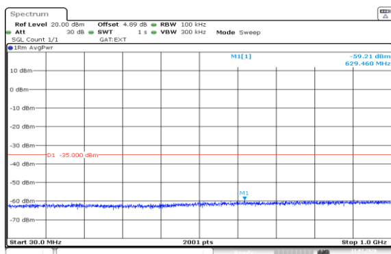
Band38-5MHz-QPSK-37775-1RB#0-30~1000-PASS
