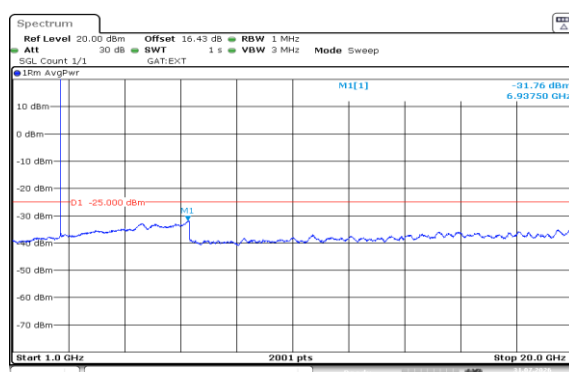
Band38-5MHz-QPSK-38225-1RB#24-1000~20000-PASS
