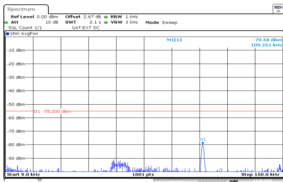
Band38-10MHz-QPSK-38200-50RB#0-0.009~0.15-PASS
