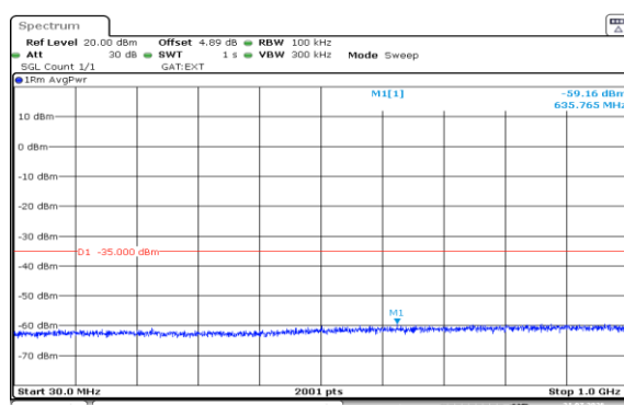
Band38-10MHz-16QAM-37800-1RB#0-30~1000-PASS
