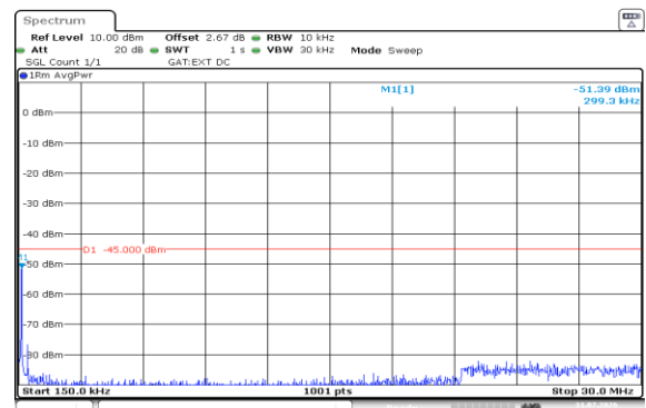
Band38-10MHz-QPSK-38000-1RB#49-0.15~30-PASS
