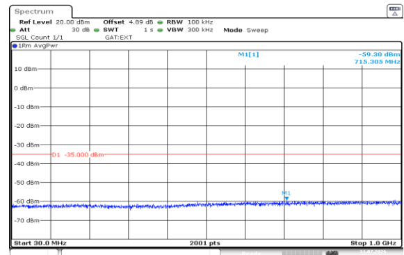
Band38-5MHz-16QAM-38000-1RB#24-30~1000-PASS
