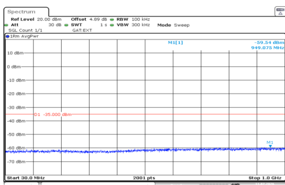
Band38-10MHz-QPSK-38200-1RB#0-30~1000-PASS
