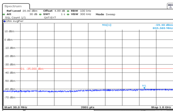
Band38-10MHz-QPSK-38000-1RB#49-30~1000-PASS
