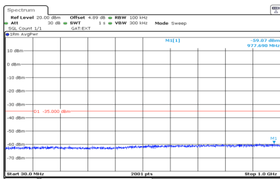
Band38-10MHz-QPSK-37800-1RB#0-30~1000-PASS
