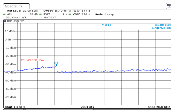
Band38-10MHz-QPSK-37800-1RB#0-1000~20000-PASS
