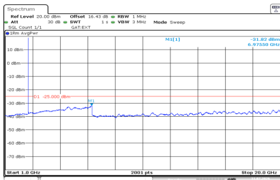
Band38-10MHz-16QAM-38000-1RB#49-1000~20000-PASS
