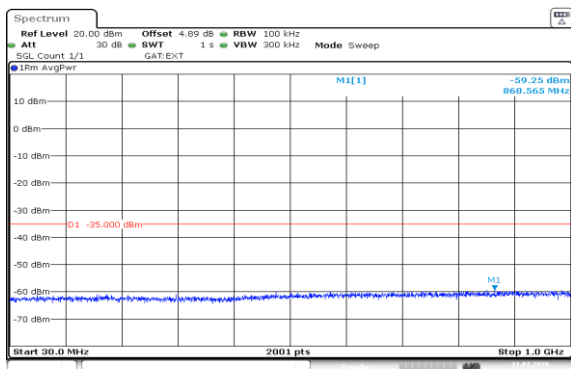
Band38-5MHz-QPSK-37775-25RB#0-30~1000-PASS
