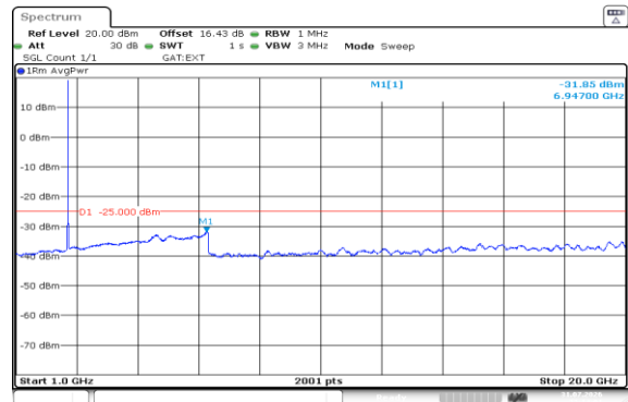
Band38-10MHz-QPSK-38200-50RB#0-1000~20000-PASS
