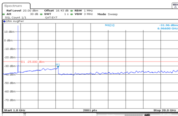
Band38-10MHz-16QAM-38200-50RB#0-1000~20000-PASS
