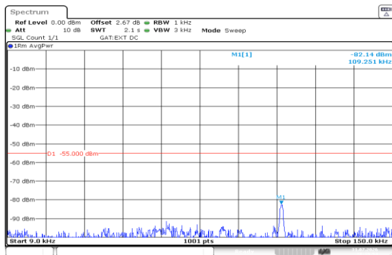
Band38-5MHz-QPSK-37775-1RB#0-0.009~0.15-PASS
