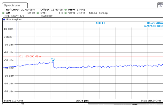
Band38-5MHz-16QAM-38000-1RB#0-1000~20000-PASS
