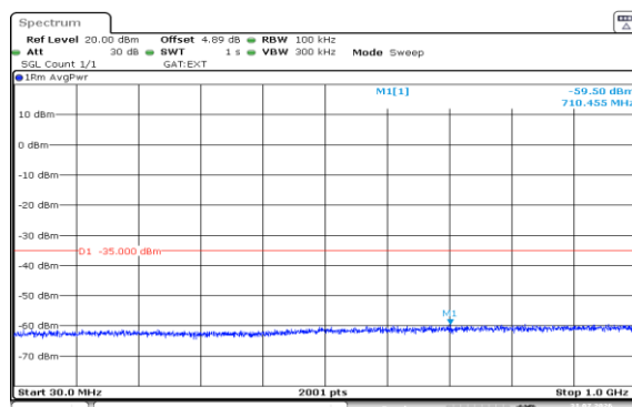
Band38-10MHz-16QAM-38200-1RB#49-30~1000-PASS
