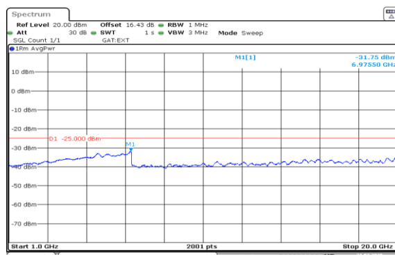
Band38-10MHz-QPSK-38000-1RB#49-1000~20000-PASS
