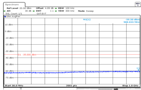
Band38-5MHz-16QAM-38225-1RB#0-30~1000-PASS
