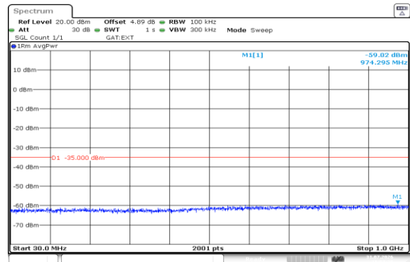
Band38-10MHz-16QAM-37800-50RB#0-30~1000-PASS
