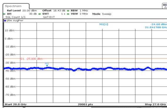
Band38-5MHz-16QAM-37775-25RB#0-20000~27000-PASS
