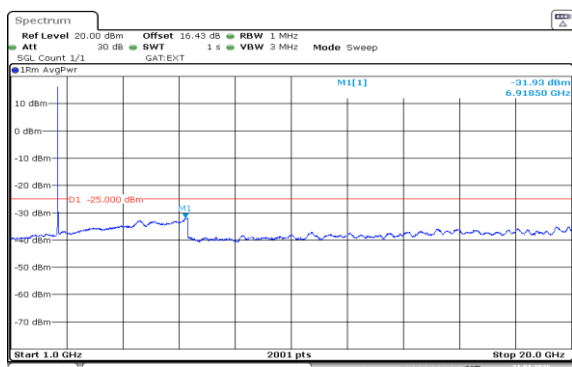
Band38-10MHz-16QAM-38000-50RB#0-1000~20000-PASS
