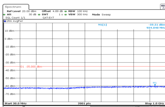
Band38-5MHz-16QAM-38000-25RB#0-30~1000-PASS
