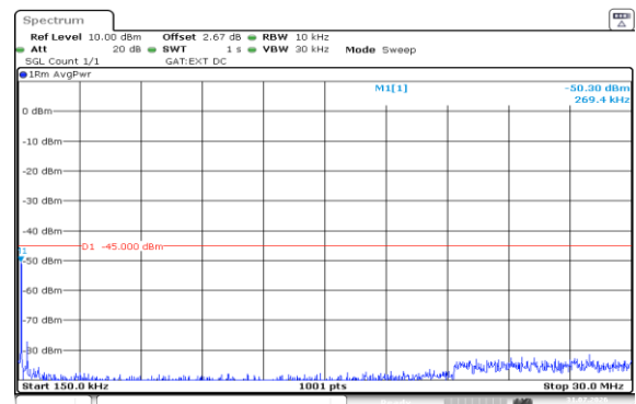
Band38-5MHz-QPSK-38225-25RB#0-0.15~30-PASS
