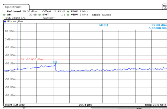
Band38-10MHz-QPSK-38200-1RB#0-1000~20000-PASS
