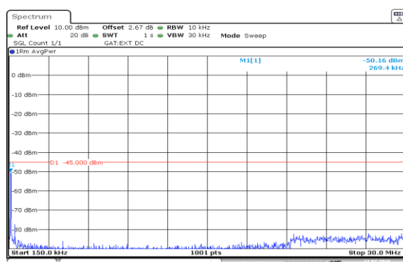
Band38-5MHz-QPSK-38225-1RB#24-0.15~30-PASS
