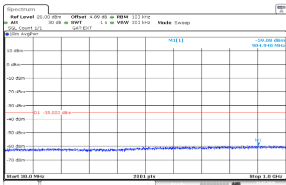
Band38-10MHz-QPSK-37800-1RB#49-30~1000-PASS
