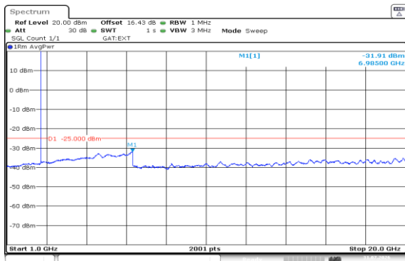
Band38-5MHz-16QAM-38225-1RB#24-1000~20000-PASS
