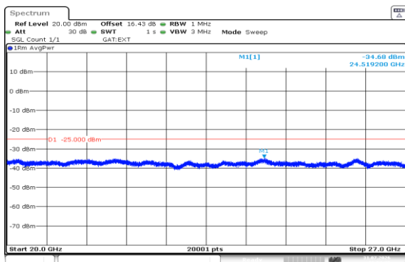
Band38-10MHz-QPSK-37800-50RB#0-20000~27000-PASS
