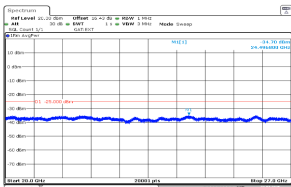
Band38-10MHz-QPSK-38200-1RB#49-20000~27000-PASS
