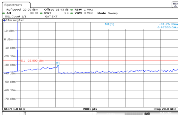
Band38-10MHz-16QAM-37800-1RB#49-1000~20000-PASS
