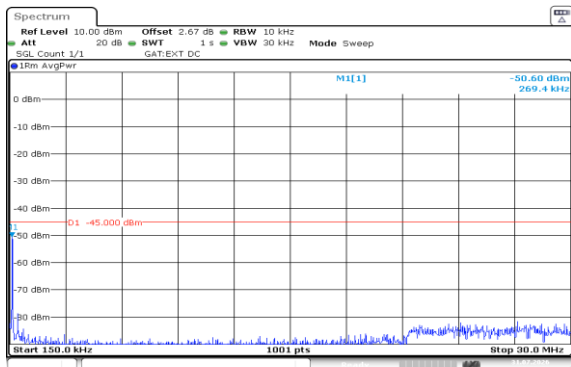
Band38-5MHz-16QAM-38000-1RB#24-0.15~30-PASS
