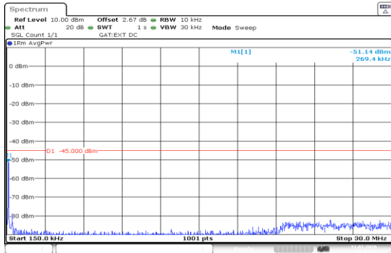
Band38-5MHz-16QAM-38225-1RB#24-0.15~30-PASS
