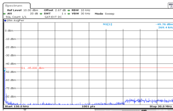
Band38-10MHz-QPSK-38200-50RB#0-0.15~30-PASS
