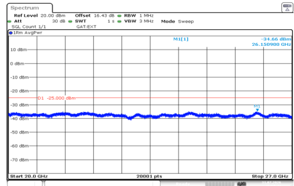
Band38-10MHz-16QAM-37800-1RB#49-20000~27000-PASS
