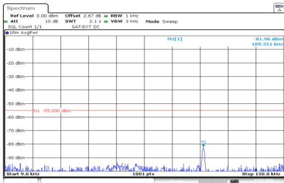
Band38-10MHz-QPSK-37800-1RB#0-0.009~0.15-PASS
