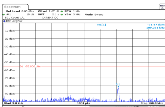
Band38-5MHz-QPSK-38225-1RB#24-0.009~0.15-PASS
