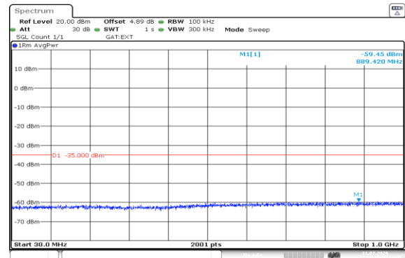
Band38-5MHz-16QAM-38000-1RB#0-30~1000-PASS
