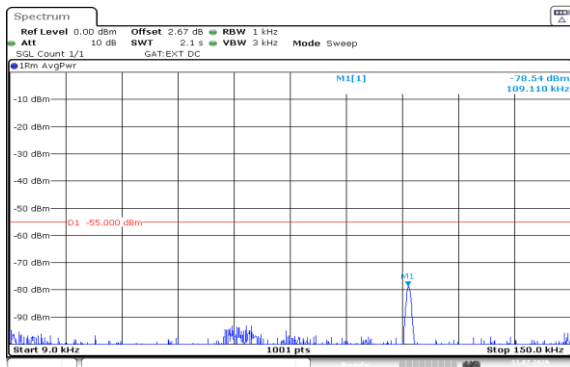
Band38-10MHz-QPSK-37800-50RB#0-0.009~0.15-PASS
