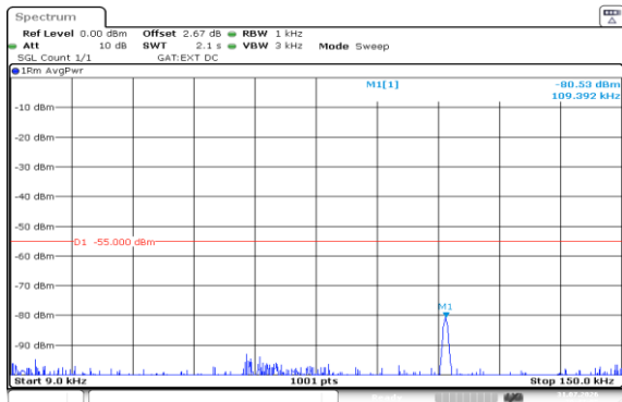
Band38-5MHz-QPSK-37775-25RB#0-0.009~0.15-PASS
