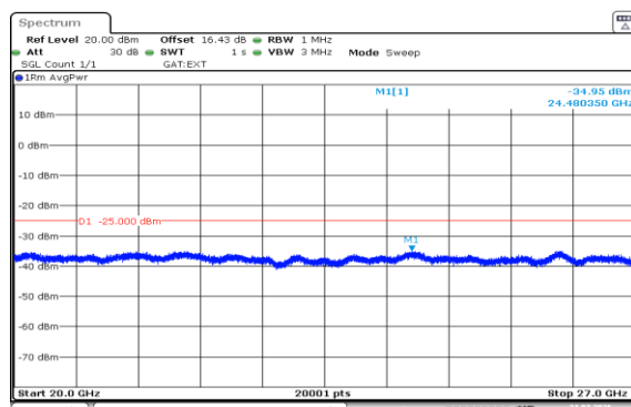
Band38-5MHz-16QAM-38225-1RB#0-20000~27000-PASS
