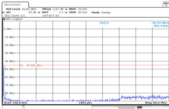
Band38-10MHz-16QAM-38200-1RB#0-0.15~30-PASS
