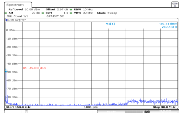
Band38-5MHz-QPSK-37775-25RB#0-0.15~30-PASS
