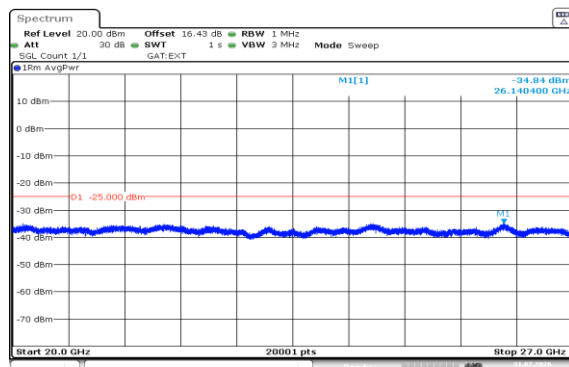
Band38-10MHz-16QAM-38000-1RB#49-20000~27000-PASS
