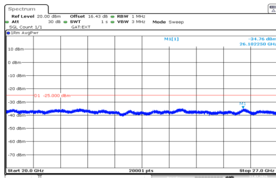
Band38-5MHz-16QAM-38000-25RB#0-20000~27000-PASS
