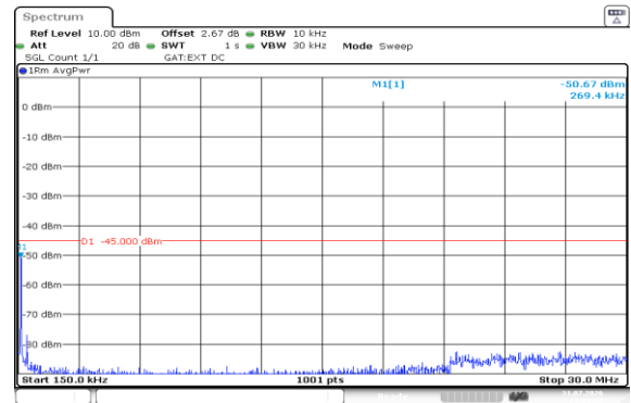
Band38-5MHz-QPSK-38225-1RB#0-0.15~30-PASS
