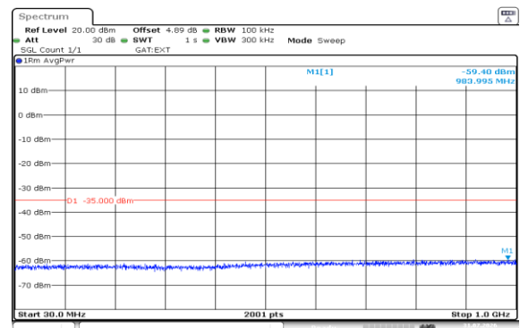
Band38-5MHz-16QAM-37775-25RB#0-30~1000-PASS
