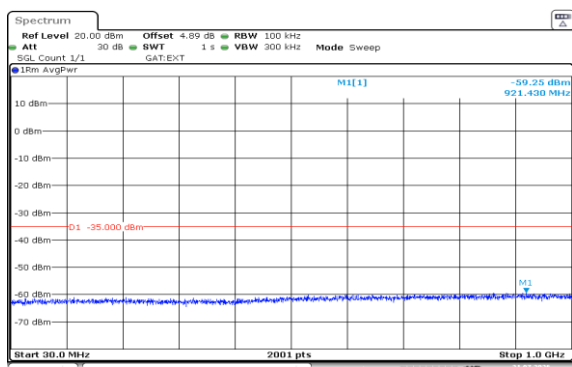
Band38-5MHz-QPSK-37775-1RB#24-30~1000-PASS
