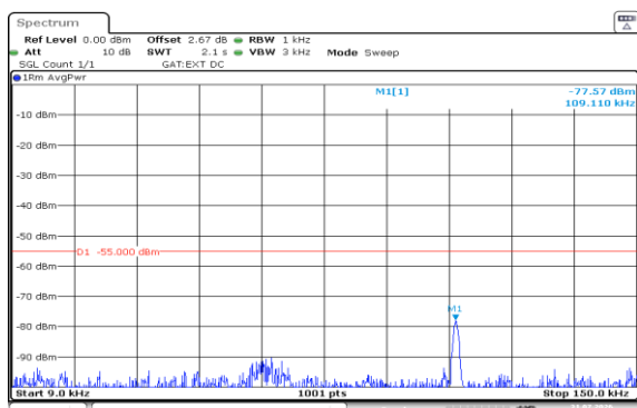
Band38-10MHz-QPSK-38200-1RB#0-0.009~0.15-PASS
