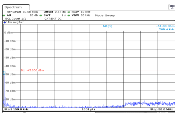
Band38-5MHz-16QAM-38000-25RB#0-0.15~30-PASS
