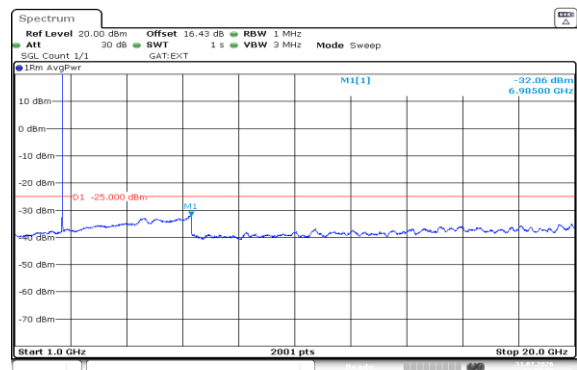
Band38-10MHz-QPSK-38200-1RB#49-1000~20000-PASS
