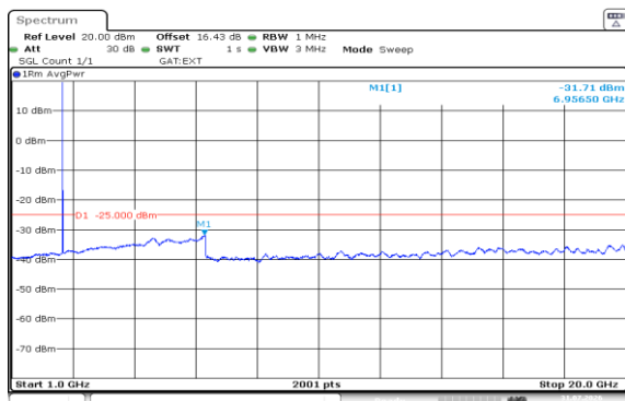
Band38-10MHz-16QAM-37800-1RB#0-1000~20000-PASS
