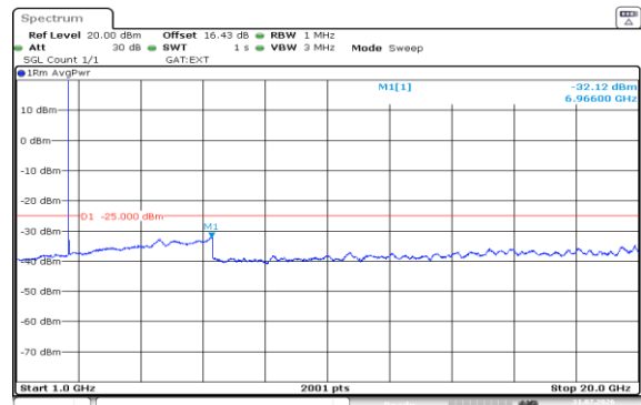
Band38-10MHz-QPSK-38000-1RB#0-1000~20000-PASS
