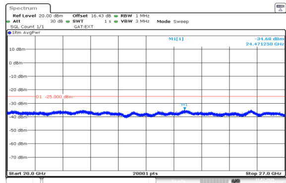
Band38-10MHz-16QAM-38200-1RB#0-20000~27000-PASS
