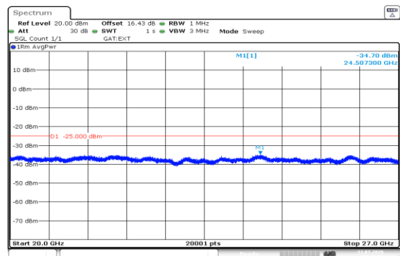
Band38-10MHz-16QAM-38200-50RB#0-20000~27000-PASS
