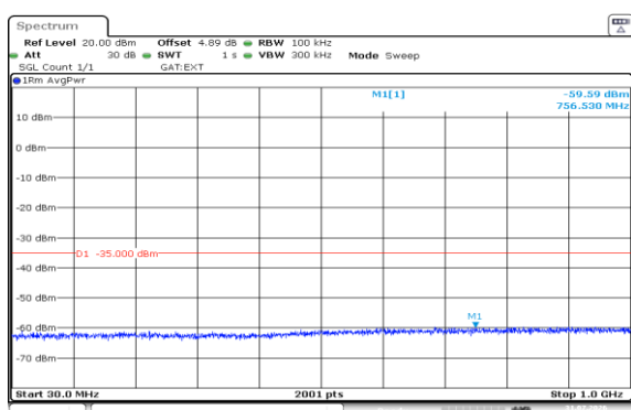
Band38-5MHz-QPSK-38225-1RB#24-30~1000-PASS
