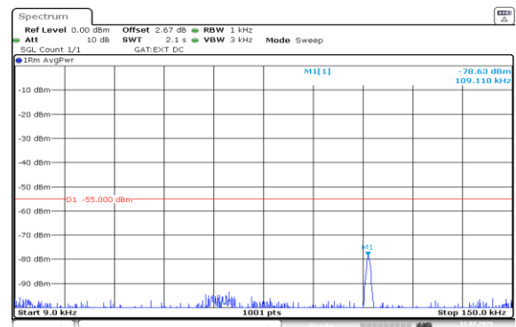
Band38-10MHz-16QAM-38000-50RB#0-0.009~0.15-PASS
