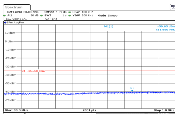
Band38-5MHz-16QAM-37775-1RB#24-30~1000-PASS
