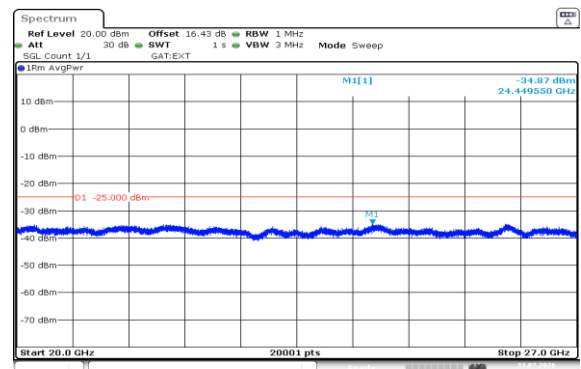
Band38-5MHz-16QAM-38225-25RB#0-20000~27000-PASS
