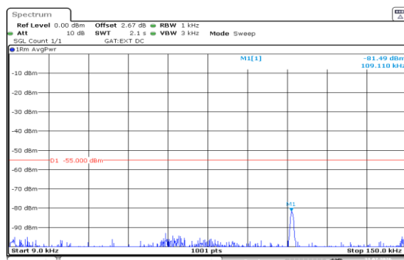
Band38-5MHz-16QAM-38000-25RB#0-0.009~0.15-PASS
