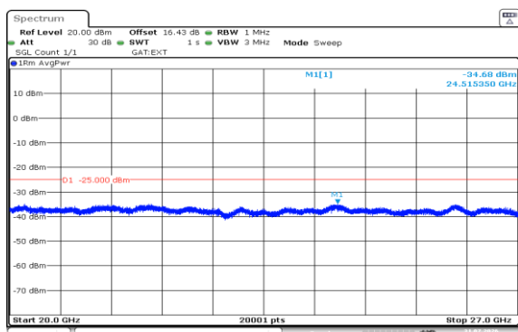
Band38-10MHz-QPSK-38200-1RB#0-20000~27000-PASS
