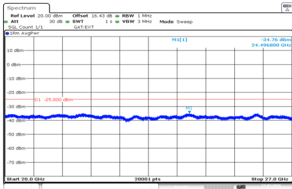
Band38-5MHz-QPSK-38000-1RB#24-20000~27000-PASS
