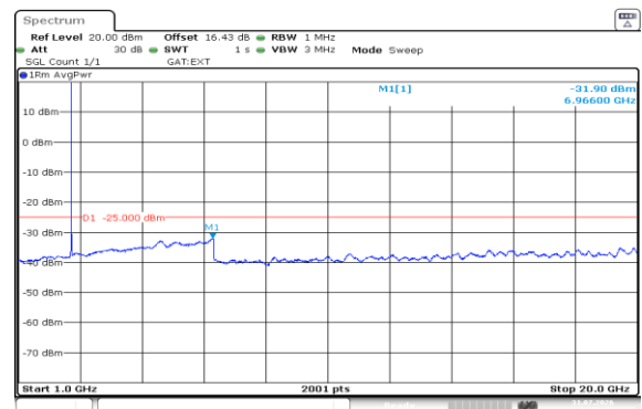
Band38-5MHz-QPSK-38225-25RB#0-1000~20000-PASS
