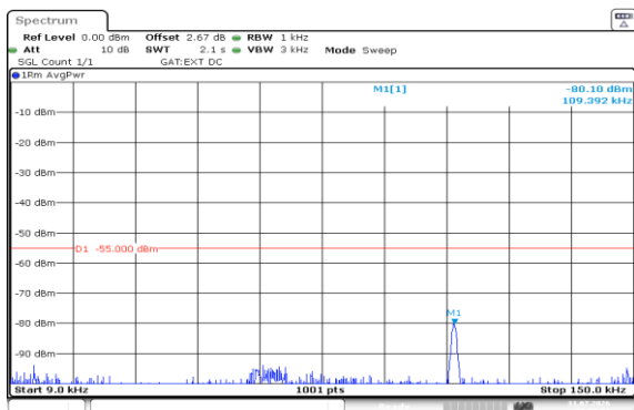
Band38-5MHz-QPSK-38000-25RB#0-0.009~0.15-PASS
