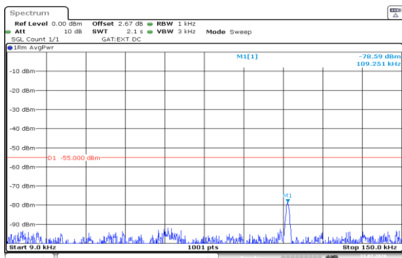
Band38-10MHz-QPSK-38000-1RB#49-0.009~0.15-PASS
