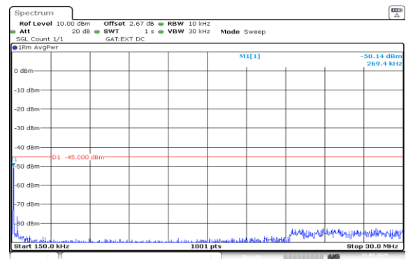
Band38-5MHz-QPSK-37775-1RB#24-0.15~30-PASS
