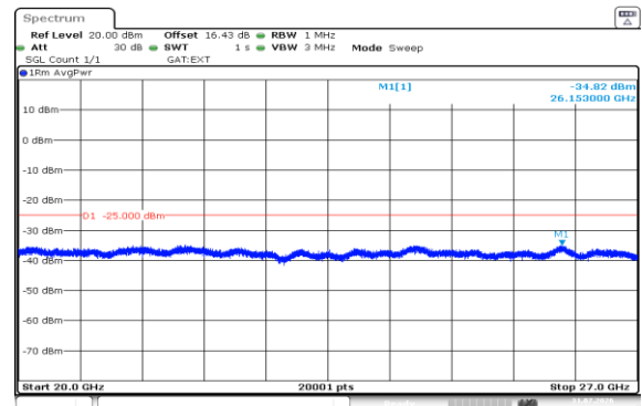
Band38-5MHz-16QAM-38225-1RB#24-20000~27000-PASS
