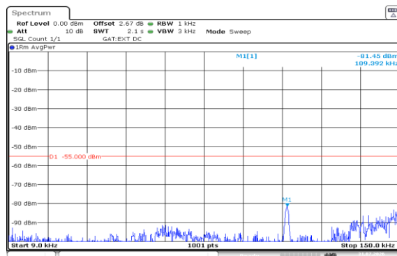
Band38-5MHz-16QAM-38000-1RB#0-0.009~0.15-PASS
