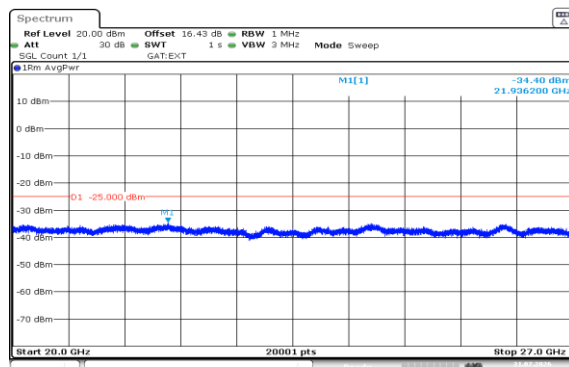
Band38-10MHz-16QAM-37800-1RB#0-20000~27000-PASS
