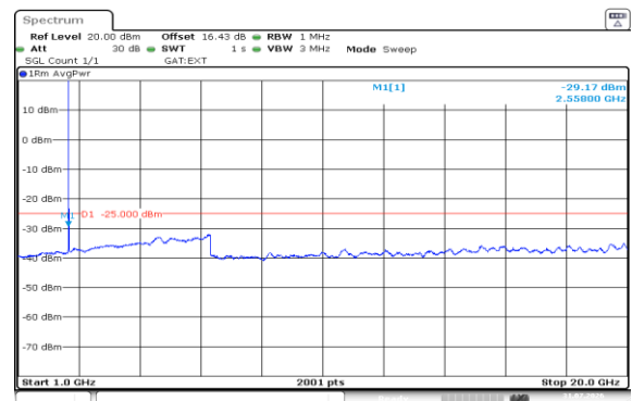
Band38-5MHz-QPSK-37775-25RB#0-1000~20000-PASS
