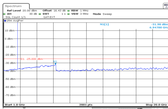
Band38-5MHz-QPSK-38000-1RB#0-1000~20000-PASS
