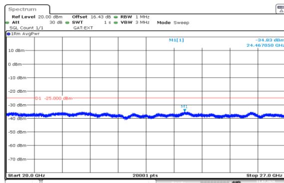
Band38-5MHz-16QAM-37775-1RB#24-20000~27000-PASS
