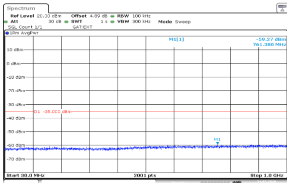
Band38-10MHz-QPSK-38000-1RB#0-30~1000-PASS
