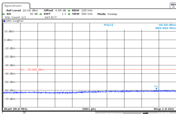
Band38-10MHz-QPSK-37800-50RB#0-30~1000-PASS
