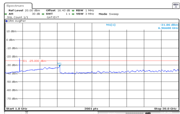
Band38-10MHz-QPSK-37800-1RB#49-1000~20000-PASS
