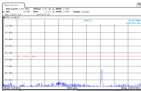
Band38-10MHz-16QAM-38200-1RB#49-0.009~0.15-PASS
