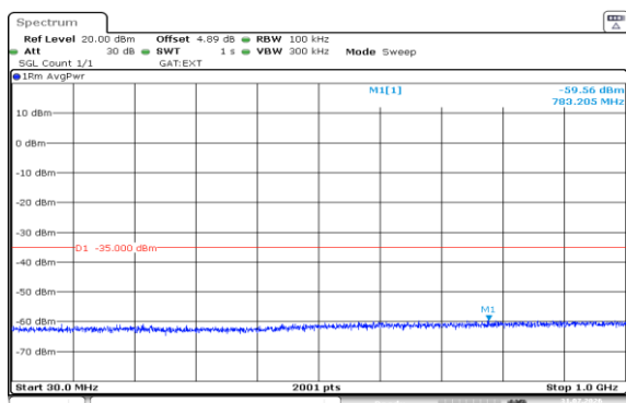
Band38-5MHz-QPSK-38000-1RB#0-30~1000-PASS
