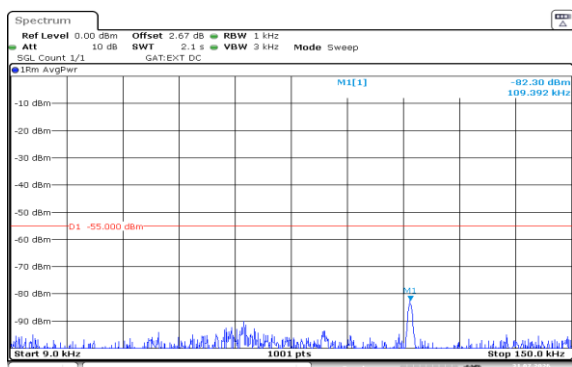
Band38-5MHz-QPSK-38000-1RB#0-0.009~0.15-PASS
