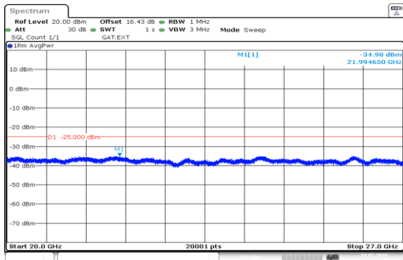
Band38-5MHz-QPSK-38225-25RB#0-20000~27000-PASS
