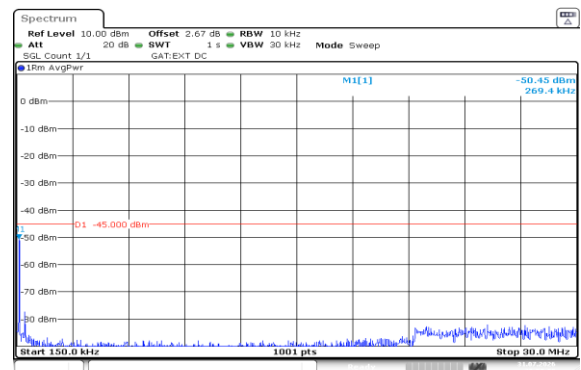
Band38-5MHz-QPSK-38000-25RB#0-0.15~30-PASS
