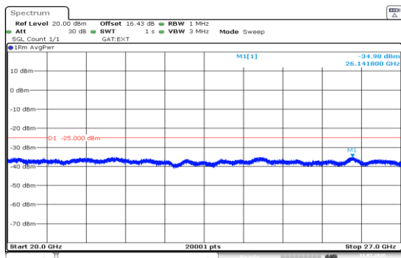
Band38-5MHz-QPSK-38225-1RB#0-20000~27000-PASS
