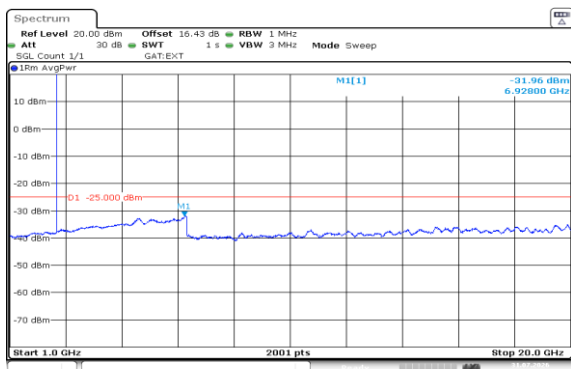
Band38-5MHz-16QAM-38000-1RB#24-1000~20000-PASS
