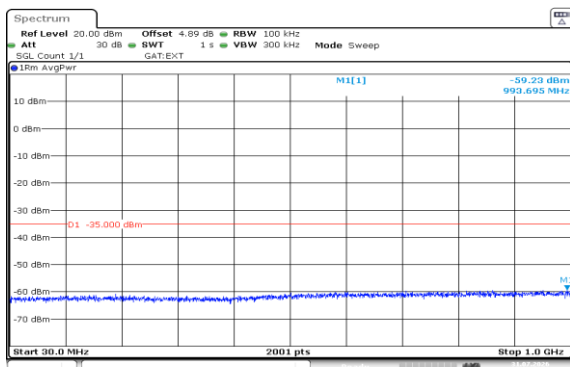
Band38-5MHz-QPSK-38000-1RB#24-30~1000-PASS
