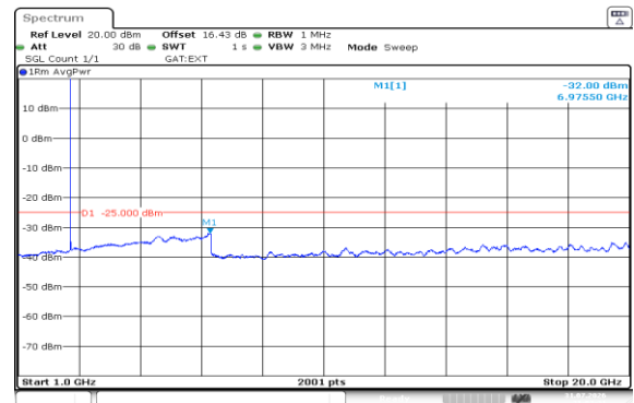
Band38-5MHz-QPSK-38225-1RB#0-1000~20000-PASS
