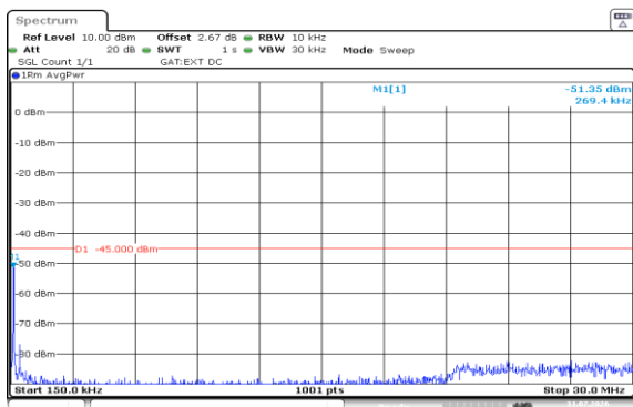
Band38-10MHz-16QAM-37800-1RB#49-0.15~30-PASS
