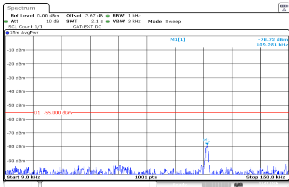
Band38-10MHz-QPSK-37800-1RB#49-0.009~0.15-PASS
