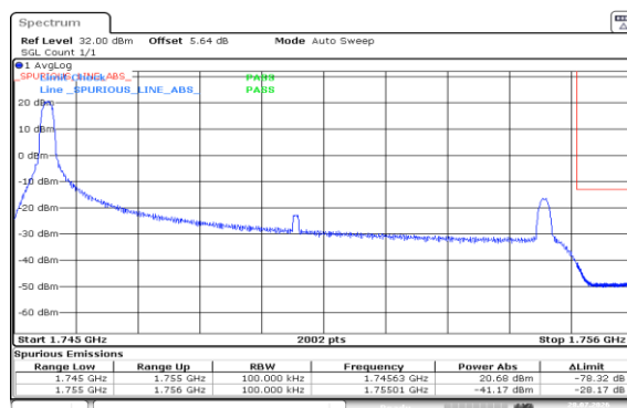
Band4-10MHz-16QAM-20350-1RB#0-PASS
