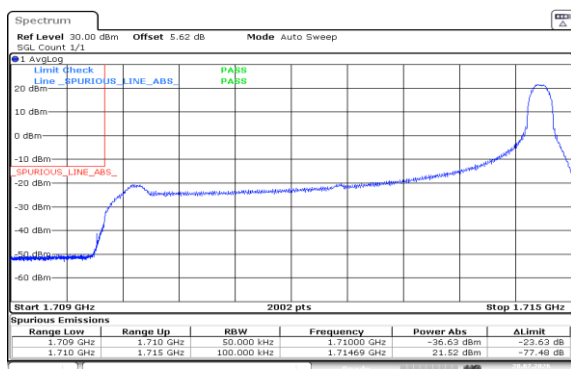
Band4-5MHz-QPSK-19975-1RB#24-PASS
