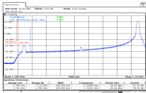
Band4-10MHz-16QAM-20000-1RB#49-PASS
