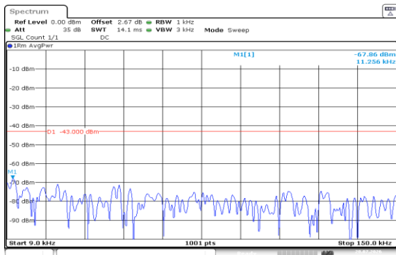
Band4-1.4MHz-16QAM-19957-1RB#0-0.009~0.15-PASS
