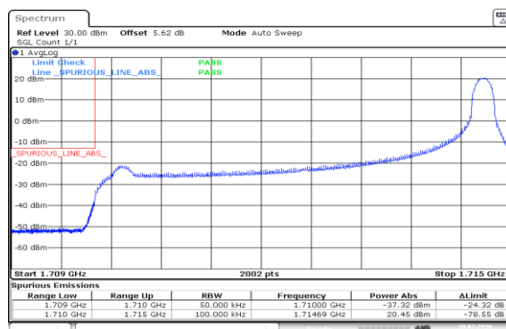
Band4-5MHz-16QAM-19975-1RB#24-PASS
