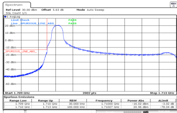
Band4-3MHz-16QAM-19965-1RB#0-PASS
