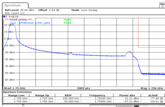
Band4-5MHz-QPSK-20375-1RB#0-PASS
