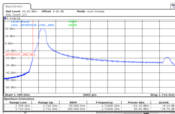
Band4-5MHz-16QAM-19975-1RB#0-PASS
