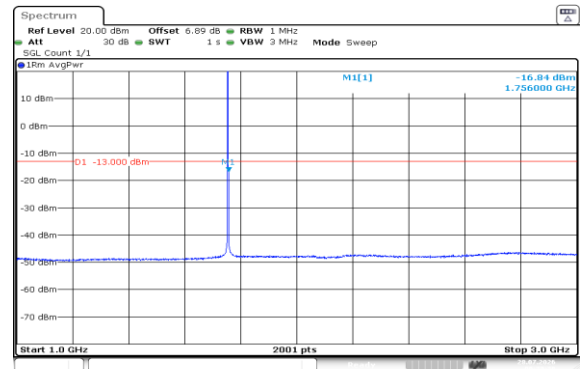
Band4-1.4MHz-QPSK-20393-1RB#0-1000~3000-PASS
