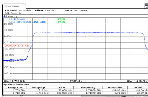
Band4-5MHz-16QAM-19975-25RB#0-PASS
