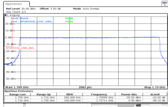
Band4-20MHz-16QAM-20050-100RB#0-PASS
