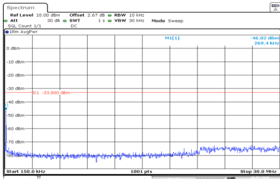
Band4-1.4MHz-16QAM-20175-1RB#5-0.15~30-PASS
