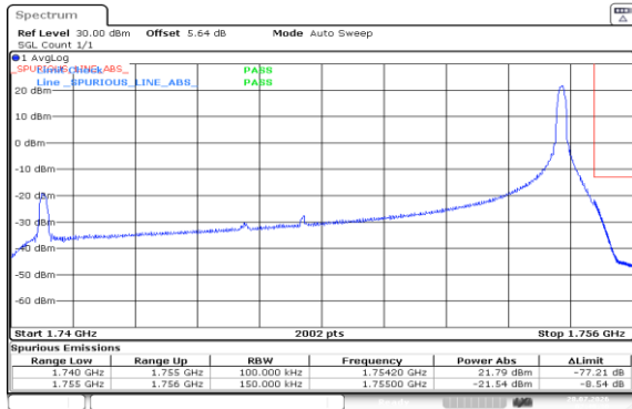
Band4-15MHz-QPSK-20325-1RB#74-PASS
