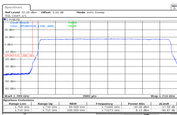
Band4-5MHz-QPSK-19975-25RB#0-PASS
