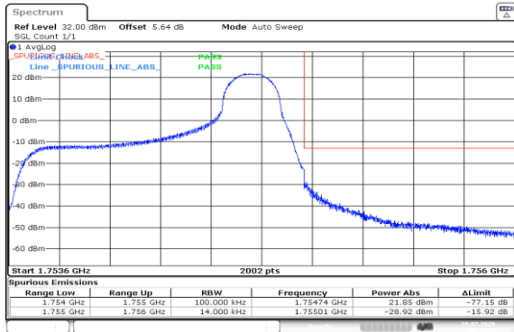
Band4-1.4MHz-QPSK-20393-1RB#5-PASS
