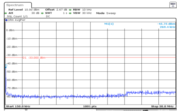
Band4-1.4MHz-16QAM-19957-1RB#5-0.15~30-PASS
