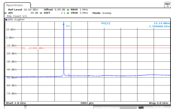
Band4-1.4MHz-QPSK-19957-1RB#0-1000~3000
