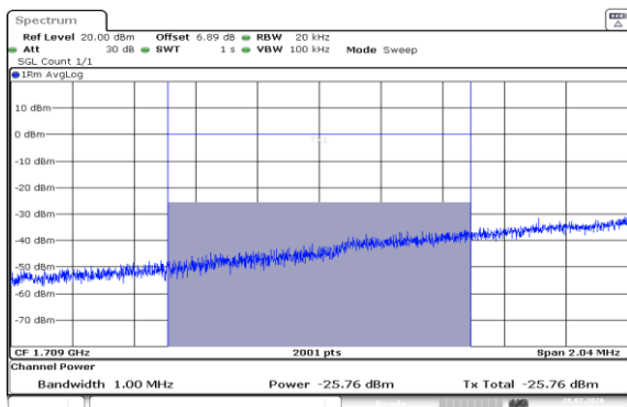
Band4-1.4MHz-16QAM-19957-6RB#0-1000~3000-PASS
