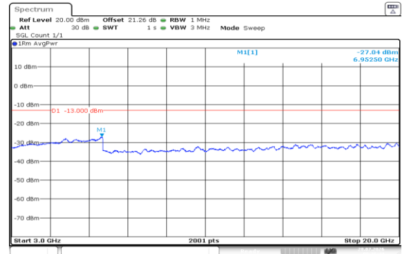
Band4-1.4MHz-16QAM-20175-1RB#0-3000~20000-PASS
