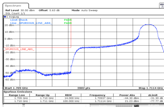
Band4-1.4MHz-16QAM-19957-1RB#5-PASS
