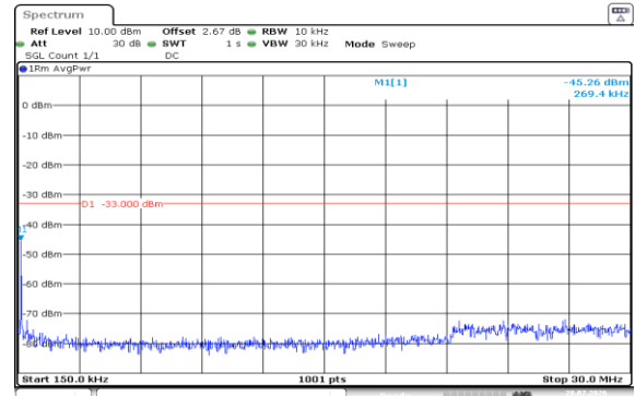
Band4-1.4MHz-QPSK-20393-1RB#5-0.15~30-PASS
