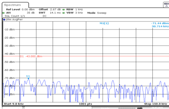
Band4-1.4MHz-16QAM-19957-6RB#0-0.009~0.15-PASS
