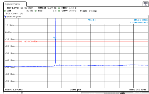
Band4-1.4MHz-16QAM-19957-1RB#5-1000~3000
