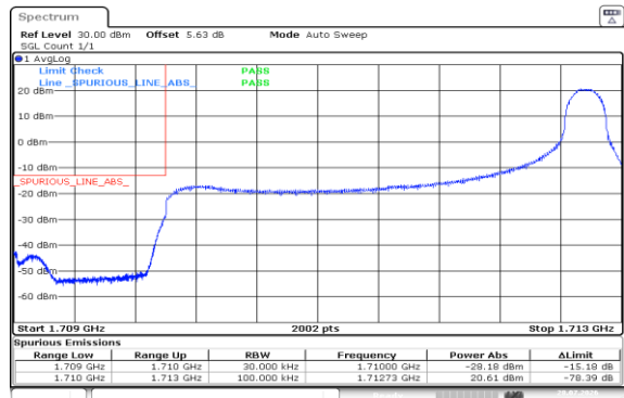
Band4-3MHz-16QAM-19965-1RB#14-PASS
