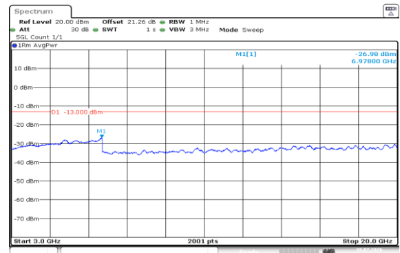
Band4-1.4MHz-16QAM-19957-1RB#5-3000~20000-PASS
