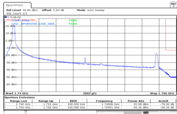
Band4-15MHz-16QAM-20325-1RB#0-PASS
