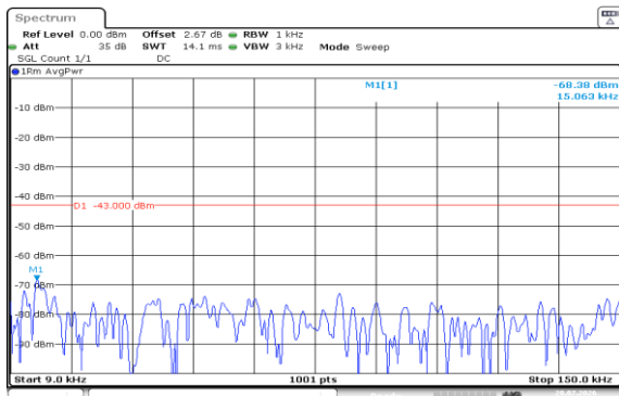
Band4-1.4MHz-16QAM-19957-1RB#5-0.009~0.15-PASS
