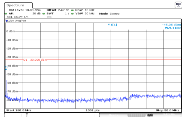
Band4-1.4MHz-QPSK-19957-1RB#0-0.15~30-PASS
