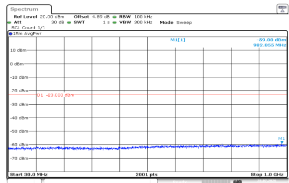
Band4-1.4MHz-16QAM-20175-6RB#0-30~1000-PASS
