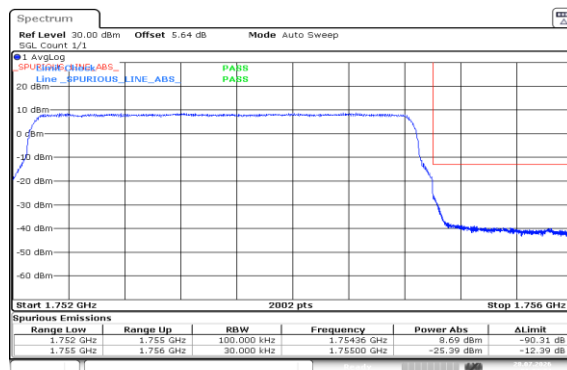
Band4-3MHz-16QAM-20385-15RB#0-PASS
