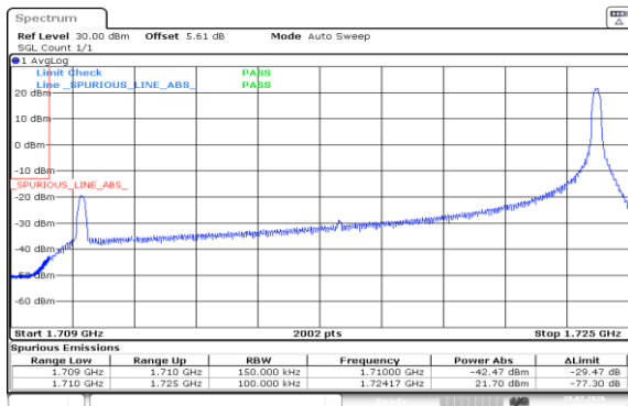
Band4-15MHz-QPSK-20025-1RB#74-PASS
