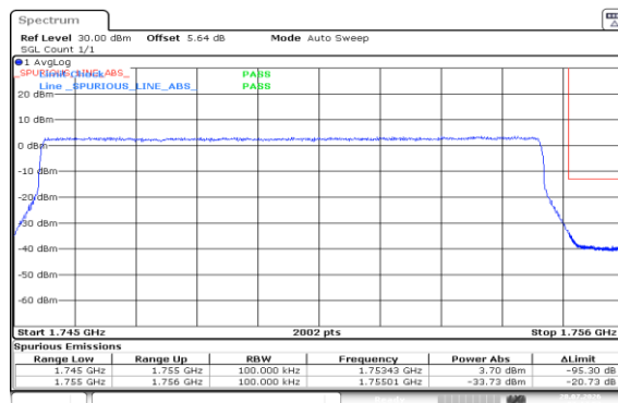
Band4-10MHz-16QAM-20350-50RB#0-PASS
