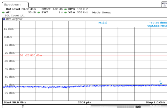
Band4-1.4MHz-QPSK-20393-1RB#0-30~1000-PASS
