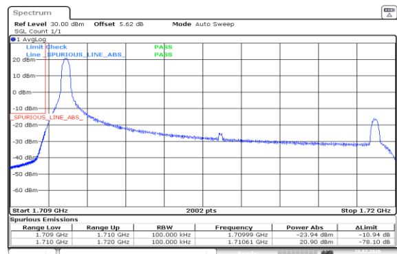
Band4-10MHz-16QAM-20000-1RB#0-PASS
