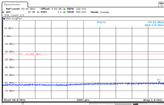
Band4-1.4MHz-16QAM-19957-1RB#5-30~1000-PASS
