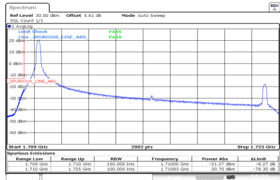
Band4-15MHz-16QAM-20025-1RB#0-PASS
