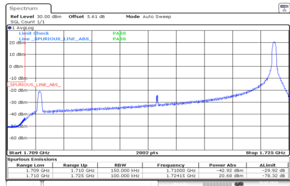
Band4-15MHz-16QAM-20025-1RB#74-PASS
