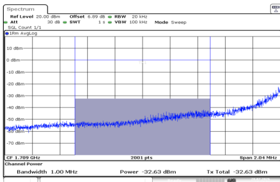
Band4-1.4MHz-16QAM-19957-1RB#0-1000~3000-PASS
