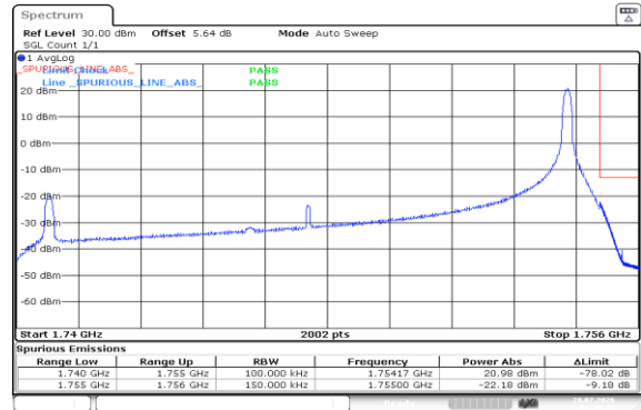
Band4-15MHz-16QAM-20325-1RB#74-PASS
