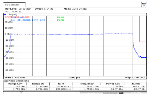
Band4-20MHz-16QAM-20300-100RB#0-PASS
