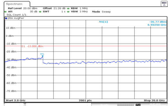
Band4-1.4MHz-QPSK-19957-1RB#0-3000~20000-PASS
