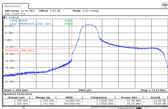
Band4-1.4MHz-QPSK-19957-1RB#0-PASS
