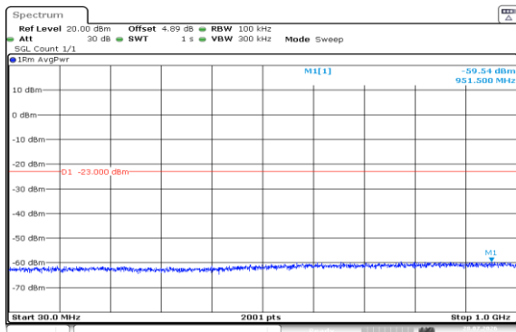
Band4-1.4MHz-QPSK-20175-1RB#5-30~1000-PASS
