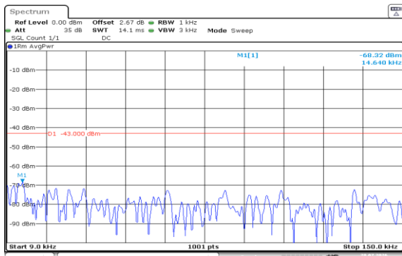
Band4-1.4MHz-16QAM-20393-1RB#5-0.009~0.15-PASS
