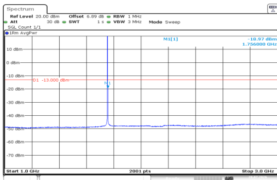
Band4-1.4MHz-16QAM-20393-1RB#0-1000~3000-PASS
