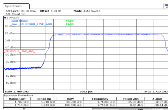
Band4-3MHz-16QAM-19965-15RB#0-PASS
