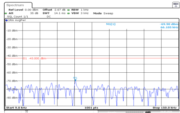
Band4-1.4MHz-16QAM-20393-1RB#0-0.009~0.15-PASS
