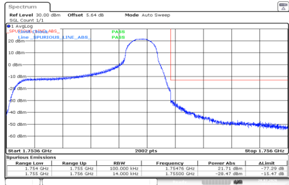
Band4-1.4MHz-16QAM-20393-1RB#5-PASS
