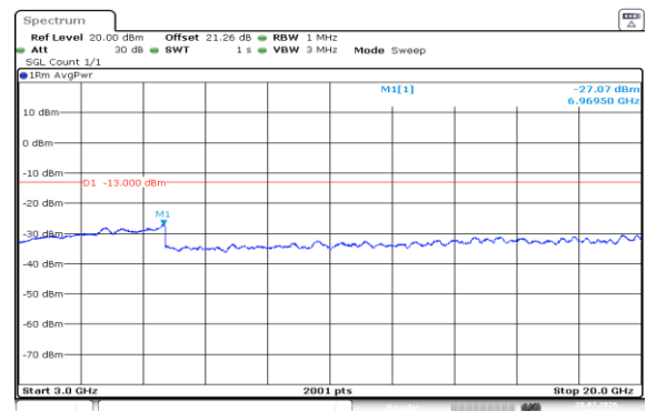
Band4-1.4MHz-16QAM-19957-1RB#0-3000~20000-PASS
