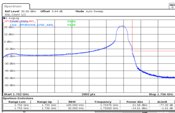
Band4-3MHz-QPSK-20385-1RB#14-PASS
