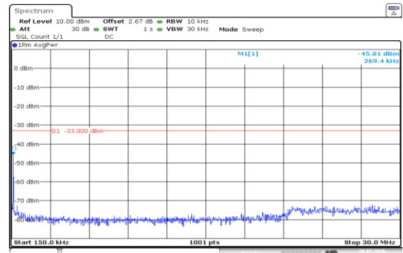
Band4-1.4MHz-QPSK-20175-1RB#0-0.15~30-PASS
