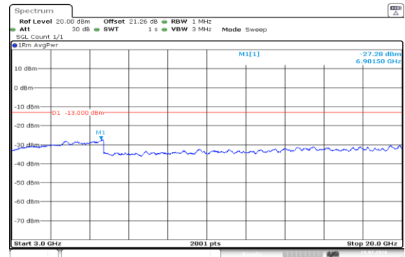
Band4-1.4MHz-QPSK-19957-6RB#0-3000~20000-PASS
