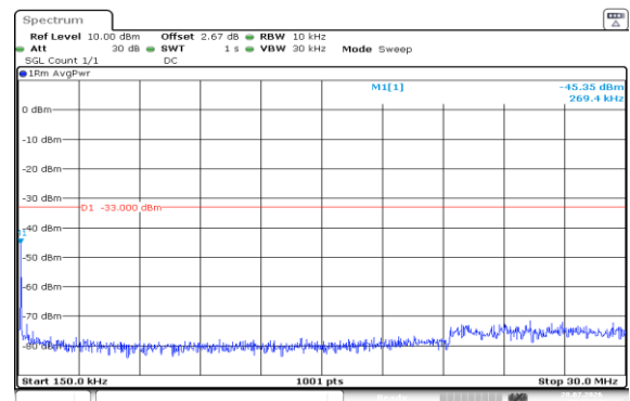
Band4-1.4MHz-QPSK-20393-1RB#0-0.15~30-PASS
