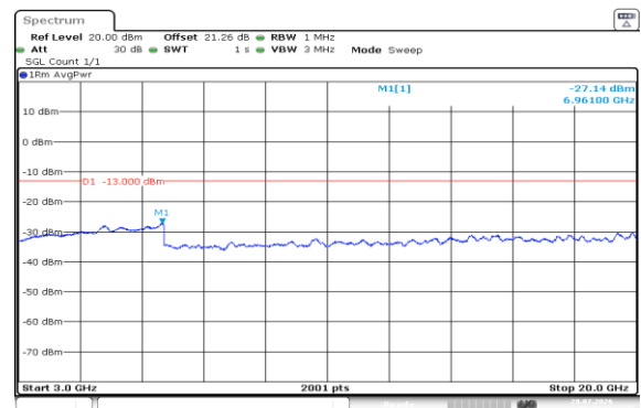
Band4-1.4MHz-16QAM-20393-1RB#0-3000~20000-PASS
