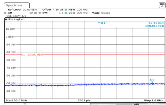
Band4-1.4MHz-16QAM-20393-1RB#0-30~1000-PASS
