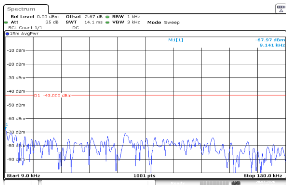
Band4-1.4MHz-QPSK-20393-1RB#0-0.009~0.15-PASS
