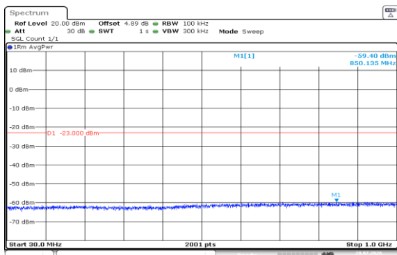
Band4-1.4MHz-QPSK-20175-6RB#0-30~1000-PASS
