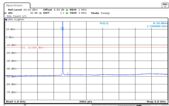
Band4-1.4MHz-QPSK-19957-6RB#0-1000~3000
