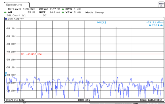
Band4-1.4MHz-16QAM-20175-1RB#0-0.009~0.15-PASS
