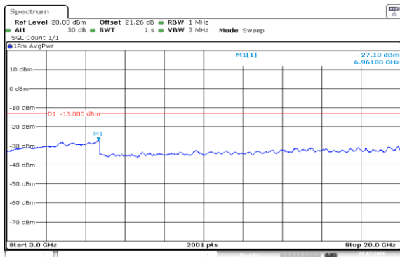
Band4-1.4MHz-QPSK-20393-1RB#0-3000~20000-PASS
