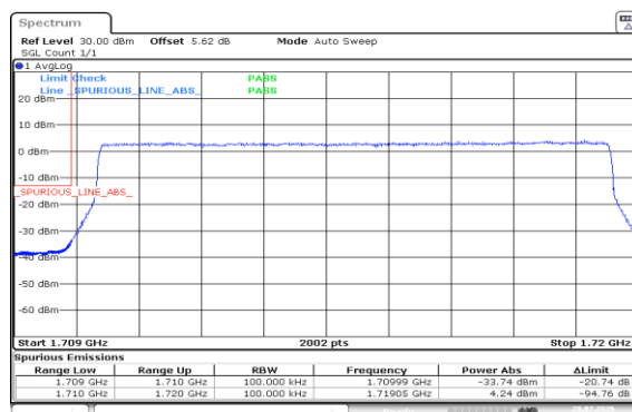
Band4-10MHz-16QAM-20000-50RB#0-PASS
