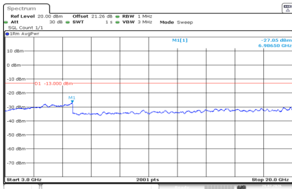
Band4-1.4MHz-QPSK-20175-1RB#5-3000~20000-PASS
