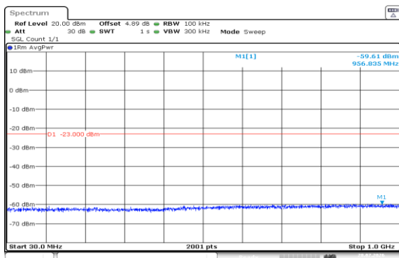
Band4-1.4MHz-16QAM-19957-6RB#0-30~1000-PASS
