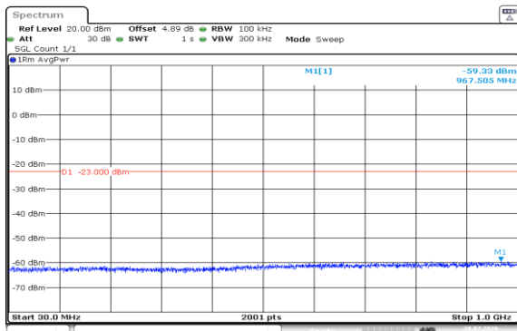
Band4-1.4MHz-QPSK-19957-1RB#5-30~1000-PASS
