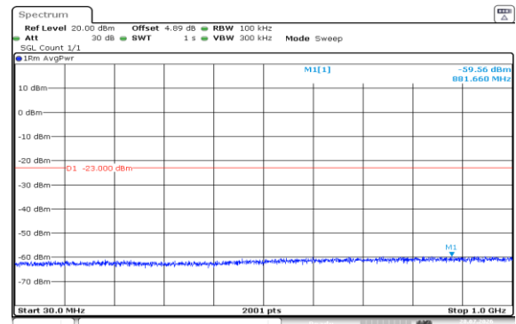
Band4-1.4MHz-16QAM-20175-1RB#0-30~1000-PASS
