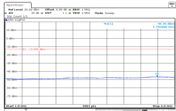
Band4-1.4MHz-QPSK-20175-1RB#5-1000~3000-PASS
