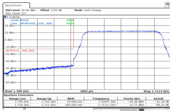
Band4-1.4MHz-16QAM-19957-6RB#0-PASS
