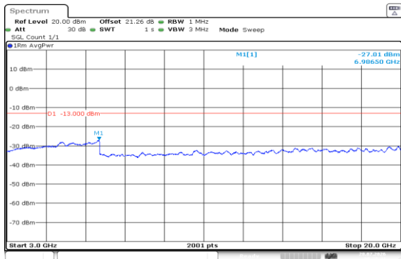
Band4-1.4MHz-QPSK-20175-6RB#0-3000~20000-PASS
