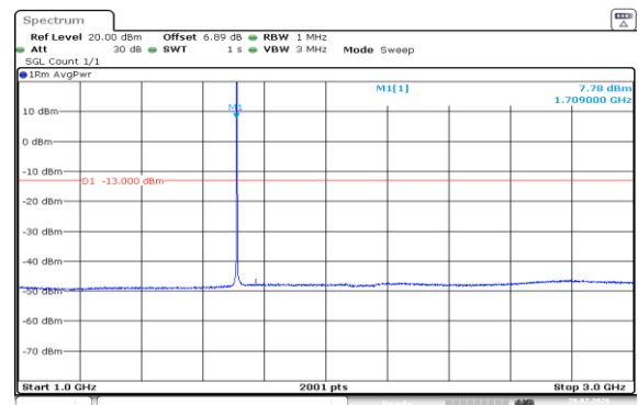
Band4-1.4MHz-16QAM-19957-6RB#0-1000~3000
