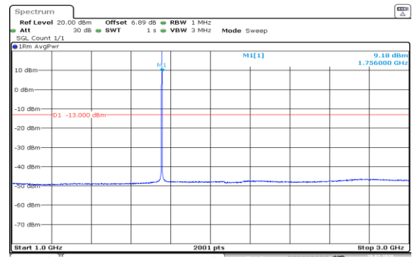
Band4-1.4MHz-QPSK-20393-1RB#5-1000~3000
