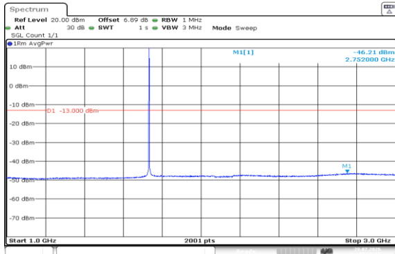
Band4-1.4MHz-16QAM-20175-1RB#0-1000~3000-PASS
