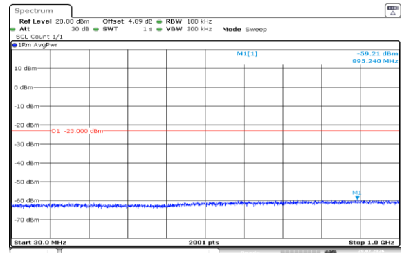
Band4-1.4MHz-16QAM-20175-1RB#5-30~1000-PASS
