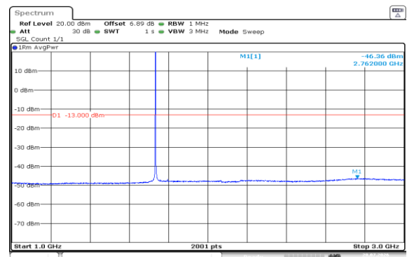
Band4-1.4MHz-QPSK-20175-6RB#0-1000~3000-PASS
