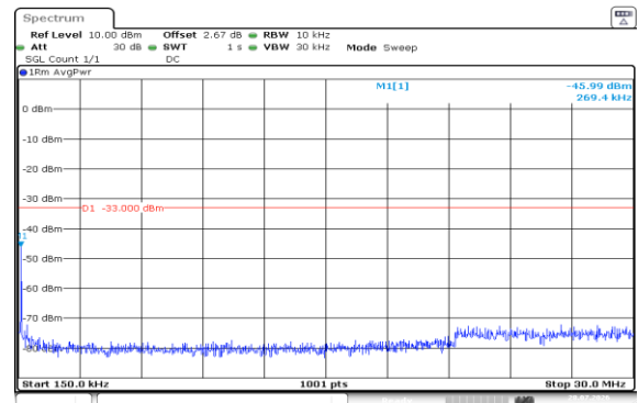
Band4-1.4MHz-QPSK-20175-1RB#5-0.15~30-PASS
