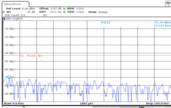
Band4-1.4MHz-QPSK-20393-1RB#5-0.009~0.15-PASS
