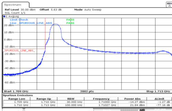
Band4-3MHz-QPSK-19965-1RB#0-PASS
