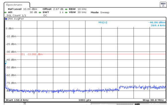
Band4-1.4MHz-16QAM-19957-6RB#0-0.15~30-PASS
