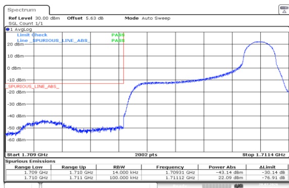
Band4-1.4MHz-QPSK-19957-1RB#5-PASS
