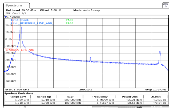
Band4-20MHz-16QAM-20050-1RB#0-PASS
