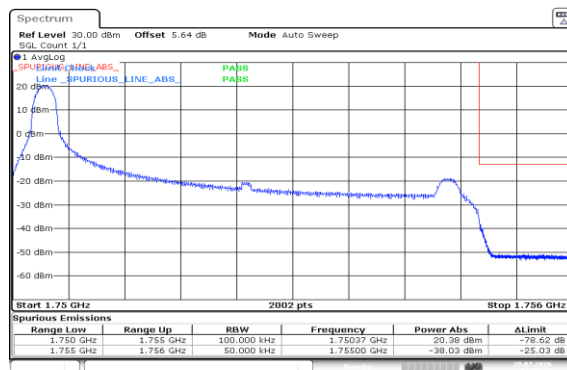
Band4-5MHz-16QAM-20375-1RB#0-PASS
