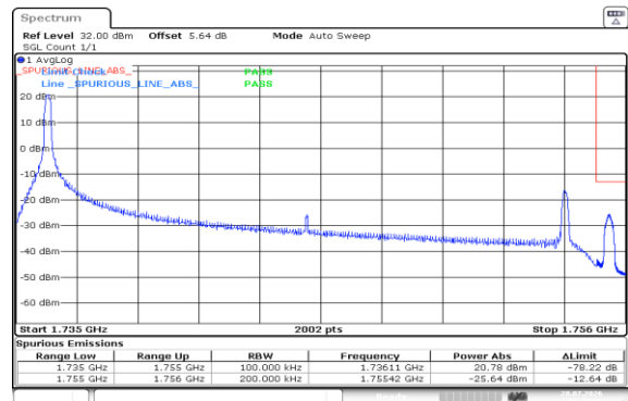
Band4-20MHz-16QAM-20300-1RB#0-PASS
