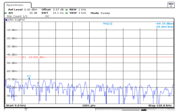
Band4-1.4MHz-16QAM-20175-1RB#5-0.009~0.15-PASS
