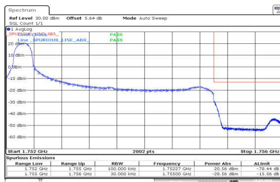
Band4-3MHz-16QAM-20385-1RB#0-PASS
