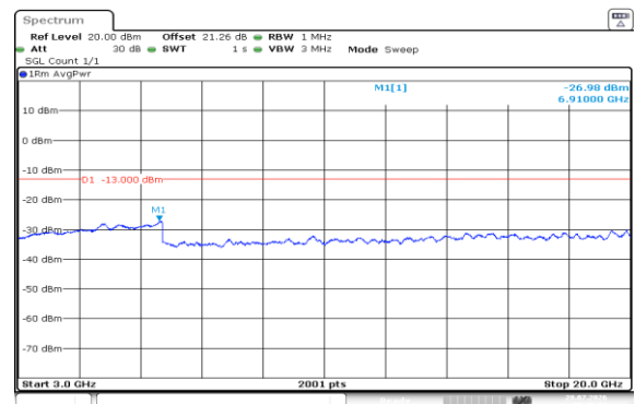
Band4-1.4MHz-16QAM-19957-6RB#0-3000~20000-PASS
