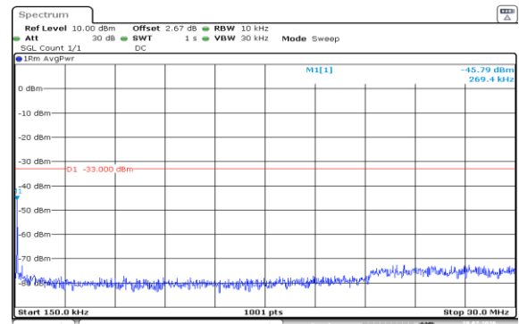
Band4-1.4MHz-16QAM-20393-1RB#5-0.15~30-PASS
