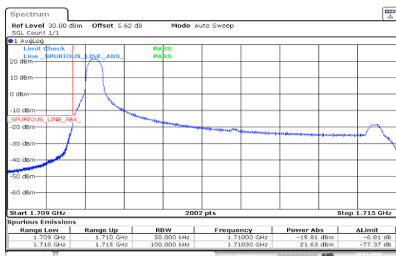
Band4-5MHz-QPSK-19975-1RB#0-PASS
