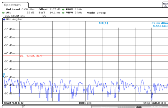
Band4-1.4MHz-QPSK-20175-1RB#5-0.009~0.15-PASS
