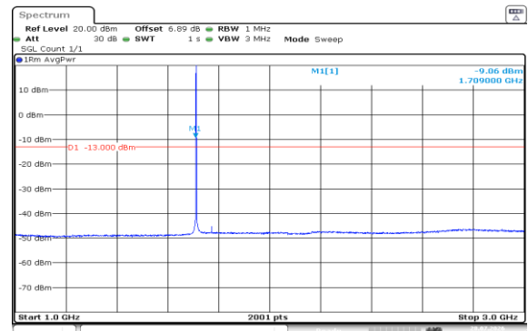
Band4-1.4MHz-QPSK-19957-1RB#5-1000~3000
