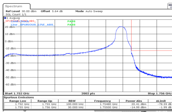
Band4-3MHz-16QAM-20385-1RB#14-PASS
