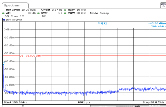
Band4-1.4MHz-16QAM-20393-1RB#0-0.15~30-PASS
