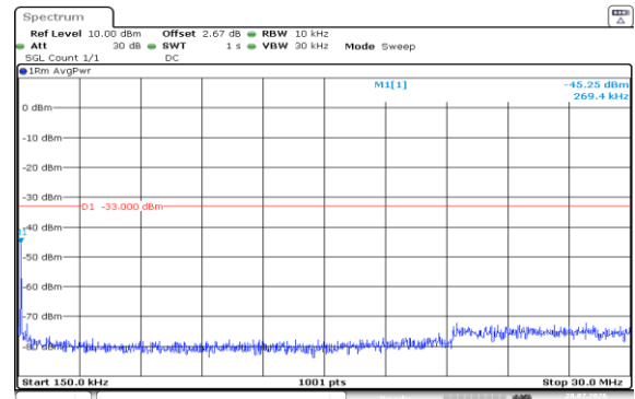
Band4-1.4MHz-QPSK-19957-1RB#5-0.15~30-PASS
