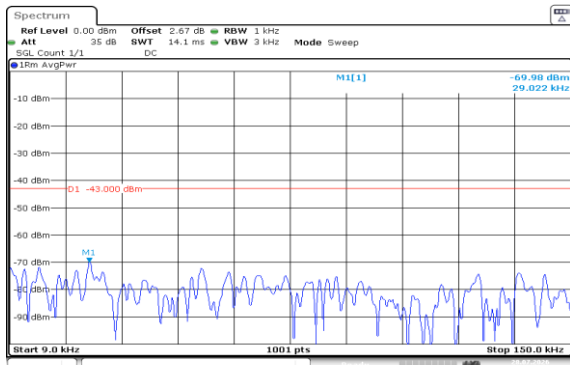
Band4-1.4MHz-QPSK-20175-1RB#0-0.009~0.15-PASS
