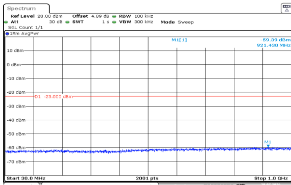
Band4-1.4MHz-QPSK-20393-1RB#5-30~1000-PASS
