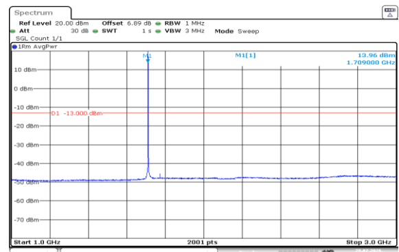
Band4-1.4MHz-16QAM-19957-1RB#0-0.15~30-PASS
