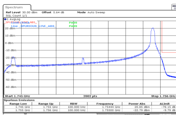
Band4-10MHz-16QAM-20350-1RB#49-PASS
