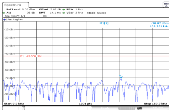
Band4-1.4MHz-QPSK-19957-1RB#0-0.009~0.15-PASS
