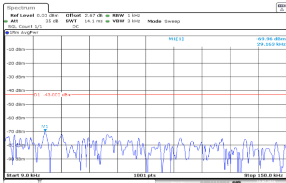
Band4-1.4MHz-QPSK-19957-1RB#5-0.009~0.15-PASS
