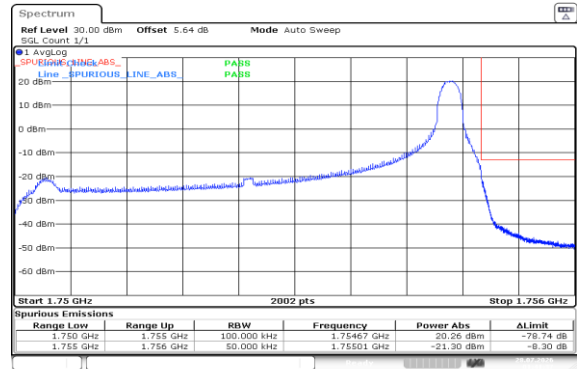
Band4-5MHz-16QAM-20375-1RB#24-PASS
