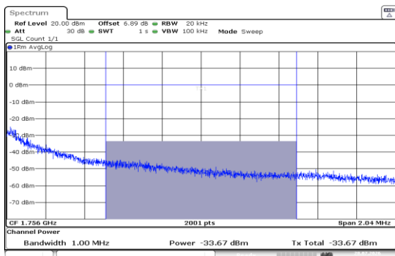
Band4-1.4MHz-QPSK-20393-1RB#5-1000~3000-PASS
