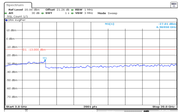
Band4-1.4MHz-16QAM-20175-1RB#5-3000~20000-PASS
