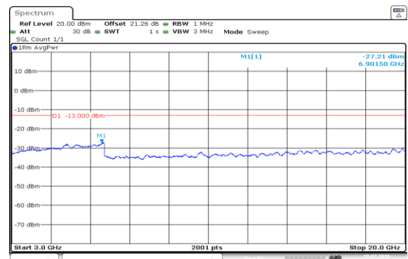
Band4-1.4MHz-QPSK-20393-1RB#5-3000~20000-PASS
