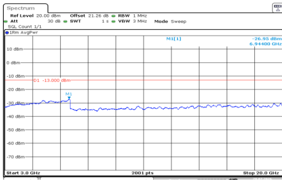
Band4-1.4MHz-QPSK-20175-1RB#0-3000~20000-PASS
