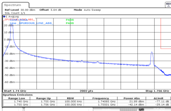
Band4-15MHz-QPSK-20325-1RB#0-PASS
