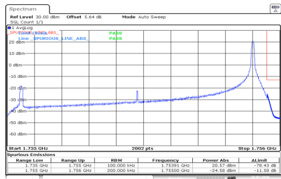
Band4-20MHz-16QAM-20300-1RB#99-PASS
