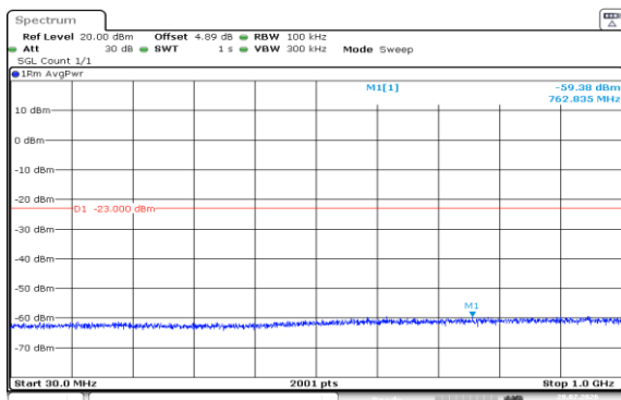
Band4-1.4MHz-QPSK-19957-6RB#0-30~1000-PASS
