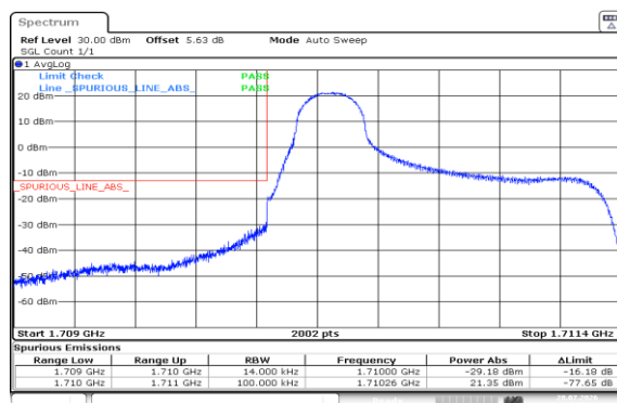
Band4-1.4MHz-16QAM-19957-1RB#0-PASS
