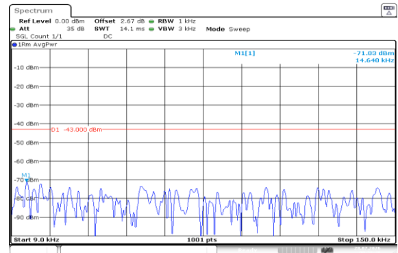
Band4-1.4MHz-16QAM-20175-6RB#0-0.009~0.15-PASS
