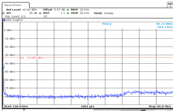
Band4-1.4MHz-16QAM-20175-1RB#0-0.15~30-PASS
