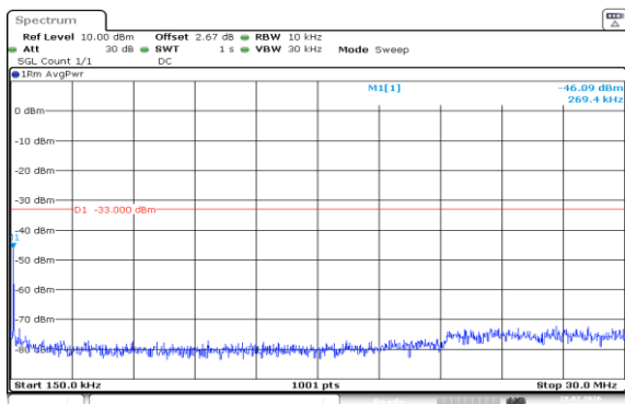
Band4-1.4MHz-16QAM-20175-6RB#0-0.15~30-PASS
