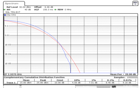
Band41(2535-2655)-5MHz-16QAM-40065-25RB#0-PASS
