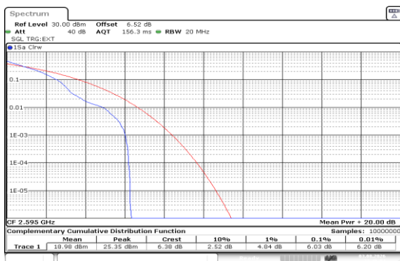
Band41(2535-2655)-15MHz-QPSK-40640-1RB#0-PASS
