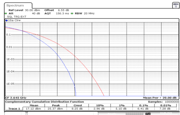
Band41(2535-2655)-20MHz-16QAM-41140-100RB#0-PASS
