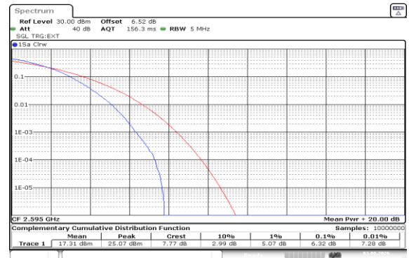
Band41(2535-2655)-5MHz-16QAM-40640-1RB#0-PASS
