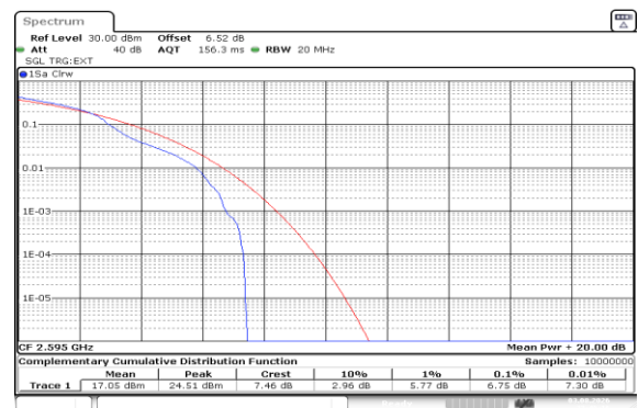
Band41(2535-2655)-15MHz-16QAM-40640-1RB#0-PASS
