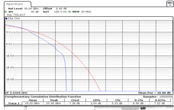
Band41(2535-2655)-15MHz-16QAM-40115-1RB#0-PASS
