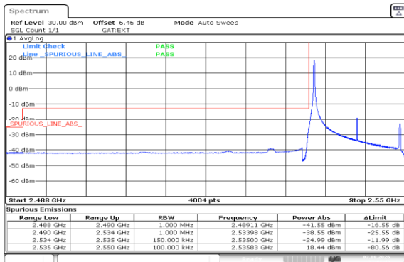
Band41(2535-2655)-15MHz-QPSK-40115-1RB#0-PASS
