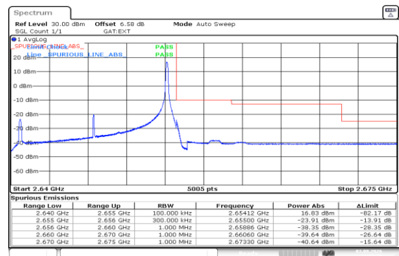
Band41(2535-2655)-15MHz-16QAM-41165-1RB#74-PASS
