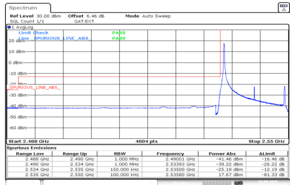
Band41(2535-2655)-15MHz-16QAM-40115-1RB#0-PASS
