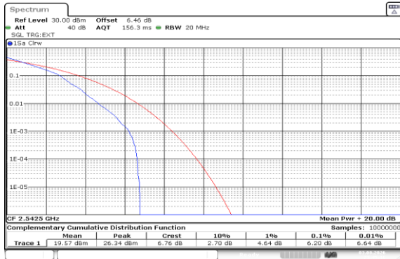
Band41(2535-2655)-15MHz-QPSK-40115-1RB#0-PASS
