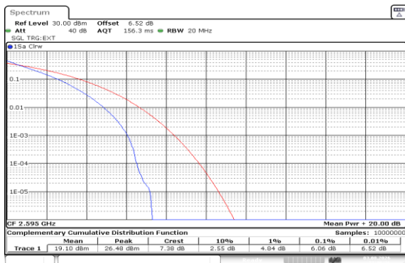
Band41(2535-2655)-15MHz-QPSK-40640-75RB#0-PASS
