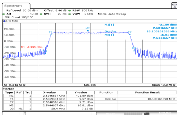
Band41(2535-2655)-20MHz-QPSK-40140-100RB#0-PASS
