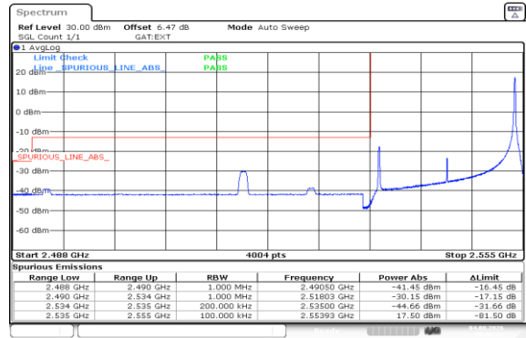
Band41(2535-2655)-20MHz-16QAM-40140-1RB#99-PASS
