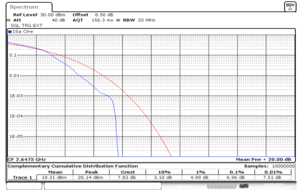
Band41(2535-2655)-15MHz-16QAM-41165-1RB#0-PASS
