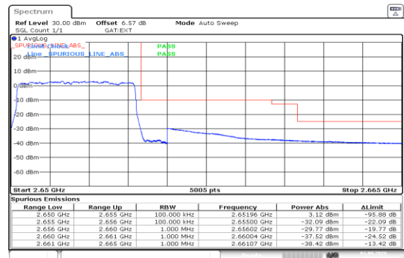
Band41(2535-2655)-5MHz-16QAM-41215-25RB#0-PASS
