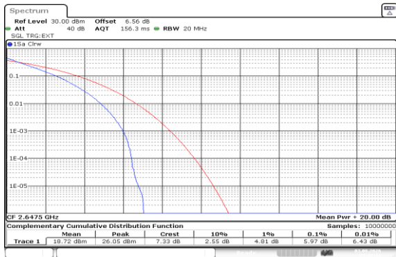
Band41(2535-2655)-15MHz-QPSK-41165-75RB#0-PASS
