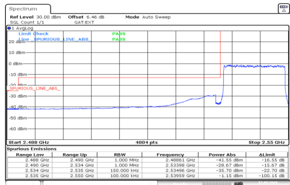
Band41(2535-2655)-15MHz-16QAM-40115-75RB#0-PASS
