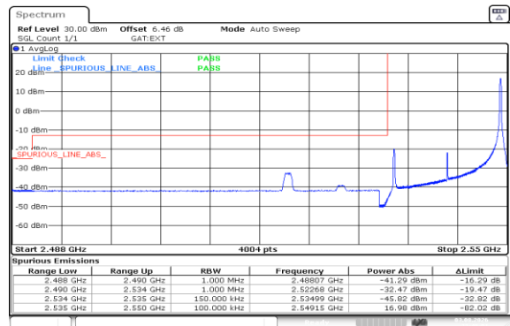
Band41(2535-2655)-15MHz-16QAM-40115-1RB#74-PASS
