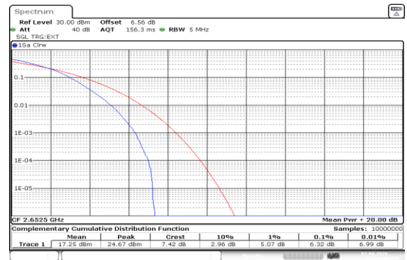
Band41(2535-2655)-5MHz-16QAM-41215-25RB#0-PASS
