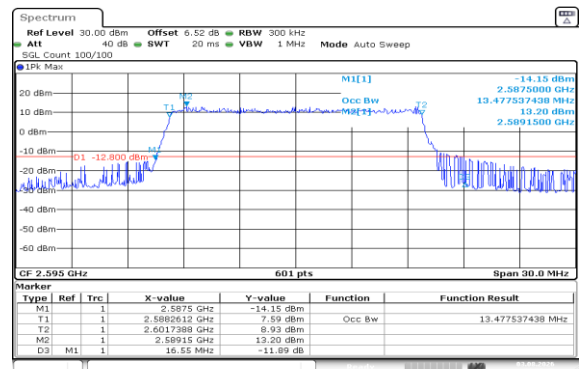
Band41(2535-2655)-15MHz-16QAM-40640-75RB#0-PASS
