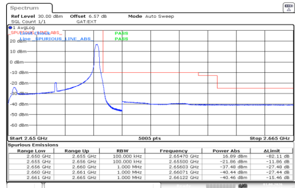
Band41(2535-2655)-5MHz-16QAM-41215-1RB#24-PASS
