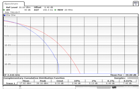
Band41(2535-2655)-20MHz-16QAM-40140-100RB#0-PASS
