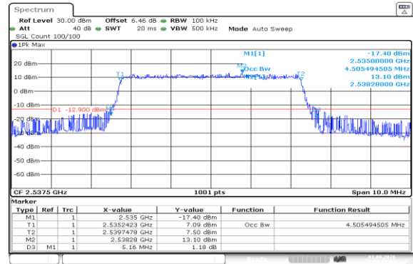
Band41(2535-2655)-5MHz-16QAM-40065-25RB#0-PASS
