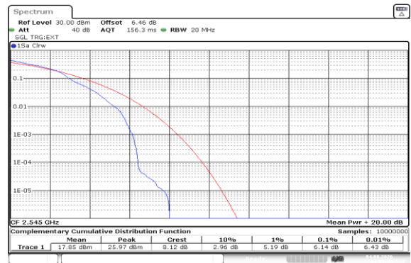
Band41(2535-2655)-20MHz-16QAM-40140-1RB#0-PASS
