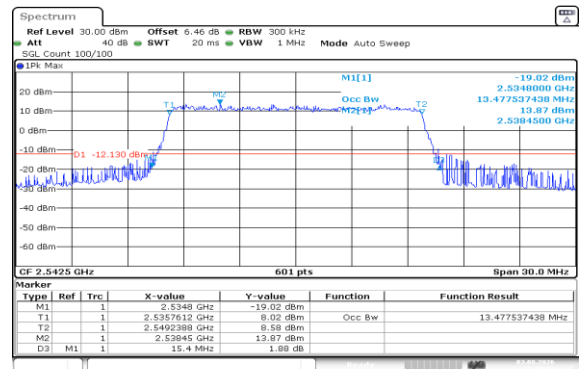
Band41(2535-2655)-15MHz-16QAM-40115-75RB#0-PASS
