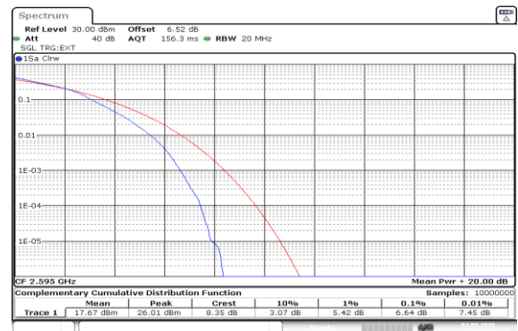
Band41(2535-2655)-15MHz-16QAM-40640-75RB#0-PASS
