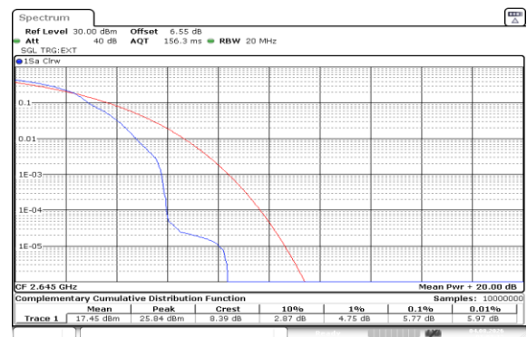
Band41(2535-2655)-20MHz-16QAM-41140-1RB#0-PASS
