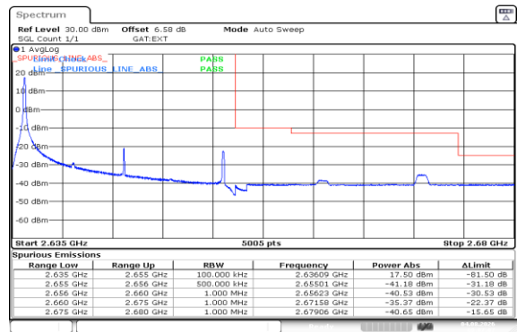
Band41(2535-2655)-20MHz-16QAM-41140-1RB#0-PASS
