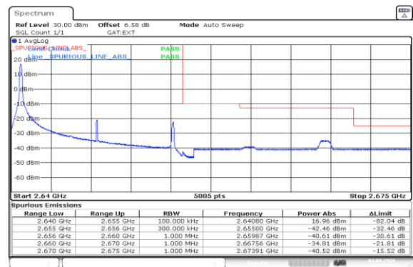
Band41(2535-2655)-15MHz-16QAM-41165-1RB#0-PASS
