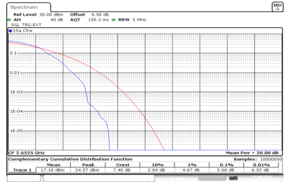
Band41(2535-2655)-5MHz-16QAM-41215-1RB#0-PASS
