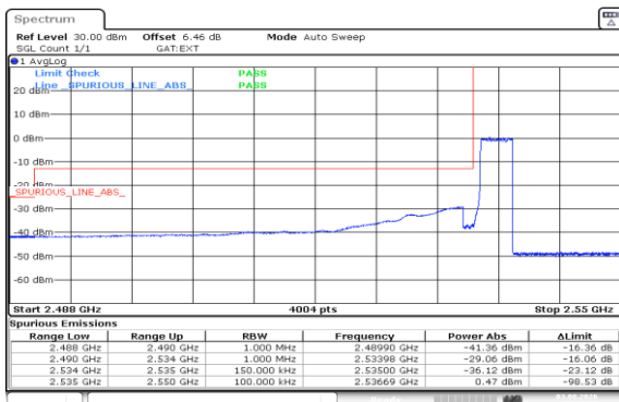
Band41(2535-2655)-15MHz-QPSK-40115-75RB#0-PASS
