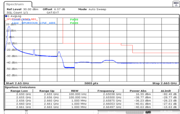
Band41(2535-2655)-5MHz-16QAM-41215-1RB#0-PASS
