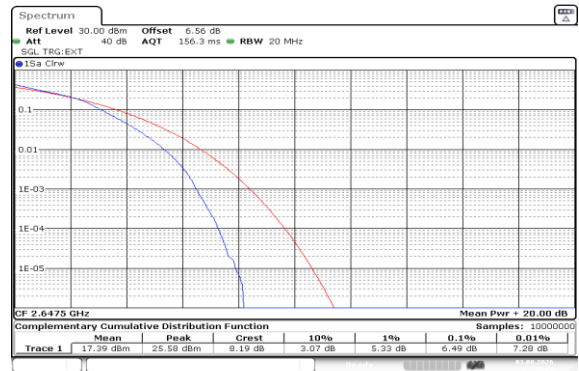
Band41(2535-2655)-15MHz-16QAM-41165-75RB#0-PASS
