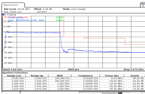
Band41(2535-2655)-15MHz-QPSK-41165-75RB#0-PASS
