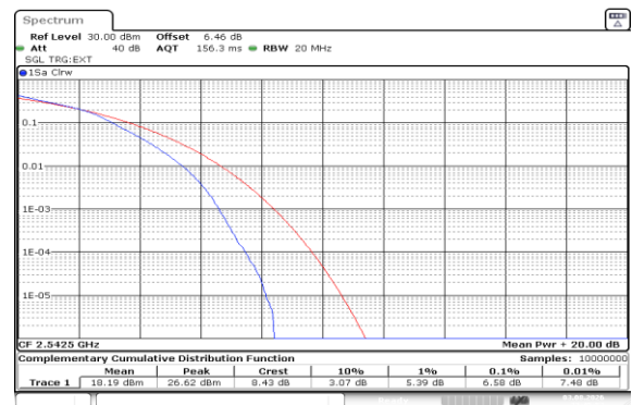
Band41(2535-2655)-15MHz-16QAM-40115-75RB#0-PASS
