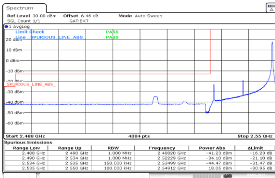
Band41(2535-2655)-15MHz-QPSK-40115-1RB#74-PASS
