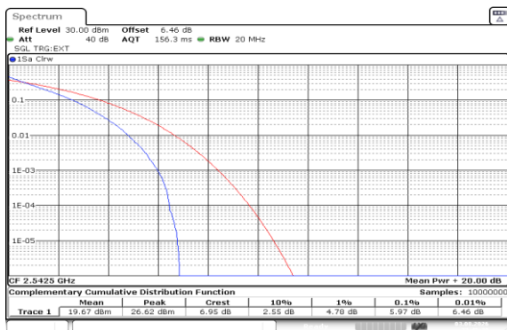
Band41(2535-2655)-15MHz-QPSK-40115-75RB#0-PASS
