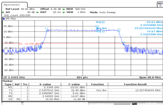
Band41(2535-2655)-15MHz-QPSK-40115-75RB#0-PASS
