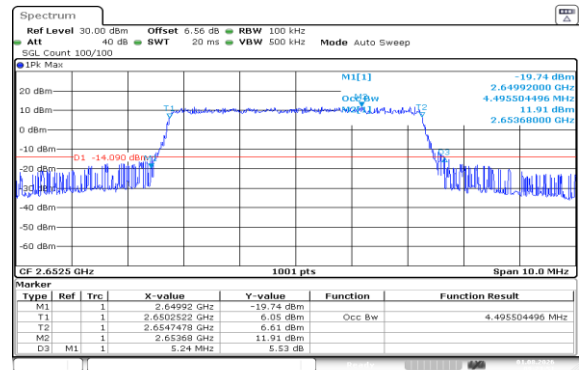
Band41(2535-2655)-5MHz-16QAM-41215-25RB#0-PASS
