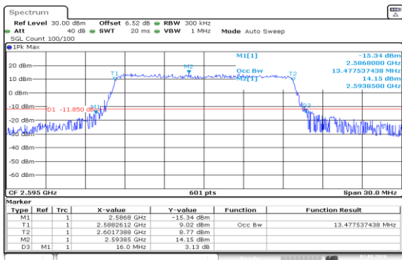
Band41(2535-2655)-15MHz-QPSK-40640-75RB#0-PASS
