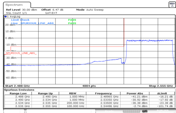
Band41(2535-2655)-20MHz-16QAM-40140-100RB#0-PASS
