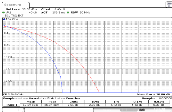
Band41(2535-2655)-20MHz-QPSK-40140-100RB#0-PASS
