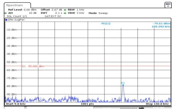
Band41(2535-2655)-5MHz-16QAM-41215-1RB#24-0.009~0.15-PASS
