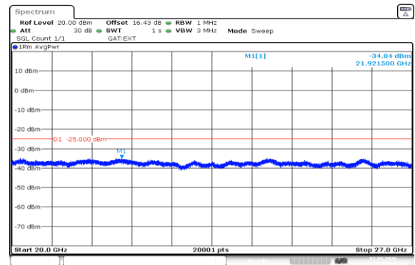
Band41(2535-2655)-10MHz-16QAM-40090-1RB#49-20000~27000-PASS
