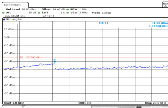
Band41(2535-2655)-5MHz-16QAM-41215-25RB#0-1000~20000-PASS
