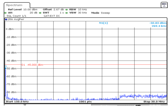
Band41(2535-2655)-5MHz-QPSK-40640-25RB#0-0.15~30-PASS
