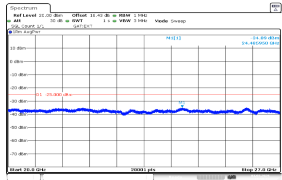
Band41(2535-2655)-5MHz-16QAM-41215-1RB#0-20000~27000-PASS
