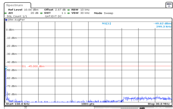
Band41(2535-2655)-5MHz-QPSK-40065-1RB#24-0.15~30-PASS
