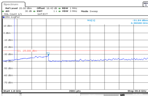
Band41(2535-2655)-5MHz-16QAM-40065-1RB#0-1000~20000-PASS
