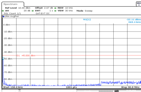
Band41(2535-2655)-10MHz-16QAM-40090-50RB#0-0.15~30-PASS
