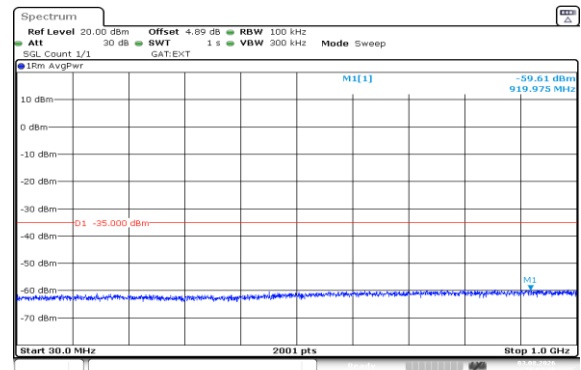
Band41(2535-2655)-5MHz-16QAM-41215-1RB#24-30~1000-PASS
