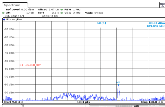
Band41(2535-2655)-5MHz-QPSK-40065-1RB#24-0.009~0.15-PASS
