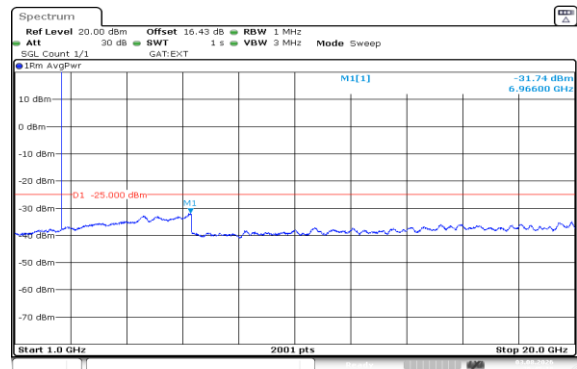
Band41(2535-2655)-5MHz-QPSK-40640-1RB#0-1000~20000-PASS
