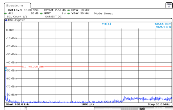
Band41(2535-2655)-10MHz-QPSK-40090-50RB#0-0.15~30-PASS
