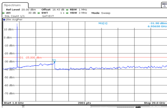
Band41(2535-2655)-10MHz-16QAM-41190-50RB#0-1000~20000-PASS
