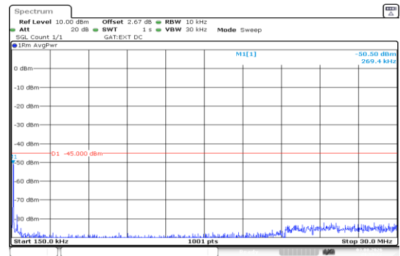
Band41(2535-2655)-10MHz-QPSK-40090-1RB#49-0.15~30-PASS
