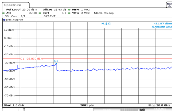
Band41(2535-2655)-10MHz-16QAM-40640-1RB#0-1000~20000-PASS
