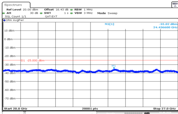
Band41(2535-2655)-5MHz-QPSK-40640-1RB#0-20000~27000-PASS
