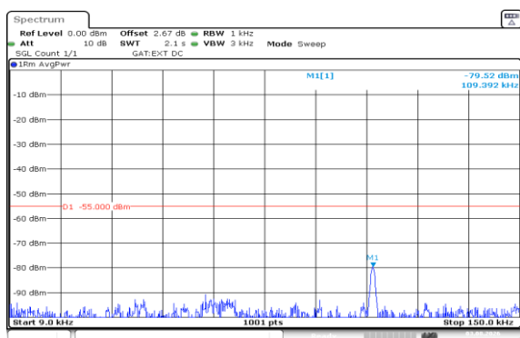
Band41(2535-2655)-5MHz-QPSK-40640-1RB#24-0.009~0.15-PASS
