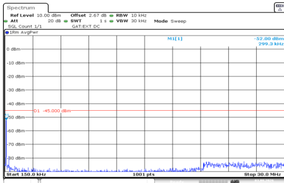
Band41(2535-2655)-5MHz-16QAM-41215-25RB#0-0.15~30-PASS
