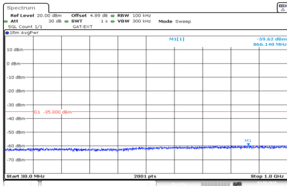
Band41(2535-2655)-5MHz-QPSK-40065-25RB#0-30~1000-PASS
