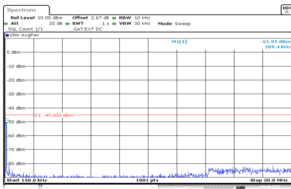
Band41(2535-2655)-10MHz-16QAM-41190-50RB#0-0.15~30-PASS
