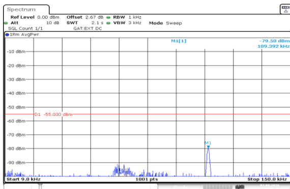
Band41(2535-2655)-10MHz-QPSK-40090-50RB#0-0.009~0.15-PASS
