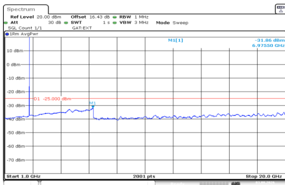
Band41(2535-2655)-5MHz-16QAM-41215-1RB#24-1000~20000-PASS
