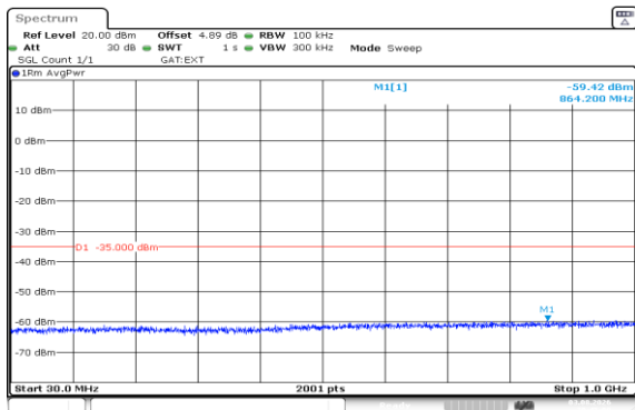
Band41(2535-2655)-5MHz-QPSK-40640-1RB#0-30~1000-PASS
