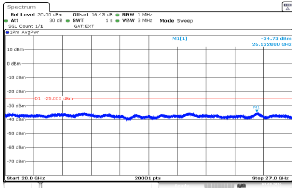
Band41(2535-2655)-5MHz-QPSK-40640-1RB#24-20000~27000-PASS
