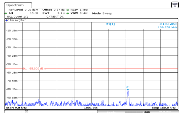
Band41(2535-2655)-5MHz-16QAM-41215-1RB#0-0.009~0.15-PASS
