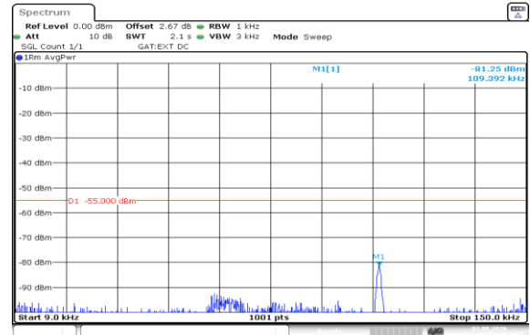
Band41(2535-2655)-5MHz-16QAM-41215-25RB#0-0.009~0.15-PASS
