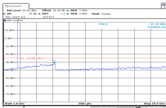
Band41(2535-2655)-5MHz-QPSK-40640-1RB#24-1000~20000-PASS
