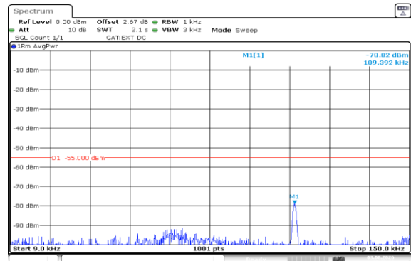
Band41(2535-2655)-5MHz-16QAM-40640-1RB#0-0.009~0.15-PASS
