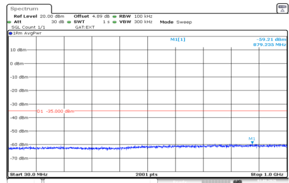
Band41(2535-2655)-10MHz-16QAM-40090-1RB#49-30~1000-PASS
