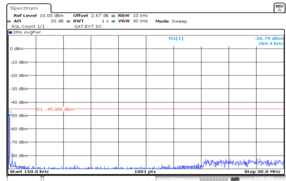
Band41(2535-2655)-5MHz-QPSK-41215-25RB#0-0.15~30-PASS
