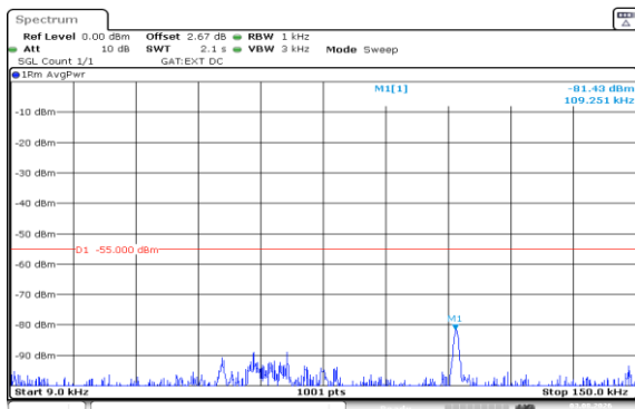
Band41(2535-2655)-10MHz-QPSK-40090-1RB#0-0.009~0.15-PASS
