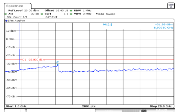
Band41(2535-2655)-5MHz-QPSK-41215-1RB#24-1000~20000-PASS
