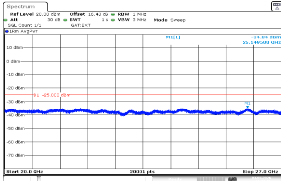
Band41(2535-2655)-5MHz-QPSK-41215-25RB#0-20000~27000-PASS
