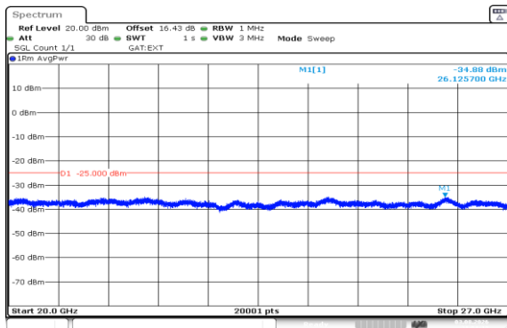
Band41(2535-2655)-10MHz-QPSK-40090-1RB#49-20000~27000-PASS
