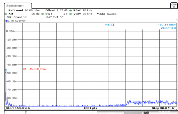
Band41(2535-2655)-5MHz-QPSK-41215-1RB#24-0.15~30-PASS
