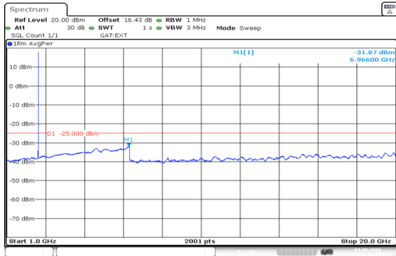
Band41(2535-2655)-5MHz-16QAM-40065-25RB#0-1000~20000-PASS
