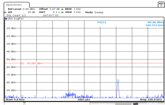
Band41(2535-2655)-5MHz-16QAM-40065-25RB#0-0.009~0.15-PASS
