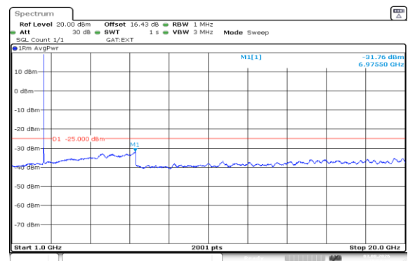
Band41(2535-2655)-10MHz-QPSK-40090-50RB#0-1000~20000-PASS
