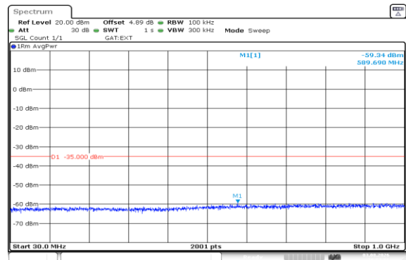
Band41(2535-2655)-5MHz-16QAM-40640-25RB#0-30~1000-PASS
