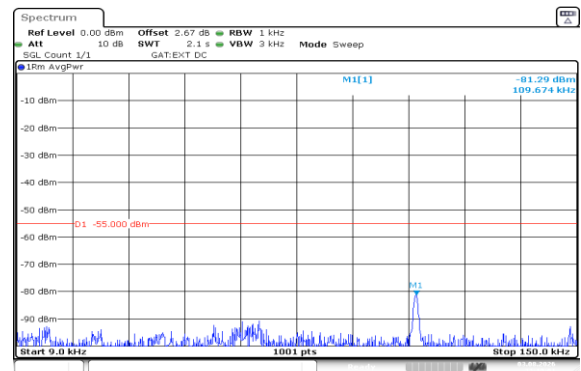
Band41(2535-2655)-10MHz-16QAM-41190-1RB#0-0.009~0.15-PASS
