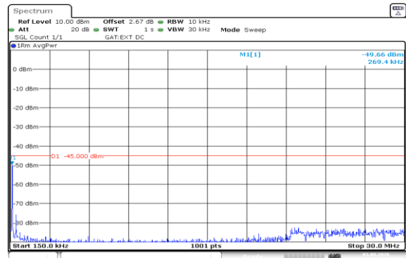
Band41(2535-2655)-5MHz-QPSK-40640-1RB#0-0.15~30-PASS
