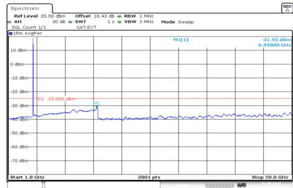
Band41(2535-2655)-10MHz-QPSK-41190-50RB#0-1000~20000-PASS
