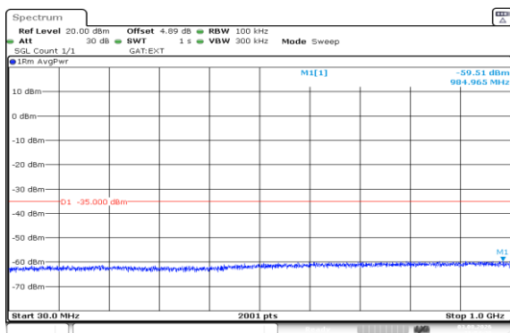
Band41(2535-2655)-10MHz-QPSK-40090-50RB#0-30~1000-PASS
