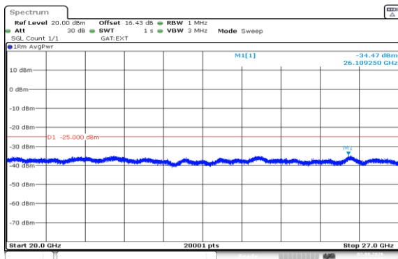
Band41(2535-2655)-10MHz-QPSK-40090-50RB#0-20000~27000-PASS
