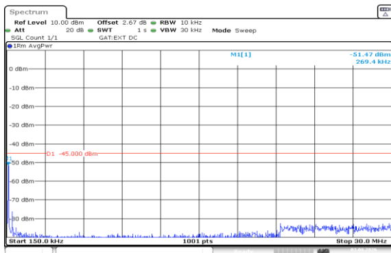
Band41(2535-2655)-10MHz-16QAM-40090-1RB#49-0.15~30-PASS
