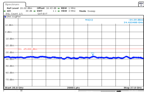
Band41(2535-2655)-10MHz-16QAM-41190-50RB#0-20000~27000-PASS
