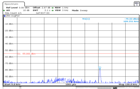
Band41(2535-2655)-10MHz-16QAM-40640-1RB#0-0.009~0.15-PASS
