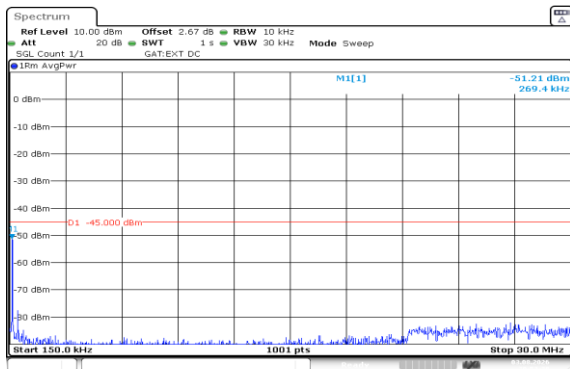
Band41(2535-2655)-5MHz-16QAM-40640-25RB#0-0.15~30-PASS
