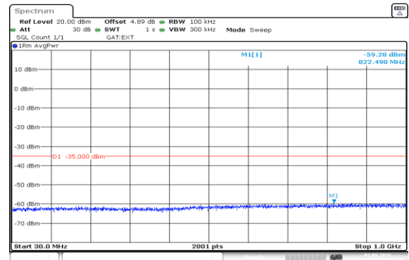
Band41(2535-2655)-5MHz-16QAM-40065-25RB#0-30~1000-PASS
