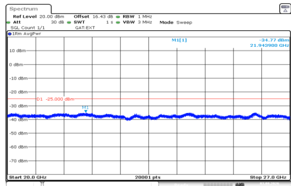
Band41(2535-2655)-5MHz-16QAM-40640-25RB#0-20000~27000-PASS
