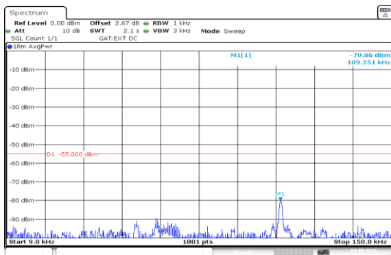
Band41(2535-2655)-10MHz-QPSK-41190-1RB#0-0.009~0.15-PASS
