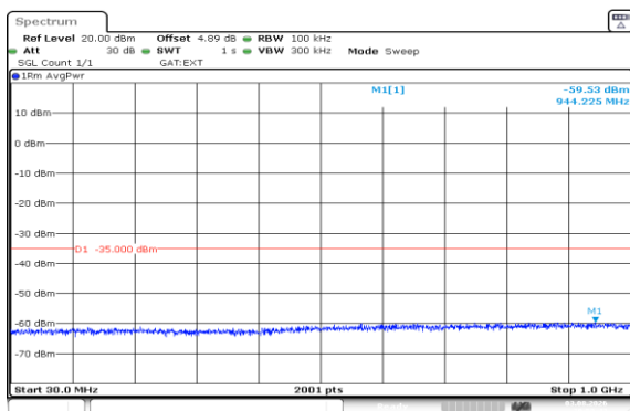
Band41(2535-2655)-5MHz-QPSK-41215-1RB#24-30~1000-PASS
