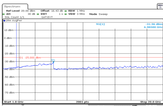
Band41(2535-2655)-5MHz-16QAM-40640-1RB#0-1000~20000-PASS
