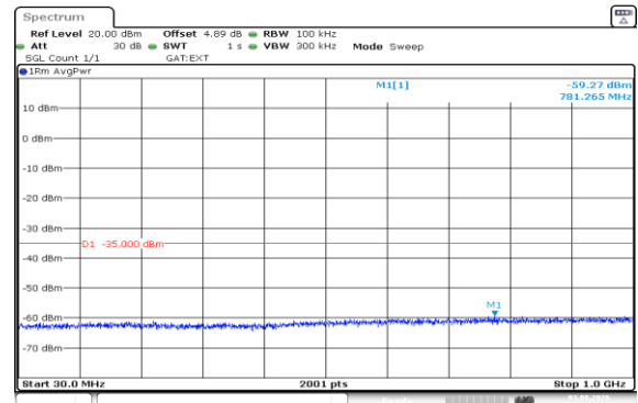
Band41(2535-2655)-5MHz-16QAM-41215-1RB#0-30~1000-PASS
