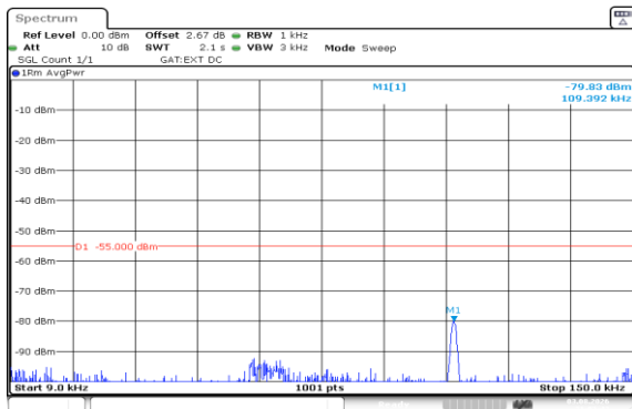
Band41(2535-2655)-5MHz-QPSK-41215-25RB#0-0.009~0.15-PASS
