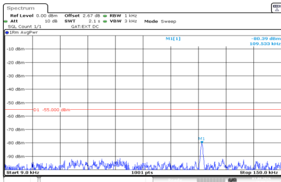
Band41(2535-2655)-5MHz-QPSK-41215-1RB#0-0.009~0.15-PASS
