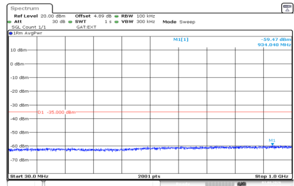
Band41(2535-2655)-10MHz-16QAM-40640-1RB#49-30~1000-PASS
