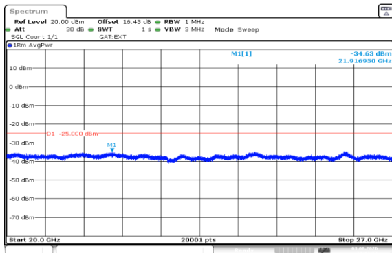
Band41(2535-2655)-5MHz-QPSK-40065-25RB#0-20000~27000-PASS
