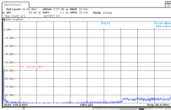
Band41(2535-2655)-5MHz-16QAM-41215-1RB#0-0.15~30-PASS
