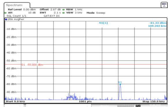
Band41(2535-2655)-10MHz-16QAM-40090-50RB#0-0.009~0.15-PASS
