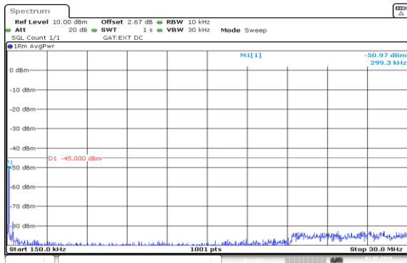
Band41(2535-2655)-5MHz-16QAM-40065-25RB#0-0.15~30-PASS
