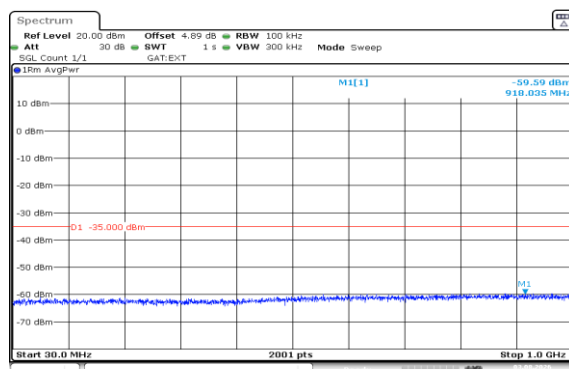
Band41(2535-2655)-5MHz-16QAM-40640-1RB#0-30~1000-PASS
