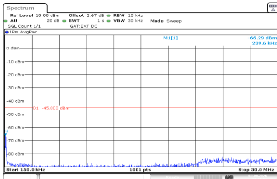
Band41(2535-2655)-10MHz-16QAM-40640-1RB#49-0.15~30-PASS
