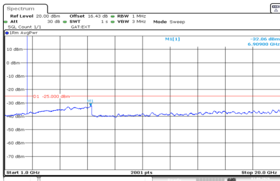
Band41(2535-2655)-5MHz-16QAM-40065-1RB#24-1000~20000-PASS
