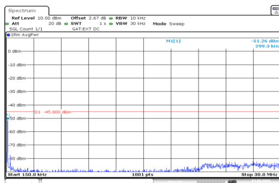
Band41(2535-2655)-5MHz-QPSK-40640-1RB#24-0.15~30-PASS
