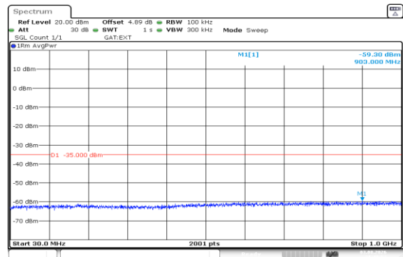
Band41(2535-2655)-10MHz-16QAM-40090-1RB#0-30~1000-PASS
