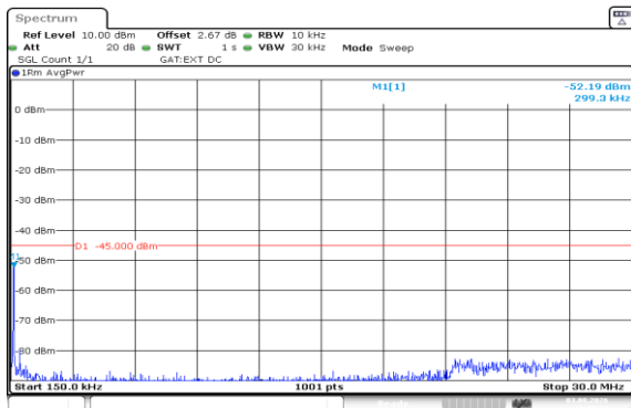
Band41(2535-2655)-10MHz-16QAM-40090-1RB#0-0.15~30-PASS
