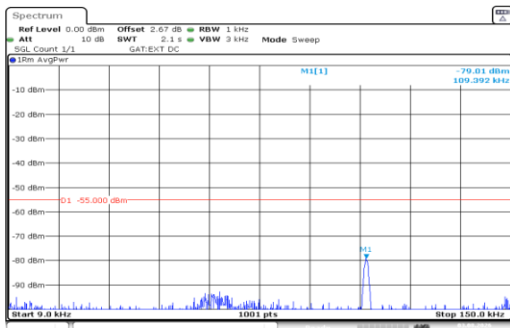
Band41(2535-2655)-5MHz-QPSK-40640-25RB#0-0.009~0.15-PASS
