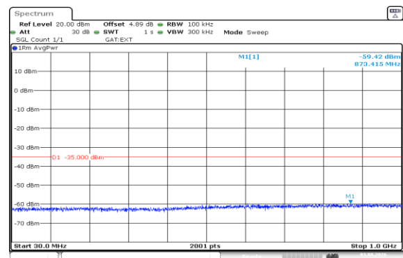
Band41(2535-2655)-10MHz-16QAM-41190-50RB#0-30~1000-PASS
