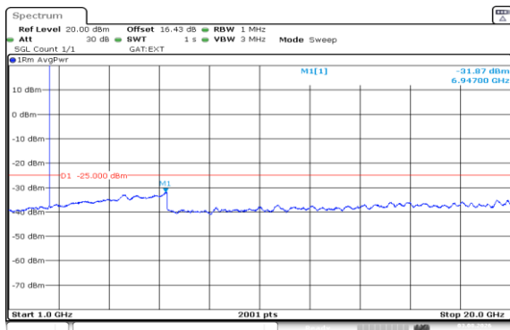
Band41(2535-2655)-10MHz-16QAM-40090-1RB#0-1000~20000-PASS
