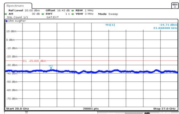
Band41(2535-2655)-5MHz-16QAM-41215-1RB#24-20000~27000-PASS
