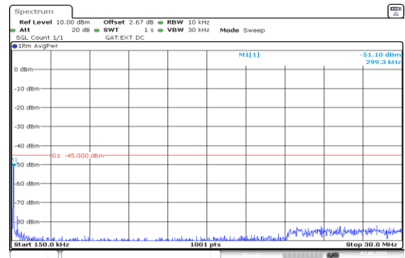
Band41(2535-2655)-5MHz-QPSK-41215-1RB#0-0.15~30-PASS
