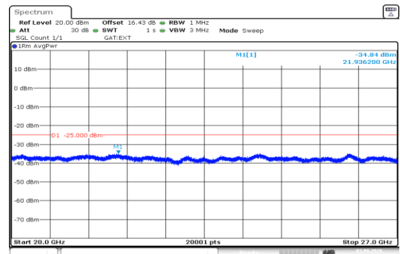
Band41(2535-2655)-5MHz-16QAM-40065-1RB#24-20000~27000-PASS
