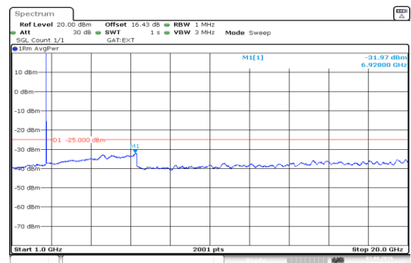
Band41(2535-2655)-10MHz-QPSK-41190-1RB#0-1000~20000-PASS
