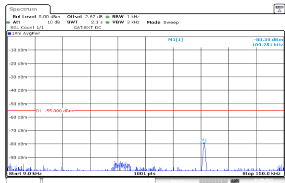
Band41(2535-2655)-5MHz-16QAM-40640-25RB#0-0.009~0.15-PASS
