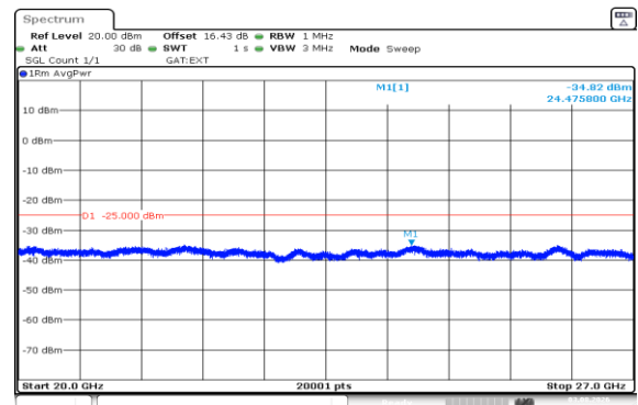
Band41(2535-2655)-10MHz-16QAM-40640-1RB#49-20000~27000-PASS
