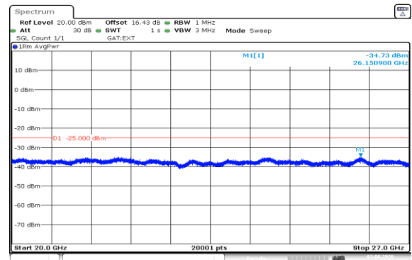
Band41(2535-2655)-5MHz-16QAM-40640-1RB#24-20000~27000-PASS
