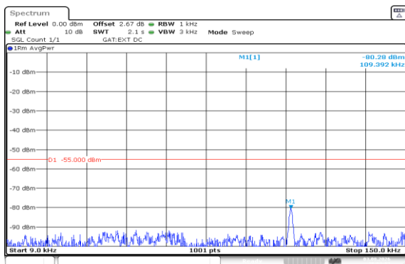
Band41(2535-2655)-5MHz-QPSK-41215-1RB#24-0.009~0.15-PASS
