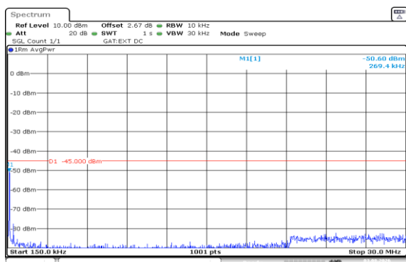
Band41(2535-2655)-5MHz-16QAM-40640-1RB#0-0.15~30-PASS
