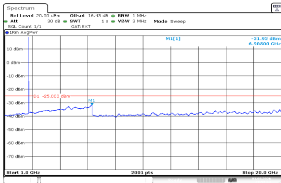
Band41(2535-2655)-5MHz-16QAM-41215-1RB#0-1000~20000-PASS
