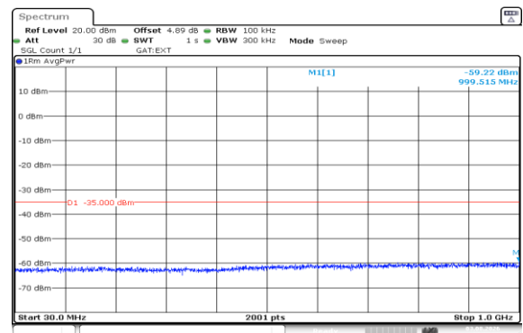
Band41(2535-2655)-5MHz-16QAM-40065-1RB#0-30~1000-PASS
