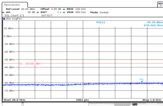
Band41(2535-2655)-5MHz-QPSK-40640-25RB#0-30~1000-PASS
