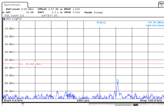
Band41(2535-2655)-10MHz-QPSK-41190-1RB#49-0.009~0.15-PASS
