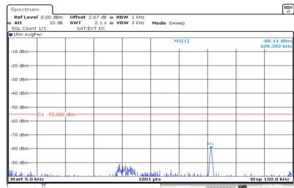
Band41(2535-2655)-10MHz-16QAM-41190-50RB#0-0.009~0.15-PASS
