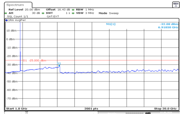
Band41(2535-2655)-5MHz-QPSK-41215-1RB#0-1000~20000-PASS
