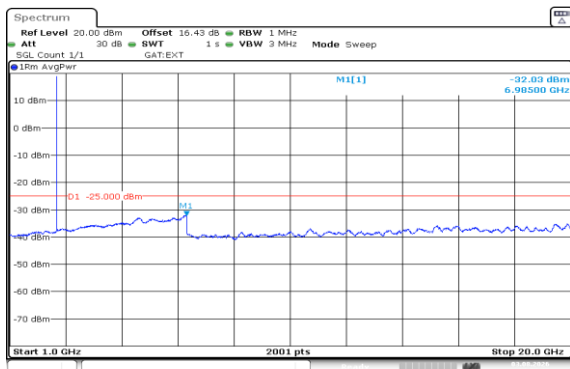
Band41(2535-2655)-10MHz-16QAM-40640-1RB#49-1000~20000-PASS
