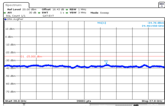
Band41(2535-2655)-10MHz-16QAM-40090-1RB#0-20000~27000-PASS
