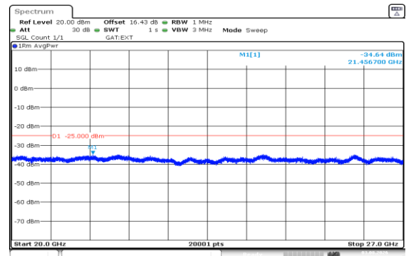
Band41(2535-2655)-5MHz-16QAM-41215-25RB#0-20000~27000-PASS
