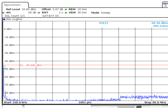
Band41(2535-2655)-5MHz-16QAM-40065-1RB#24-0.15~30-PASS
