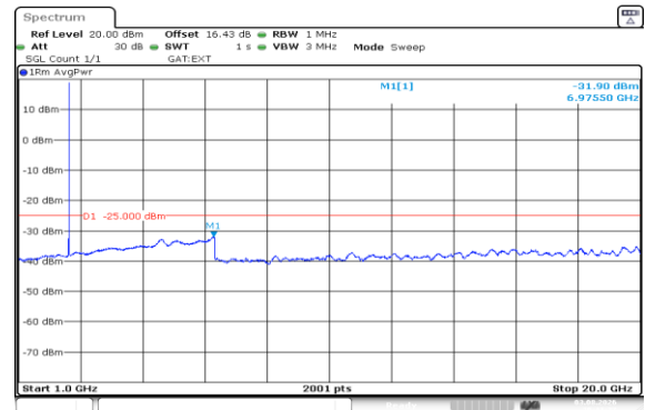
Band41(2535-2655)-5MHz-QPSK-40065-25RB#0-1000~20000-PASS
