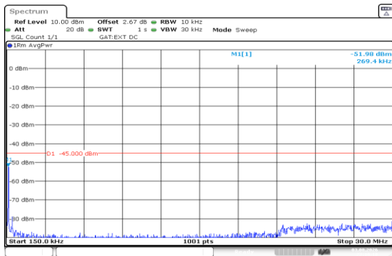
Band41(2535-2655)-10MHz-16QAM-41190-1RB#0-0.15~30-PASS
