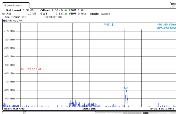
Band41(2535-2655)-10MHz-QPSK-41190-50RB#0-0.009~0.15-PASS
