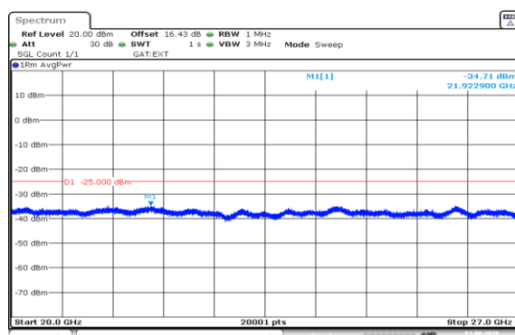
Band41(2535-2655)-5MHz-16QAM-40640-1RB#0-20000~27000-PASS
