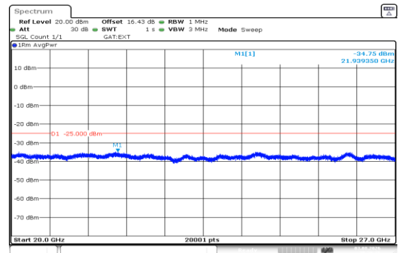
Band41(2535-2655)-5MHz-16QAM-40065-1RB#0-20000~27000-PASS
