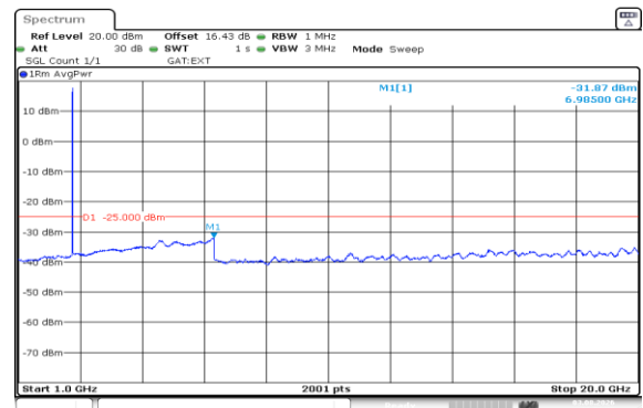
Band41(2535-2655)-5MHz-QPSK-41215-25RB#0-1000~20000-PASS
