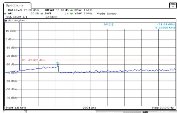
Band41(2535-2655)-10MHz-QPSK-41190-1RB#49-1000~20000-PASS
