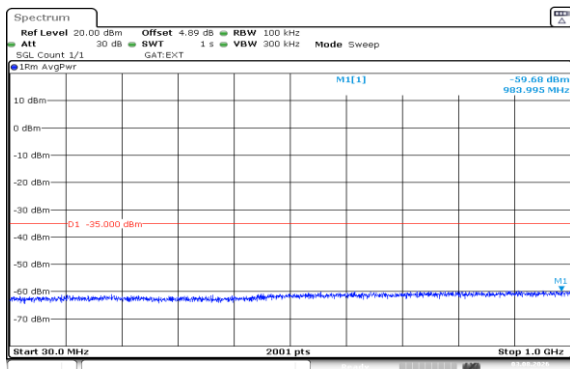
Band41(2535-2655)-5MHz-QPSK-41215-25RB#0-30~1000-PASS
