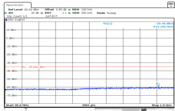
Band41(2535-2655)-5MHz-16QAM-40065-1RB#24-30~1000-PASS
