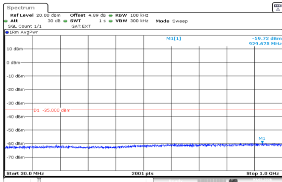
Band41(2535-2655)-5MHz-QPSK-41215-1RB#0-30~1000-PASS
