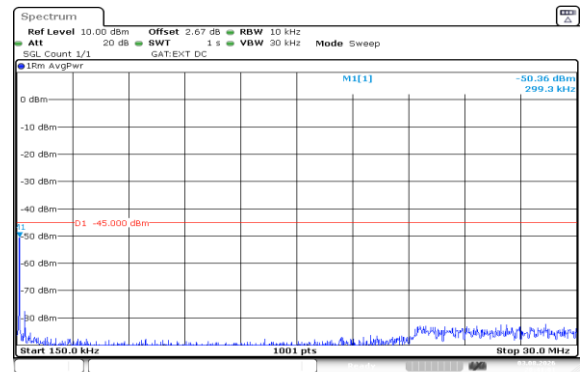
Band41(2535-2655)-5MHz-QPSK-40065-25RB#0-0.15~30-PASS
