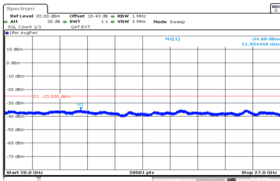
Band41(2535-2655)-5MHz-QPSK-41215-1RB#24-20000~27000-PASS
