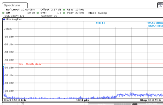
Band41(2535-2655)-5MHz-16QAM-40065-1RB#0-0.15~30-PASS
