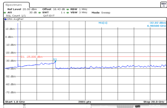
Band41(2535-2655)-5MHz-QPSK-40640-25RB#0-1000~20000-PASS
