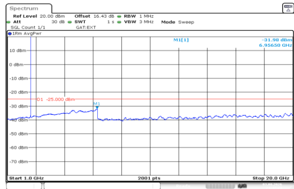
Band41(2535-2655)-10MHz-QPSK-40090-1RB#0-1000~20000-PASS
