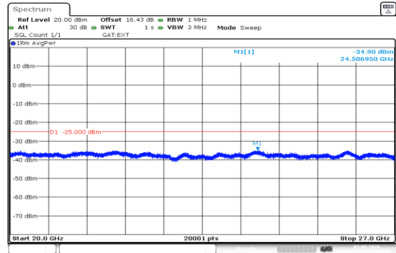
Band41(2535-2655)-5MHz-16QAM-40065-25RB#0-20000~27000-PASS
