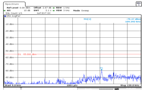
Band41(2535-2655)-10MHz-16QAM-40090-1RB#49-0.009~0.15-PASS
