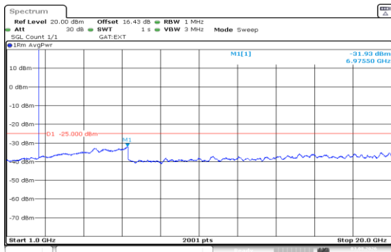
Band41(2535-2655)-5MHz-16QAM-40640-1RB#24-1000~20000-PASS
