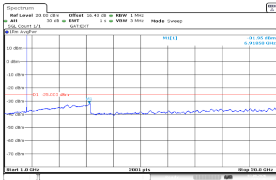
Band41(2535-2655)-10MHz-16QAM-40090-1RB#49-1000~20000-PASS
