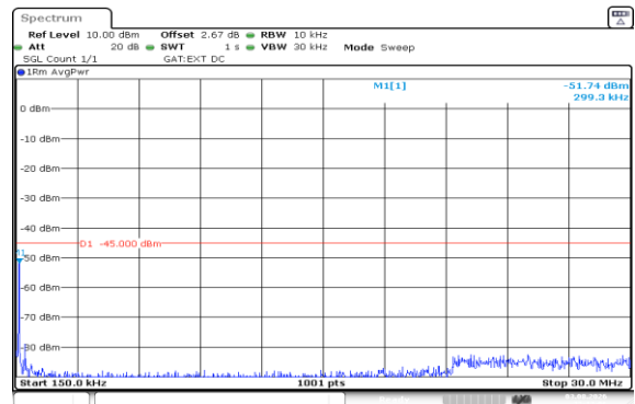
Band41(2535-2655)-10MHz-QPSK-41190-1RB#49-0.15~30-PASS
