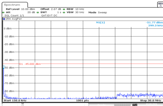
Band41(2535-2655)-5MHz-16QAM-41215-1RB#24-0.15~30-PASS
