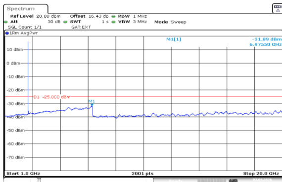
Band41(2535-2655)-5MHz-16QAM-40640-25RB#0-1000~20000-PASS
