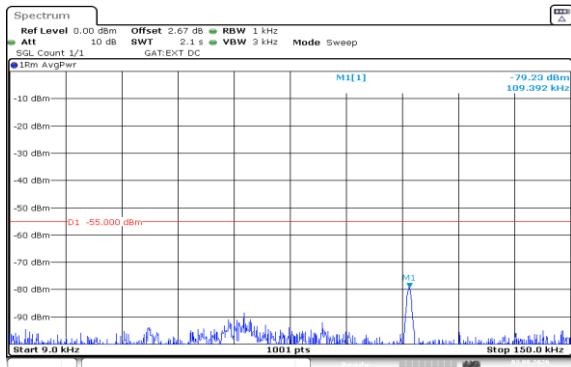
Band41(2535-2655)-5MHz-QPSK-40640-1RB#0-0.009~0.15-PASS
