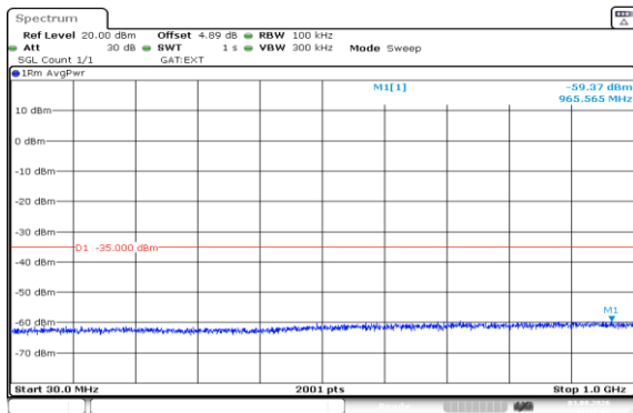
Band41(2535-2655)-10MHz-QPSK-40090-1RB#0-30~1000-PASS
