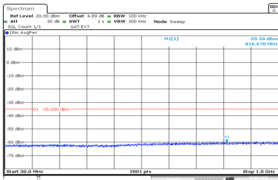
Band41(2535-2655)-20MHz-QPSK-40140-1RB#99-30~1000-PASS
