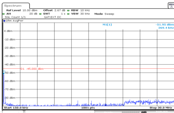
Band41(2535-2655)-20MHz-16QAM-40640-100RB#0-0.15~30-PASS
