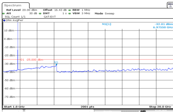
Band41(2535-2655)-15MHz-16QAM-41165-1RB#74-1000~20000-PASS
