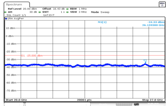
Band41(2535-2655)-20MHz-16QAM-41140-100RB#0-20000~27000-PASS
