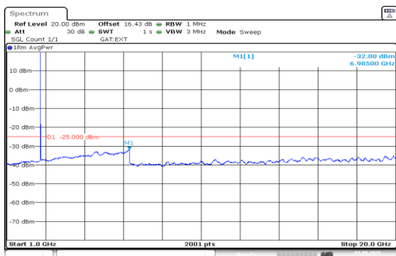
Band41(2535-2655)-15MHz-16QAM-41165-1RB#0-1000~20000-PASS
