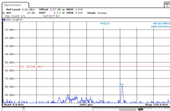
Band41(2535-2655)-15MHz-QPSK-40115-1RB#0-0.009~0.15-PASS
