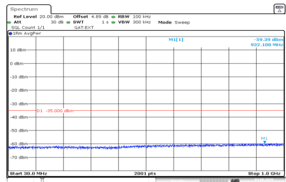
Band41(2535-2655)-20MHz-16QAM-40140-1RB#99-30~1000-PASS
