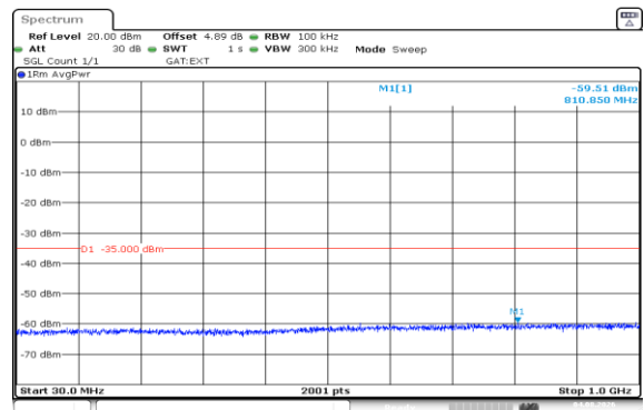
Band41(2535-2655)-20MHz-16QAM-40640-1RB#0-30~1000-PASS
