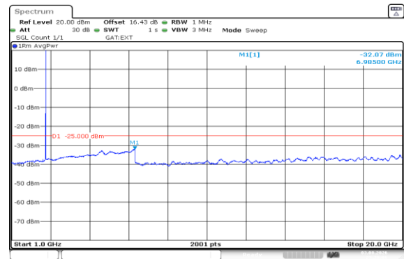
Band41(2535-2655)-15MHz-QPSK-41165-1RB#74-1000~20000-PASS
