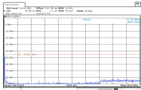
Band41(2535-2655)-15MHz-QPSK-40640-75RB#0-0.15~30-PASS
