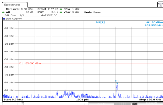
Band41(2535-2655)-15MHz-QPSK-41165-1RB#0-0.009~0.15-PASS
