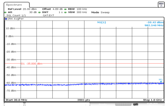
Band41(2535-2655)-20MHz-16QAM-40140-1RB#0-30~1000-PASS
