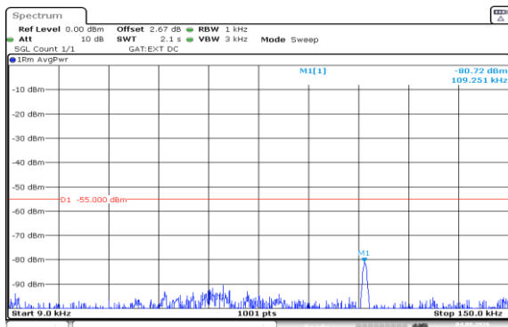
Band41(2535-2655)-20MHz-QPSK-41140-1RB#0-0.009~0.15-PASS
