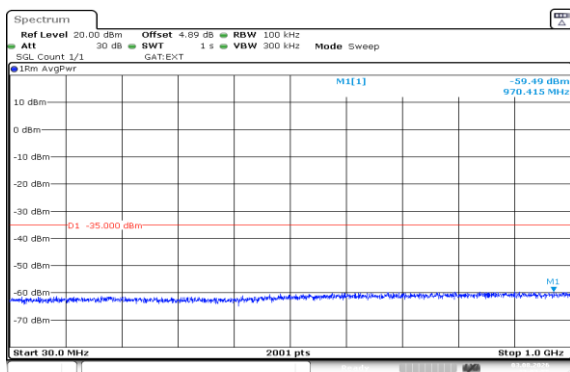
Band41(2535-2655)-15MHz-QPSK-40115-1RB#74-30~1000-PASS
