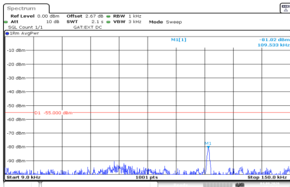
Band41(2535-2655)-20MHz-QPSK-40140-1RB#99-0.009~0.15-PASS
