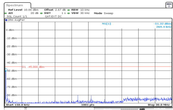
Band41(2535-2655)-20MHz-QPSK-40140-100RB#0-0.15~30-PASS
