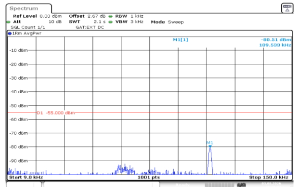
Band41(2535-2655)-15MHz-16QAM-41165-75RB#0-0.009~0.15-PASS
