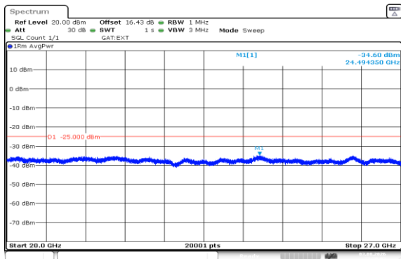
Band41(2535-2655)-15MHz-QPSK-41165-75RB#0-20000~27000-PASS
