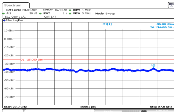
Band41(2535-2655)-15MHz-QPSK-40115-1RB#74-20000~27000-PASS
