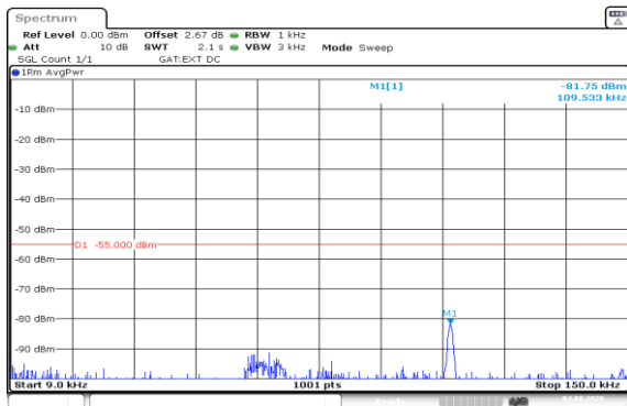
Band41(2535-2655)-20MHz-QPSK-40640-100RB#0-0.009~0.15-PASS
