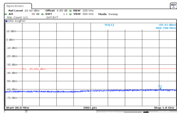
Band41(2535-2655)-20MHz-16QAM-40140-100RB#0-30~1000-PASS
