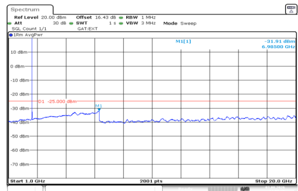
Band41(2535-2655)-15MHz-QPSK-40115-1RB#0-1000~20000-PASS
