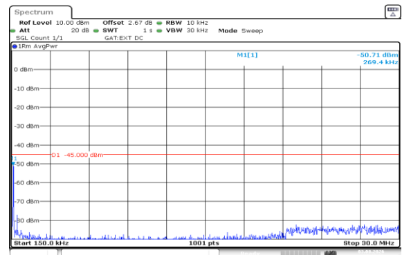
Band41(2535-2655)-15MHz-QPSK-40640-1RB#0-0.15~30-PASS
