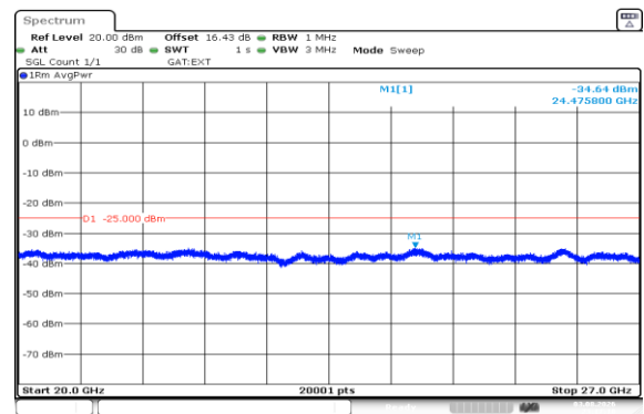
Band41(2535-2655)-15MHz-16QAM-40640-1RB#74-20000~27000-PASS
