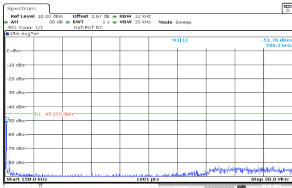
Band41(2535-2655)-20MHz-16QAM-41140-1RB#0-0.15~30-PASS
