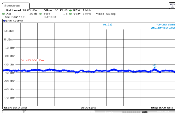
Band41(2535-2655)-20MHz-QPSK-40140-100RB#0-20000~27000-PASS
