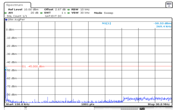
Band41(2535-2655)-15MHz-QPSK-40115-75RB#0-0.15~30-PASS
