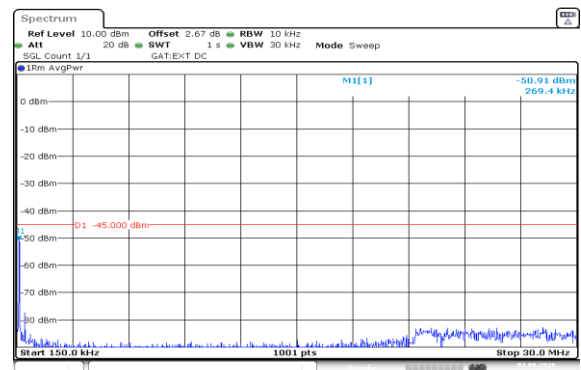
Band41(2535-2655)-15MHz-QPSK-40115-1RB#74-0.15~30-PASS
