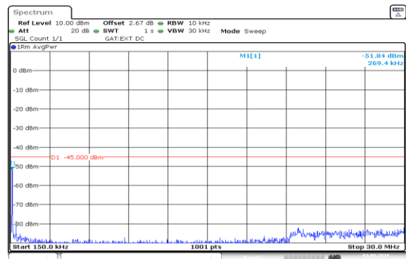
Band41(2535-2655)-15MHz-QPSK-41165-1RB#74-0.15~30-PASS
