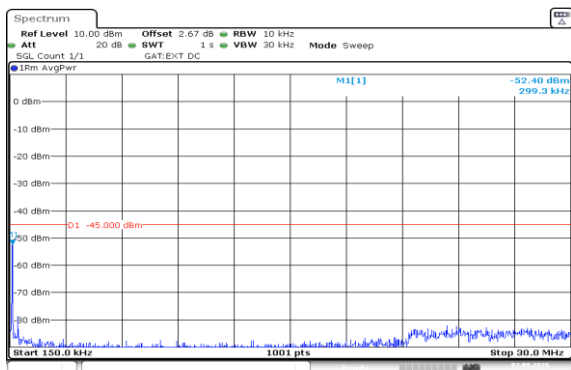
Band41(2535-2655)-15MHz-16QAM-41165-1RB#0-0.15~30-PASS
