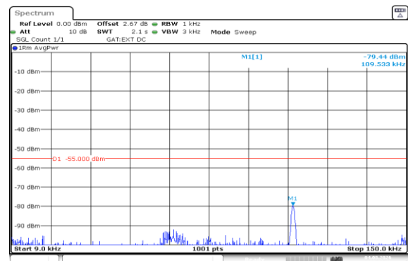
Band41(2535-2655)-20MHz-16QAM-40140-100RB#0-0.009~0.15-PASS
