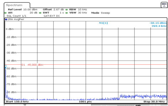
Band41(2535-2655)-20MHz-QPSK-41140-1RB#0-0.15~30-PASS
