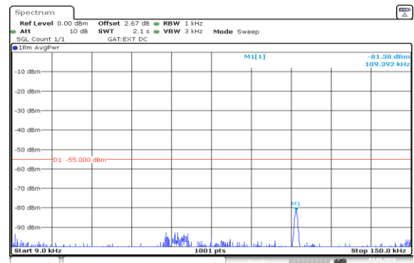
Band41(2535-2655)-20MHz-16QAM-41140-100RB#0-0.009~0.15-PASS
