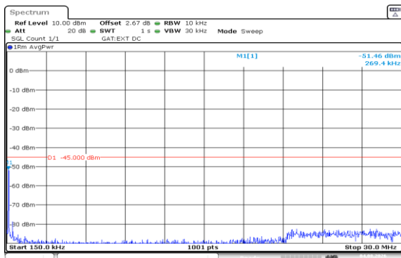
Band41(2535-2655)-20MHz-16QAM-41140-1RB#99-0.15~30-PASS
