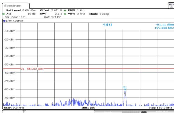
Band41(2535-2655)-20MHz-QPSK-40140-1RB#0-0.009~0.15-PASS
