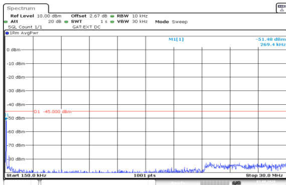
Band41(2535-2655)-15MHz-16QAM-40640-1RB#0-0.15~30-PASS
