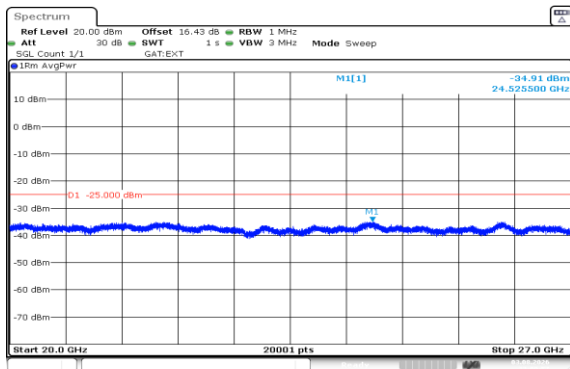
Band41(2535-2655)-15MHz-QPSK-40115-1RB#0-20000~27000-PASS
