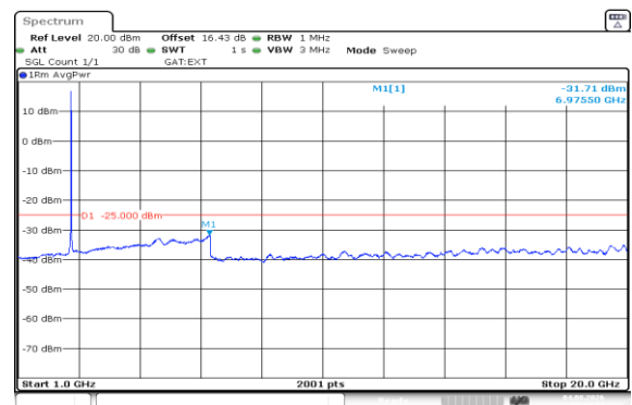
Band41(2535-2655)-20MHz-QPSK-41140-100RB#0-1000~20000-PASS
