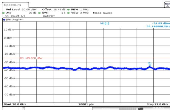
Band41(2535-2655)-20MHz-QPSK-40140-1RB#99-20000~27000-PASS
