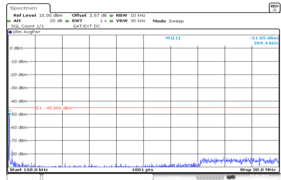
Band41(2535-2655)-15MHz-QPSK-40115-1RB#0-0.15~30-PASS
