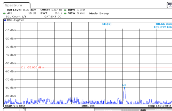
Band41(2535-2655)-20MHz-16QAM-40640-1RB#99-0.009~0.15-PASS
