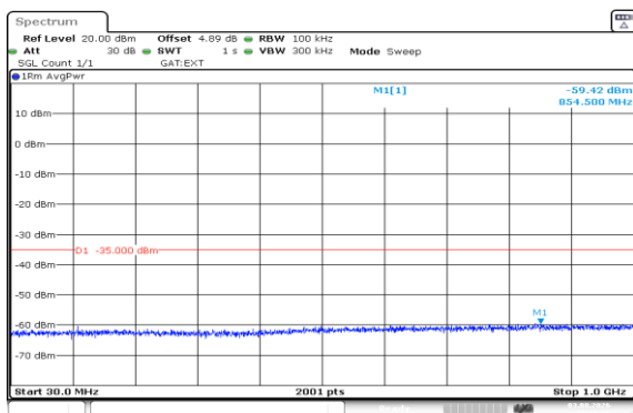
Band41(2535-2655)-15MHz-QPSK-40640-75RB#0-30~1000-PASS
