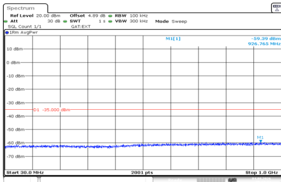
Band41(2535-2655)-20MHz-QPSK-40140-100RB#0-30~1000-PASS
