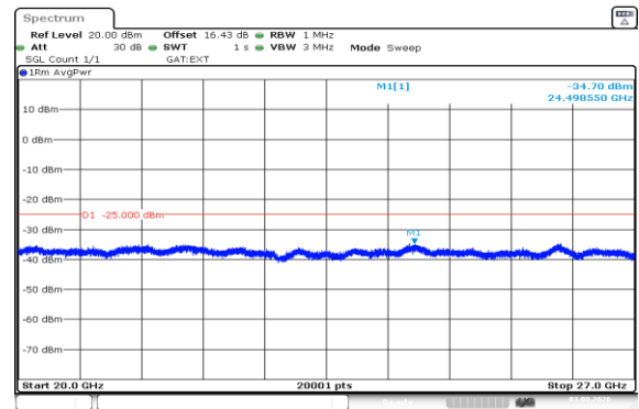
Band41(2535-2655)-15MHz-16QAM-41165-75RB#0-20000~27000-PASS
