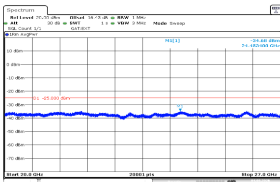
Band41(2535-2655)-20MHz-QPSK-40140-1RB#0-20000~27000-PASS
