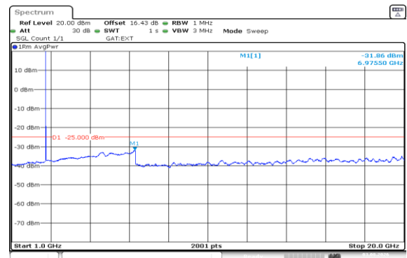
Band41(2535-2655)-15MHz-QPSK-41165-1RB#0-1000~20000-PASS
