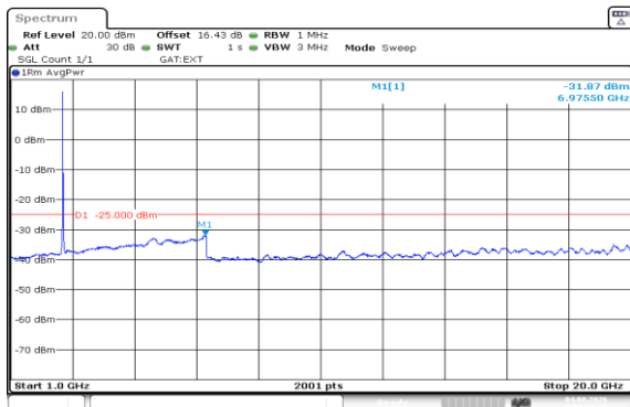
Band41(2535-2655)-20MHz-16QAM-40640-100RB#0-1000~20000-PASS
