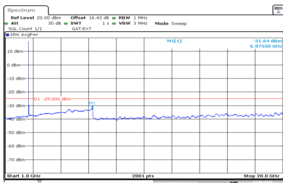
Band41(2535-2655)-20MHz-16QAM-40640-1RB#0-1000~20000-PASS
