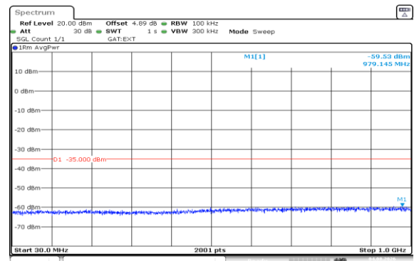
Band41(2535-2655)-20MHz-16QAM-41140-1RB#99-30~1000-PASS
