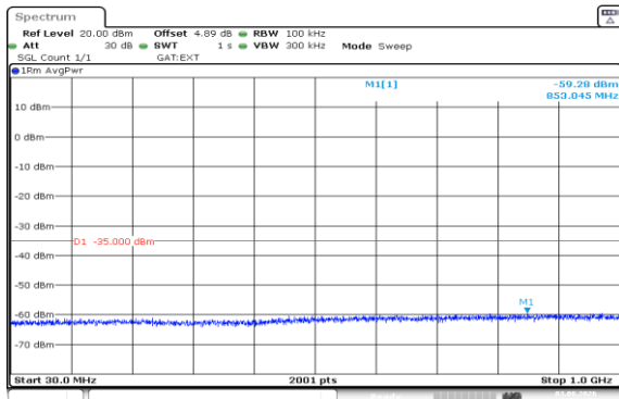
Band41(2535-2655)-15MHz-QPSK-40640-1RB#74-30~1000-PASS
