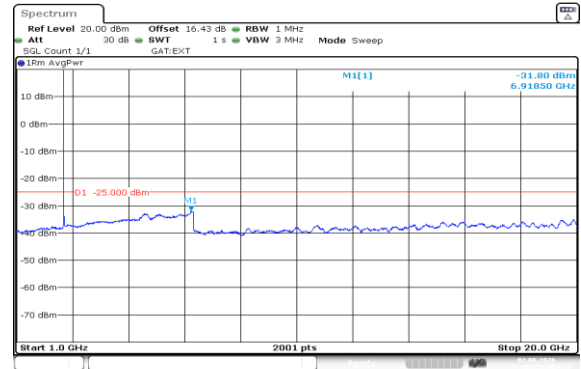
Band41(2535-2655)-15MHz-QPSK-40640-1RB#0-1000~20000-PASS
