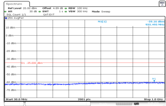
Band41(2535-2655)-20MHz-16QAM-41140-100RB#0-30~1000-PASS
