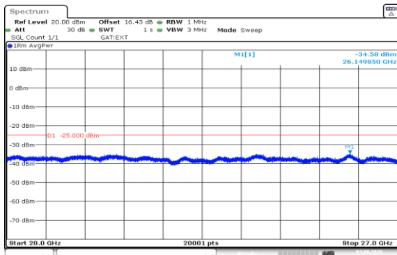
Band41(2535-2655)-20MHz-QPSK-41140-1RB#99-20000~27000-PASS
