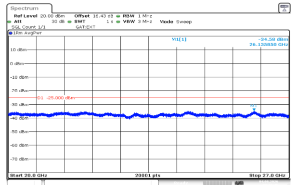
Band41(2535-2655)-20MHz-16QAM-40640-100RB#0-20000~27000-PASS
