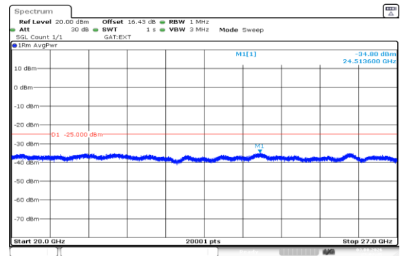
Band41(2535-2655)-15MHz-16QAM-40115-1RB#0-20000~27000-PASS
