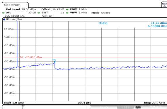
Band41(2535-2655)-20MHz-16QAM-41140-1RB#99-1000~20000-PASS
