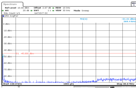
Band41(2535-2655)-15MHz-16QAM-41165-75RB#0-0.15~30-PASS
