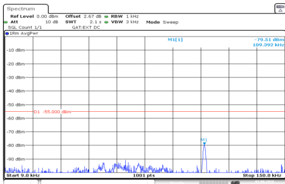
Band41(2535-2655)-15MHz-QPSK-40640-1RB#0-0.009~0.15-PASS
