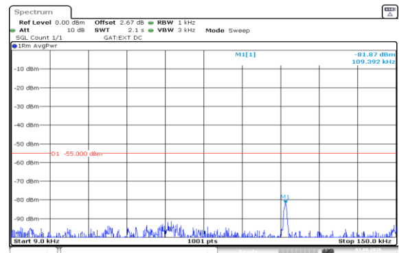
Band41(2535-2655)-15MHz-16QAM-40115-1RB#74-0.009~0.15-PASS
