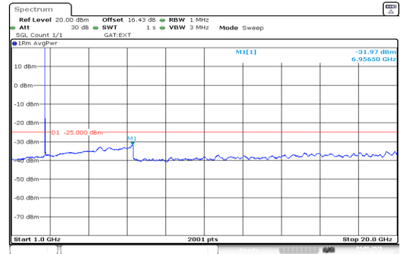
Band41(2535-2655)-20MHz-QPSK-41140-1RB#0-1000~20000-PASS
