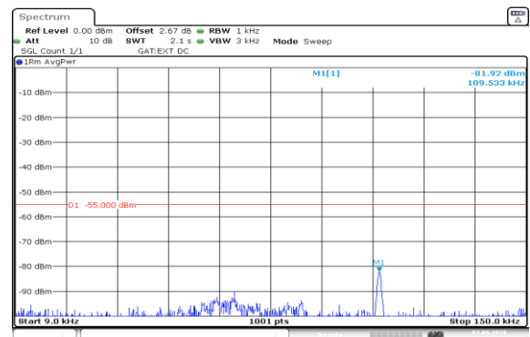
Band41(2535-2655)-15MHz-16QAM-40640-1RB#0-0.009~0.15-PASS
