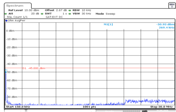
Band41(2535-2655)-20MHz-QPSK-40140-1RB#0-0.15~30-PASS
