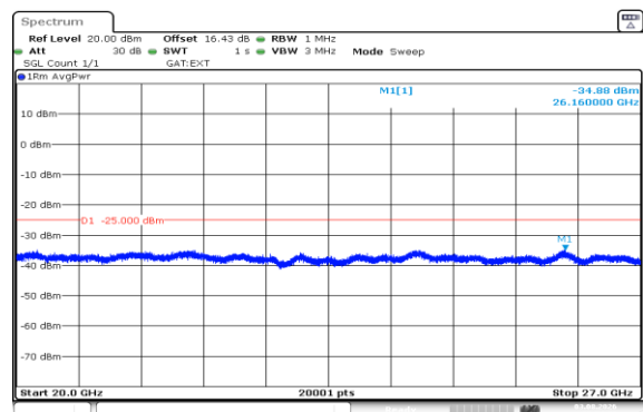
Band41(2535-2655)-15MHz-16QAM-41165-1RB#0-20000~27000-PASS
