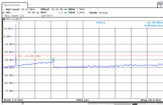
Band41(2535-2655)-20MHz-16QAM-40140-100RB#0-1000~20000-PASS
