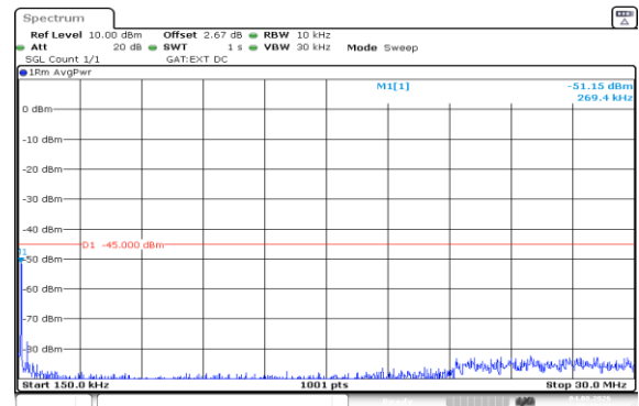
Band41(2535-2655)-20MHz-QPSK-40140-1RB#99-0.15~30-PASS
