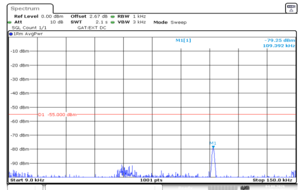
Band41(2535-2655)-20MHz-16QAM-40640-100RB#0-0.009~0.15-PASS
