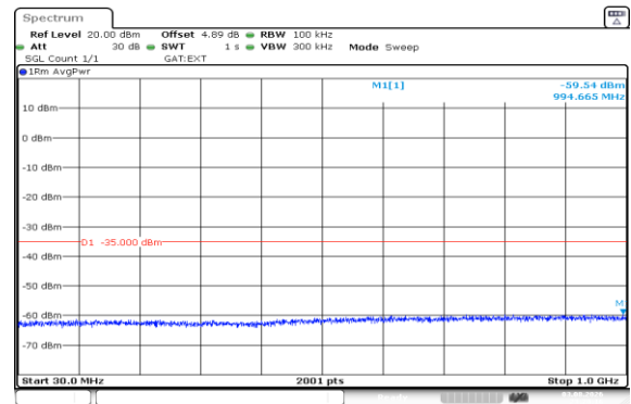
Band41(2535-2655)-15MHz-16QAM-40640-75RB#0-30~1000-PASS
