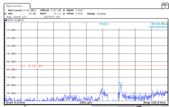
Band41(2535-2655)-20MHz-16QAM-40140-1RB#0-0.009~0.15-PASS
