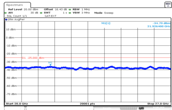
Band41(2535-2655)-20MHz-16QAM-41140-1RB#99-20000~27000-PASS
