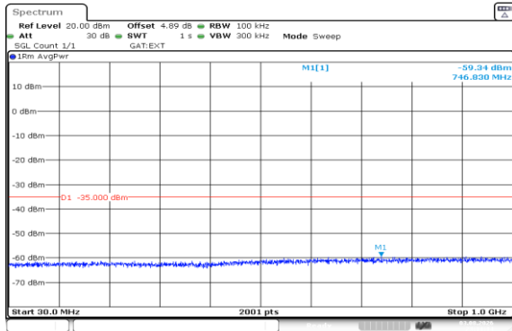
Band41(2535-2655)-15MHz-QPSK-40640-1RB#0-30~1000-PASS
