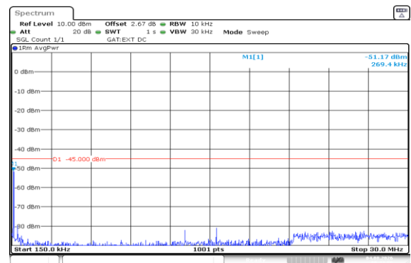
Band41(2535-2655)-20MHz-QPSK-41140-100RB#0-0.15~30-PASS
