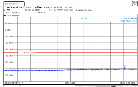
Band41(2535-2655)-15MHz-16QAM-40640-1RB#74-30~1000-PASS
