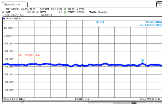
Band41(2535-2655)-20MHz-QPSK-41140-1RB#0-20000~27000-PASS
