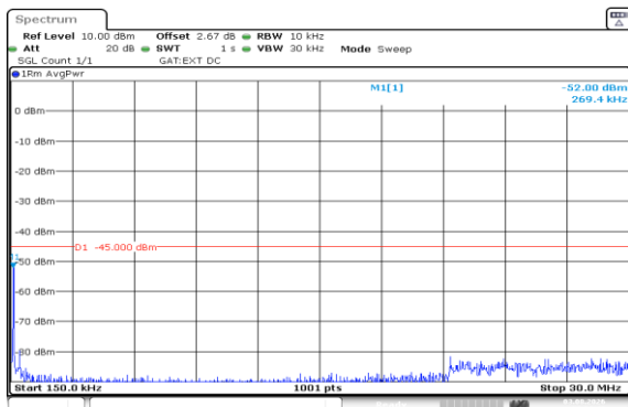
Band41(2535-2655)-15MHz-16QAM-40115-1RB#0-0.15~30-PASS
