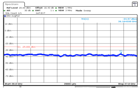
Band41(2535-2655)-15MHz-16QAM-40640-1RB#0-20000~27000-PASS
