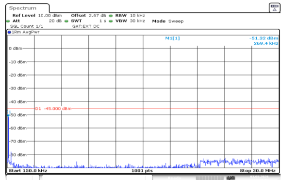
Band41(2535-2655)-15MHz-QPSK-41165-75RB#0-0.15~30-PASS
