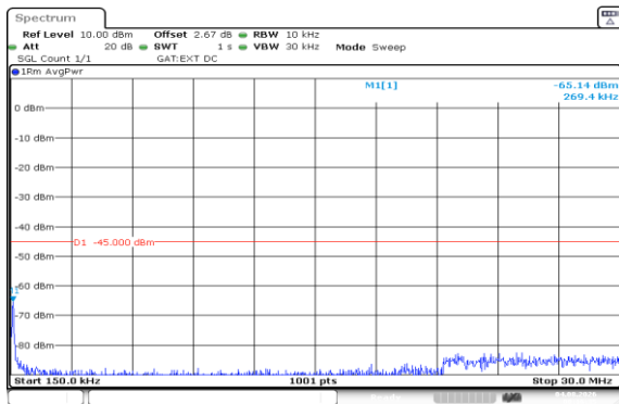
Band41(2535-2655)-20MHz-16QAM-40140-1RB#0-0.15~30-PASS
