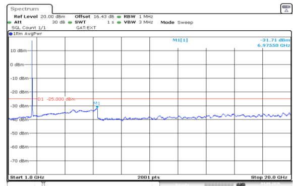
Band41(2535-2655)-20MHz-QPSK-40640-100RB#0-1000~20000-PASS
