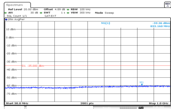
Band41(2535-2655)-15MHz-16QAM-41165-1RB#74-30~1000-PASS
