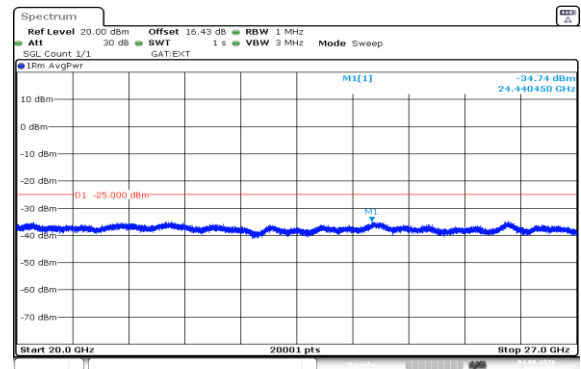
Band41(2535-2655)-20MHz-16QAM-40140-1RB#99-20000~27000-PASS
