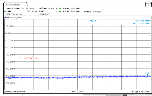
Band41(2535-2655)-15MHz-16QAM-40115-1RB#0-30~1000-PASS
