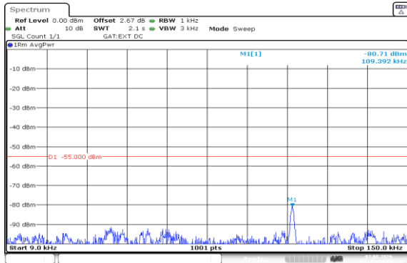
Band41(2535-2655)-15MHz-QPSK-40640-1RB#74-0.009~0.15-PASS
