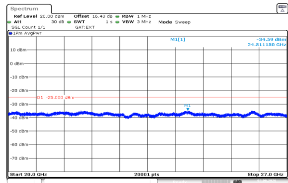
Band41(2535-2655)-15MHz-16QAM-41165-1RB#74-20000~27000-PASS
