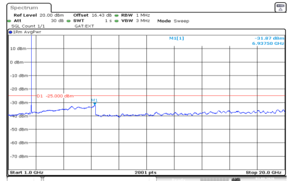
Band41(2535-2655)-15MHz-QPSK-40640-1RB#74-1000~20000-PASS
