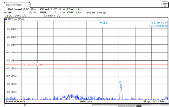
Band41(2535-2655)-15MHz-16QAM-40115-1RB#0-0.009~0.15-PASS
