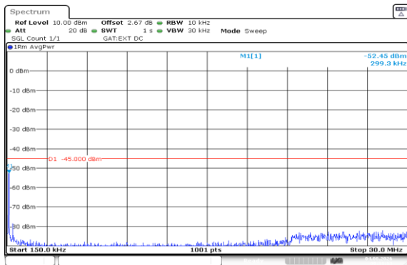
Band41(2535-2655)-20MHz-16QAM-40640-1RB#99-0.15~30-PASS
