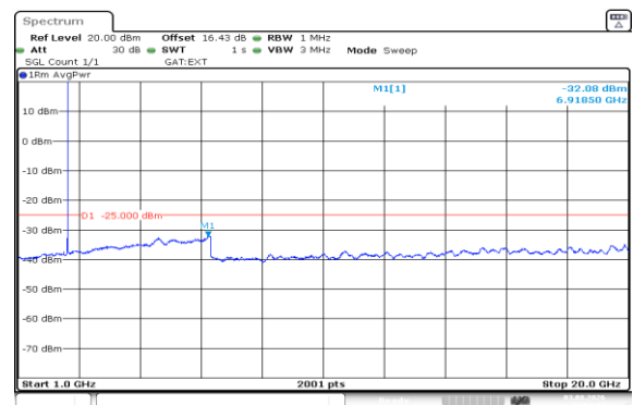
Band41(2535-2655)-15MHz-QPSK-40115-1RB#74-1000~20000-PASS
