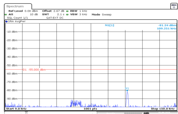
Band41(2535-2655)-15MHz-16QAM-40640-75RB#0-0.009~0.15-PASS
