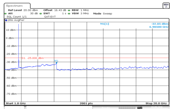
Band41(2535-2655)-15MHz-QPSK-40640-75RB#0-1000~20000-PASS
