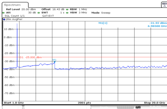
Band41(2535-2655)-15MHz-16QAM-41165-75RB#0-1000~20000-PASS
