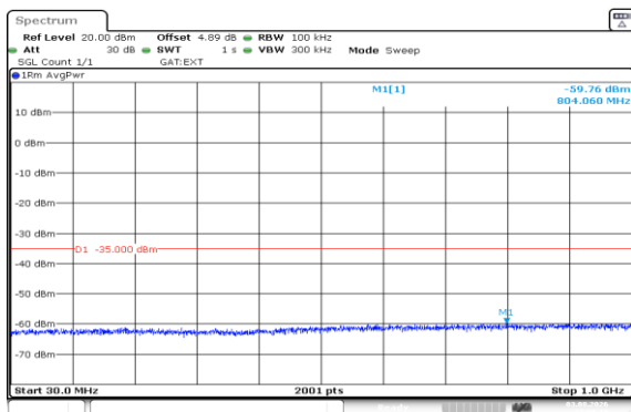
Band41(2535-2655)-15MHz-QPSK-40115-1RB#0-30~1000-PASS
