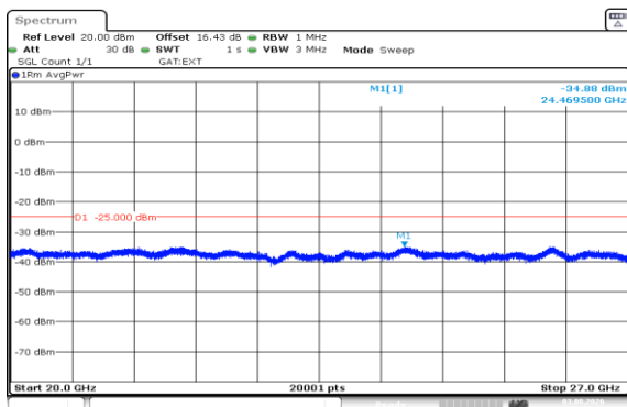
Band41(2535-2655)-15MHz-QPSK-40640-1RB#0-20000~27000-PASS
