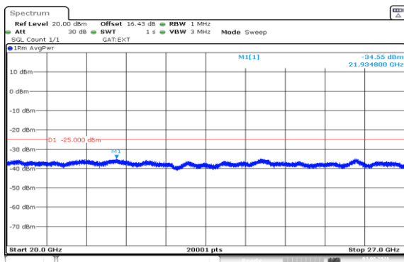
Band41(2535-2655)-15MHz-QPSK-41165-1RB#74-20000~27000-PASS
