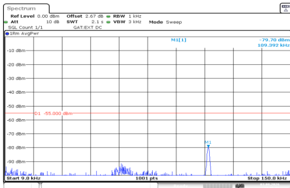
Band41(2535-2655)-15MHz-QPSK-40115-75RB#0-0.009~0.15-PASS
