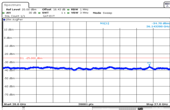
Band41(2535-2655)-15MHz-QPSK-41165-1RB#0-20000~27000-PASS
