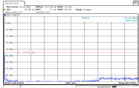
Band41(2535-2655)-15MHz-QPSK-40640-1RB#74-0.15~30-PASS
