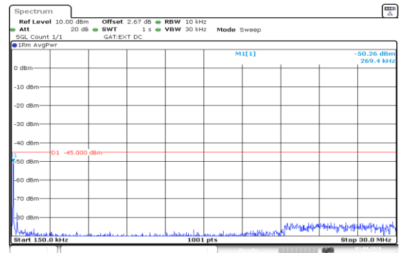
Band41(2535-2655)-15MHz-QPSK-41165-1RB#0-0.15~30-PASS
