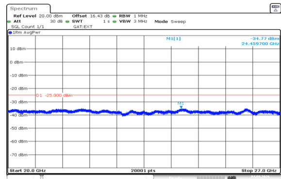
Band41(2535-2655)-20MHz-16QAM-40140-100RB#0-20000~27000-PASS
