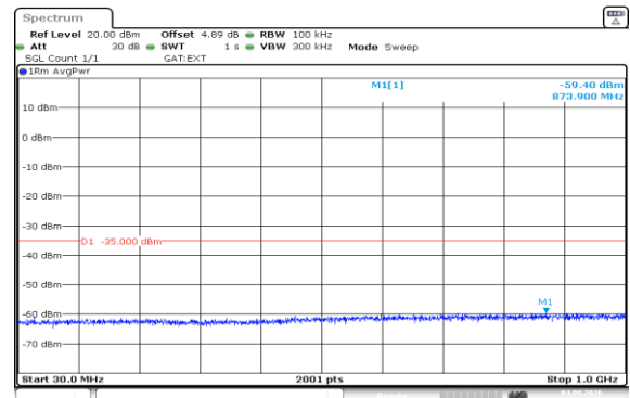
Band41(2535-2655)-20MHz-16QAM-41140-1RB#0-30~1000-PASS
