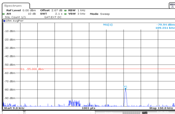
Band41(2535-2655)-15MHz-QPSK-40640-75RB#0-0.009~0.15-PASS
