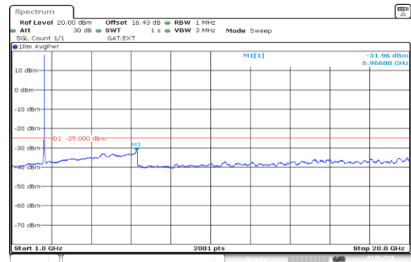
Band41(2535-2655)-20MHz-QPSK-40140-100RB#0-1000~20000-PASS
