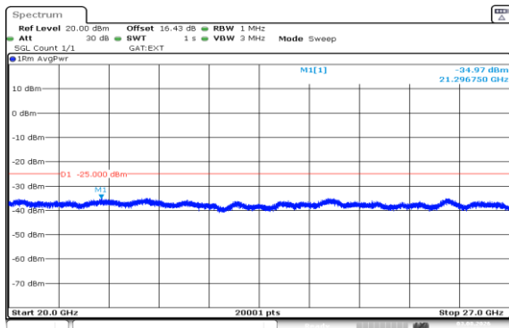
Band41(2535-2655)-15MHz-QPSK-40640-1RB#74-20000~27000-PASS
