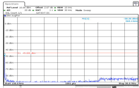
Band41(2535-2655)-20MHz-QPSK-41140-1RB#99-0.15~30-PASS
