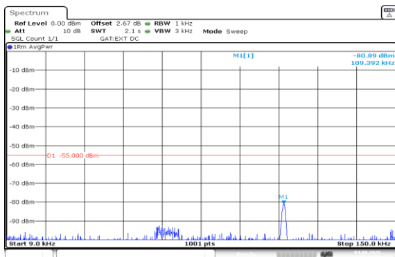
Band41(2535-2655)-20MHz-QPSK-41140-100RB#0-0.009~0.15-PASS
