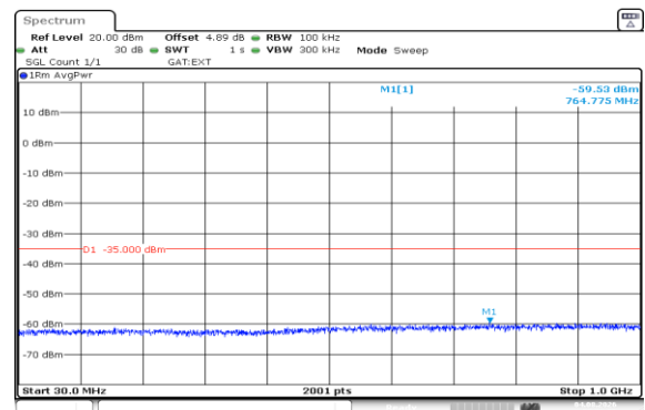
Band41(2535-2655)-20MHz-16QAM-40640-100RB#0-30~1000-PASS
