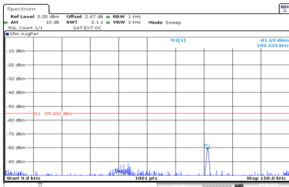
Band41(2535-2655)-20MHz-QPSK-40140-100RB#0-0.009~0.15-PASS
