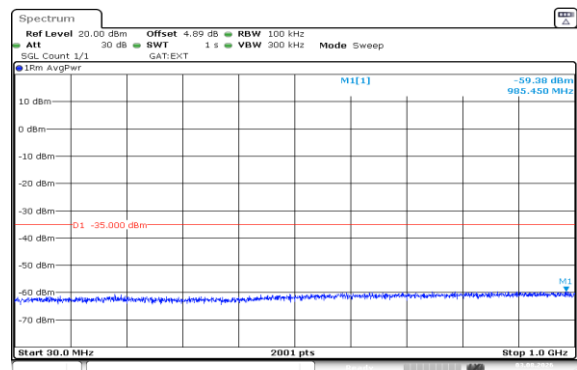
Band41(2535-2655)-15MHz-16QAM-41165-1RB#0-30~1000-PASS
