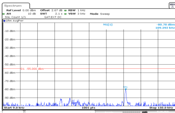
Band41(2535-2655)-15MHz-QPSK-40115-1RB#74-0.009~0.15-PASS
