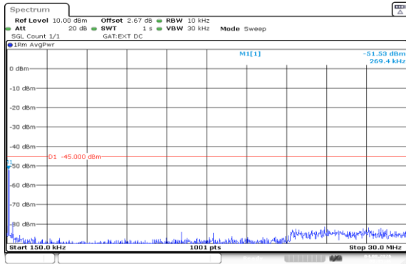
Band41(2535-2655)-20MHz-16QAM-41140-100RB#0-0.15~30-PASS
