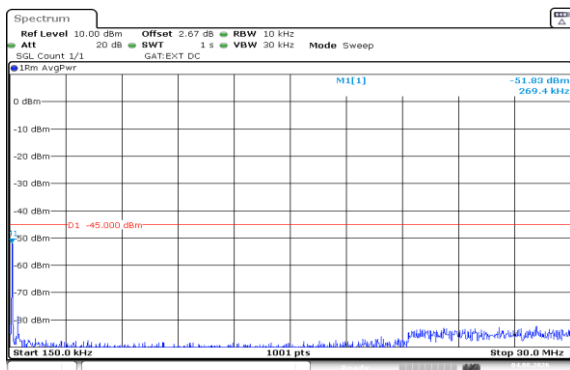
Band41(2535-2655)-20MHz-16QAM-40140-1RB#99-0.15~30-PASS
