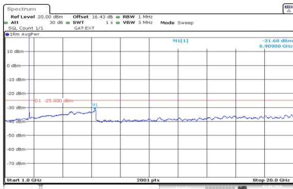
Band41(2535-2655)-15MHz-16QAM-40640-1RB#0-1000~20000-PASS
