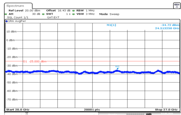
Band41(2535-2655)-20MHz-16QAM-40140-1RB#0-20000~27000-PASS
