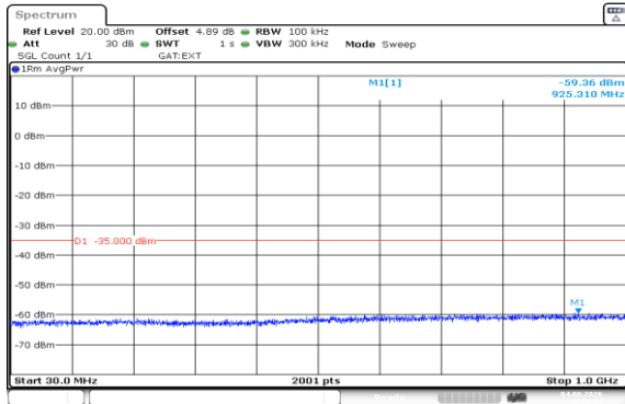
Band41(2535-2655)-20MHz-QPSK-41140-1RB#0-30~1000-PASS
