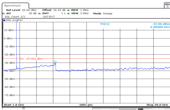
Band41(2535-2655)-20MHz-16QAM-40140-1RB#0-1000~20000-PASS
