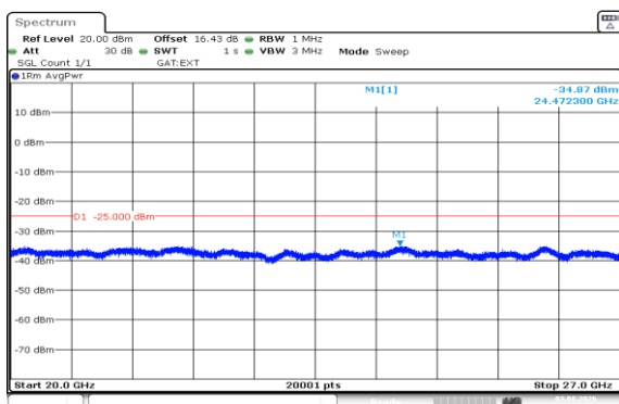
Band41(2535-2655)-15MHz-QPSK-40640-75RB#0-20000~27000-PASS
