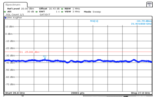
Band41(2535-2655)-20MHz-16QAM-41140-1RB#0-20000~27000-PASS
