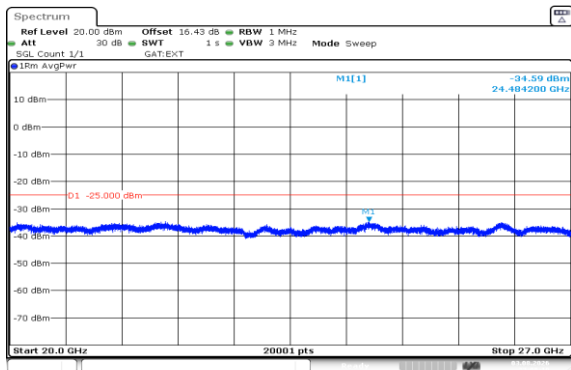
Band41(2535-2655)-15MHz-QPSK-40115-75RB#0-20000~27000-PASS
