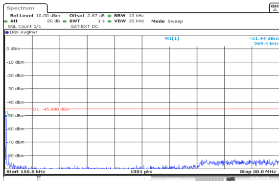
Band41(2535-2655)-15MHz-16QAM-41165-1RB#74-0.15~30-PASS
