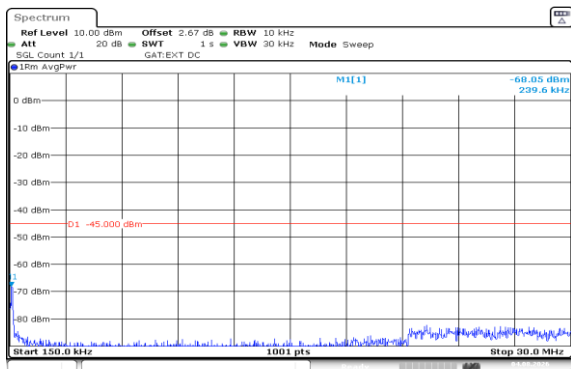
Band41(2535-2655)-20MHz-16QAM-40640-1RB#0-0.15~30-PASS
