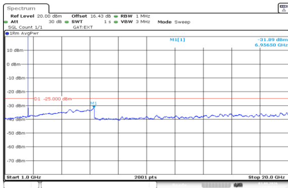
Band41(2535-2655)-15MHz-16QAM-40115-1RB#0-1000~20000-PASS
