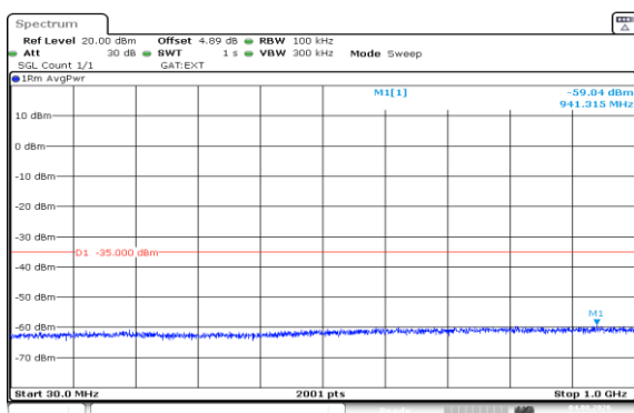
Band41(2535-2655)-20MHz-QPSK-40140-1RB#0-30~1000-PASS
