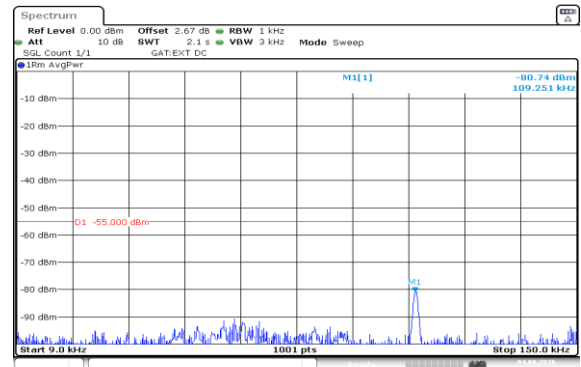
Band41(2535-2655)-20MHz-16QAM-41140-1RB#0-0.009~0.15-PASS
