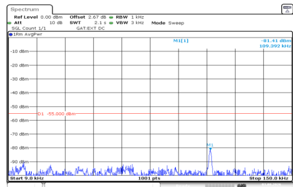
Band41(2535-2655)-15MHz-16QAM-41165-1RB#74-0.009~0.15-PASS
