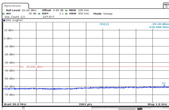
Band41(2535-2655)-20MHz-QPSK-41140-100RB#0-30~1000-PASS
