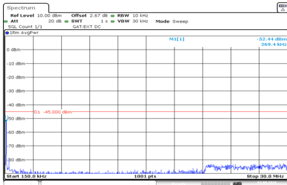
Band41(2535-2655)-15MHz-16QAM-40640-1RB#74-0.15~30-PASS
