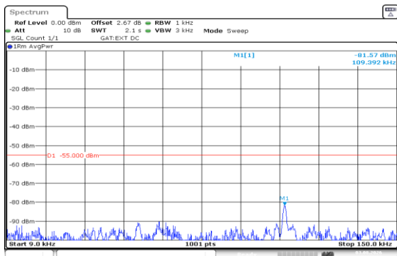
Band41(2535-2655)-15MHz-QPSK-41165-1RB#74-0.009~0.15-PASS
