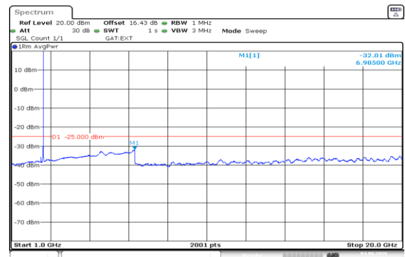
Band41(2535-2655)-20MHz-QPSK-40140-1RB#99-1000~20000-PASS
