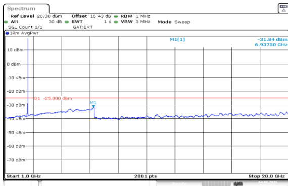
Band41(2535-2655)-20MHz-16QAM-40140-1RB#99-1000~20000-PASS
