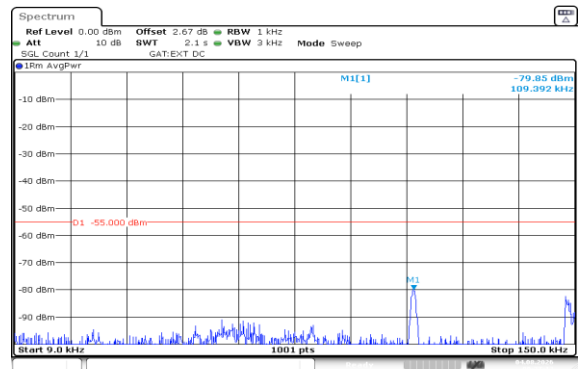
Band41(2535-2655)-20MHz-16QAM-40640-1RB#0-0.009~0.15-PASS
