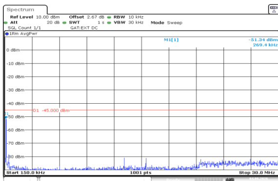
Band41(2535-2655)-20MHz-16QAM-40140-100RB#0-0.15~30-PASS
