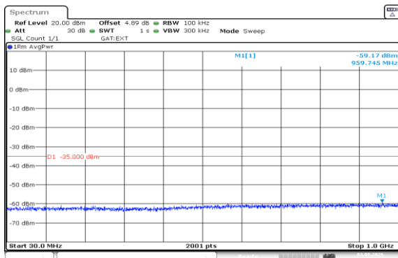
Band41(2535-2655)-15MHz-QPSK-41165-1RB#0-30~1000-PASS
