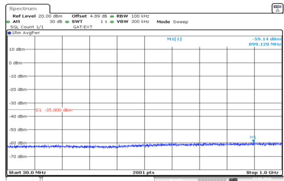
Band41(2535-2655)-15MHz-16QAM-41165-75RB#0-30~1000-PASS
