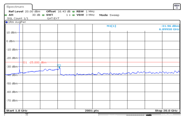
Band41(2535-2655)-20MHz-QPSK-40140-1RB#0-1000~20000-PASS
