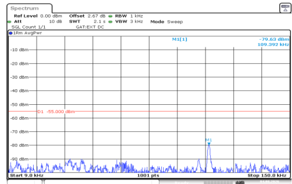
Band41(2535-2655)-20MHz-16QAM-41140-1RB#99-0.009~0.15-PASS
