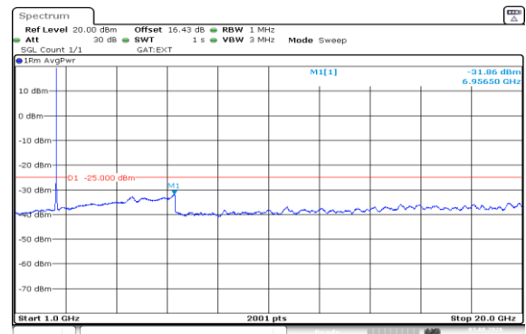
Band41(2535-2655)-15MHz-QPSK-40115-75RB#0-1000~20000-PASS
