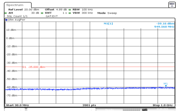
Band41(2535-2655)-15MHz-16QAM-40640-1RB#0-30~1000-PASS
