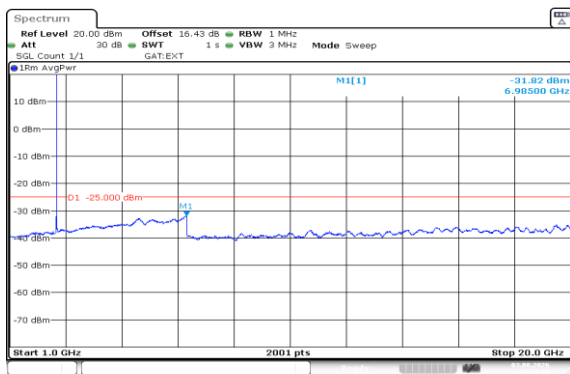
Band41(2535-2655)-15MHz-16QAM-40640-1RB#74-1000~20000-PASS
