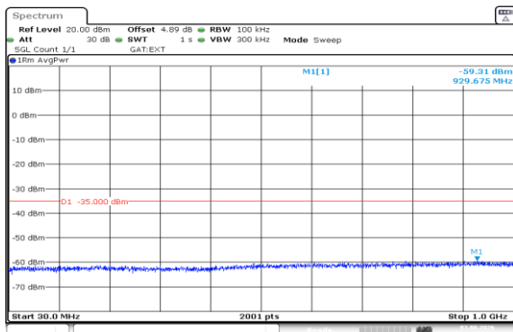
Band41(2535-2655)-15MHz-QPSK-40115-75RB#0-30~1000-PASS
