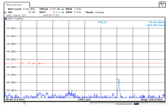
Band41(2535-2655)-20MHz-16QAM-40140-1RB#99-0.009~0.15-PASS
