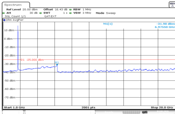
Band41(2535-2655)-20MHz-16QAM-41140-100RB#0-1000~20000-PASS
