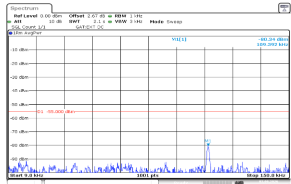
Band41(2535-2655)-15MHz-16QAM-40640-1RB#74-0.009~0.15-PASS
