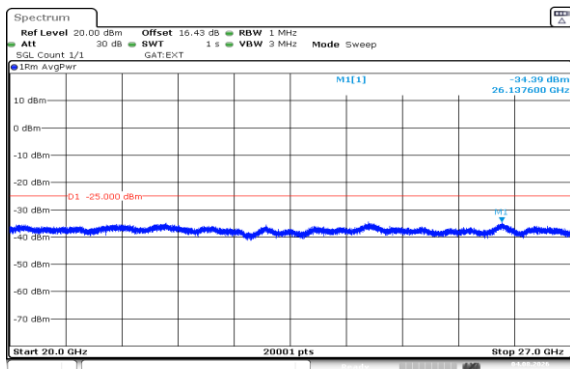
Band41(2535-2655)-20MHz-QPSK-41140-100RB#0-20000~27000-PASS
