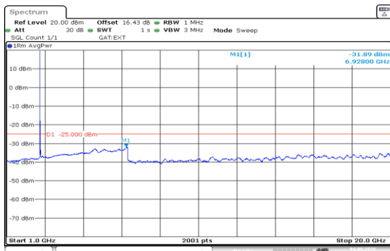
Band41(2535-2655)-20MHz-16QAM-41140-1RB#0-1000~20000-PASS
