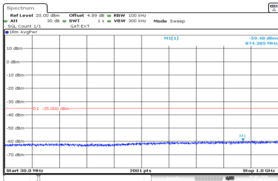
Band41(2535-2655)-15MHz-QPSK-41165-1RB#74-30~1000-PASS
