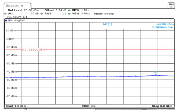
Band5-3MHz-QPSK-20635-1RB#14-1000~3000-PASS
