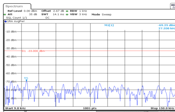
Band5-1.4MHz-16QAM-20407-6RB#0-0.009~0.15-PASS
