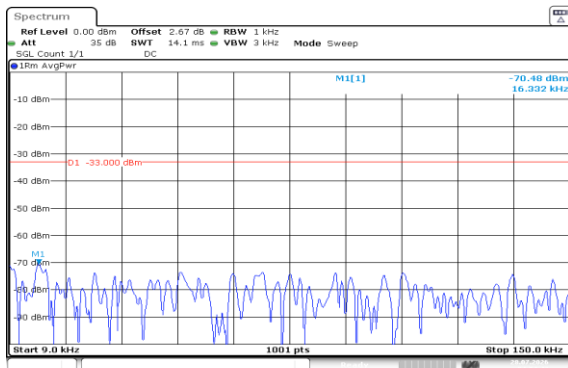
Band5-1.4MHz-QPSK-20407-1RB#5-0.009~0.15-PASS
