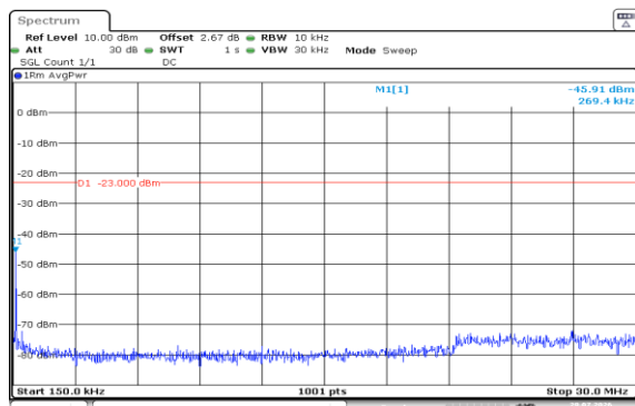
Band5-3MHz-16QAM-20525-15RB#0-0.15~30-PASS
