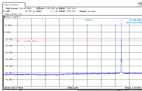
Band5-1.4MHz-16QAM-20643-1RB#0-30~1000-PASS
