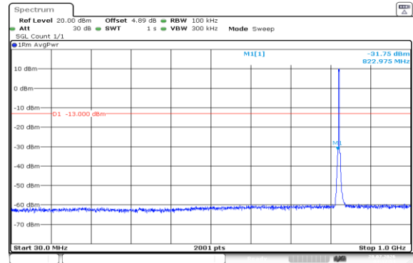
Band5-3MHz-16QAM-20415-15RB#0-30~1000-PASS
