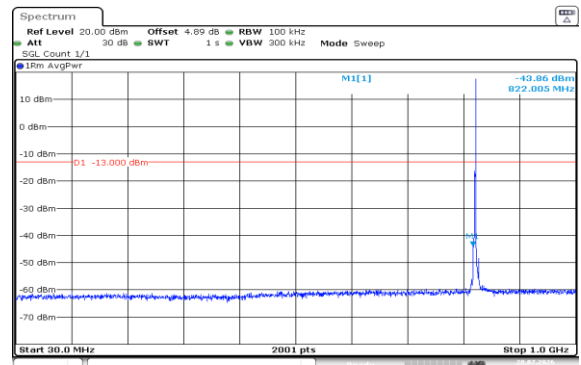
Band5-3MHz-16QAM-20415-1RB#14-30~1000-PASS
