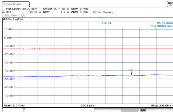
Band5-3MHz-16QAM-20525-15RB#0-1000~3000-PASS
