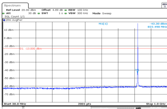
Band5-1.4MHz-QPSK-20407-1RB#0-30~1000-PASS
