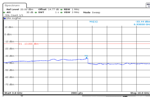
Band5-3MHz-16QAM-20415-1RB#0-3000~10000-PASS
