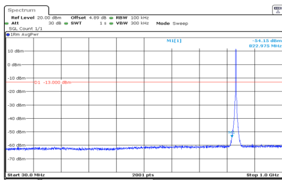
Band5-3MHz-QPSK-20525-15RB#0-30~1000-PASS
