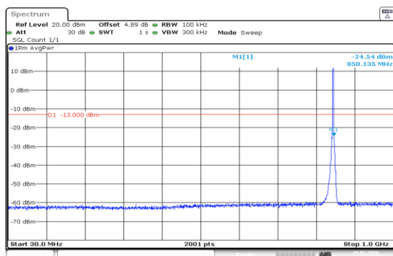
Band5-3MHz-QPSK-20635-15RB#0-30~1000-PASS
