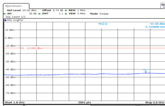
Band5-3MHz-QPSK-20415-15RB#0-1000~3000-PASS
