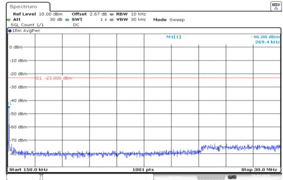
Band5-3MHz-QPSK-20415-1RB#14-0.15~30-PASS
