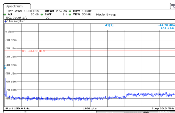
Band5-1.4MHz-QPSK-20643-1RB#0-0.15~30-PASS
