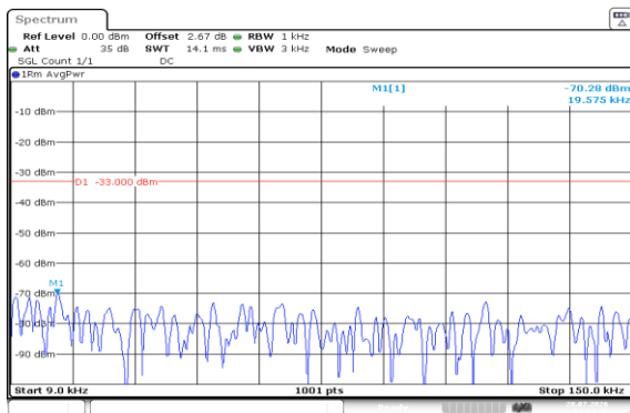
Band5-1.4MHz-QPSK-20407-1RB#0-0.009~0.15-PASS
