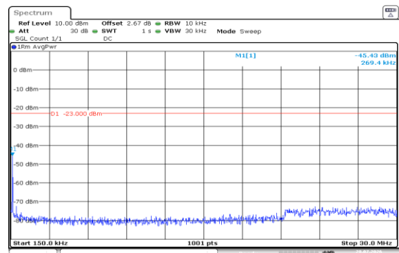
Band5-3MHz-QPSK-20635-1RB#14-0.15~30-PASS
