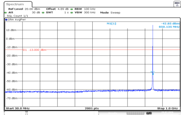
Band5-1.4MHz-16QAM-20643-1RB#5-30~1000-PASS
