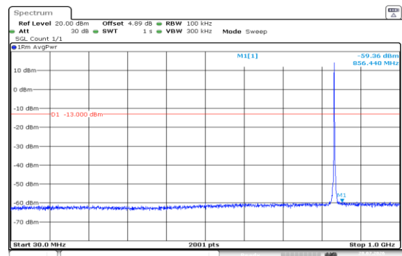
Band5-1.4MHz-16QAM-20525-6RB#0-30~1000-PASS
