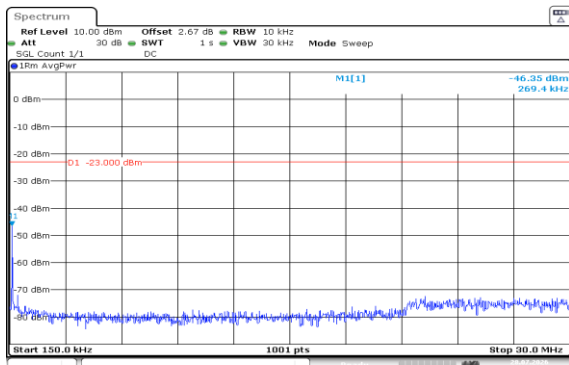
Band5-3MHz-16QAM-20415-1RB#14-0.15~30-PASS
