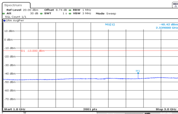
Band5-3MHz-16QAM-20635-1RB#0-1000~3000-PASS
