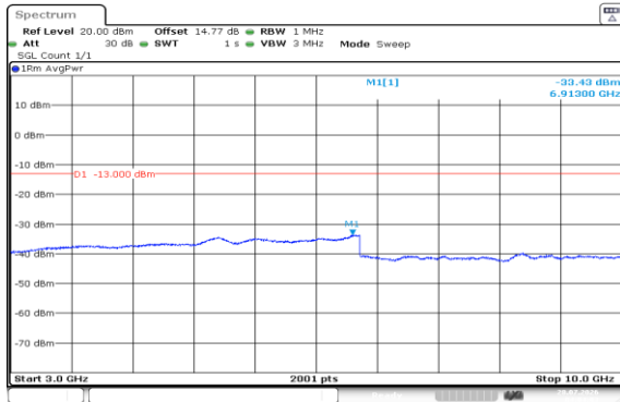
Band5-1.4MHz-QPSK-20407-1RB#0-3000~10000-PASS
