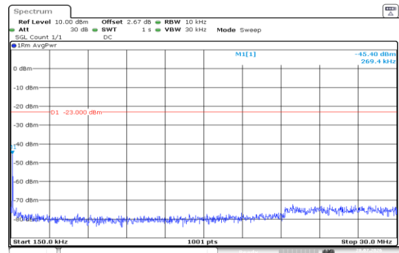
Band5-1.4MHz-QPSK-20525-1RB#5-0.15~30-PASS
