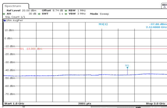
Band5-3MHz-16QAM-20525-1RB#14-1000~3000-PASS
