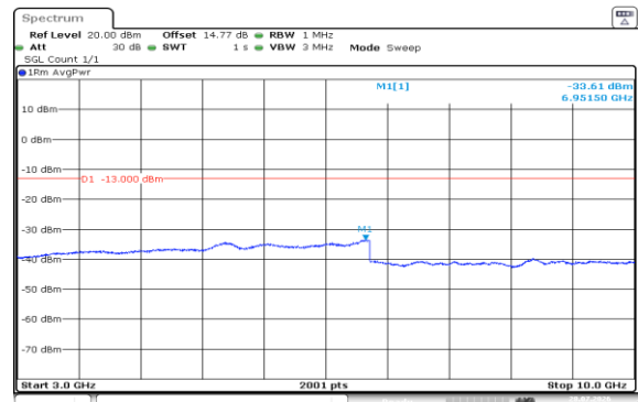
Band5-3MHz-16QAM-20635-1RB#0-3000~10000-PASS
