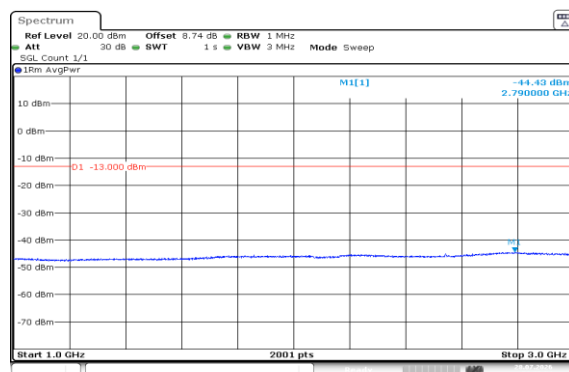
Band5-3MHz-QPSK-20635-15RB#0-1000~3000-PASS
