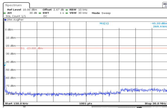
Band5-1.4MHz-QPSK-20407-6RB#0-0.15~30-PASS
