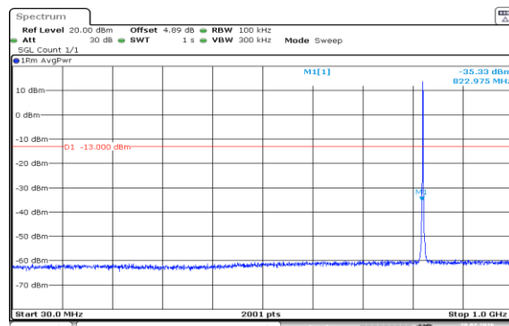
Band5-1.4MHz-16QAM-20407-6RB#0-30~1000-PASS
