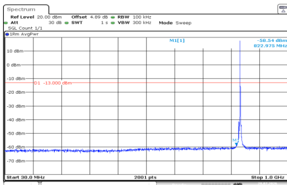
Band5-3MHz-QPSK-20525-1RB#0-30~1000-PASS
