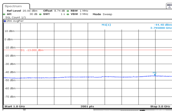
Band5-3MHz-16QAM-20635-15RB#0-1000~3000-PASS
