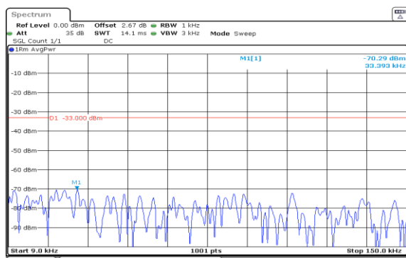
Band5-3MHz-QPSK-20415-15RB#0-0.009~0.15-PASS
