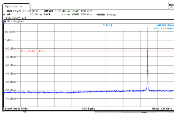
Band5-1.4MHz-QPSK-20643-1RB#5-30~1000-PASS
