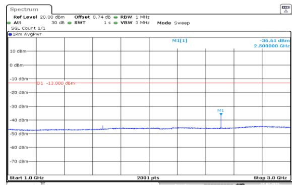
Band5-1.4MHz-QPSK-20525-1RB#0-1000~3000-PASS
