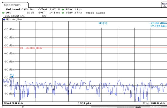
Band5-1.4MHz-QPSK-20525-1RB#5-0.009~0.15-PASS
