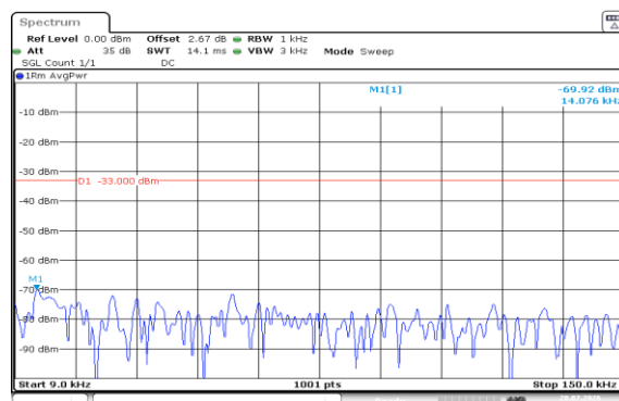
Band5-3MHz-16QAM-20415-1RB#0-0.009~0.15-PASS
