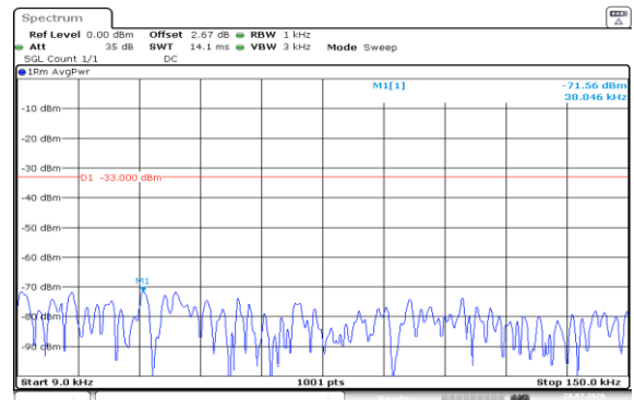
Band5-3MHz-16QAM-20415-1RB#14-0.009~0.15-PASS
