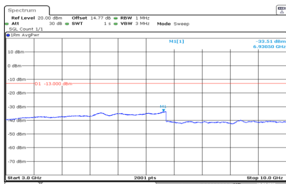
Band5-3MHz-QPSK-20525-15RB#0-3000~10000-PASS
