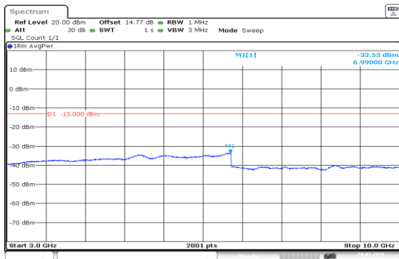
Band5-1.4MHz-QPSK-20525-6RB#0-3000~10000-PASS
