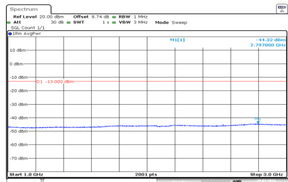
Band5-1.4MHz-QPSK-20643-6RB#0-1000~3000-PASS
