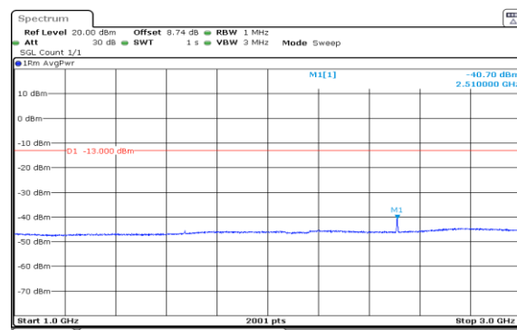
Band5-3MHz-QPSK-20525-15RB#0-1000~3000-PASS
