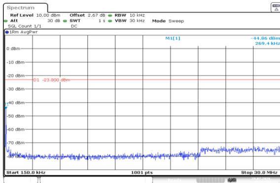
Band5-3MHz-16QAM-20635-1RB#0-0.15~30-PASS
