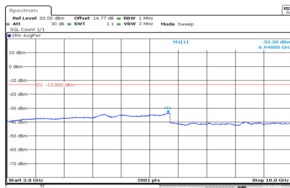
Band5-3MHz-16QAM-20635-15RB#0-3000~10000-PASS
