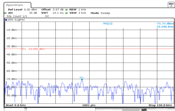
Band5-1.4MHz-16QAM-20525-6RB#0-0.009~0.15-PASS
