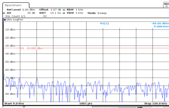
Band5-3MHz-QPSK-20525-15RB#0-0.009~0.15-PASS
