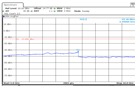
Band5-1.4MHz-QPSK-20407-6RB#0-3000~10000-PASS
