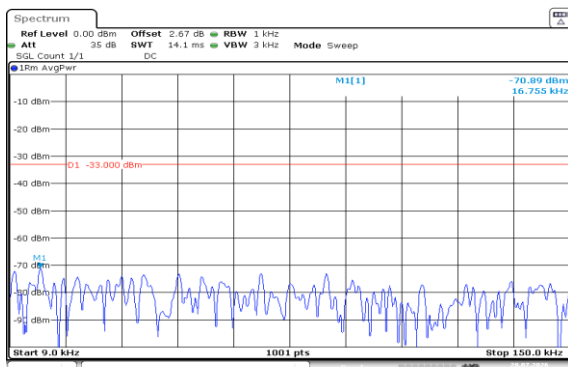
Band5-3MHz-QPSK-20635-1RB#14-0.009~0.15-PASS
