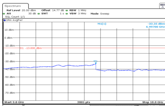
Band5-3MHz-QPSK-20415-15RB#0-3000~10000-PASS
