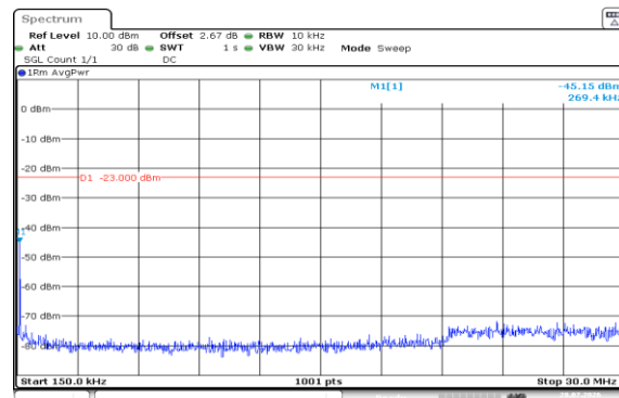
Band5-3MHz-QPSK-20525-15RB#0-0.15~30-PASS
