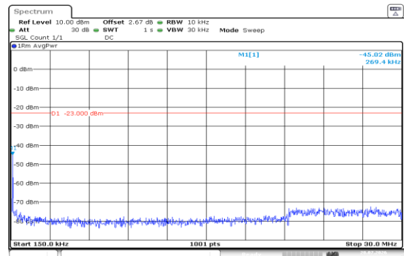
Band5-1.4MHz-QPSK-20525-1RB#0-0.15~30-PASS
