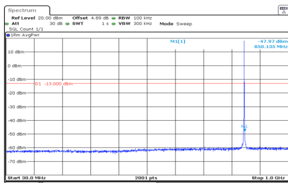
Band5-1.4MHz-QPSK-20643-1RB#0-30~1000-PASS
