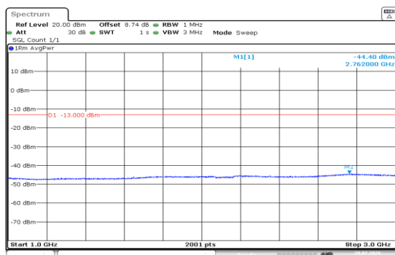
Band5-3MHz-16QAM-20415-1RB#0-1000~3000-PASS
