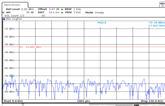
Band5-1.4MHz-QPSK-20525-1RB#0-0.009~0.15-PASS
