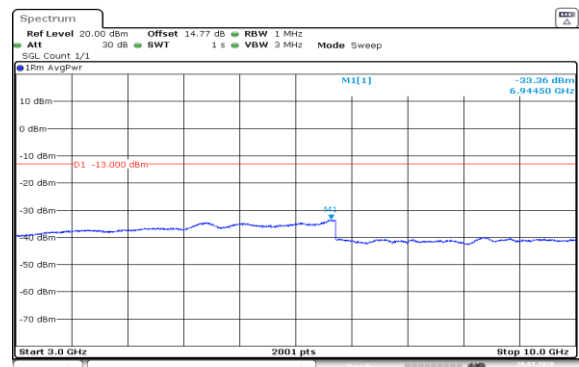
Band5-1.4MHz-16QAM-20525-6RB#0-3000~10000-PASS
