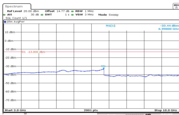
Band5-3MHz-QPSK-20635-15RB#0-3000~10000-PASS
