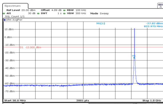
Band5-3MHz-QPSK-20415-15RB#0-30~1000-PASS
