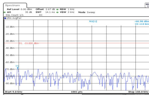
Band5-3MHz-16QAM-20525-15RB#0-0.009~0.15-PASS
