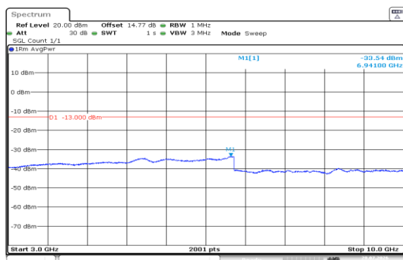
Band5-3MHz-QPSK-20415-1RB#0-3000~10000-PASS
