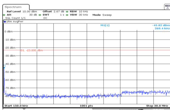
Band5-3MHz-16QAM-20415-1RB#0-0.15~30-PASS
