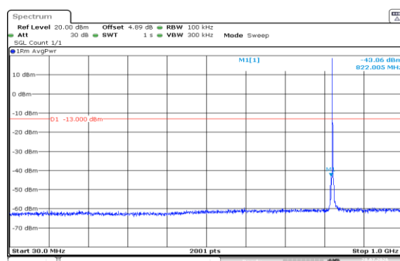
Band5-3MHz-16QAM-20415-1RB#0-30~1000-PASS
