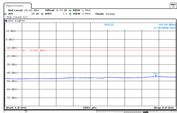
Band5-1.4MHz-QPSK-20407-1RB#0-1000~3000-PASS
