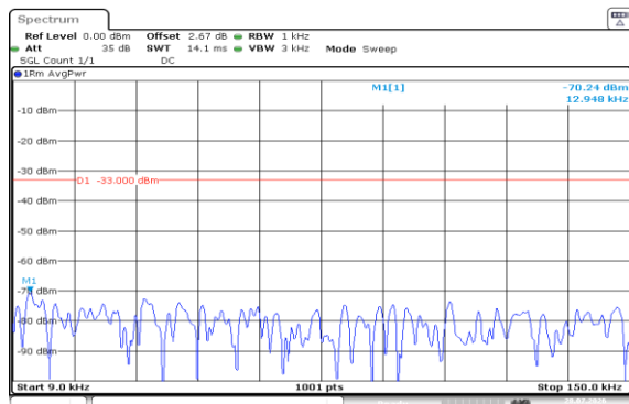
Band5-1.4MHz-QPSK-20407-6RB#0-0.009~0.15-PASS
