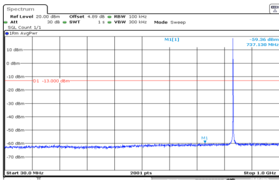
Band5-1.4MHz-QPSK-20525-1RB#0-30~1000-PASS
