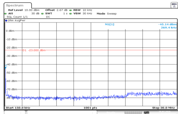
Band5-1.4MHz-QPSK-20407-1RB#0-0.15~30-PASS
