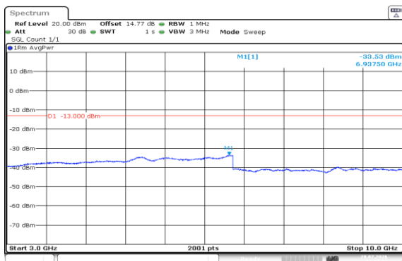
Band5-1.4MHz-QPSK-20525-1RB#0-3000~10000-PASS
