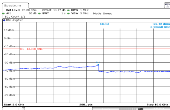
Band5-3MHz-QPSK-20635-1RB#0-3000~10000-PASS
