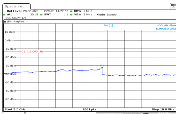
Band5-3MHz-QPSK-20525-1RB#14-3000~10000-PASS
