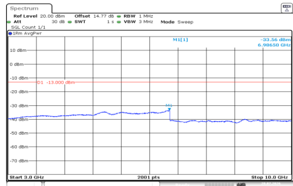
Band5-3MHz-16QAM-20415-15RB#0-3000~10000-PASS
