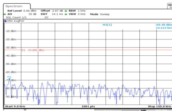
Band5-3MHz-16QAM-20525-1RB#14-0.009~0.15-PASS
