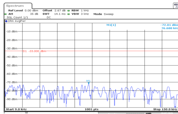
Band5-1.4MHz-16QAM-20643-1RB#5-0.009~0.15-PASS
