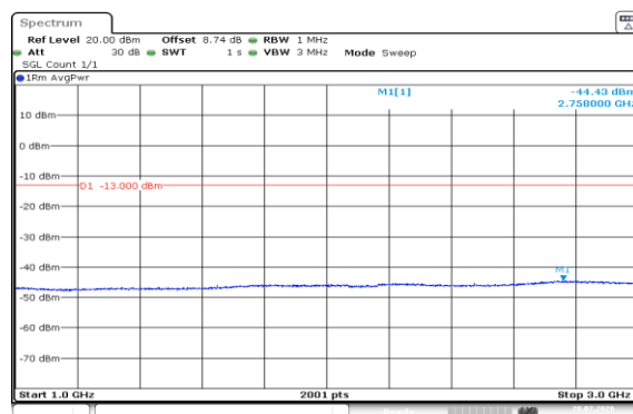
Band5-3MHz-QPSK-20415-1RB#0-1000~3000-PASS
