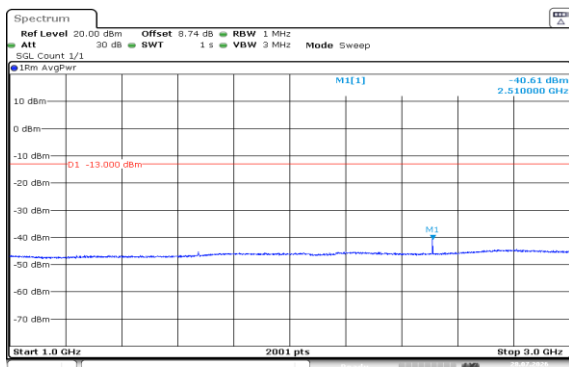
Band5-1.4MHz-16QAM-20525-6RB#0-1000~3000-PASS
