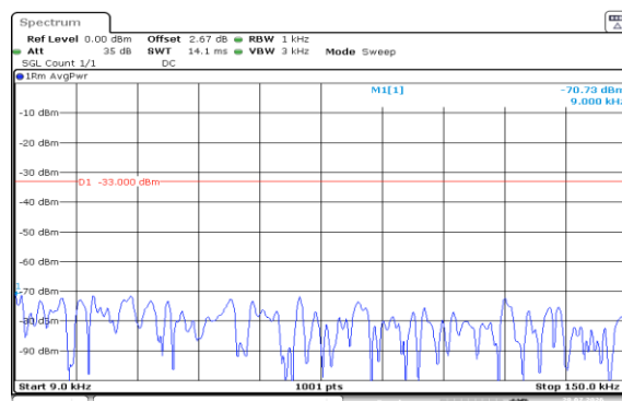
Band5-3MHz-16QAM-20415-15RB#0-0.009~0.15-PASS
