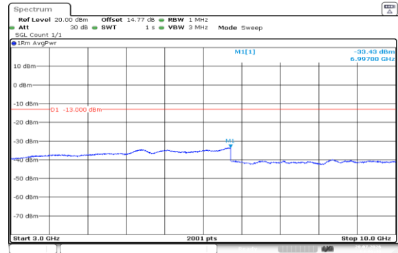
Band5-1.4MHz-16QAM-20407-6RB#0-3000~10000-PASS
