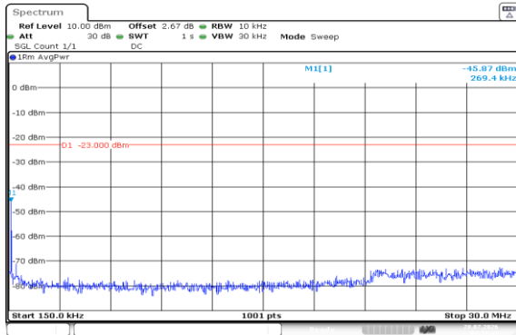
Band5-3MHz-16QAM-20415-15RB#0-0.15~30-PASS
