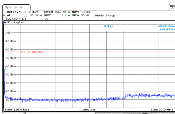
Band5-3MHz-16QAM-20635-15RB#0-0.15~30-PASS
