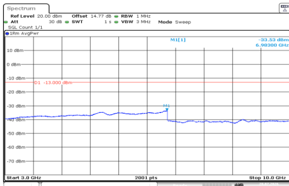
Band5-3MHz-QPSK-20415-1RB#14-3000~10000-PASS
