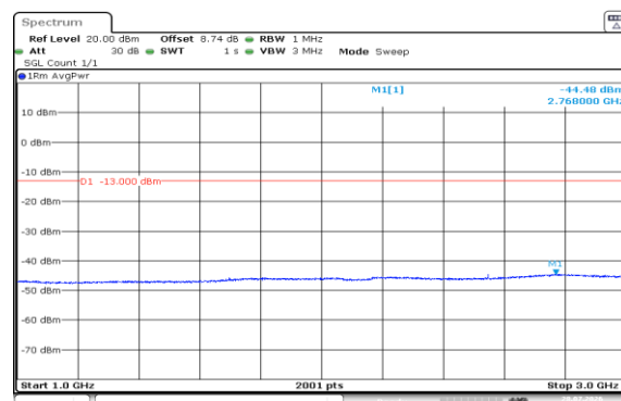
Band5-1.4MHz-QPSK-20643-1RB#5-1000~3000-PASS
