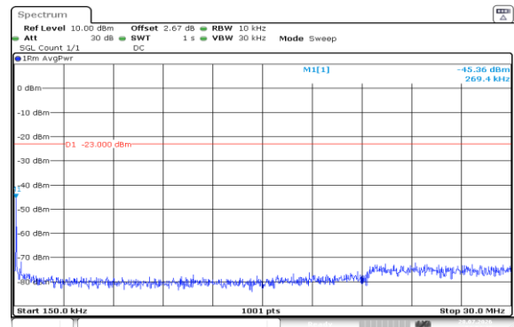
Band5-1.4MHz-QPSK-20407-1RB#5-0.15~30-PASS
