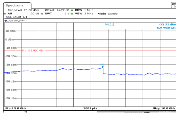
Band5-3MHz-16QAM-20415-1RB#14-3000~10000-PASS
