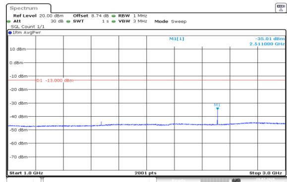
Band5-1.4MHz-QPSK-20525-1RB#5-1000~3000-PASS
