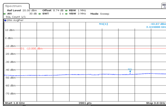
Band5-1.4MHz-QPSK-20643-1RB#0-1000~3000-PASS
