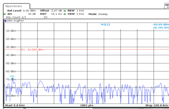
Band5-1.4MHz-16QAM-20643-1RB#0-0.009~0.15-PASS
