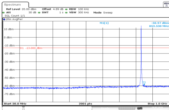
Band5-1.4MHz-QPSK-20525-6RB#0-30~1000-PASS
