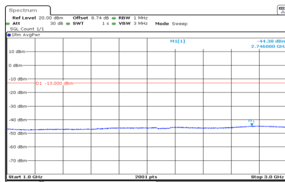
Band5-1.4MHz-QPSK-20407-6RB#0-1000~3000-PASS
