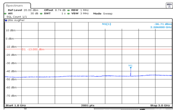
Band5-3MHz-QPSK-20525-1RB#0-1000~3000-PASS
