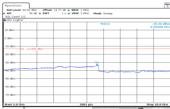
Band5-1.4MHz-QPSK-20643-1RB#5-3000~10000-PASS
