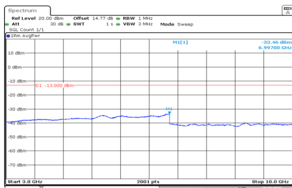
Band5-1.4MHz-QPSK-20643-1RB#0-3000~10000-PASS
