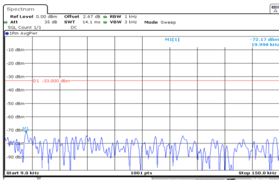
Band5-3MHz-QPSK-20525-1RB#0-0.009~0.15-PASS
