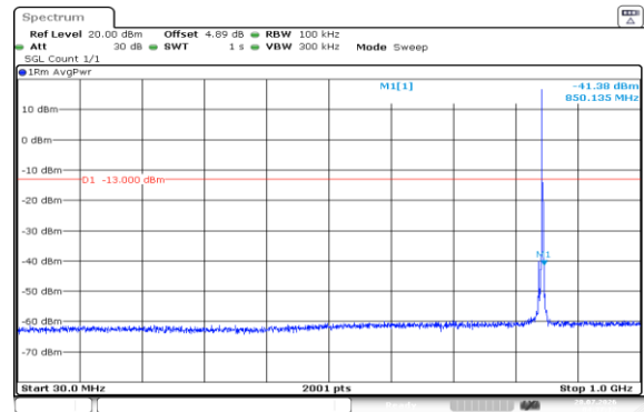
Band5-3MHz-16QAM-20635-1RB#0-30~1000-PASS
