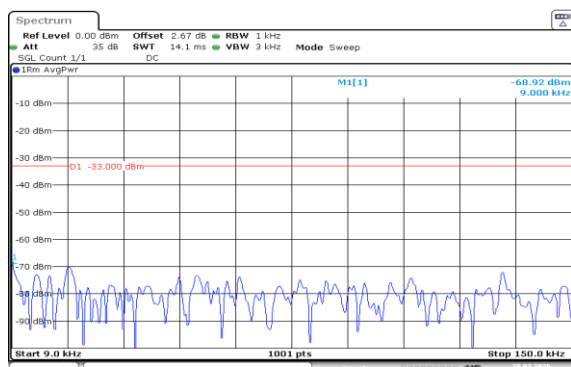
Band5-1.4MHz-QPSK-20643-1RB#5-0.009~0.15-PASS
