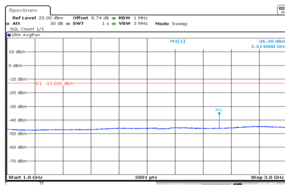
Band5-3MHz-QPSK-20525-1RB#14-1000~3000-PASS
