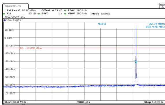
Band5-1.4MHz-QPSK-20407-6RB#0-30~1000-PASS
