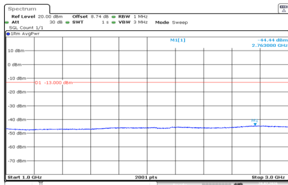
Band5-3MHz-16QAM-20415-1RB#14-1000~3000-PASS
