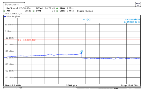
Band5-1.4MHz-16QAM-20407-1RB#5-3000~10000-PASS
