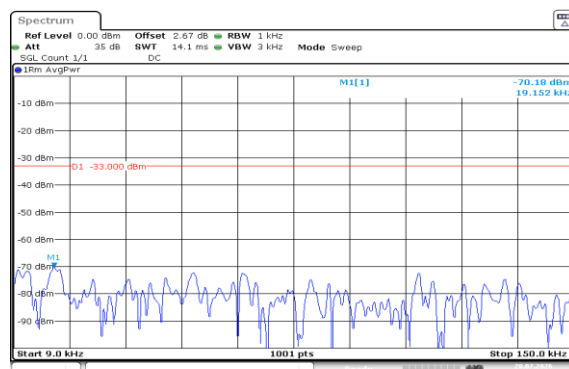
Band5-3MHz-16QAM-20635-15RB#0-0.009~0.15-PASS
