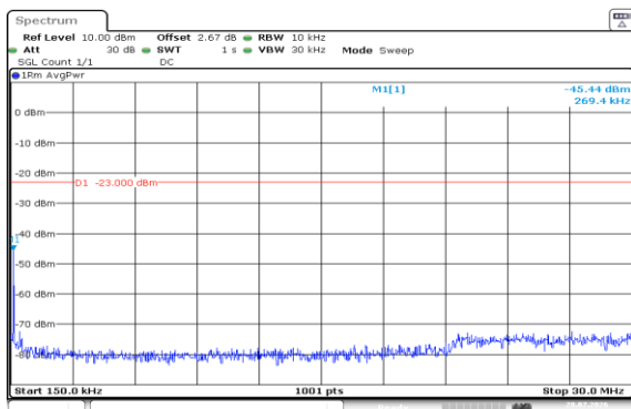
Band5-1.4MHz-16QAM-20525-6RB#0-0.15~30-PASS
