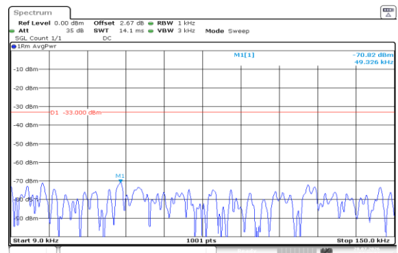
Band5-3MHz-16QAM-20635-1RB#0-0.009~0.15-PASS
