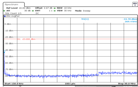
Band5-3MHz-QPSK-20525-1RB#0-0.15~30-PASS
