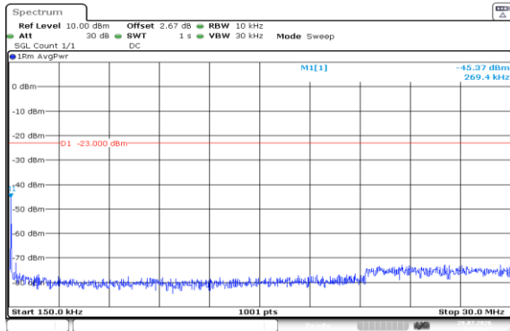
Band5-1.4MHz-16QAM-20525-1RB#0-0.15~30-PASS
