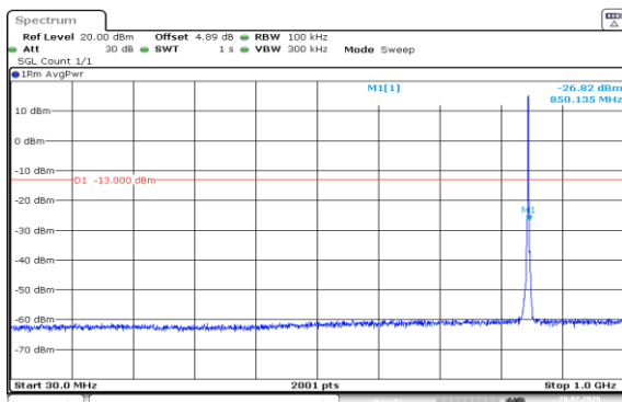
Band5-1.4MHz-QPSK-20643-6RB#0-30~1000-PASS
