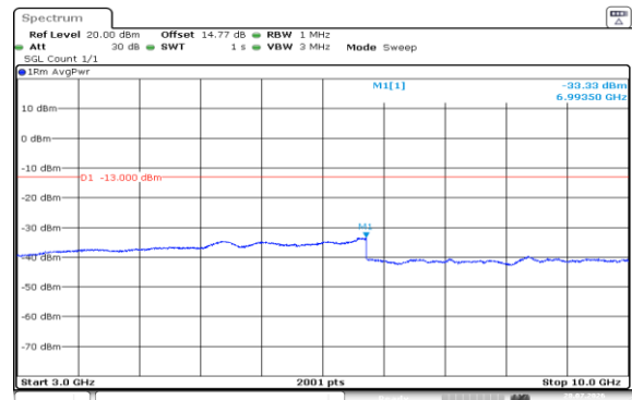
Band5-1.4MHz-16QAM-20407-1RB#0-3000~10000-PASS
