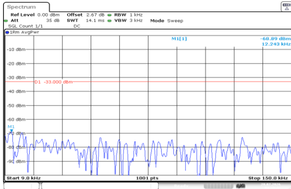
Band5-3MHz-QPSK-20415-1RB#14-0.009~0.15-PASS
