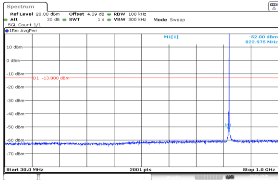
Band5-1.4MHz-QPSK-20407-1RB#5-30~1000-PASS
