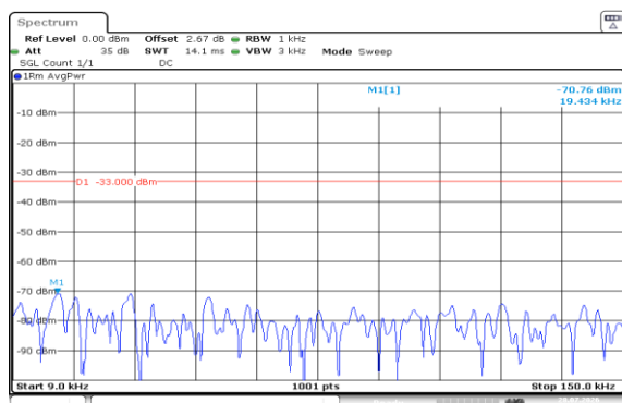
Band5-1.4MHz-QPSK-20643-1RB#0-0.009~0.15-PASS
