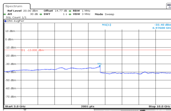
Band5-3MHz-16QAM-20525-1RB#14-3000~10000-PASS
