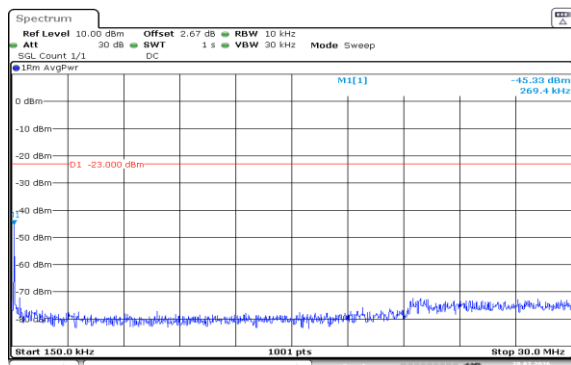
Band5-1.4MHz-16QAM-20643-1RB#0-0.15~30-PASS
