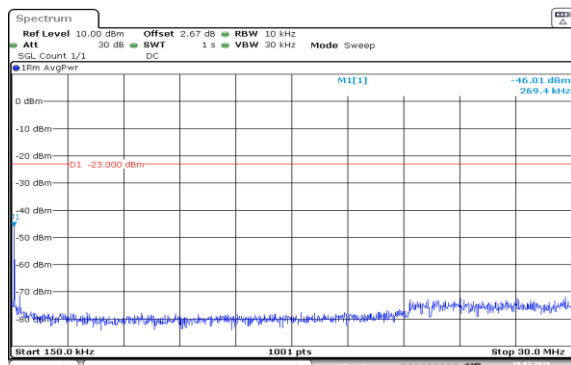
Band5-1.4MHz-16QAM-20407-6RB#0-0.15~30-PASS
