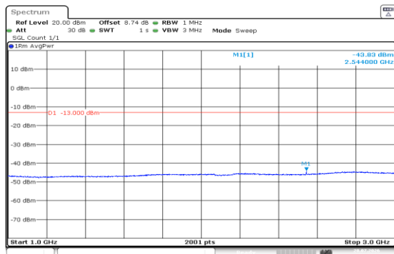
Band5-1.4MHz-16QAM-20643-1RB#0-1000~3000-PASS
