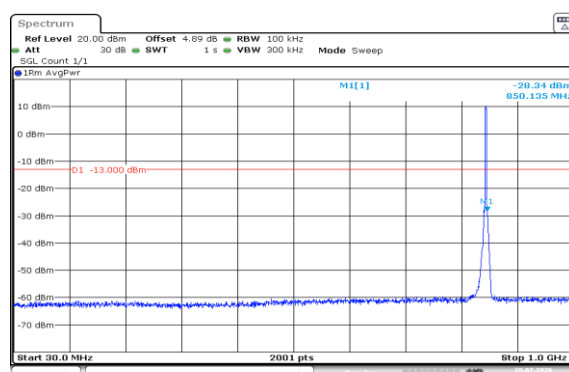
Band5-3MHz-16QAM-20635-15RB#0-30~1000-PASS
