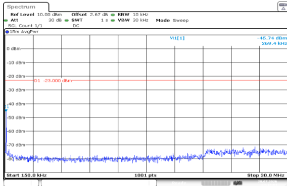
Band5-1.4MHz-16QAM-20643-1RB#5-0.15~30-PASS
