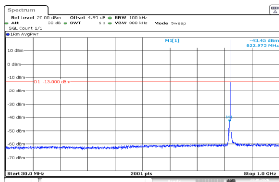
Band5-3MHz-QPSK-20415-1RB#0-30~1000-PASS
