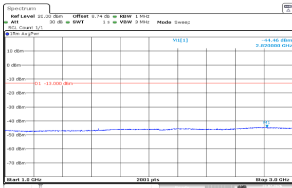
Band5-1.4MHz-16QAM-20407-1RB#0-1000~3000-PASS
