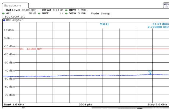
Band5-1.4MHz-16QAM-20407-1RB#5-1000~3000-PASS
