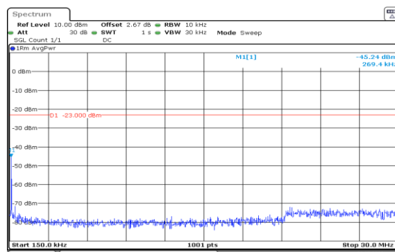
Band5-3MHz-QPSK-20415-15RB#0-0.15~30-PASS
