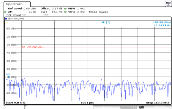
Band5-1.4MHz-16QAM-20407-1RB#0-0.009~0.15-PASS
