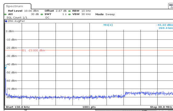
Band5-1.4MHz-QPSK-20643-1RB#5-0.15~30-PASS
