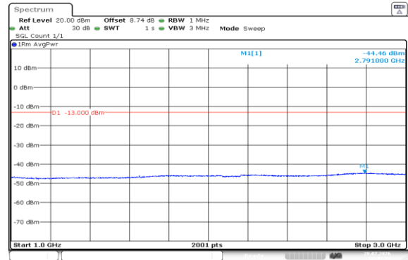
Band5-1.4MHz-QPSK-20407-1RB#5-1000~3000-PASS
