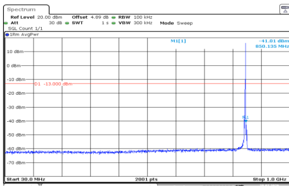
Band5-3MHz-QPSK-20635-1RB#14-30~1000-PASS
