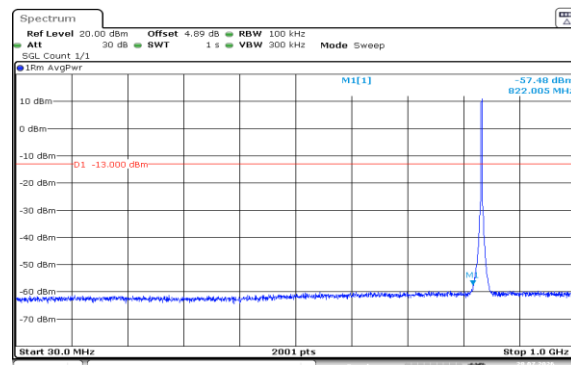
Band5-3MHz-16QAM-20525-15RB#0-30~1000-PASS
