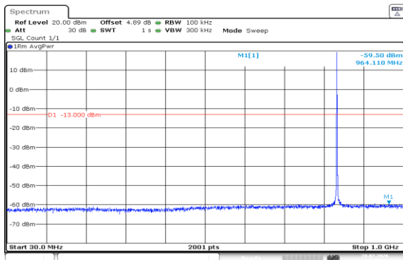
Band5-1.4MHz-QPSK-20525-1RB#5-30~1000-PASS
