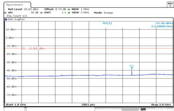
Band5-1.4MHz-QPSK-20525-6RB#0-1000~3000-PASS
