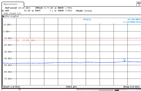
Band5-3MHz-16QAM-20415-15RB#0-1000~3000-PASS
