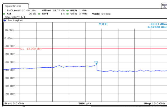
Band5-5MHz-QPSK-20425-1RB#0-3000~10000-PASS
