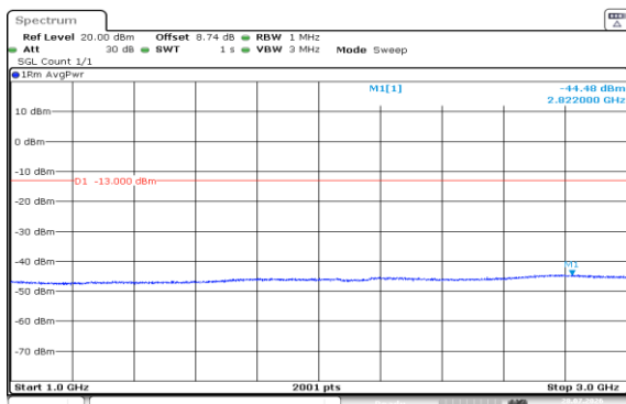
Band5-5MHz-16QAM-20625-1RB#24-1000~3000-PASS
