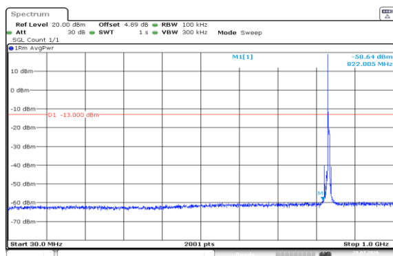
Band5-5MHz-QPSK-20525-1RB#0-30~1000-PASS
