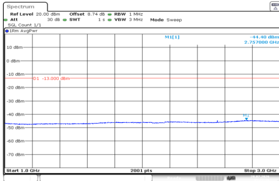
Band5-10MHz-16QAM-20600-1RB#49-1000~3000-PASS
