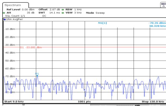
Band5-10MHz-QPSK-20600-1RB#49-0.009~0.15-PASS
