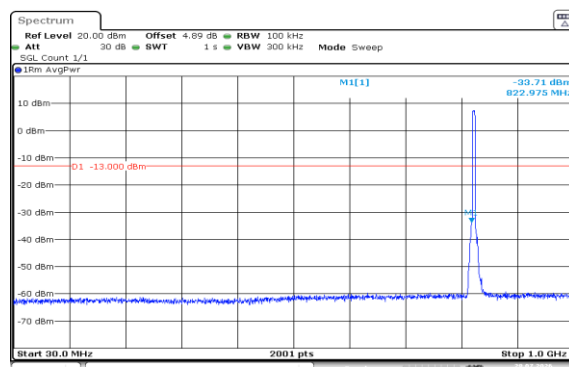
Band5-5MHz-16QAM-20425-25RB#0-30~1000-PASS
