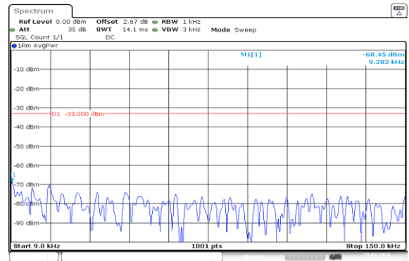
Band5-5MHz-16QAM-20625-1RB#0-0.009~0.15-PASS
