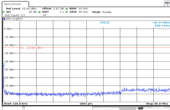
Band5-10MHz-16QAM-20525-1RB#49-0.15~30-PASS
