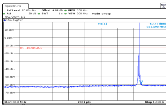
Band5-5MHz-QPSK-20525-1RB#24-30~1000-PASS
