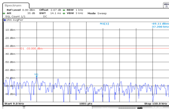
Band5-5MHz-QPSK-20525-1RB#0-0.009~0.15-PASS
