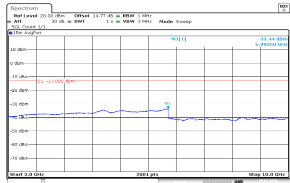
Band5-10MHz-16QAM-20600-50RB#0-3000~10000-PASS
