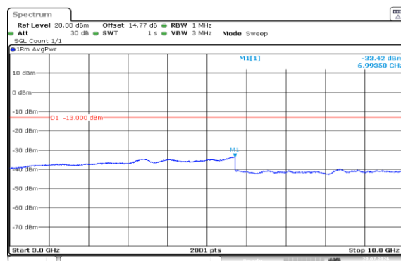
Band5-5MHz-16QAM-20425-1RB#0-3000~10000-PASS
