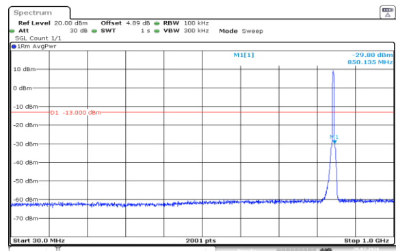
Band5-5MHz-16QAM-20625-25RB#0-30~1000-PASS
