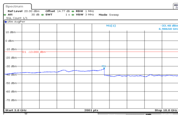
Band5-5MHz-16QAM-20525-1RB#0-3000~10000-PASS
