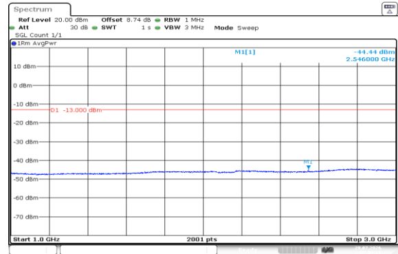
Band5-5MHz-QPSK-20625-1RB#24-1000~3000-PASS
