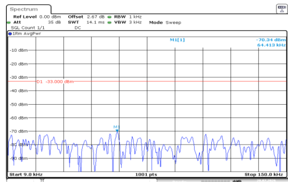
Band5-10MHz-16QAM-20600-50RB#0-0.009~0.15-PASS
