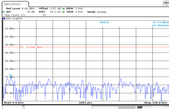
Band5-5MHz-QPSK-20625-25RB#0-0.009~0.15-PASS
