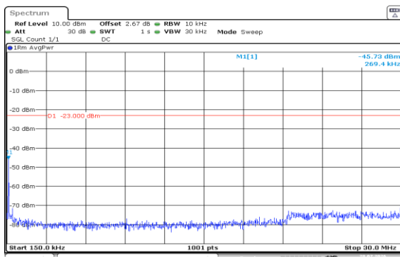
Band5-10MHz-16QAM-20525-1RB#0-0.15~30-PASS
