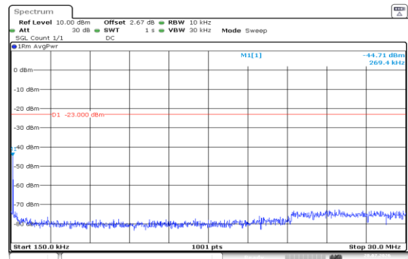
Band5-10MHz-QPSK-20600-50RB#0-0.15~30-PASS
