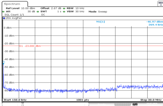
Band5-5MHz-16QAM-20425-1RB#24-0.15~30-PASS
