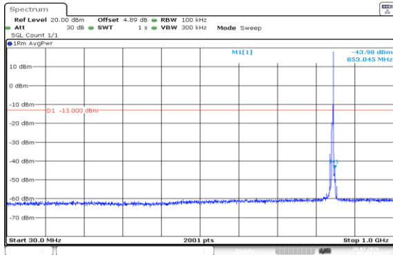
Band5-5MHz-QPSK-20625-1RB#24-30~1000-PASS
