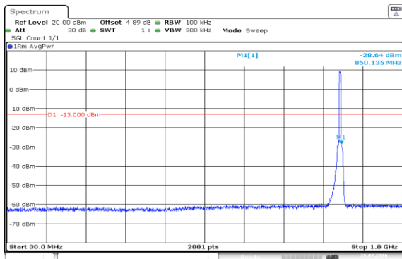
Band5-5MHz-QPSK-20625-25RB#0-30~1000-PASS
