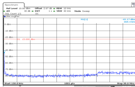
Band5-5MHz-QPSK-20425-1RB#0-0.15~30-PASS
