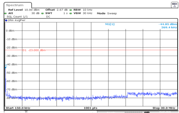
Band5-5MHz-QPSK-20625-1RB#0-0.15~30-PASS
