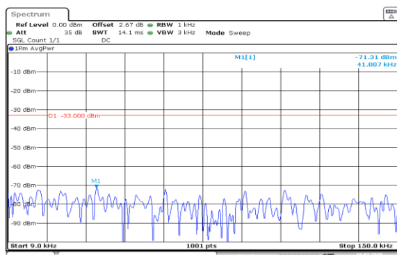
Band5-5MHz-QPSK-20525-25RB#0-0.009~0.15-PASS
