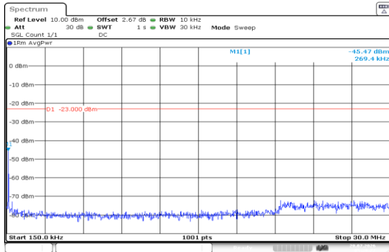
Band5-10MHz-16QAM-20600-50RB#0-0.15~30-PASS
