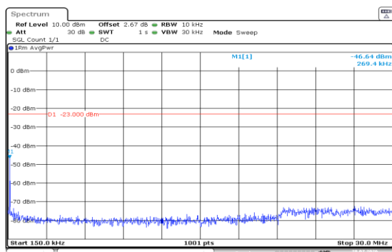
Band5-5MHz-16QAM-20425-25RB#0-0.15~30-PASS
