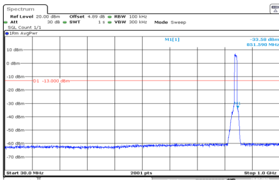
Band5-10MHz-QPSK-20600-50RB#0-30~1000-PASS
