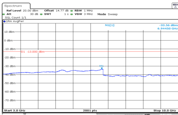
Band5-5MHz-QPSK-20625-25RB#0-3000~10000-PASS
