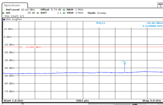
Band5-10MHz-16QAM-20600-1RB#0-1000~3000-PASS
