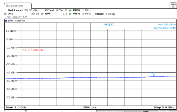
Band5-5MHz-QPSK-20425-25RB#0-1000~3000-PASS
