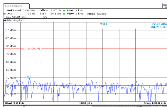
Band5-5MHz-16QAM-20525-25RB#0-0.009~0.15-PASS
