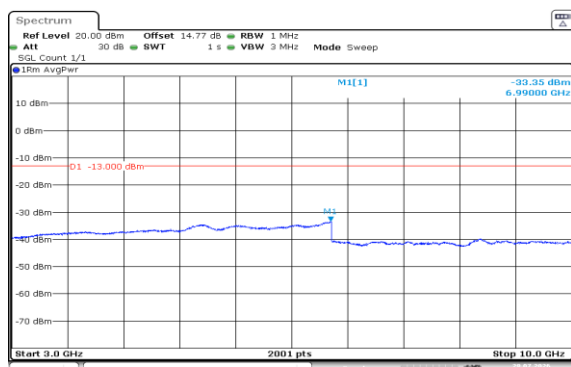
Band5-5MHz-QPSK-20425-1RB#24-3000~10000-PASS
