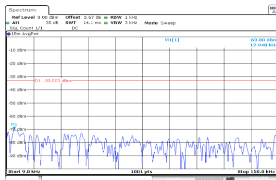
Band5-5MHz-16QAM-20425-25RB#0-0.009~0.15-PASS
