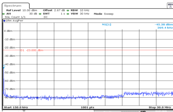
Band5-5MHz-16QAM-20625-25RB#0-0.15~30-PASS
