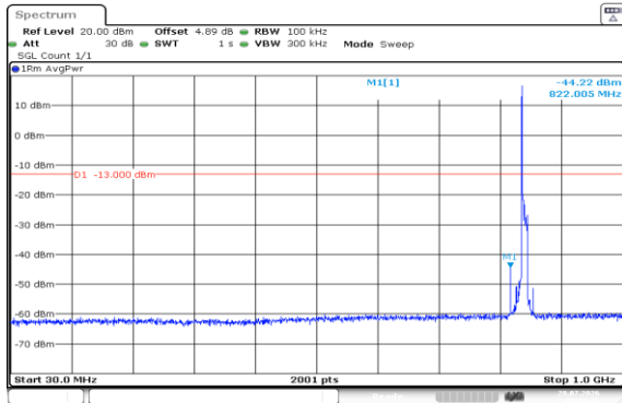
Band5-10MHz-QPSK-20600-1RB#0-30~1000-PASS
