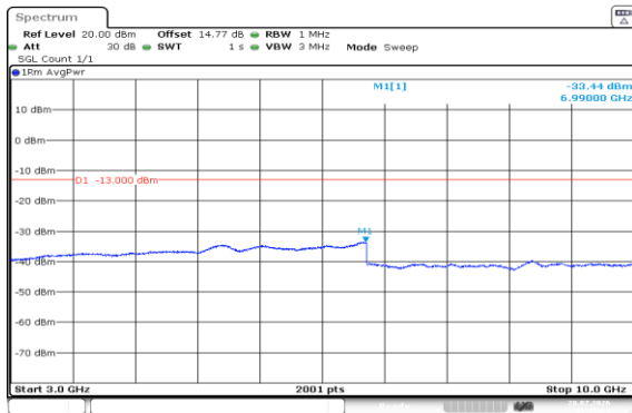
Band5-5MHz-QPSK-20625-1RB#0-3000~10000-PASS
