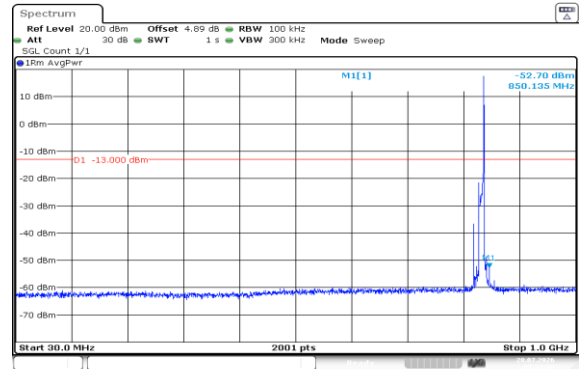
Band5-10MHz-16QAM-20525-1RB#49-30~1000-PASS
