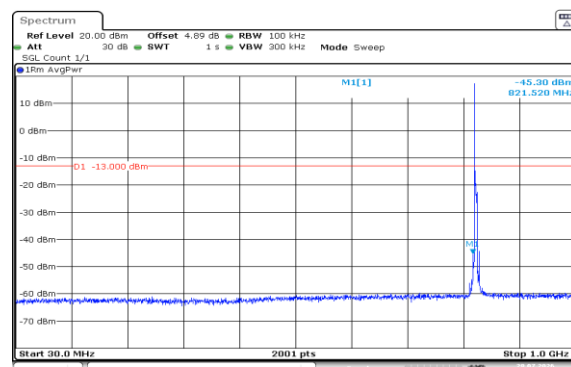
Band5-5MHz-16QAM-20425-1RB#0-30~1000-PASS
