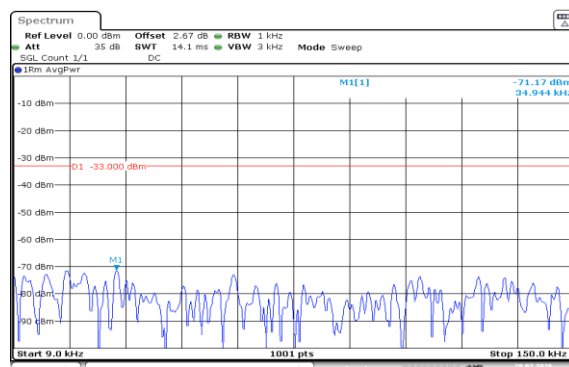
Band5-5MHz-16QAM-20425-1RB#24-0.009~0.15-PASS
