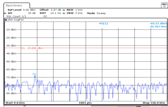
Band5-5MHz-16QAM-20625-25RB#0-0.009~0.15-PASS
