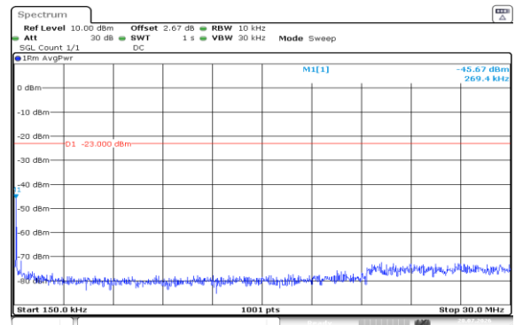
Band5-10MHz-QPSK-20525-1RB#49-0.15~30-PASS
