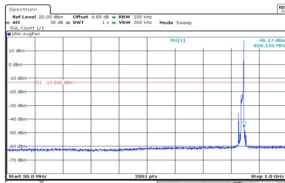
Band5-10MHz-16QAM-20600-1RB#49-30~1000-PASS
