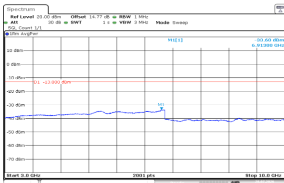
Band5-10MHz-QPSK-20600-50RB#0-3000~10000-PASS
