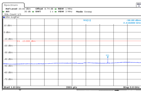
Band5-5MHz-16QAM-20525-1RB#24-1000~3000-PASS
