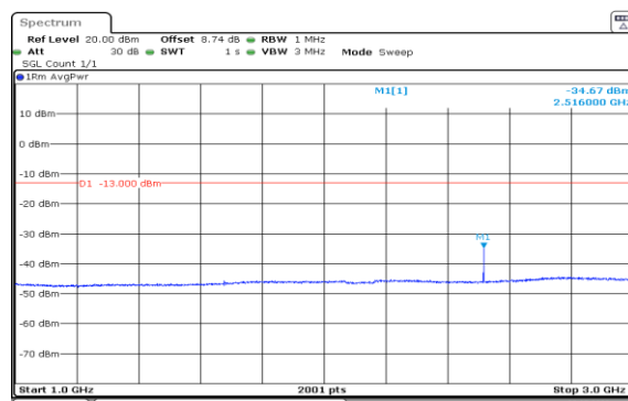
Band5-5MHz-QPSK-20525-1RB#24-1000~3000-PASS
