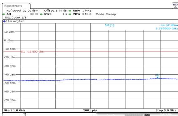
Band5-10MHz-16QAM-20450-50RB#0-1000~3000-PASS
