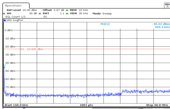
Band5-5MHz-16QAM-20525-1RB#24-0.15~30-PASS
