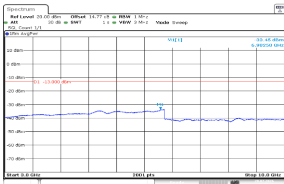
Band5-10MHz-QPSK-20525-1RB#49-3000~10000-PASS
