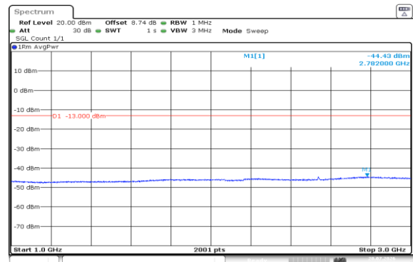
Band5-5MHz-QPSK-20625-25RB#0-1000~3000-PASS
