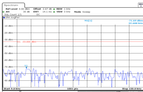
Band5-5MHz-QPSK-20425-1RB#24-0.009~0.15-PASS
