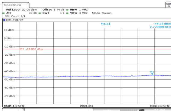
Band5-10MHz-16QAM-20600-50RB#0-1000~3000-PASS
