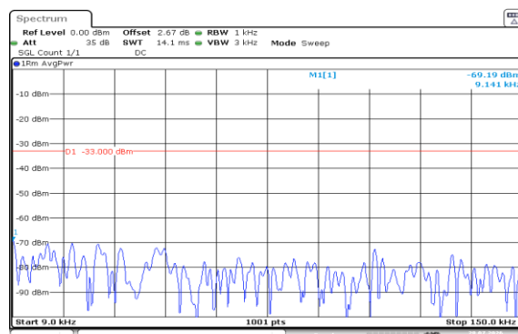
Band5-5MHz-16QAM-20525-1RB#0-0.009~0.15-PASS
