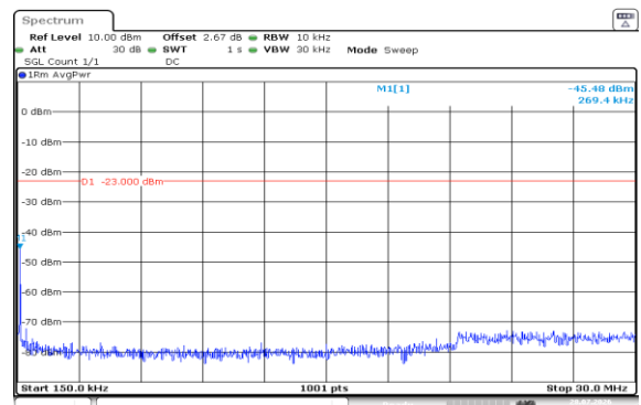
Band5-5MHz-QPSK-20625-1RB#24-0.15~30-PASS
