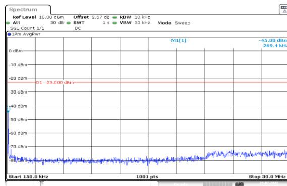
Band5-5MHz-QPSK-20525-1RB#0-0.15~30-PASS
