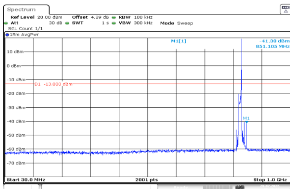
Band5-10MHz-QPSK-20450-1RB#49-30~1000-PASS
