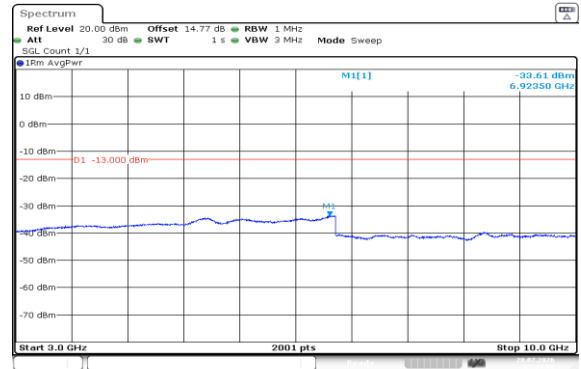
Band5-5MHz-16QAM-20625-25RB#0-3000~10000-PASS
