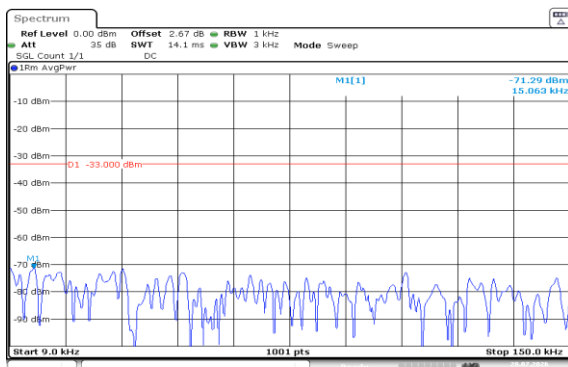
Band5-5MHz-QPSK-20625-1RB#24-0.009~0.15-PASS
