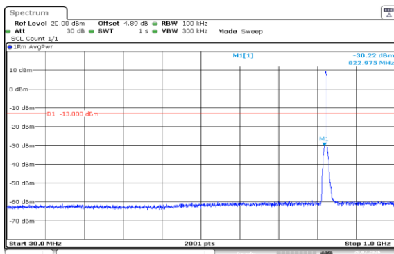
Band5-5MHz-QPSK-20425-25RB#0-30~1000-PASS
