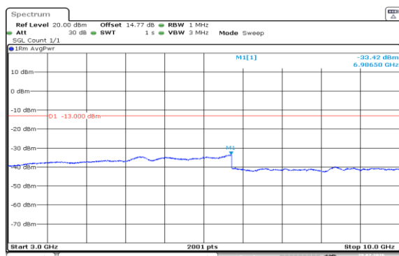
Band5-5MHz-QPSK-20525-25RB#0-3000~10000-PASS
