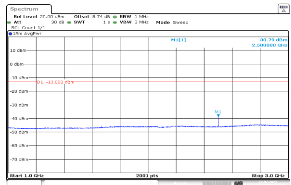
Band5-10MHz-QPSK-20450-1RB#49-1000~3000-PASS
