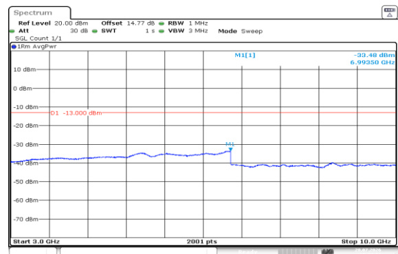
Band5-10MHz-16QAM-20450-50RB#0-3000~10000-PASS
