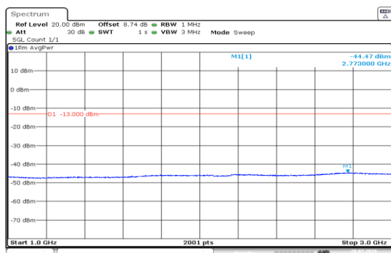
Band5-5MHz-16QAM-20425-1RB#0-1000~3000-PASS
