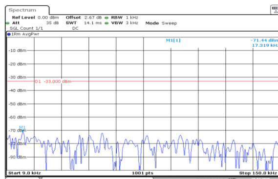
Band5-10MHz-16QAM-20600-1RB#49-0.009~0.15-PASS
