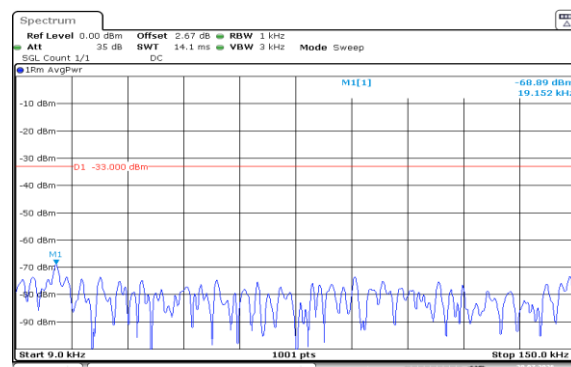
Band5-5MHz-16QAM-20425-1RB#0-0.009~0.15-PASS
