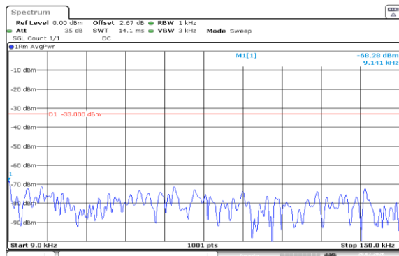
Band5-5MHz-QPSK-20525-1RB#24-0.009~0.15-PASS
