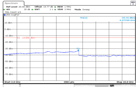
Band5-10MHz-16QAM-20600-1RB#49-3000~10000-PASS
