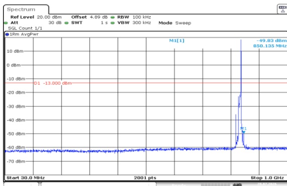
Band5-10MHz-QPSK-20525-1RB#49-30~1000-PASS
