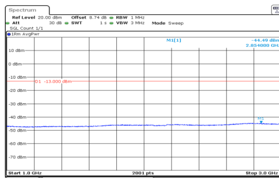
Band5-10MHz-QPSK-20600-1RB#49-1000~3000-PASS
