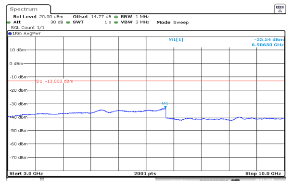
Band5-5MHz-16QAM-20625-1RB#24-3000~10000-PASS
