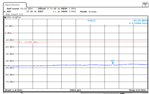
Band5-10MHz-QPSK-20525-50RB#0-1000~3000-PASS
