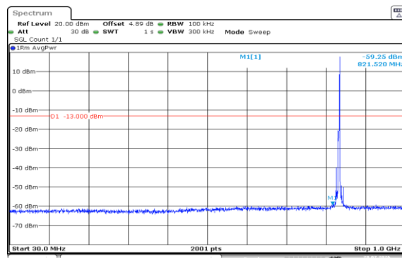
Band5-5MHz-16QAM-20525-1RB#24-30~1000-PASS
