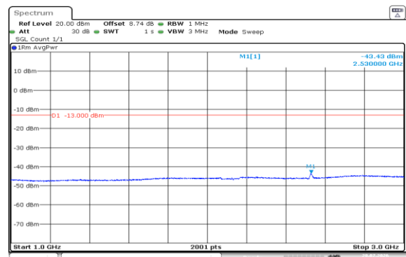
Band5-10MHz-QPSK-20600-50RB#0-1000~3000-PASS
