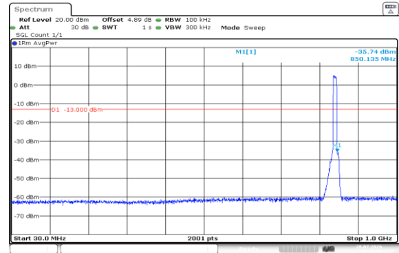
Band5-10MHz-16QAM-20600-50RB#0-30~1000-PASS
