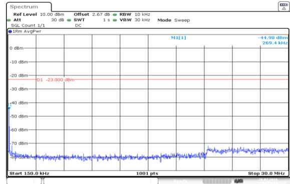
Band5-5MHz-QPSK-20625-25RB#0-0.15~30-PASS
