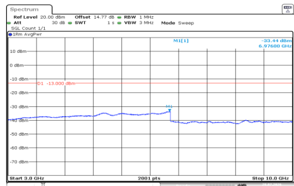
Band5-10MHz-16QAM-20600-1RB#0-3000~10000-PASS
