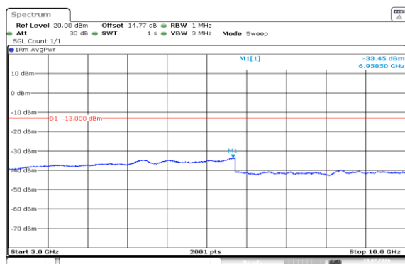
Band5-5MHz-QPSK-20425-25RB#0-3000~10000-PASS
