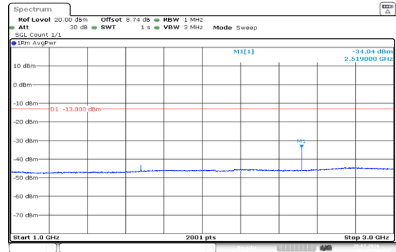
Band5-10MHz-QPSK-20600-1RB#0-1000~3000-PASS
