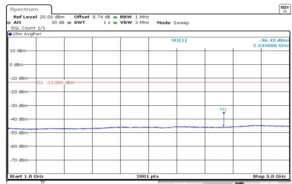
Band5-5MHz-QPSK-20625-1RB#0-1000~3000-PASS
