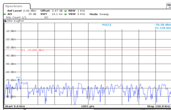
Band5-5MHz-16QAM-20525-1RB#24-0.009~0.15-PASS
