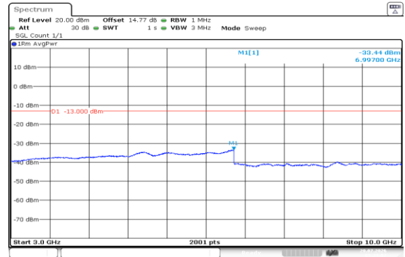
Band5-10MHz-16QAM-20525-1RB#0-3000~10000-PASS
