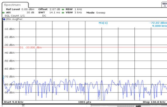
Band5-10MHz-QPSK-20600-50RB#0-0.009~0.15-PASS
