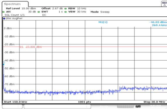
Band5-10MHz-16QAM-20450-1RB#0-0.15~30-PASS
