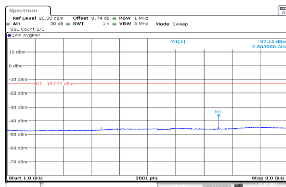
Band5-5MHz-QPSK-20525-1RB#0-1000~3000-PASS
