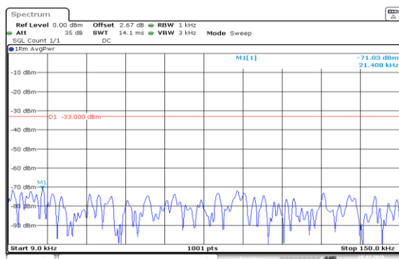
Band5-5MHz-QPSK-20425-1RB#0-0.009~0.15-PASS
