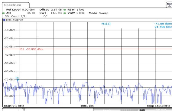
Band5-10MHz-QPSK-20525-1RB#49-0.009~0.15-PASS
