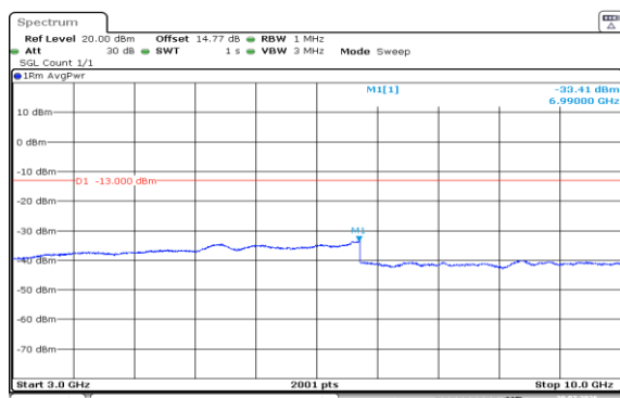
Band5-5MHz-QPSK-20525-1RB#24-3000~10000-PASS
