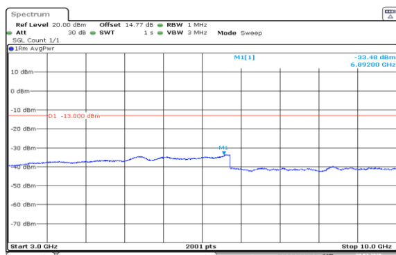
Band5-10MHz-QPSK-20600-1RB#49-3000~10000-PASS
