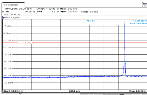
Band5-5MHz-QPSK-20625-1RB#0-30~1000-PASS
