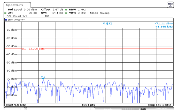
Band5-5MHz-16QAM-20625-1RB#24-0.009~0.15-PASS
