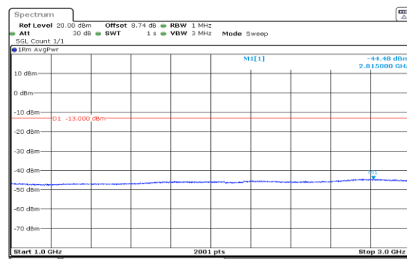
Band5-5MHz-QPSK-20425-1RB#0-1000~3000-PASS
