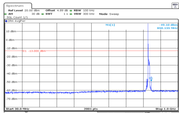
Band5-10MHz-16QAM-20525-1RB#0-30~1000-PASS
