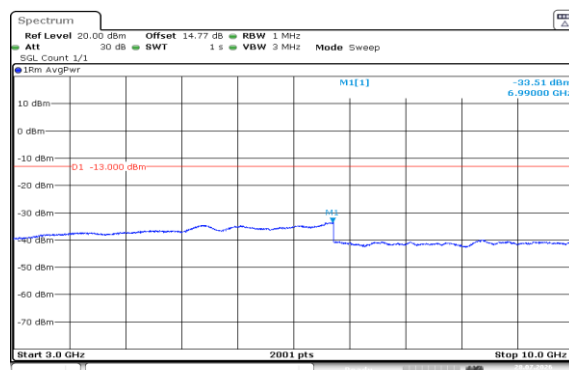
Band5-5MHz-16QAM-20525-1RB#24-3000~10000-PASS
