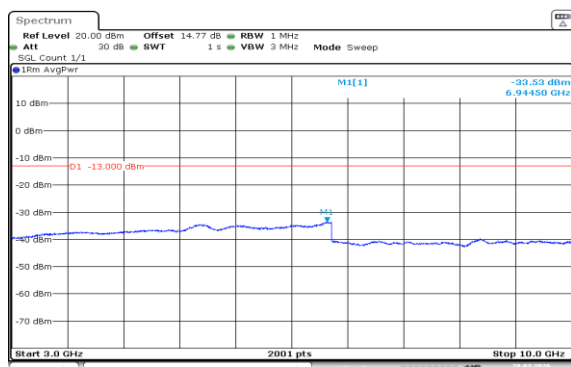
Band5-5MHz-QPSK-20525-1RB#0-3000~10000-PASS
