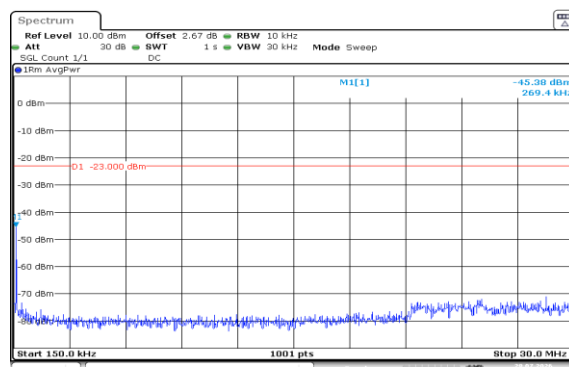
Band5-5MHz-QPSK-20525-25RB#0-0.15~30-PASS
