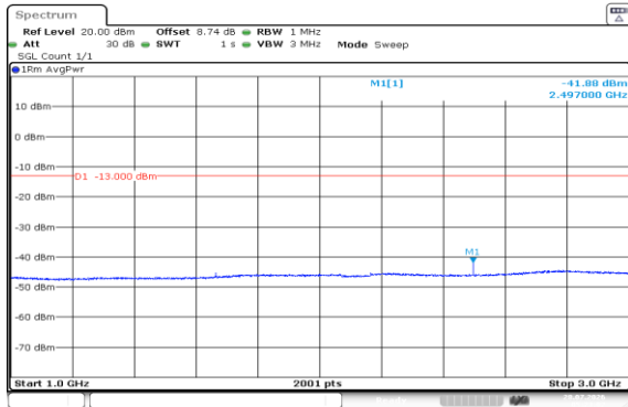
Band5-10MHz-16QAM-20525-1RB#0-1000~3000-PASS
