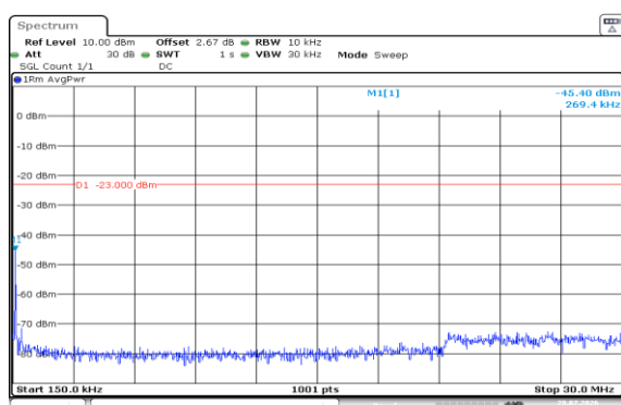
Band5-5MHz-16QAM-20525-1RB#0-0.15~30-PASS
