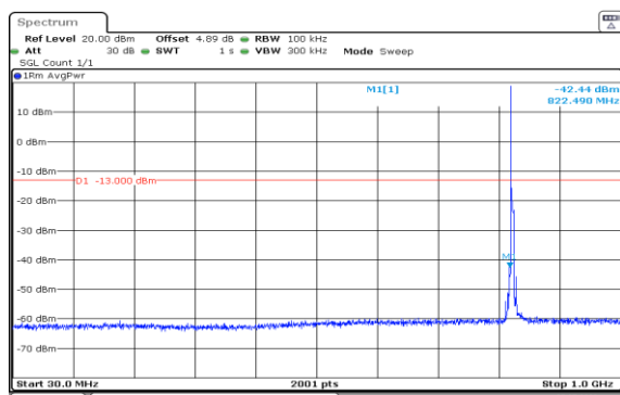
Band5-5MHz-QPSK-20425-1RB#0-30~1000-PASS
