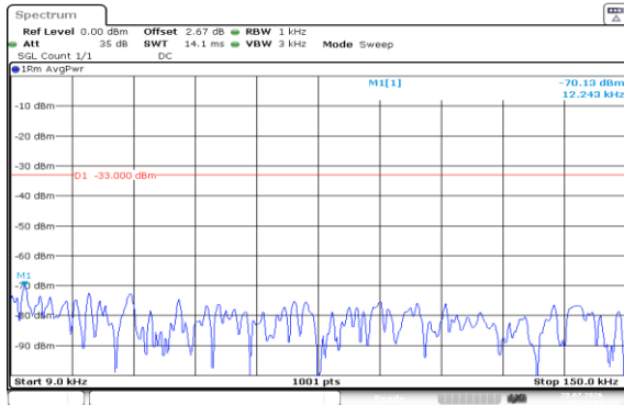
Band5-10MHz-QPSK-20525-1RB#0-0.009~0.15-PASS
