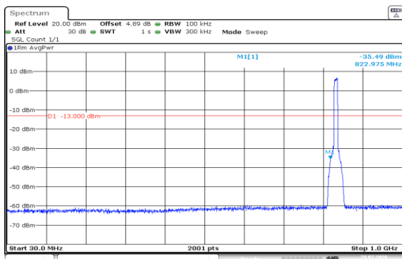
Band5-10MHz-QPSK-20525-50RB#0-30~1000-PASS
