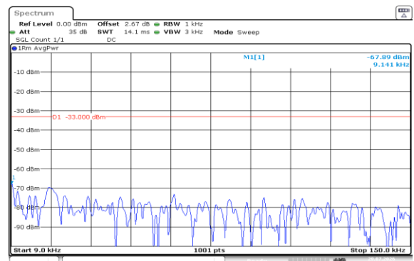
Band5-10MHz-16QAM-20450-1RB#0-0.009~0.15-PASS
