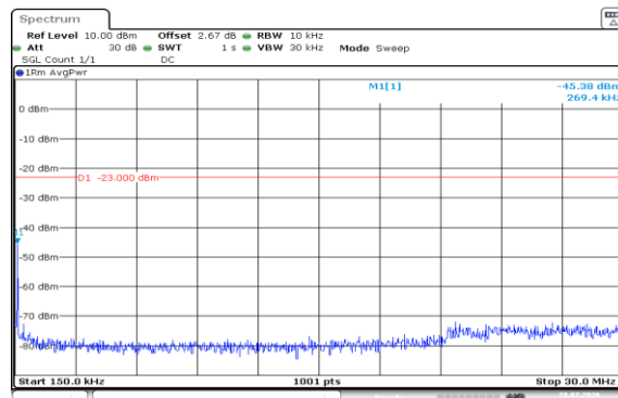
Band5-10MHz-QPSK-20600-1RB#49-0.15~30-PASS
