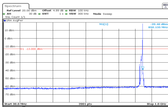
Band5-10MHz-QPSK-20600-1RB#49-30~1000-PASS
