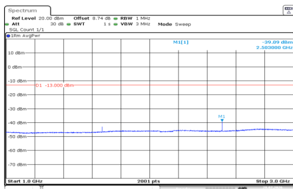
Band5-5MHz-16QAM-20525-1RB#0-1000~3000-PASS
