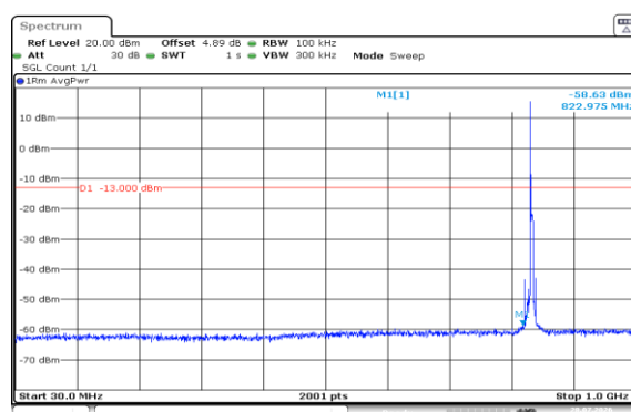
Band5-5MHz-16QAM-20525-1RB#0-30~1000-PASS
