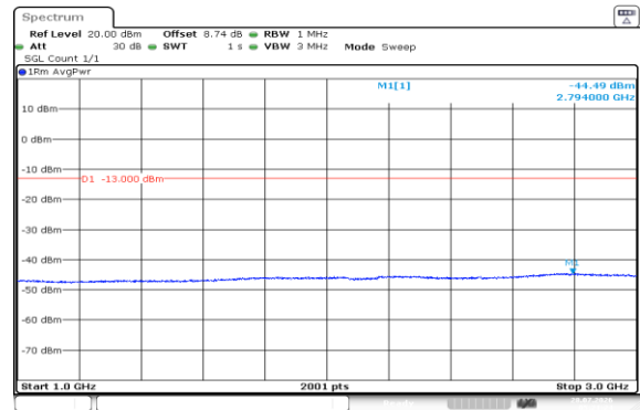
Band5-10MHz-QPSK-20450-50RB#0-1000~3000-PASS
