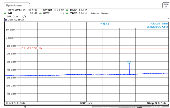
Band5-10MHz-QPSK-20525-1RB#49-1000~3000-PASS
