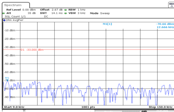
Band5-5MHz-QPSK-20625-1RB#0-0.009~0.15-PASS
