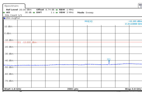
Band5-5MHz-QPSK-20525-25RB#0-1000~3000-PASS
