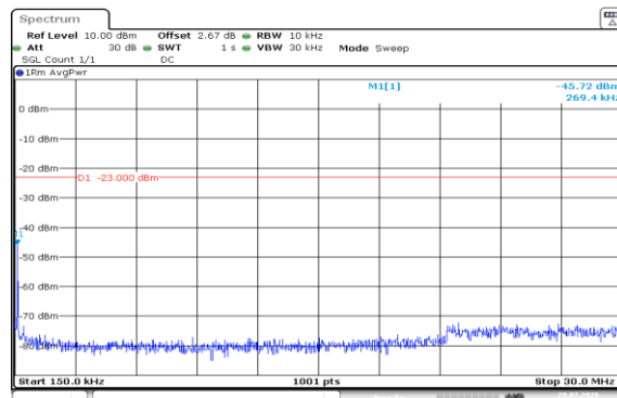
Band5-5MHz-QPSK-20525-1RB#24-0.15~30-PASS
