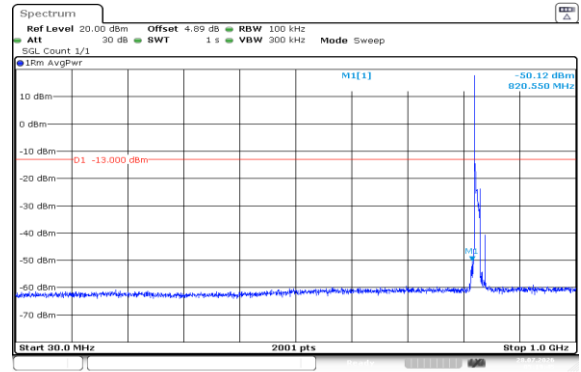
Band5-10MHz-16QAM-20450-1RB#0-30~1000-PASS
