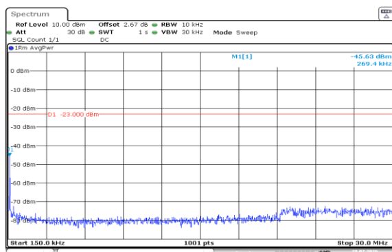
Band5-5MHz-16QAM-20425-1RB#0-0.15~30-PASS
