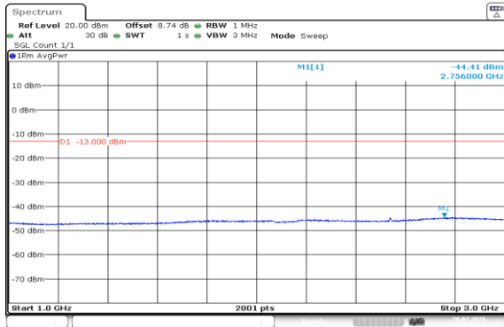
Band5-5MHz-16QAM-20625-25RB#0-1000~3000-PASS
