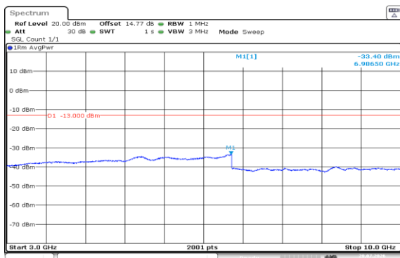
Band5-10MHz-QPSK-20450-1RB#0-3000~10000-PASS
