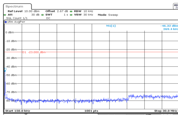
Band5-5MHz-QPSK-20425-1RB#24-0.15~30-PASS
