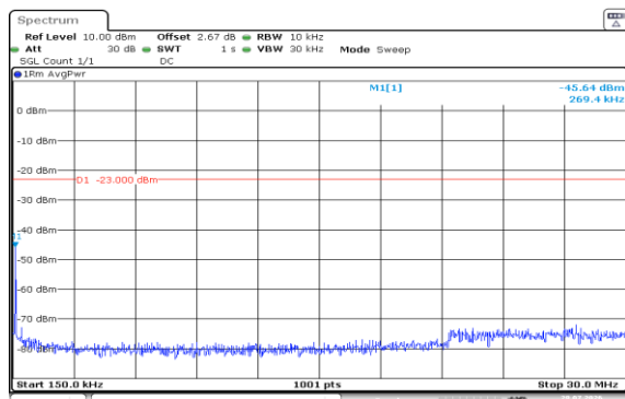
Band5-10MHz-16QAM-20600-1RB#49-0.15~30-PASS
