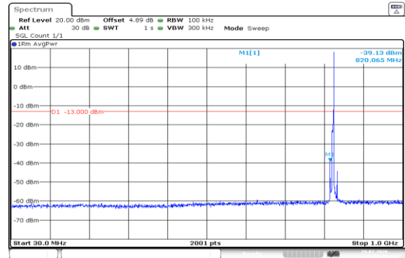
Band5-5MHz-16QAM-20425-1RB#24-30~1000-PASS
