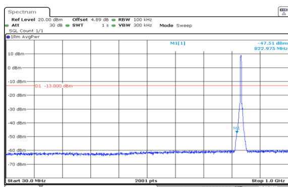
Band5-5MHz-QPSK-20525-25RB#0-30~1000-PASS
