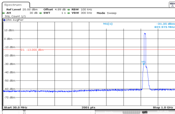
Band5-10MHz-QPSK-20450-50RB#0-30~1000-PASS
