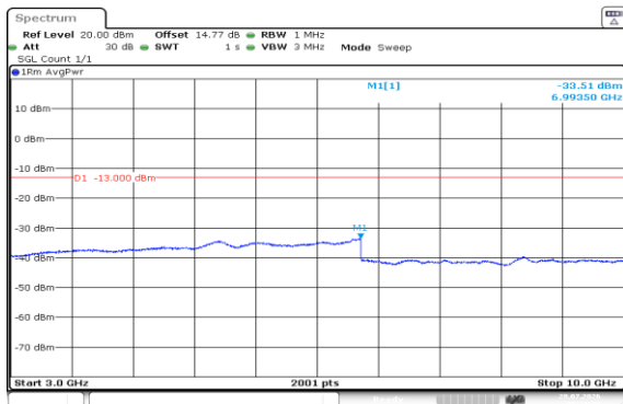
Band5-10MHz-QPSK-20450-50RB#0-3000~10000-PASS
