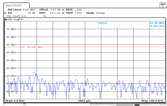
Band5-10MHz-16QAM-20525-1RB#49-0.009~0.15-PASS
