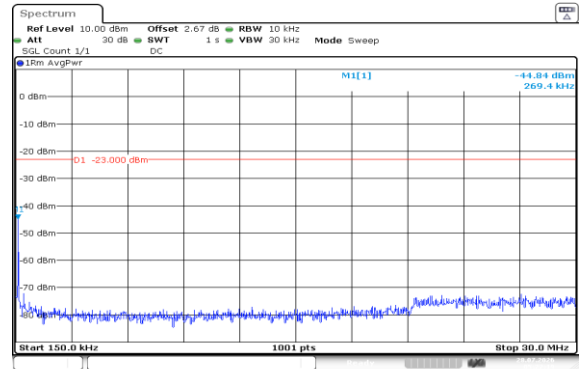
Band5-10MHz-QPSK-20525-1RB#0-0.15~30-PASS
