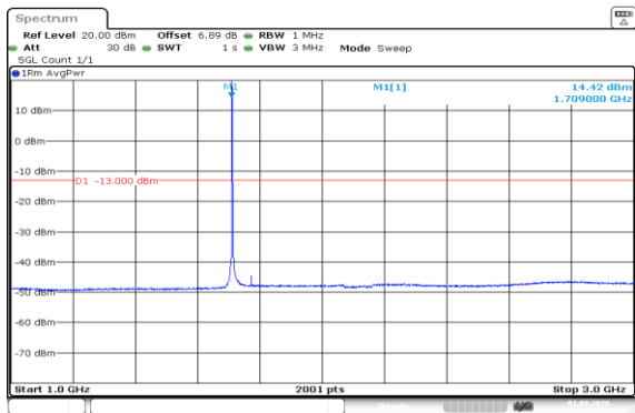
Band66-3MHz-QPSK-131987-1RB#0-1000~3000
