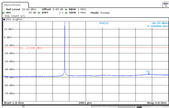
Band66-3MHz-QPSK-132322-1RB#14-1000~3000-PASS
