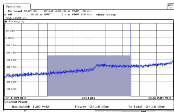
Band66-1.4MHz-QPSK-131979-6RB#0-1000~3000-PASS
