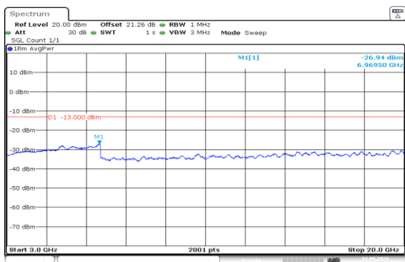
Band66-1.4MHz-16QAM-131979-1RB#0-3000~20000-PASS
