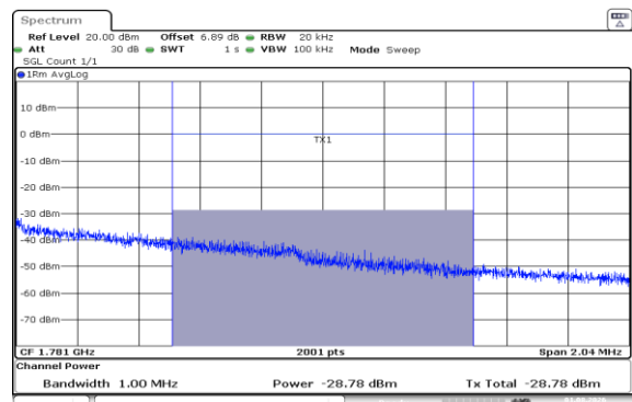
Band66-1.4MHz-16QAM-132665-6RB#0-1000~3000-PASS
