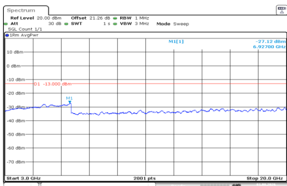
Band66-1.4MHz-QPSK-131979-6RB#0-3000~20000-PASS
