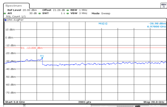
Band66-1.4MHz-QPSK-132322-6RB#0-3000~20000-PASS
