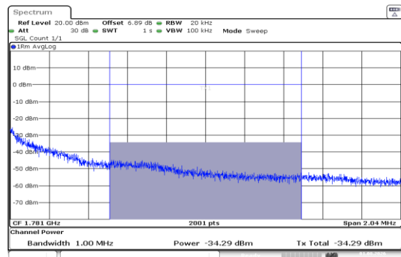
Band66-1.4MHz-16QAM-132665-1RB#5-1000~3000-PASS
