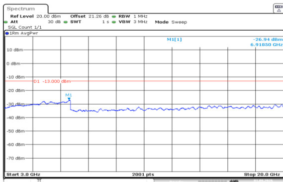
Band66-1.4MHz-16QAM-132322-1RB#0-3000~20000-PASS
