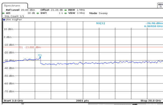
Band66-1.4MHz-16QAM-131979-6RB#0-3000~20000-PASS
