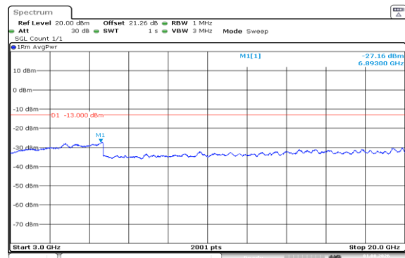
Band66-3MHz-QPSK-132322-15RB#0-3000~20000-PASS
