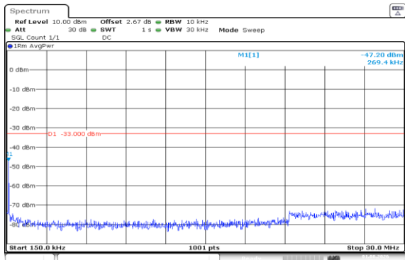
Band66-3MHz-QPSK-131987-1RB#14-0.15~30-PASS
