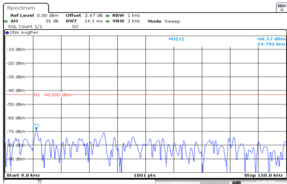
Band66-3MHz-16QAM-131987-1RB#14-0.009~0.15-PASS
