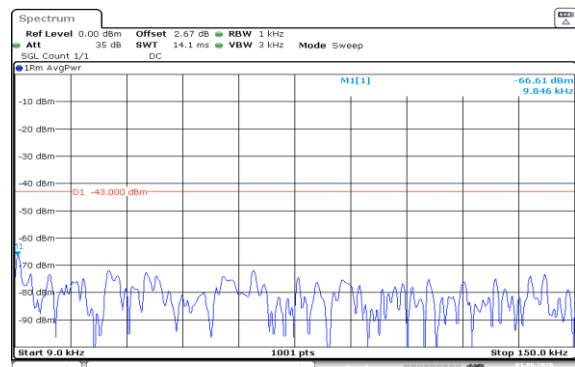
Band66-3MHz-QPSK-132322-15RB#0-0.009~0.15-PASS
