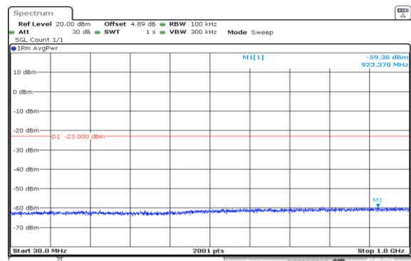
Band66-1.4MHz-QPSK-131979-6RB#0-30~1000-PASS
