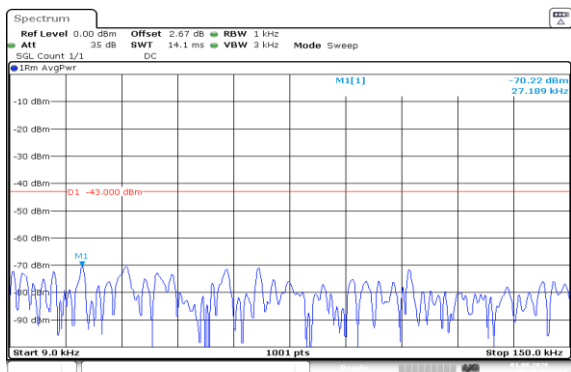
Band66-1.4MHz-16QAM-131979-1RB#0-0.009~0.15-PASS
