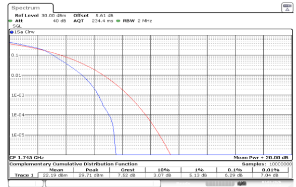
Band66-1.4MHz-16QAM-132322-6RB#0-PASS
