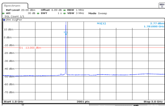
Band66-1.4MHz-QPSK-132665-6RB#0-1000~3000
