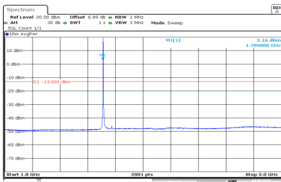
Band66-3MHz-16QAM-131987-15RB#0-1000~3000
