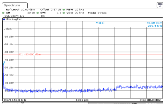
Band66-1.4MHz-QPSK-131979-6RB#0-0.15~30-PASS
