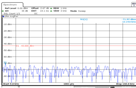
Band66-3MHz-16QAM-132322-1RB#0-0.009~0.15-PASS
