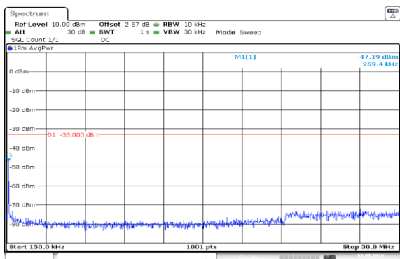
Band66-1.4MHz-16QAM-131979-1RB#5-0.15~30-PASS
