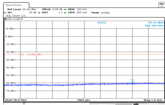
Band66-1.4MHz-QPSK-131979-1RB#5-30~1000-PASS
