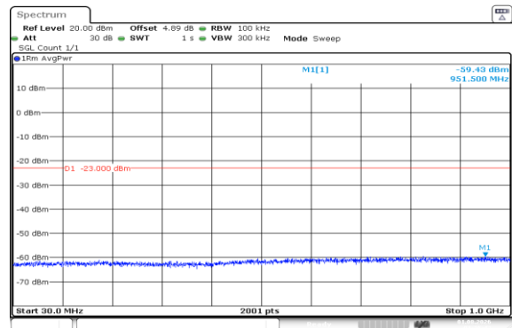
Band66-1.4MHz-16QAM-132665-6RB#0-30~1000-PASS
