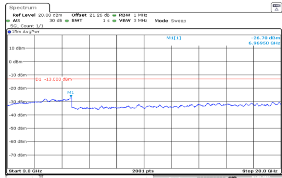
Band66-3MHz-QPSK-132322-1RB#0-3000~20000-PASS
