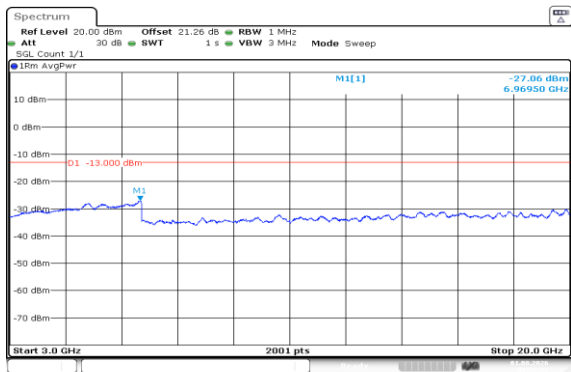
Band66-3MHz-16QAM-131987-1RB#0-3000~20000-PASS
