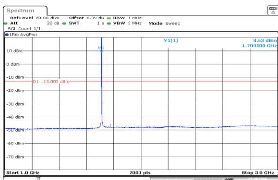
Band66-1.4MHz-QPSK-131979-6RB#0-1000~3000
