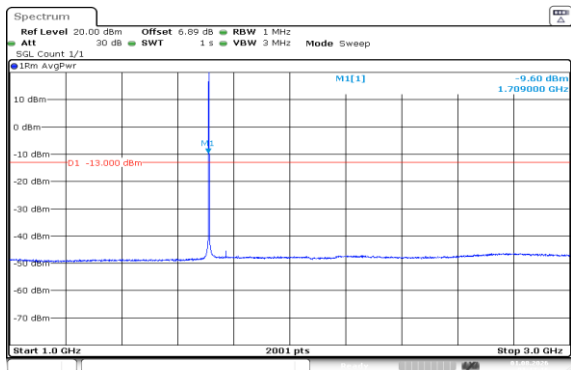
Band66-1.4MHz-QPSK-131979-1RB#5-1000~3000
