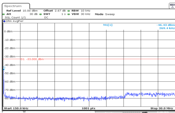
Band66-1.4MHz-QPSK-132665-1RB#0-0.15~30-PASS
