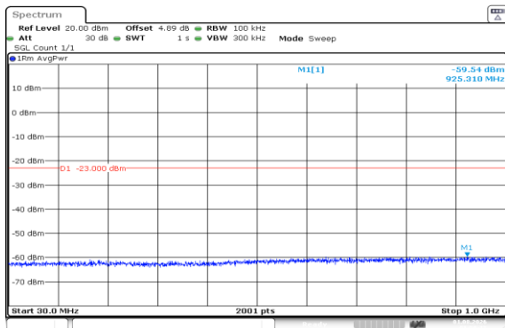
Band66-3MHz-16QAM-131987-1RB#14-30~1000-PASS
