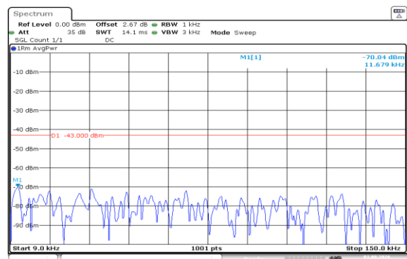
Band66-1.4MHz-QPSK-132322-1RB#0-0.009~0.15-PASS
