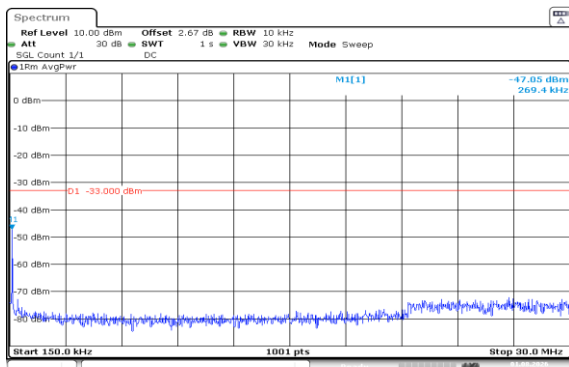
Band66-1.4MHz-QPSK-132322-1RB#0-0.15~30-PASS
