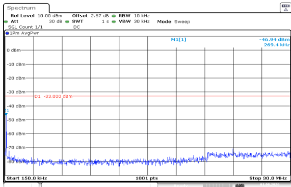
Band66-3MHz-QPSK-132322-1RB#14-0.15~30-PASS
