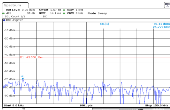
Band66-1.4MHz-16QAM-132322-6RB#0-0.009~0.15-PASS
