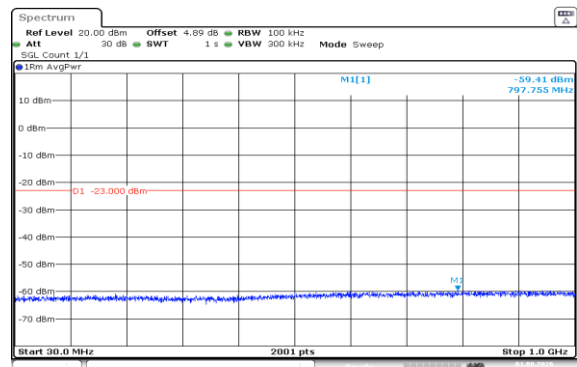
Band66-1.4MHz-QPSK-132665-1RB#5-30~1000-PASS
