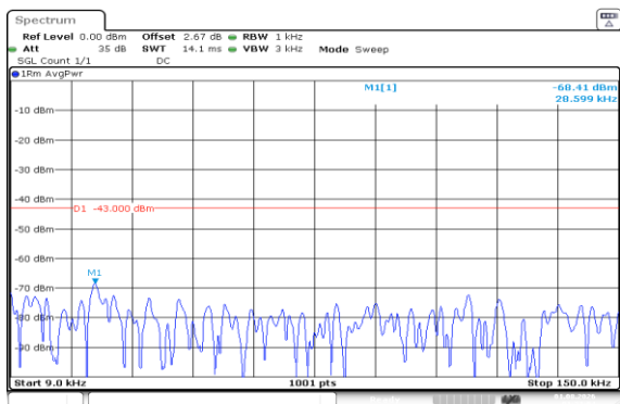
Band66-1.4MHz-16QAM-132665-1RB#0-0.009~0.15-PASS
