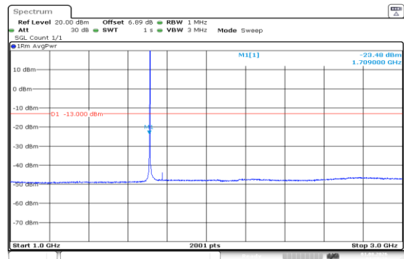
Band66-3MHz-16QAM-131987-1RB#14-1000~3000-PASS
