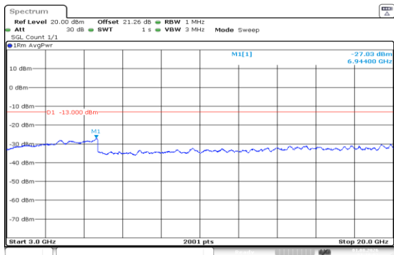
Band66-1.4MHz-16QAM-131979-1RB#5-3000~20000-PASS
