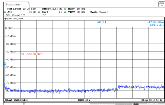
Band66-3MHz-16QAM-131987-1RB#14-0.15~30-PASS
