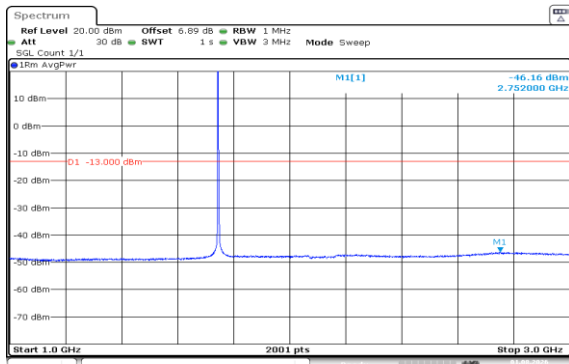
Band66-3MHz-QPSK-132322-1RB#0-1000~3000-PASS
