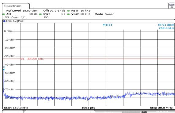
Band66-1.4MHz-16QAM-132665-1RB#5-0.15~30-PASS
