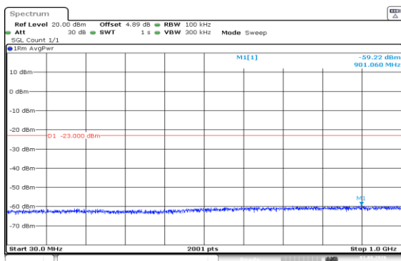
Band66-1.4MHz-16QAM-132322-1RB#0-30~1000-PASS
