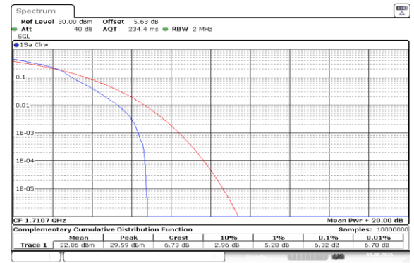
Band66-1.4MHz-16QAM-131979-1RB#0-PASS
