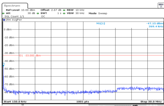
Band66-3MHz-QPSK-132322-15RB#0-0.15~30-PASS
