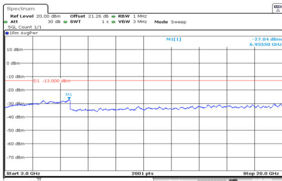
Band66-3MHz-16QAM-131987-15RB#0-3000~20000-PASS
