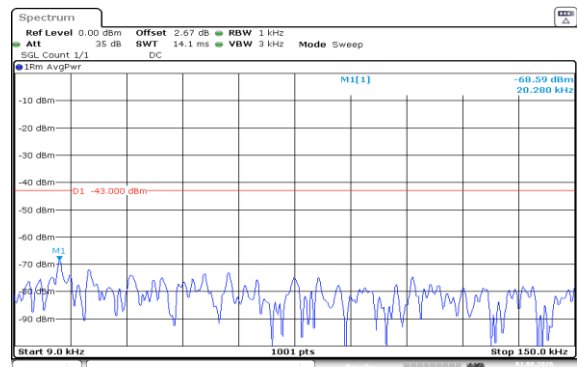
Band66-1.4MHz-16QAM-132665-6RB#0-0.009~0.15-PASS
