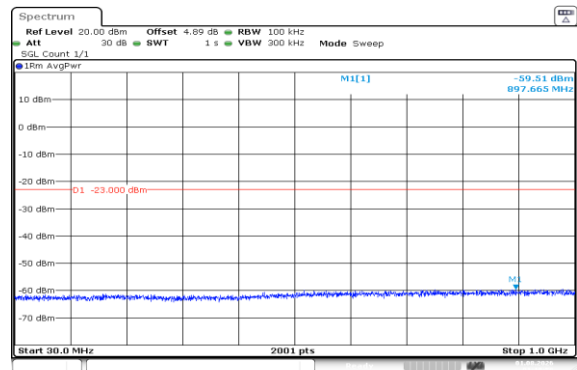
Band66-1.4MHz-16QAM-131979-6RB#0-30~1000-PASS
