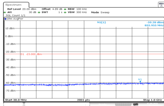
Band66-1.4MHz-QPSK-132322-1RB#5-30~1000-PASS
