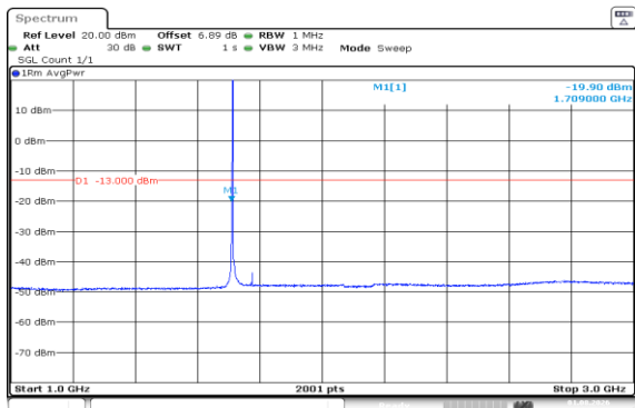
Band66-3MHz-QPSK-131987-1RB#14-1000~3000-PASS
