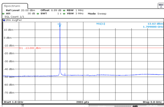
Band66-3MHz-16QAM-131987-1RB#0-1000~3000
