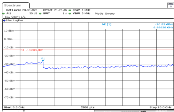
Band66-1.4MHz-QPSK-132665-6RB#0-3000~20000-PASS
