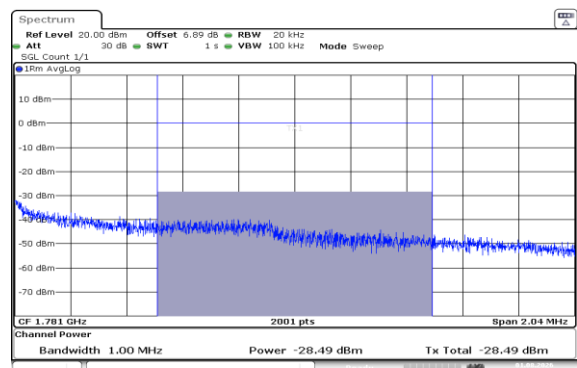
Band66-1.4MHz-QPSK-132665-6RB#0-1000~3000-PASS
