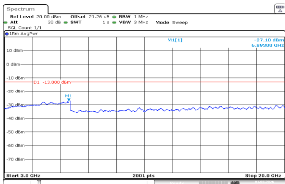
Band66-3MHz-QPSK-131987-1RB#0-3000~20000-PASS
