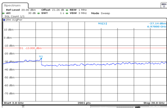
Band66-1.4MHz-QPSK-131979-1RB#5-3000~20000-PASS
