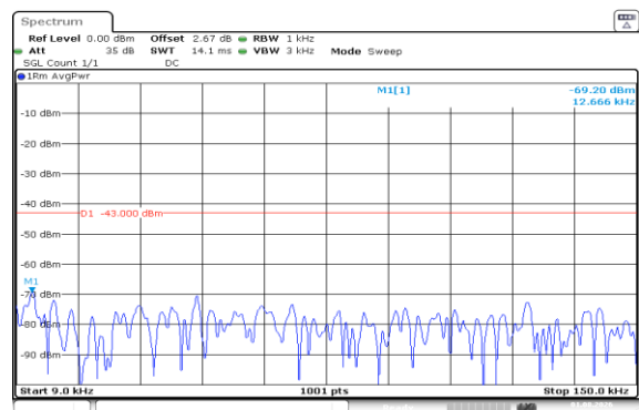
Band66-1.4MHz-QPSK-132665-1RB#5-0.009~0.15-PASS
