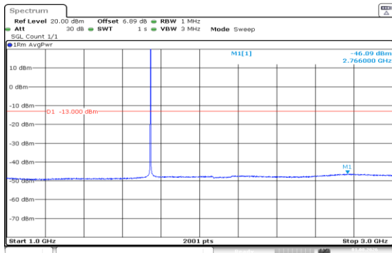
Band66-1.4MHz-QPSK-132322-1RB#5-1000~3000-PASS
