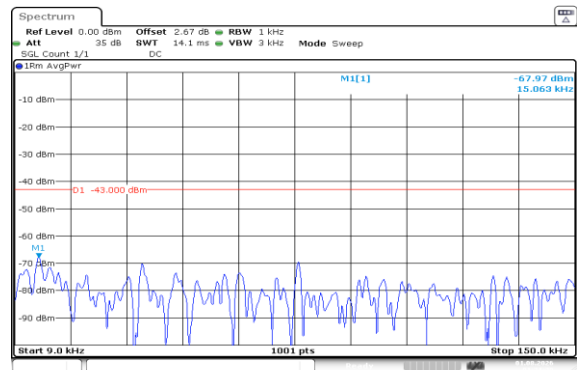
Band66-1.4MHz-QPSK-132322-6RB#0-0.009~0.15-PASS
