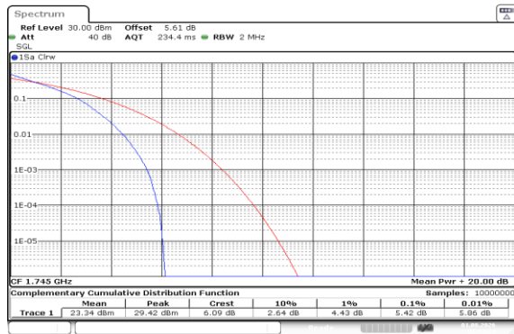
Band66-1.4MHz-QPSK-132322-6RB#0-PASS
