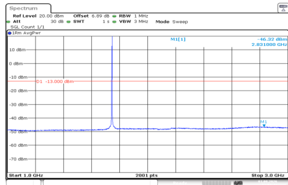
Band66-3MHz-16QAM-132322-1RB#14-1000~3000-PASS
