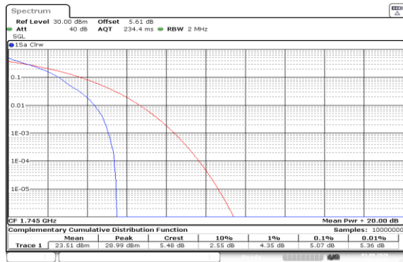
Band66-1.4MHz-QPSK-132322-1RB#0-PASS
