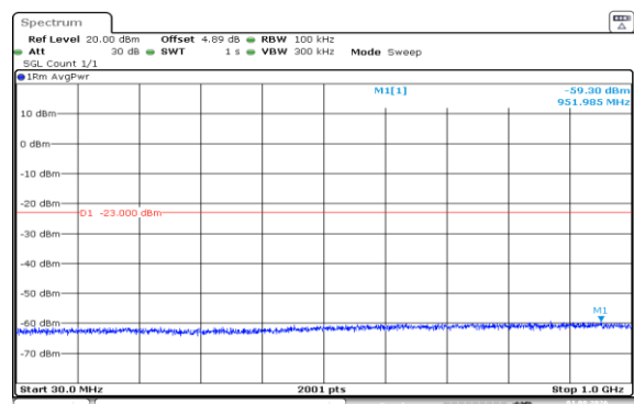
Band66-3MHz-QPSK-131987-1RB#0-30~1000-PASS
