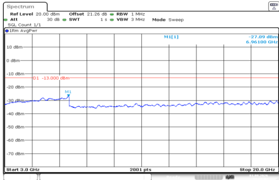
Band66-1.4MHz-16QAM-132665-1RB#5-3000~20000-PASS
