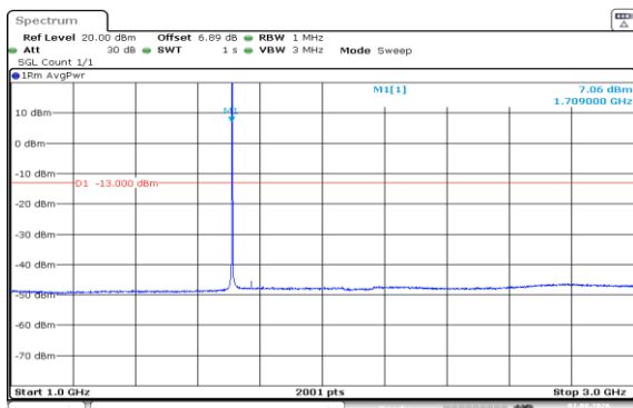
Band66-1.4MHz-16QAM-131979-6RB#0-1000~3000
