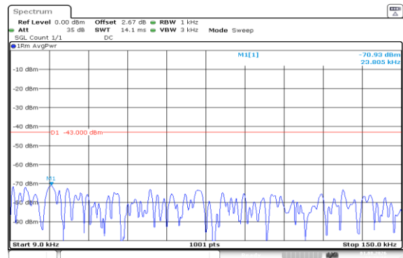
Band66-1.4MHz-QPSK-131979-6RB#0-0.009~0.15-PASS
