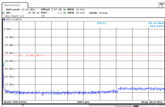
Band66-1.4MHz-QPSK-131979-1RB#5-0.15~30-PASS
