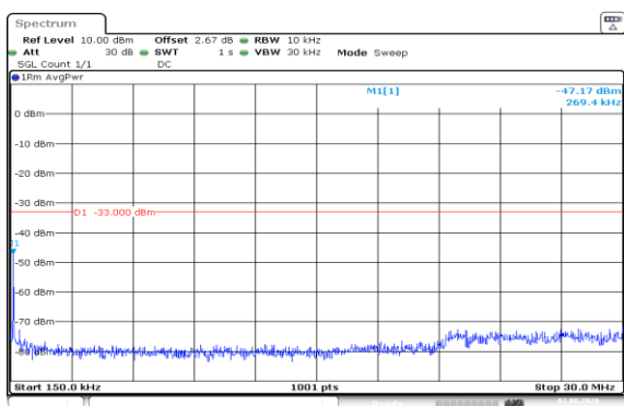
Band66-3MHz-16QAM-131987-1RB#0-0.15~30-PASS
