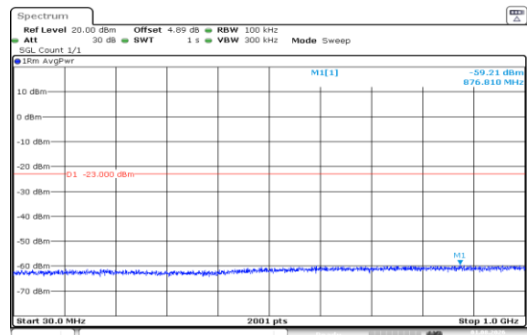
Band66-1.4MHz-QPSK-132322-1RB#0-30~1000-PASS
