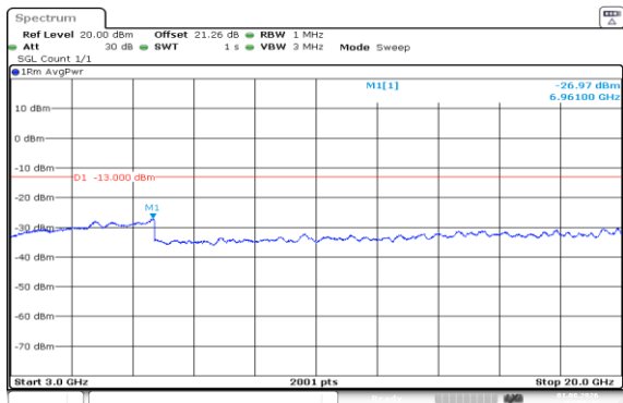
Band66-3MHz-16QAM-132322-1RB#0-3000~20000-PASS
