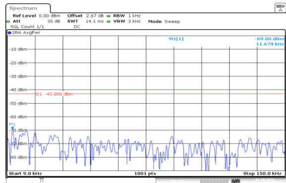
Band66-3MHz-QPSK-132322-1RB#14-0.009~0.15-PASS
