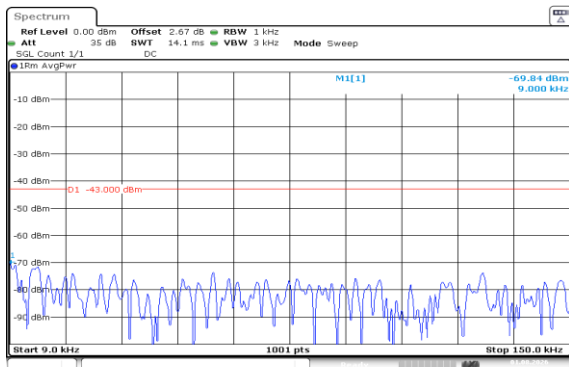
Band66-1.4MHz-16QAM-132322-1RB#5-0.009~0.15-PASS
