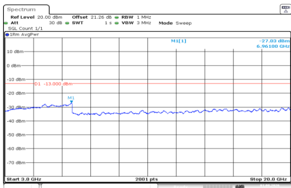
Band66-1.4MHz-QPSK-132665-1RB#5-3000~20000-PASS
