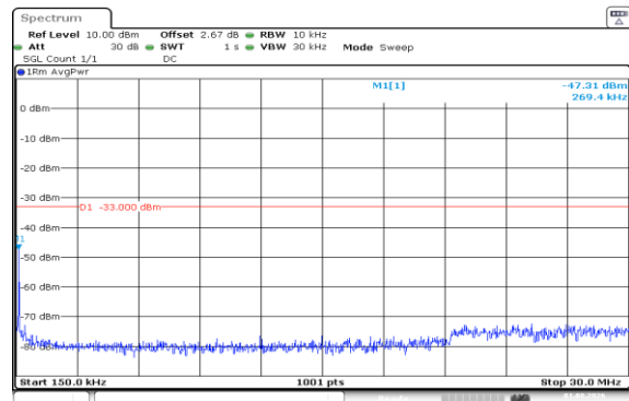
Band66-1.4MHz-16QAM-132322-1RB#5-0.15~30-PASS
