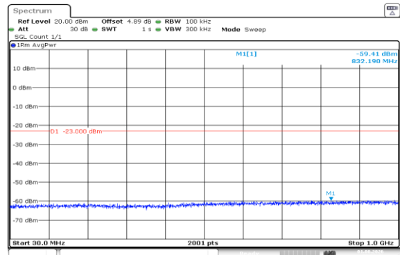
Band66-3MHz-QPSK-131987-1RB#14-30~1000-PASS
