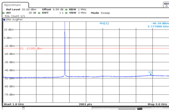
Band66-1.4MHz-QPSK-132322-1RB#0-1000~3000-PASS
