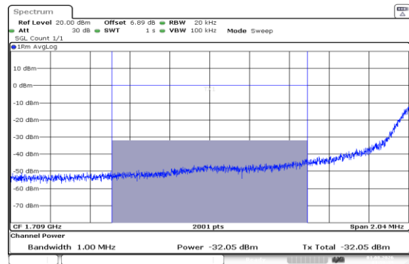
Band66-3MHz-QPSK-131987-1RB#0-1000~3000-PASS
