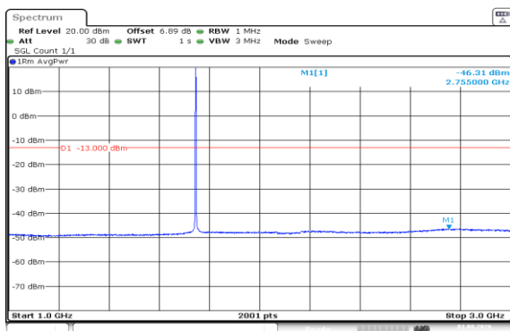
Band66-1.4MHz-QPSK-132322-6RB#0-1000~3000-PASS
