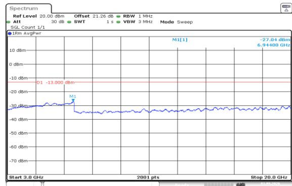
Band66-3MHz-QPSK-131987-1RB#14-3000~20000-PASS
