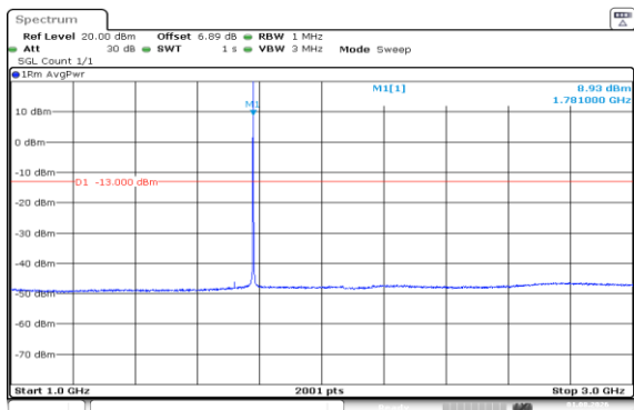
Band66-1.4MHz-16QAM-132665-1RB#5-1000~3000
