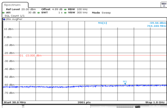
Band66-3MHz-16QAM-132322-1RB#14-30~1000-PASS
