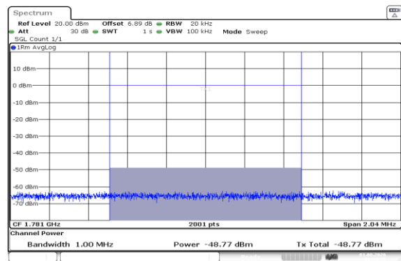
Band66-1.4MHz-QPSK-132665-1RB#5-1000~3000-PASS
