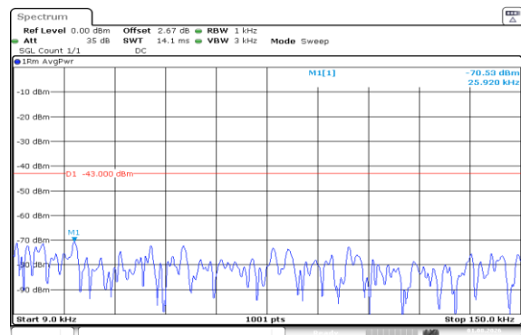
Band66-1.4MHz-16QAM-132665-1RB#5-0.009~0.15-PASS
