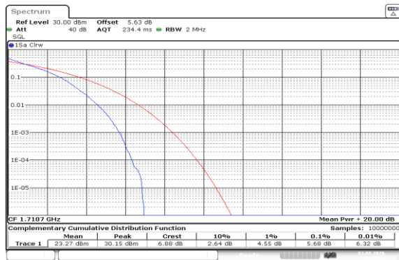
Band66-1.4MHz-QPSK-131979-6RB#0-PASS
