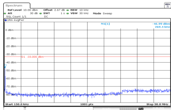
Band66-1.4MHz-16QAM-131979-1RB#0-0.15~30-PASS
