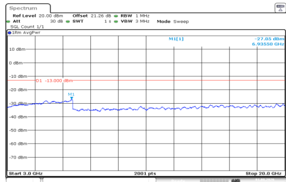
Band66-3MHz-QPSK-132322-1RB#14-3000~20000-PASS
