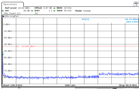
Band66-1.4MHz-QPSK-132665-1RB#5-0.15~30-PASS
