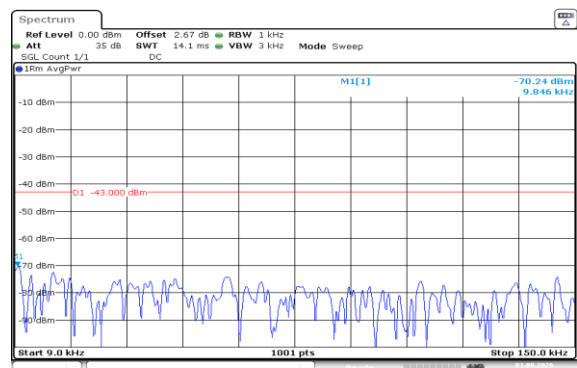
Band66-3MHz-QPSK-131987-1RB#0-0.009~0.15-PASS
