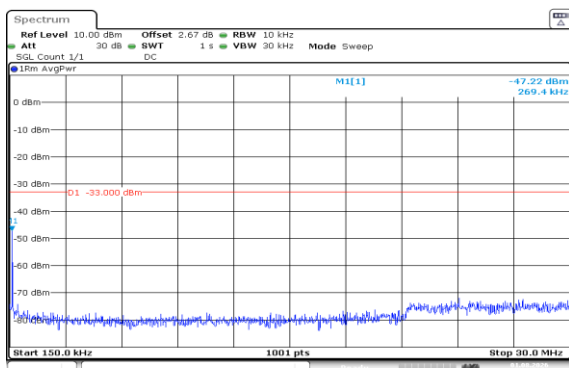
Band66-3MHz-QPSK-131987-15RB#0-0.15~30-PASS
