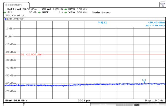
Band66-3MHz-QPSK-132322-1RB#0-30~1000-PASS
