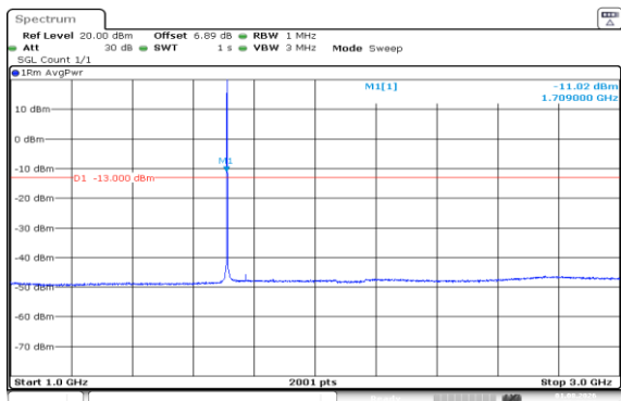
Band66-1.4MHz-16QAM-131979-1RB#5-1000~3000
