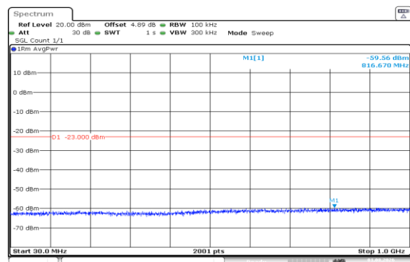
Band66-3MHz-QPSK-132322-15RB#0-30~1000-PASS
