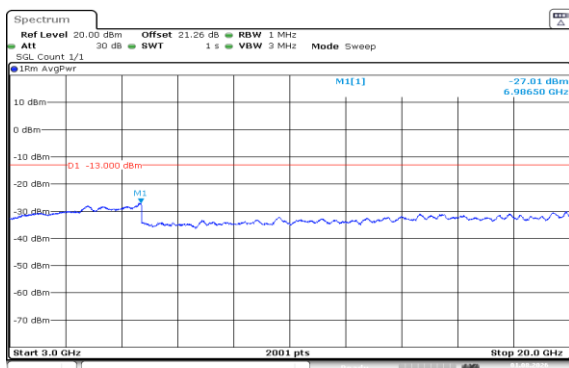
Band66-1.4MHz-16QAM-132665-6RB#0-3000~20000-PASS
