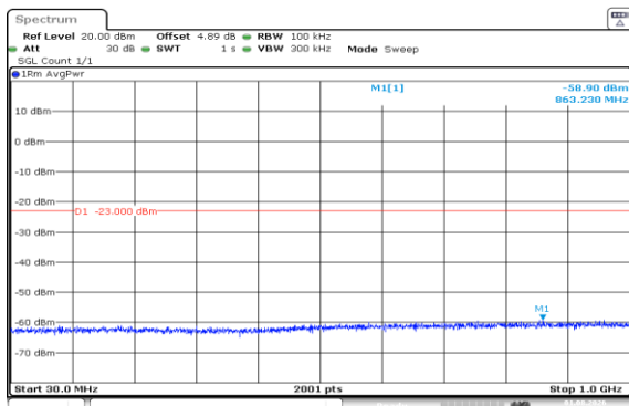
Band66-1.4MHz-16QAM-132322-1RB#5-30~1000-PASS
