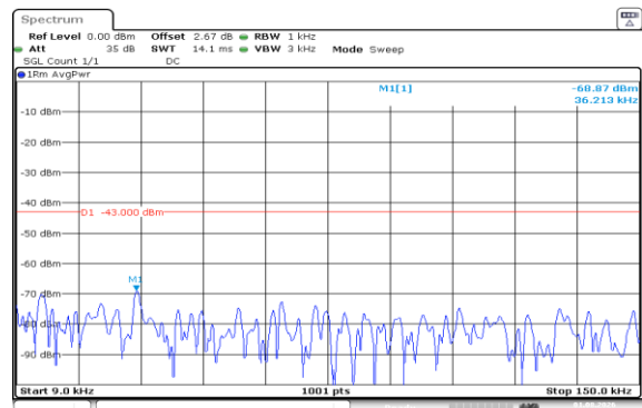
Band66-3MHz-QPSK-132322-1RB#0-0.009~0.15-PASS
