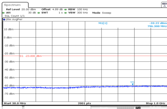
Band66-1.4MHz-16QAM-132322-6RB#0-30~1000-PASS
