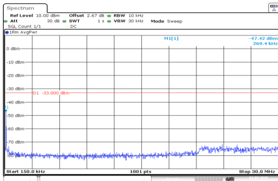
Band66-1.4MHz-16QAM-131979-6RB#0-0.15~30-PASS
