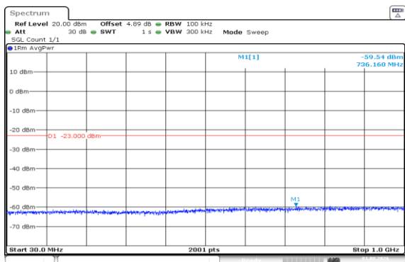
Band66-1.4MHz-16QAM-131979-1RB#0-30~1000-PASS
