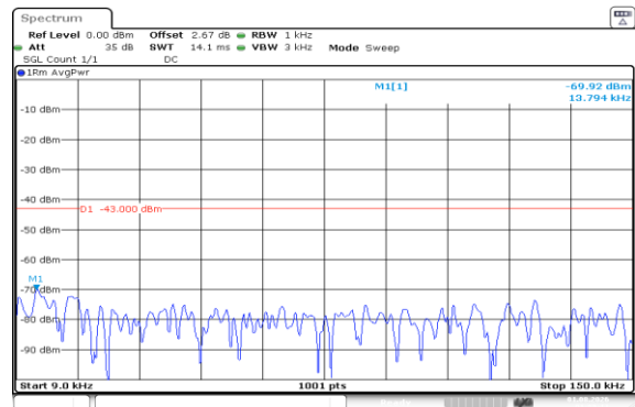
Band66-3MHz-16QAM-131987-15RB#0-0.009~0.15-PASS
