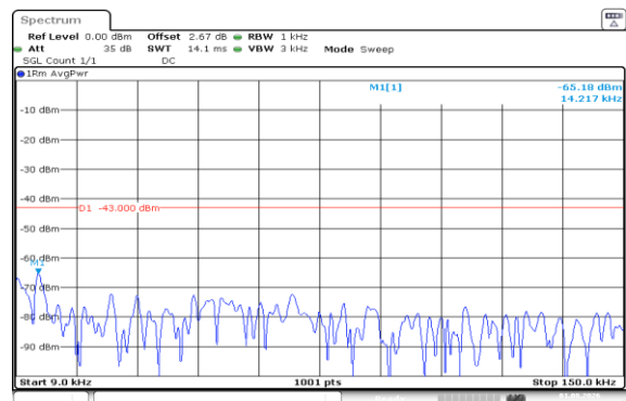
Band66-1.4MHz-16QAM-131979-1RB#5-0.009~0.15-PASS
