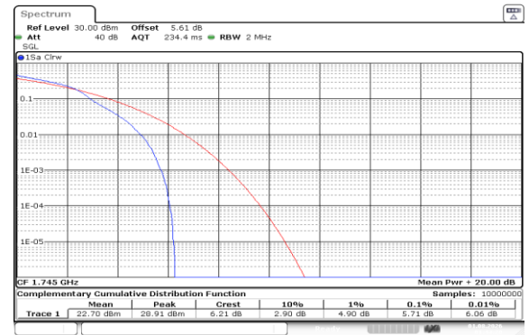
Band66-1.4MHz-16QAM-132322-1RB#0-PASS
