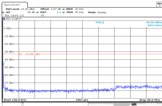
Band66-1.4MHz-QPSK-132322-1RB#5-0.15~30-PASS
