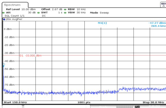
Band66-1.4MHz-16QAM-132665-6RB#0-0.15~30-PASS
