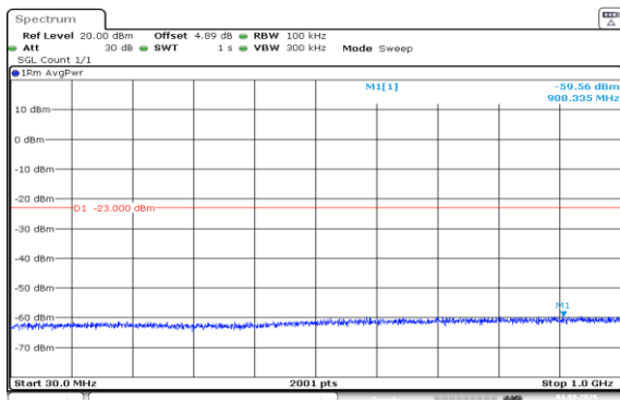
Band66-3MHz-16QAM-132322-1RB#0-30~1000-PASS
