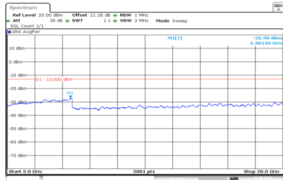
Band66-1.4MHz-QPSK-132322-1RB#5-3000~20000-PASS
