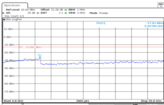
Band66-3MHz-16QAM-132322-1RB#14-3000~20000-PASS
