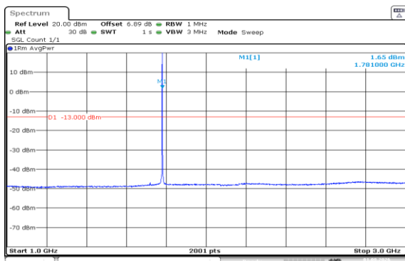
Band66-1.4MHz-16QAM-132665-6RB#0-1000~3000
