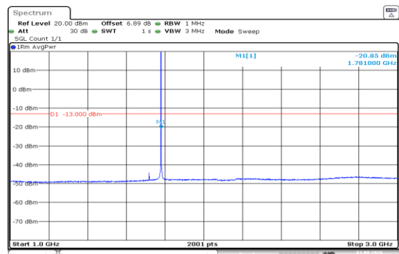
Band66-1.4MHz-16QAM-132665-1RB#0-1000~3000-PASS
