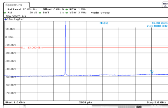
Band66-1.4MHz-16QAM-132322-6RB#0-1000~3000-PASS
