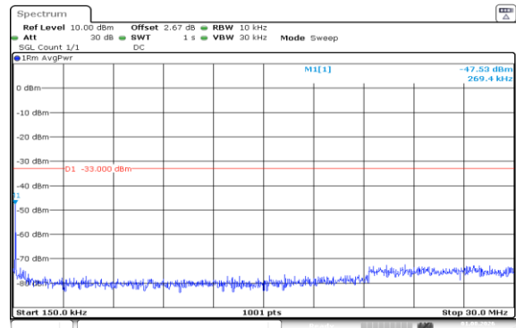
Band66-3MHz-16QAM-132322-1RB#14-0.15~30-PASS
