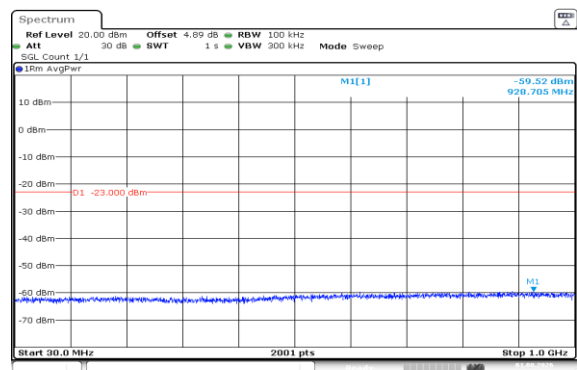
Band66-1.4MHz-16QAM-131979-1RB#5-30~1000-PASS
