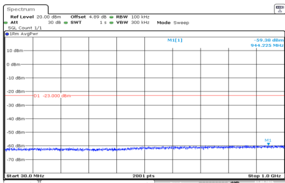
Band66-1.4MHz-16QAM-132665-1RB#0-30~1000-PASS
