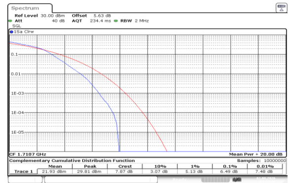
Band66-1.4MHz-16QAM-131979-6RB#0-PASS
