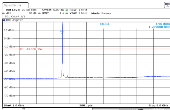
Band66-3MHz-QPSK-131987-15RB#0-1000~3000
