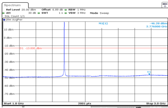
Band66-3MHz-QPSK-132322-15RB#0-1000~3000-PASS
