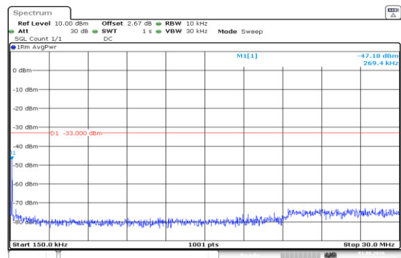
Band66-1.4MHz-16QAM-132665-1RB#0-0.15~30-PASS
