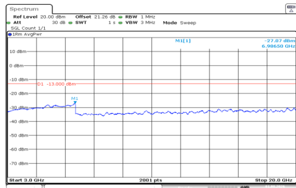
Band66-1.4MHz-QPSK-132665-1RB#0-3000~20000-PASS
