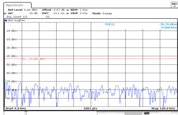
Band66-3MHz-QPSK-131987-1RB#14-0.009~0.15-PASS
