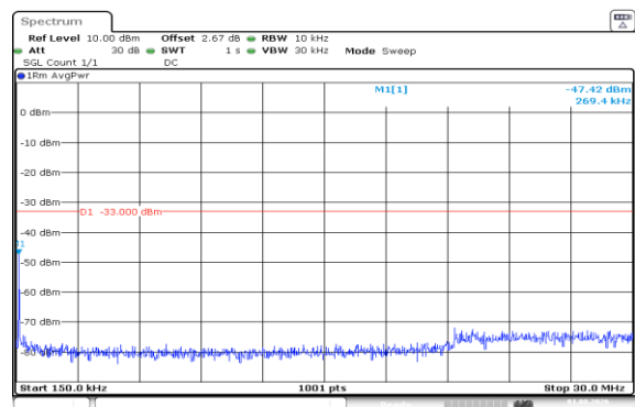
Band66-3MHz-16QAM-132322-1RB#0-0.15~30-PASS
