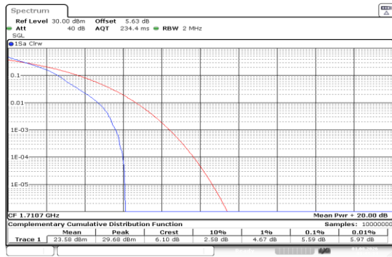
Band66-1.4MHz-QPSK-131979-1RB#0-PASS
