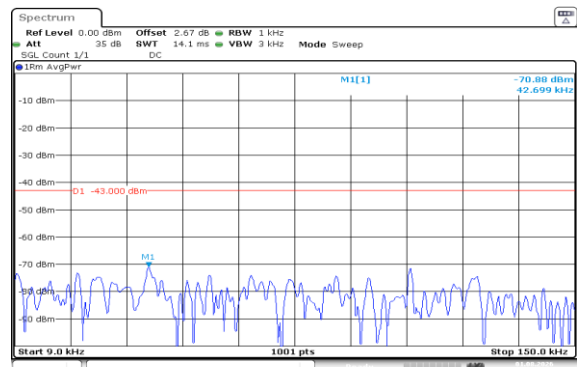
Band66-1.4MHz-QPSK-132322-1RB#5-0.009~0.15-PASS
