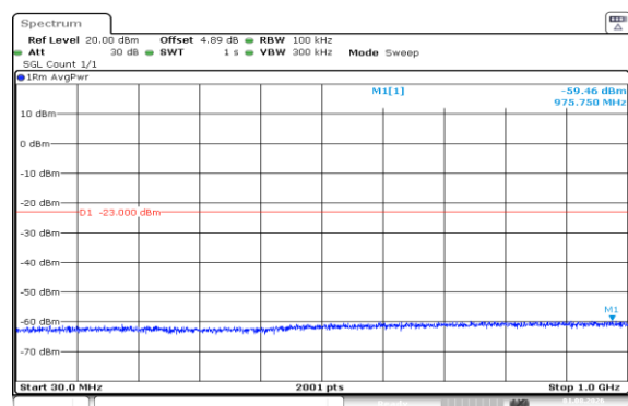
Band66-3MHz-16QAM-131987-1RB#0-30~1000-PASS
