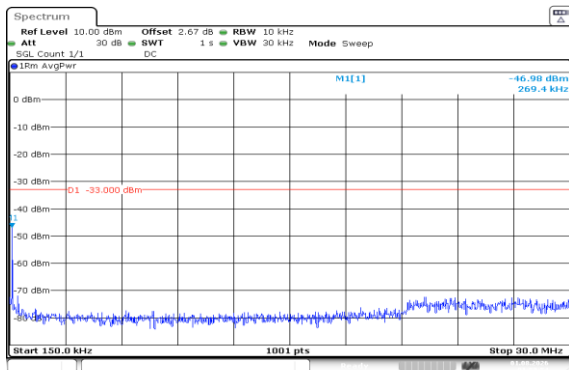
Band66-3MHz-QPSK-132322-1RB#0-0.15~30-PASS
