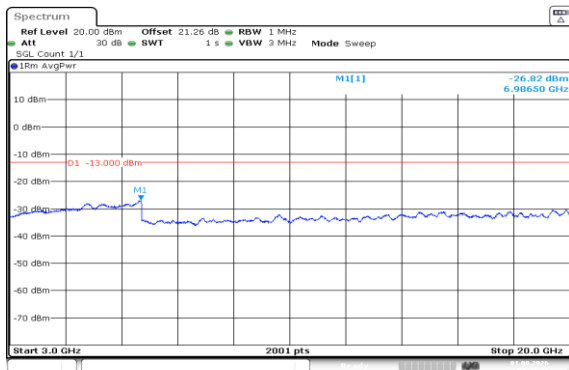
Band66-1.4MHz-16QAM-132322-1RB#5-3000~20000-PASS
