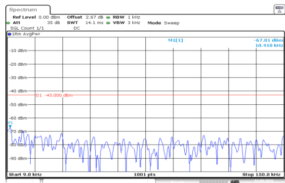
Band66-1.4MHz-QPSK-131979-1RB#5-0.009~0.15-PASS
