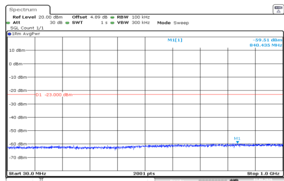
Band66-3MHz-QPSK-131987-15RB#0-30~1000-PASS
