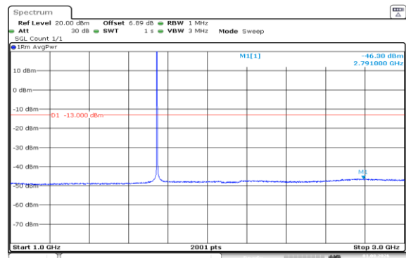
Band66-3MHz-16QAM-132322-1RB#0-1000~3000-PASS
