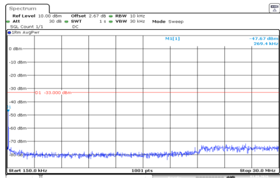
Band66-1.4MHz-16QAM-132322-6RB#0-0.15~30-PASS
