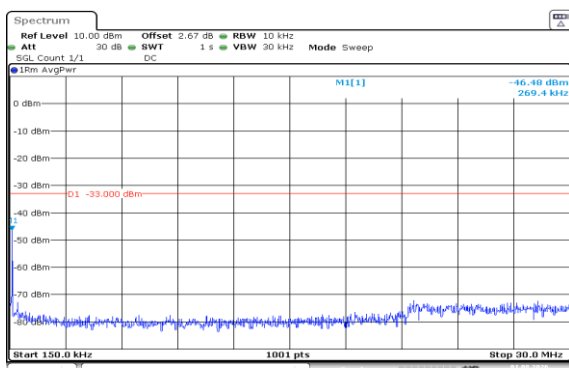
Band66-3MHz-QPSK-131987-1RB#0-0.15~30-PASS
