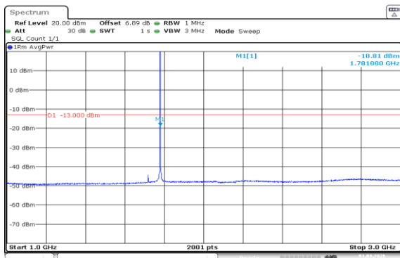
Band66-1.4MHz-QPSK-132665-1RB#0-1000~3000-PASS
