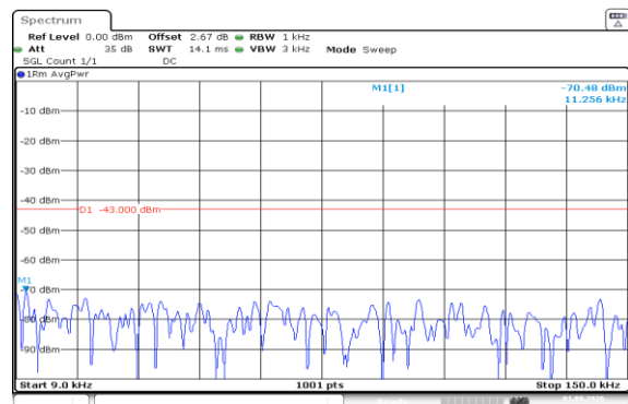
Band66-3MHz-16QAM-131987-1RB#0-0.009~0.15-PASS
