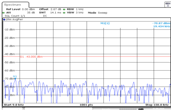
Band66-3MHz-16QAM-132322-1RB#14-0.009~0.15-PASS
