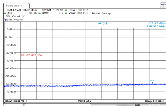
Band66-1.4MHz-16QAM-132665-1RB#5-30~1000-PASS
