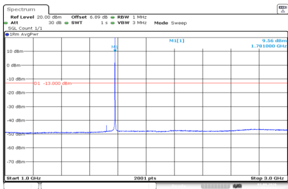
Band66-1.4MHz-QPSK-132665-1RB#5-1000~3000
