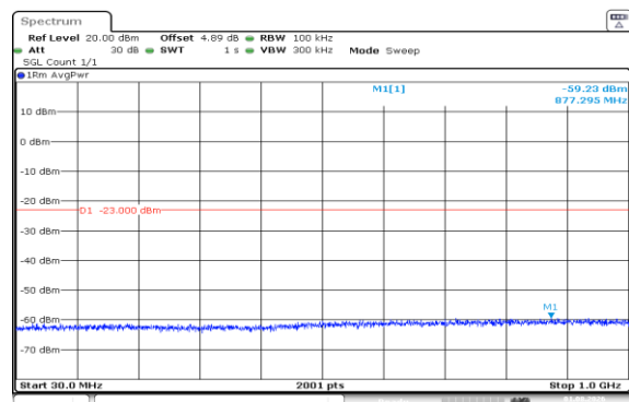
Band66-1.4MHz-QPSK-132665-1RB#0-30~1000-PASS
