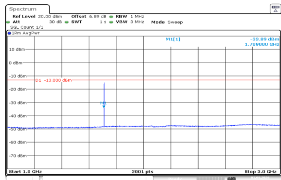
Band66-1.4MHz-16QAM-131979-1RB#0-1000~3000-PASS
