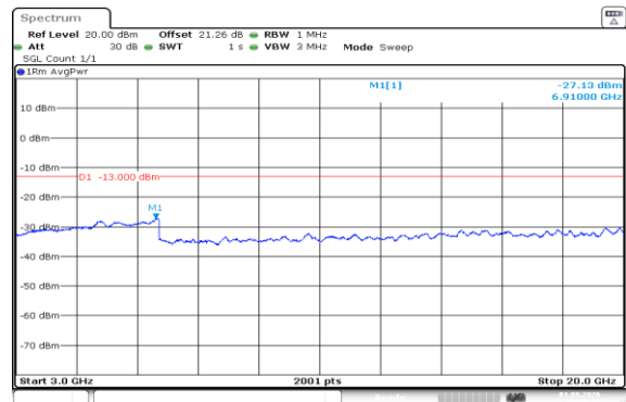
Band66-1.4MHz-QPSK-132322-1RB#0-3000~20000-PASS
