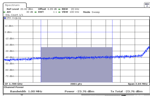
Band66-3MHz-16QAM-131987-15RB#0-1000~3000-PASS
