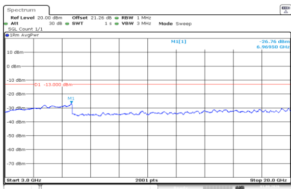
Band66-1.4MHz-16QAM-132665-1RB#0-3000~20000-PASS
