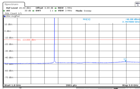
Band66-1.4MHz-16QAM-132322-1RB#5-1000~3000-PASS
