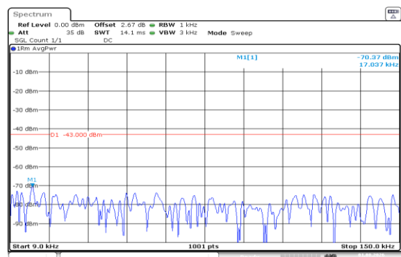
Band66-1.4MHz-16QAM-131979-6RB#0-0.009~0.15-PASS
