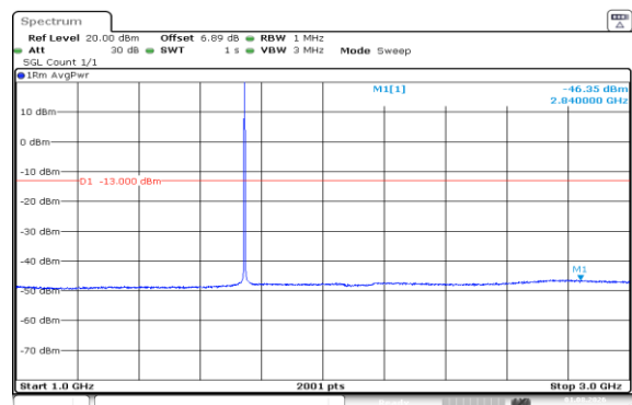
Band66-1.4MHz-16QAM-132322-1RB#0-1000~3000-PASS
