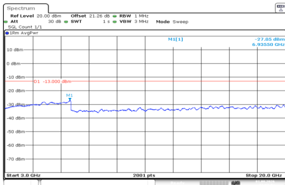
Band66-3MHz-QPSK-131987-15RB#0-3000~20000-PASS
