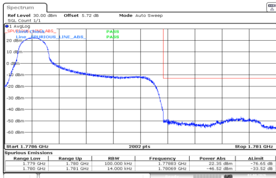
Band66-1.4MHz-QPSK-132665-1RB#0-PASS
