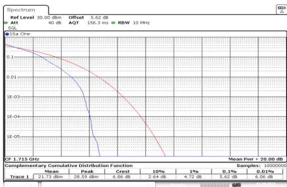
Band66-10MHz-QPSK-132022-1RB#0-PASS
