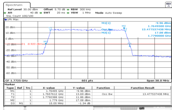
Band66-15MHz-16QAM-132597-75RB#0-PASS
