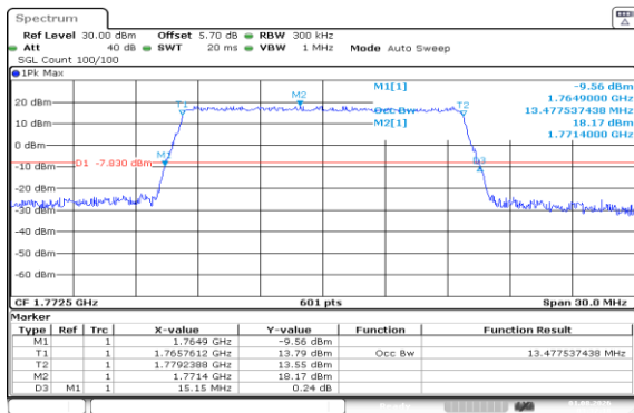
Band66-15MHz-QPSK-132597-75RB#0-PASS
