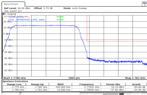
Band66-1.4MHz-QPSK-132665-6RB#0-PASS
