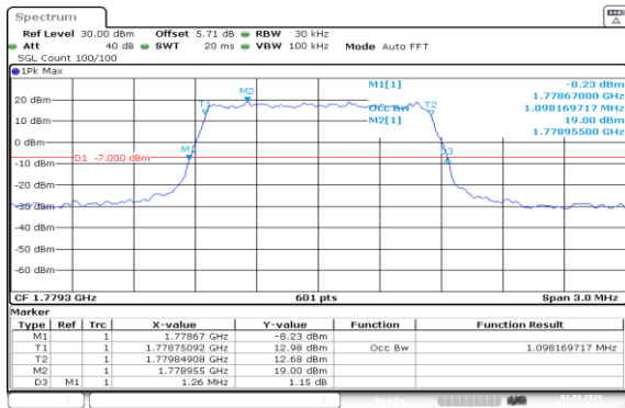
Band66-1.4MHz-QPSK-132665-6RB#0-PASS
