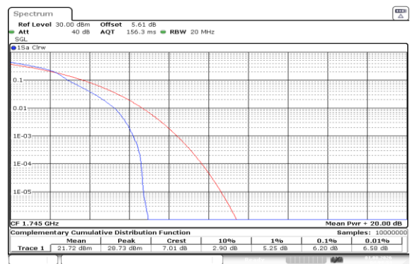
Band66-15MHz-16QAM-132322-1RB#0-PASS
