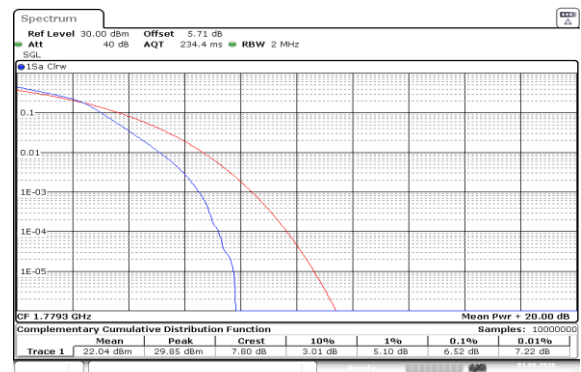
Band66-1.4MHz-16QAM-132665-6RB#0-PASS
