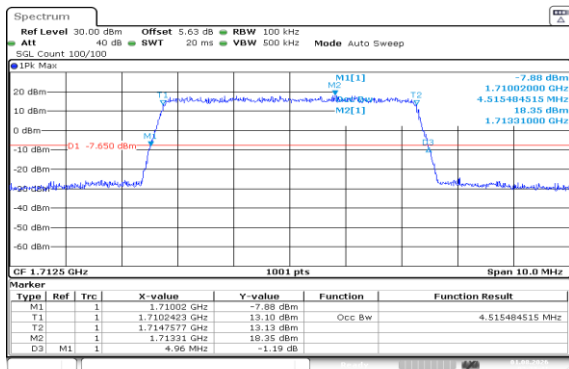
Band66-5MHz-QPSK-131997-25RB#0-PASS
