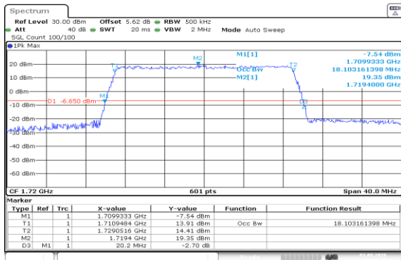
Band66-20MHz-QPSK-132072-100RB#0-PASS
