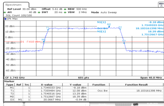
Band66-20MHz-16QAM-132322-100RB#0-PASS
