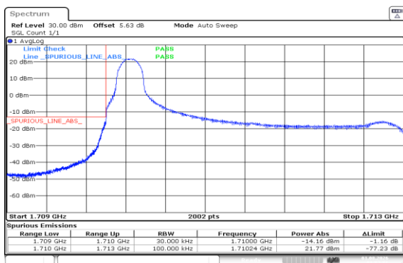
Band66-3MHz-QPSK-131987-1RB#0-PASS
