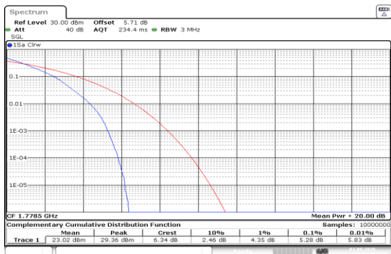
Band66-3MHz-QPSK-132657-15RB#0-PASS
