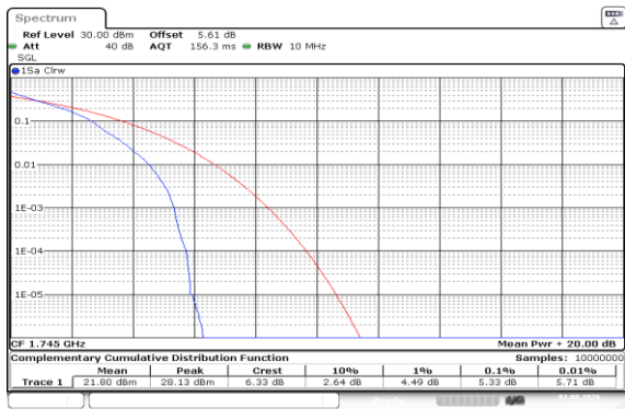
Band66-10MHz-QPSK-132322-1RB#0-PASS
