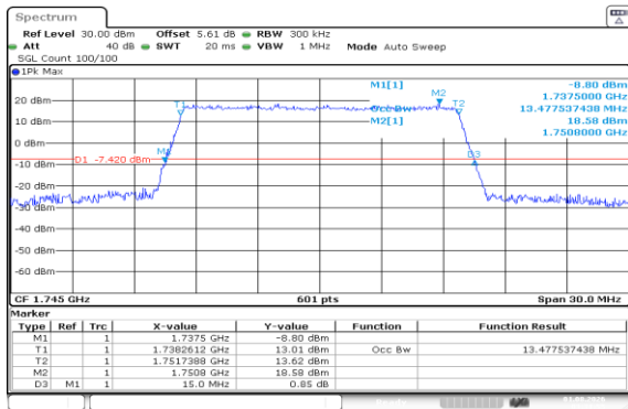
Band66-15MHz-QPSK-132322-75RB#0-PASS
