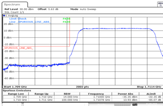
Band66-1.4MHz-QPSK-131979-6RB#0-PASS
