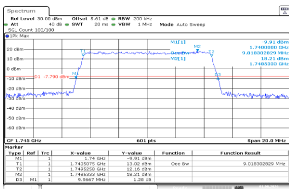
Band66-10MHz-QPSK-132322-50RB#0-PASS
