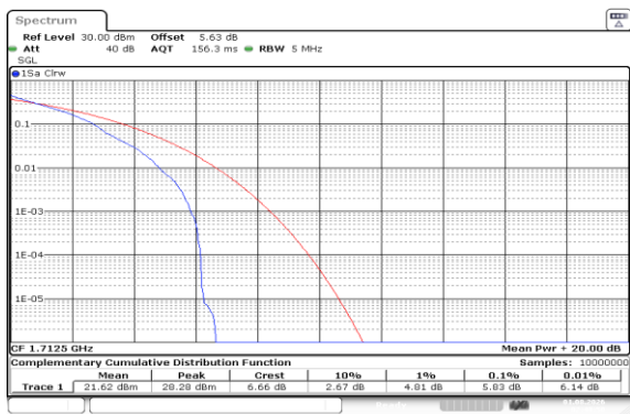
Band66-5MHz-QPSK-131997-1RB#0-PASS
