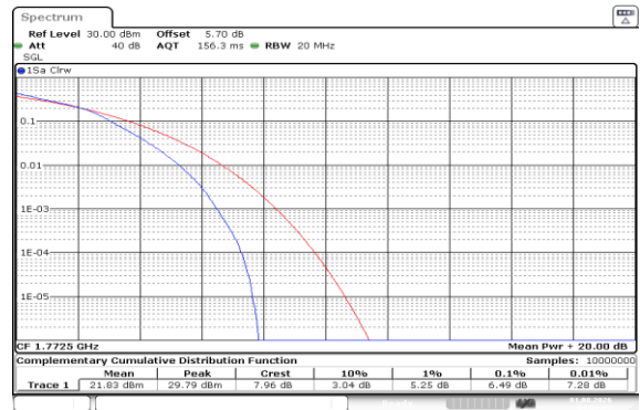
Band66-15MHz-16QAM-132597-75RB#0-PASS
