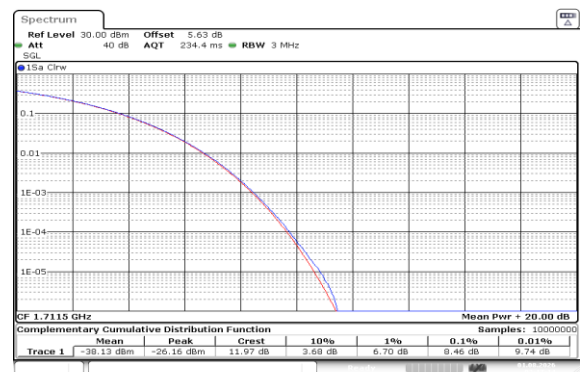
Band66-3MHz-16QAM-131987-1RB#0-PASS
