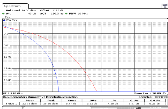
Band66-10MHz-QPSK-132022-50RB#0-PASS
