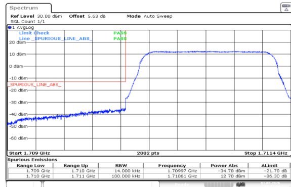
Band66-1.4MHz-16QAM-131979-6RB#0-PASS
