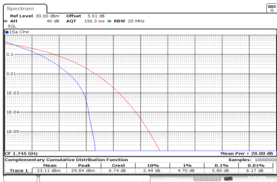
Band66-15MHz-QPSK-132322-75RB#0-PASS
