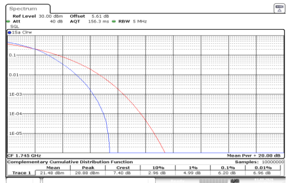
Band66-5MHz-16QAM-132322-25RB#0-PASS
