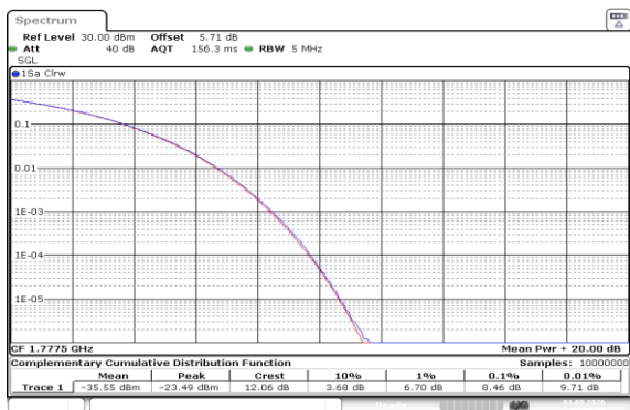
Band66-5MHz-QPSK-132647-25RB#0-PASS
