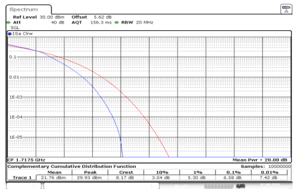
Band66-15MHz-16QAM-132047-75RB#0-PASS
