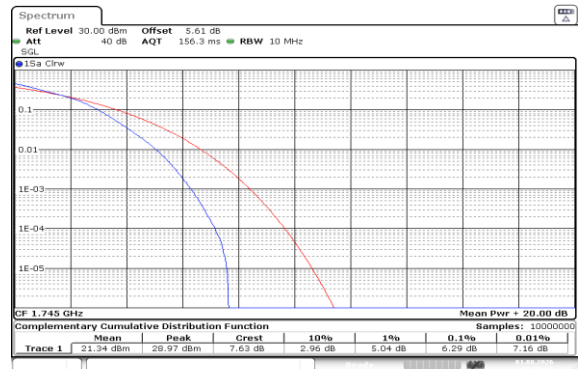
Band66-10MHz-16QAM-132322-50RB#0-PASS
