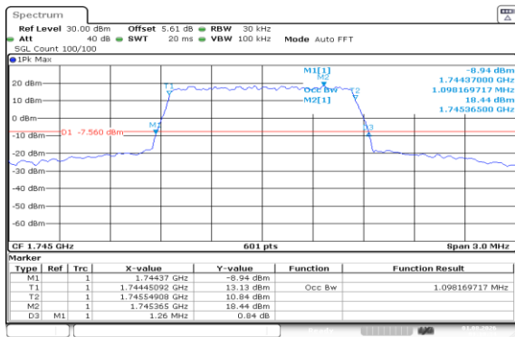
Band66-1.4MHz-QPSK-132322-6RB#0-PASS
