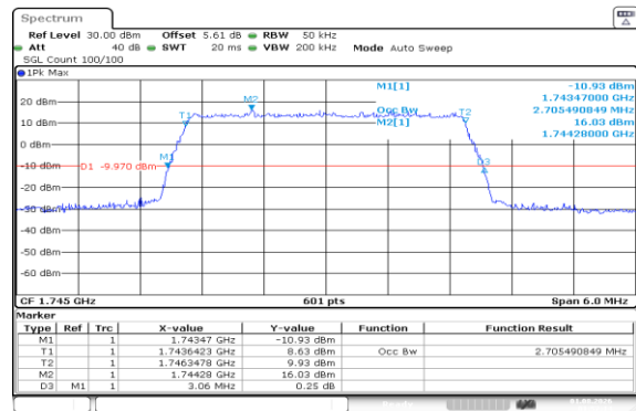
Band66-3MHz-16QAM-132322-15RB#0-PASS
