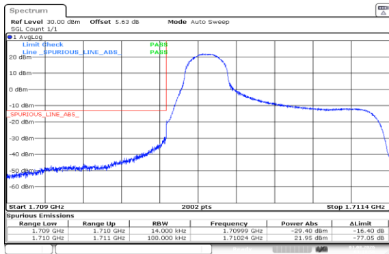
Band66-1.4MHz-QPSK-131979-1RB#0-PASS
