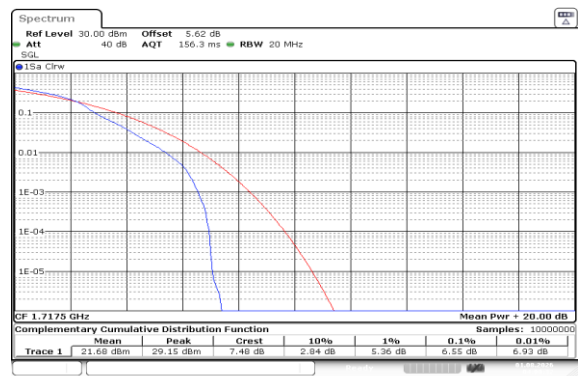
Band66-15MHz-16QAM-132047-1RB#0-PASS
