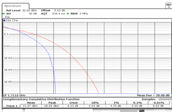
Band66-3MHz-QPSK-131987-1RB#0-PASS
