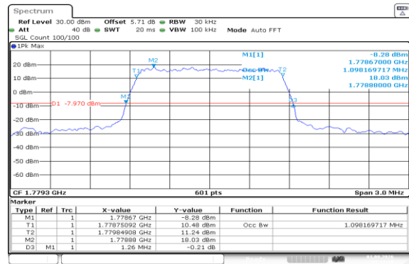
Band66-1.4MHz-16QAM-132665-6RB#0-PASS
