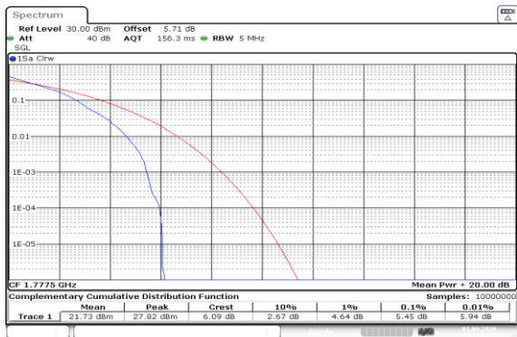
Band66-5MHz-QPSK-132647-1RB#0-PASS
