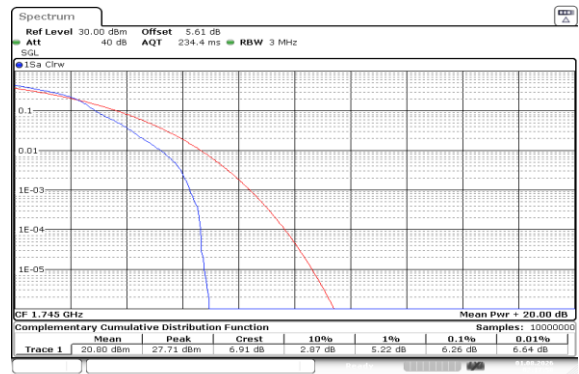
Band66-3MHz-16QAM-132322-1RB#0-PASS
