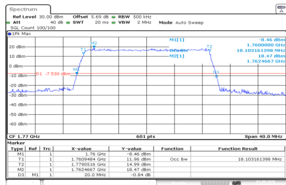
Band66-20MHz-16QAM-132572-100RB#0-PASS
