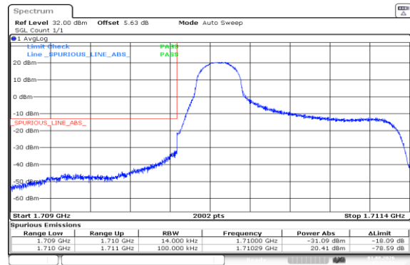
Band66-1.4MHz-16QAM-131979-1RB#0-PASS
