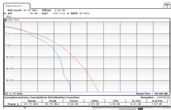
Band66-20MHz-16QAM-132572-1RB#0-PASS
