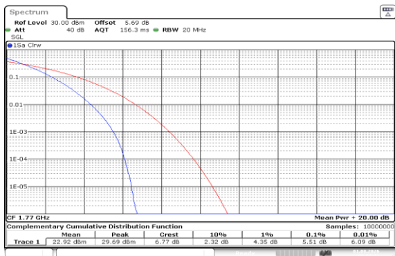
Band66-20MHz-QPSK-132572-100RB#0-PASS
