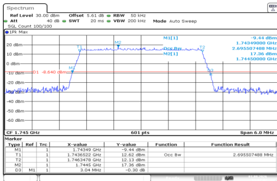
Band66-3MHz-QPSK-132322-15RB#0-PASS
