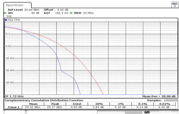
Band66-20MHz-16QAM-132072-1RB#0-PASS
