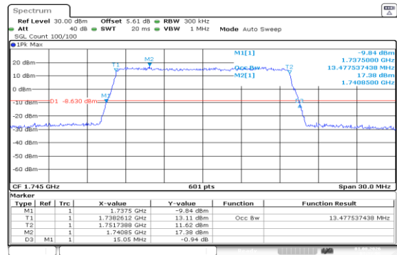
Band66-15MHz-16QAM-132322-75RB#0-PASS
