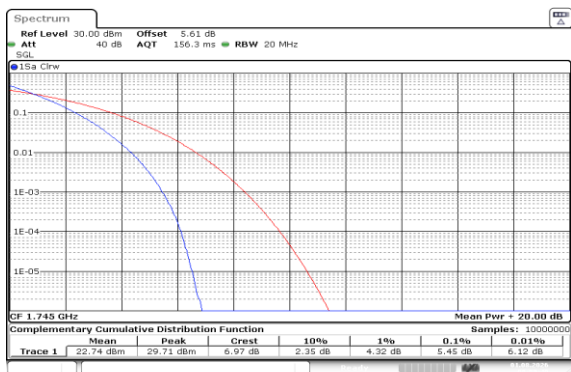
Band66-20MHz-QPSK-132322-100RB#0-PASS
