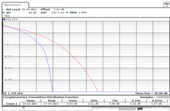
Band66-3MHz-QPSK-132322-1RB#0-PASS
