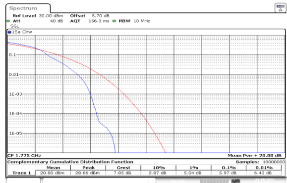
Band66-10MHz-16QAM-132622-1RB#0-PASS
