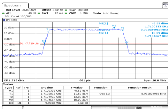
Band66-10MHz-QPSK-132022-50RB#0-PASS
