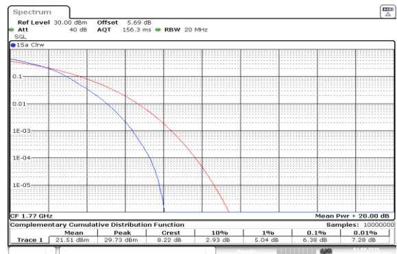
Band66-20MHz-16QAM-132572-100RB#0-PASS
