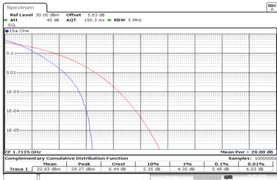
Band66-5MHz-QPSK-131997-25RB#0-PASS
