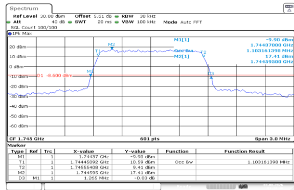
Band66-1.4MHz-16QAM-132322-6RB#0-PASS
