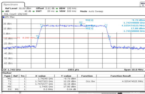
Band66-5MHz-QPSK-132322-25RB#0-PASS
