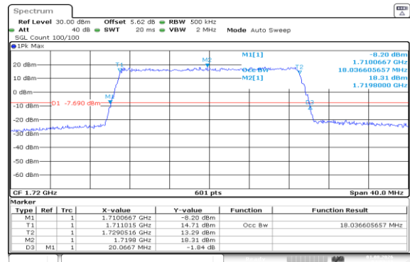
Band66-20MHz-16QAM-132072-100RB#0-PASS
