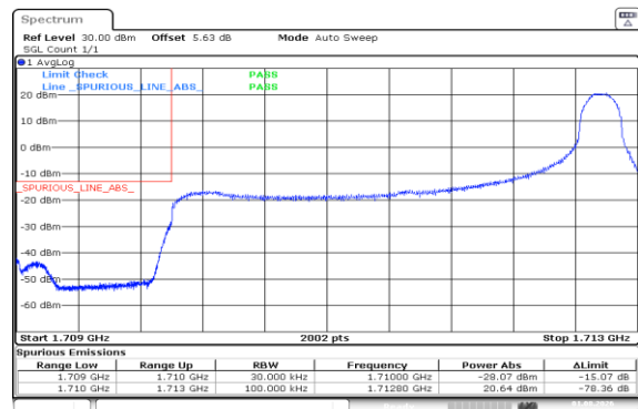
Band66-3MHz-16QAM-131987-1RB#14-PASS
