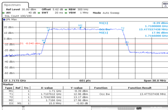
Band66-15MHz-QPSK-132047-75RB#0-PASS
