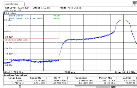
Band66-1.4MHz-16QAM-131979-1RB#5-PASS
