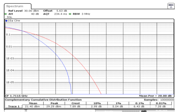
Band66-3MHz-16QAM-131987-15RB#0-PASS
