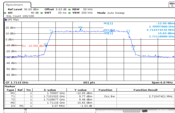
Band66-3MHz-16QAM-131987-15RB#0-PASS
