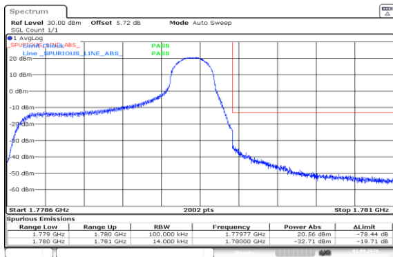
Band66-1.4MHz-QPSK-132665-1RB#5-PASS
