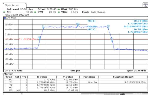
Band66-10MHz-16QAM-132622-50RB#0-PASS
