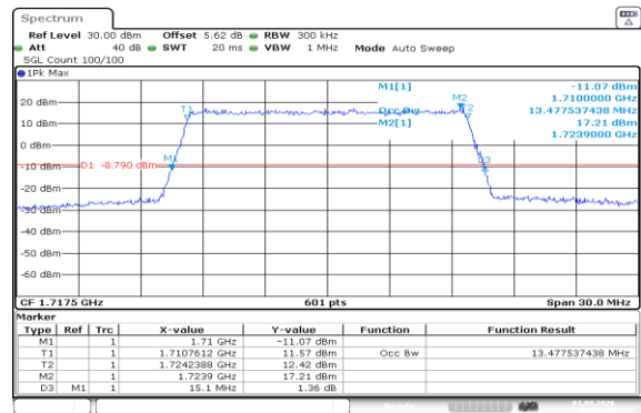
Band66-15MHz-16QAM-132047-75RB#0-PASS
