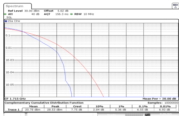
Band66-10MHz-16QAM-132022-1RB#0-PASS
