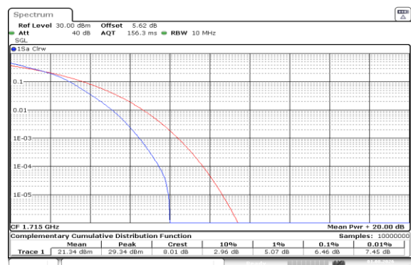
Band66-10MHz-16QAM-132022-50RB#0-PASS
