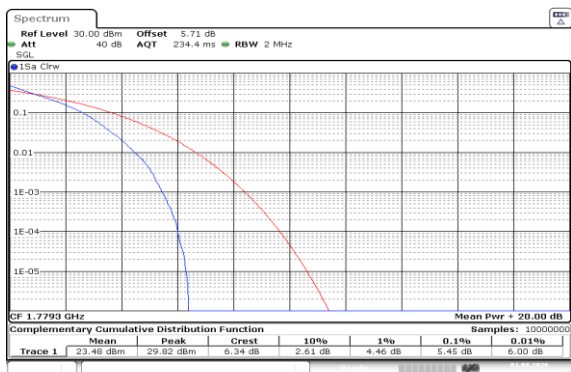
Band66-1.4MHz-QPSK-132665-6RB#0-PASS
