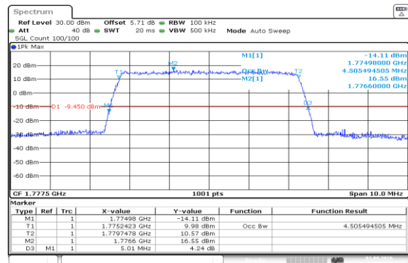
Band66-5MHz-16QAM-132647-25RB#0-PASS
