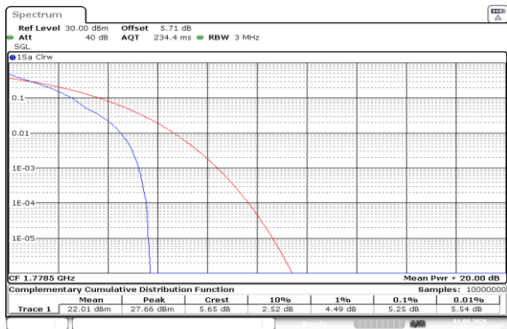
Band66-3MHz-QPSK-132657-1RB#0-PASS
