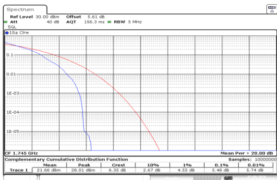
Band66-5MHz-QPSK-132322-1RB#0-PASS
