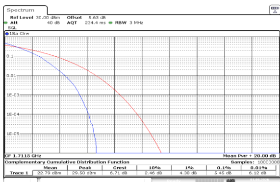
Band66-3MHz-QPSK-131987-15RB#0-PASS
