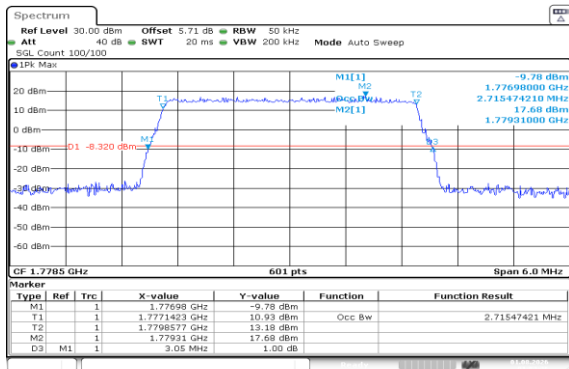
Band66-3MHz-QPSK-132657-15RB#0-PASS
