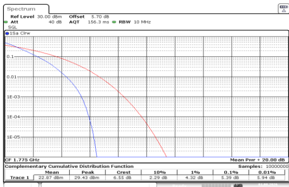
Band66-10MHz-QPSK-132622-50RB#0-PASS
