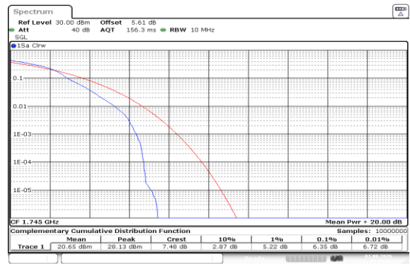
Band66-10MHz-16QAM-132322-1RB#0-PASS
