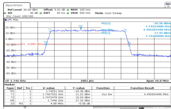
Band66-5MHz-16QAM-132322-25RB#0-PASS
