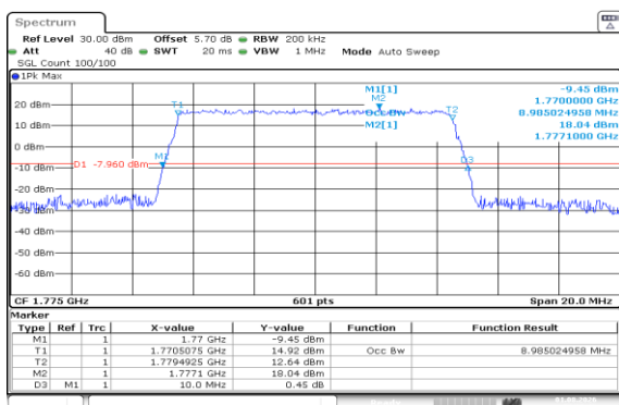
Band66-10MHz-QPSK-132622-50RB#0-PASS
