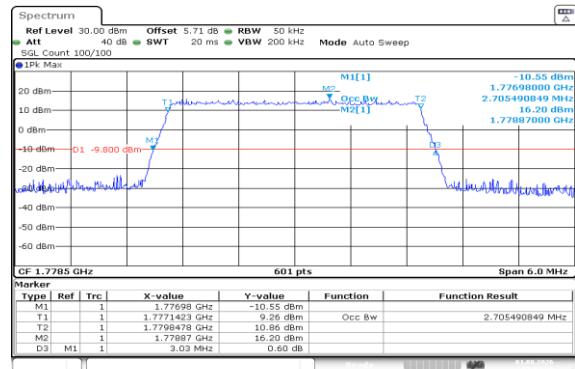
Band66-3MHz-16QAM-132657-15RB#0-PASS
