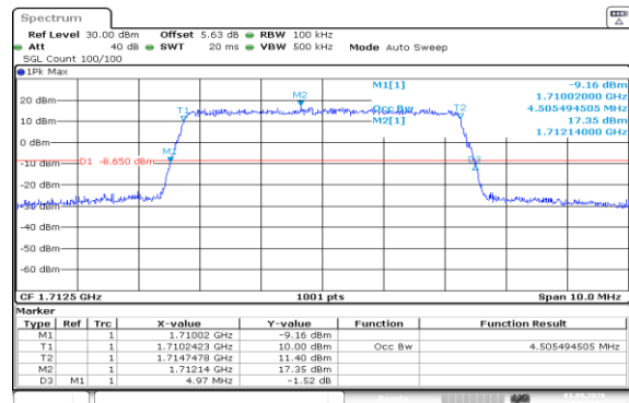
Band66-5MHz-16QAM-131997-25RB#0-PASS
