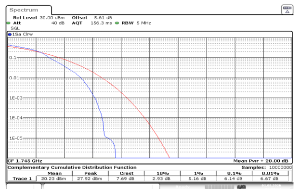
Band66-5MHz-16QAM-132322-1RB#0-PASS
