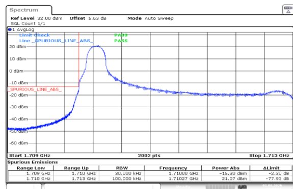
Band66-3MHz-16QAM-131987-1RB#0-PASS
