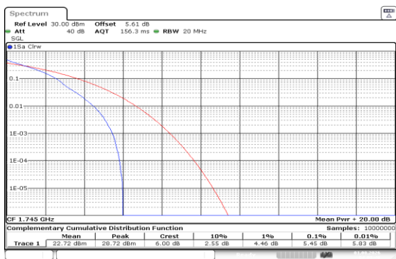
Band66-15MHz-QPSK-132322-1RB#0-PASS
