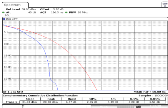
Band66-10MHz-QPSK-132622-1RB#0-PASS
