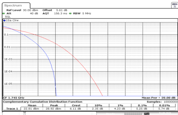
Band66-5MHz-QPSK-132322-25RB#0-PASS
