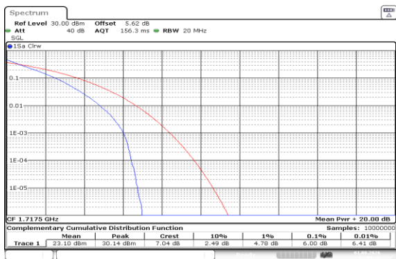
Band66-15MHz-QPSK-132047-75RB#0-PASS
