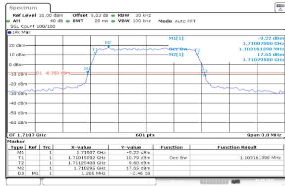
Band66-1.4MHz-16QAM-131979-6RB#0-PASS
