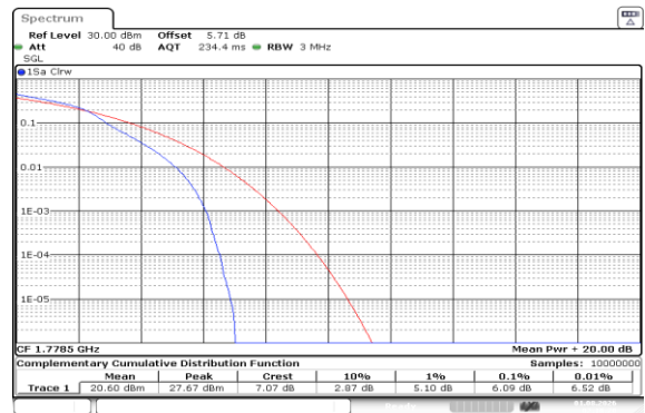
Band66-3MHz-16QAM-132657-1RB#0-PASS
