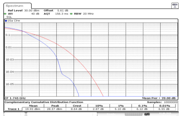
Band66-20MHz-16QAM-132322-1RB#0-PASS
