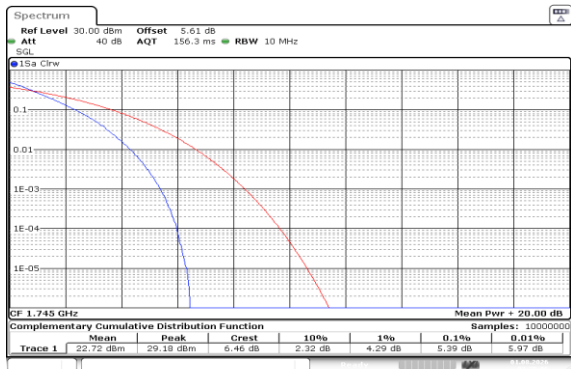
Band66-10MHz-QPSK-132322-50RB#0-PASS
