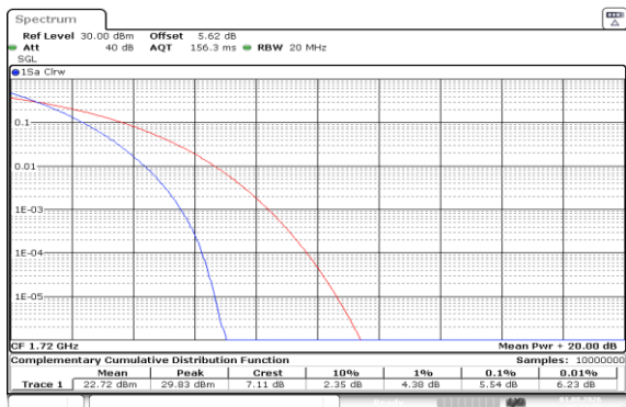
Band66-20MHz-QPSK-132072-100RB#0-PASS
