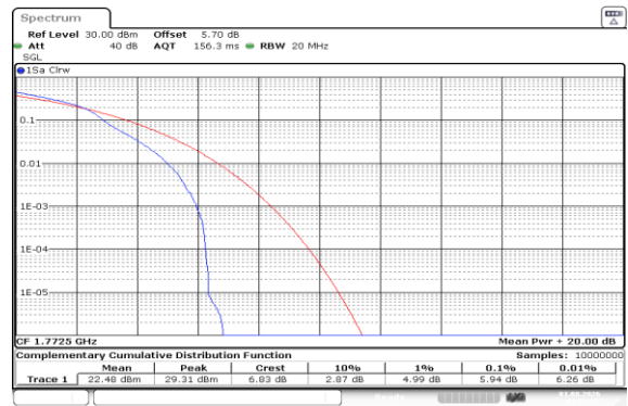
Band66-15MHz-16QAM-132597-1RB#0-PASS
