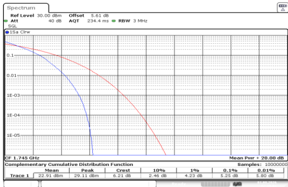
Band66-3MHz-QPSK-132322-15RB#0-PASS
