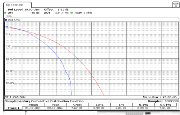
Band66-3MHz-16QAM-132322-15RB#0-PASS
