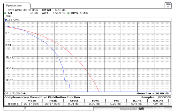
Band66-5MHz-16QAM-131997-1RB#0-PASS
