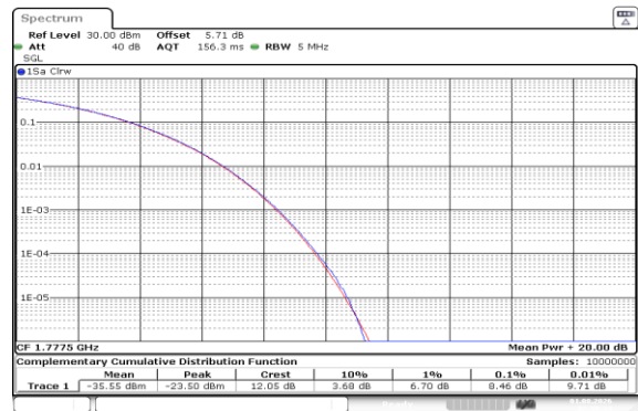
Band66-5MHz-16QAM-132647-1RB#0-PASS
