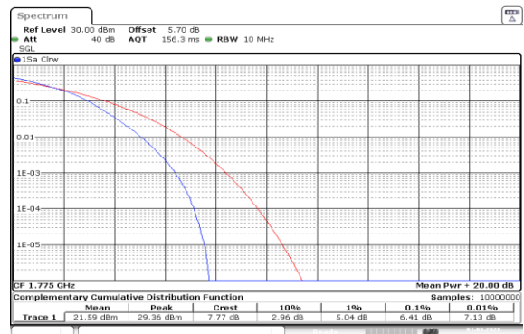
Band66-10MHz-16QAM-132622-50RB#0-PASS
