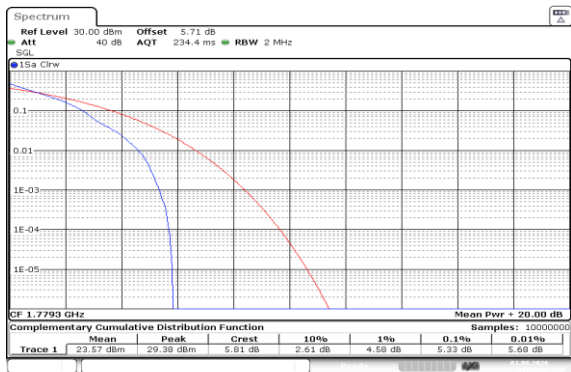
Band66-1.4MHz-QPSK-132665-1RB#0-PASS
