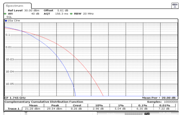
Band66-20MHz-16QAM-132322-100RB#0-PASS
