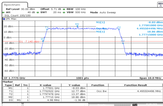
Band66-5MHz-QPSK-132647-25RB#0-PASS
