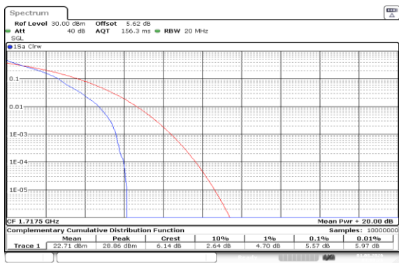
Band66-15MHz-QPSK-132047-1RB#0-PASS
