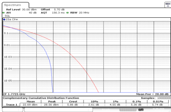
Band66-15MHz-QPSK-132597-1RB#0-PASS
