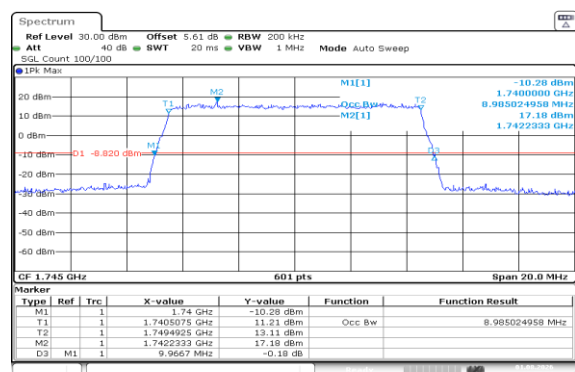
Band66-10MHz-16QAM-132322-50RB#0-PASS
