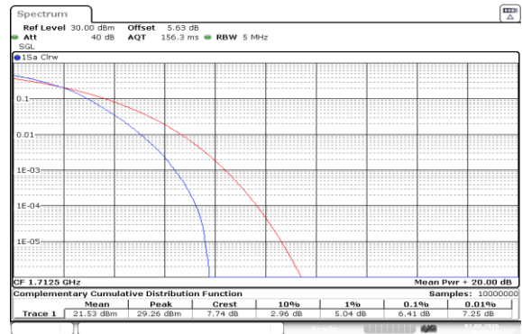
Band66-5MHz-16QAM-131997-25RB#0-PASS
