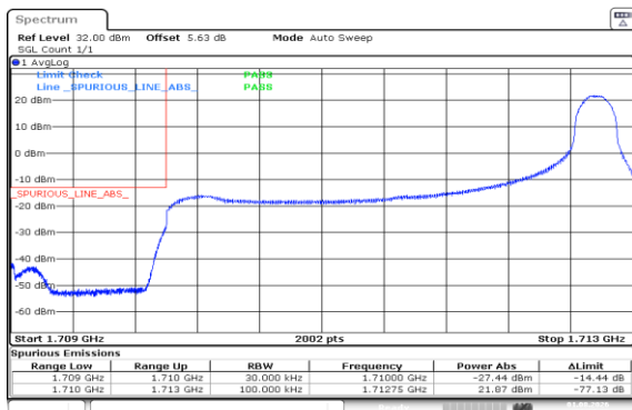
Band66-3MHz-QPSK-131987-1RB#14-PASS
