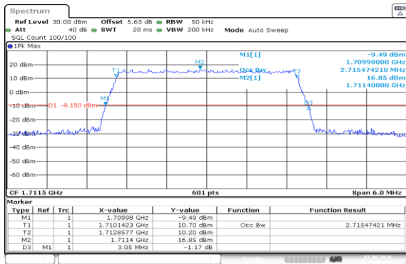
Band66-3MHz-QPSK-131987-15RB#0-PASS
