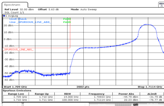
Band66-1.4MHz-QPSK-131979-1RB#5-PASS
