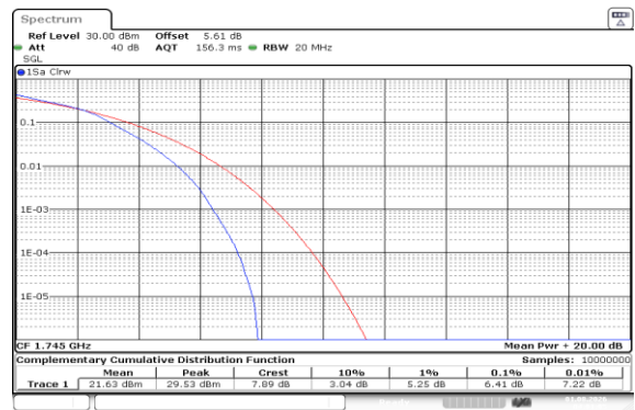
Band66-15MHz-16QAM-132322-75RB#0-PASS
