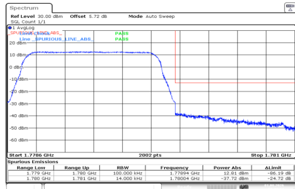
Band66-1.4MHz-16QAM-132665-6RB#0-PASS
