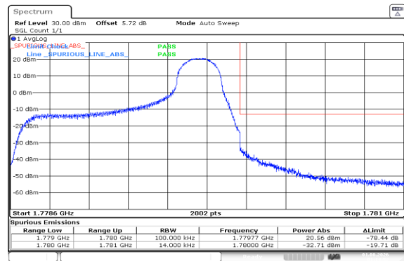
Band66-1.4MHz-16QAM-132665-1RB#5-PASS
