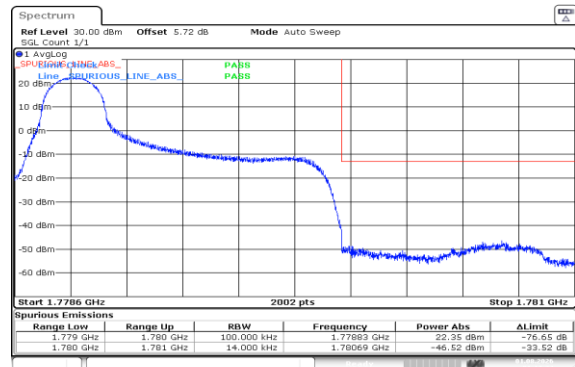
Band66-1.4MHz-16QAM-132665-1RB#0-PASS
