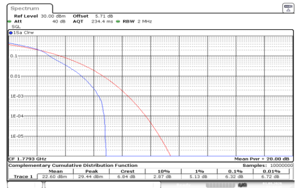
Band66-1.4MHz-16QAM-132665-1RB#0-PASS
