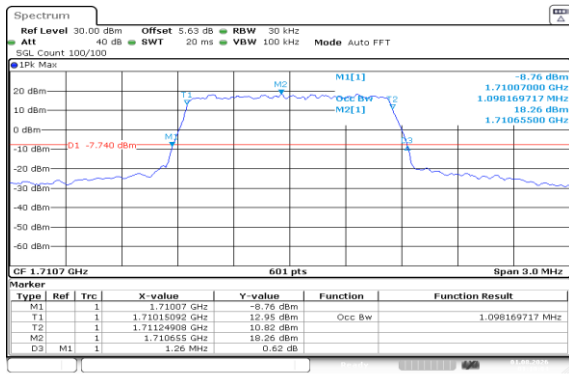
Band66-1.4MHz-QPSK-131979-6RB#0-PASS
