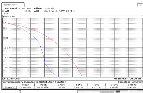
Band66-20MHz-QPSK-132322-1RB#0-PASS
