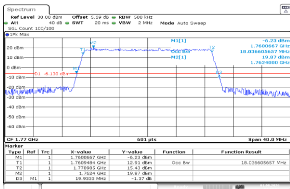
Band66-20MHz-QPSK-132572-100RB#0-PASS
