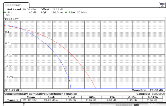
Band66-20MHz-16QAM-132072-100RB#0-PASS
