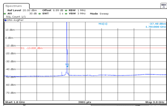
Band66-10MHz-16QAM-132622-1RB#0-1000~3000-PASS
