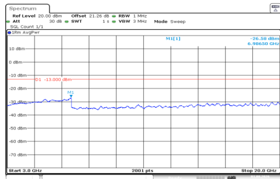
Band66-10MHz-QPSK-132022-1RB#49-3000~20000-PASS
