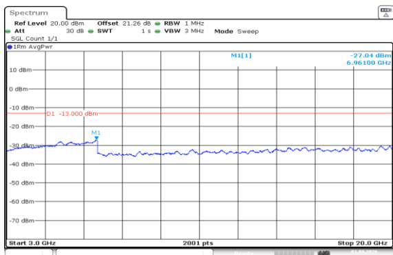
Band66-15MHz-16QAM-132322-1RB#74-3000~20000-PASS
