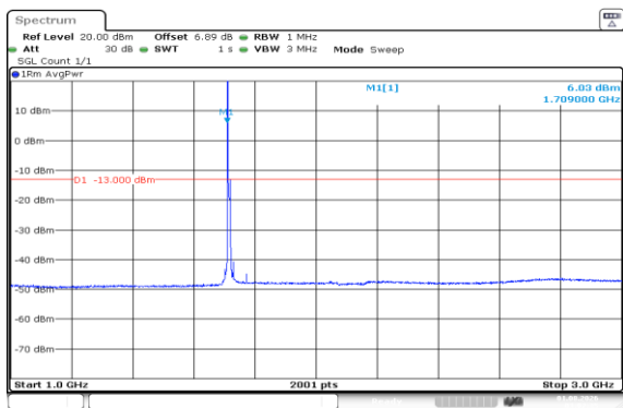
Band66-10MHz-16QAM-132022-1RB#0-1000~3000
