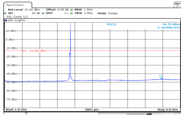
Band66-10MHz-16QAM-132322-1RB#49-1000~3000-PASS
