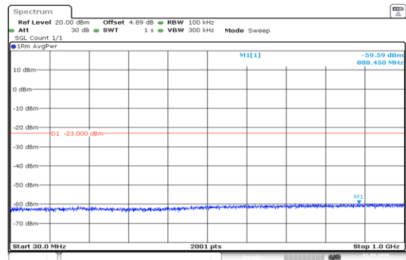
Band66-10MHz-16QAM-132622-1RB#49-30~1000-PASS
