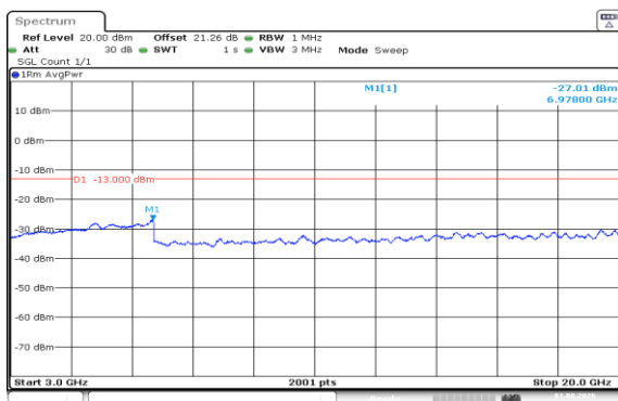
Band66-10MHz-QPSK-132022-1RB#0-3000~20000-PASS
