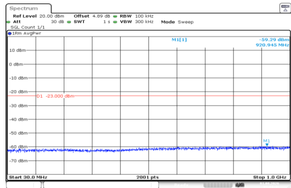
Band66-10MHz-QPSK-132022-1RB#0-30~1000-PASS
