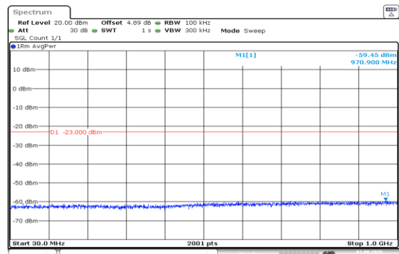
Band66-10MHz-QPSK-132322-50RB#0-30~1000-PASS
