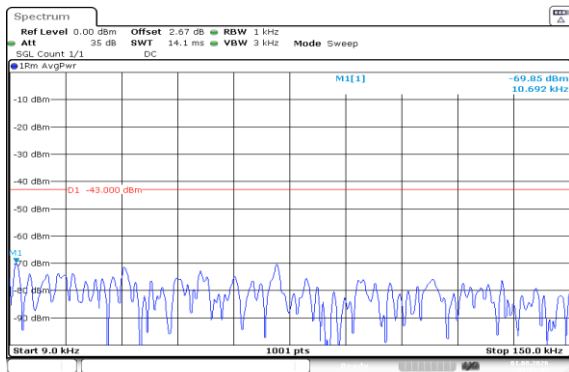
Band66-10MHz-16QAM-132322-1RB#49-0.009~0.15-PASS
