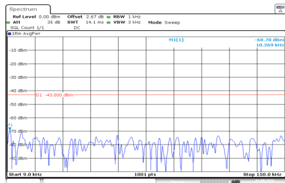
Band66-15MHz-QPSK-132047-1RB#74-0.009~0.15-PASS
