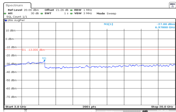
Band66-15MHz-QPSK-132322-75RB#0-3000~20000-PASS
