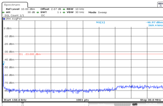
Band66-10MHz-QPSK-132022-1RB#0-0.15~30-PASS
