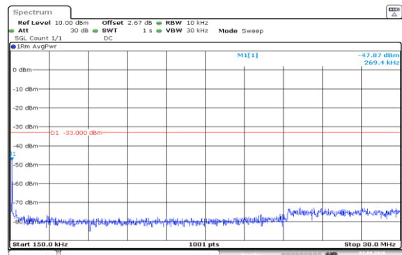
Band66-15MHz-16QAM-132322-1RB#74-0.15~30-PASS
