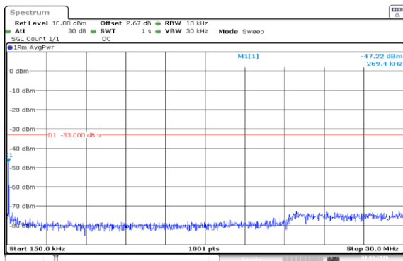
Band66-10MHz-QPSK-132022-50RB#0-0.15~30-PASS
