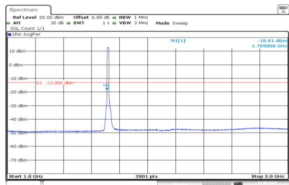
Band66-15MHz-16QAM-132047-75RB#0-1000~3000-PASS
