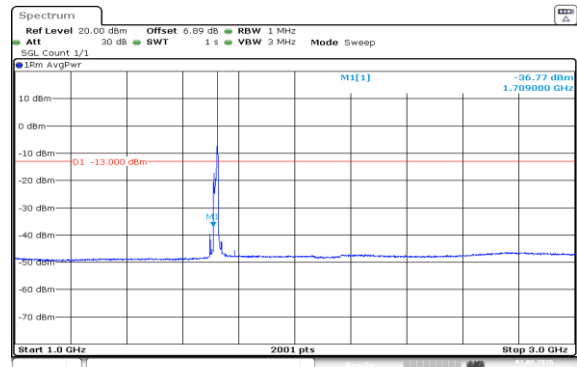
Band66-15MHz-16QAM-132047-1RB#74-1000~3000-PASS
