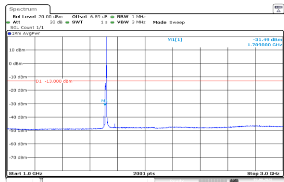
Band66-10MHz-16QAM-132022-1RB#49-1000~3000-PASS
