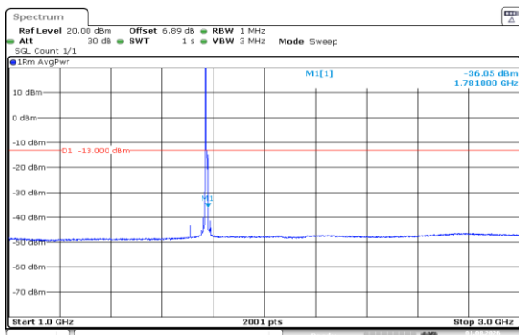
Band66-10MHz-QPSK-132622-1RB#0-1000~3000-PASS
