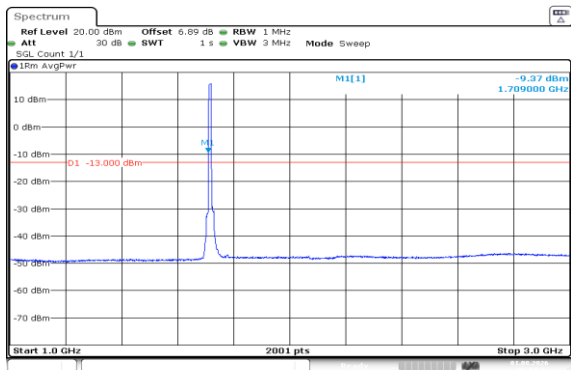
Band66-10MHz-QPSK-132022-50RB#0-1000~3000
