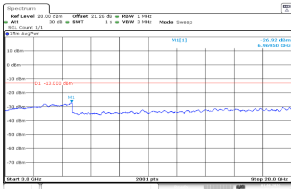
Band66-5MHz-QPSK-132647-25RB#0-3000~20000-PASS
