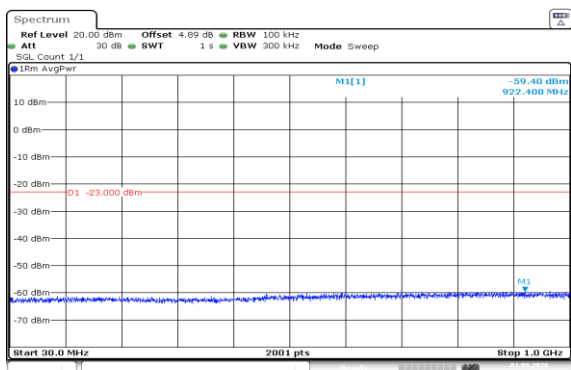
Band66-10MHz-16QAM-132322-50RB#0-30~1000-PASS
