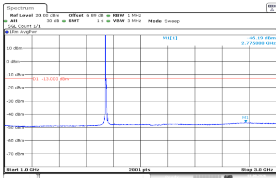
Band66-10MHz-QPSK-132322-1RB#0-1000~3000-PASS
