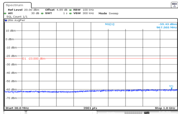
Band66-15MHz-QPSK-132047-1RB#0-30~1000-PASS
