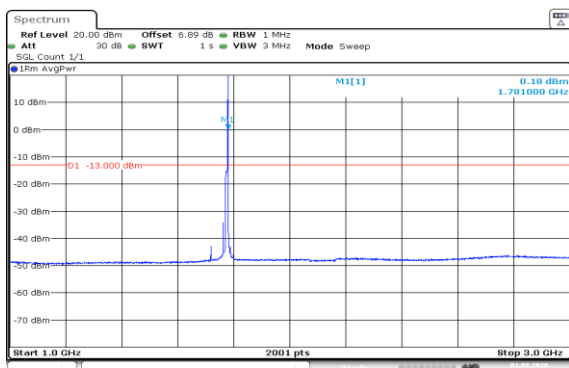
Band66-10MHz-QPSK-132622-1RB#49-1000~3000
