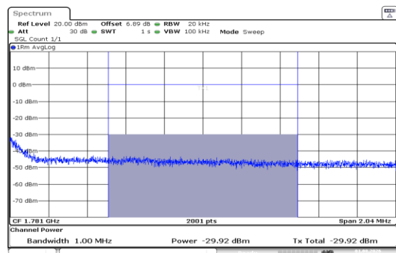
Band66-5MHz-16QAM-132647-25RB#0-1000~3000-PASS
