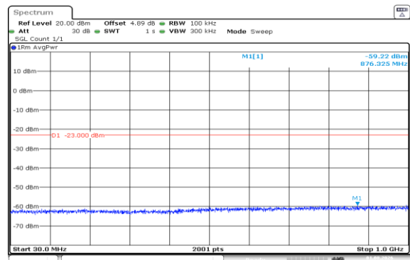
Band66-10MHz-QPSK-132622-50RB#0-30~1000-PASS
