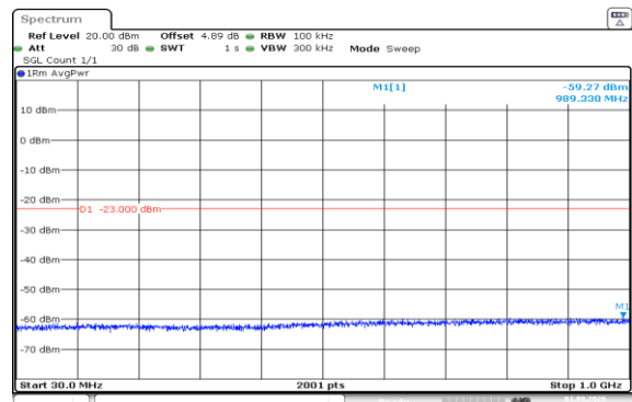
Band66-15MHz-QPSK-132597-1RB#0-30~1000-PASS
