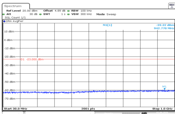
Band66-15MHz-16QAM-132047-75RB#0-30~1000-PASS
