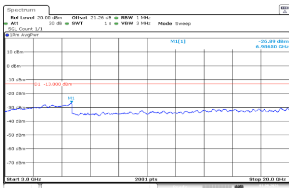
Band66-10MHz-16QAM-132622-1RB#49-3000~20000-PASS
