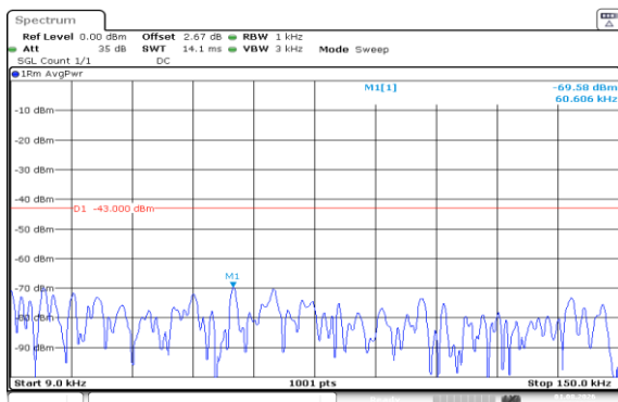
Band66-10MHz-16QAM-132622-50RB#0-0.009~0.15-PASS
