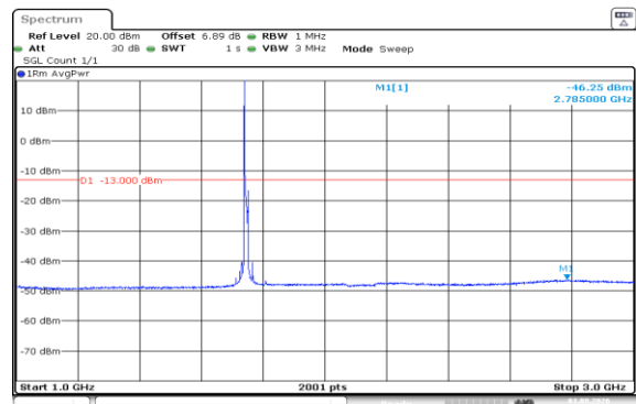
Band66-15MHz-16QAM-132322-1RB#0-1000~3000-PASS
