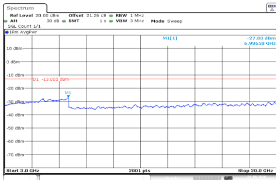
Band66-10MHz-16QAM-132022-50RB#0-3000~20000-PASS
