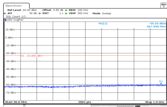
Band66-15MHz-QPSK-132322-75RB#0-30~1000-PASS
