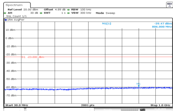
Band66-10MHz-QPSK-132622-1RB#0-30~1000-PASS
