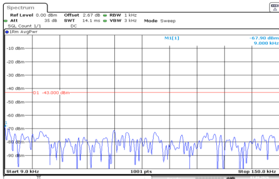
Band66-10MHz-16QAM-132322-1RB#0-0.009~0.15-PASS
