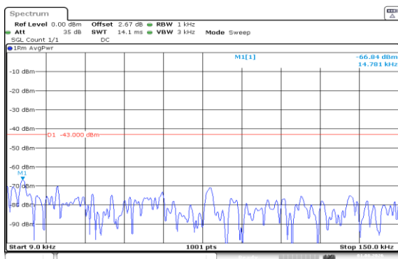
Band66-15MHz-16QAM-132322-1RB#0-0.009~0.15-PASS
