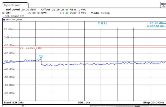
Band66-10MHz-QPSK-132622-1RB#49-3000~20000-PASS
