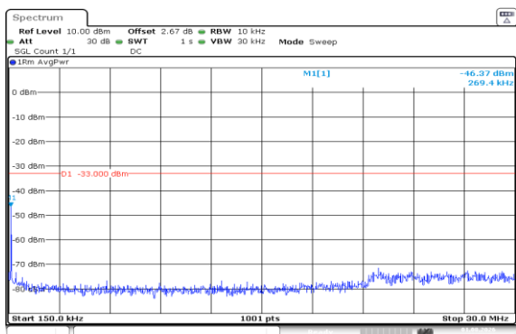
Band66-10MHz-QPSK-132022-1RB#49-0.15~30-PASS
