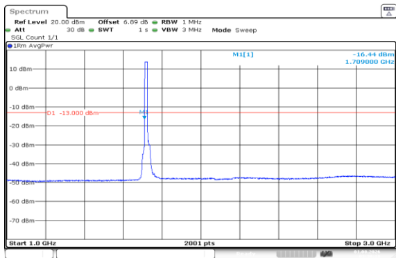
Band66-15MHz-QPSK-132047-75RB#0-1000~3000-PASS
