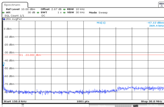
Band66-15MHz-QPSK-132047-1RB#0-0.15~30-PASS
