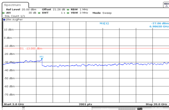
Band66-10MHz-16QAM-132622-1RB#0-3000~20000-PASS
