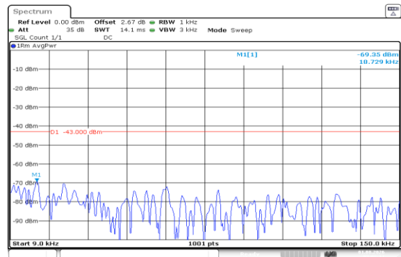
Band66-10MHz-QPSK-132322-1RB#0-0.009~0.15-PASS
