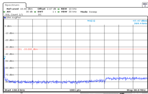
Band66-10MHz-16QAM-132622-1RB#0-0.15~30-PASS
