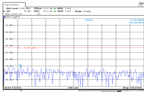
Band66-10MHz-QPSK-132022-1RB#49-0.009~0.15-PASS
