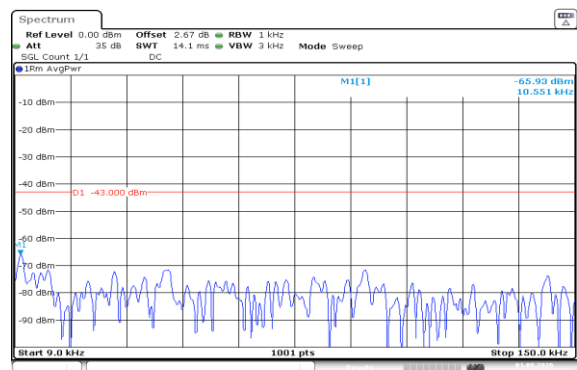
Band66-15MHz-16QAM-132047-1RB#0-0.009~0.15-PASS
