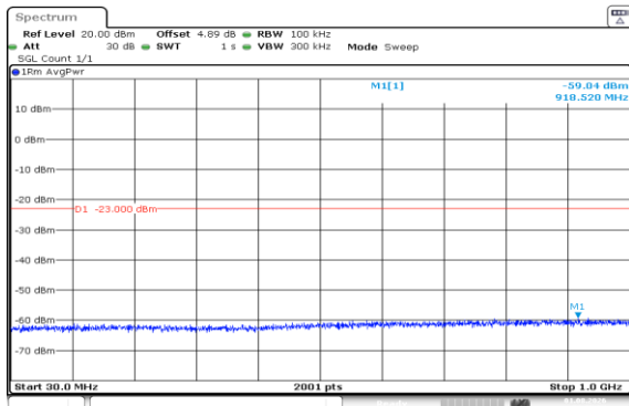
Band66-10MHz-16QAM-132322-1RB#49-30~1000-PASS
