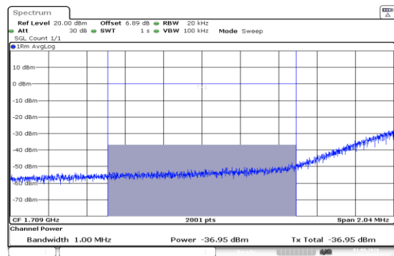
Band66-15MHz-16QAM-132047-1RB#0-1000~3000-PASS
