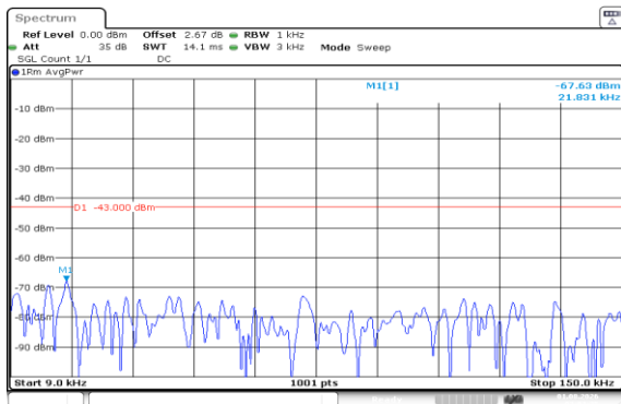
Band66-10MHz-16QAM-132022-1RB#49-0.009~0.15-PASS
