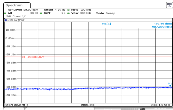
Band66-15MHz-16QAM-132047-1RB#0-30~1000-PASS
