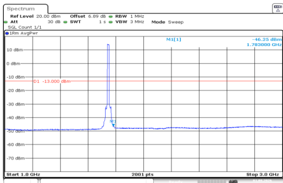
Band66-15MHz-QPSK-132322-75RB#0-1000~3000-PASS
