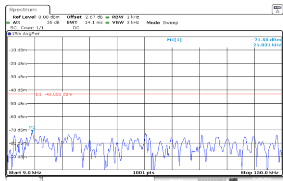
Band66-10MHz-QPSK-132022-50RB#0-0.009~0.15-PASS
