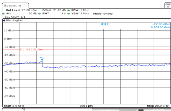
Band66-10MHz-16QAM-132022-1RB#0-3000~20000-PASS
