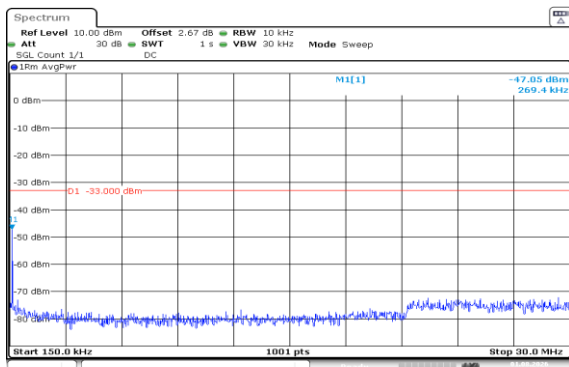
Band66-10MHz-QPSK-132622-50RB#0-0.15~30-PASS
