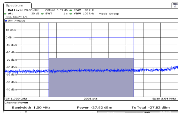
Band66-10MHz-16QAM-132022-50RB#0-1000~3000-PASS
