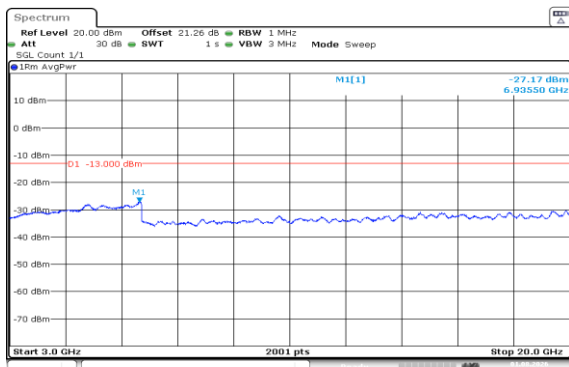
Band66-5MHz-16QAM-132647-25RB#0-3000~20000-PASS
