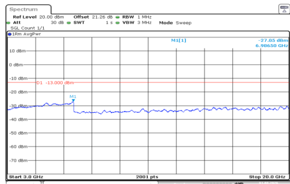
Band66-10MHz-QPSK-132622-1RB#0-3000~20000-PASS
