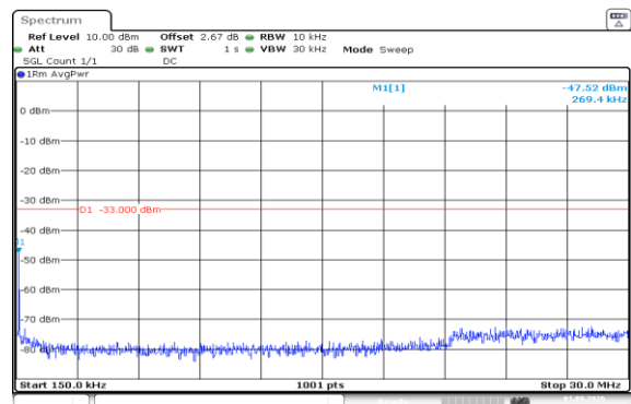
Band66-10MHz-16QAM-132622-50RB#0-0.15~30-PASS
