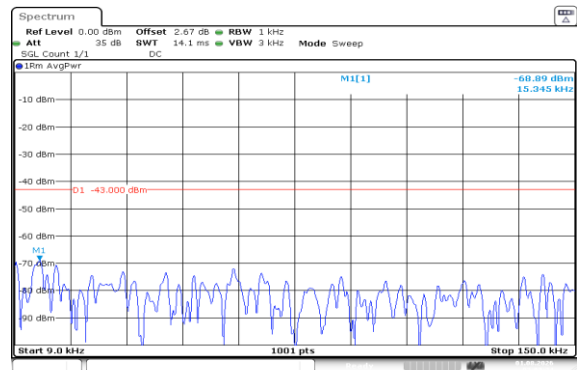
Band66-10MHz-QPSK-132622-1RB#49-0.009~0.15-PASS
