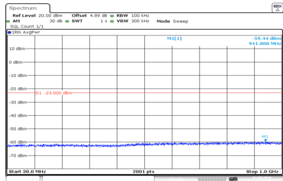
Band66-15MHz-QPSK-132322-1RB#0-30~1000-PASS
