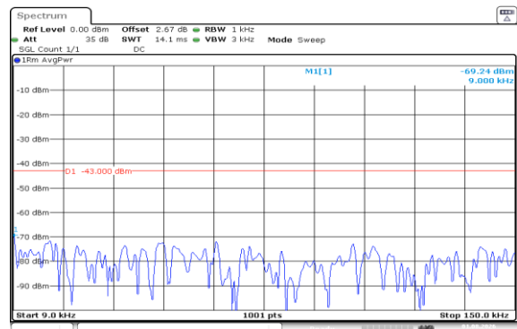
Band66-10MHz-16QAM-132622-1RB#49-0.009~0.15-PASS
