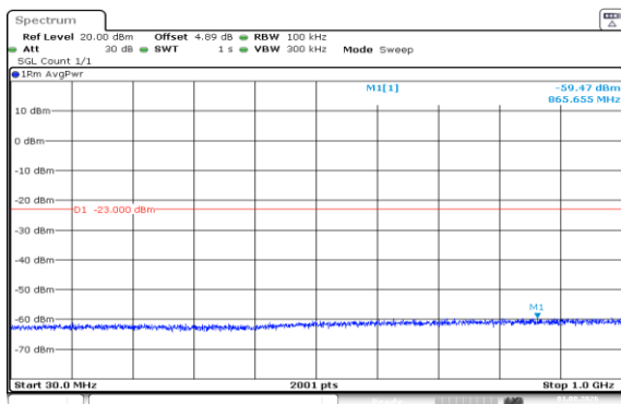
Band66-10MHz-16QAM-132022-1RB#49-30~1000-PASS
