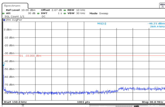
Band66-15MHz-QPSK-132047-1RB#74-0.15~30-PASS
