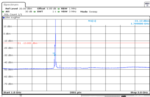
Band66-10MHz-QPSK-132022-1RB#49-1000~3000-PASS
