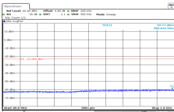
Band66-10MHz-16QAM-132622-1RB#0-30~1000-PASS
