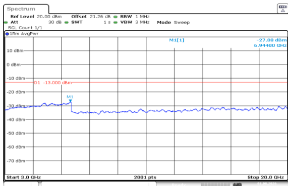
Band66-10MHz-16QAM-132322-50RB#0-3000~20000-PASS
