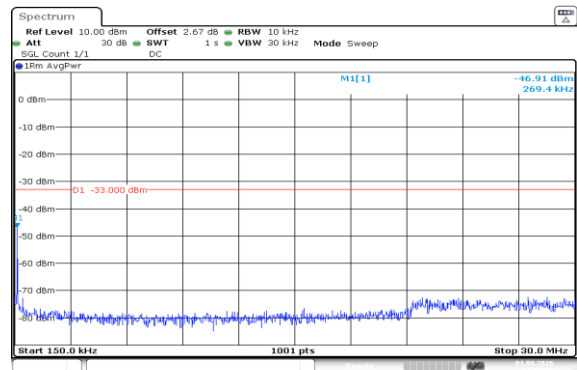
Band66-10MHz-16QAM-132022-1RB#49-0.15~30-PASS
