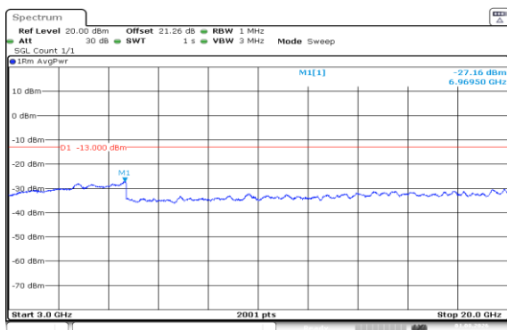
Band66-10MHz-16QAM-132022-1RB#49-3000~20000-PASS
