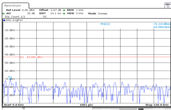
Band66-15MHz-16QAM-132047-75RB#0-0.009~0.15-PASS
