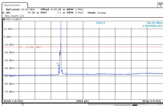
Band66-15MHz-QPSK-132047-1RB#74-1000~3000-PASS
