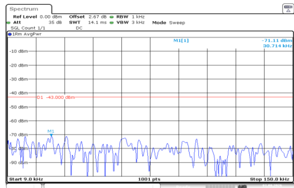
Band66-10MHz-QPSK-132622-1RB#0-0.009~0.15-PASS
