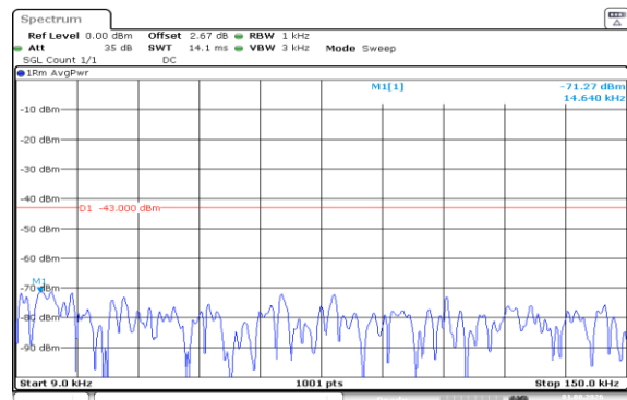
Band66-10MHz-QPSK-132022-1RB#0-0.009~0.15-PASS
