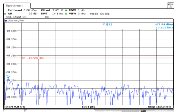
Band66-15MHz-QPSK-132322-75RB#0-0.009~0.15-PASS
