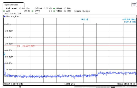
Band66-15MHz-16QAM-132322-1RB#0-0.15~30-PASS
