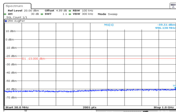
Band66-10MHz-16QAM-132022-50RB#0-30~1000-PASS
