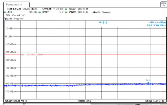
Band66-10MHz-QPSK-132322-1RB#0-30~1000-PASS
