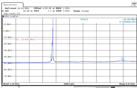
Band66-15MHz-QPSK-132322-1RB#74-1000~3000-PASS
