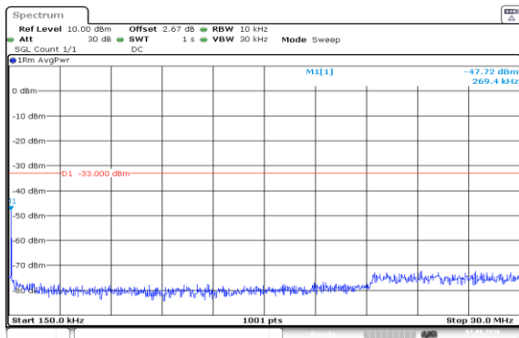
Band66-15MHz-QPSK-132322-1RB#0-0.15~30-PASS
