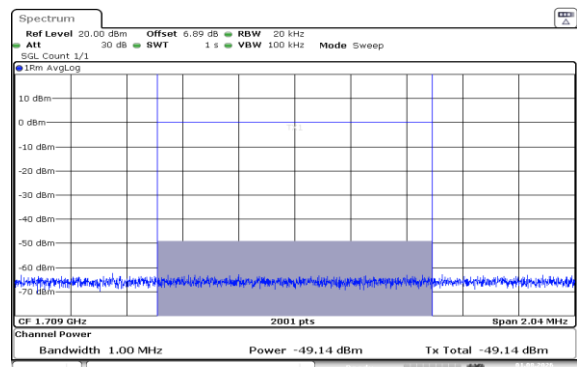
Band66-10MHz-QPSK-132022-1RB#0-30~1000-PASS
