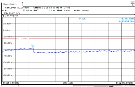
Band66-15MHz-16QAM-132047-75RB#0-3000~20000-PASS
