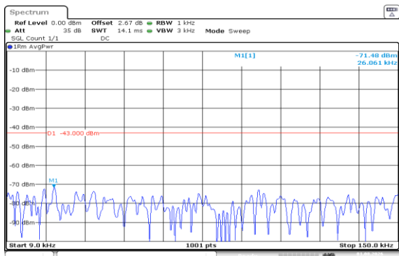
Band66-15MHz-16QAM-132322-1RB#74-0.009~0.15-PASS
