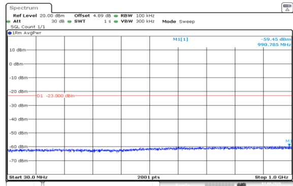
Band66-15MHz-QPSK-132047-75RB#0-30~1000-PASS
