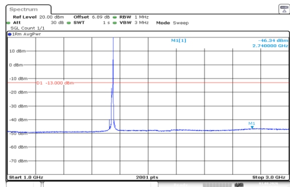
Band66-15MHz-16QAM-132322-1RB#74-1000~3000-PASS
