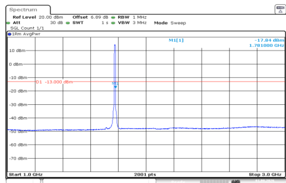
Band66-10MHz-16QAM-132622-50RB#0-1000~3000-PASS
