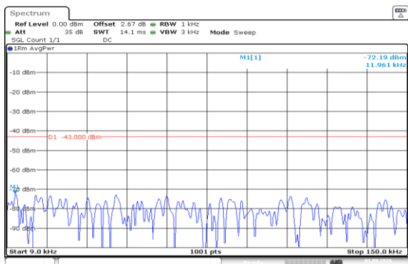
Band66-10MHz-16QAM-132322-50RB#0-0.009~0.15-PASS
