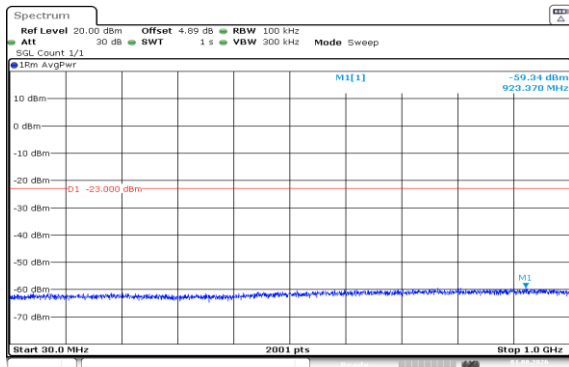
Band66-15MHz-16QAM-132047-1RB#74-30~1000-PASS
