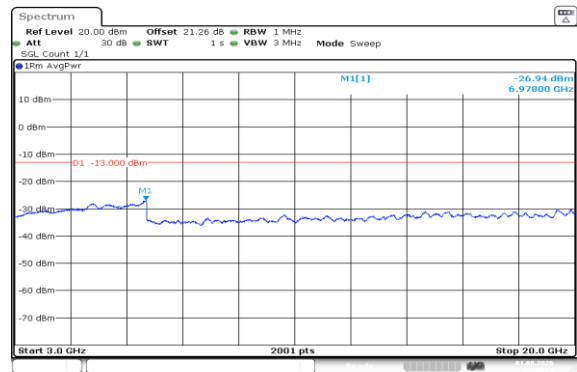
Band66-15MHz-QPSK-132047-75RB#0-3000~20000-PASS
