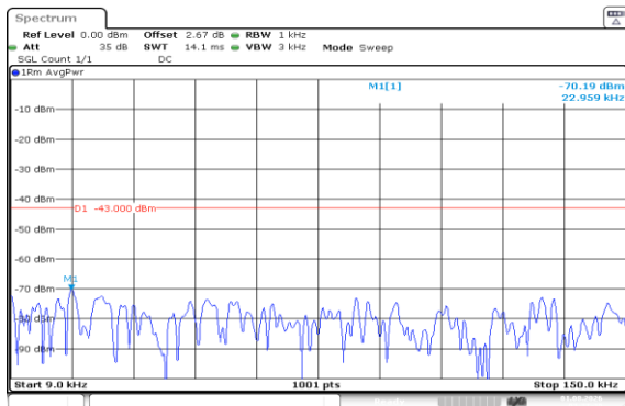
Band66-15MHz-16QAM-132047-1RB#74-0.009~0.15-PASS
