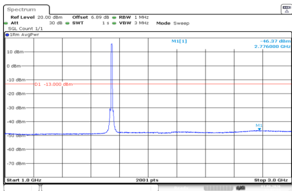
Band66-10MHz-QPSK-132322-50RB#0-1000~3000-PASS
