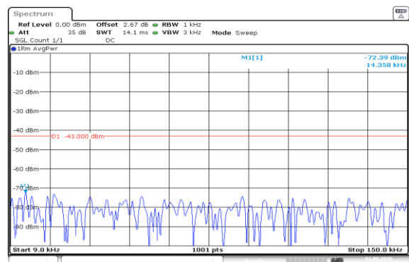
Band66-10MHz-QPSK-132622-50RB#0-0.009~0.15-PASS
