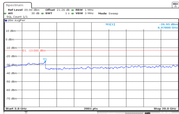
Band66-10MHz-QPSK-132322-1RB#0-3000~20000-PASS
