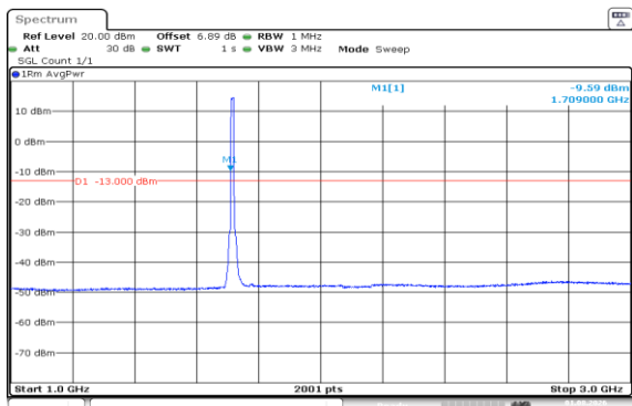
Band66-10MHz-16QAM-132022-50RB#0-1000~3000
