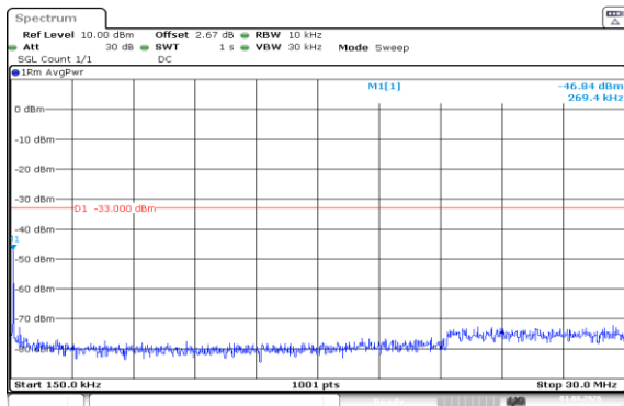
Band66-10MHz-QPSK-132622-1RB#0-0.15~30-PASS
