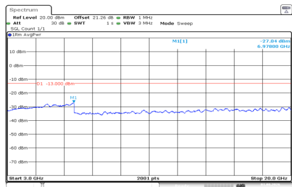
Band66-15MHz-QPSK-132322-1RB#74-3000~20000-PASS
