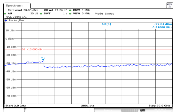
Band66-10MHz-QPSK-132322-50RB#0-3000~20000-PASS
