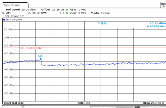
Band66-10MHz-16QAM-132622-50RB#0-3000~20000-PASS
