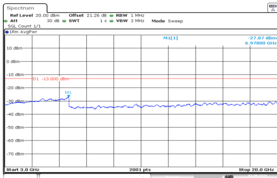
Band66-10MHz-16QAM-132322-1RB#49-3000~20000-PASS
