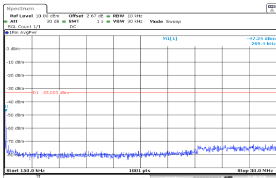
Band66-10MHz-16QAM-132022-1RB#0-0.15~30-PASS
