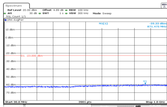
Band66-15MHz-QPSK-132047-1RB#74-30~1000-PASS
