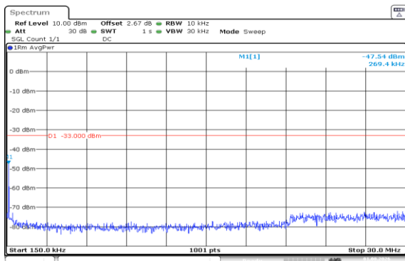
Band66-15MHz-QPSK-132597-1RB#0-0.15~30-PASS
