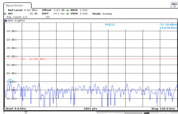
Band66-15MHz-QPSK-132322-1RB#0-0.009~0.15-PASS
