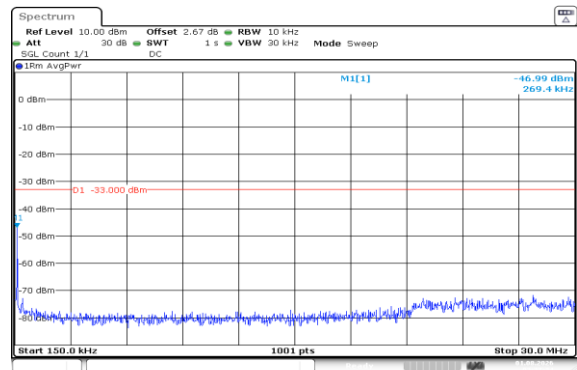
Band66-15MHz-16QAM-132047-1RB#74-0.15~30-PASS
