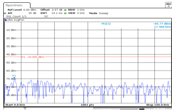
Band66-15MHz-QPSK-132047-1RB#0-0.009~0.15-PASS
