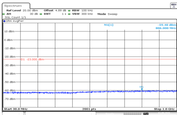
Band66-15MHz-16QAM-132322-1RB#74-30~1000-PASS
