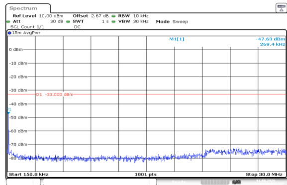
Band66-10MHz-16QAM-132322-1RB#49-0.15~30-PASS
