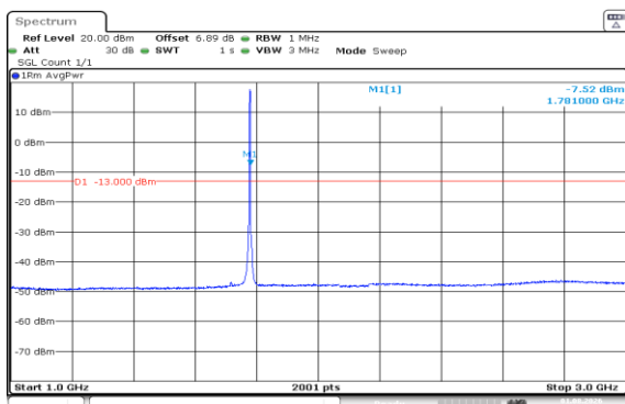
Band66-5MHz-16QAM-132647-25RB#0-1000~3000
