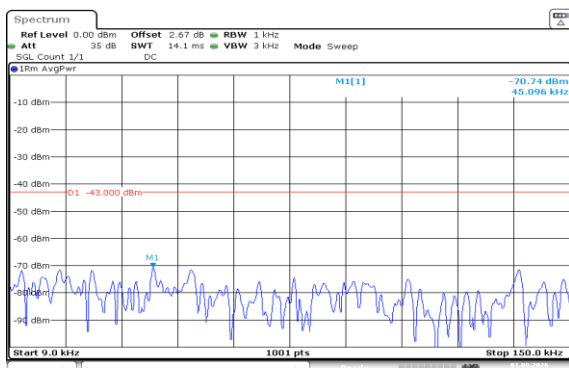
Band66-10MHz-16QAM-132622-1RB#0-0.009~0.15-PASS
