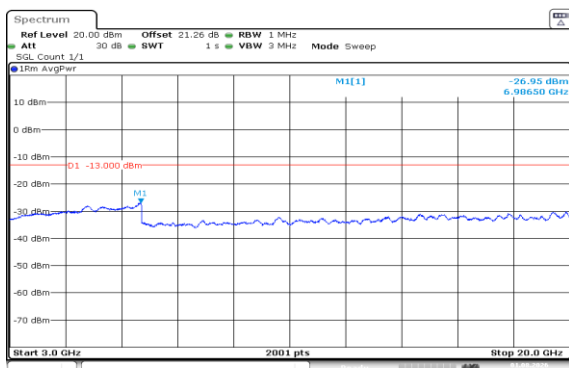
Band66-15MHz-16QAM-132322-75RB#0-3000~20000-PASS
