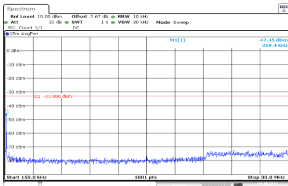
Band66-15MHz-16QAM-132047-1RB#0-0.15~30-PASS
