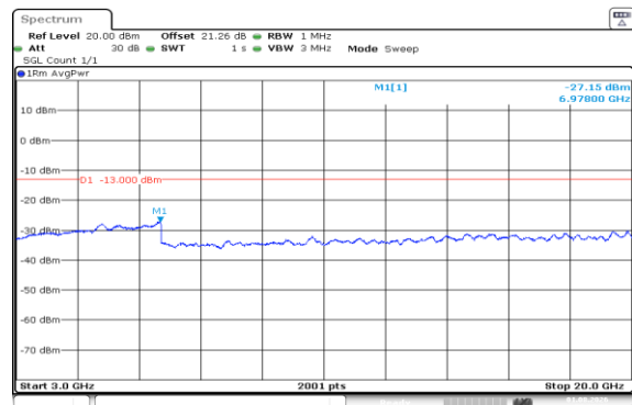
Band66-15MHz-QPSK-132047-1RB#74-3000~20000-PASS
