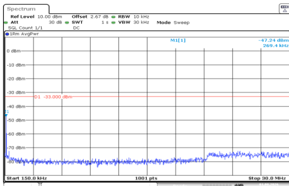
Band66-10MHz-QPSK-132322-50RB#0-0.15~30-PASS
