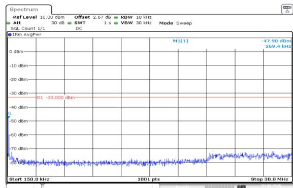
Band66-10MHz-16QAM-132322-50RB#0-0.15~30-PASS
