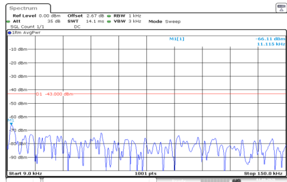
Band66-15MHz-QPSK-132047-75RB#0-0.009~0.15-PASS
