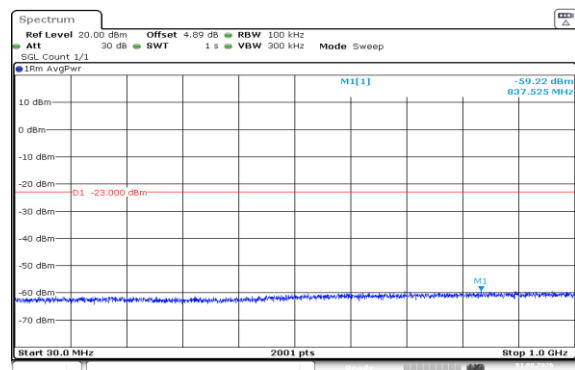
Band66-10MHz-QPSK-132022-1RB#49-30~1000-PASS
