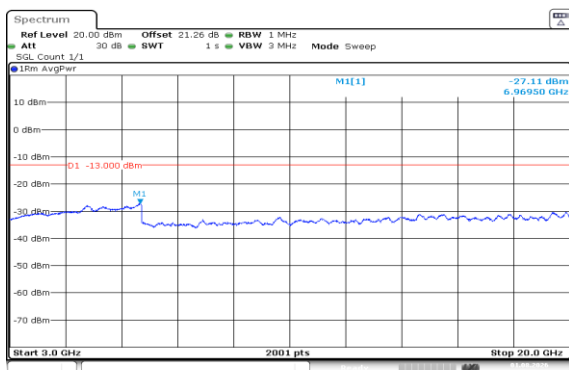
Band66-15MHz-QPSK-132047-1RB#0-3000~20000-PASS
