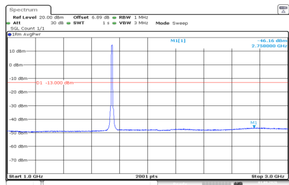
Band66-10MHz-16QAM-132322-50RB#0-1000~3000-PASS
