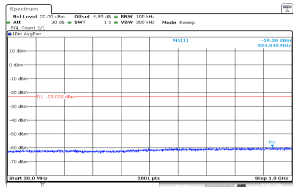
Band66-10MHz-QPSK-132022-50RB#0-30~1000-PASS
