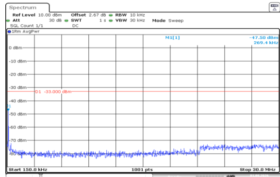
Band66-10MHz-16QAM-132322-1RB#0-0.15~30-PASS
