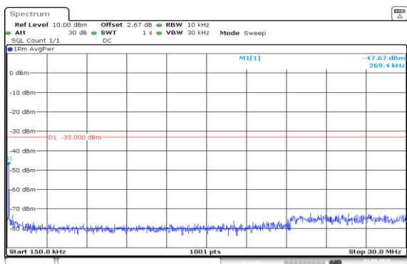
Band66-15MHz-QPSK-132322-75RB#0-0.15~30-PASS
