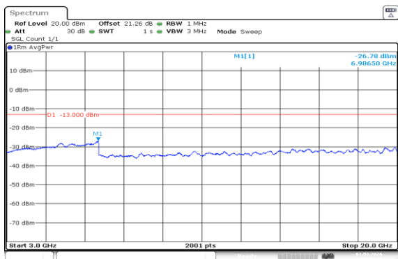
Band66-15MHz-16QAM-132322-1RB#0-3000~20000-PASS
