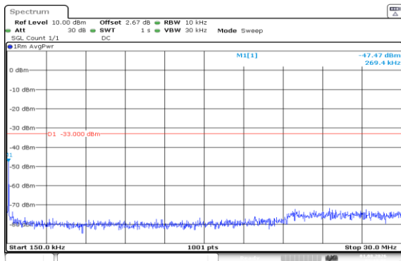
Band66-10MHz-16QAM-132622-1RB#49-0.15~30-PASS
