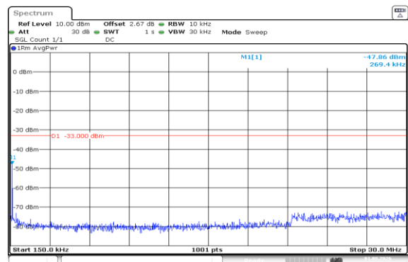
Band66-15MHz-16QAM-132047-75RB#0-0.15~30-PASS
