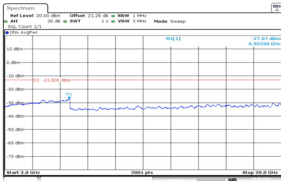
Band66-15MHz-16QAM-132047-1RB#74-3000~20000-PASS
