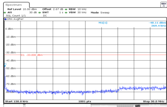
Band66-15MHz-16QAM-132322-75RB#0-0.15~30-PASS
