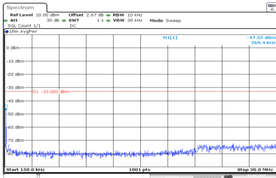
Band66-15MHz-QPSK-132047-75RB#0-0.15~30-PASS
