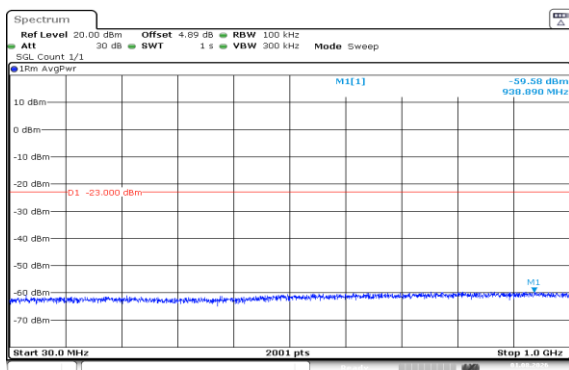
Band66-10MHz-16QAM-132622-50RB#0-30~1000-PASS
