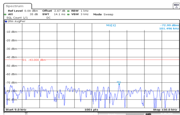
Band66-10MHz-16QAM-132022-1RB#0-0.009~0.15-PASS
