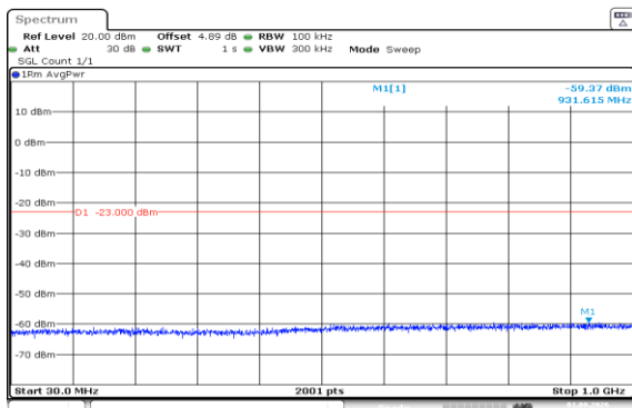
Band66-15MHz-16QAM-132322-1RB#0-30~1000-PASS
