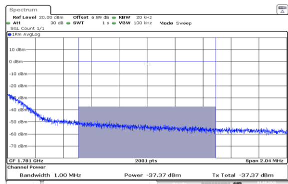
Band66-10MHz-QPSK-132622-1RB#49-1000~3000-PASS
