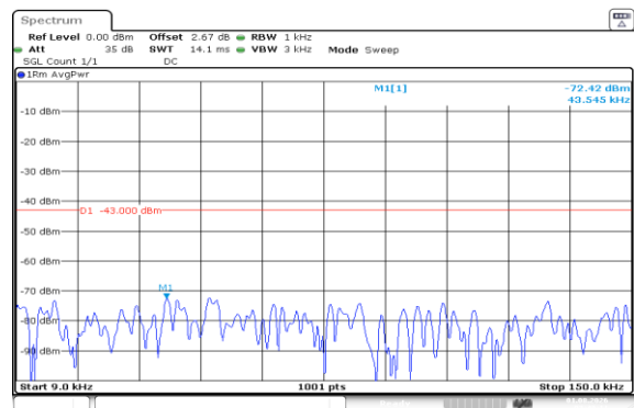
Band66-15MHz-QPSK-132322-1RB#74-0.009~0.15-PASS
