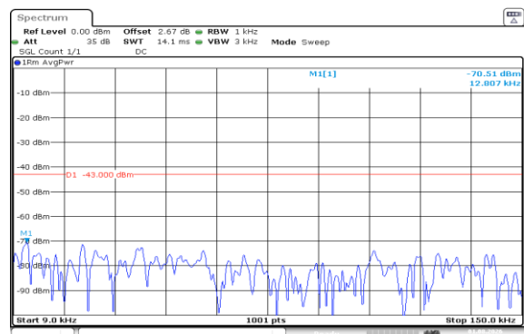
Band66-15MHz-QPSK-132597-1RB#0-0.009~0.15-PASS
