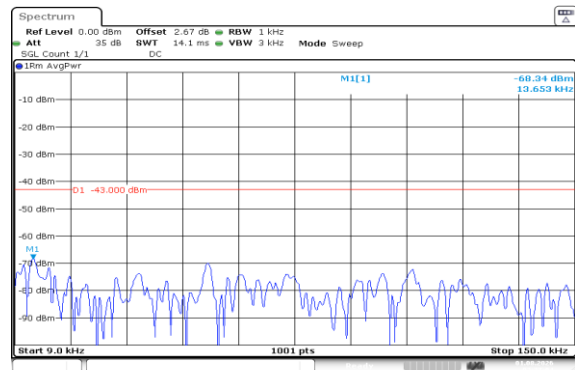
Band66-5MHz-16QAM-132647-25RB#0-0.009~0.15-PASS
