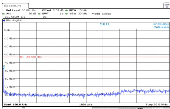
Band66-10MHz-16QAM-132022-50RB#0-0.15~30-PASS
