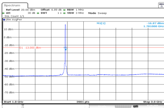
Band66-10MHz-QPSK-132622-50RB#0-1000~3000-PASS
