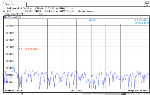
Band66-10MHz-QPSK-132322-50RB#0-0.009~0.15-PASS
