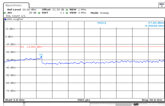
Band66-10MHz-QPSK-132622-50RB#0-3000~20000-PASS
