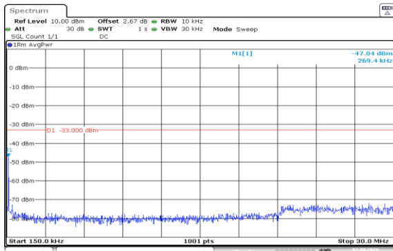
Band66-10MHz-QPSK-132322-1RB#0-0.15~30-PASS
