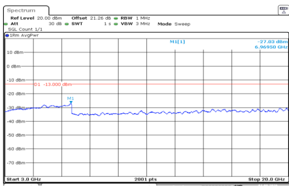
Band66-20MHz-16QAM-132572-1RB#99-3000~20000-PASS
