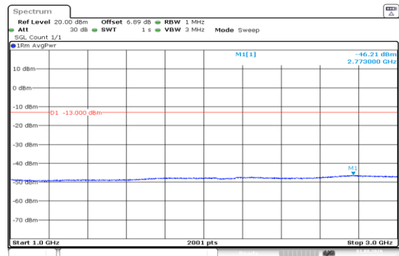
Band66-20MHz-16QAM-132322-100RB#0-1000~3000-PASS
