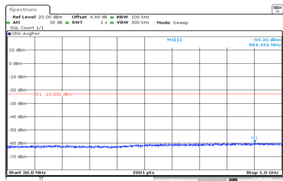
Band66-20MHz-QPSK-132072-100RB#0-30~1000-PASS
