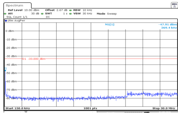
Band66-20MHz-16QAM-132072-1RB#99-0.15~30-PASS
