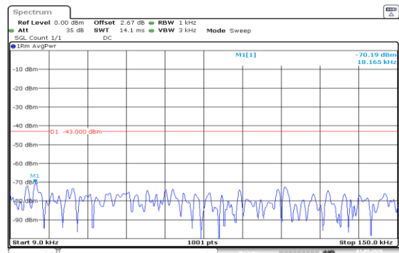
Band66-20MHz-QPSK-132322-1RB#99-0.009~0.15-PASS
