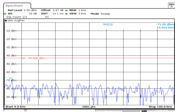
Band66-20MHz-16QAM-132072-1RB#0-0.009~0.15-PASS
