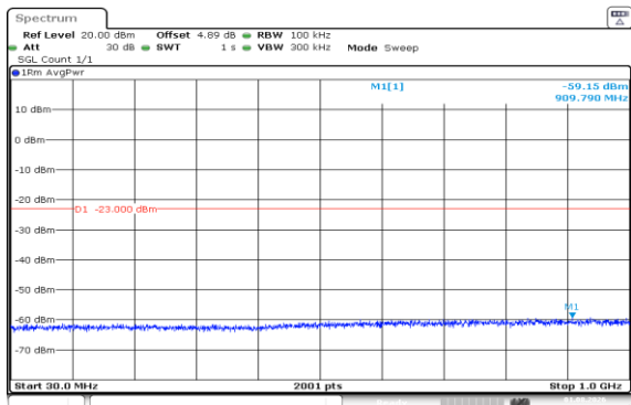
Band66-15MHz-16QAM-132597-1RB#0-30~1000-PASS
