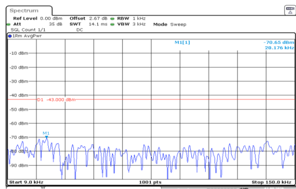
Band66-20MHz-QPSK-132572-100RB#0-0.009~0.15-PASS
