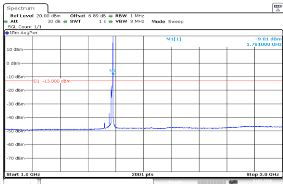
Band66-15MHz-16QAM-132597-1RB#74-1000~3000
