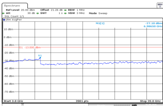
Band66-15MHz-16QAM-132597-75RB#0-3000~20000-PASS
