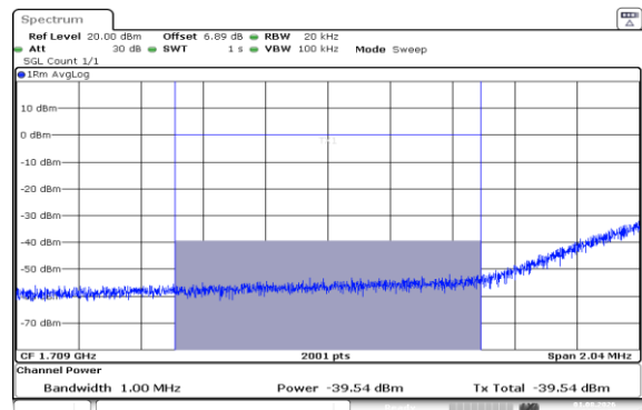
Band66-20MHz-16QAM-132072-1RB#0-1000~3000-PASS
