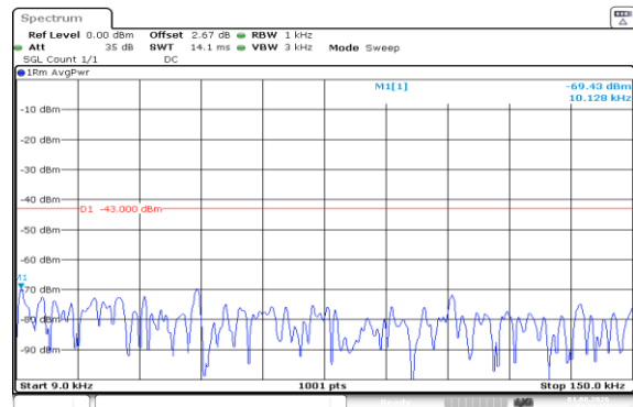
Band66-20MHz-QPSK-132322-100RB#0-0.009~0.15-PASS
