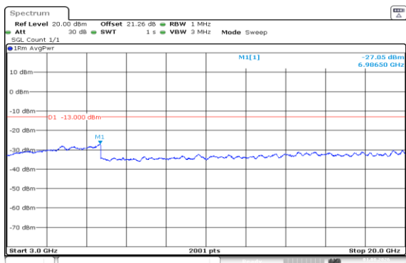
Band66-20MHz-QPSK-132072-1RB#0-3000~20000-PASS
