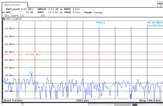
Band66-20MHz-16QAM-132572-1RB#0-0.009~0.15-PASS
