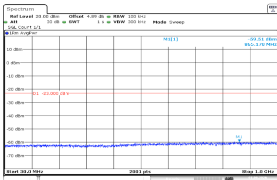
Band66-20MHz-16QAM-132072-100RB#0-30~1000-PASS
