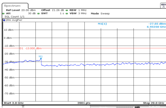
Band66-20MHz-16QAM-132072-100RB#0-3000~20000-PASS
