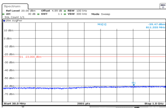
Band66-20MHz-16QAM-132572-1RB#99-30~1000-PASS
