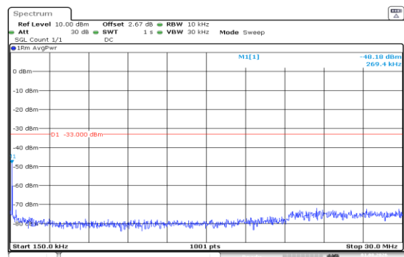
Band66-20MHz-16QAM-132572-100RB#0-0.15~30-PASS
