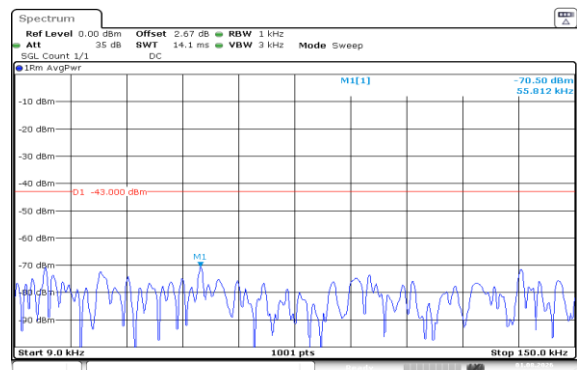
Band66-20MHz-QPSK-132072-100RB#0-0.009~0.15-PASS
