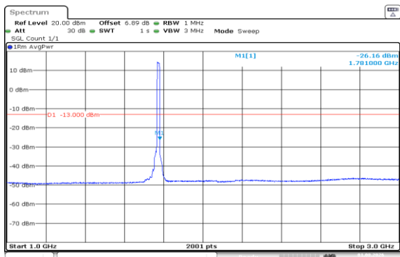
Band66-15MHz-QPSK-132597-75RB#0-1000~3000-PASS
