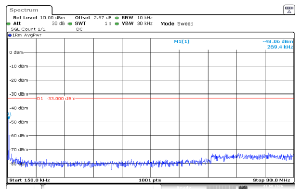
Band66-20MHz-16QAM-132322-1RB#99-0.15~30-PASS
