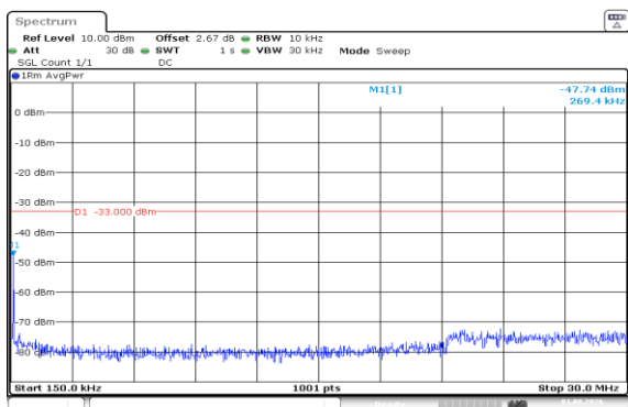
Band66-20MHz-16QAM-132072-1RB#0-0.15~30-PASS
