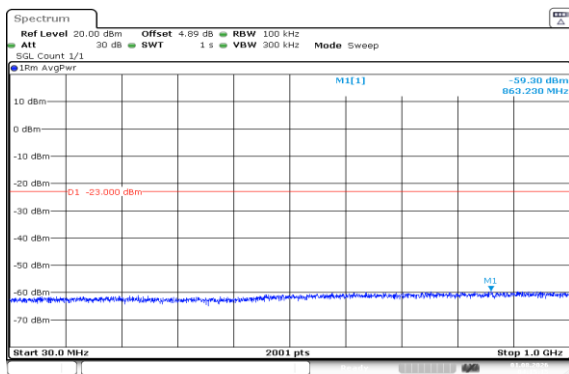
Band66-20MHz-16QAM-132072-1RB#99-30~1000-PASS
