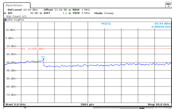
Band66-15MHz-QPSK-132597-75RB#0-3000~20000-PASS
