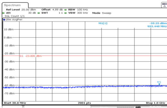
Band66-20MHz-16QAM-132322-1RB#99-30~1000-PASS
