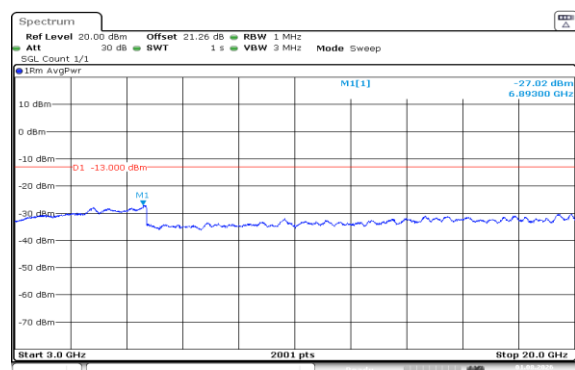
Band66-20MHz-QPSK-132322-100RB#0-3000~20000-PASS
