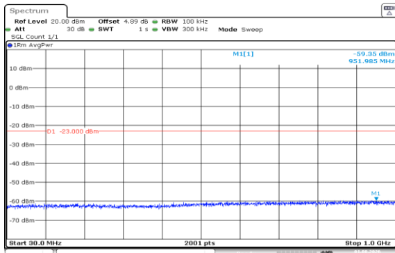
Band66-20MHz-16QAM-132572-1RB#0-30~1000-PASS
