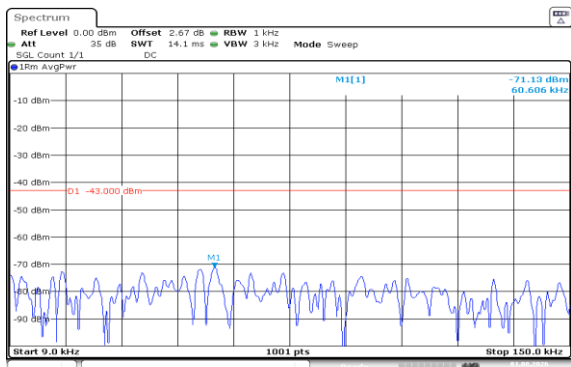
Band66-20MHz-16QAM-132072-1RB#99-0.009~0.15-PASS
