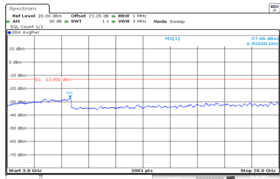
Band66-20MHz-QPSK-132072-100RB#0-3000~20000-PASS
