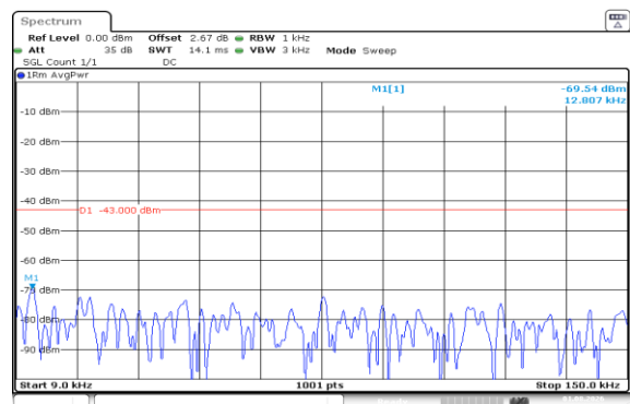
Band66-20MHz-QPSK-132072-1RB#0-0.009~0.15-PASS
