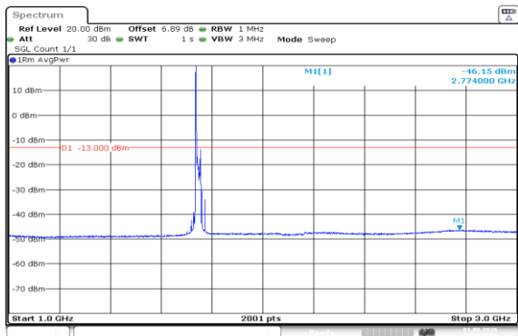
Band66-20MHz-QPSK-132322-1RB#0-1000~3000-PASS
