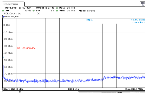
Band66-20MHz-QPSK-132572-1RB#99-0.15~30-PASS
