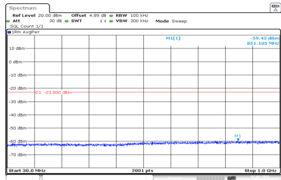
Band66-15MHz-QPSK-132597-1RB#74-30~1000-PASS
