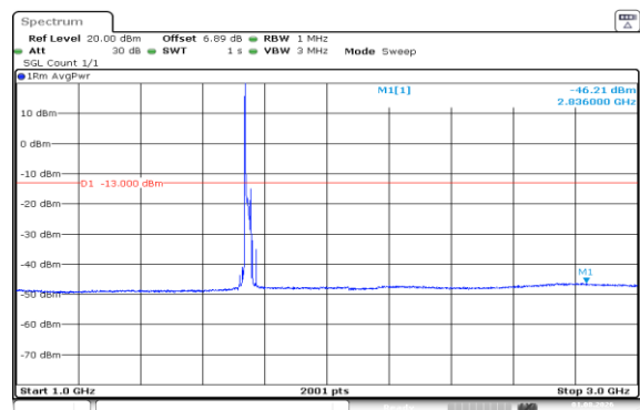
Band66-20MHz-16QAM-132322-1RB#0-1000~3000-PASS
