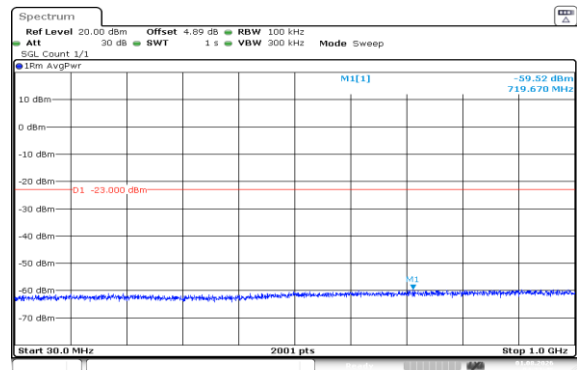
Band66-20MHz-QPSK-132572-100RB#0-30~1000-PASS
