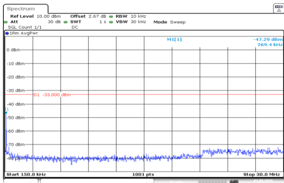
Band66-20MHz-QPSK-132072-1RB#0-0.15~30-PASS
