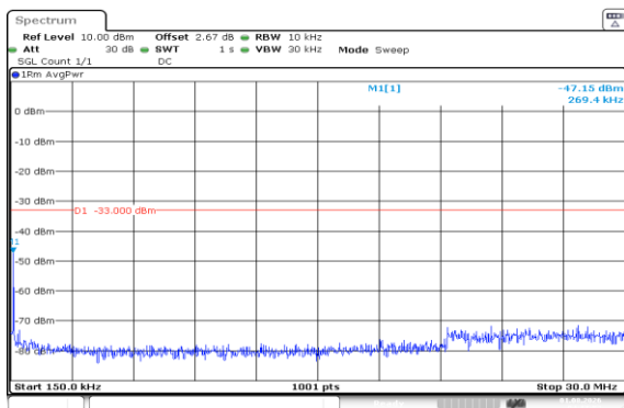
Band66-20MHz-QPSK-132322-1RB#99-0.15~30-PASS
