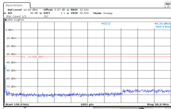
Band66-20MHz-16QAM-132322-100RB#0-0.15~30-PASS
