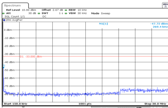
Band66-20MHz-16QAM-132322-1RB#99-3000~20000-PASS
