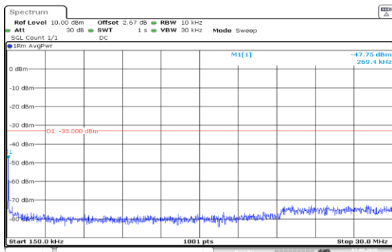
Band66-15MHz-16QAM-132597-1RB#74-0.15~30-PASS
