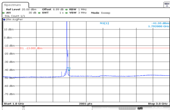
Band66-15MHz-QPSK-132597-1RB#0-1000~3000-PASS
