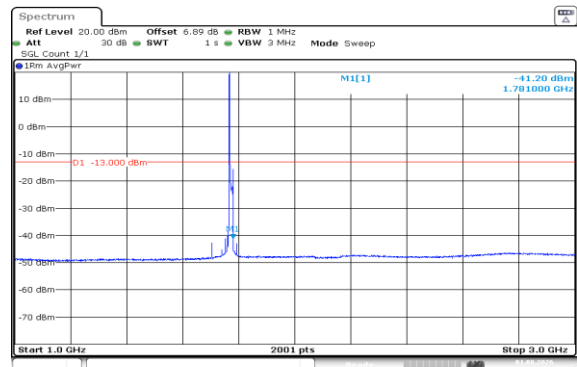
Band66-15MHz-16QAM-132597-1RB#0-1000~3000-PASS
