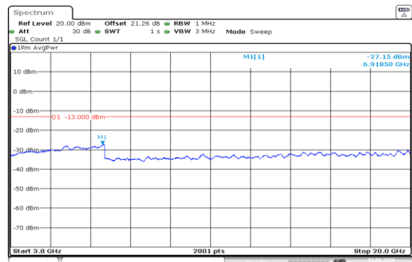
Band66-20MHz-QPSK-132572-1RB#0-3000~20000-PASS
