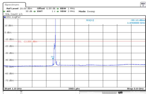
Band66-20MHz-16QAM-132072-1RB#99-1000~3000-PASS
