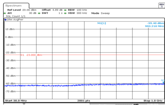
Band66-20MHz-QPSK-132572-1RB#0-30~1000-PASS
