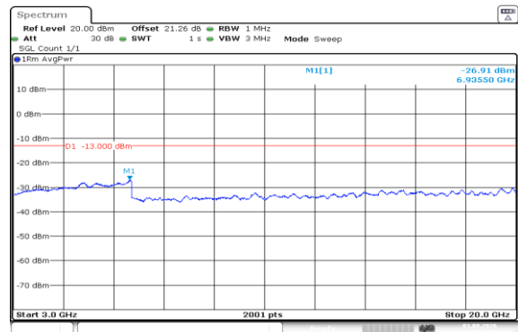
Band66-20MHz-QPSK-132572-1RB#99-3000~20000-PASS
