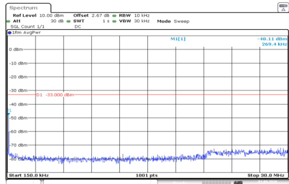
Band66-15MHz-16QAM-132597-1RB#0-0.15~30-PASS
