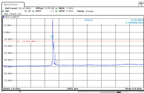
Band66-20MHz-16QAM-132072-1RB#0-1000~3000
