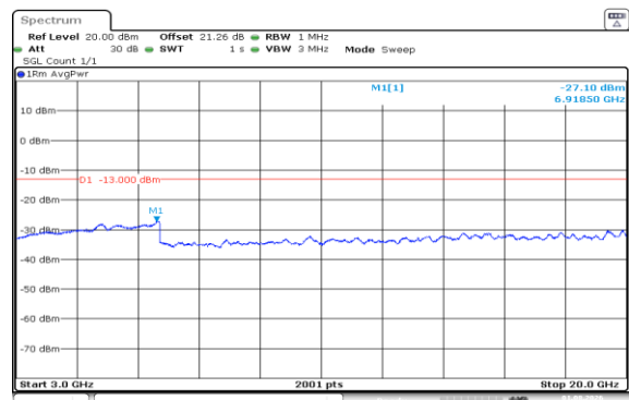
Band66-20MHz-QPSK-132322-1RB#99-3000~20000-PASS
