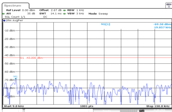
Band66-15MHz-16QAM-132597-75RB#0-0.009~0.15-PASS
