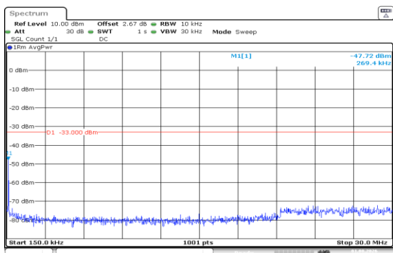
Band66-20MHz-QPSK-132572-1RB#0-0.15~30-PASS
