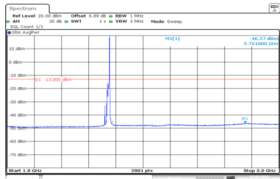
Band66-20MHz-16QAM-132322-1RB#99-1000~3000-PASS
