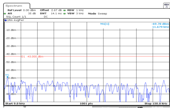
Band66-15MHz-16QAM-132597-1RB#74-0.009~0.15-PASS
