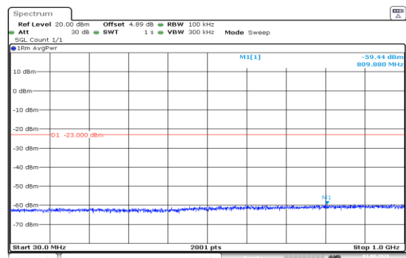
Band66-15MHz-QPSK-132597-75RB#0-30~1000-PASS
