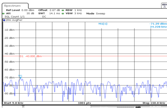
Band66-20MHz-16QAM-132322-1RB#99-0.009~0.15-PASS
