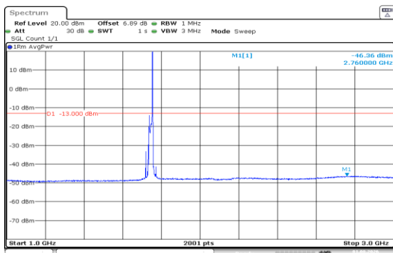
Band66-20MHz-QPSK-132322-1RB#99-1000~3000-PASS
