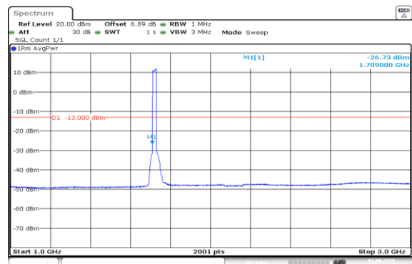
Band66-20MHz-16QAM-132072-100RB#0-1000~3000-PASS
