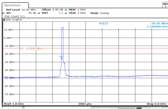
Band66-20MHz-QPSK-132072-100RB#0-1000~3000-PASS
