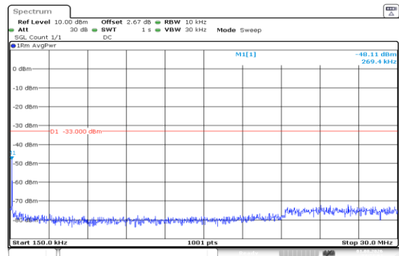
Band66-20MHz-16QAM-132572-1RB#0-0.15~30-PASS
