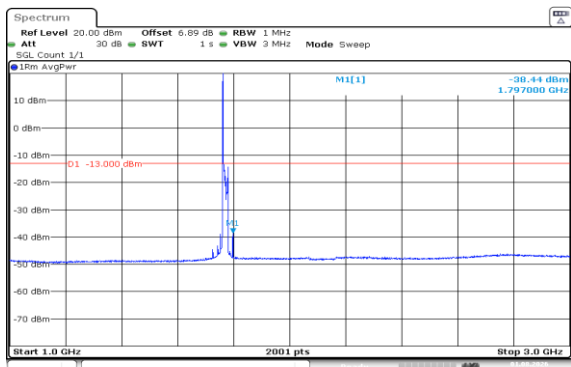
Band66-20MHz-QPSK-132572-1RB#0-1000~3000-PASS
