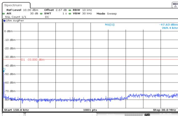
Band66-20MHz-QPSK-132572-100RB#0-0.15~30-PASS
