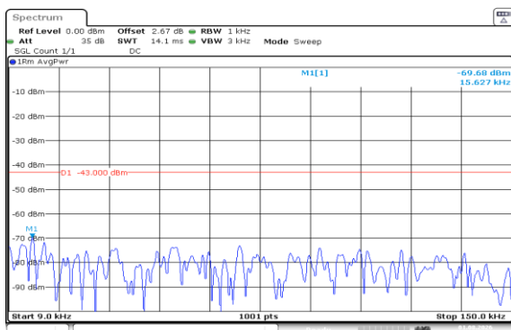
Band66-20MHz-16QAM-132572-100RB#0-0.009~0.15-PASS
