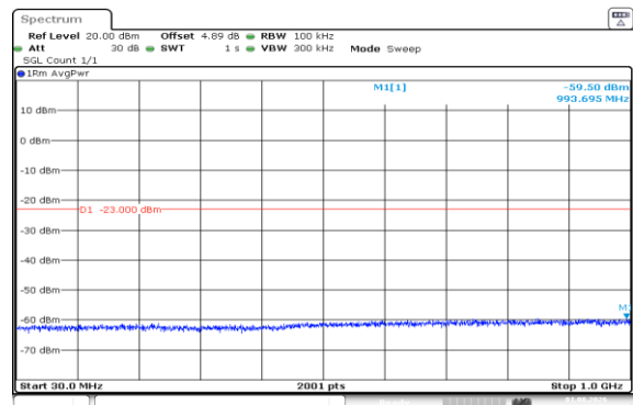
Band66-20MHz-QPSK-132072-1RB#0-30~1000-PASS
