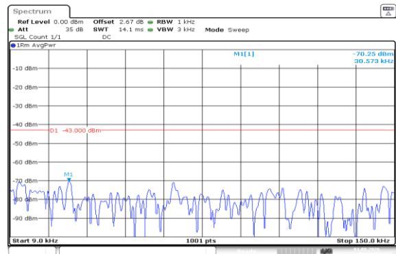
Band66-20MHz-QPSK-132072-1RB#99-0.009~0.15-PASS
