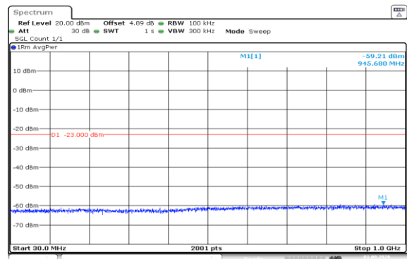
Band66-15MHz-16QAM-132597-1RB#74-30~1000-PASS
