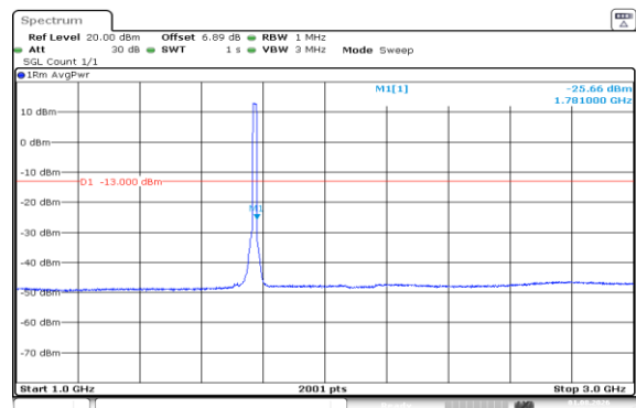
Band66-15MHz-16QAM-132597-75RB#0-1000~3000-PASS
