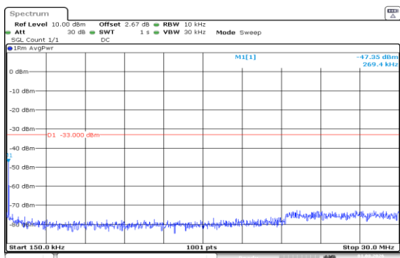
Band66-15MHz-QPSK-132597-75RB#0-0.15~30-PASS
