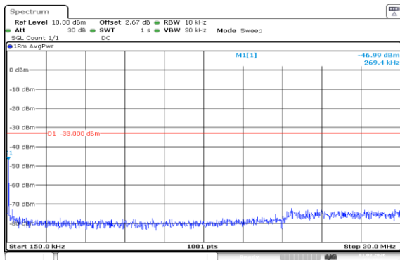
Band66-15MHz-QPSK-132597-1RB#74-0.15~30-PASS
