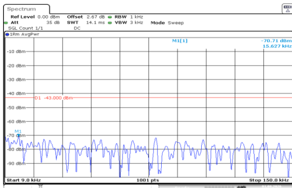
Band66-20MHz-16QAM-132322-100RB#0-0.009~0.15-PASS
