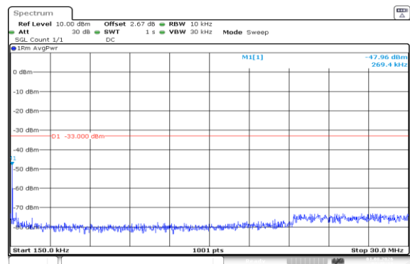
Band66-15MHz-16QAM-132597-75RB#0-0.15~30-PASS
