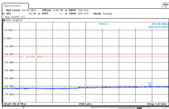
Band66-20MHz-16QAM-132322-1RB#0-30~1000-PASS
