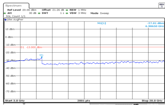
Band66-20MHz-QPSK-132072-1RB#99-3000~20000-PASS
