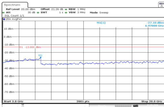
Band66-20MHz-16QAM-132322-1RB#99-3000~20000-PASS
