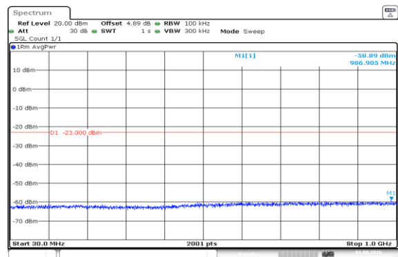
Band66-20MHz-QPSK-132322-1RB#99-30~1000-PASS
