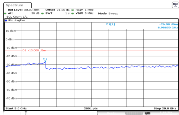
Band66-15MHz-QPSK-132597-1RB#0-3000~20000-PASS
