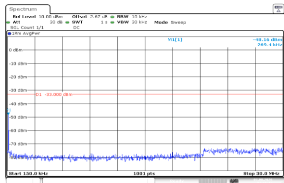
Band66-20MHz-16QAM-132072-100RB#0-0.15~30-PASS
