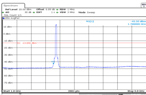
Band66-20MHz-QPSK-132322-100RB#0-1000~3000-PASS
