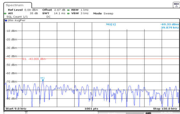
Band66-20MHz-QPSK-132572-1RB#99-0.009~0.15-PASS
