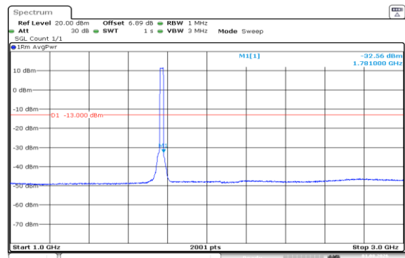
Band66-20MHz-16QAM-132572-100RB#0-1000~3000-PASS
