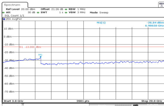
Band66-20MHz-16QAM-132572-1RB#0-3000~20000-PASS
