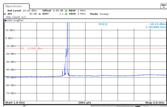
Band66-20MHz-16QAM-132572-1RB#99-1000~3000-PASS
