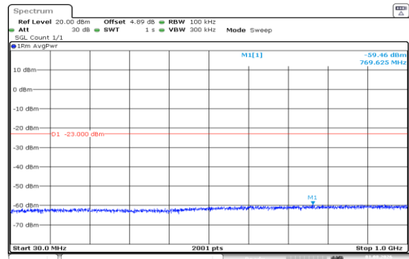
Band66-20MHz-QPSK-132572-1RB#99-30~1000-PASS
