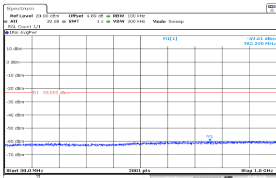
Band66-20MHz-16QAM-132572-100RB#0-30~1000-PASS
