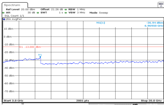
Band66-20MHz-16QAM-132322-1RB#0-3000~20000-PASS
