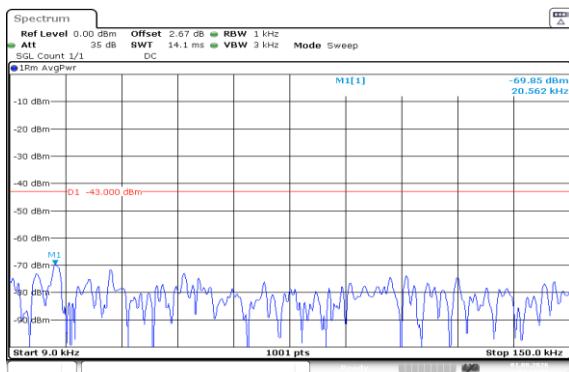
Band66-20MHz-16QAM-132072-100RB#0-0.009~0.15-PASS
