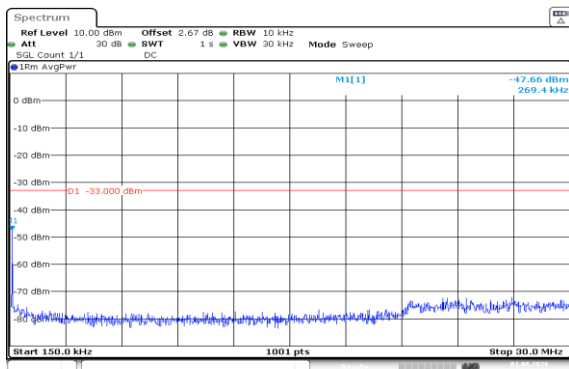
Band66-20MHz-QPSK-132322-1RB#0-0.15~30-PASS
