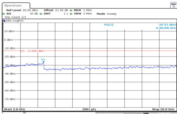
Band66-15MHz-16QAM-132597-1RB#0-3000~20000-PASS
