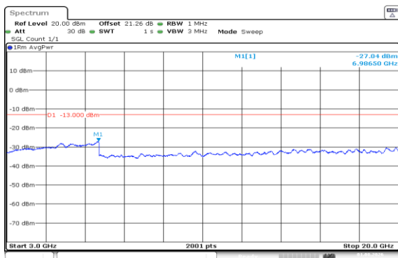
Band66-20MHz-16QAM-132072-1RB#99-3000~20000-PASS
