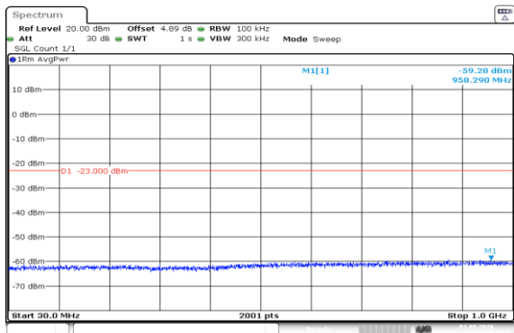
Band66-20MHz-16QAM-132322-100RB#0-30~1000-PASS
