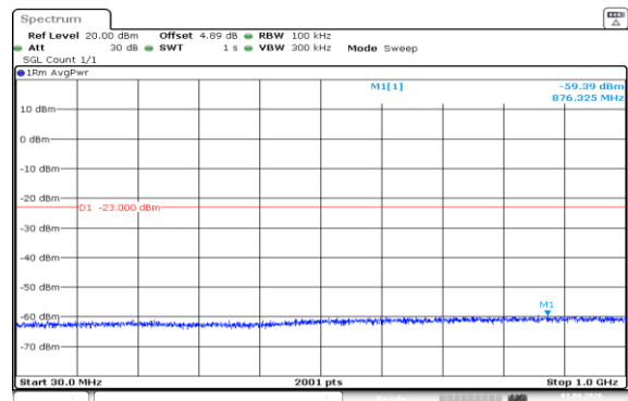
Band66-20MHz-QPSK-132322-1RB#0-30~1000-PASS
