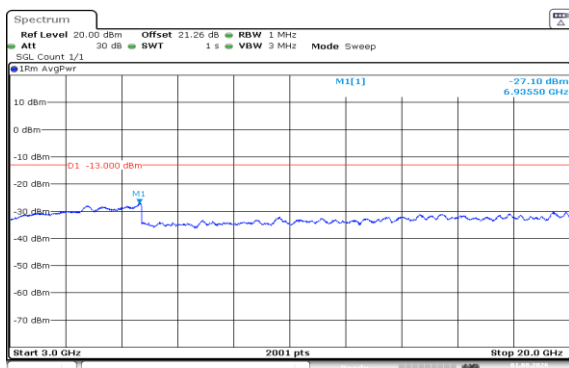
Band66-15MHz-QPSK-132597-1RB#74-3000~20000-PASS
