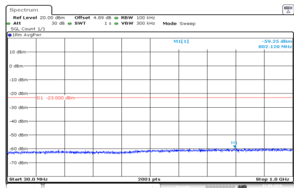
Band66-20MHz-16QAM-132072-1RB#0-30~1000-PASS
