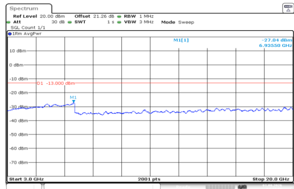
Band66-20MHz-QPSK-132322-1RB#0-3000~20000-PASS
