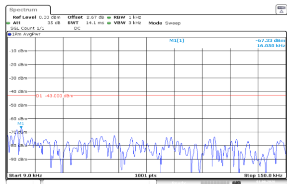
Band66-20MHz-QPSK-132322-1RB#0-0.009~0.15-PASS
