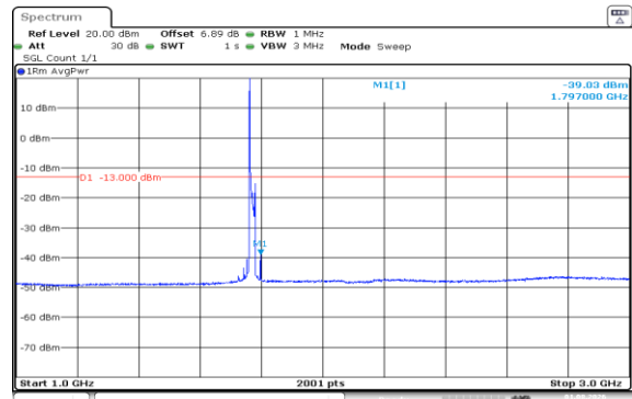
Band66-20MHz-16QAM-132572-1RB#0-1000~3000-PASS
