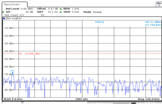
Band66-15MHz-16QAM-132597-1RB#0-0.009~0.15-PASS
