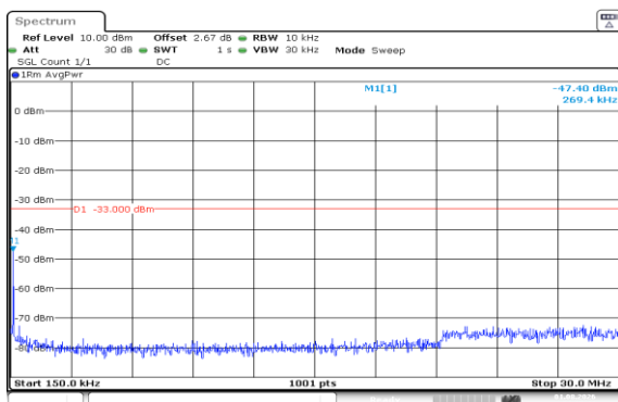
Band66-20MHz-QPSK-132072-100RB#0-0.15~30-PASS
