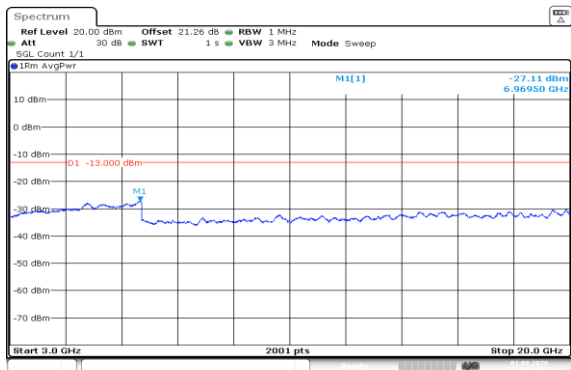
Band66-20MHz-16QAM-132072-1RB#0-3000~20000-PASS
