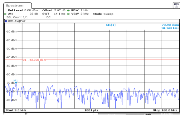
Band66-15MHz-QPSK-132597-1RB#74-0.009~0.15-PASS
