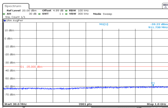
Band7-15MHz-16QAM-21100-1RB#74-30~1000-PASS
