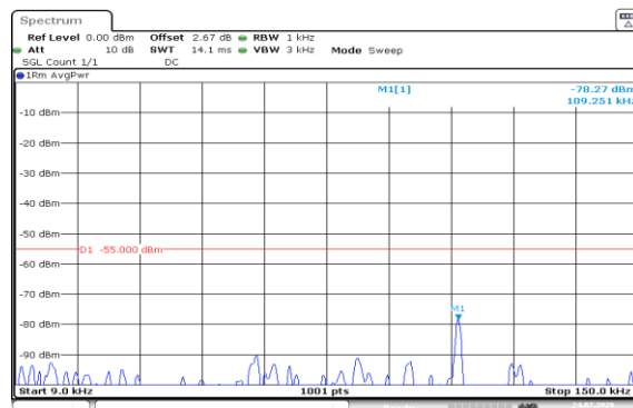
Band7-15MHz-QPSK-21375-1RB#0-0.009~0.15-PASS
