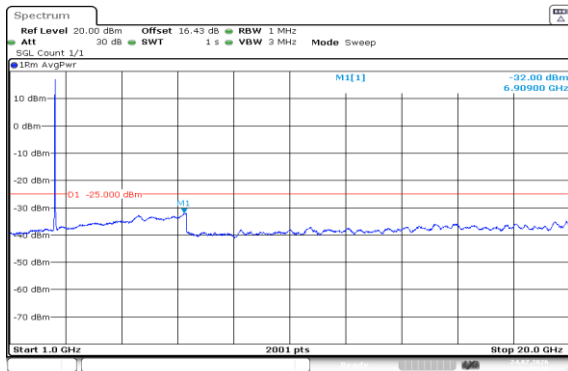
Band7-20MHz-16QAM-21100-100RB#0-1000~20000-PASS
