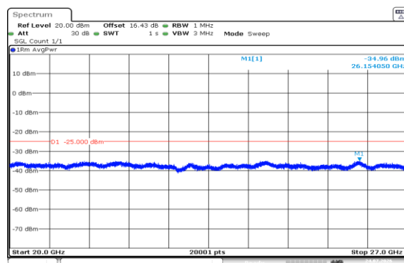
Band7-15MHz-QPSK-21100-75RB#0-20000~27000-PASS
