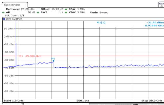
Band7-15MHz-QPSK-21375-1RB#0-1000~20000-PASS
