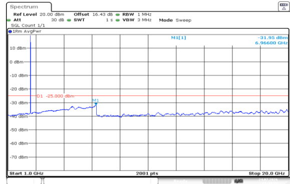
Band7-15MHz-16QAM-21100-1RB#0-1000~20000-PASS
