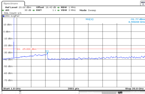
Band7-15MHz-QPSK-20825-1RB#74-1000~20000-PASS
