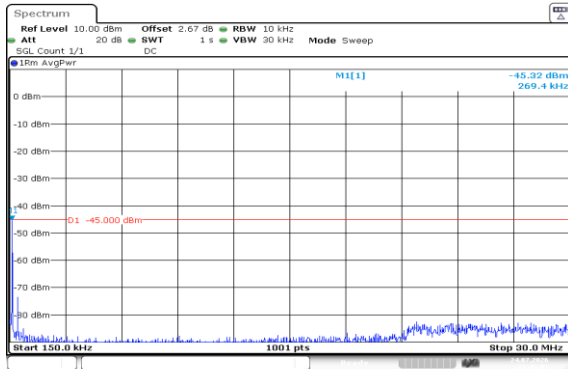
Band7-15MHz-QPSK-20825-75RB#0-0.15~30-PASS
