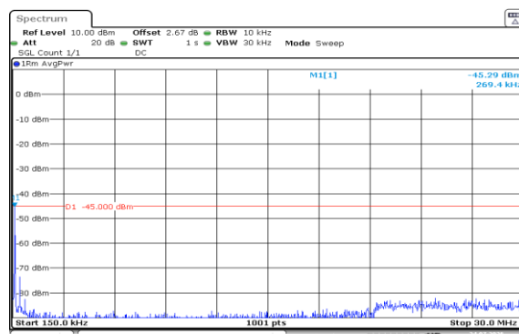
Band7-20MHz-QPSK-21350-1RB#99-0.15~30-PASS
