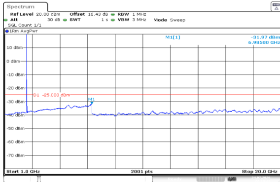
Band7-20MHz-QPSK-20850-1RB#0-1000~20000-PASS
