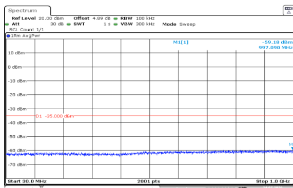
Band7-10MHz-QPSK-21400-50RB#0-30~1000-PASS
