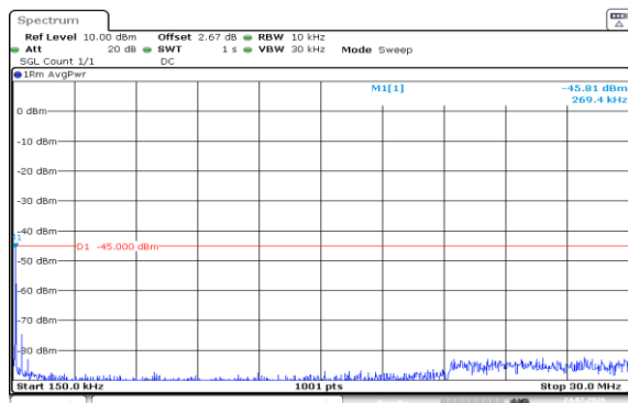
Band7-10MHz-16QAM-21400-50RB#0-0.15~30-PASS
