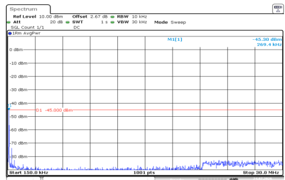
Band7-20MHz-QPSK-21100-1RB#99-0.15~30-PASS
