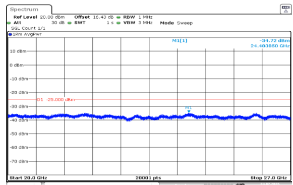
Band7-20MHz-16QAM-21100-1RB#0-20000~27000-PASS
