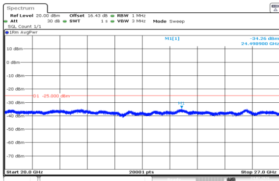
Band7-20MHz-16QAM-20850-1RB#0-20000~27000-PASS
