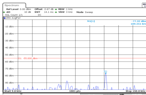
Band7-20MHz-16QAM-21100-1RB#99-0.009~0.15-PASS
