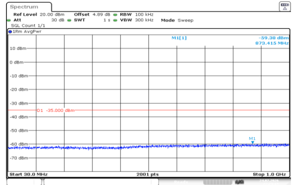
Band7-20MHz-QPSK-21350-100RB#0-30~1000-PASS
