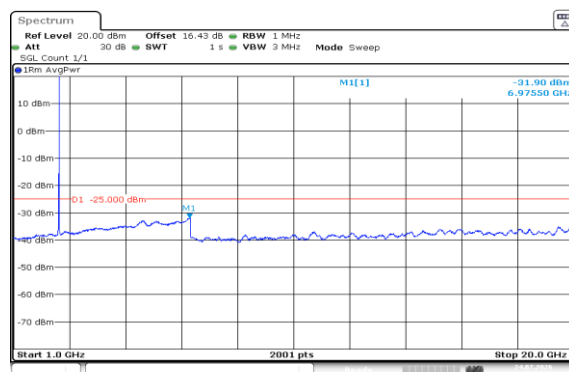
Band7-20MHz-QPSK-21100-1RB#99-1000~20000-PASS
