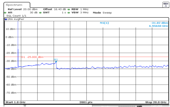
Band7-20MHz-QPSK-21350-1RB#0-1000~20000-PASS
