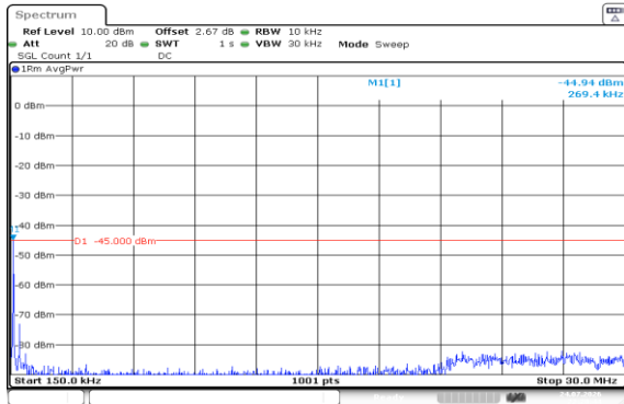
Band7-20MHz-QPSK-20850-1RB#99-0.15~30
