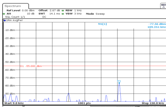
Band7-20MHz-QPSK-20850-100RB#0-0.009~0.15-PASS
