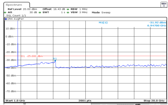
Band7-15MHz-16QAM-21375-1RB#0-1000~20000-PASS
