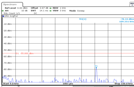
Band7-20MHz-QPSK-21100-1RB#0-0.009~0.15-PASS
