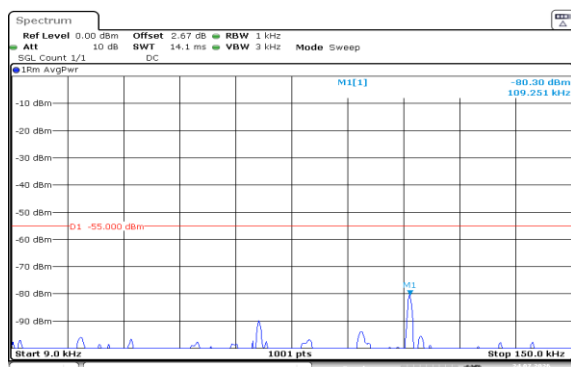
Band7-15MHz-16QAM-21100-75RB#0-0.009~0.15-PASS
