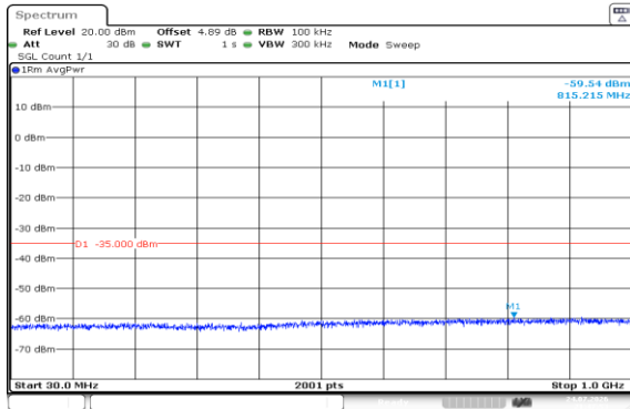
Band7-15MHz-16QAM-21100-1RB#0-30~1000-PASS
