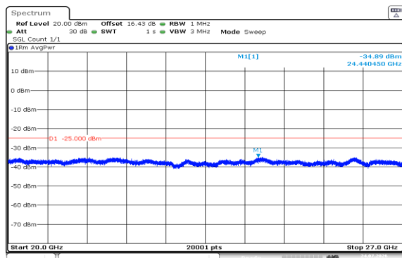
Band7-15MHz-16QAM-21100-75RB#0-20000~27000-PASS
