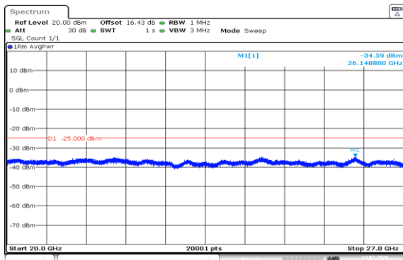
Band7-20MHz-QPSK-20850-1RB#99-20000~27000-PASS
