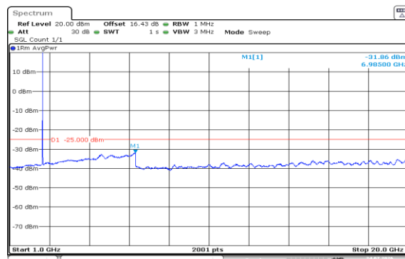
Band7-20MHz-QPSK-21350-1RB#99-1000~20000-PASS
