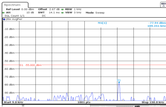
Band7-15MHz-QPSK-20825-1RB#74-0.009~0.15-PASS
