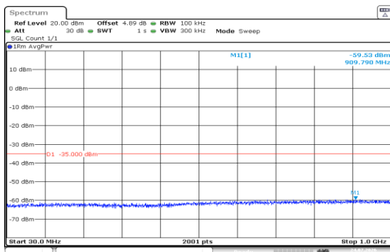
Band7-20MHz-QPSK-21100-1RB#0-30~1000-PASS
