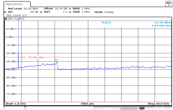
Band7-15MHz-16QAM-21375-1RB#74-1000~20000-PASS
