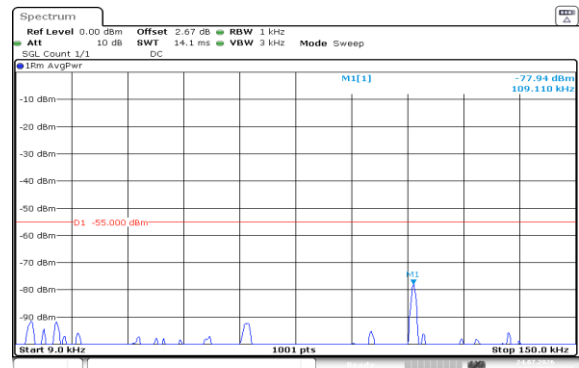
Band7-15MHz-QPSK-20825-75RB#0-0.009~0.15-PASS
