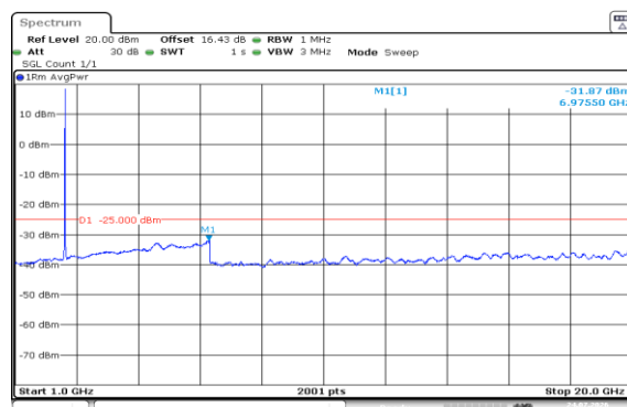
Band7-15MHz-16QAM-21100-75RB#0-1000~20000-PASS
