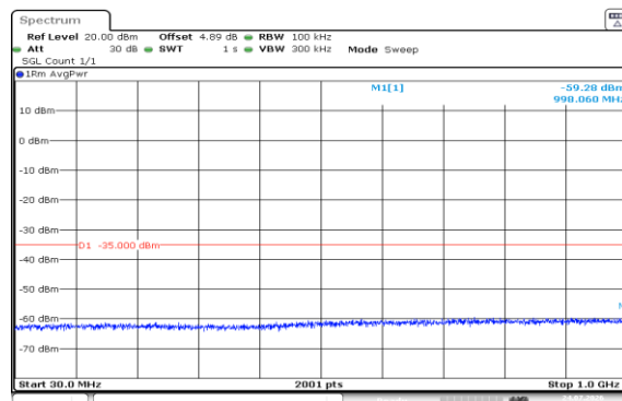
Band7-15MHz-QPSK-21100-75RB#0-30~1000-PASS
