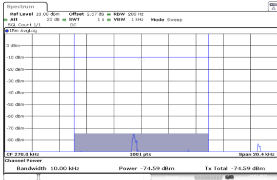
Band7-20MHz-QPSK-21350-100RB#0-0.15~30-PASS
