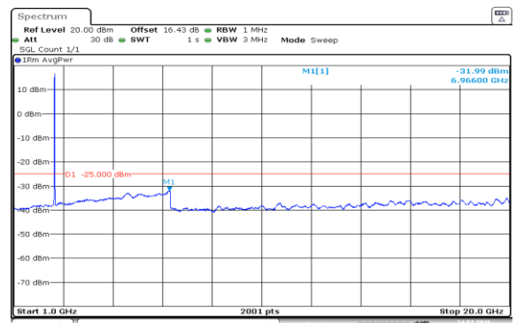
Band7-20MHz-16QAM-21350-100RB#0-1000~20000-PASS
