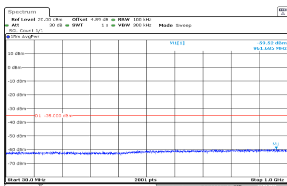
Band7-20MHz-QPSK-20850-100RB#0-30~1000-PASS
