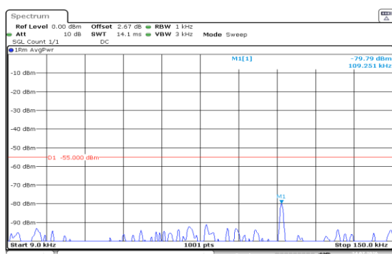
Band7-15MHz-QPSK-20825-1RB#0-0.009~0.15-PASS
