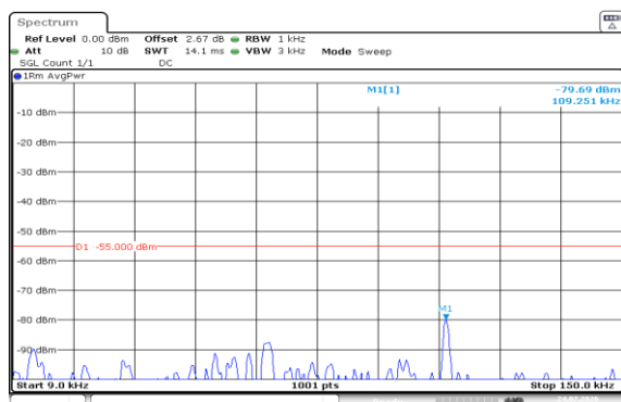
Band7-15MHz-16QAM-21100-1RB#74-0.009~0.15-PASS
