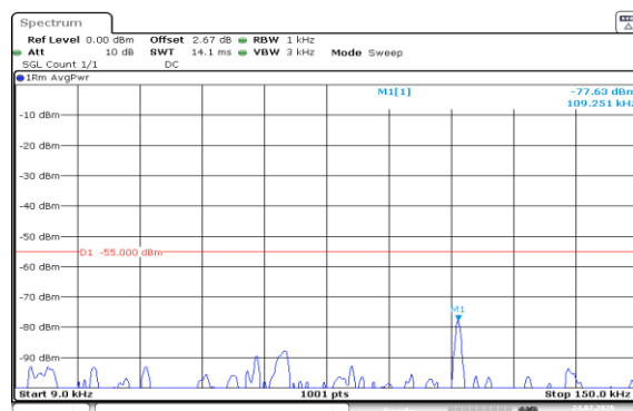
Band7-15MHz-16QAM-20825-1RB#0-0.009~0.15-PASS
