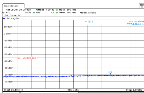
Band7-15MHz-QPSK-20825-1RB#0-30~1000-PASS
