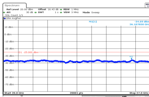
Band7-20MHz-16QAM-20850-1RB#99-20000~27000-PASS
