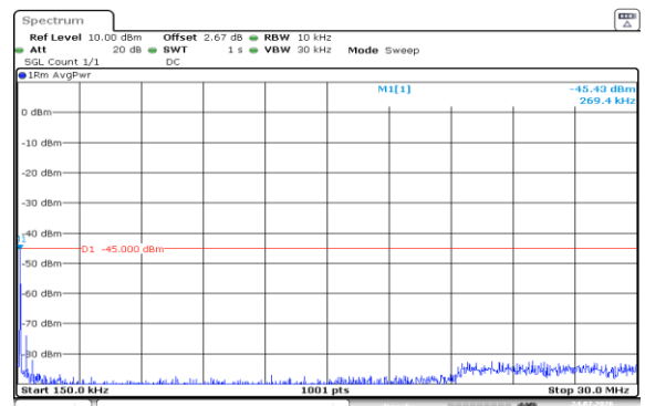
Band7-20MHz-QPSK-21100-1RB#0-0.15~30-PASS
