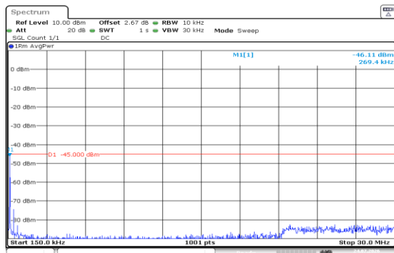
Band7-20MHz-16QAM-21350-1RB#0-0.15~30-PASS
