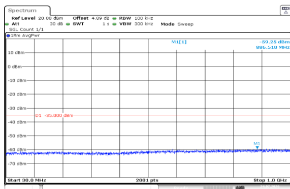
Band7-20MHz-QPSK-21100-1RB#99-30~1000-PASS
