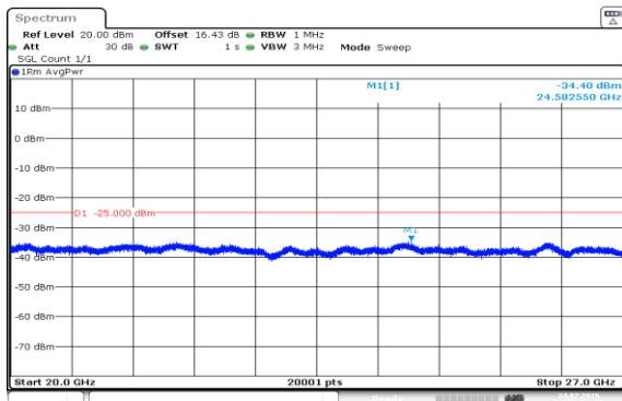
Band7-15MHz-16QAM-21375-1RB#74-20000~27000-PASS
