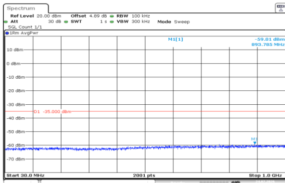
Band7-15MHz-16QAM-21375-1RB#0-30~1000-PASS
