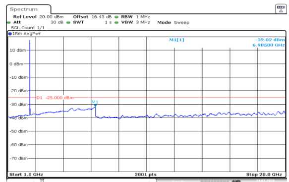
Band7-15MHz-16QAM-20825-75RB#0-1000~20000-PASS
