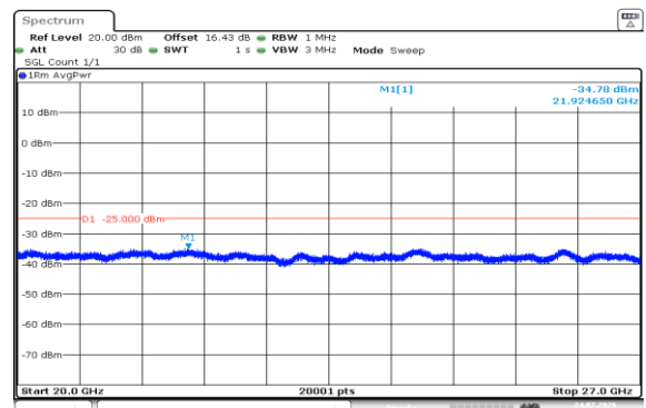
Band7-15MHz-QPSK-21375-75RB#0-20000~27000-PASS
