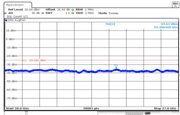
Band7-20MHz-16QAM-21100-100RB#0-20000~27000-PASS
