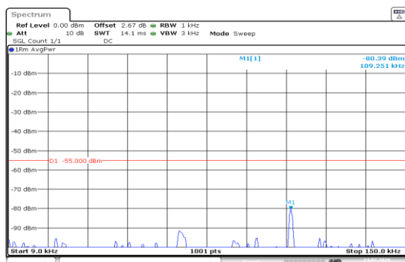
Band7-10MHz-QPSK-21400-50RB#0-0.009~0.15-PASS
