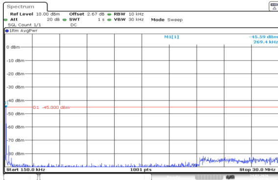
Band7-20MHz-16QAM-20850-100RB#0-0.15~30-PASS
