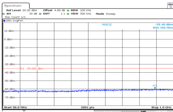
Band7-15MHz-16QAM-20825-75RB#0-30~1000-PASS
