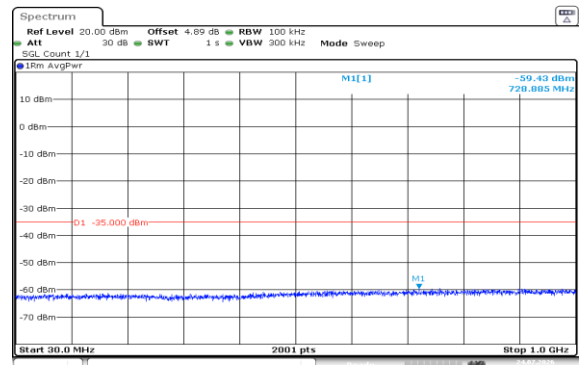
Band7-15MHz-QPSK-20825-1RB#74-30~1000-PASS
