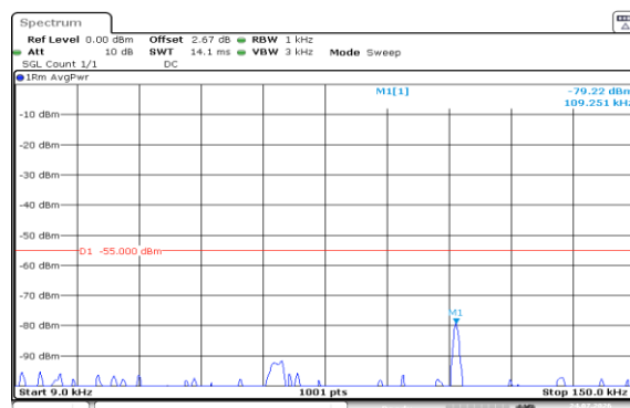
Band7-15MHz-QPSK-21100-75RB#0-0.009~0.15-PASS
