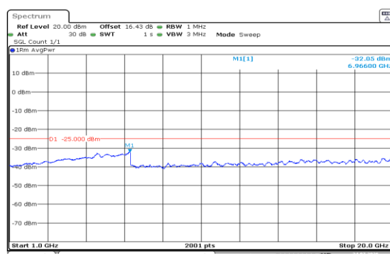
Band7-15MHz-QPSK-20825-1RB#0-1000~20000-PASS
