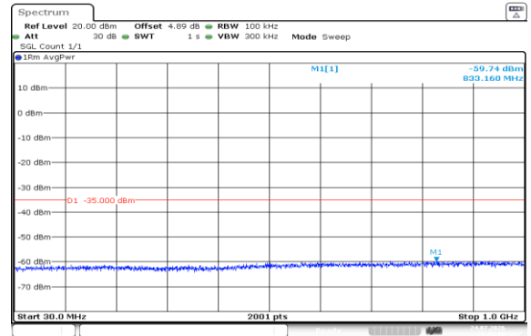
Band7-15MHz-QPSK-20825-75RB#0-30~1000-PASS
