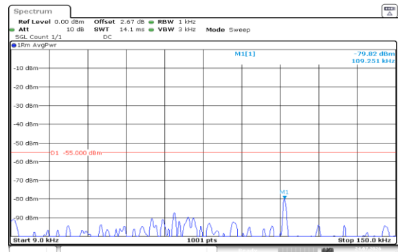
Band7-15MHz-QPSK-21100-1RB#74-0.009~0.15-PASS
