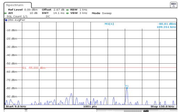
Band7-20MHz-QPSK-20850-1RB#99-0.009~0.15-PASS
