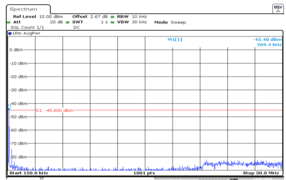
Band7-20MHz-16QAM-21350-100RB#0-0.15~30-PASS
