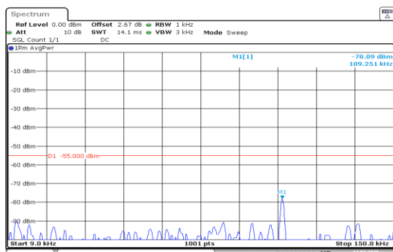
Band7-20MHz-QPSK-21350-1RB#99-0.009~0.15-PASS
