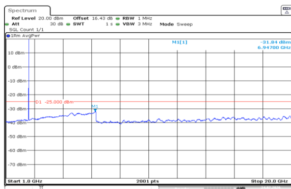
Band7-20MHz-16QAM-20850-1RB#99-1000~20000-PASS
