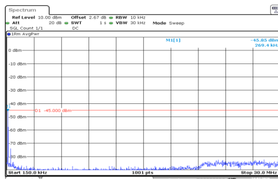
Band7-15MHz-16QAM-21100-75RB#0-0.15~30-PASS
