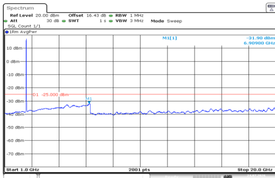
Band7-20MHz-16QAM-20850-100RB#0-1000~20000-PASS
