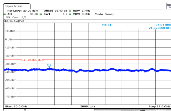
Band7-10MHz-16QAM-21400-50RB#0-20000~27000-PASS
