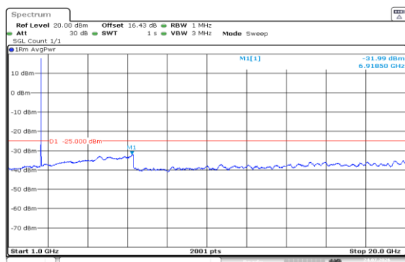
Band7-10MHz-16QAM-21400-50RB#0-1000~20000-PASS
