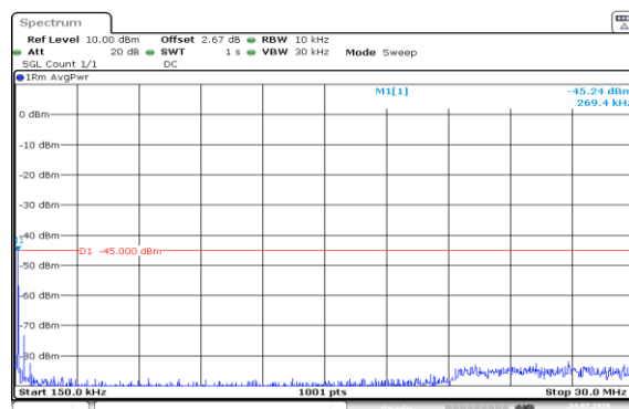
Band7-10MHz-QPSK-21400-50RB#0-0.15~30-PASS
