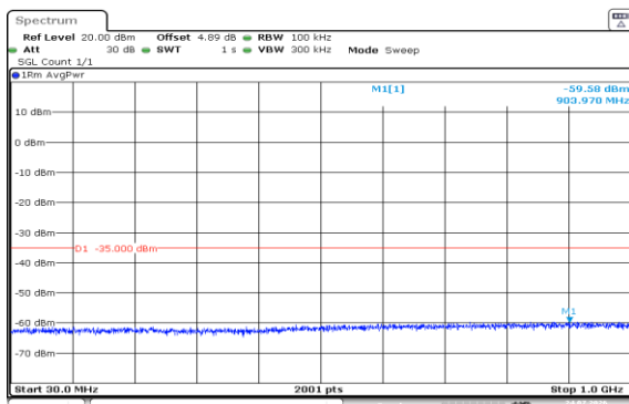
Band7-20MHz-16QAM-21350-100RB#0-30~1000-PASS
