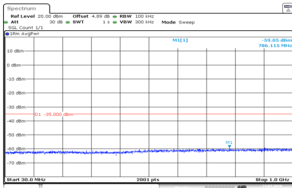
Band7-15MHz-16QAM-20825-1RB#74-30~1000-PASS
