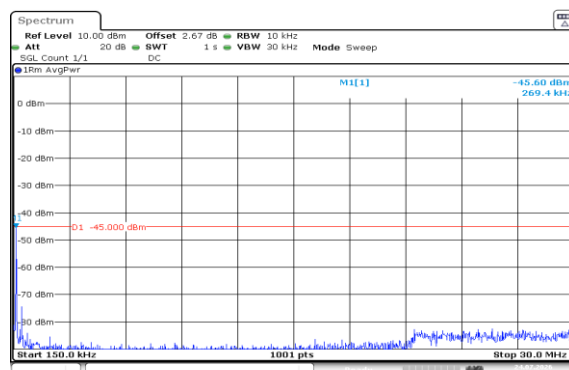
Band7-15MHz-16QAM-21100-1RB#74-0.15~30-PASS
