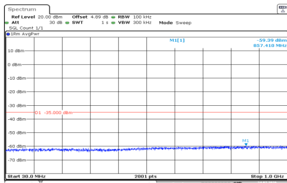
Band7-20MHz-QPSK-21350-1RB#99-30~1000-PASS
