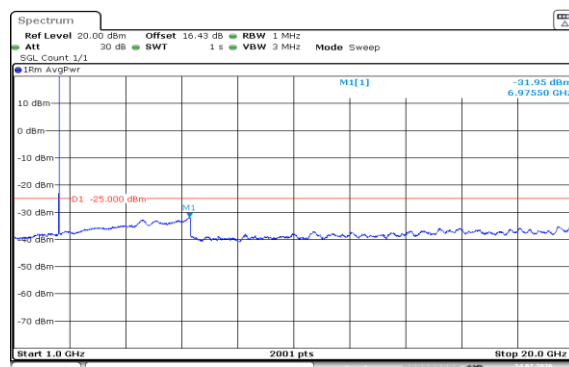
Band7-15MHz-16QAM-21100-1RB#74-1000~20000-PASS
