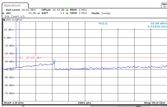
Band7-20MHz-16QAM-21100-1RB#0-1000~20000-PASS
