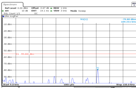
Band7-20MHz-16QAM-21350-100RB#0-0.009~0.15-PASS
