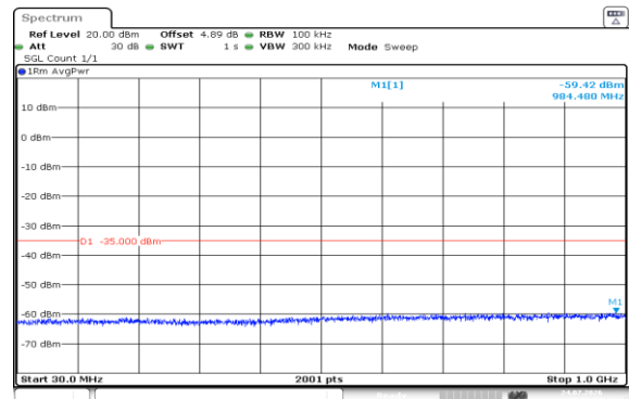
Band7-20MHz-16QAM-20850-1RB#99-30~1000-PASS
