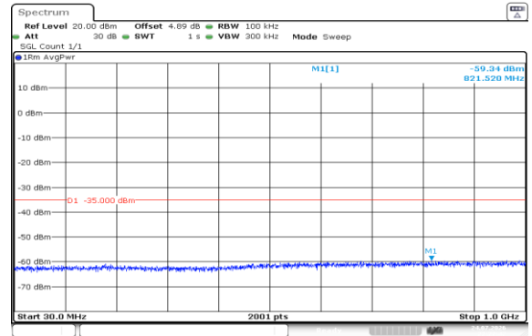
Band7-20MHz-16QAM-20850-100RB#0-30~1000-PASS
