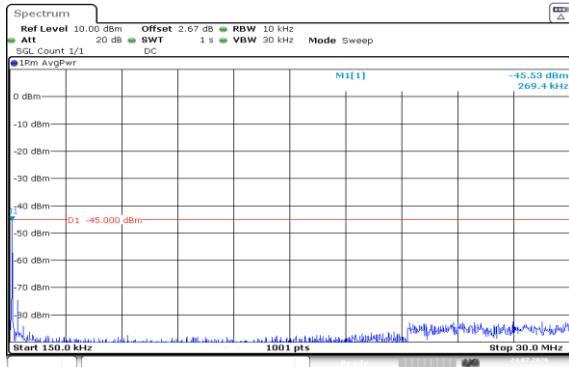
Band7-15MHz-QPSK-21375-1RB#0-0.15~30-PASS
