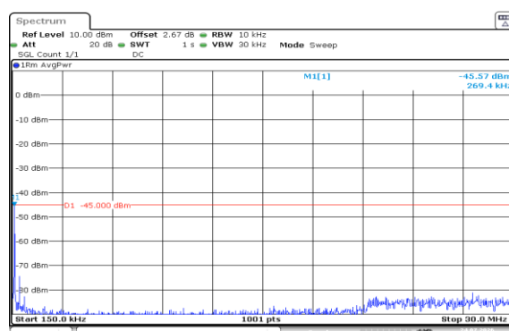
Band7-15MHz-QPSK-20825-1RB#0-0.15~30-PASS
