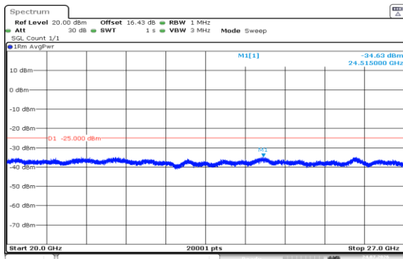
Band7-20MHz-QPSK-21350-1RB#0-20000~27000-PASS
