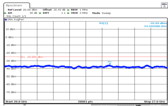
Band7-15MHz-QPSK-21100-1RB#74-20000~27000-PASS
