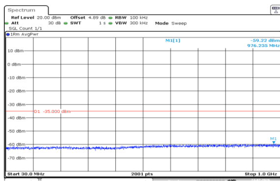
Band7-15MHz-16QAM-21100-75RB#0-30~1000-PASS
