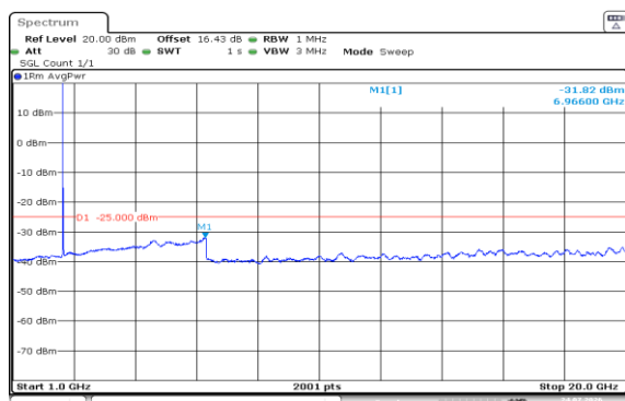
Band7-20MHz-16QAM-21350-1RB#0-1000~20000-PASS
