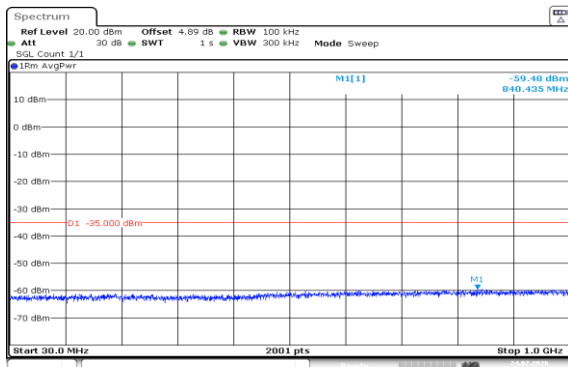
Band7-20MHz-QPSK-21350-1RB#0-30~1000-PASS
