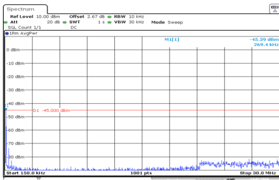
Band7-15MHz-QPSK-21375-75RB#0-0.15~30-PASS
