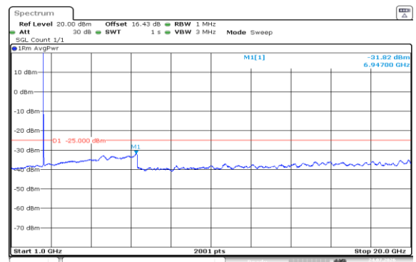
Band7-20MHz-QPSK-21100-1RB#0-1000~20000-PASS
