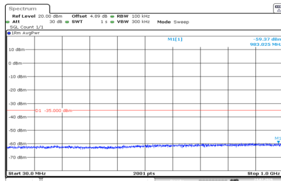
Band7-20MHz-16QAM-21350-1RB#0-30~1000-PASS
