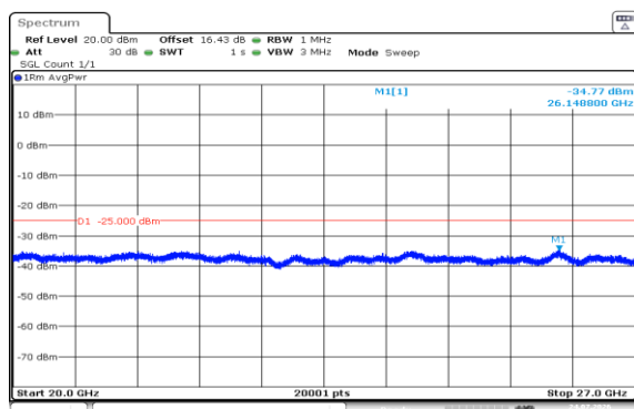
Band7-10MHz-QPSK-21400-50RB#0-20000~27000-PASS
