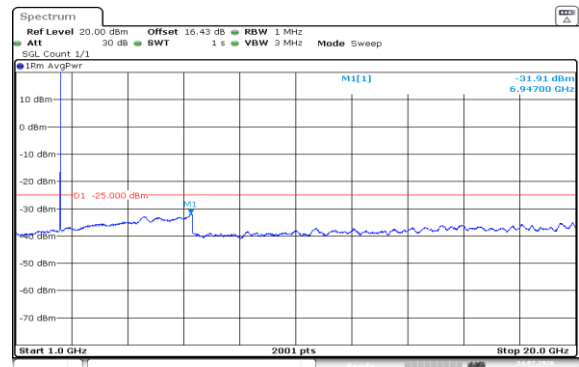
Band7-15MHz-16QAM-20825-1RB#74-1000~20000-PASS
