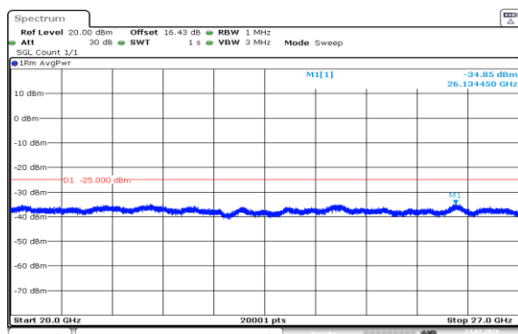
Band7-20MHz-QPSK-21100-1RB#99-20000~27000-PASS
