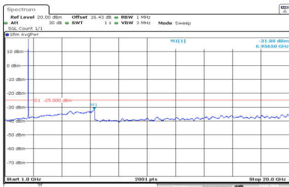
Band7-15MHz-QPSK-21375-75RB#0-1000~20000-PASS
