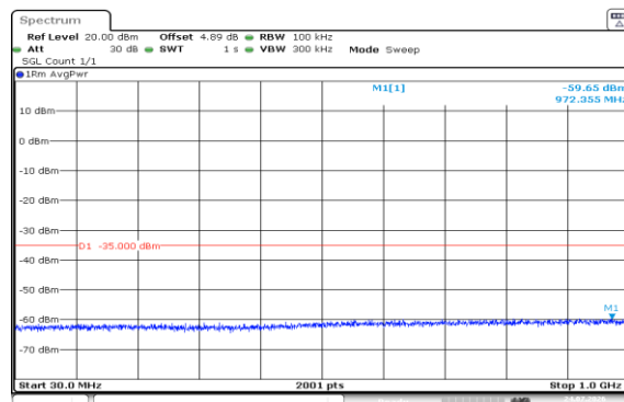
Band7-10MHz-16QAM-21400-50RB#0-30~1000-PASS
