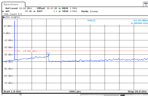
Band7-20MHz-QPSK-21350-100RB#0-1000~20000-PASS
