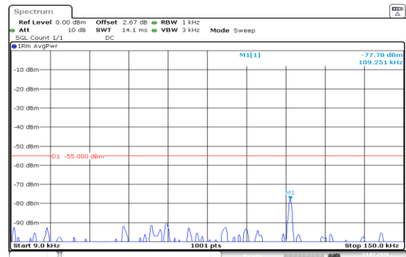
Band7-20MHz-16QAM-20850-1RB#99-0.009~0.15-PASS
