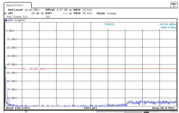
Band7-15MHz-QPSK-20825-1RB#74-0.15~30
