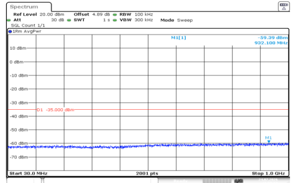
Band7-15MHz-QPSK-21375-1RB#0-30~1000-PASS
