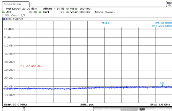
Band7-15MHz-16QAM-21375-1RB#74-30~1000-PASS
