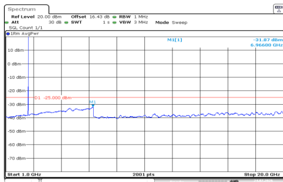
Band7-20MHz-16QAM-21100-1RB#99-1000~20000-PASS
