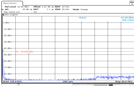
Band7-15MHz-16QAM-20825-1RB#0-0.15~30-PASS
