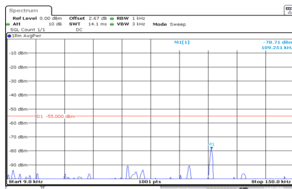
Band7-10MHz-16QAM-21400-50RB#0-0.009~0.15-PASS
