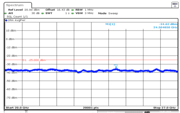
Band7-20MHz-16QAM-20850-100RB#0-20000~27000-PASS
