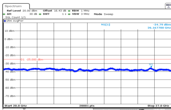
Band7-15MHz-16QAM-21100-1RB#74-20000~27000-PASS
