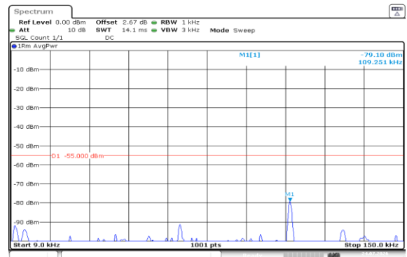
Band7-15MHz-QPSK-21375-75RB#0-0.009~0.15-PASS
