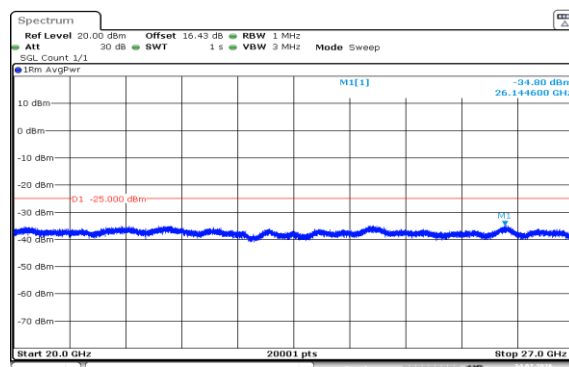
Band7-20MHz-16QAM-21350-1RB#0-20000~27000-PASS
