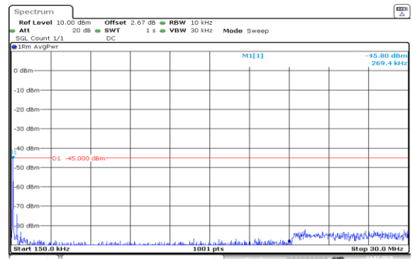
Band7-15MHz-16QAM-21375-1RB#0-0.15~30-PASS
