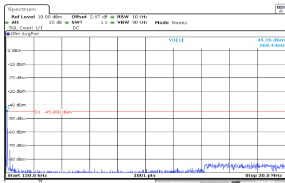
Band7-15MHz-QPSK-21100-75RB#0-0.15~30-PASS
