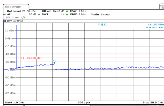
Band7-20MHz-QPSK-20850-100RB#0-1000~20000-PASS
