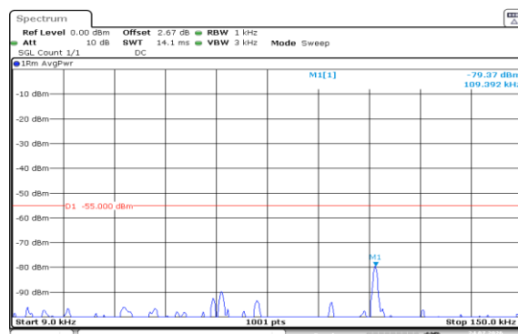
Band7-20MHz-16QAM-20850-100RB#0-0.009~0.15-PASS
