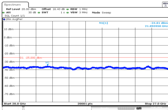
Band7-20MHz-QPSK-21100-1RB#0-20000~27000-PASS
