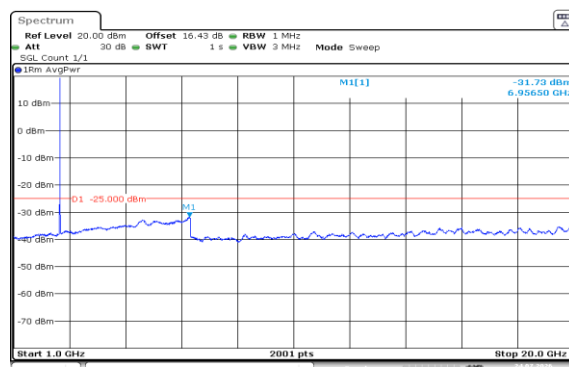
Band7-10MHz-QPSK-21400-50RB#0-1000~20000-PASS
