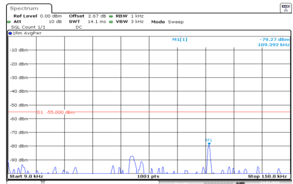
Band7-20MHz-16QAM-21350-1RB#0-0.009~0.15-PASS
