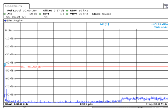
Band7-20MHz-QPSK-20850-100RB#0-0.15~30-PASS
