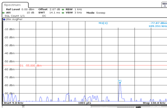
Band7-20MHz-16QAM-20850-1RB#0-0.009~0.15-PASS
