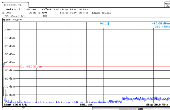
Band7-20MHz-16QAM-20850-1RB#99-0.15~30-PASS
