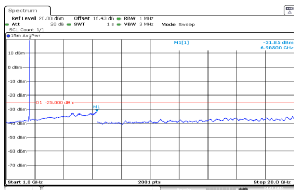
Band7-15MHz-QPSK-21100-75RB#0-1000~20000-PASS
