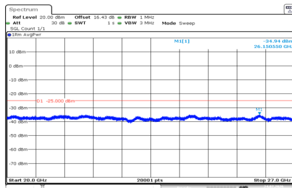
Band7-20MHz-16QAM-21100-1RB#99-20000~27000-PASS
