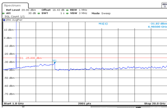
Band7-15MHz-QPSK-21100-1RB#74-1000~20000-PASS
