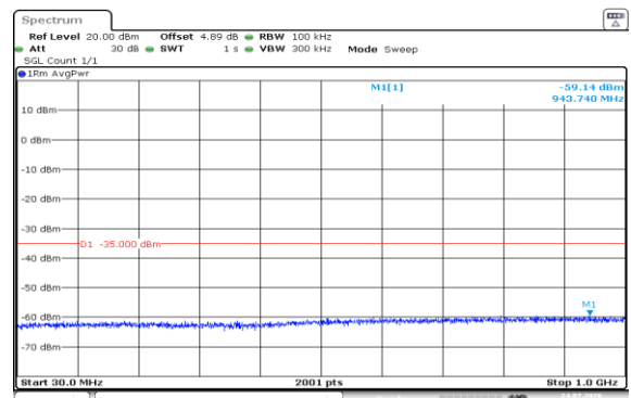
Band7-15MHz-QPSK-21375-75RB#0-30~1000-PASS
