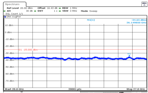
Band7-15MHz-QPSK-21375-1RB#0-20000~27000-PASS
