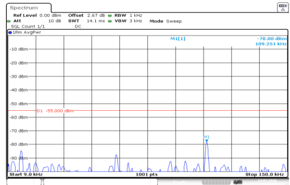
Band7-20MHz-16QAM-21100-1RB#0-0.009~0.15-PASS
