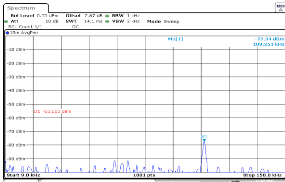
Band7-15MHz-16QAM-21375-1RB#0-0.009~0.15-PASS
