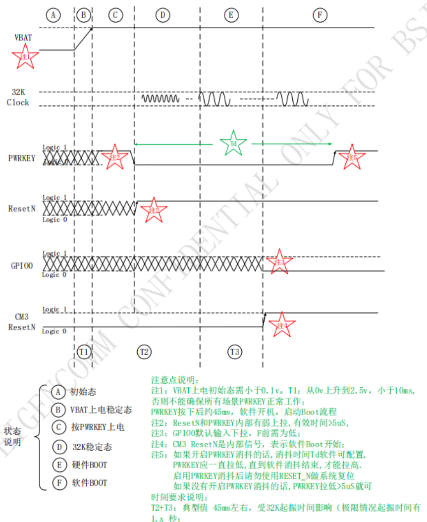
Figure 10: Power-on timing diagram
