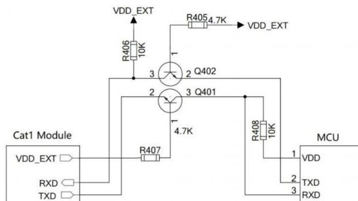
Figure 12: Transistor level conversion circuit
