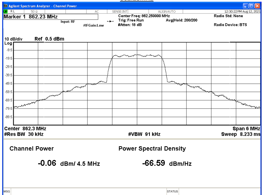
Graph 2: Output Power – Port 2A – Middle Channel
