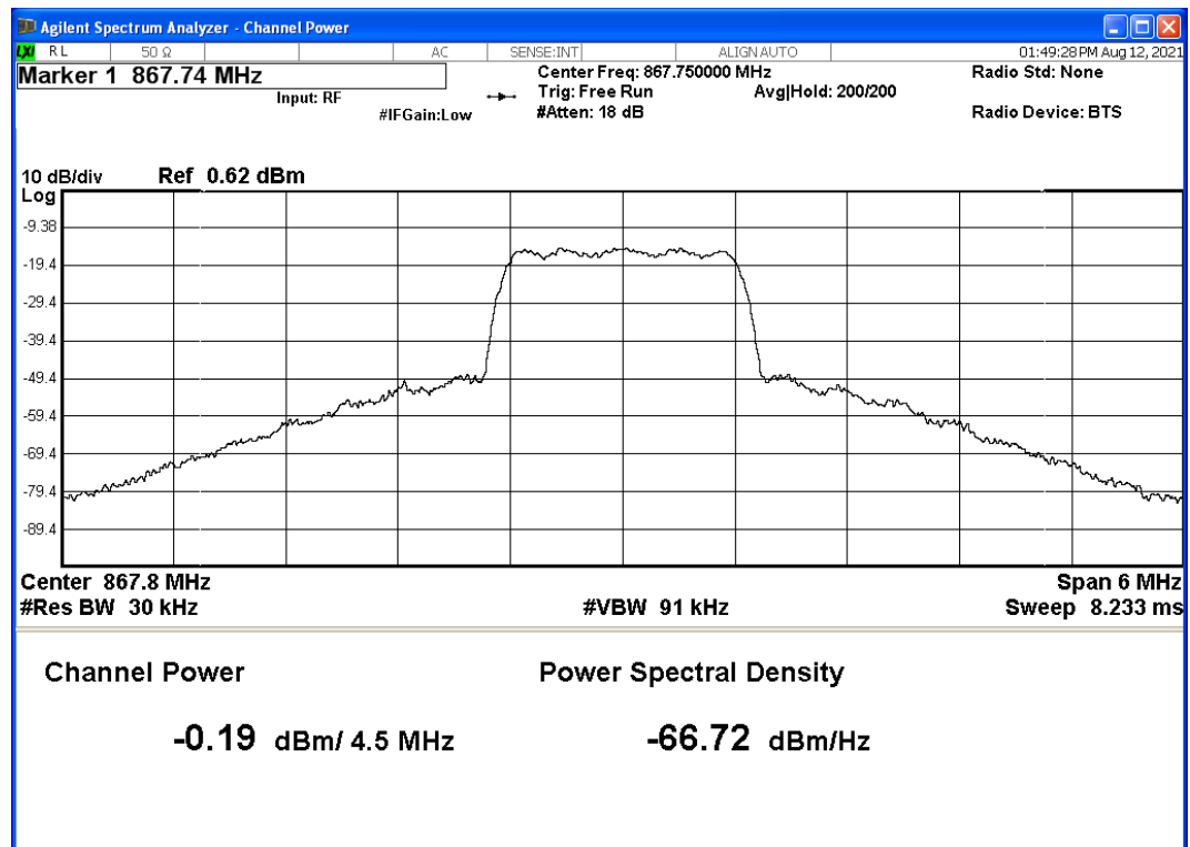
Graph 3: Output Power – Port 1A – Top Channel
