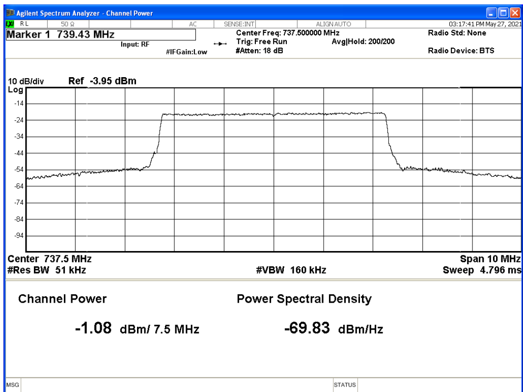
Graph 2: Output Power – Port 1B – Middle Channel
