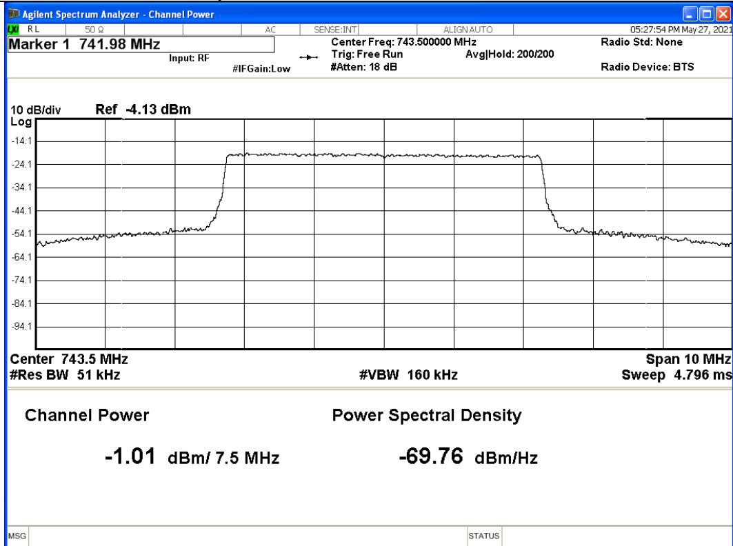
Graph 3: Output Power – Port 1A – Top Channel
