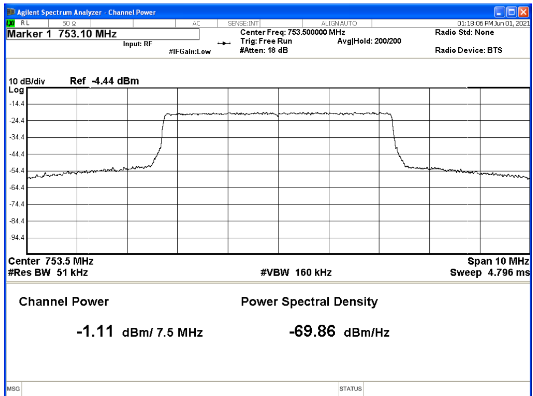
Graph 3: Output Power – Port 2B – Top Channel
