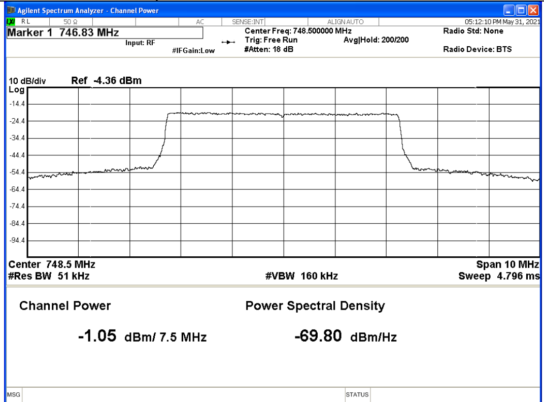
Graph 1: Output Power – Port 2B – Bottom Channel
