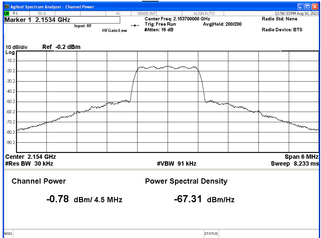
Graph 3: Output Power – Port 1A – Bottom Channel
