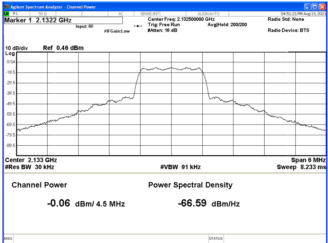
Graph 2: Output Power – Port 1A – Bottom Channel
