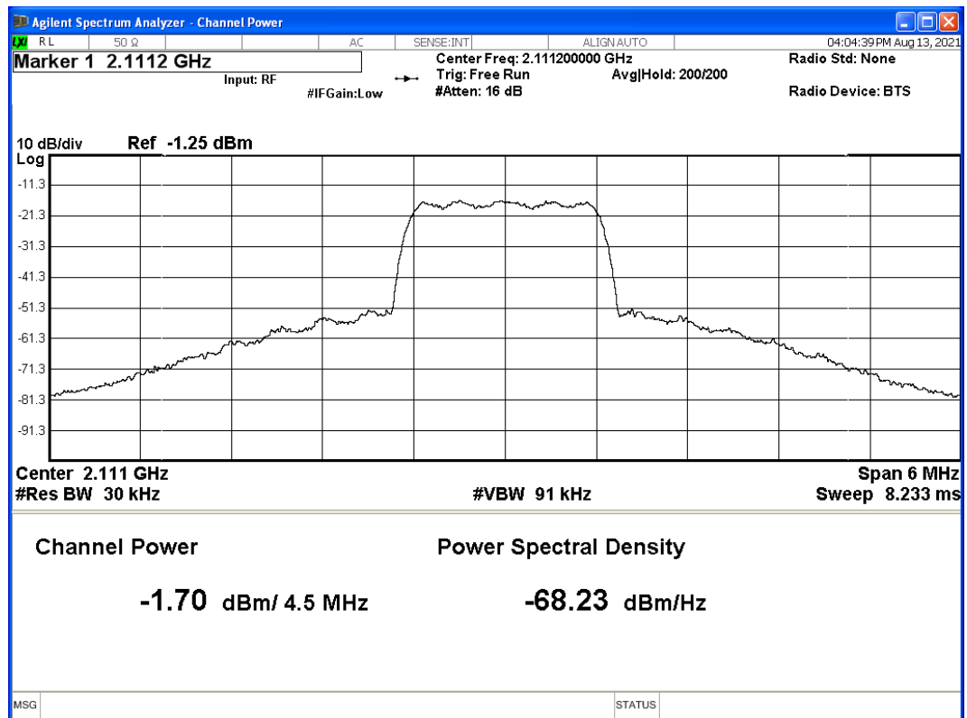
Graph 1: Output Power – Port 1A – Bottom Channel
