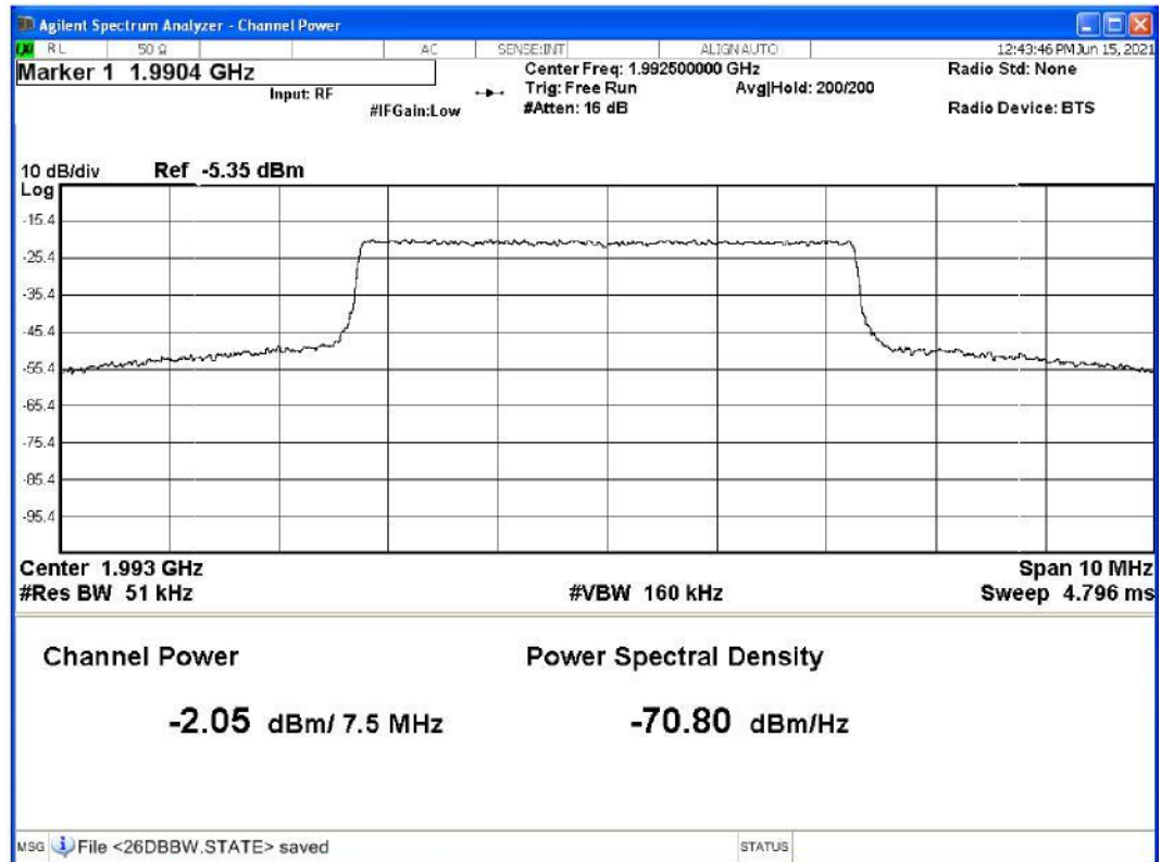
Graph 5: Output Power – Port 1A – Top Channel
