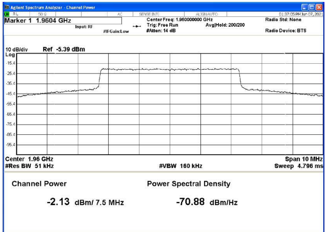
Graph 2: Output Power – Port 2B – Middle Channel
