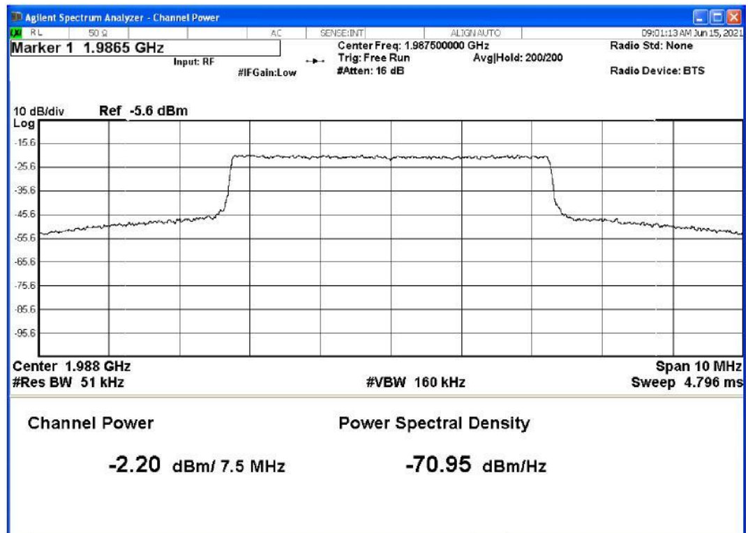
Graph 4: Output Power – Port 1A – Bottom/Top Channel
