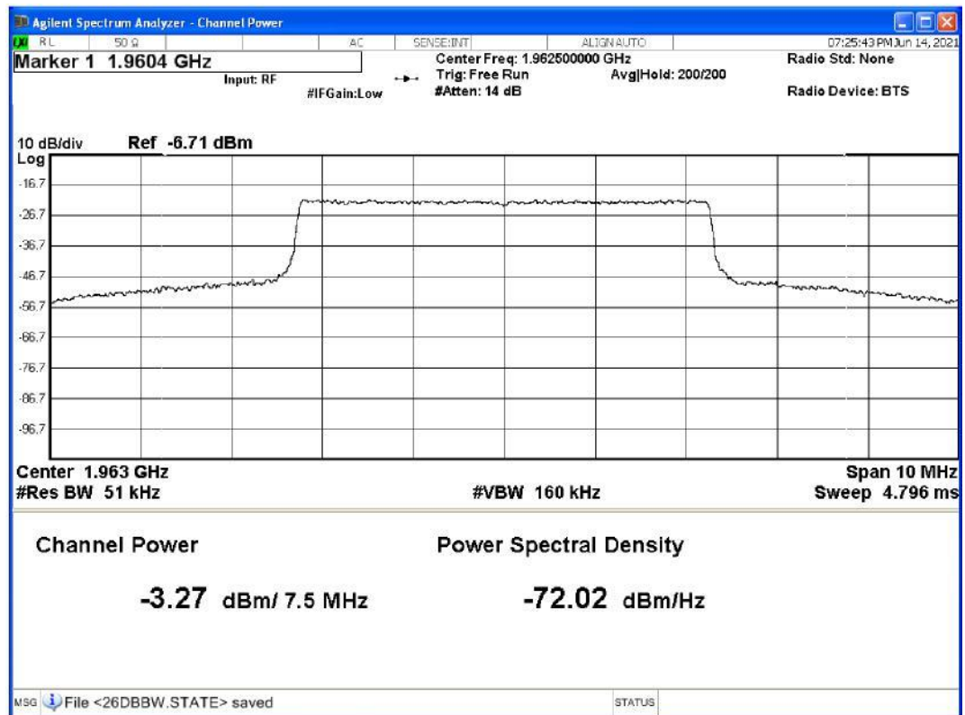
Graph 3: Output Power – Port 1A – Middle Channel
