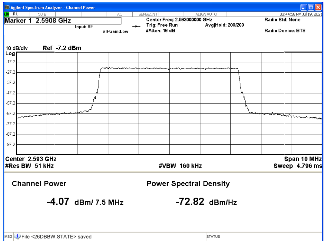
Graph 2: Output Power – Port 1A – Middle Channel: 2593 MHz
