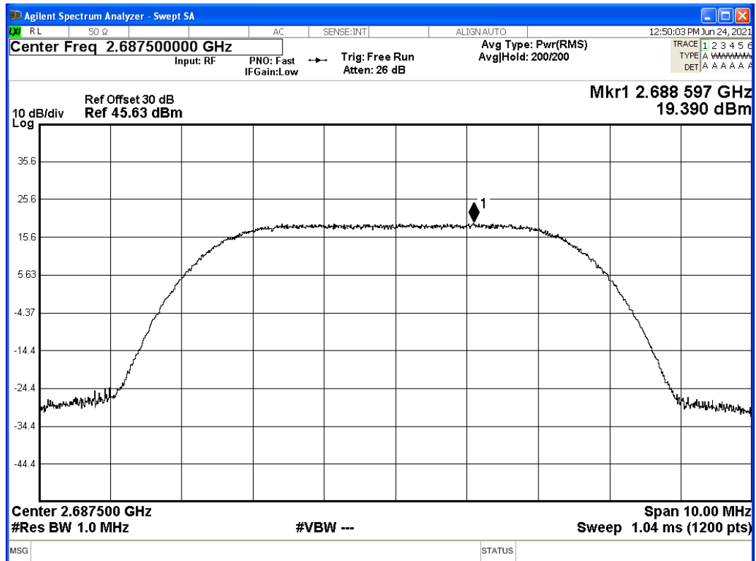
Graph 4: PSD – Port 1A – Top Channel: 2687.5 MHz
