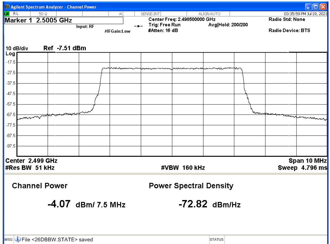
Graph 1: Output Power – Port 2A – Bottom Channel: 2498.5 MHz
