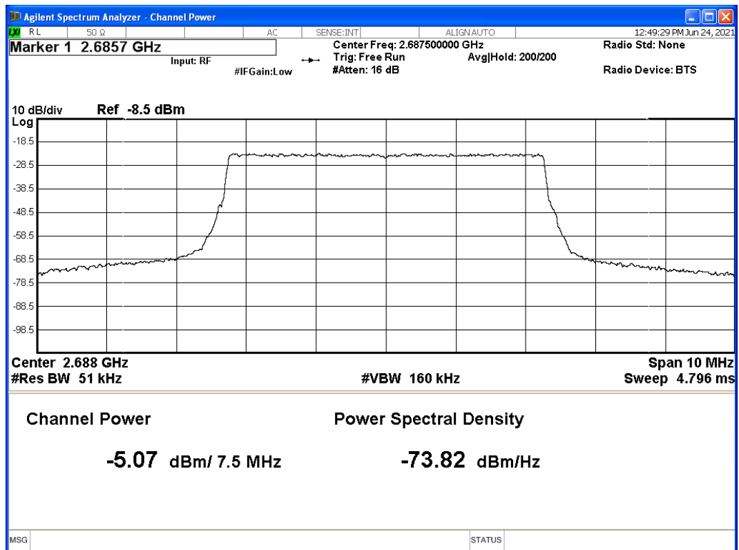
Graph 3: Output Power – Port 2A – Top Channel: 2687.5 MHz
