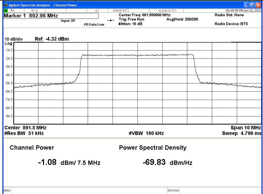
Graph 3: Output Power – Port 2B – Top Channel
