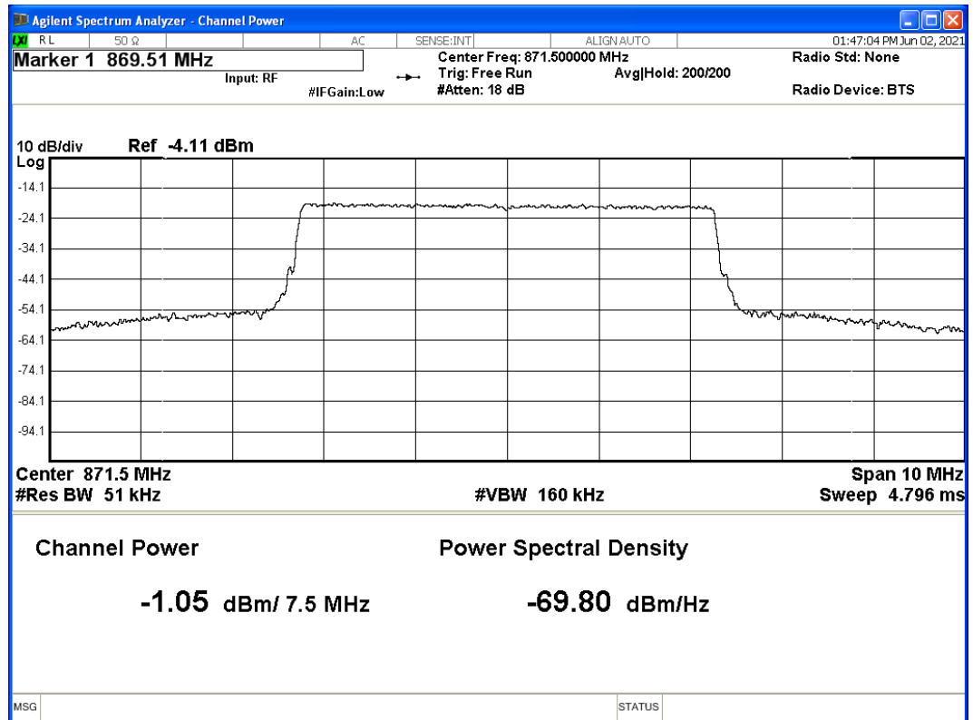
Graph 1: Output Power – Port 1B – Bottom Channel
