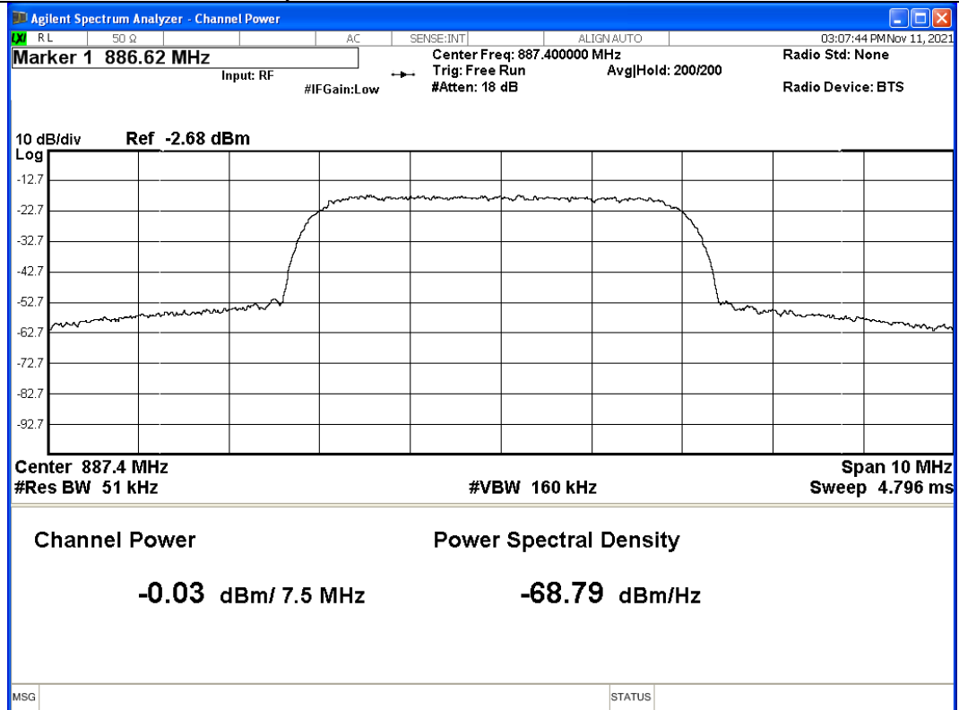
Graph 4: Output Power – Port 2B – Top Channel
