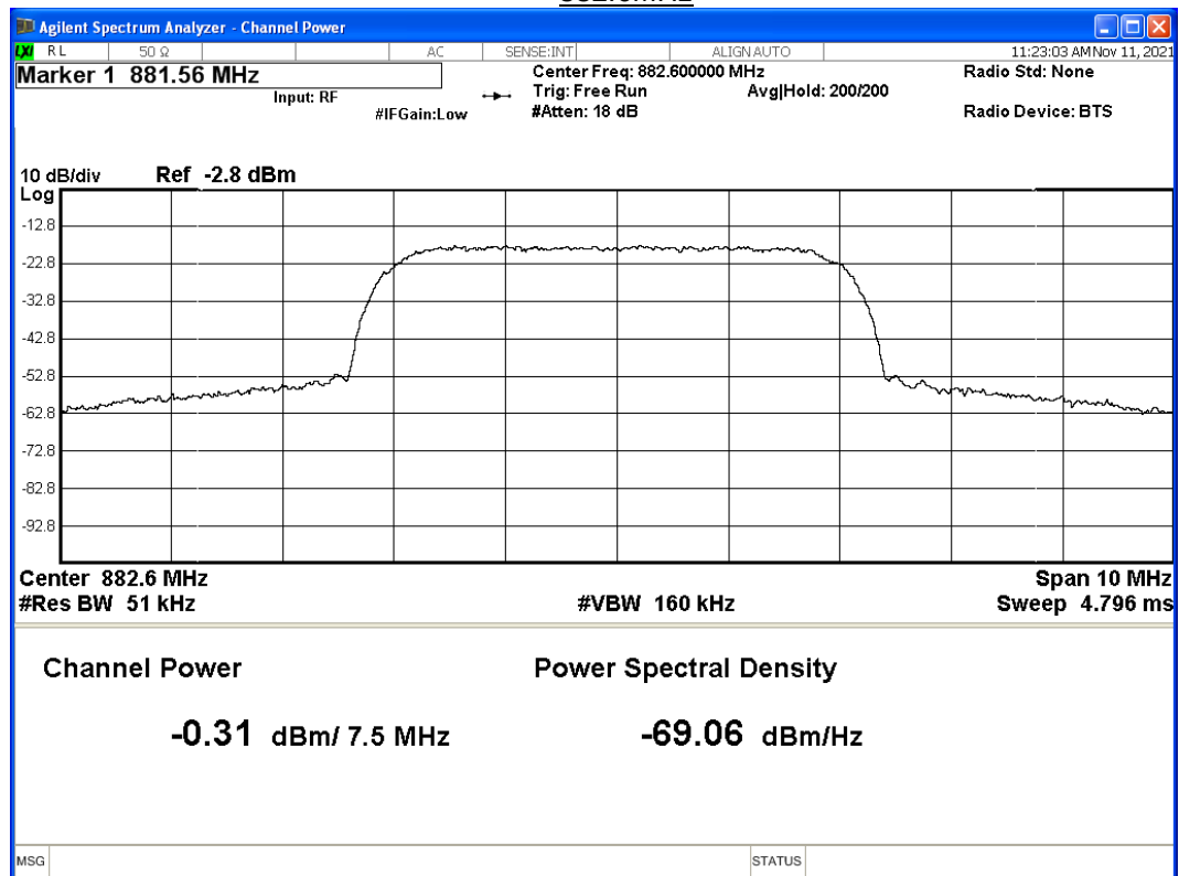
Graph 3: Output Power – Port 2B – Middle Channel
