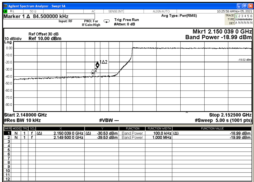
Modulation QPSK - Carrier Bandwidth 5.0 MHz – Top – Channel Position: 2152.5 MHz (Band Power 100kHz & 1MHz)
