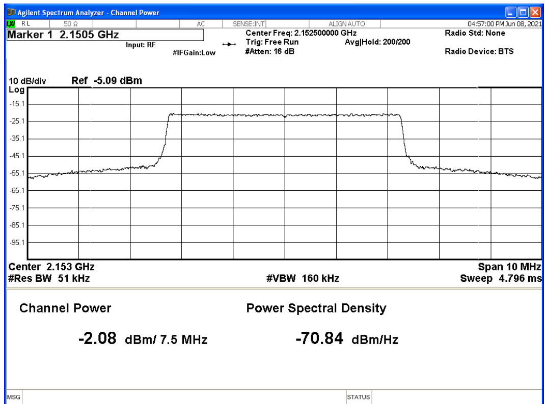
Graph 3: Output Power – Port 1B – Channel: 2152.5 MHz
