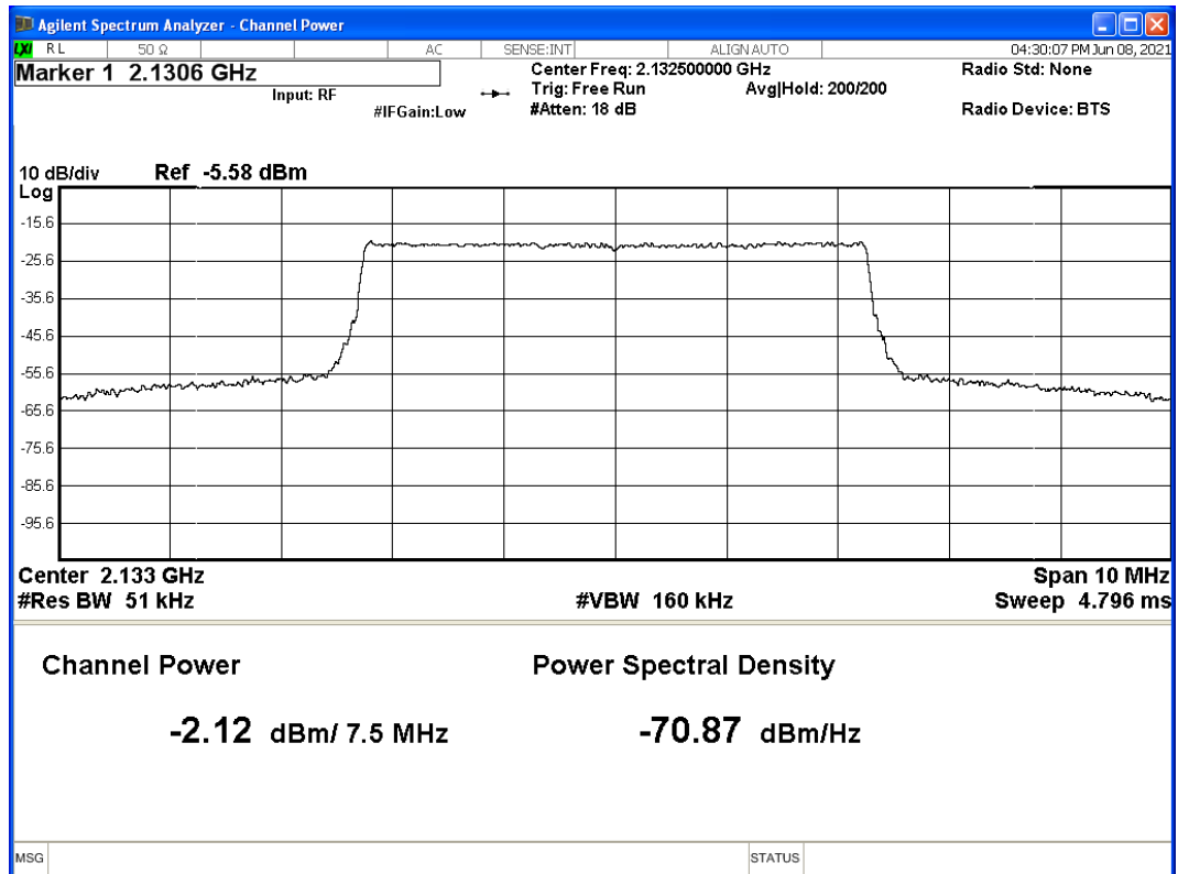
Graph 2: Output Power – Port 2A – Channel: 2132.5 MHz
