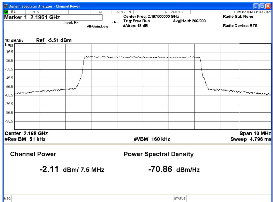
Graph 5: Output Power – Port 2B – Channel: 2197.5 MHz
