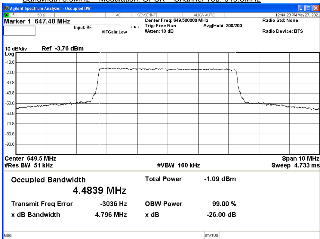
Bandwidth 5.0MHz – Modulation: QPSK – Channel Top: 649.5MHz
