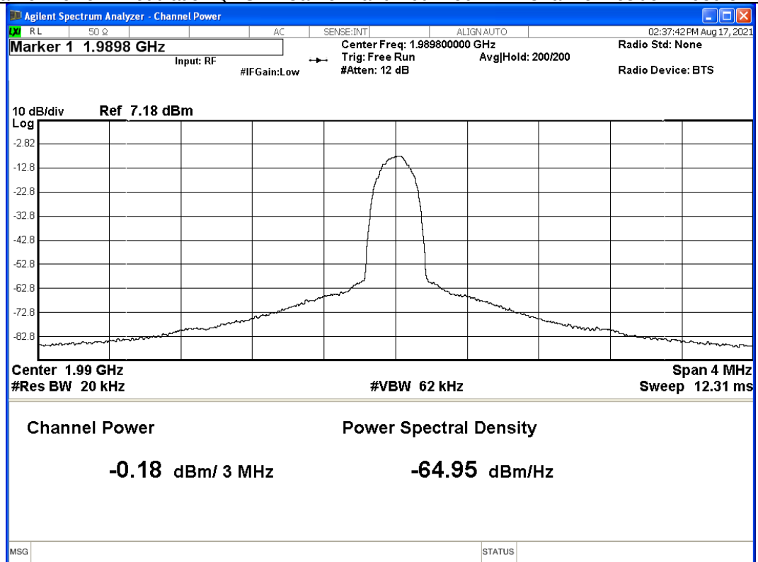
Graph 2: Output Power – Port 2B – Top Channel
