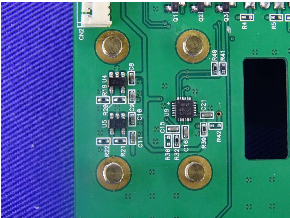
(32) EUT Photo
