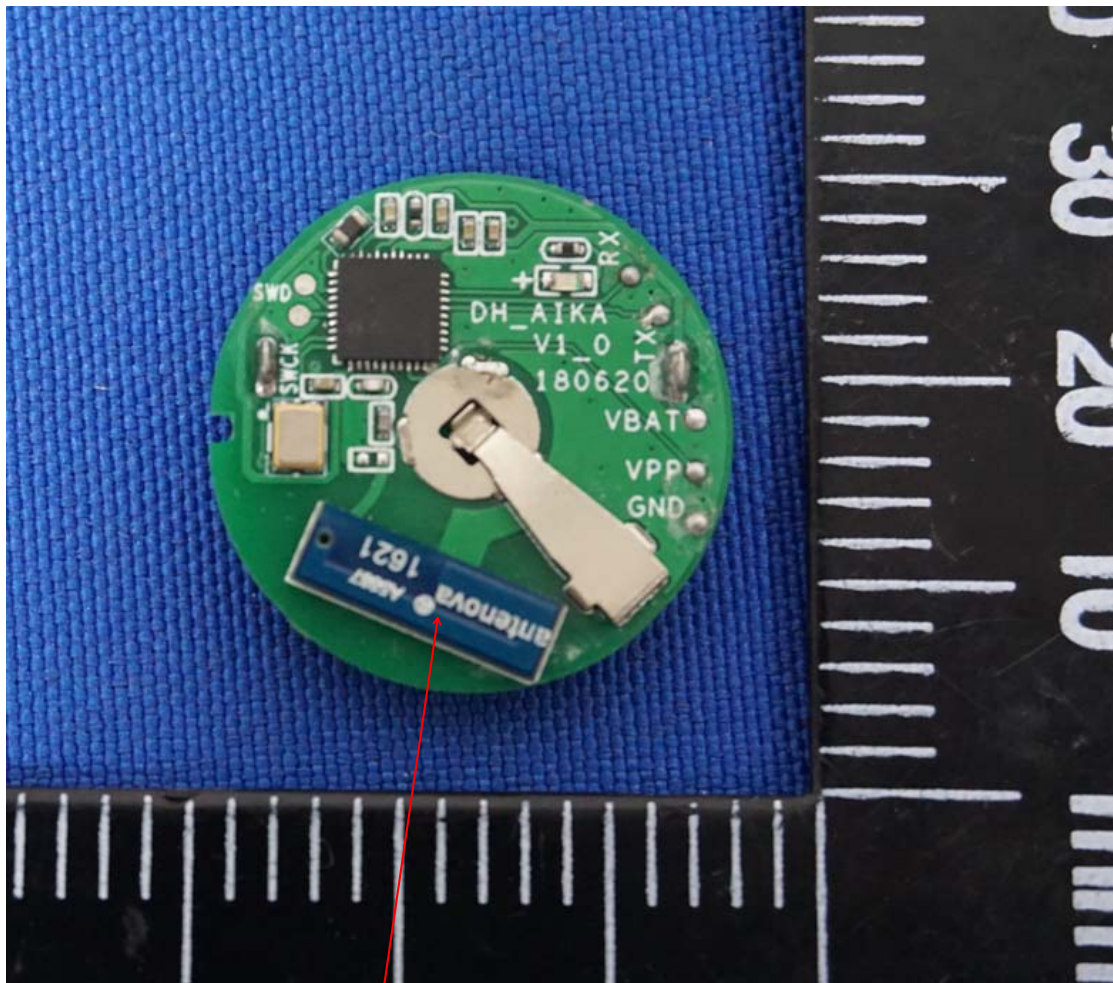
Chip antenna
