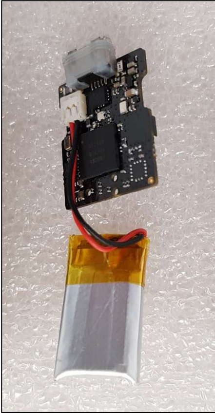
Figure 2. KickAI component side.
