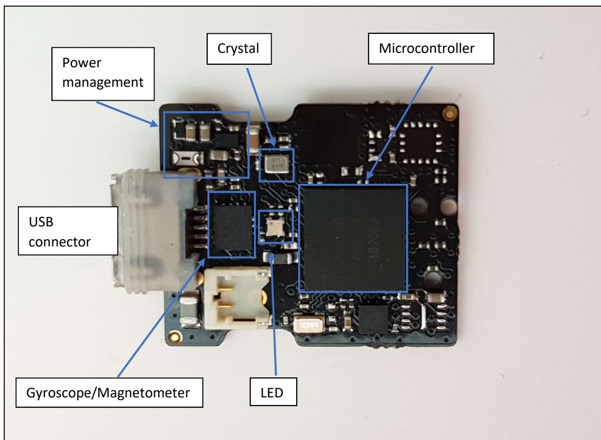
Figure 4. Main parts.
