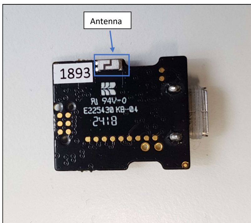
Figure 5. KickAI Antenna.
