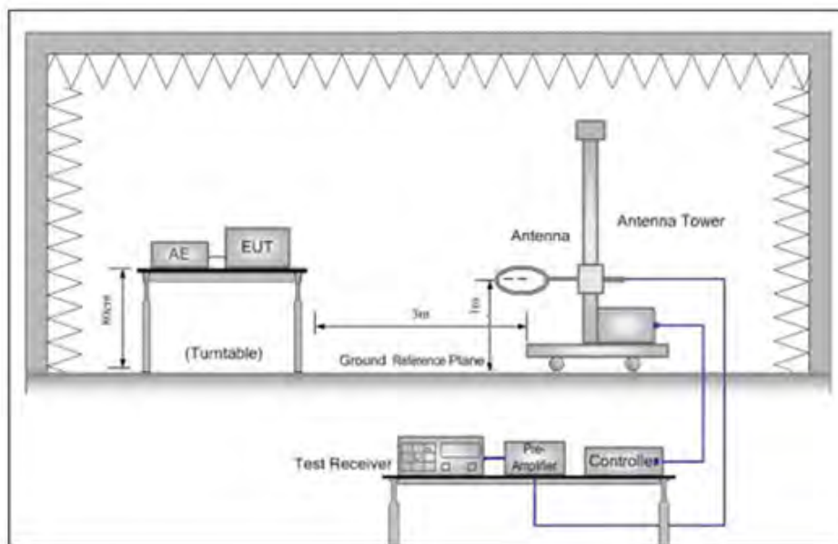
Figure 1. Below 30MHz
