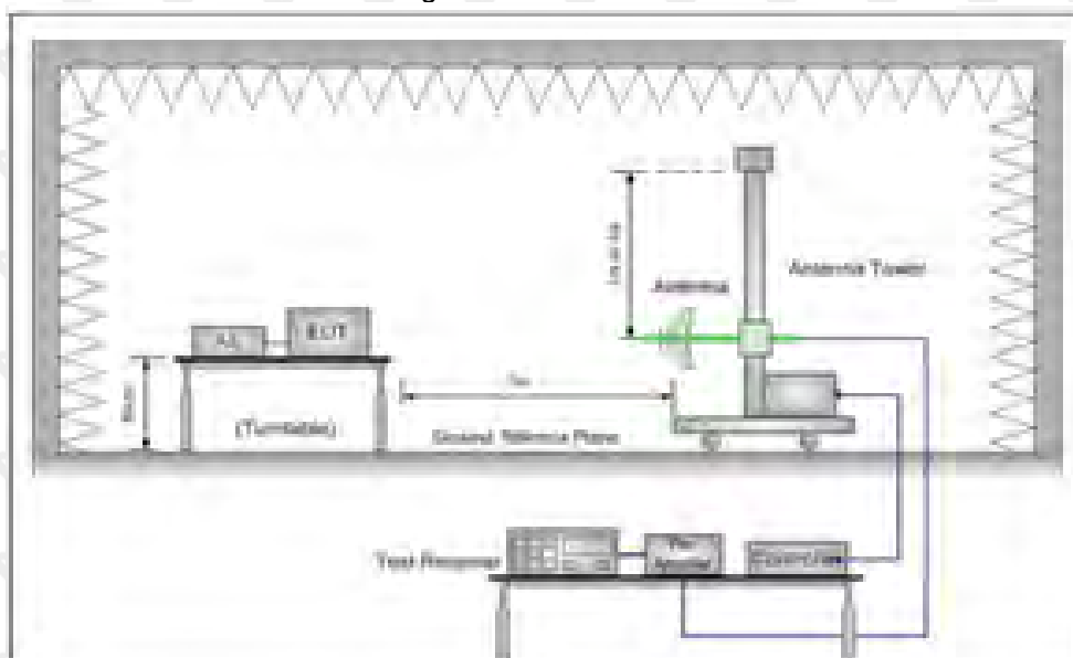
Figure 2. 30MHz to 1GHz
