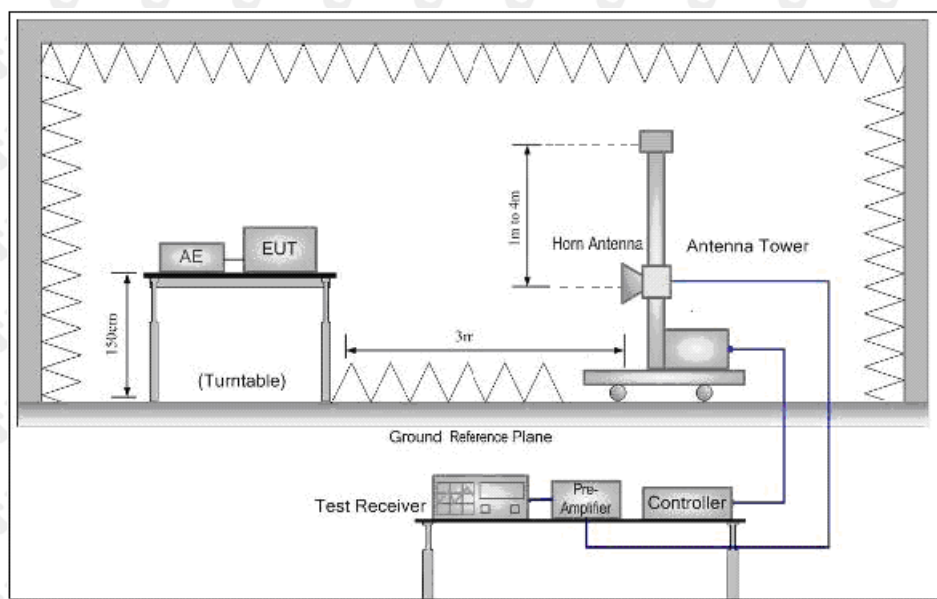
Figure 3. Above 1GHz
