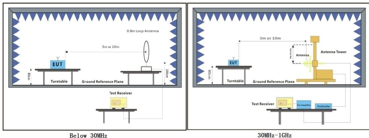
Below 30MHz
