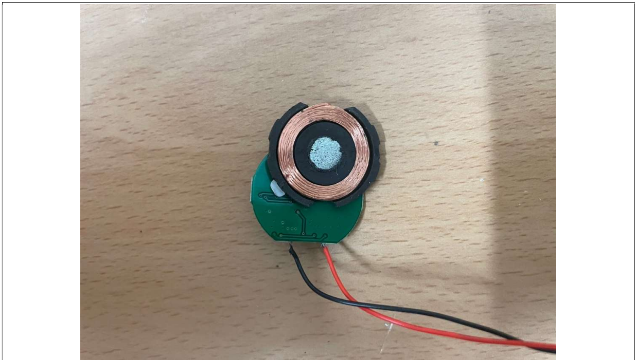
Sub Board1_Rear (Ant.: Smart Watch Charging Area)
