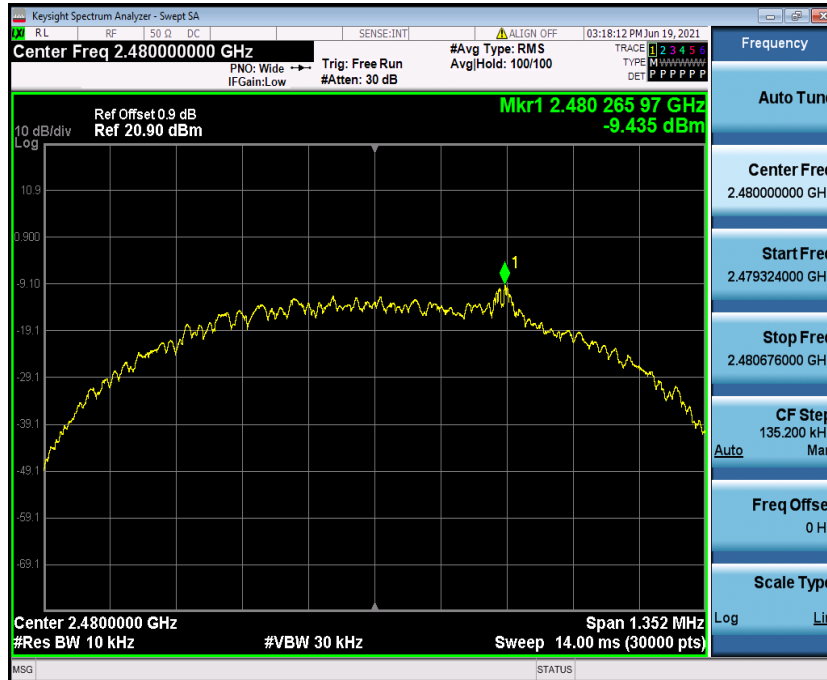
BLE_1M_Ant1_2480
