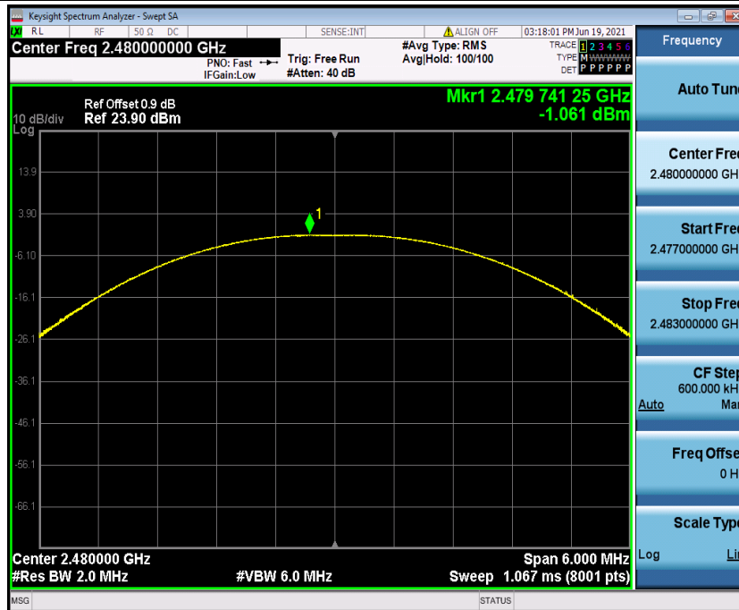
BLE_1M_Ant1_2480
