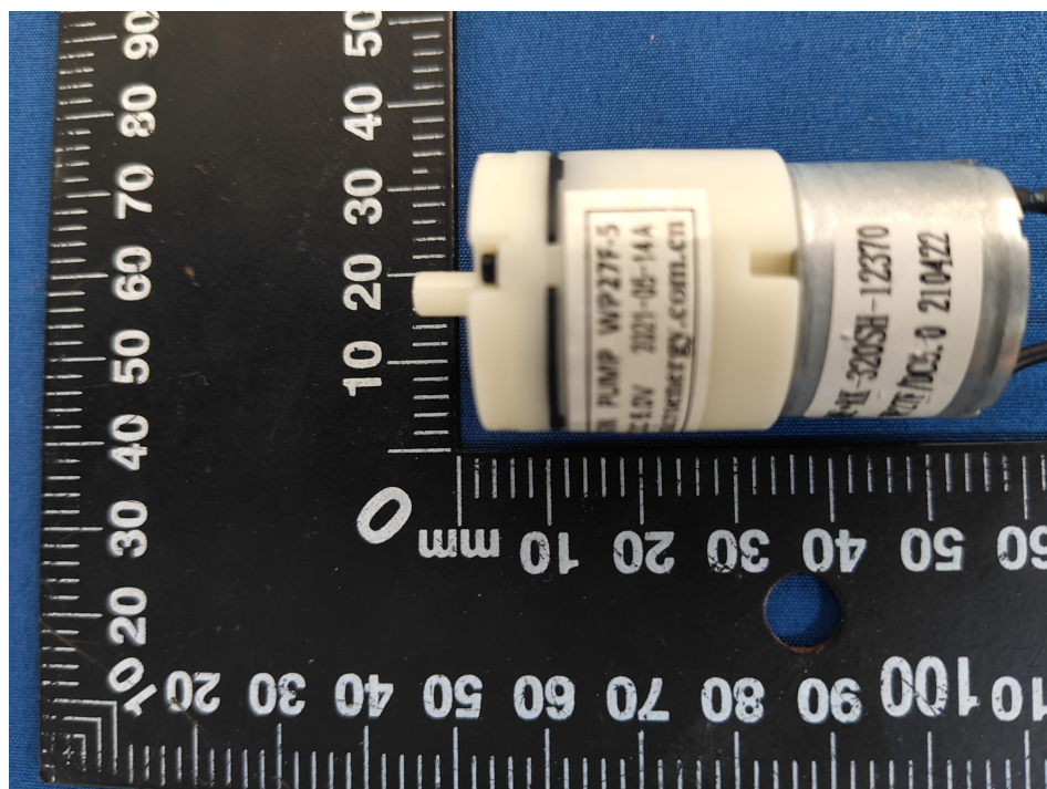
Fig.8 Motor:WP27F-5
