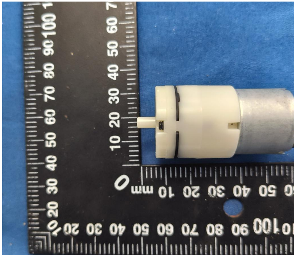
Fig.7 Motor:CAP27A02-310-5V
