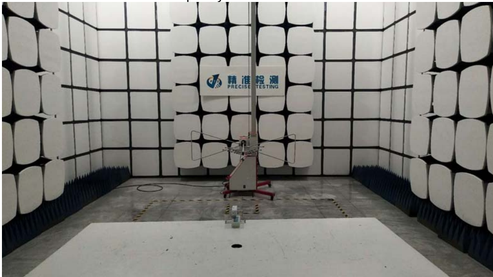
Radiated Spurious Emissions Test Frequency From 30MHz-1000MHz
