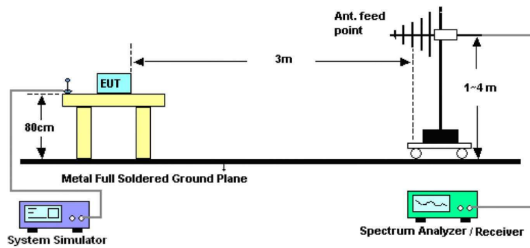
Figure 3. Above 1 GHz
