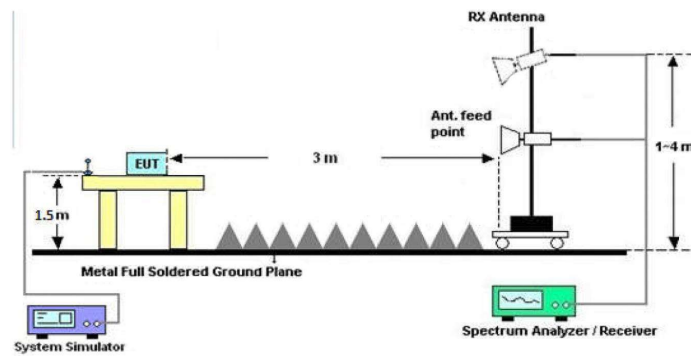
Figure 3. Above 1 GHz
