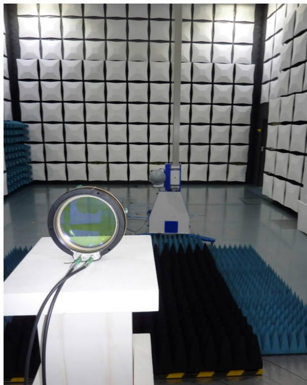
212050_10: Test setup 1 GHz to 6 GHz EUT in X position
