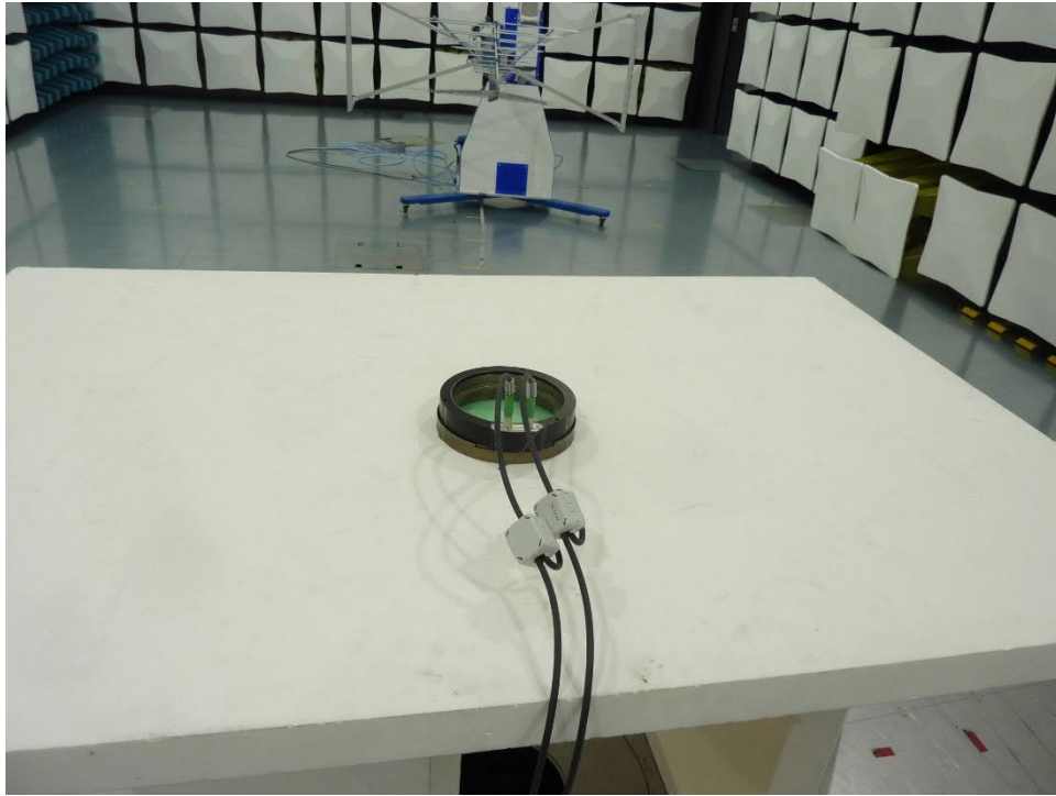
212050_05: Test setup 30 MHz to 1000 MHz EUT in Z Position
