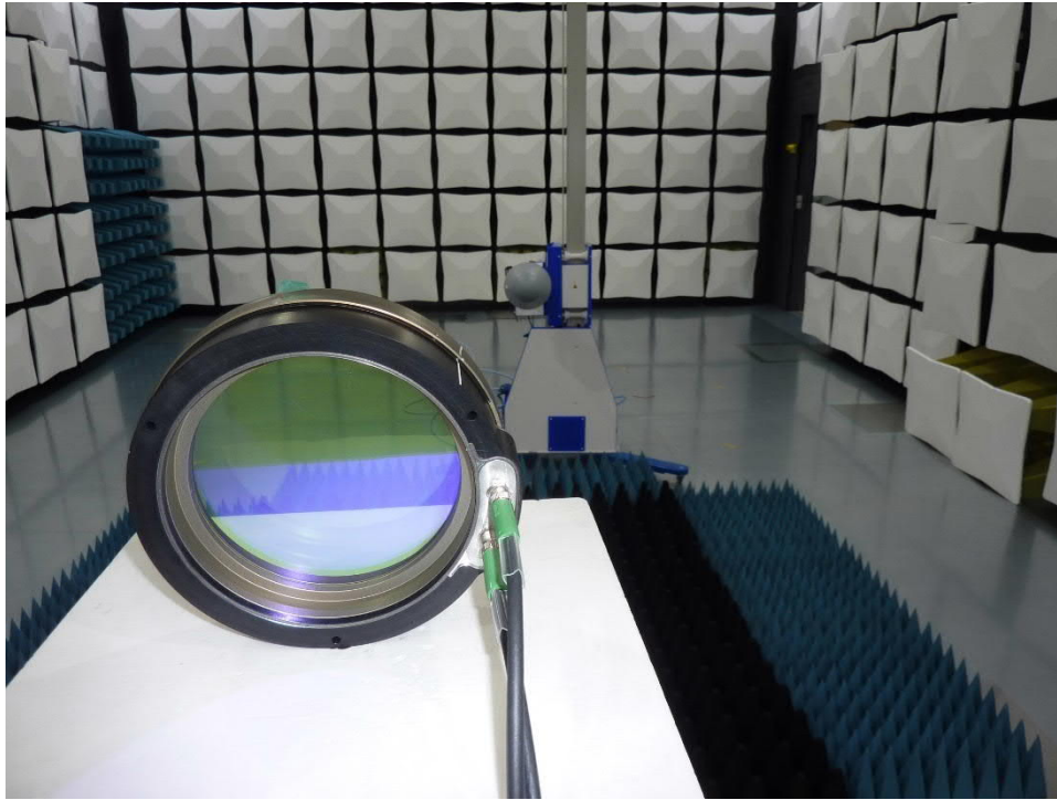
212050_11: Test setup 1 GHz to 6 GHz EUT in Y position
