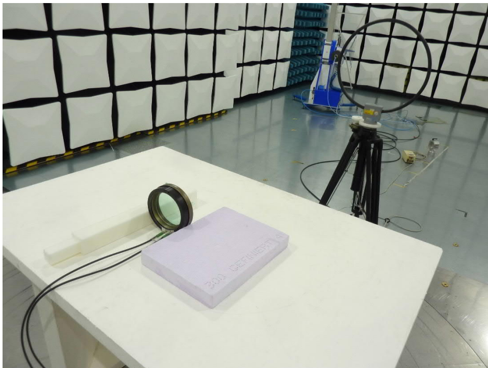
212050_04: Test setup 500 kHz to 30 MHz EUT in X Position
