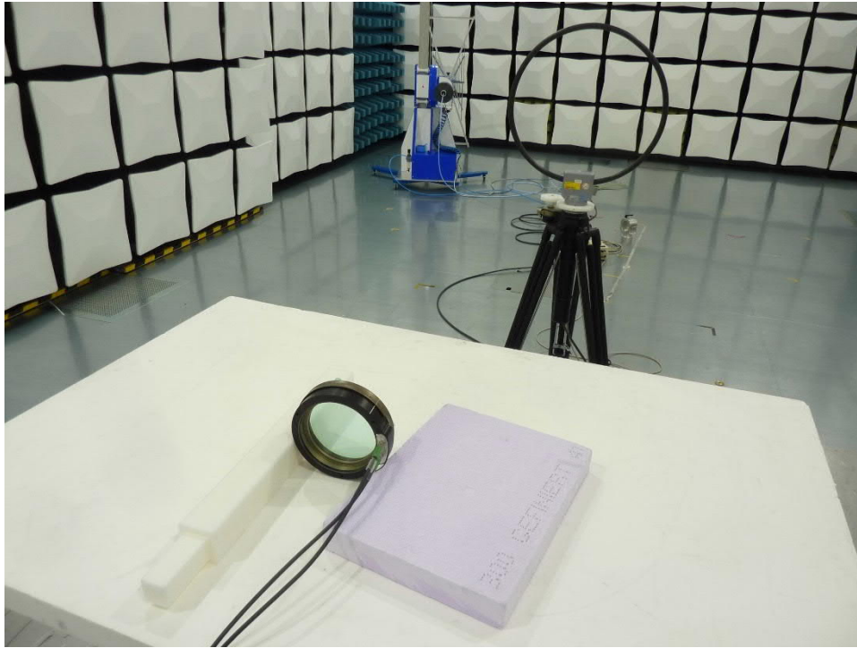
212050_03 Test setup 500 kHz to 30 MHz EUT in Y Position
