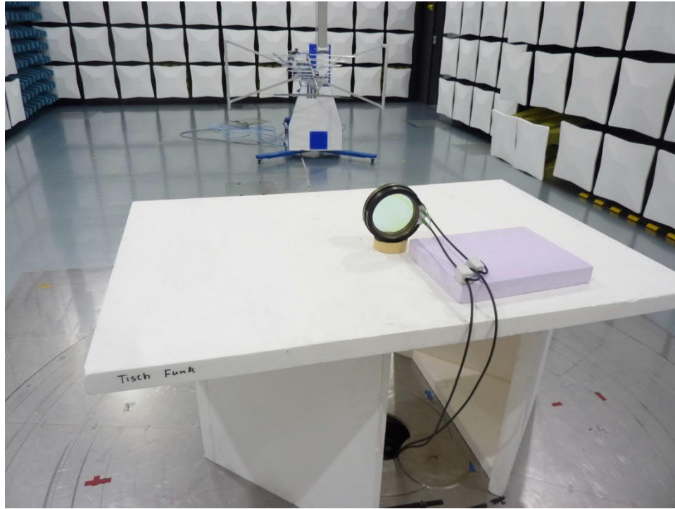
212050_07: Test setup 30 MHz to 1000 MHz EUT in Y Position
