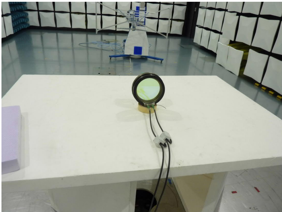
212050_06: Test setup 30 MHz to 1000 MHz EUT in X Position
