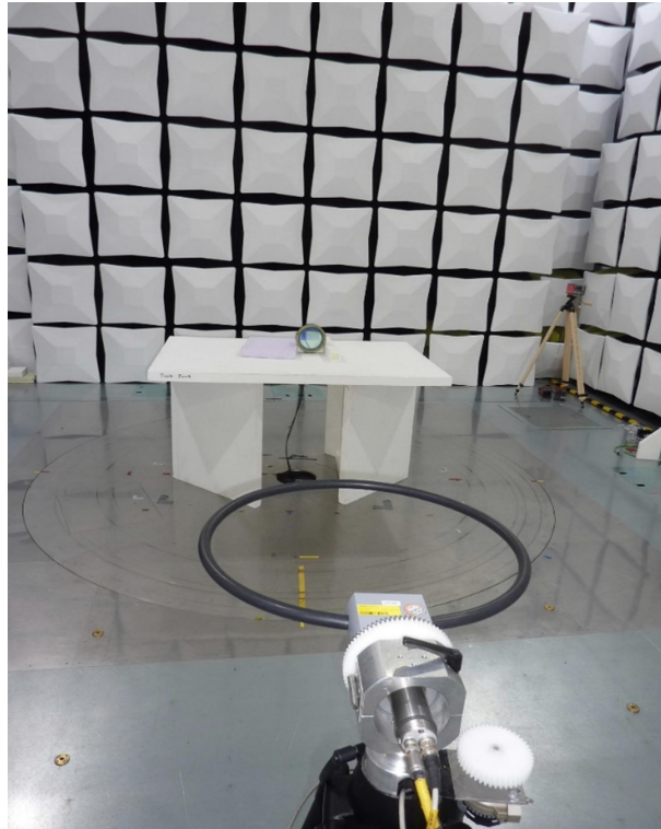
212050_01:Test setup 500 kHz to 30 MHz
