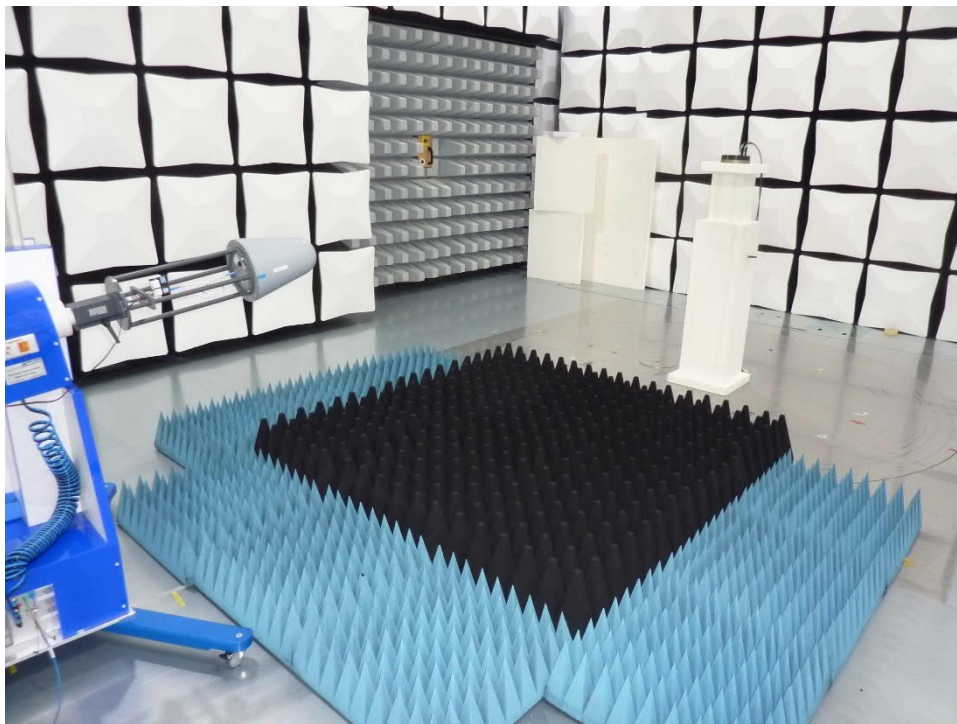
212050_12: Test setup 1 GHz to 6 GHz
