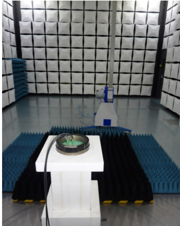
212050_09: Test setup 1 GHz to 6 GHz EUT in Z position
