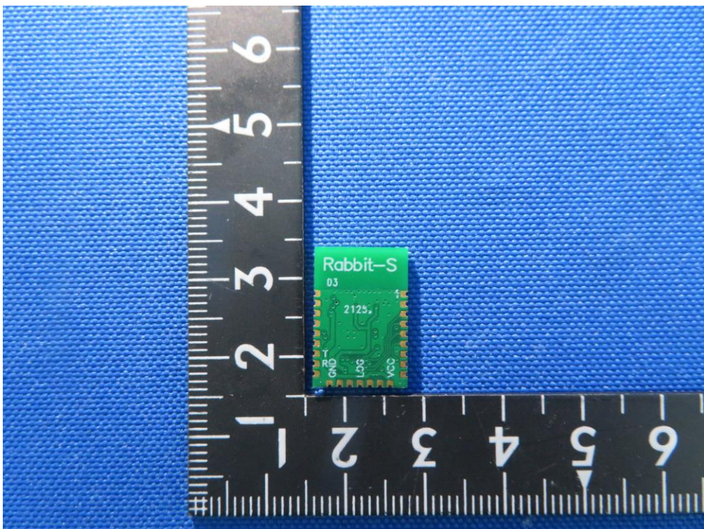
(2) EUT Photo (Rabbit-S)
