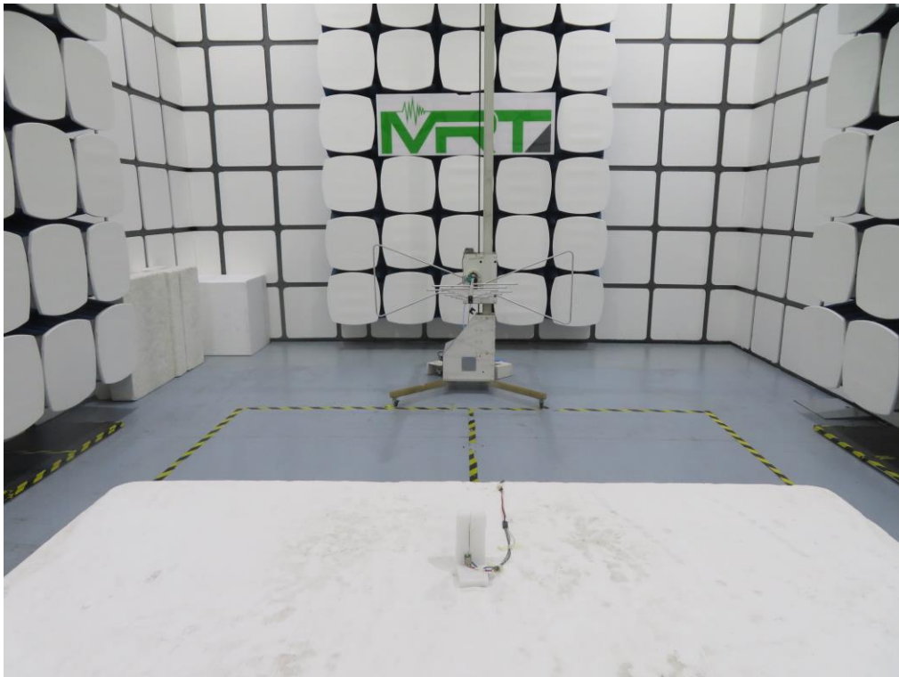
Description: Radiated Spurious Emission Test Setup for below 1GHz (Rabbit-C)
