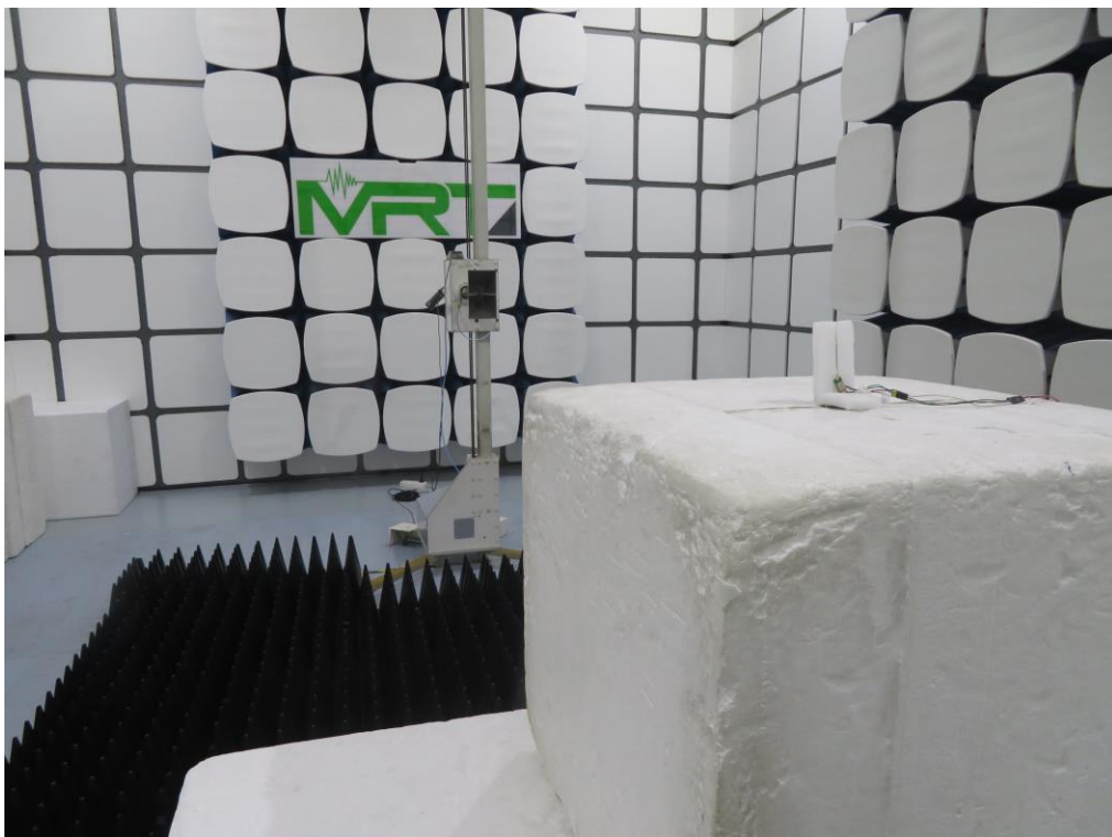
Description: Radiated Spurious Emission Test Setup for above 1GHz (Rabbit-C)
