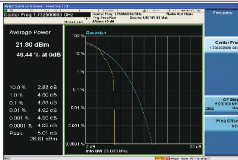
Band4-1.4MHz-16QAM-20175-1RB#0
