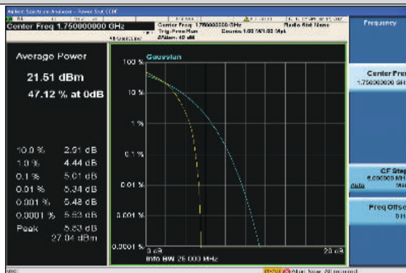
Band4-10MHz-16QAM-20350-50RB#0
