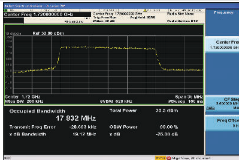
Band4-20MHz-16QAM-20050-100RB#0-17.832
