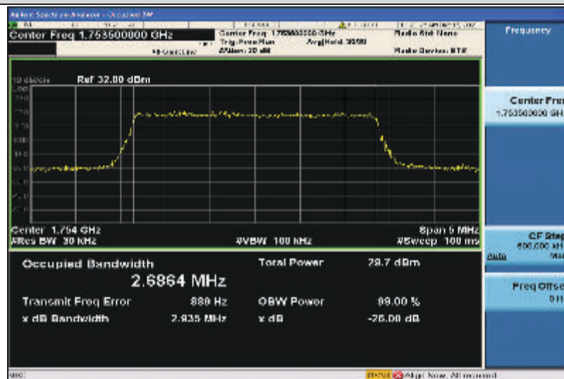
Band4-3MHz-16QAM-20385-15RB#0-2.6864
