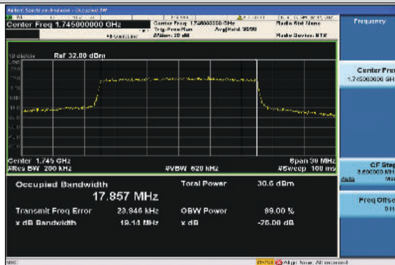
Band4-20MHz-16QAM-20300-100RB#0-17.857
