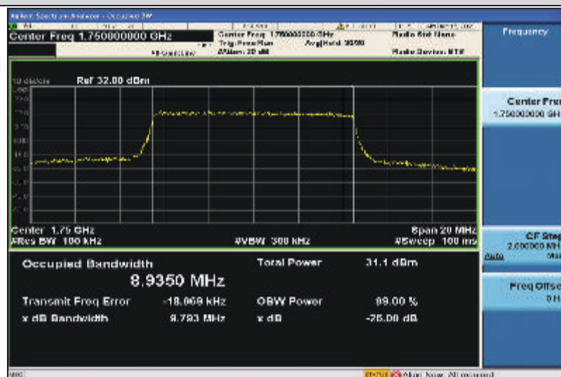
Band4-10MHz-QPSK-20350-50RB#0-8.9350
