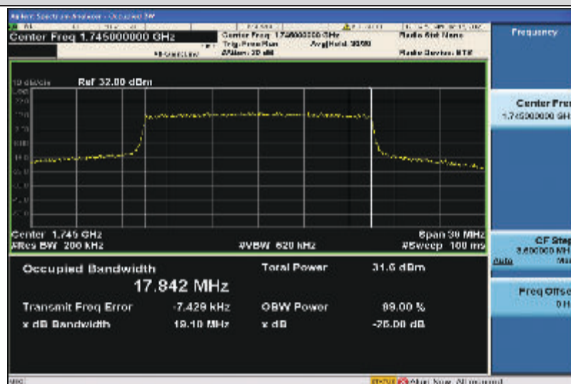
Band4-20MHz-QPSK-20300-100RB#0-17.842
