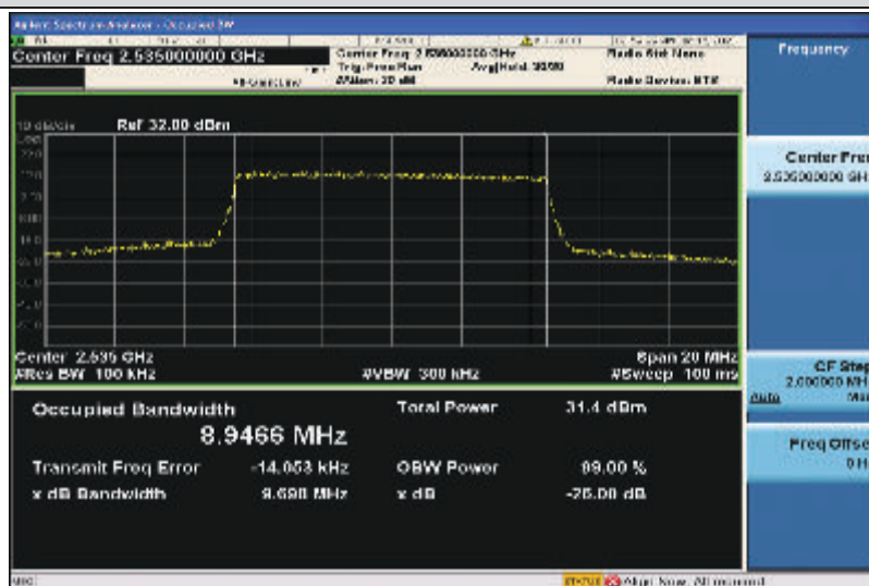
Band7-10MHz-16QAM-21100-50RB#0-8.9466
