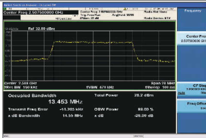
Band7-15MHz-QPSK-20825-75RB#0-9.0021
