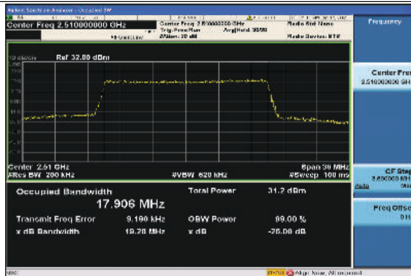
Band7-20MHz-QPSK-20850-100RB#0-17.906
