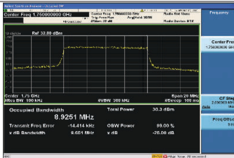
Band4-10MHz-16QAM-20350-50RB#0-8.9251
