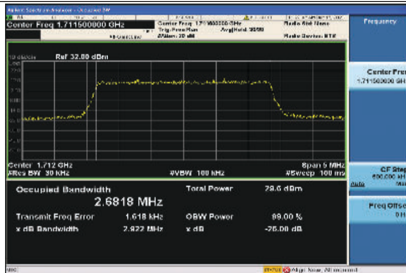
Band4-3MHz-16QAM-19965-15RB#0-2.6818
