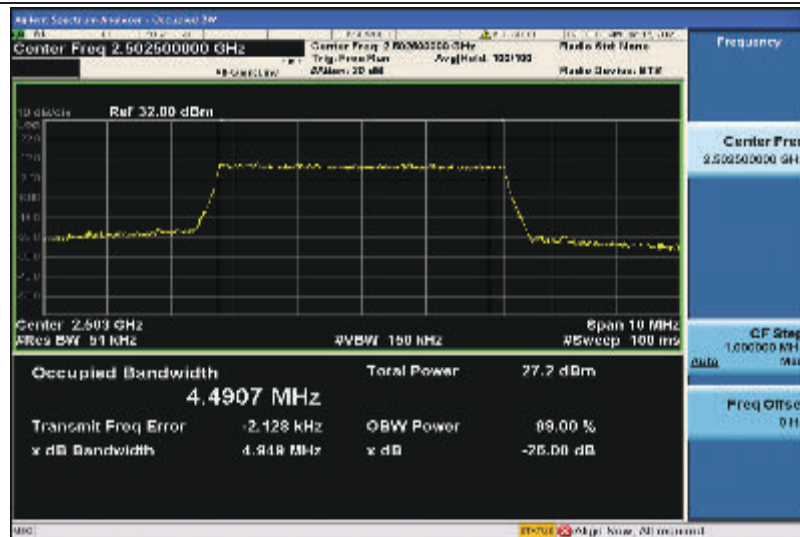
Band7-5MHz-QPSK-20775-25RB#0-4.4907
