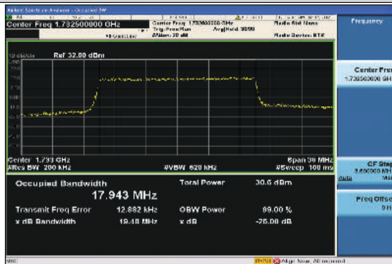
Band4-20MHz-16QAM-20175-100RB#0-17.943
