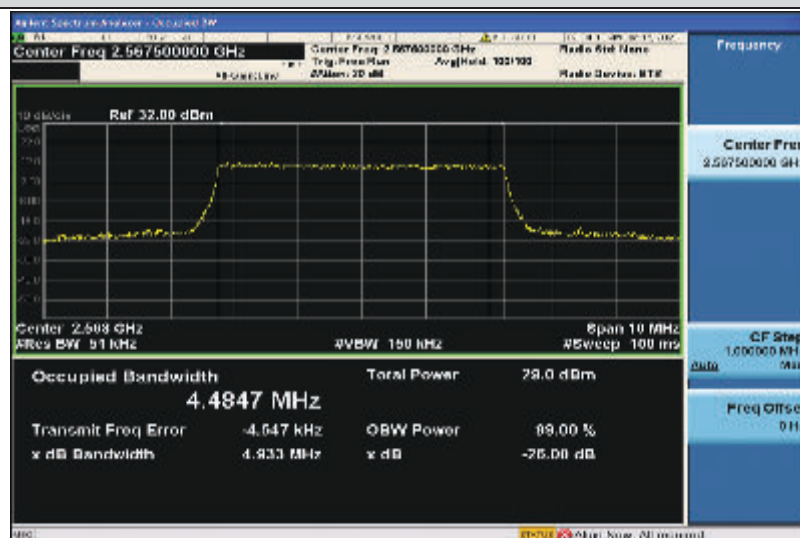
Band7-5MHz-QPSK-21425-25RB#0-4.4847
