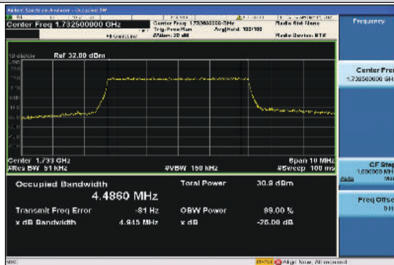
Band4-5MHz-QPSK-17325-25RB#0-4.4860
