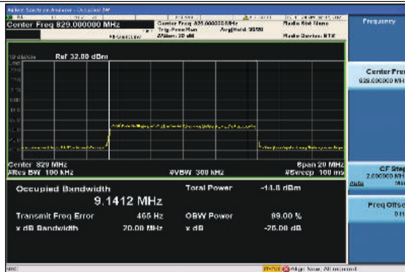
Band5-10MHz-QPSK-20450-50RB#0-9.1412
