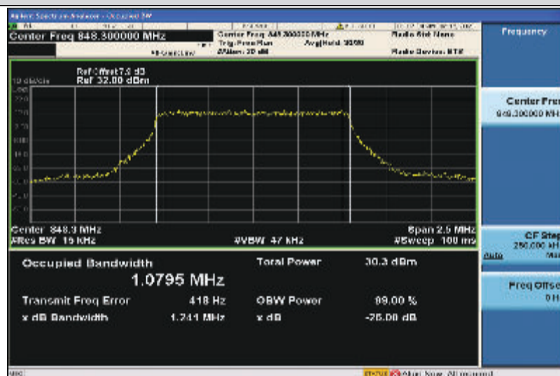
Band5-1.4MHz-QPSK-20643-6RB#0-1.0795
