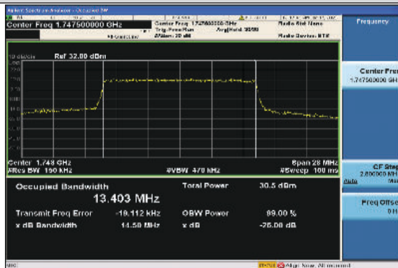
Band4-15MHz-16QAM-20325-75RB#0-13.403
