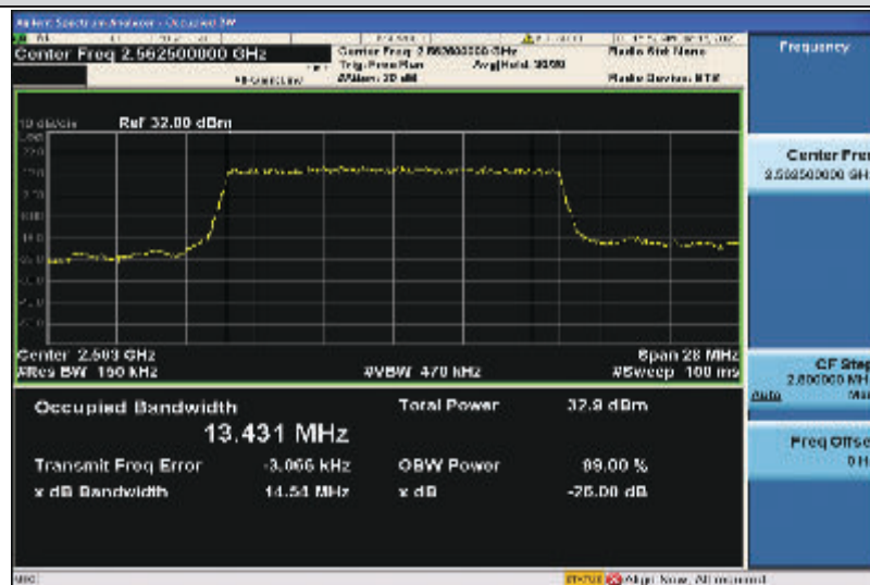
Band7-15MHz-QPSK-21375-75RB#0-13.431
