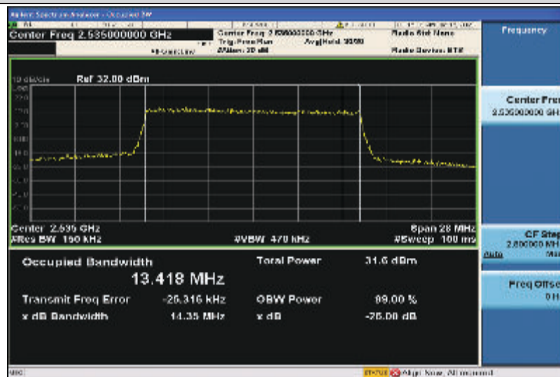
Band7-15MHz-QPSK-21100-75RB#0-13.418
