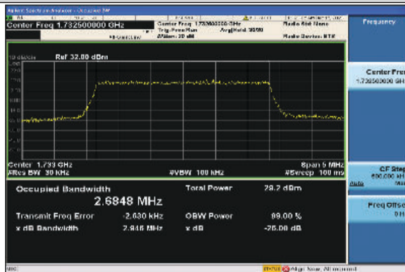
Band4-3MHz-16QAM-20175-15RB#0-2.6848
