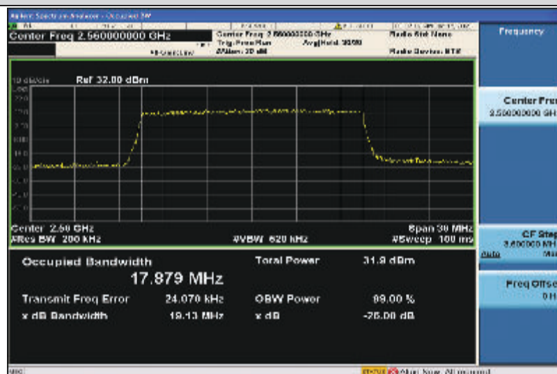
Band7-20MHz-16QAM-21350-100RB#0-17.879
