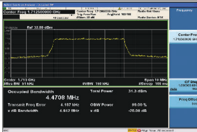
Band4-5MHz-QPSK-19975-25RB#0-4.4708
