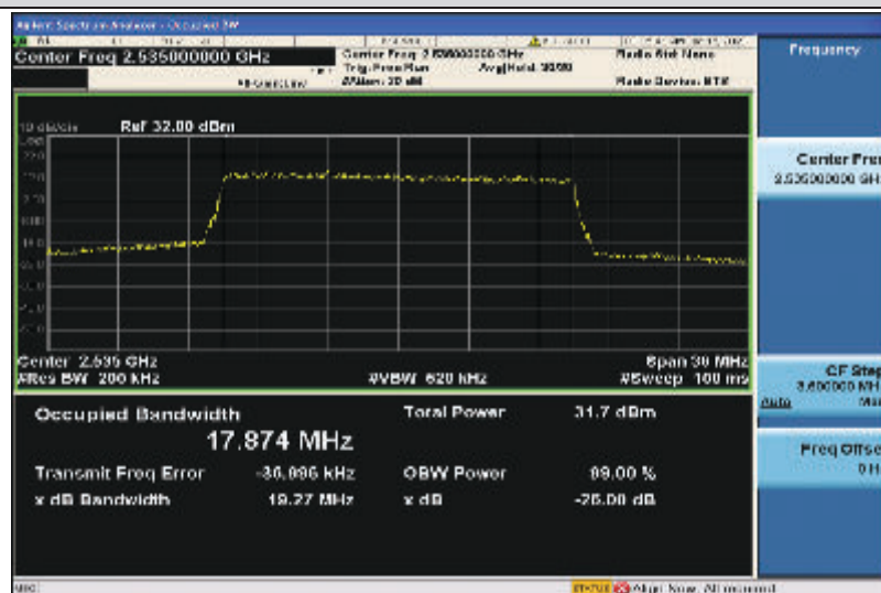
Band7-20MHz-16QAM-21100-100RB#0-17.874
