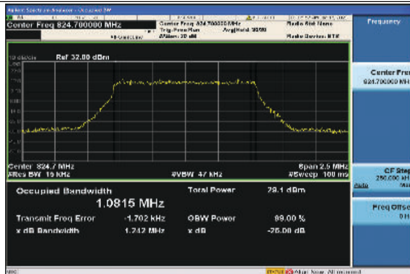
Band5-1.4MHz-16QAM-20407-6RB#0-1.0815
