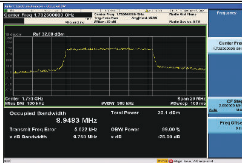
Band4-10MHz-16QAM-20175-50RB#0-8.9483
