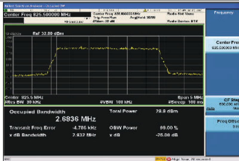
Band5-3MHz-QPSK-20415-15RB#0-2.6836
