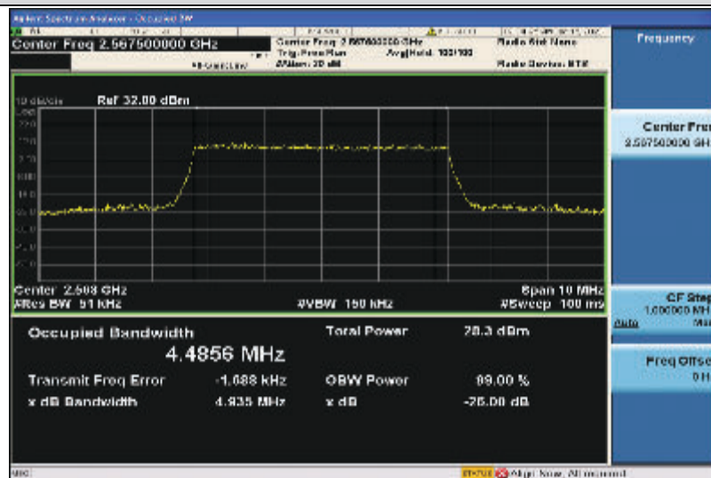
Band7-5MHz-16QAM-21425-25RB#0-4.4856
