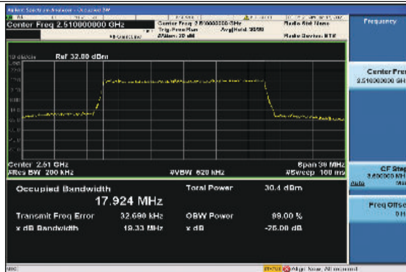
Band7-20MHz-16QAM-20850-100RB#0-17.924
