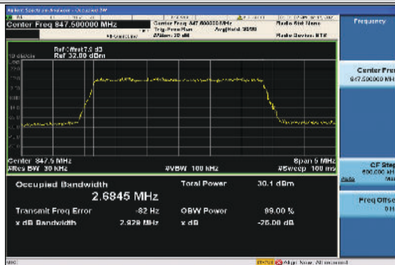
Band5-3MHz-16QAM-20635-15RB#0-2.6845
