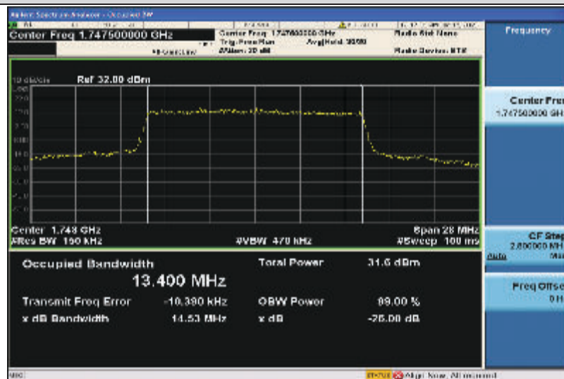
Band4-15MHz-QPSK-20325-75RB#0-13.400
