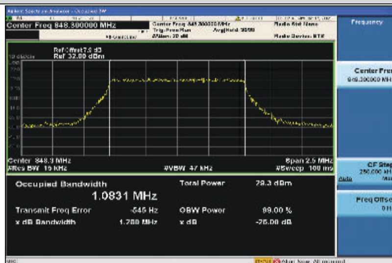
Band5-1.4MHz-16QAM-20643-6RB#0-1.0831
