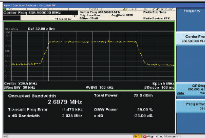
Band5-3MHz-16QAM-20525-15RB#0-2.6879
