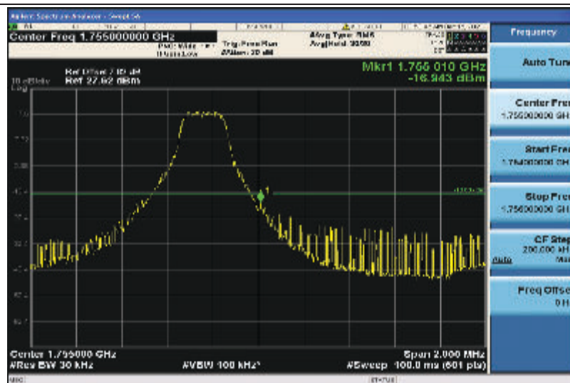
Band4-3MHz-QPSK-20385-1RB#14
