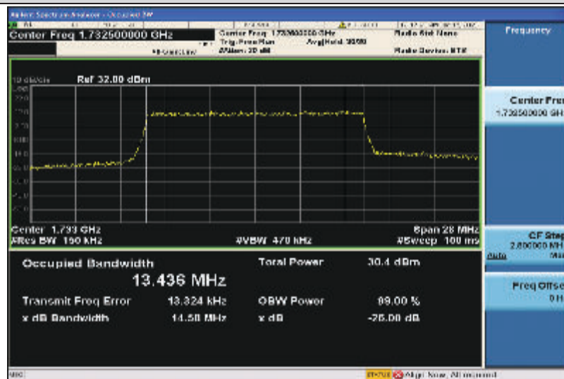
Band4-15MHz-16QAM-20175-75RB#0-13.436
