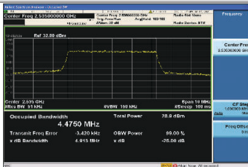
Band7-5MHz-QPSK-21100-25RB#0-4.4750
