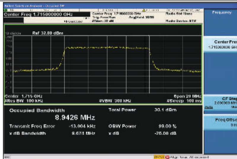
Band4-10MHz-16QAM-20000-50RB#0-8.9426
