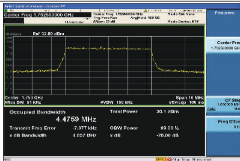
Band4-5MHz-16QAM-20375-25RB#0-4.4759
