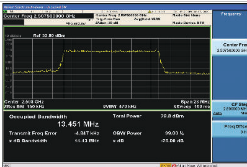
Band7-15MHz-16QAM-20825-75RB#0-13.451
