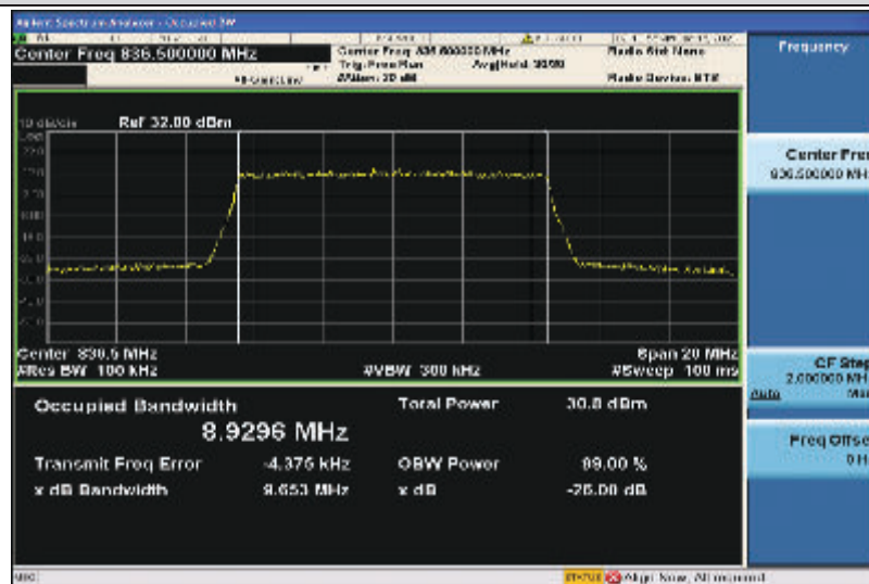
Band5-10MHz-16QAM-20525-50RB#0-8.9296
