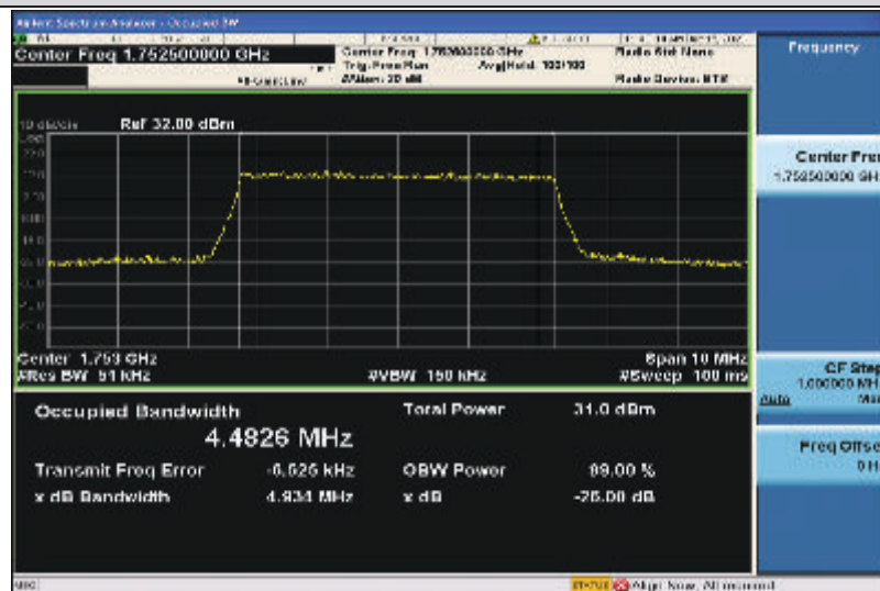
Band4-5MHz-QPSK-20375-25RB#0-4.4826
