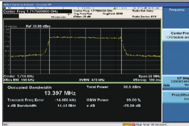
Band4-15MHz-16QAM-20025-75RB#0-13.397
