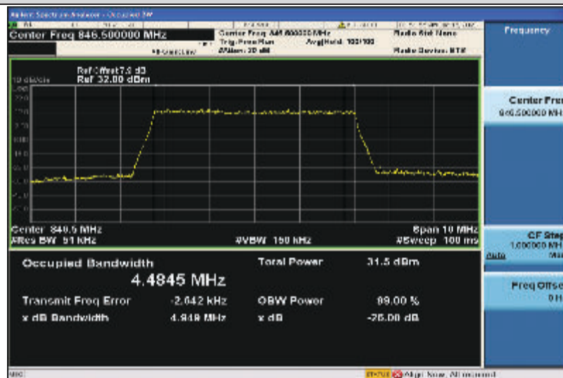
Band5-5MHz-QPSK-20625-25RB#0-4.4845
