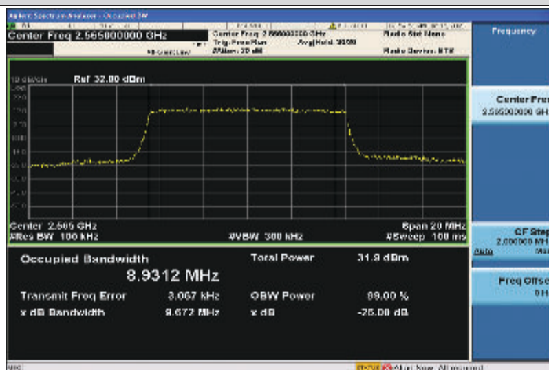
Band7-10MHz-16QAM-21400-50RB#0-8.9312
