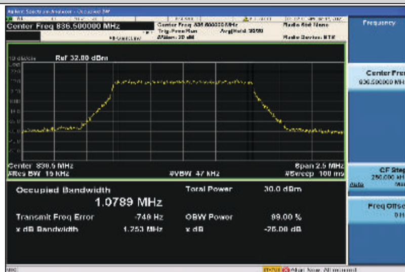
Band5-1.4MHz-QPSK-20525-6RB#0-1.0789
