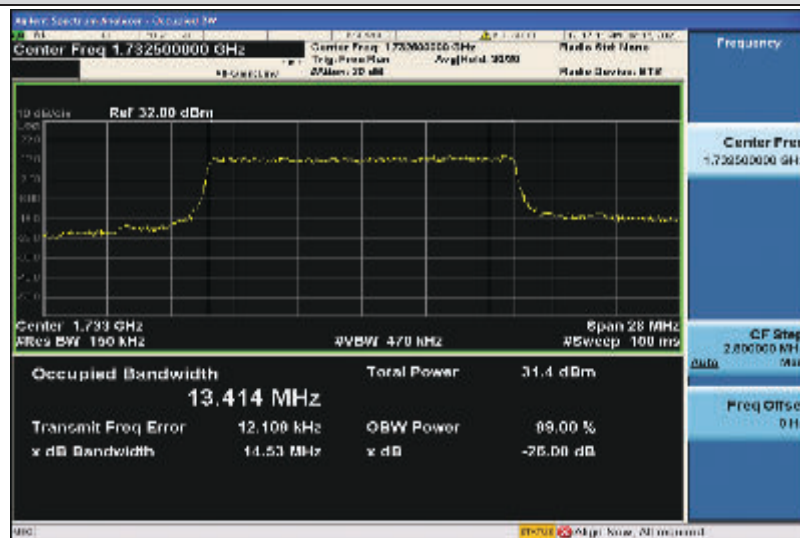
Band4-15MHz-QPSK-20175-75RB#0-13.414
