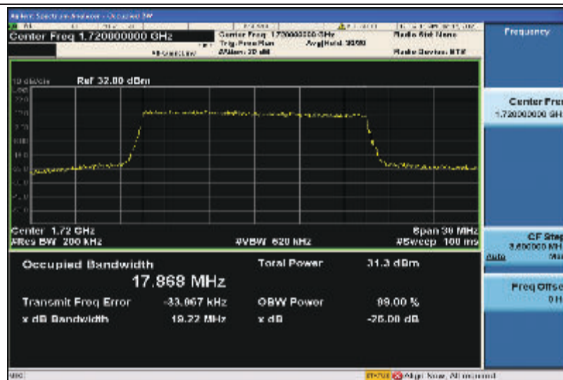
Band4-20MHz-QPSK-20050-100RB#0-17.868
