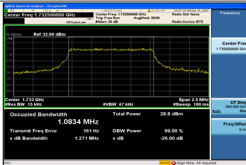
Band4-1.4MHz-16QAM-20175-6RB#0-1.0834
