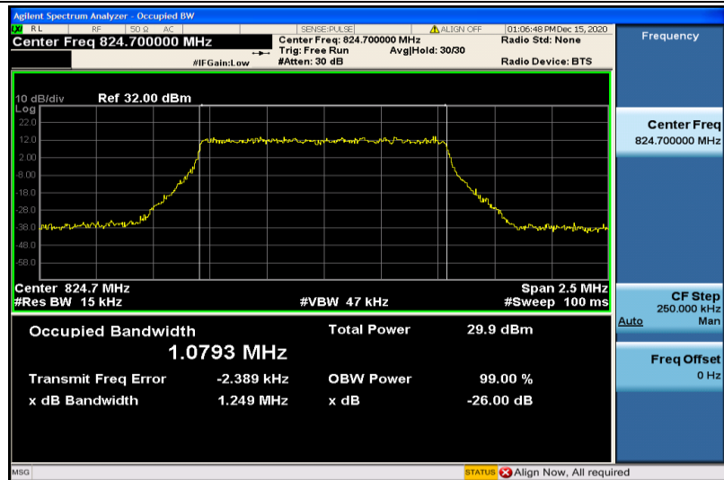
Band5-1.4MHz-QPSK-20407-6RB#0-1.0793
