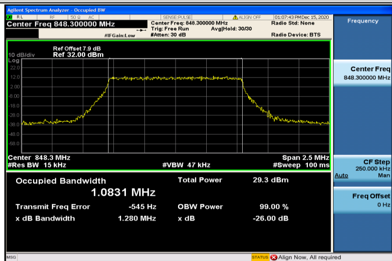
Band5-1.4MHz-16QAM-20643-6RB#0-1.0831
