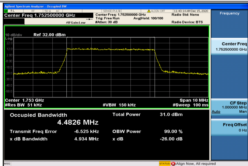
Band4-5MHz-QPSK-20375-25RB#0-4.4826
