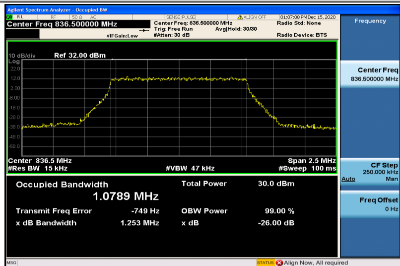
Band5-1.4MHz-QPSK-20525-6RB#0-1.0789
