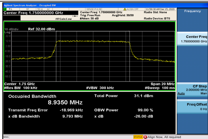
Band4-10MHz-QPSK-20350-50RB#0-8.9350
