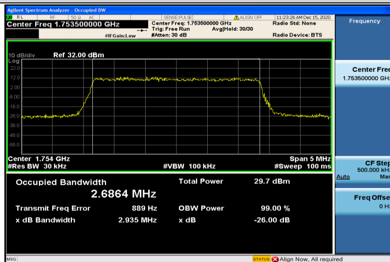
Band4-3MHz-16QAM-20385-15RB#0-2.6864
