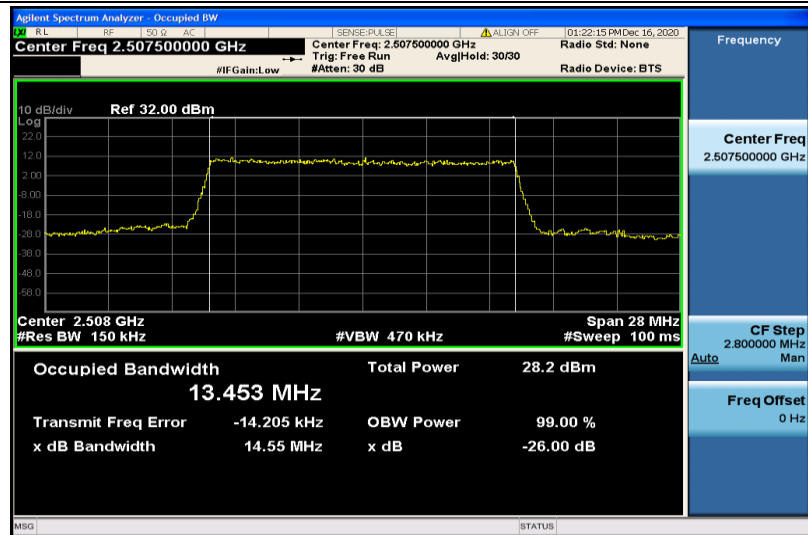
Band7-15MHz-QPSK-20825-75RB#0-9.0021
