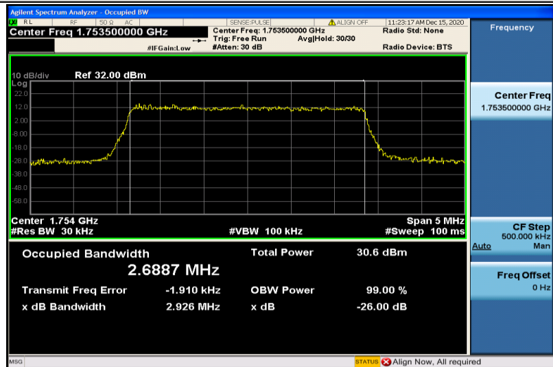
Band4-3MHz-QPSK-20385-15RB#0-2.6887
