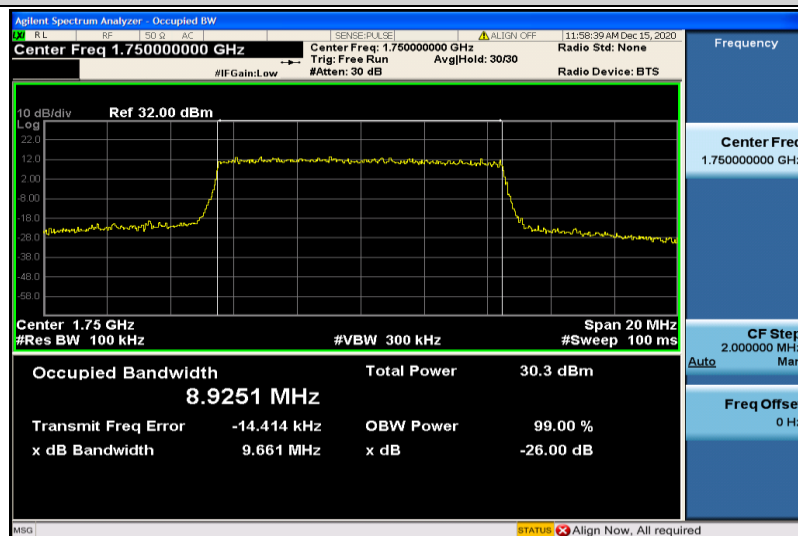
Band4-10MHz-16QAM-20350-50RB#0-8.9251
