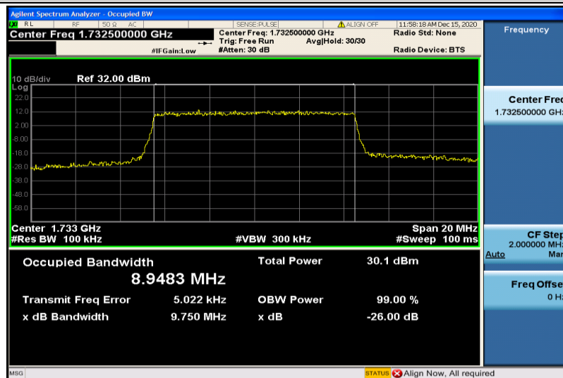
Band4-10MHz-16QAM-20175-50RB#0-8.9483
