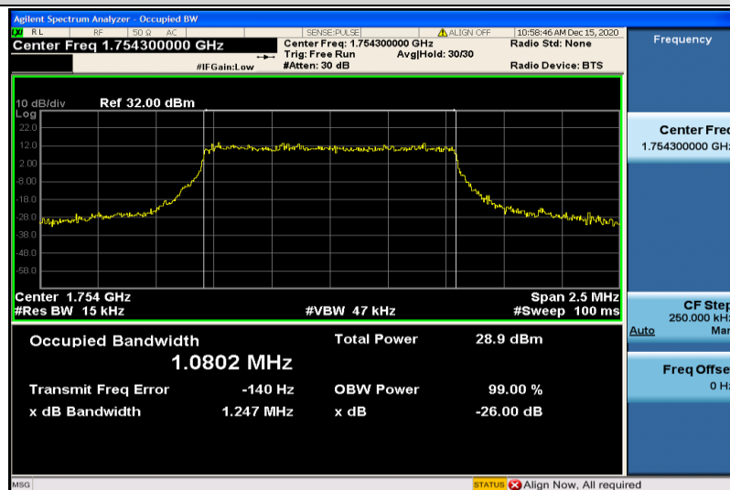
Band4-1.4MHz-16QAM-20393-6RB#0-1.0802
