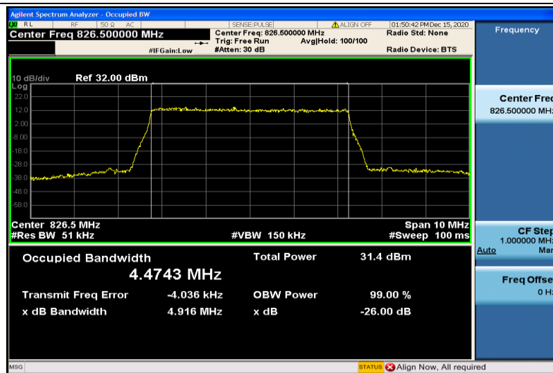
Band5-5MHz-QPSK-20425-25RB#0-4.4743
