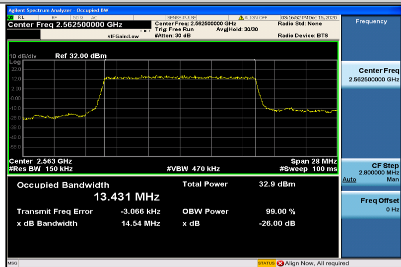
Band7-15MHz-QPSK-21375-75RB#0-13.431
