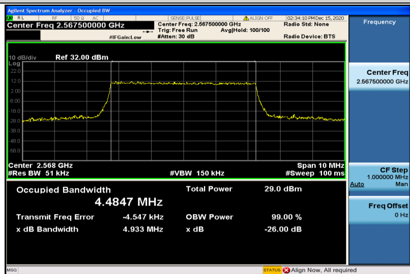
Band7-5MHz-QPSK-21425-25RB#0-4.4847
