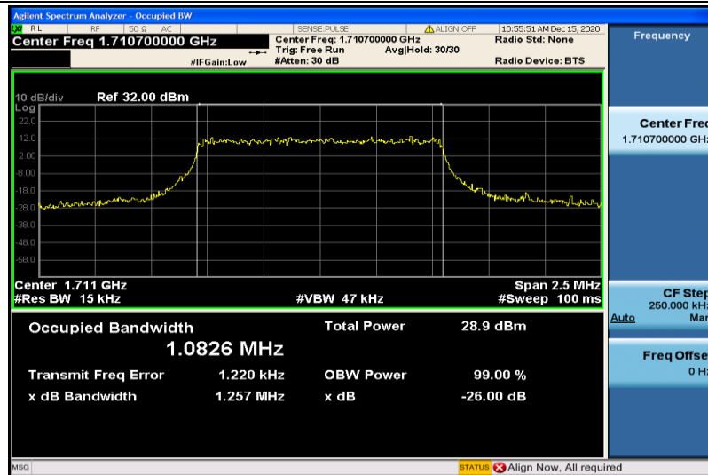
Band4-1.4MHz-16QAM-19957-6RB#0-1.0826
