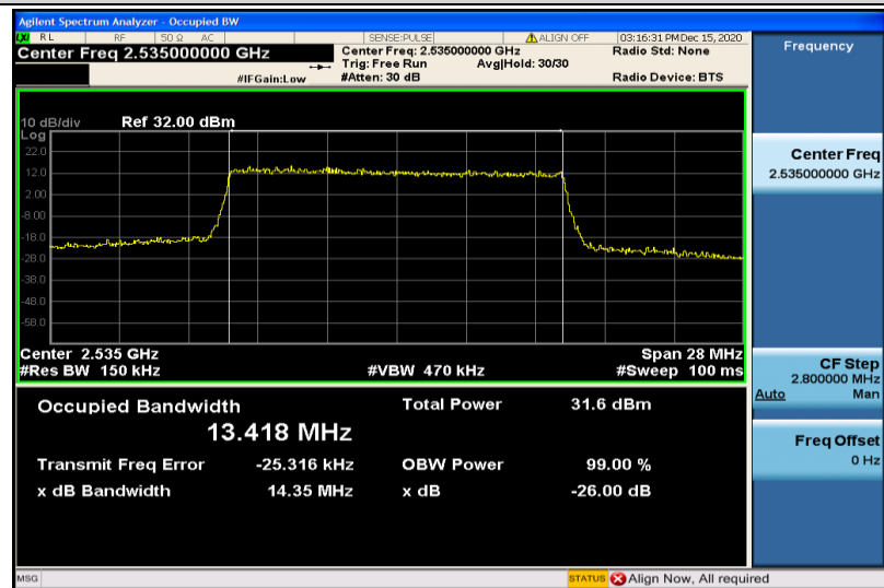
Band7-15MHz-QPSK-21100-75RB#0-13.418
