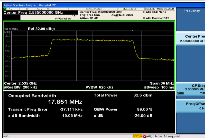
Band7-20MHz-QPSK-21100-100RB#0-17.851
