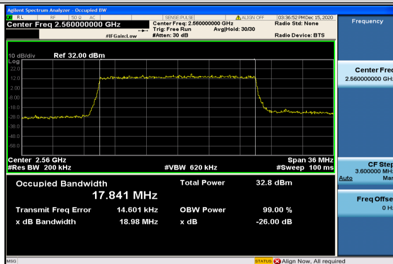
Band7-20MHz-QPSK-21350-100RB#0-17.841
