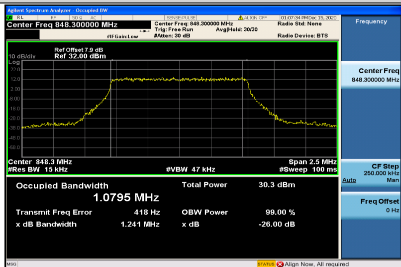
Band5-1.4MHz-QPSK-20643-6RB#0-1.0795
