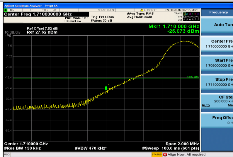
Band4-15MHz-QPSK-20025-1RB#0
