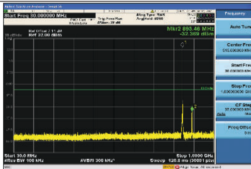
Band5-3MHz-16QAM-20635-1RB#0-30~1000MHz
