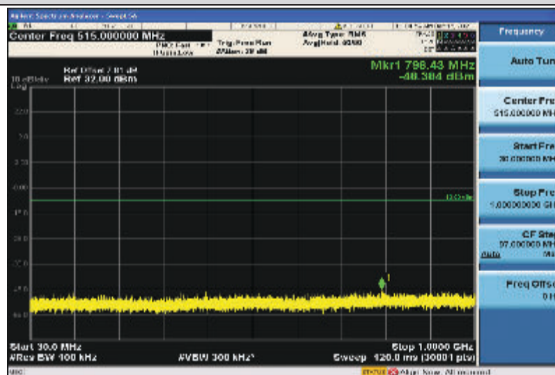
Band4-1.4MHz-16QAM-20393-1RB#0-30~1000MHz
