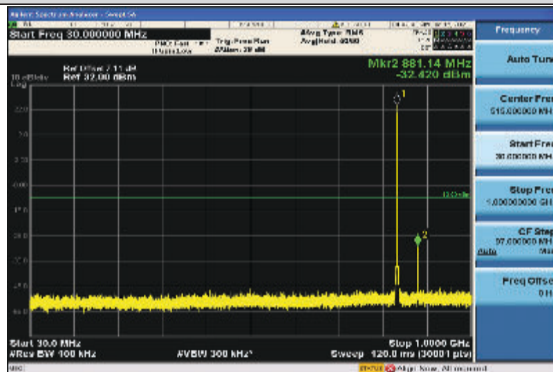
Band5-1.4MHz-QPSK-20525-1RB#0-30~1000MHz
