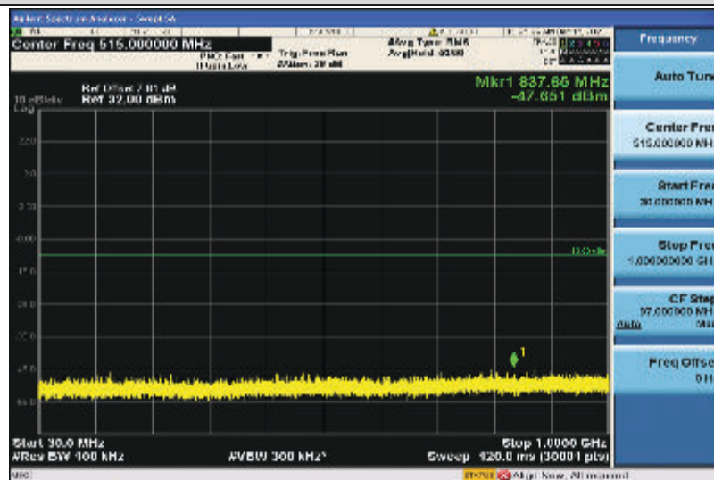
Band4-3MHz-16QAM-20175-1RB#0-30~1000MHz
