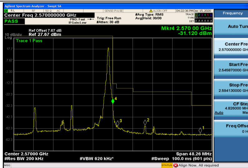
Band7-20MHz-16QAM-21350-1RB#99
