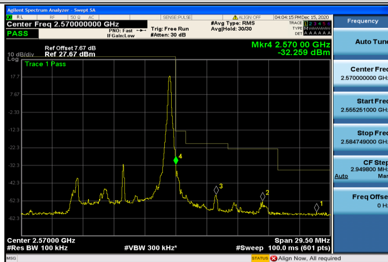
Band7-10MHz-QPSK-21400-1RB#49
