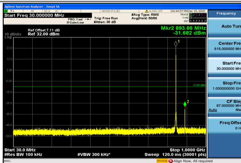
Band5-1.4MHz-16QAM-20643-1RB#0-30~1000MHz
