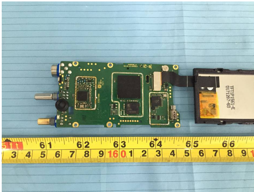
EUT – Main Board 2 Top View 3
